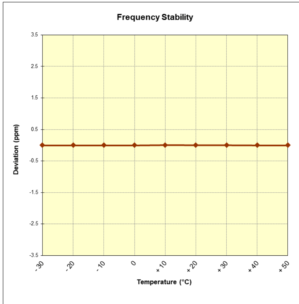
Figure 7-13. Frequency Stability Graph (PCS WCDMA Mode – Ch. 9400)
