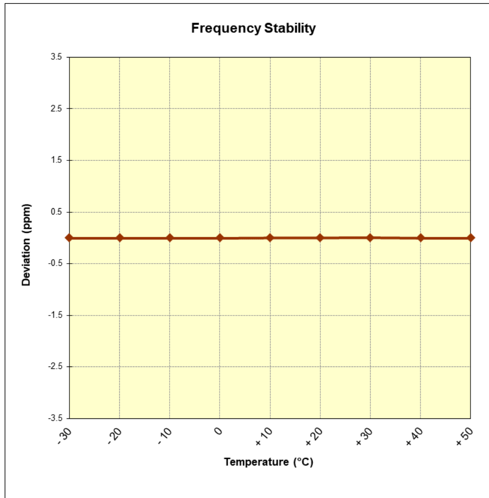
Figure 7-11. Frequency Stability Graph (AWS WCDMA Mode – Ch. 1413)
