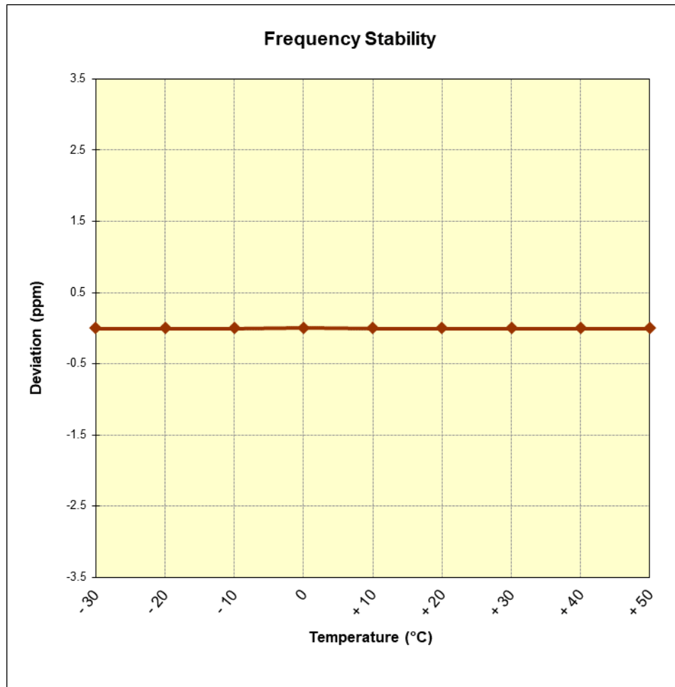
Figure 7-12. Frequency Stability Graph (PCS GPRS Mode – Ch. 661)
