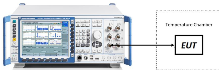
Figure 7-11. Test Instrument & Measurement Setup
