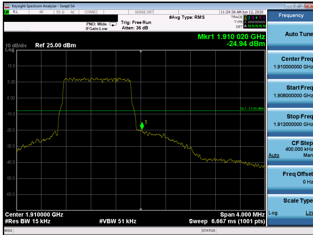
Plot 7-279. Upper Band Edge Plot (Band 2 - 1.4MHz QPSK - Full RB Configuration)
