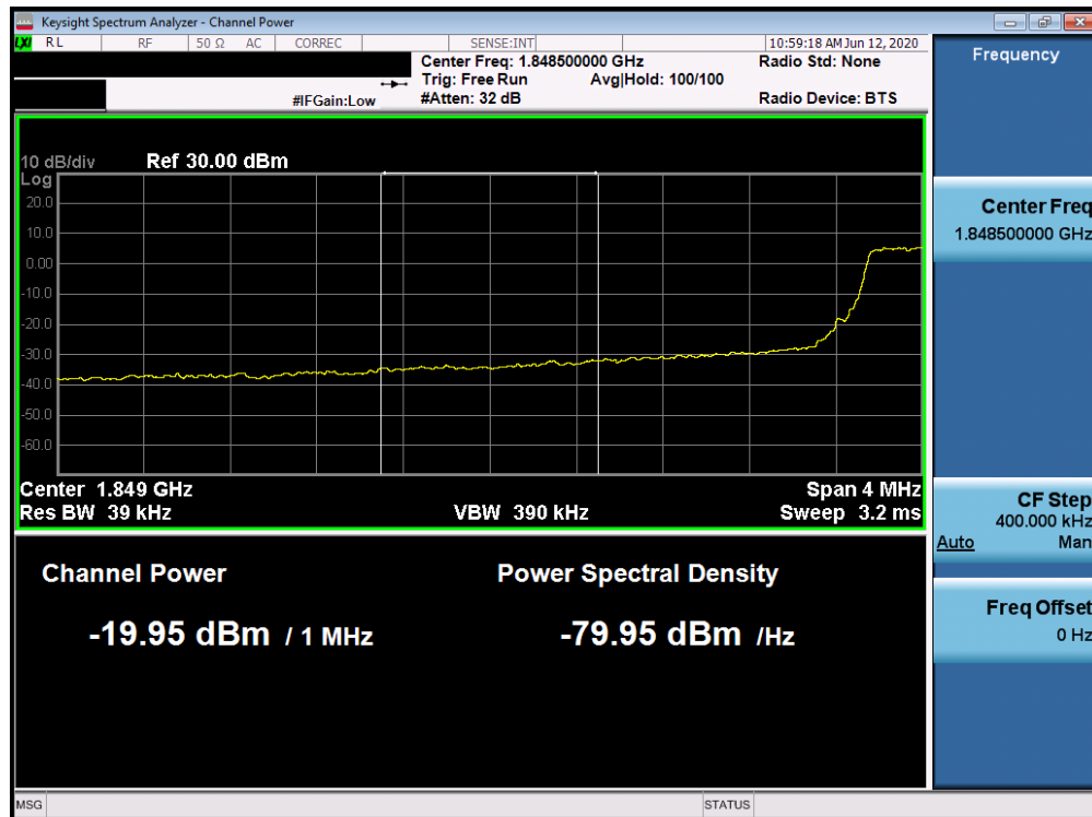
Plot 7-286. Lower Extended Band Edge Plot (Band 2 - 5.0MHz QPSK - Full RB Configuration)
