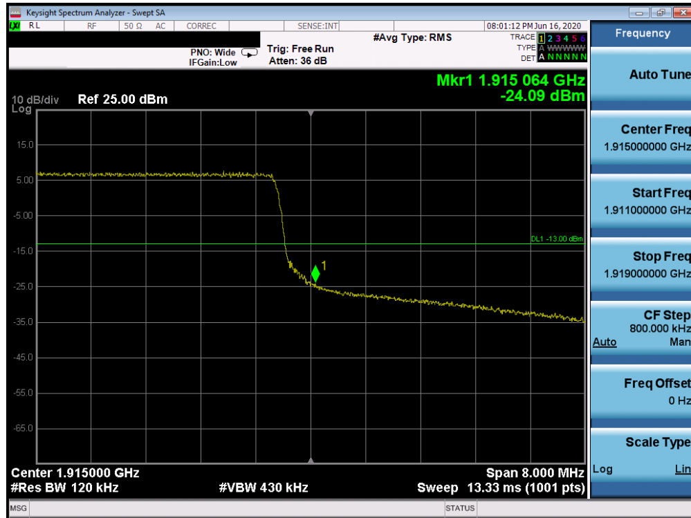
Plot 7-267. Upper Band Edge Plot (Band 25 - 10.0MHz QPSK - Full RB Configuration)
