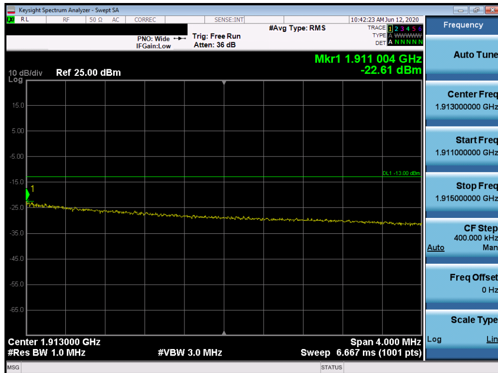
Plot 7-296. Upper Extended Band Edge Plot (Band 2 - 15.0MHz QPSK - Full RB Configuration)
