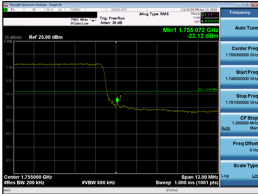
Plot 7-247. Upper Band Edge Plot (Band 4 - 15.0MHz QPSK - Full RB Configuration)
