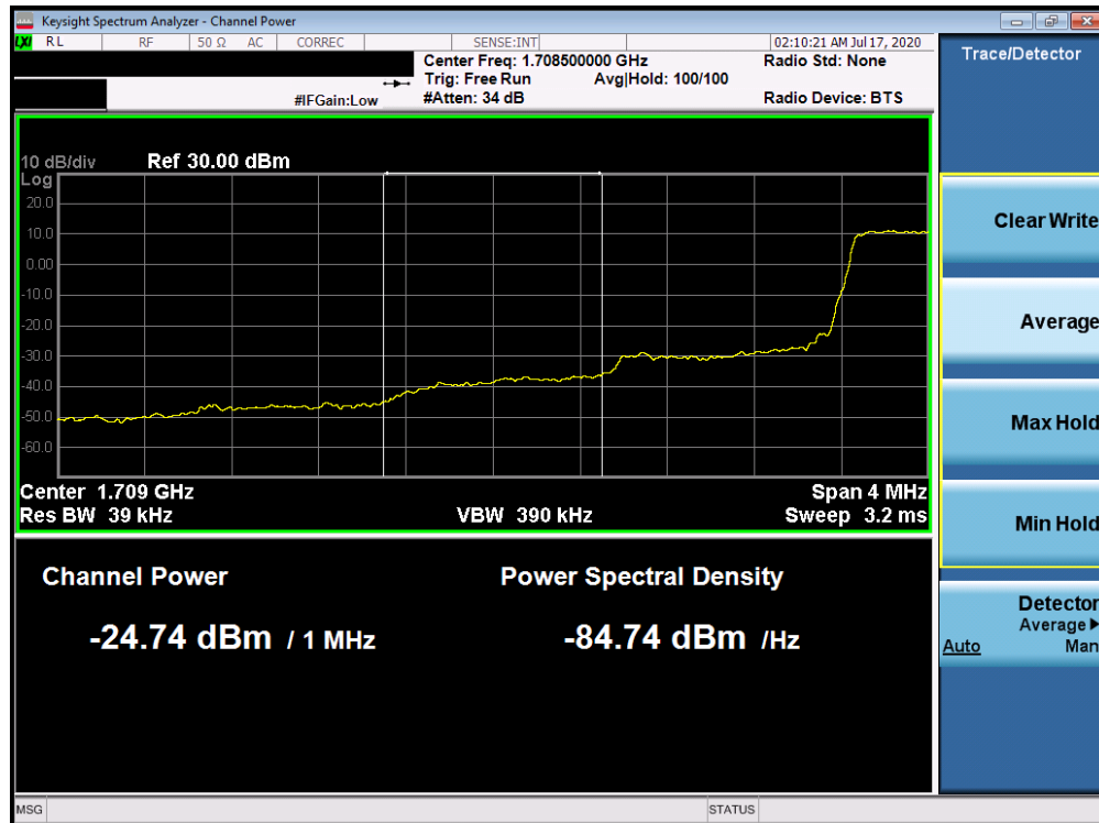
Plot 7-206. Lower Extended Band Edge Plot (Band 66 - 1.4MHz QPSK - Full RB Configuration)
