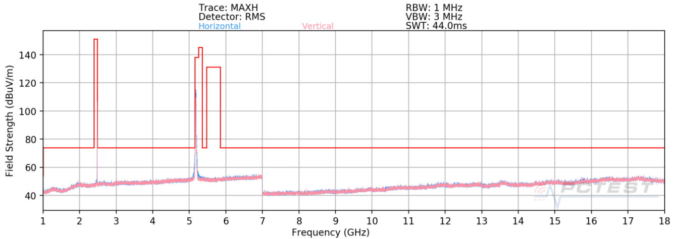
Plot 7-34. Radiated Spurious Emissions above 1GHz Simultaneous Tx
