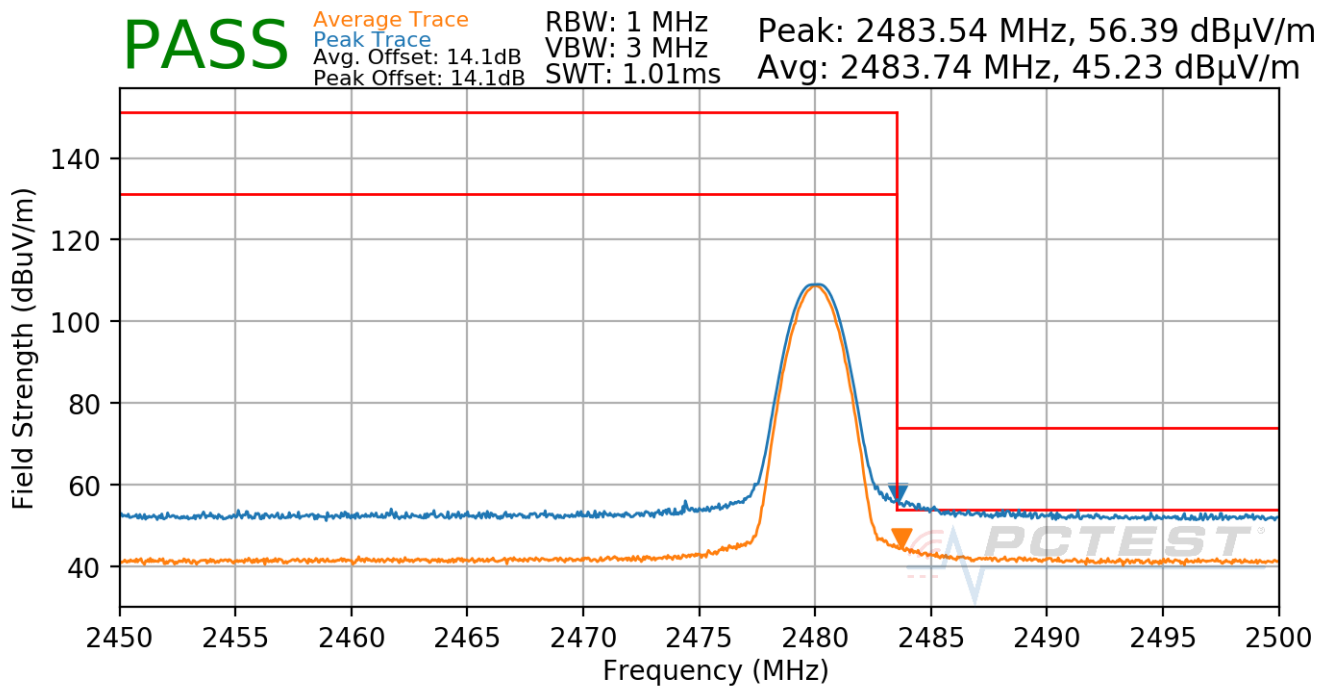
Plot 7-39. Radiated Restricted Upper Band Edge Measurement (Average & Peak)
