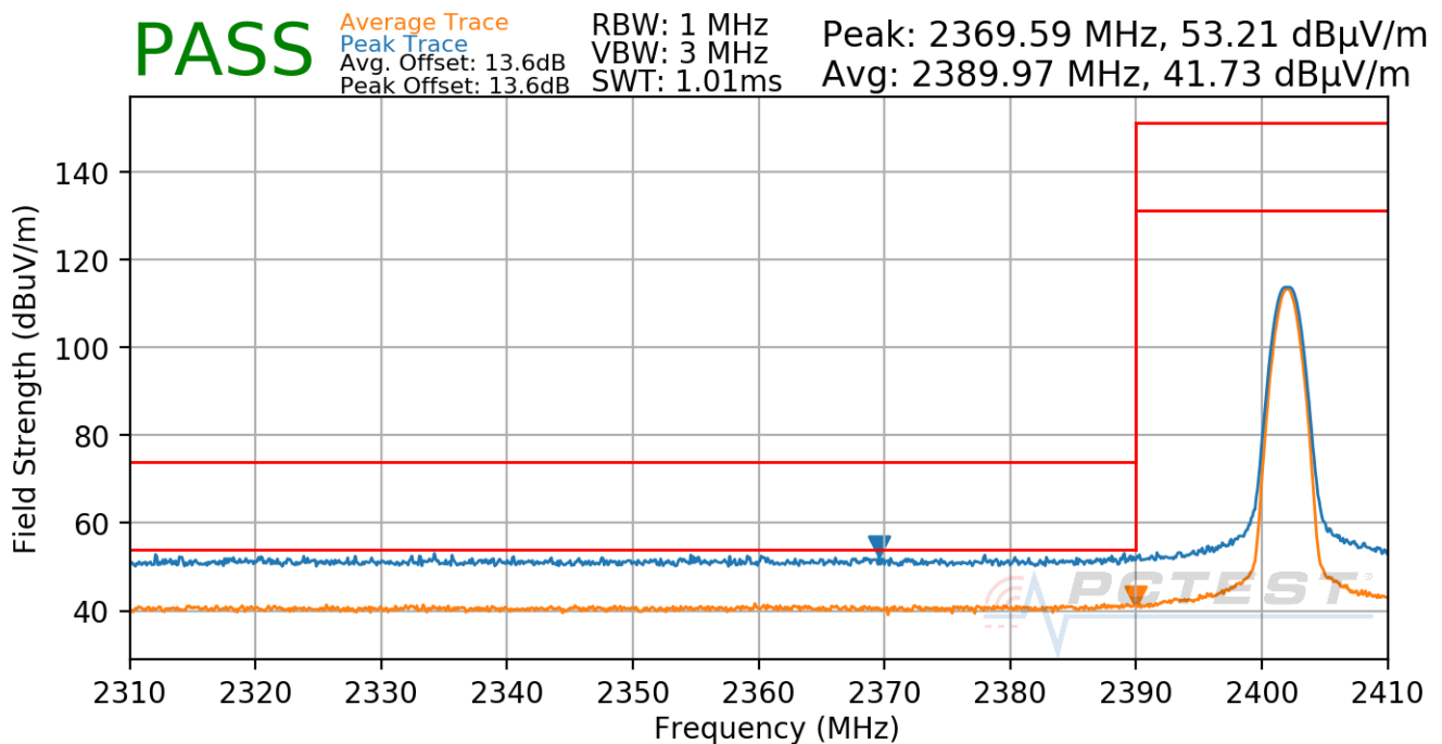
Plot 7-37. Radiated Restricted Lower Band Edge Measurement (Average & Peak)
