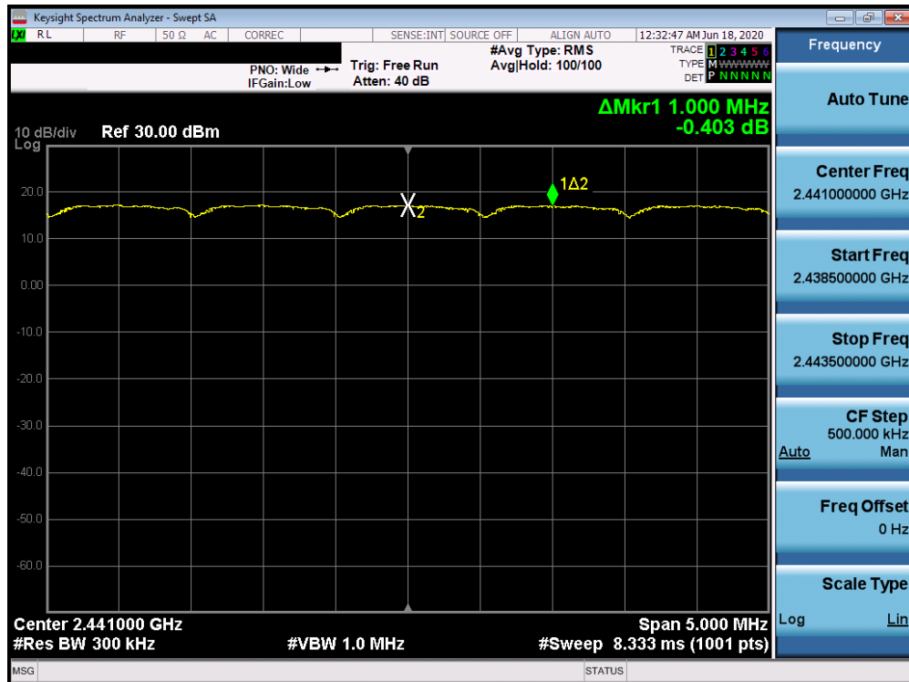
Plot 7-16. Channel Separation (Bluetooth, 8DPSK, ePA)
