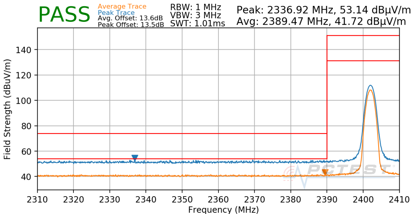
Plot 7-38. Radiated Restricted Lower Band Edge Measurement (Average & Peak)
