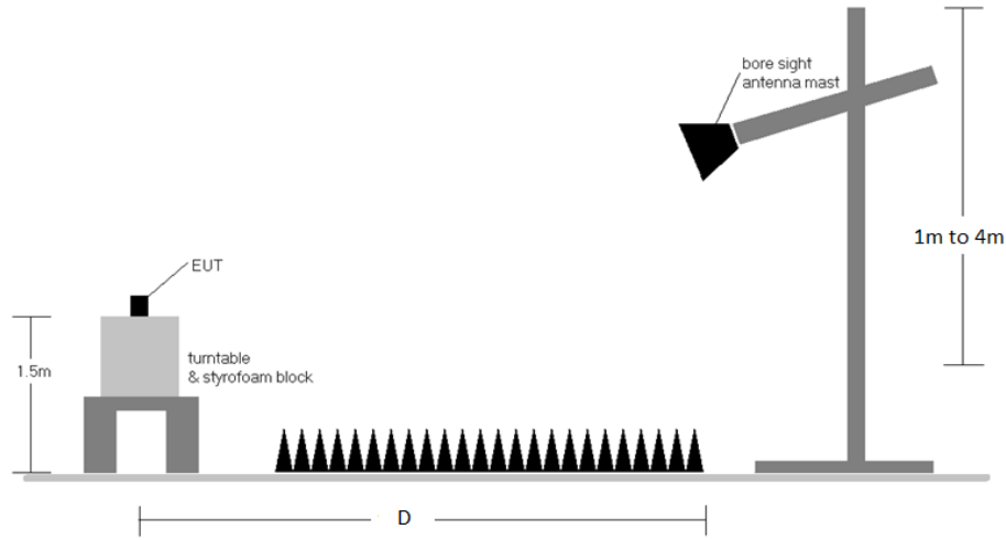
Figure 7-8. Radiated Test Setup >1GHz
