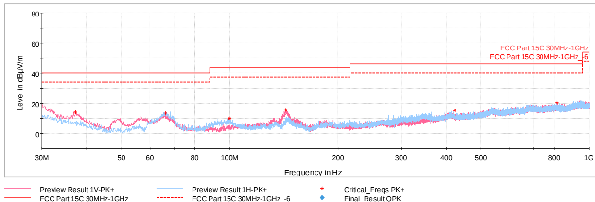
Plot 7-41. Radiated Spurious Emissions below 1GHz GFSK ePA – Ch.39 , with AC/DC Adapter)
