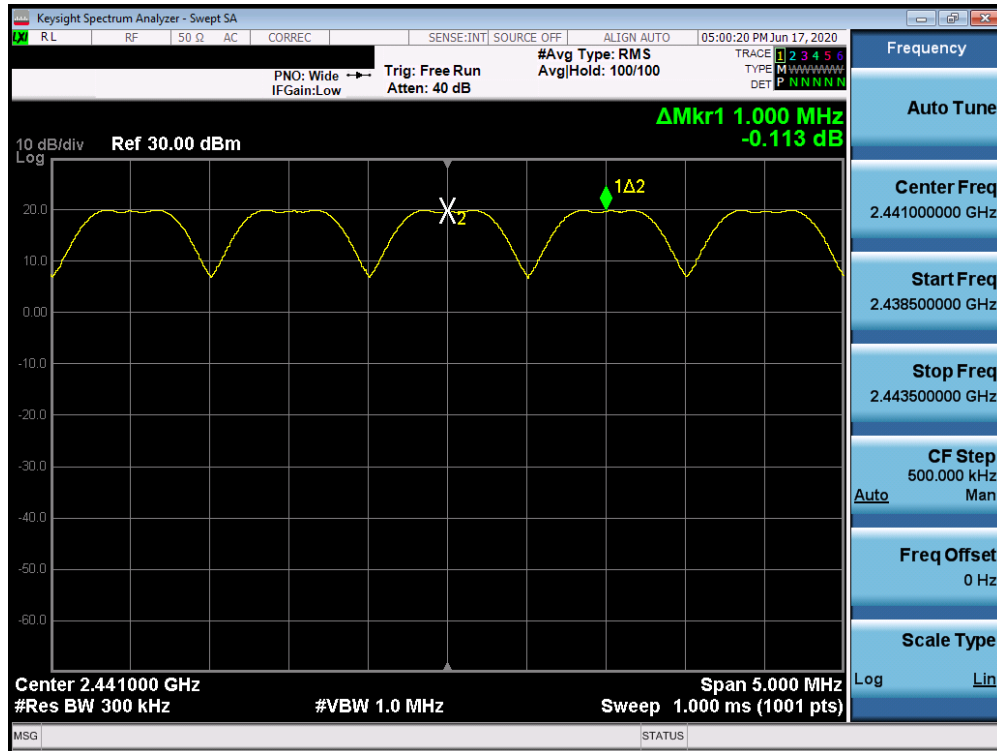
Plot 7-15. Channel Separation (Bluetooth, GFSK, ePA)
