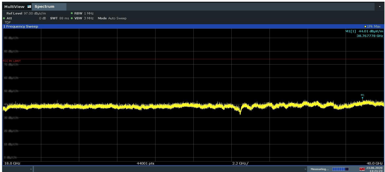
Plot 7-36. Radiated Spurious Emissions Simultaneous Tx 18GHz– 40GHz Pol. V
