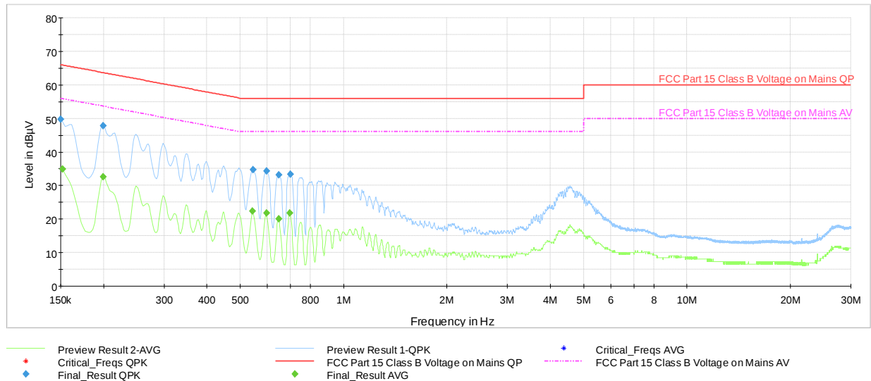
Plot 7-44. AC Line-Conducted Test Plot- Ch.39 (N, with AC/DC Adapter)
