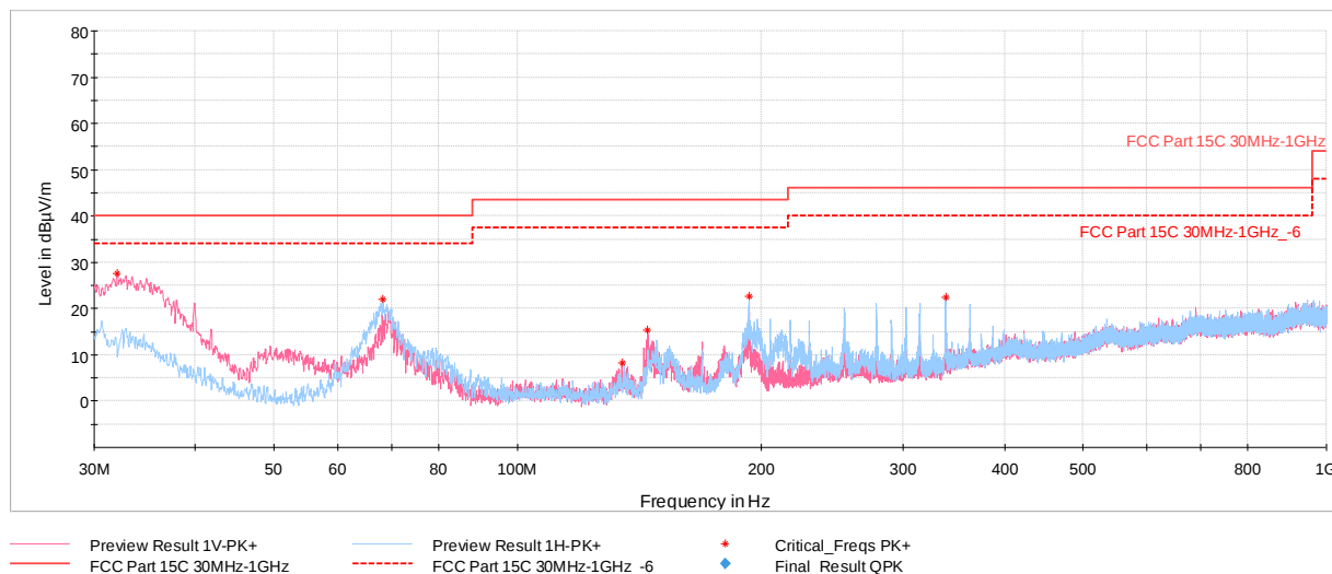
Plot 7-42. Radiated Spurious Emissions below 1GHz Simultaneous Tx, with AC/DC Adapter
