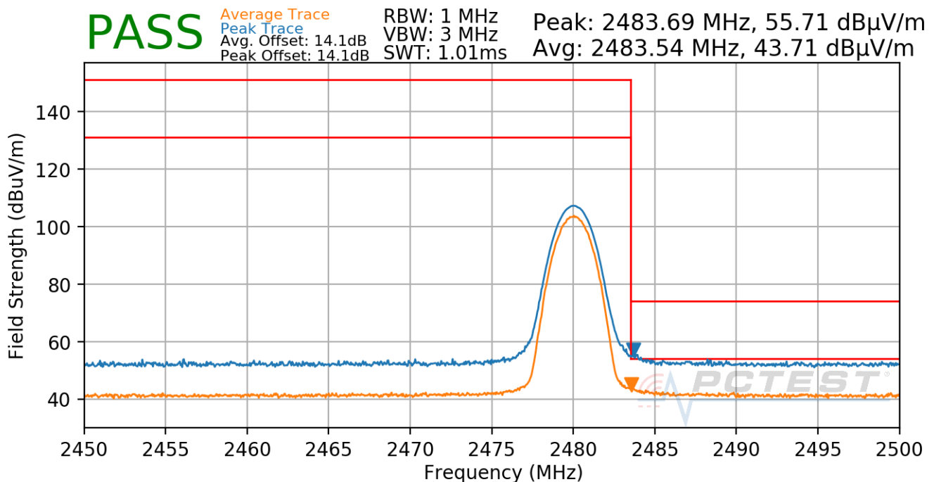
Plot 7-40. Radiated Restricted Upper Band Edge Measurement (Average & Peak)
