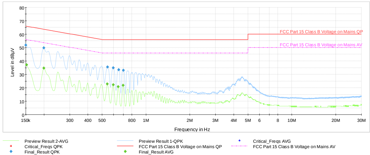
Plot 7-43. AC Line-Conducted Test Plot- Ch.39 (L1, with AC/DC Adapter)
