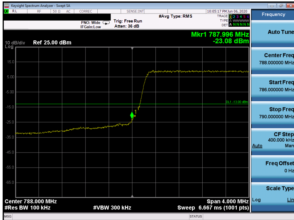
Plot 7-39. Lower Band Edge Plot (Band 14 - 5MHz QPSK - Full RB Configuration)
