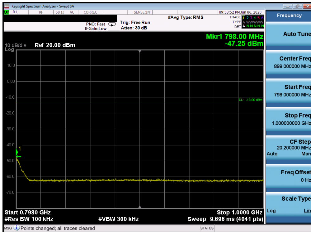
Plot 7-26. Conducted Spurious Plot (Band 14 - 10MHz QPSK - RB Size 1, RB Offset 0 - Mid Channel)
