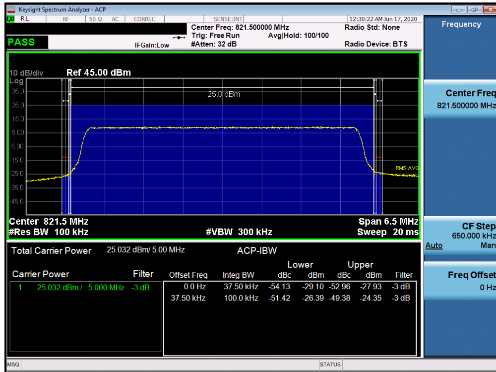
Plot 7-30. Channel Edge Plot (LTE Band 26 - 5MHz QPSK - High Channel)
