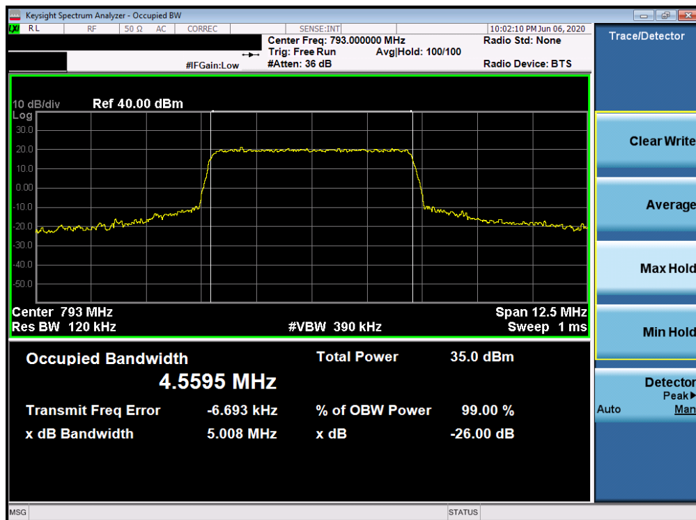
Plot 7-16. Occupied Bandwidth Plot (Band 14 - 5MHz QPSK - Full RB Configuration)
