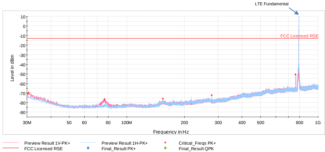
Plot 7-45. Radiated Spurious Emissions Below 1GHz (Band 14)
