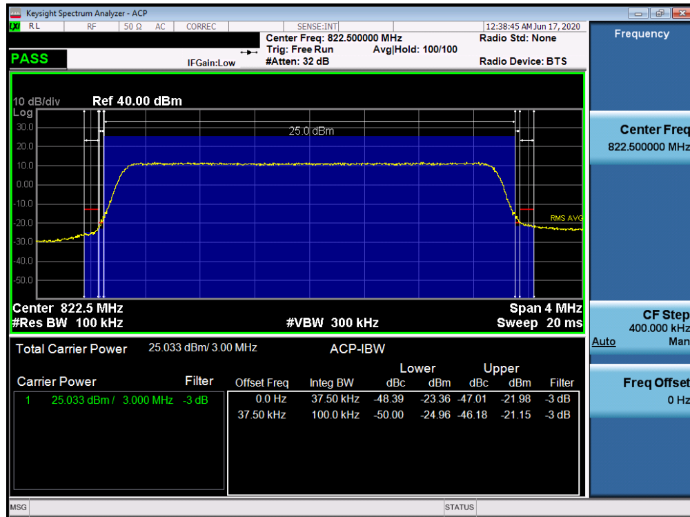
Plot 7-32. Channel Edge Plot (LTE Band 26 - 3MHz QPSK - High Channel)
