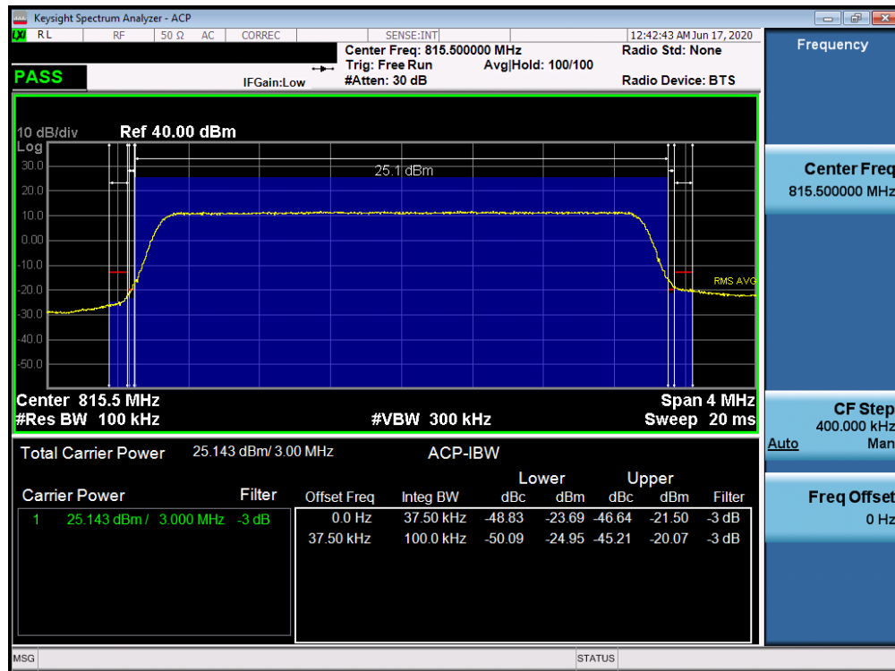
Plot 7-31. Channel Edge Plot (LTE Band 26 - 3MHz QPSK - Low Channel)
