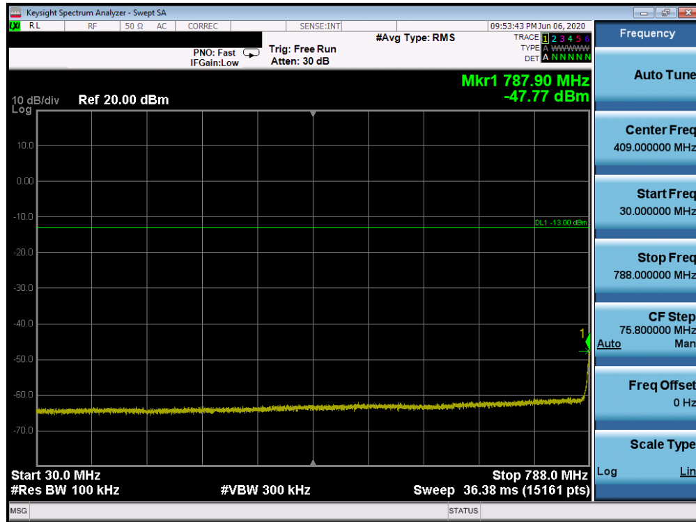
Plot 7-25. Conducted Spurious Plot (Band 14 - 10MHz QPSK - RB Size 1, RB Offset 0 - Mid Channel)
