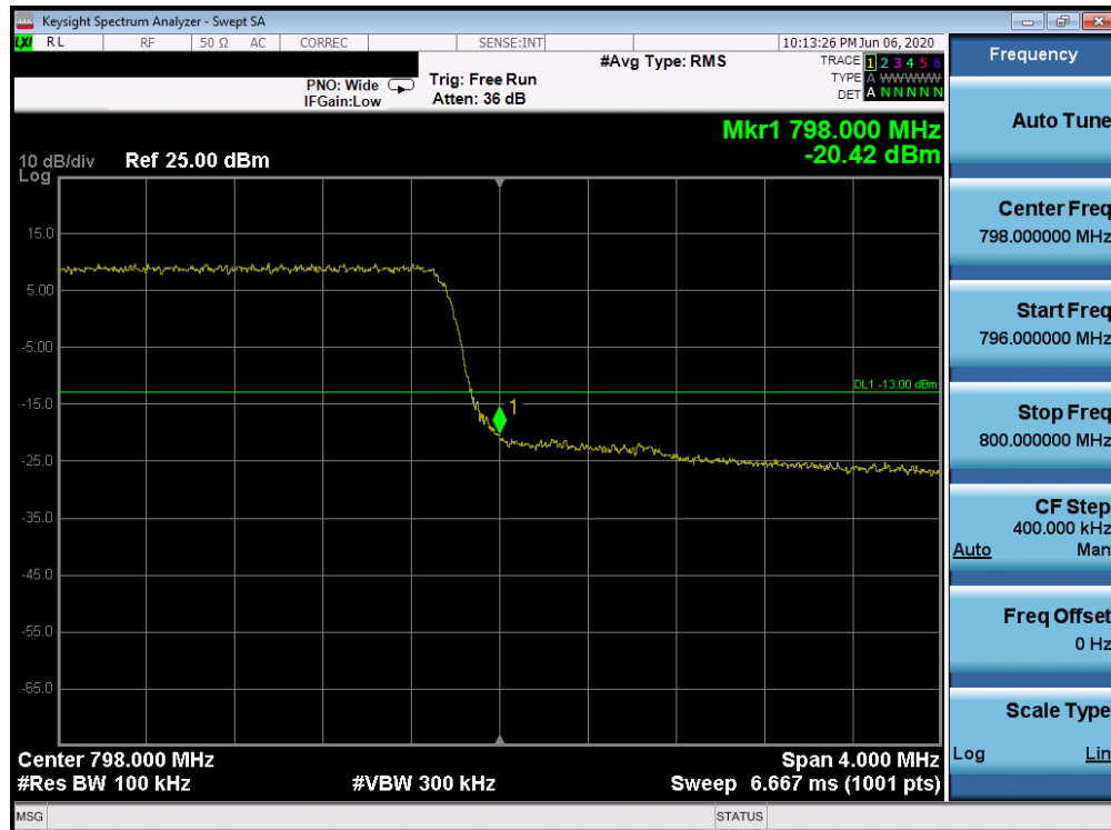
Plot 7-41. Upper Band Edge Plot (Band 14 - 5MHz QPSK - Full RB Configuration)
