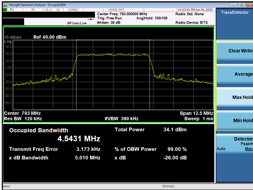
Plot 7-17. Occupied Bandwidth Plot (Band 14 - 5MHz 16-QAM - Full RB Configuration)
