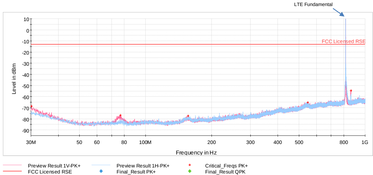
Plot 7-43. Radiated Spurious Emissions Below 1GHz (Band 26)
