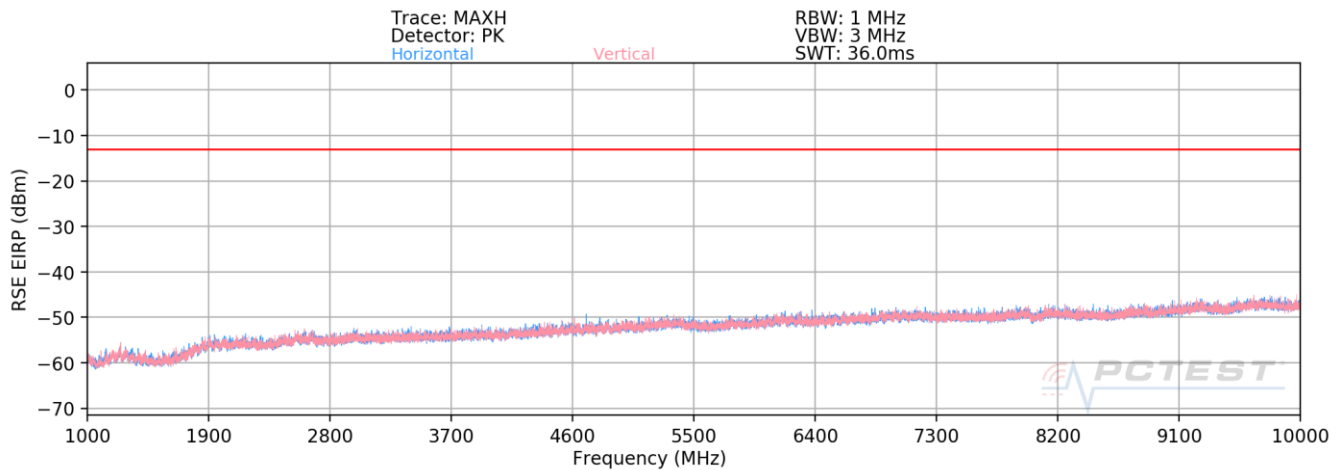
Plot 7-44. Radiated Spurious Emissions Above 1GHz (Band 26)
