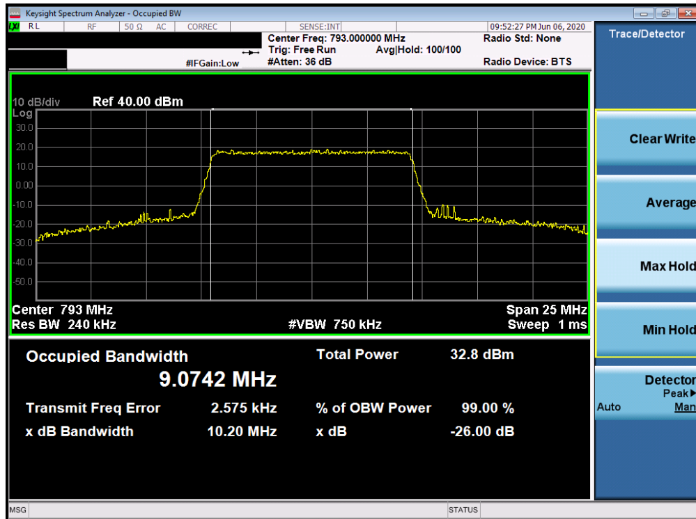
Plot 7-15. Occupied Bandwidth Plot (Band 14 - 10MHz 64-QAM - Full RB Configuration)
