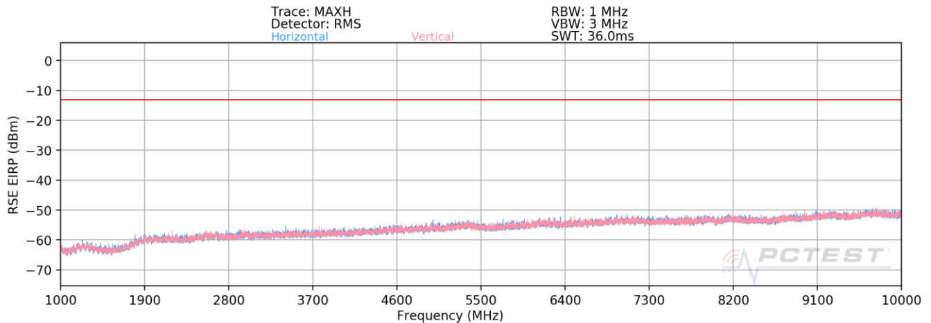
Plot 7-46. Radiated Spurious Emissions Above 1GHz (Band 14)
