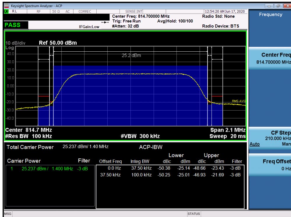
Plot 7-33. Channel Edge Plot (LTE Band 26 - 1.4MHz QPSK - Low Channel)
