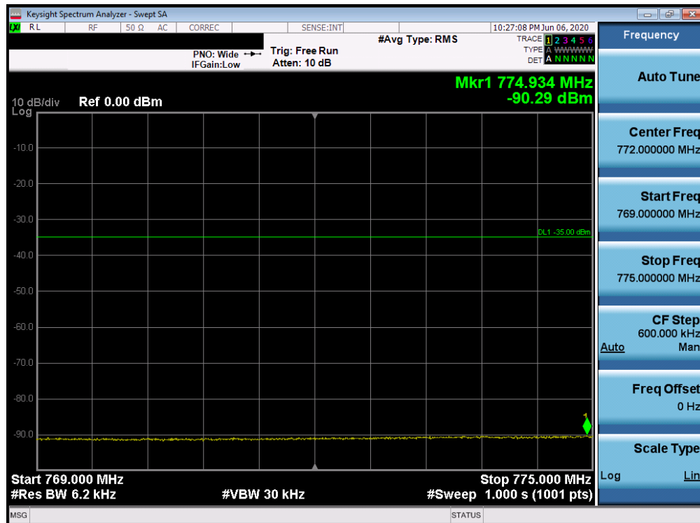
Plot 7-40. Lower Extended Band Edge Plot (Band 14 - 5MHz QPSK - Full RB Configuration)
