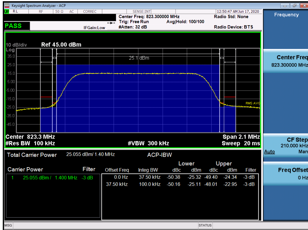
Plot 7-34. Channel Edge Plot (LTE Band 26 - 1.4MHz QPSK - High Channel)
