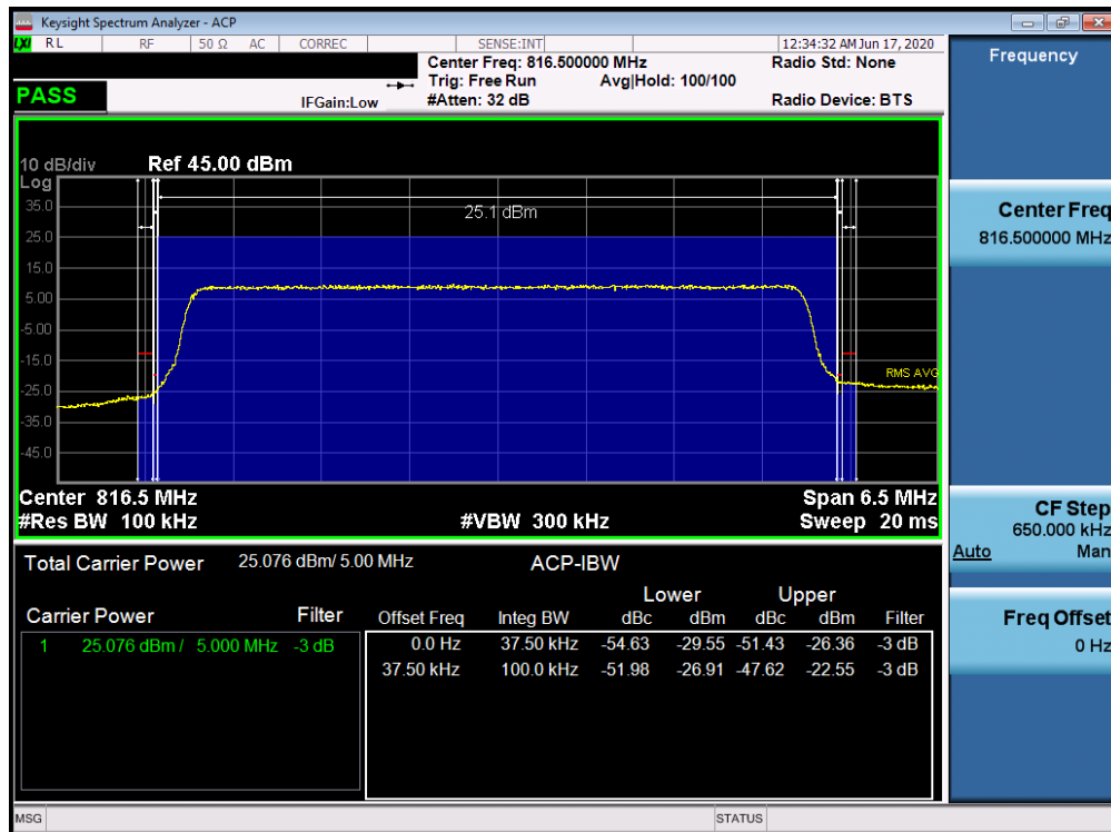
Plot 7-29. Channel Edge Plot (LTE Band 26 - 5MHz QPSK - Low Channel)
