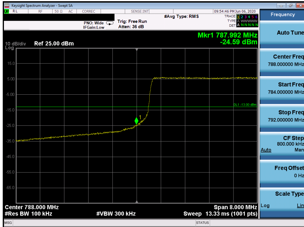
Plot 7-35. Lower Band Edge Plot (Band 14 - 10MHz QPSK - Full RB Configuration)
