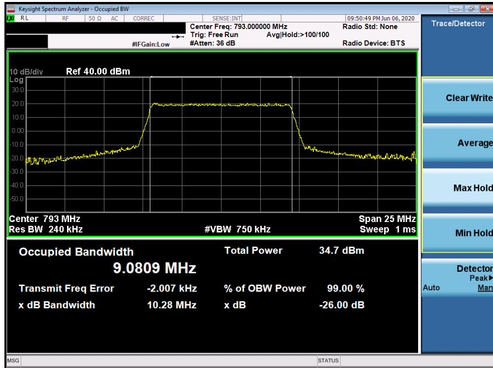
Plot 7-13. Occupied Bandwidth Plot (Band 14 - 10MHz QPSK - Full RB Configuration)
