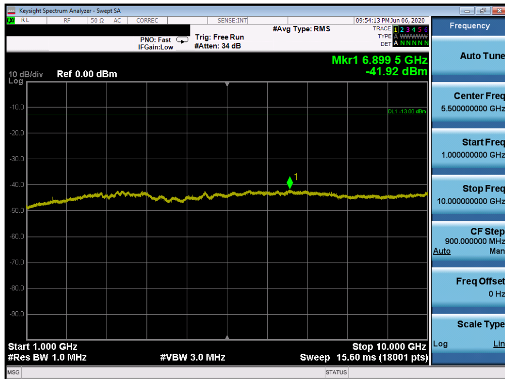
Plot 7-27. Conducted Spurious Plot (Band 14 - 10MHz QPSK - RB Size 1, RB Offset 0 - Mid Channel)
