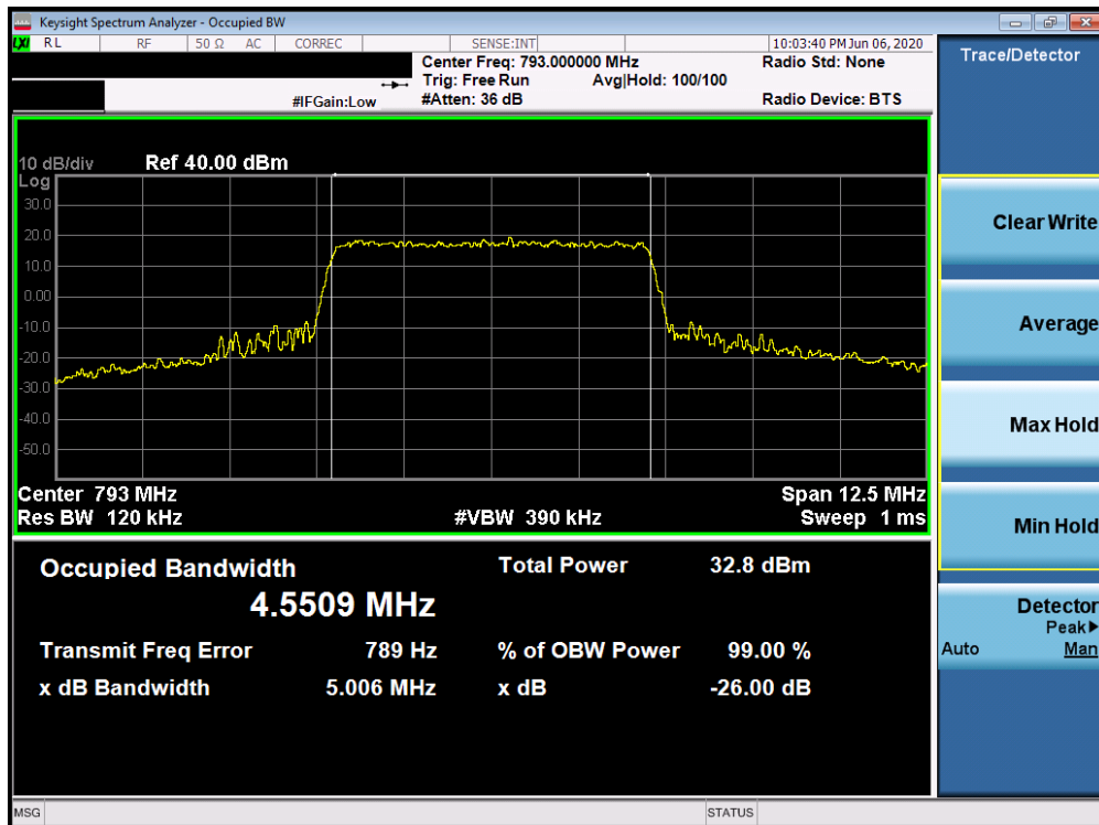
Plot 7-18. Occupied Bandwidth Plot (Band 14 - 5MHz 64-QAM - Full RB Configuration)
