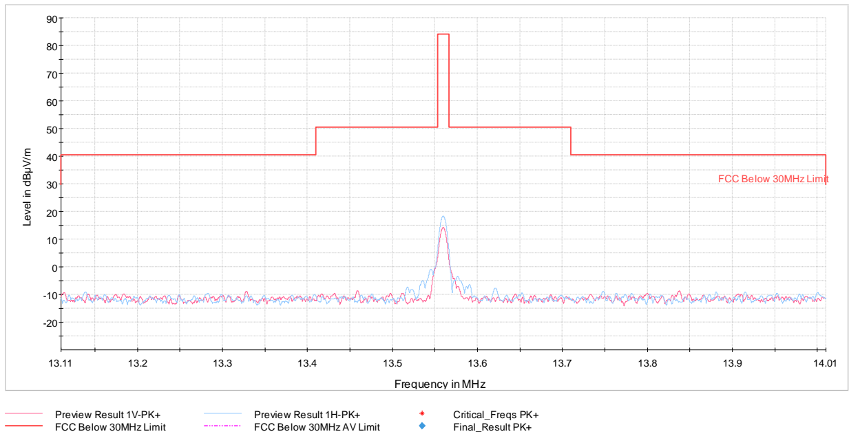
Plot 7-6. In Band Radiated Spurious Emissions (CE A 848kbps, with WCP + AC/DC Adapter)
