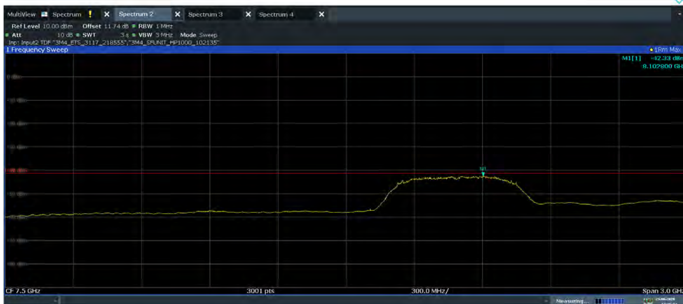
Plot 7-72. Average Radiated Power (Ch. 9, Config 0/Payload 65)
