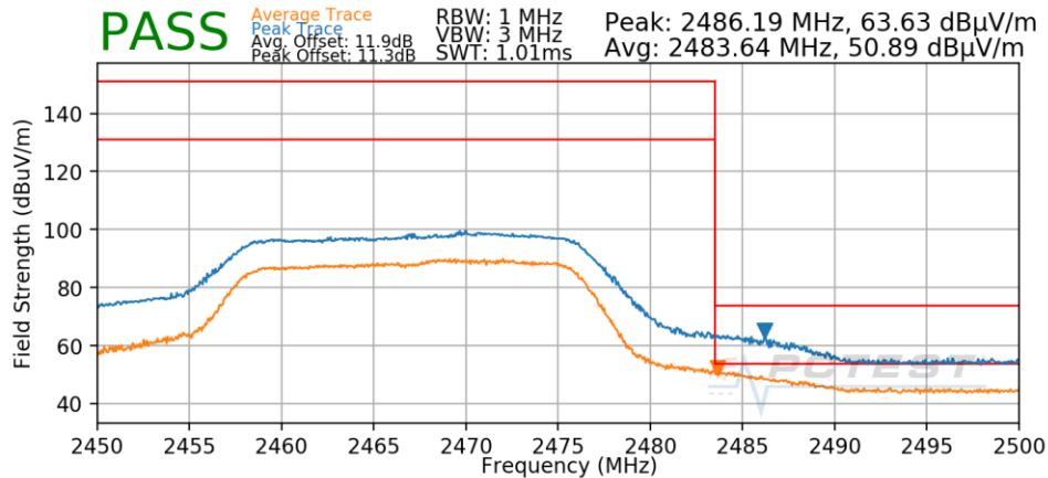
Plot 7-60. Radiated Restricted Upper Band Edge Measurement
