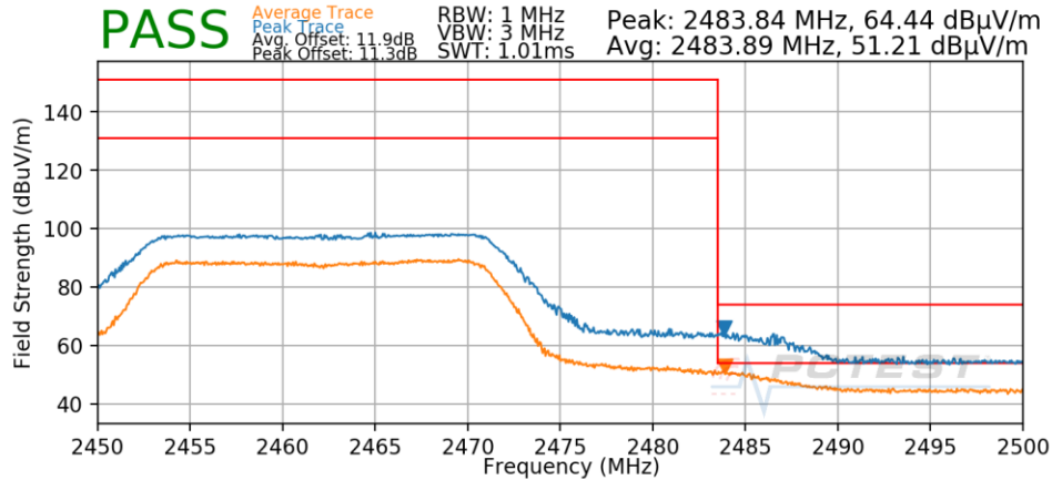
Plot 7-59. Radiated Restricted Upper Band Edge Measurement
