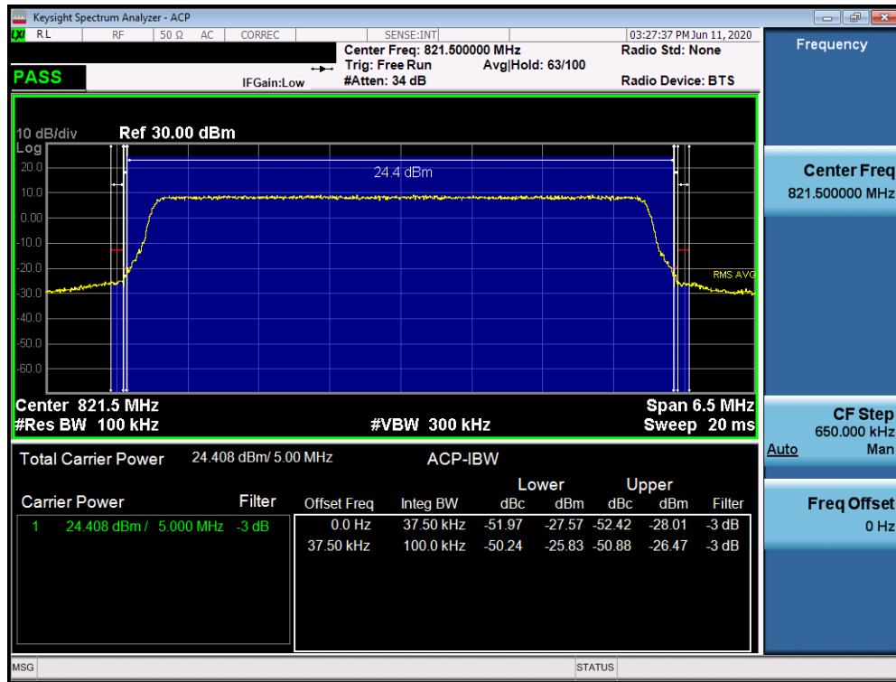
Plot 7-17. Channel Edge Plot (LTE Band 26 - 5MHz QPSK - High Channel)
