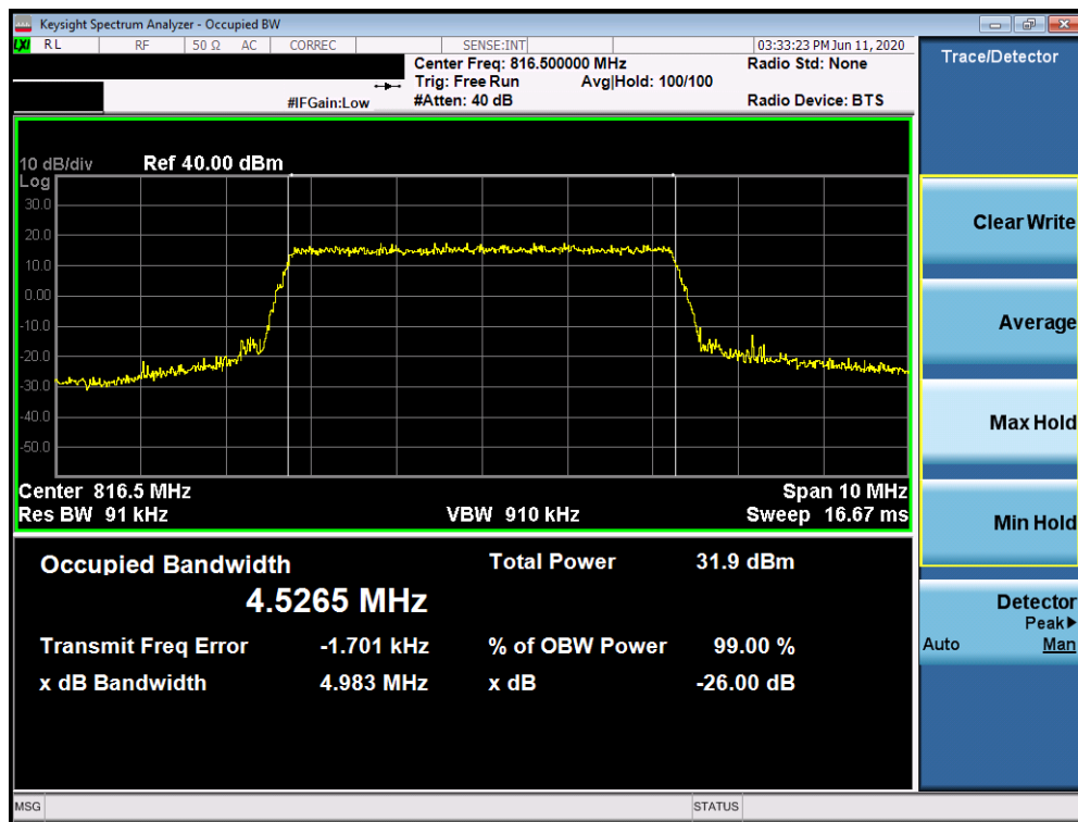
Plot 7-4. Occupied Bandwidth Plot (LTE Band 26 - 5MHz 16-QAM - Full RB Configuration)
