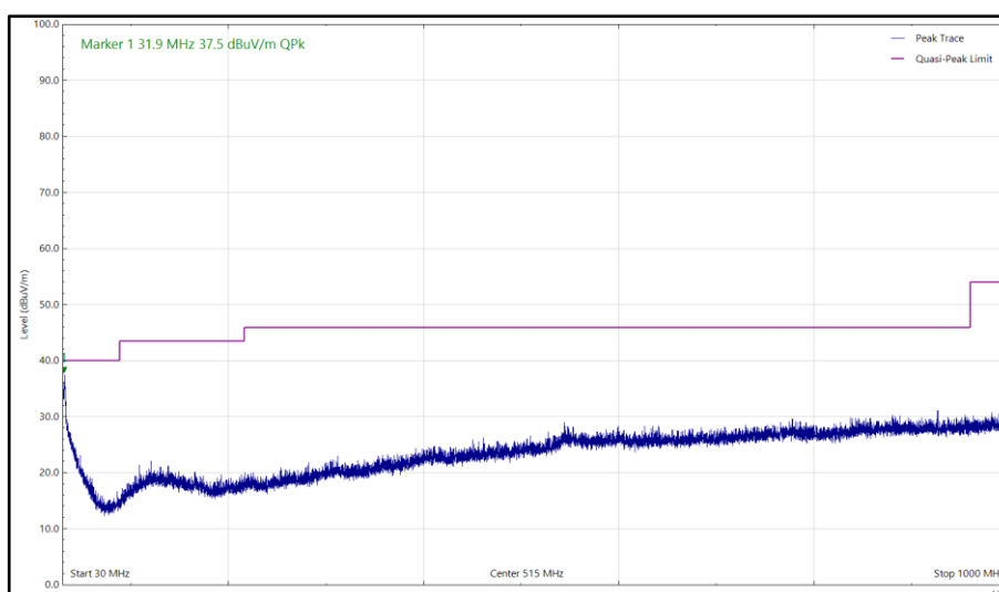
Figure 27 – 2417 MHz (CH2), HT20, CDD, Core 0 + Core 1 and U-NII 1 5200 MHz, HT20, CDD, Core 0 + Core 1, 30 MHz to 1 GHz, Vertical, Q-Peak
