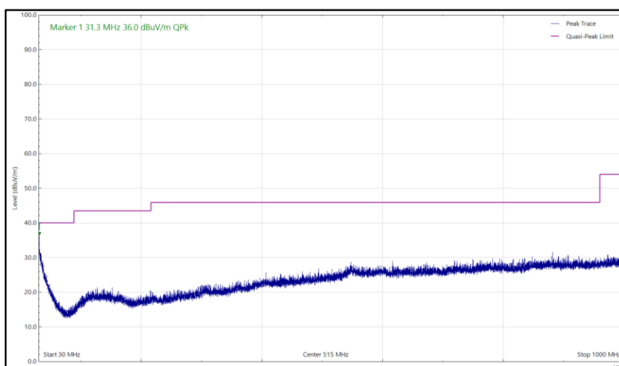
Figure 33 – 2452 MHz (CH9), HT20, CDD, Core 0 + Core 1 and U-NII 1 5680 MHz (CH138), HT20 CDD, Core 0 + Core 1, 30 MHz to 1 GHz, Vertical, Q-Peak
