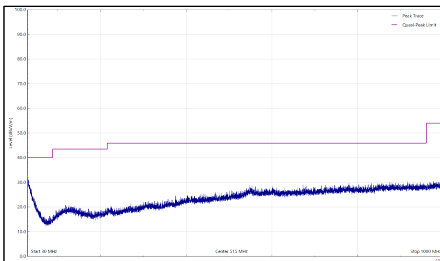
Figure 32 – 2452 MHz (CH9), HT20, CDD, Core 0 + Core 1 and U-NII 1 5680 MHz (CH138), HT20 CDD, Core 0 + Core 1, 30 MHz to 1 GHz, Horizontal, Q-Peak
