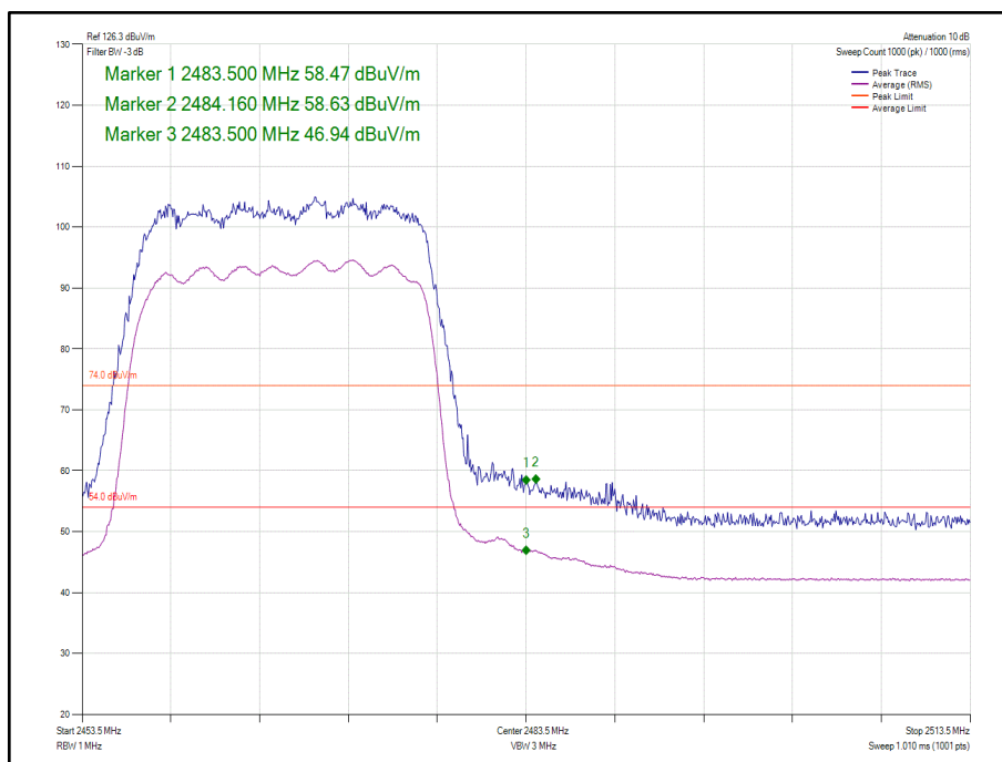
Figure 154 - 802.11ax HE20, Core 0-1, SU - 2467 MHz, Band Edge Frequency 2483.5 MHz
