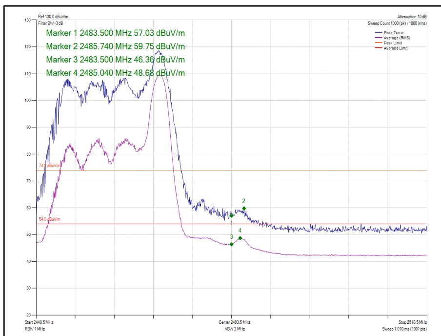
Figure 153 - 802.11ax HE20, Core 0-1, 26-8 - 2462 MHz, Band Edge Frequency 2483.5 MHz
