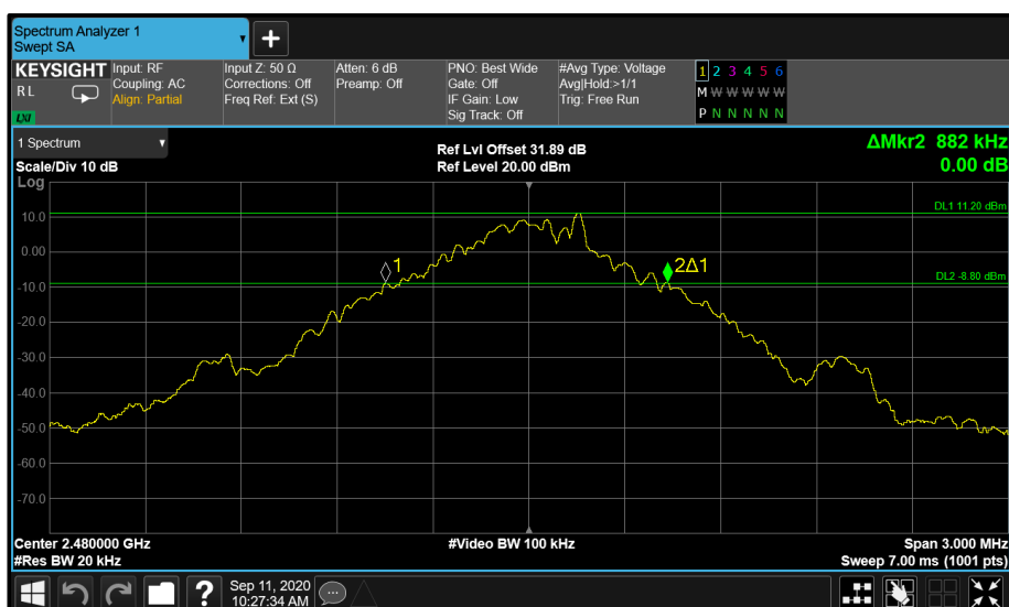
Figure 25 - Core 0 GFSK 2480 MHz (CH78)
