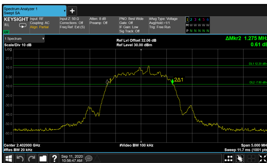
Figure 59 - Core 1 8-DPSK 2402 MHz (CH0)
