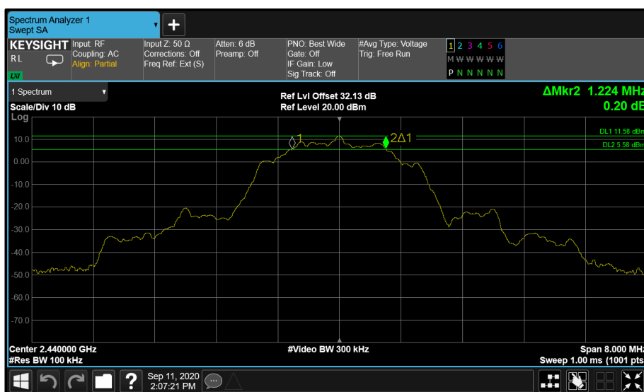
Figure 11 - Core 1 LE 2M 2440 MHz (CH19)
