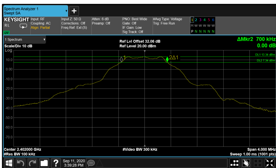
Figure 61 - Core 1 LE 1M 2402 MHz (CH0)
