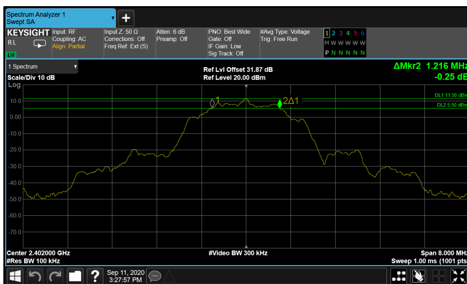
Figure 32 - Core 0 LE 2M 2402 MHz (CH0)
