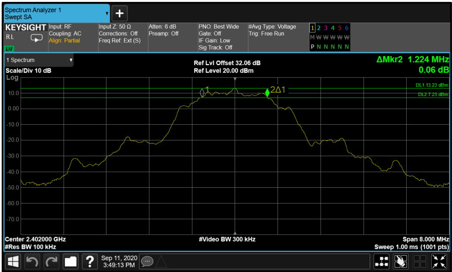
Figure 67 - Core 1 LE 2M 2402 MHz (CH0)
