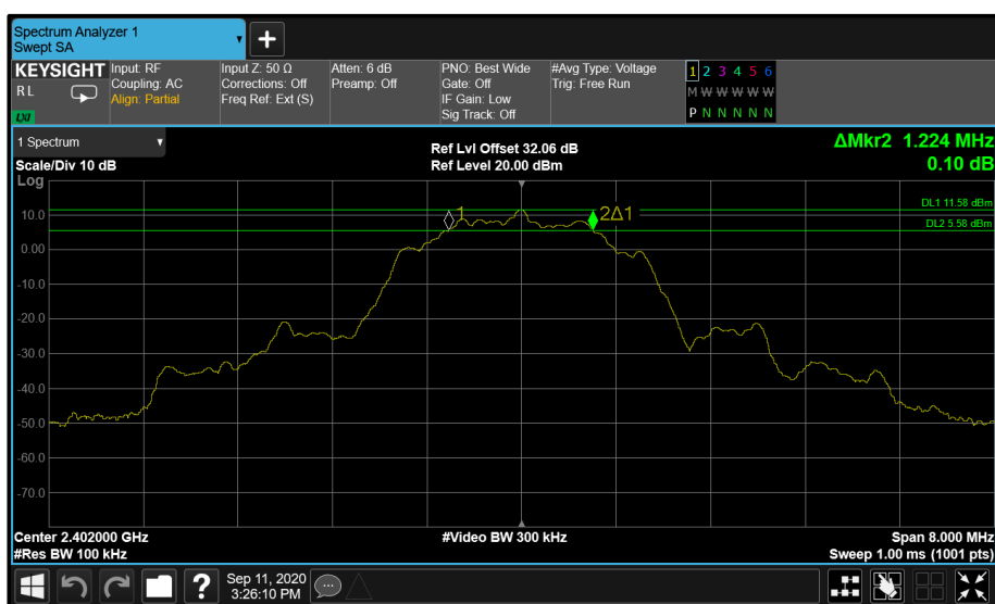
Figure 31 - Core 1 LE 2M 2402 MHz (CH0)
