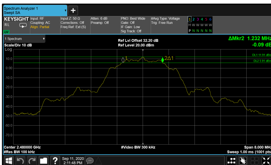
Figure 12 - Core 1 LE 2M 2480 MHz (CH39)
