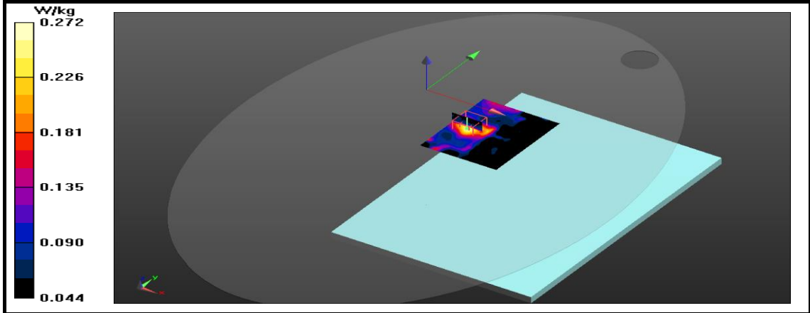
Figure 16: SAR Body Testing Results for the A2337 at 5270 MHz.
