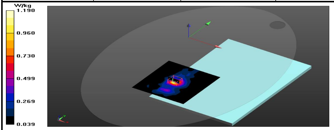
Figure 15: SAR Body Testing Results for the A2337 at 5270 MHz.
