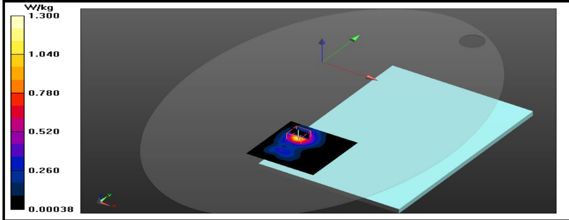
Figure 32: SAR Body Testing Results for the A2337 at 5775 MHz.
