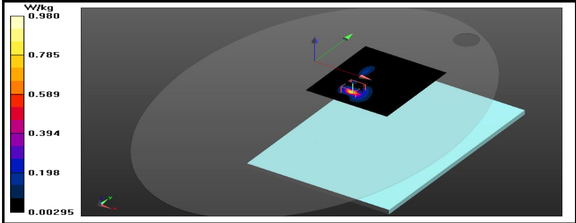
Figure 9: SAR Body Testing Results for the A2337 at 2452 MHz.
