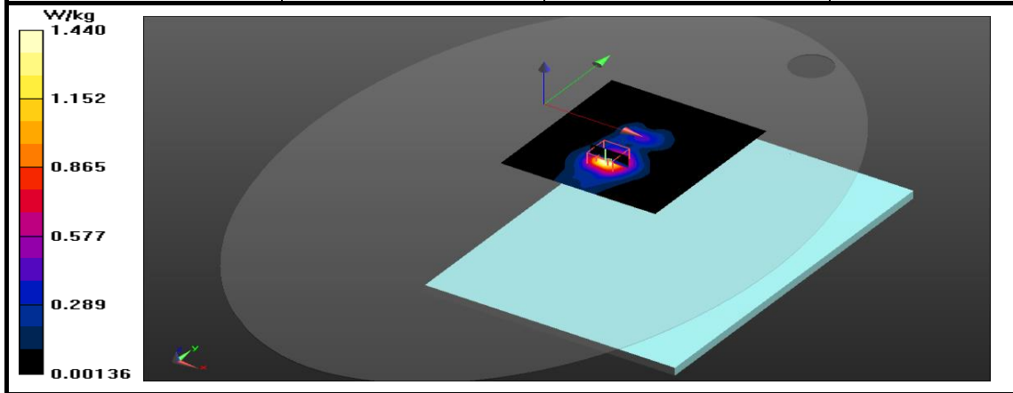
Figure 21: SAR Body Testing Results for the A2337 at 5610 MHz.
