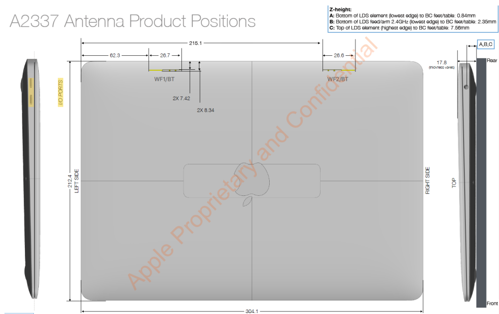
Figure 1 Antenna Location Diagram
