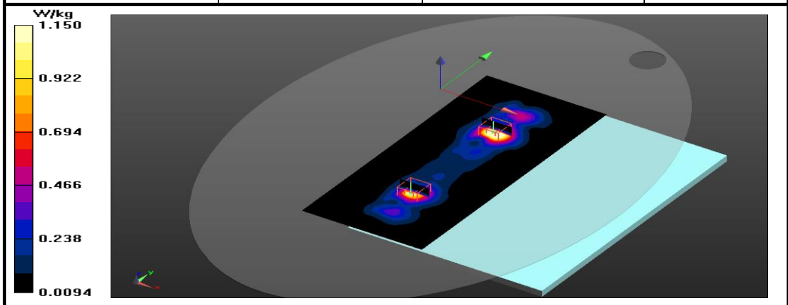
Figure 17: SAR Body Testing Results for the A2337 at 5270 MHz.
