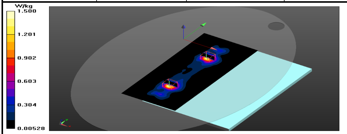
Figure 27: SAR Body Testing Results for the A2337 at 5690 MHz.
