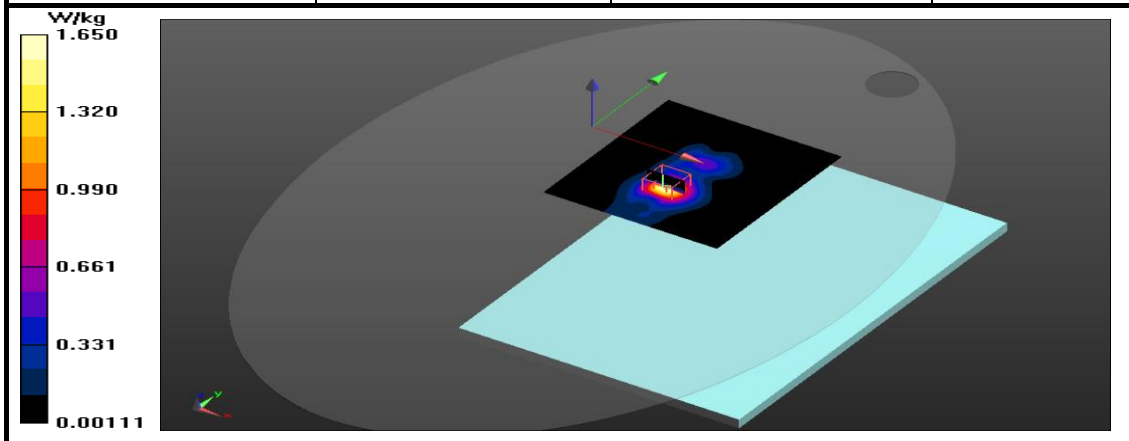
Figure 14: SAR Body Testing Results for the A2337 at 5310 MHz
