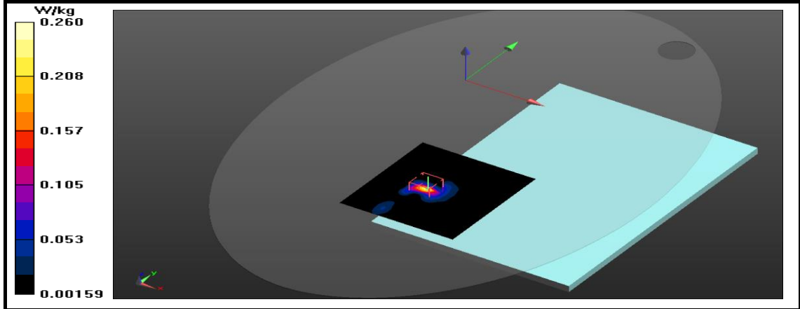
Figure 5: SAR Body Testing Results for the A2337 at 2480 MHz.
