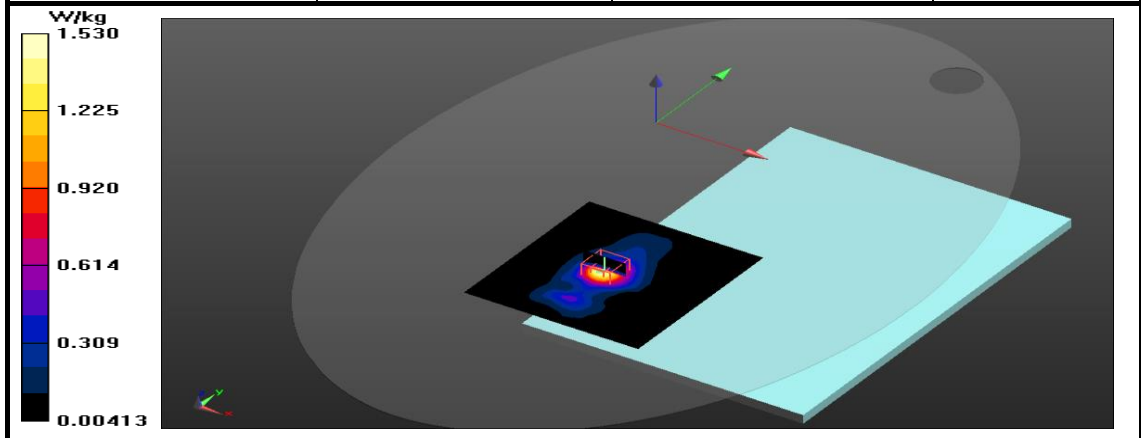
Figure 23: SAR Body Testing Results for the A2337 at 5690 MHz.
