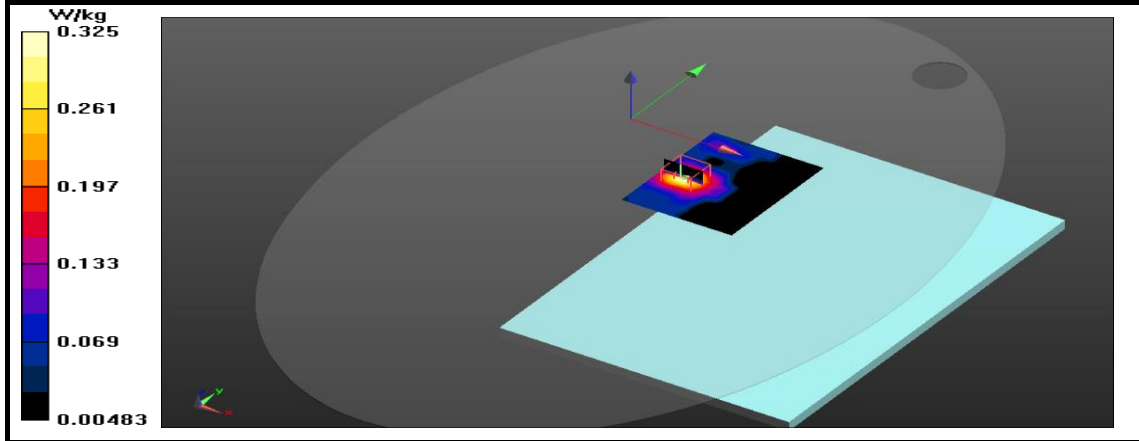
Figure 24: SAR Body Testing Results for the A2337 at 5690 MHz.
