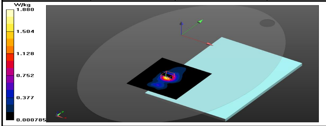
Figure 25: SAR Body Testing Results for the A2337 at 5610 MHz.
