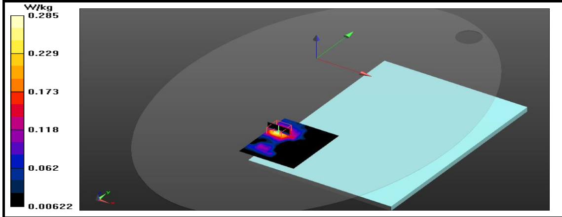
Figure 20: SAR Body Testing Results for the A2337 at 5690 MHz.
