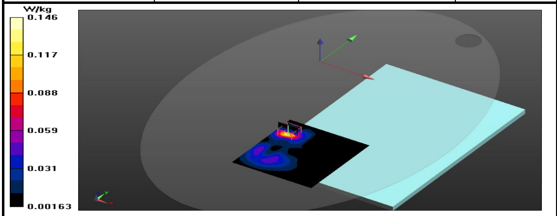
Figure 10: SAR Body Testing Results for the A2337 at 2452 MHz.
