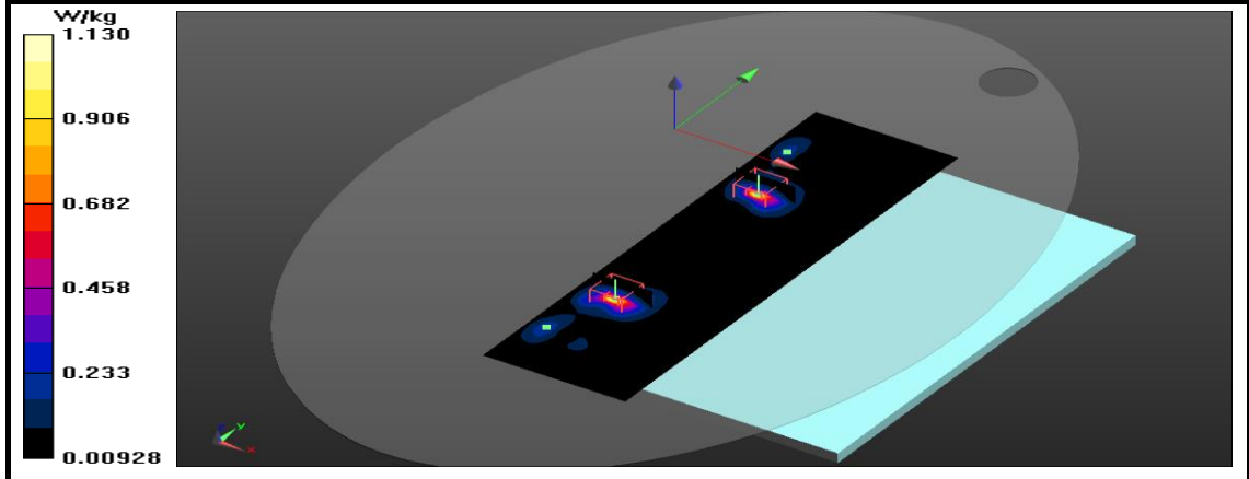
Figure 11: SAR Body Testing Results for the A2337 at 2437 MHz.
