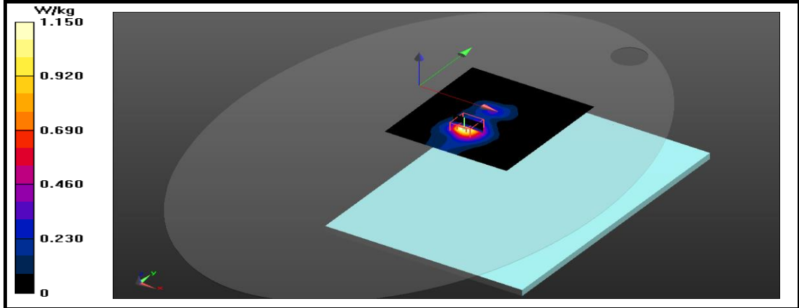
Figure 22: SAR Body Testing Results for the A2337 at 5530 MHz.
