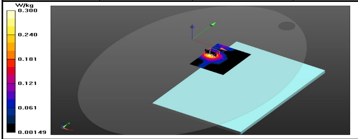
Figure 33: SAR Body Testing Results for the A2337 at 5775 MHz.
