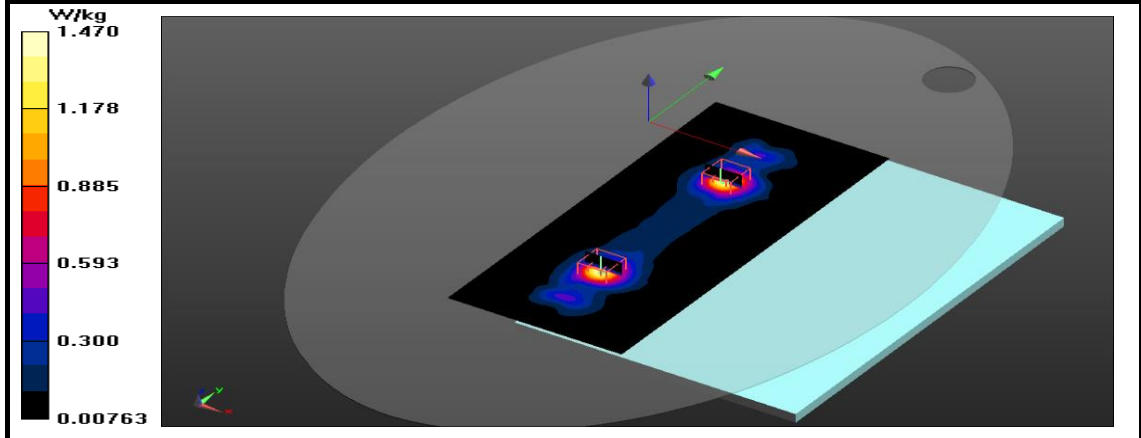
Figure 34: SAR Body Testing Results for the A2337 at 5775 MHz.
