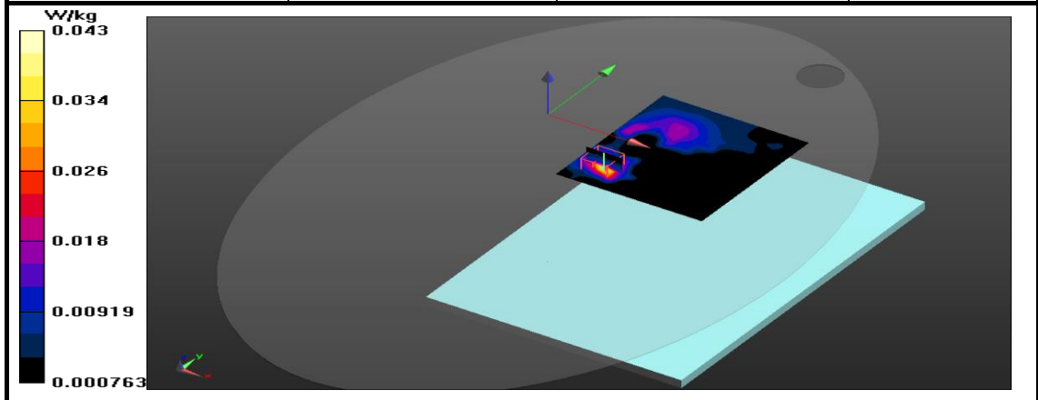
Figure 6: SAR Body Testing Results for the A2337 at 2480 MHz.
