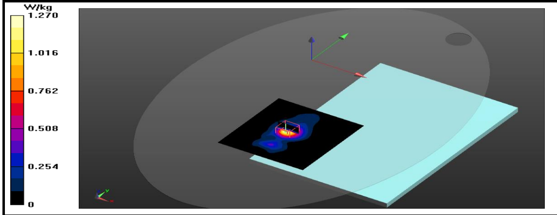
Figure 26: SAR Body Testing Results for the A2337 at 5530 MHz.
