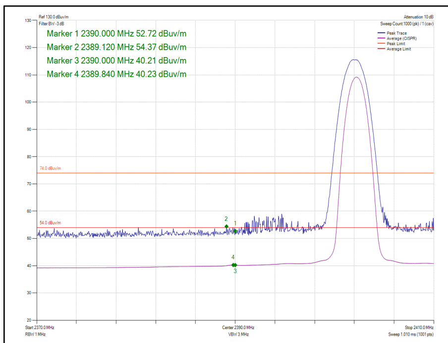
Figure 126 - Core 1 - \pi/4 DQPSK/2DH5 - 2402 MHz - Band Edge Frequency 2390.0 MHz
