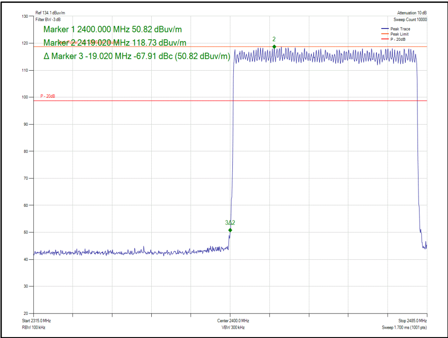
Figure 99 - Hopping - Core 0-1- π/4 DQPSK/2DH5 - Band Edge Frequency 2400.0 MHz
