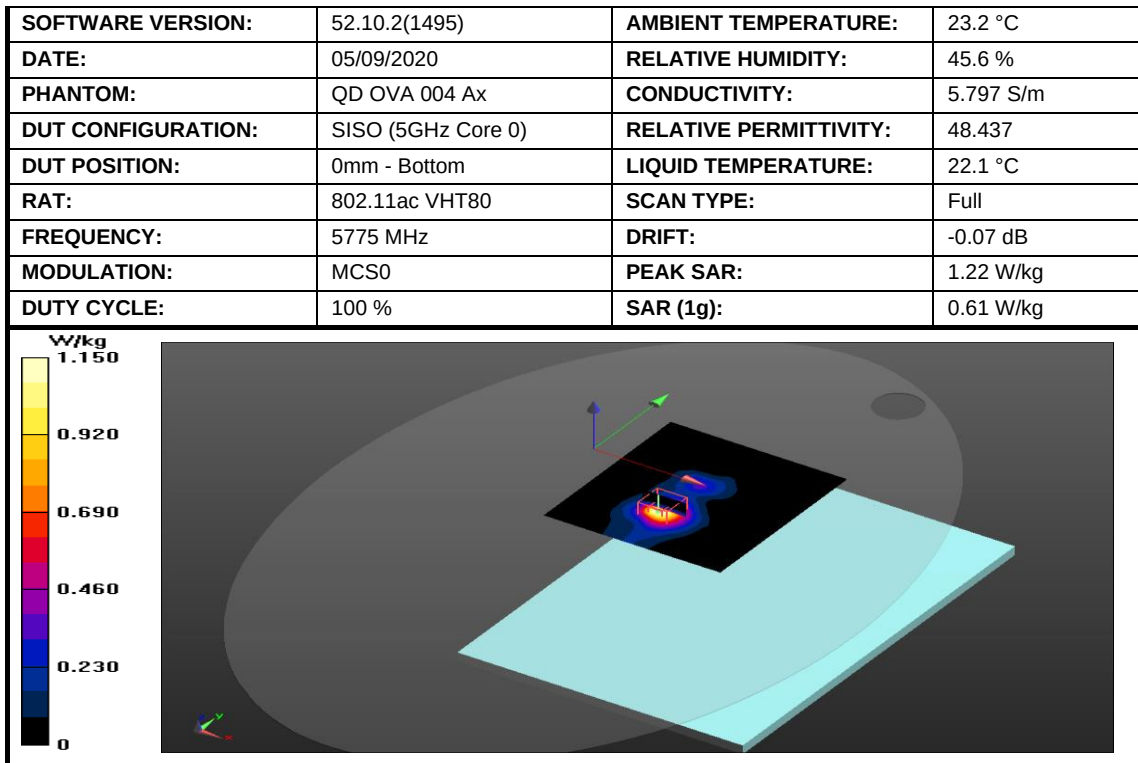
Figure 30: SAR Body Testing Results for the A2337 at 5775 MHz
