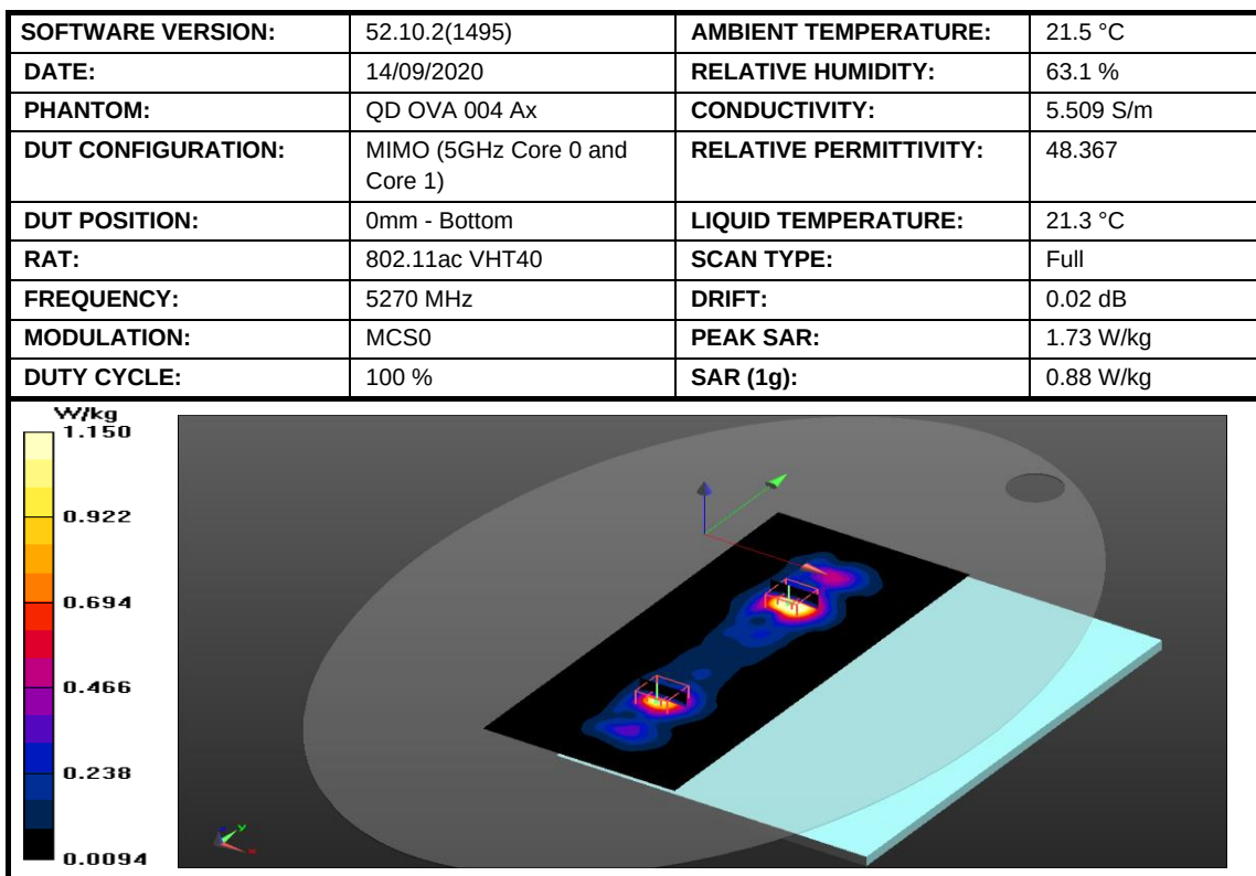
Figure 17: SAR Body Testing Results for the A2337 at 5270 MHz.
