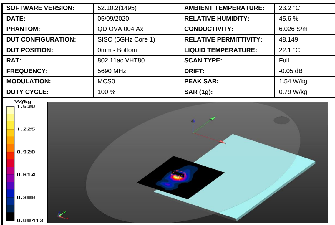
Figure 23: SAR Body Testing Results for the A2337 at 5690 MHz.
