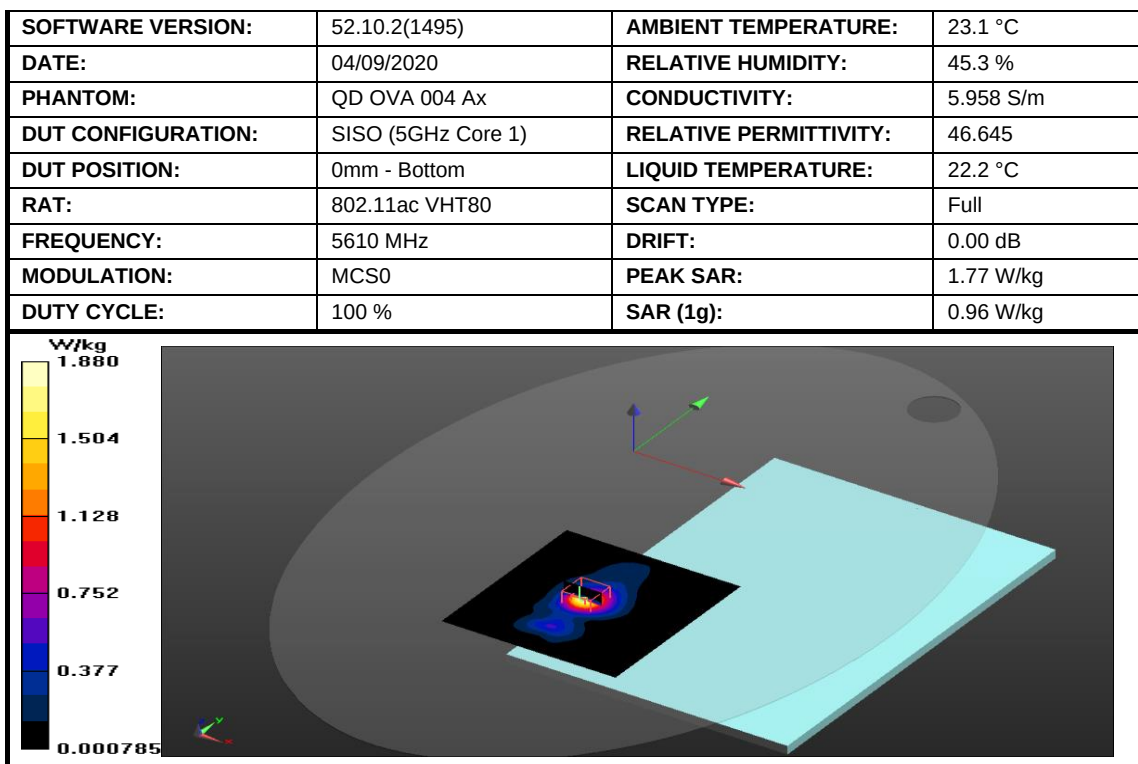
Figure 25: SAR Body Testing Results for the A2337 at 5610 MHz.
