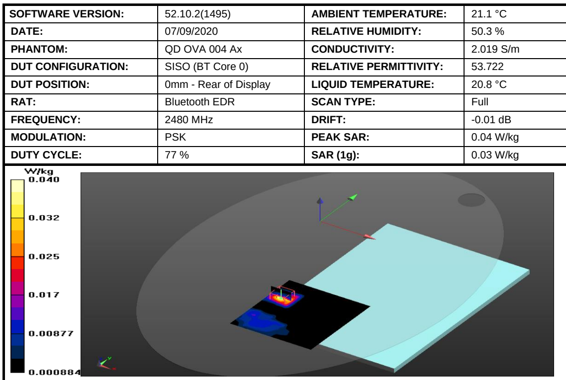
Figure 4: SAR Body Testing Results for the A2337 at 2480 MHz.
