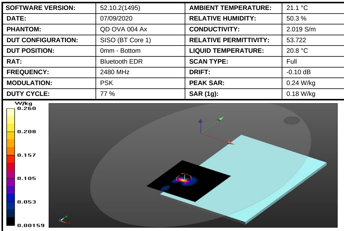
Figure 5: SAR Body Testing Results for the A2337 at 2480 MHz.
