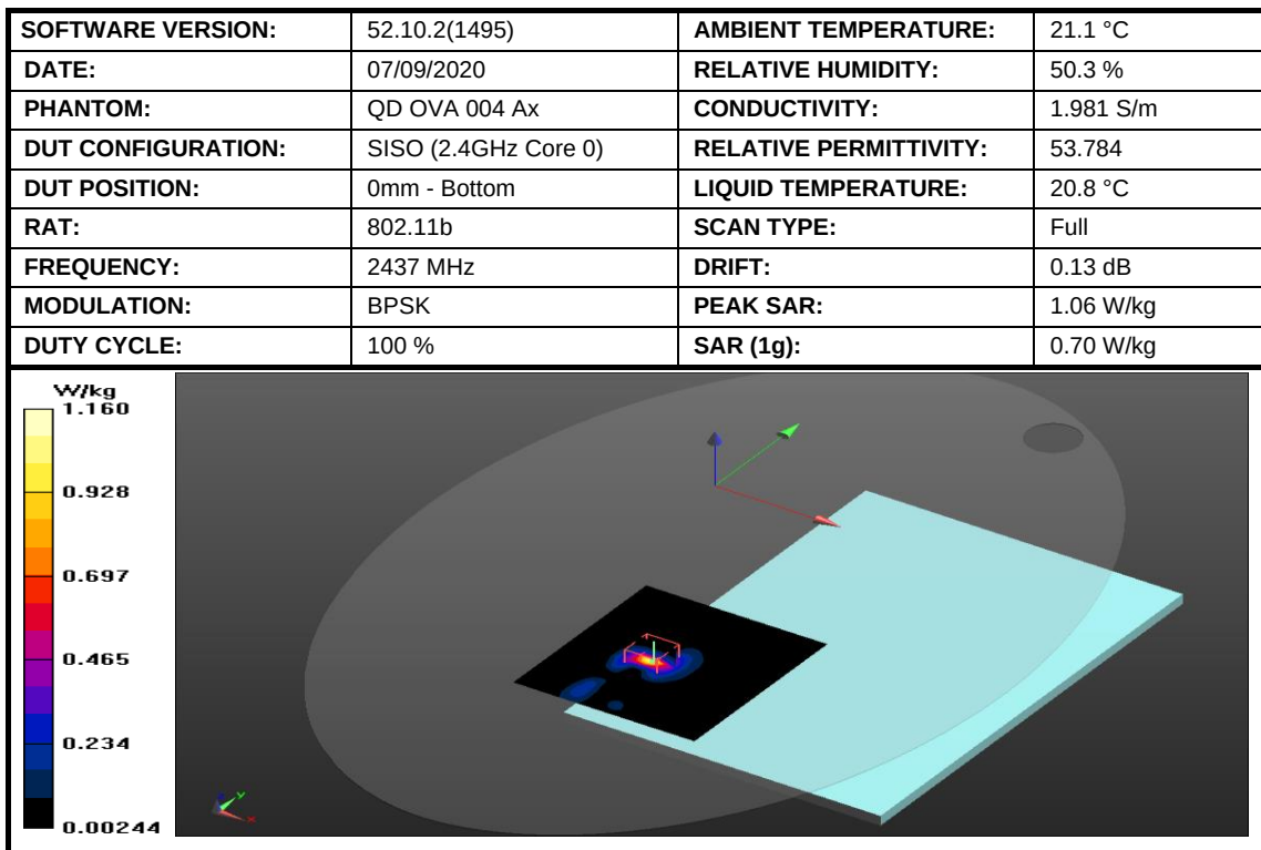
Figure 7: SAR Body Testing Results for the A2337 at 2437 MHz.
