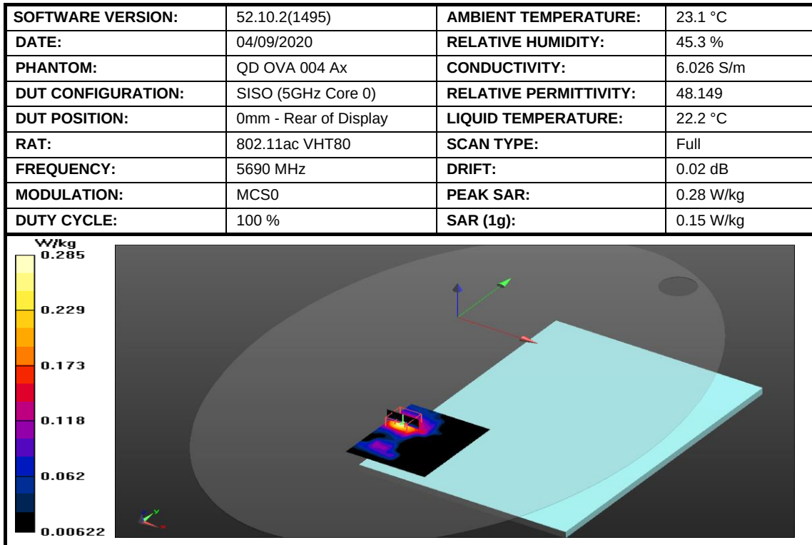
Figure 20: SAR Body Testing Results for the A2337 at 5690 MHz.
