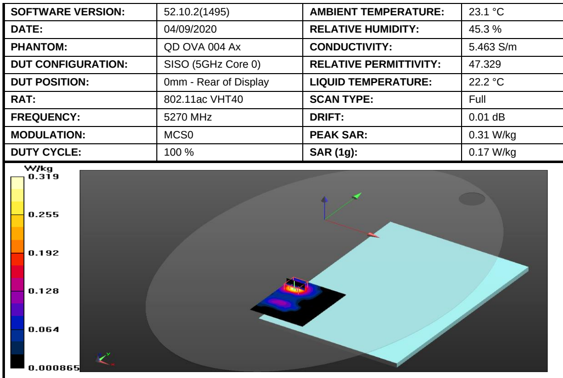
Figure 13: SAR Body Testing Results for the A2337 at 5270 MHz.
