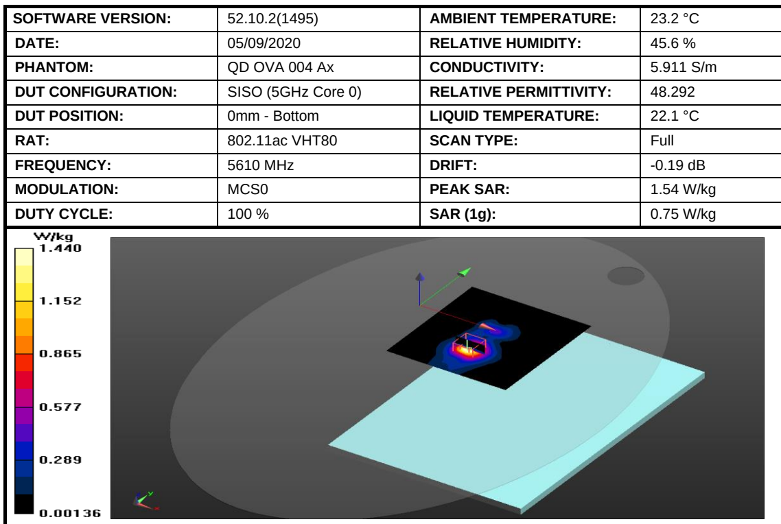
Figure 21: SAR Body Testing Results for the A2337 at 5610 MHz.
