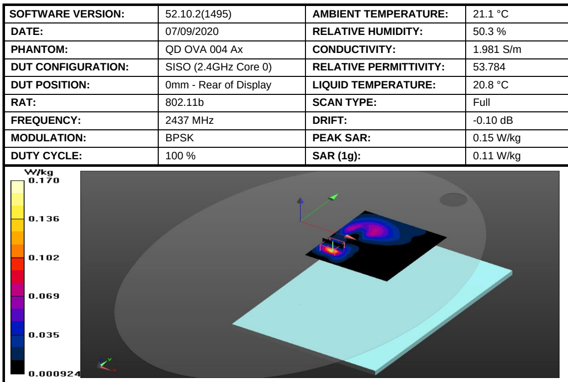
Figure 8: SAR Body Testing Results for the A2337 at 2437 MHz.
