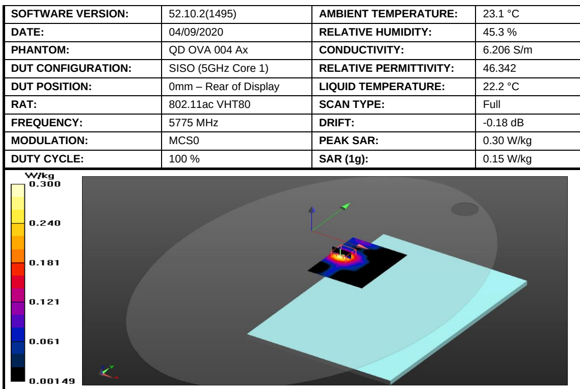
Figure 33: SAR Body Testing Results for the A2337 at 5775 MHz.
