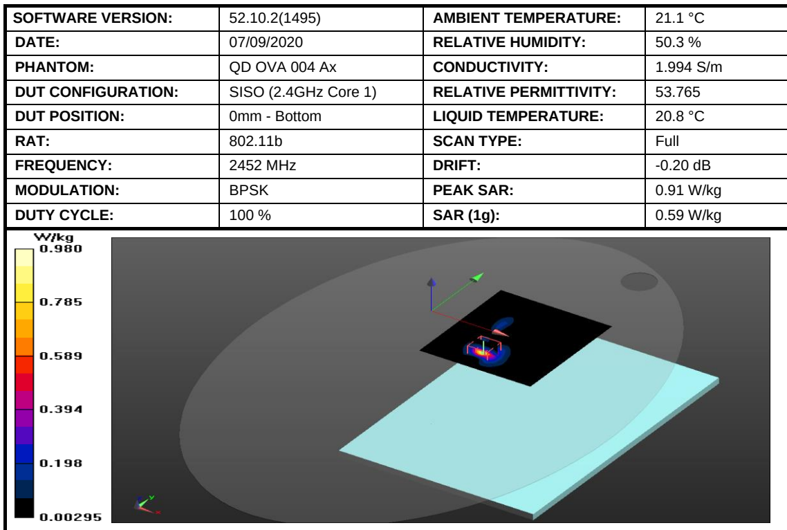
Figure 9: SAR Body Testing Results for the A2337 at 2452 MHz.
