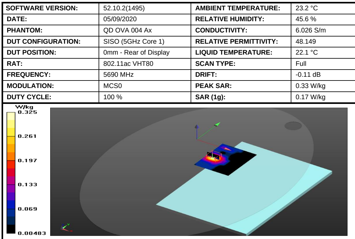
Figure 24: SAR Body Testing Results for the A2337 at 5690 MHz.
