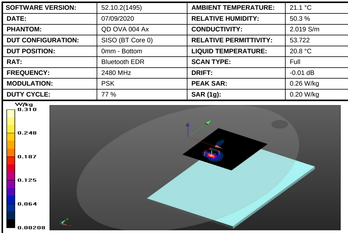
Figure 3: SAR Body Testing Results for the A2337 at 2480 MHz.
