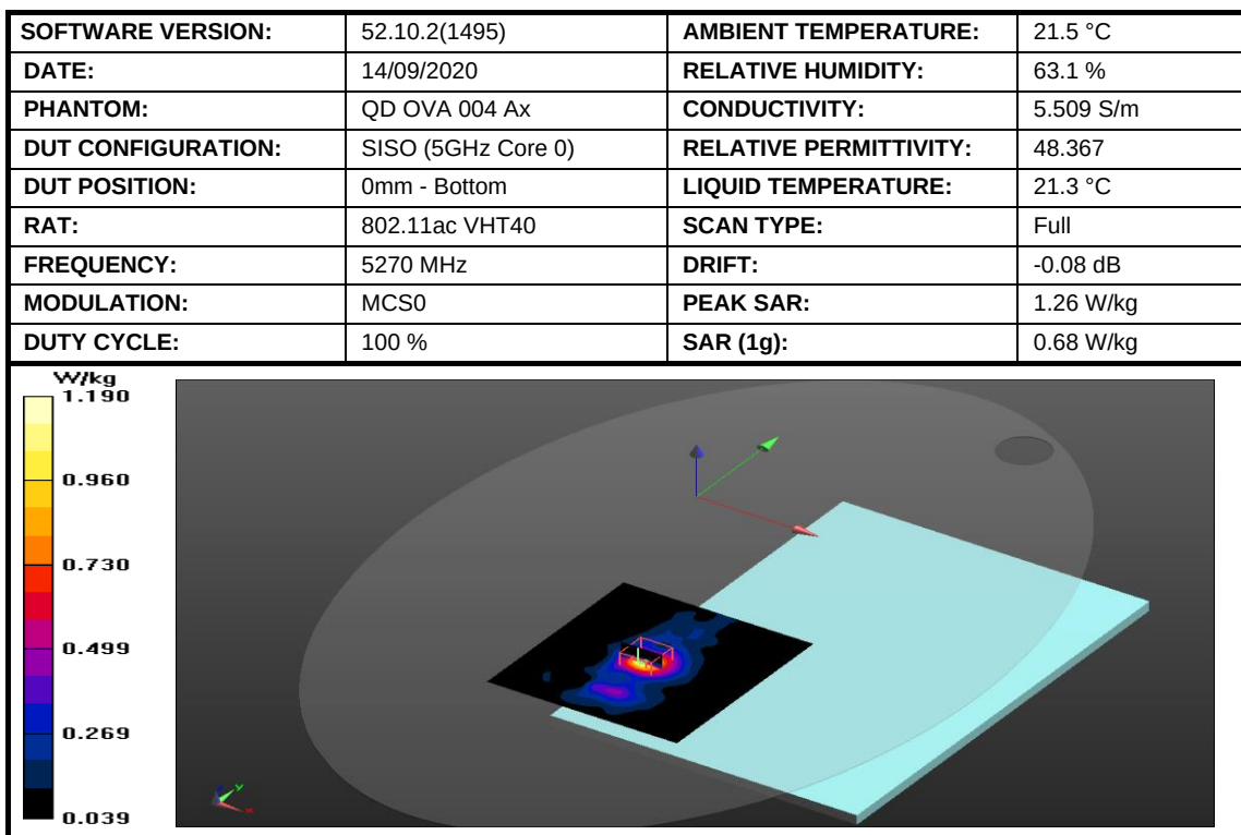
Figure 15: SAR Body Testing Results for the A2337 at 5270 MHz.
