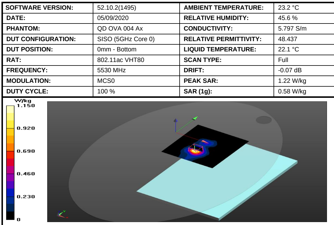
Figure 22: SAR Body Testing Results for the A2337 at 5530 MHz.
