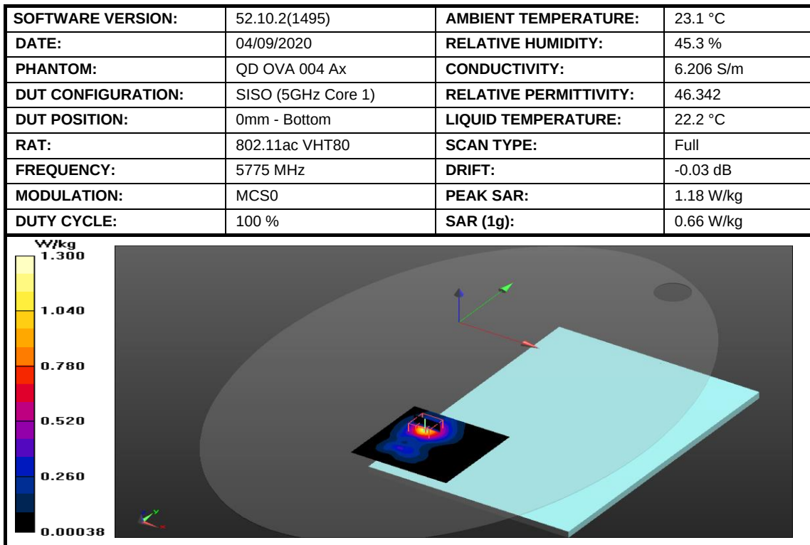
Figure 32: SAR Body Testing Results for the A2337 at 5775 MHz.
