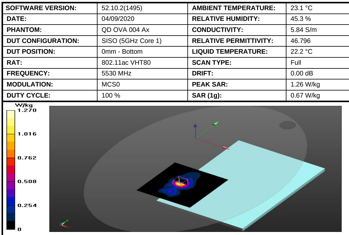
Figure 26: SAR Body Testing Results for the A2337 at 5530 MHz.
