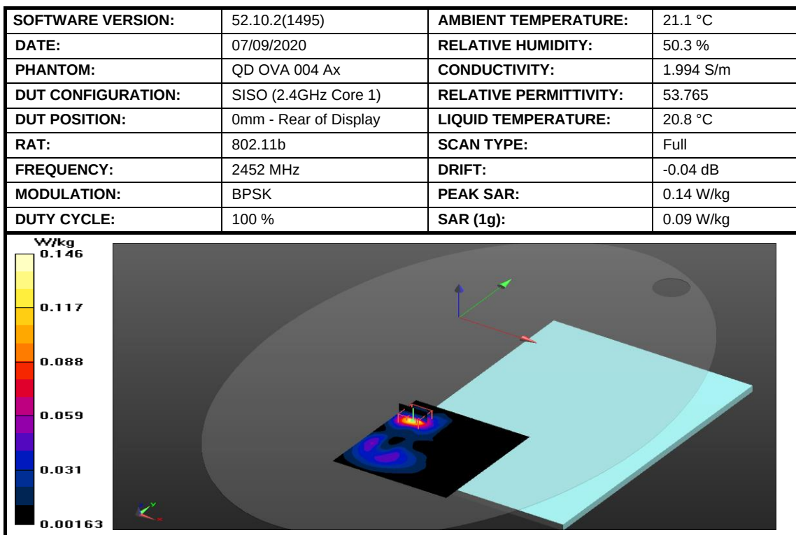
Figure 10: SAR Body Testing Results for the A2337 at 2452 MHz.
