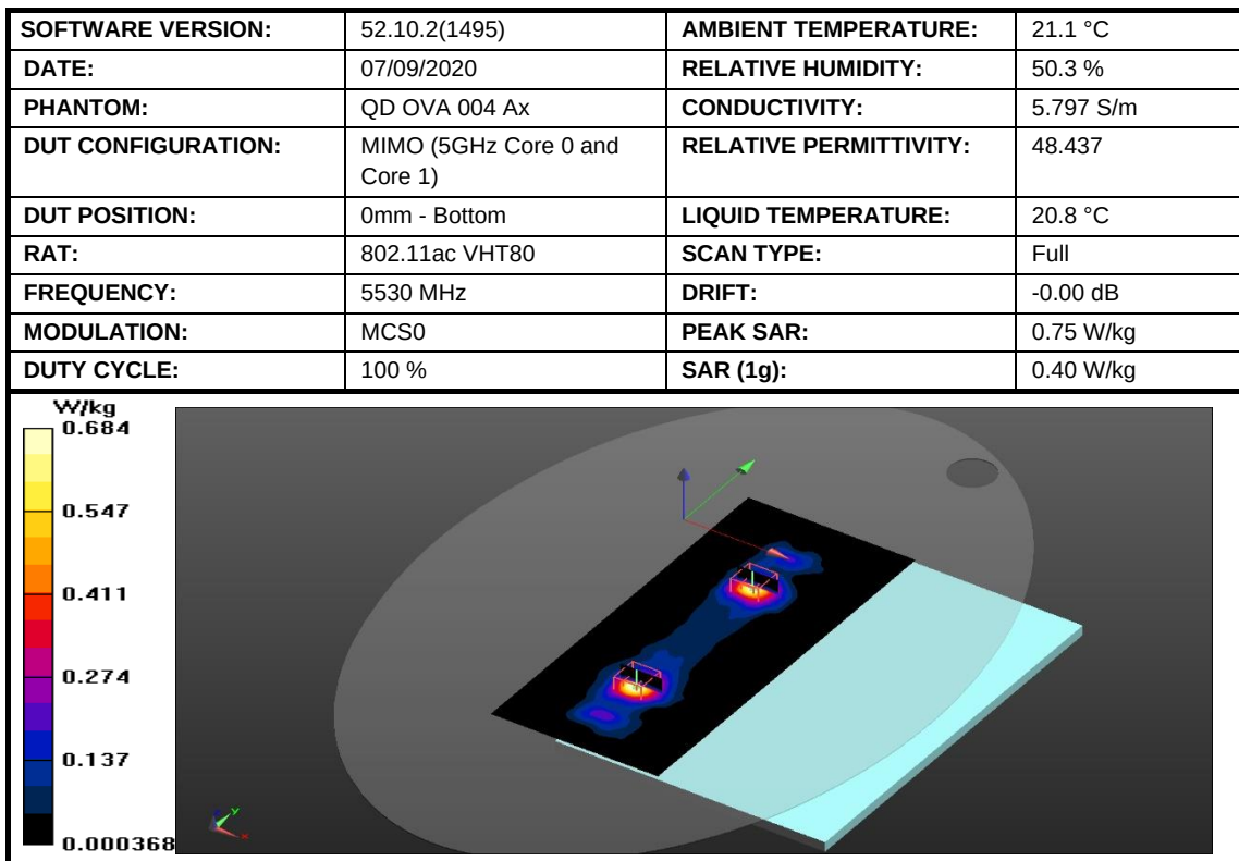
Figure 29: SAR Body Testing Results for the A2337 at 5530 MHz.
