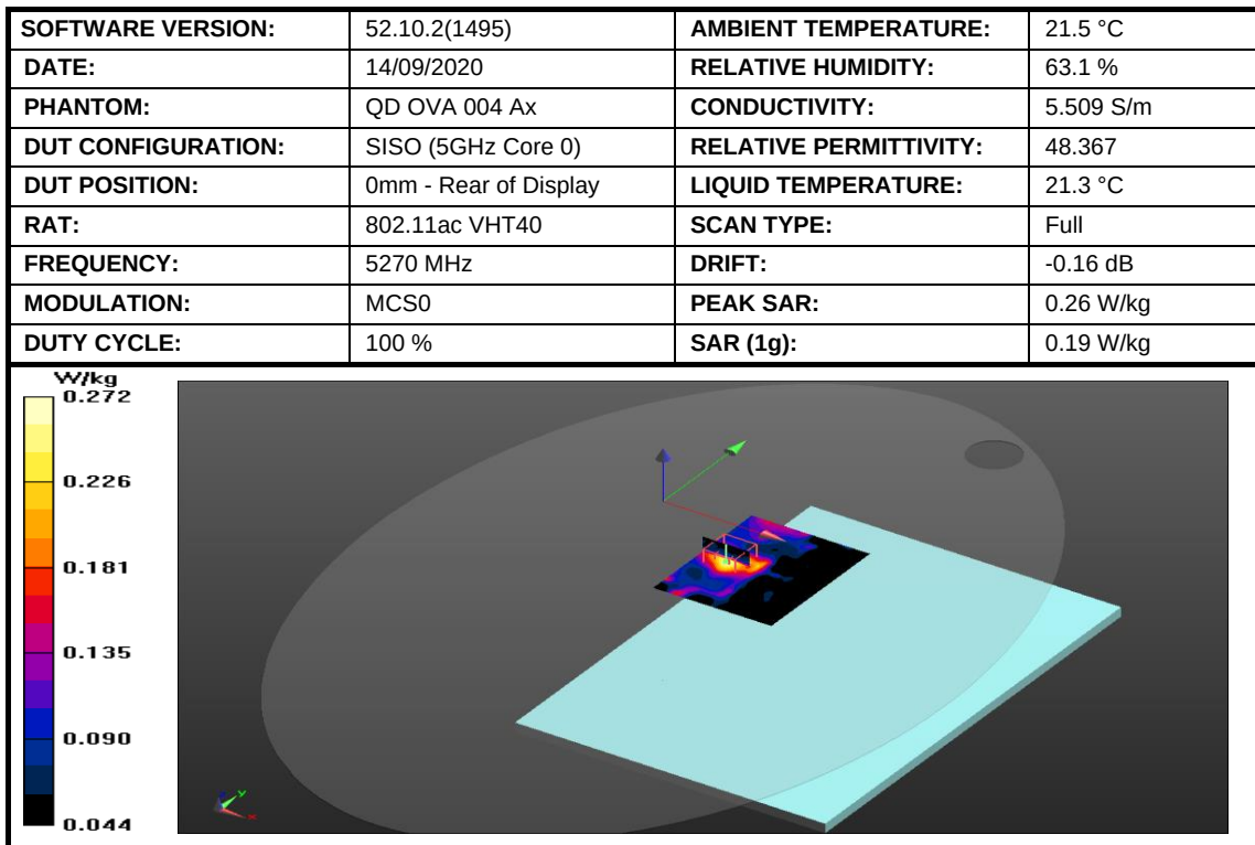
Figure 16: SAR Body Testing Results for the A2337 at 5270 MHz.
