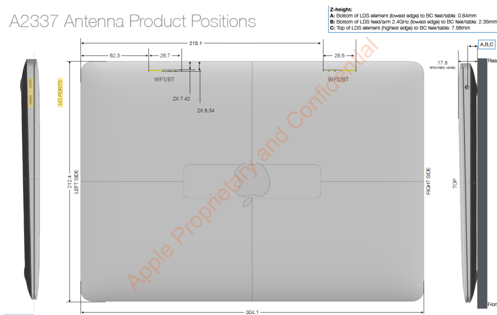
Figure 1 Antenna Location Diagram
