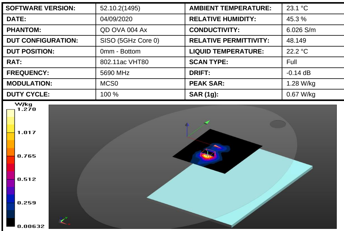
Figure 19: SAR Body Testing Results for the A2337 at 5690 MHz.
