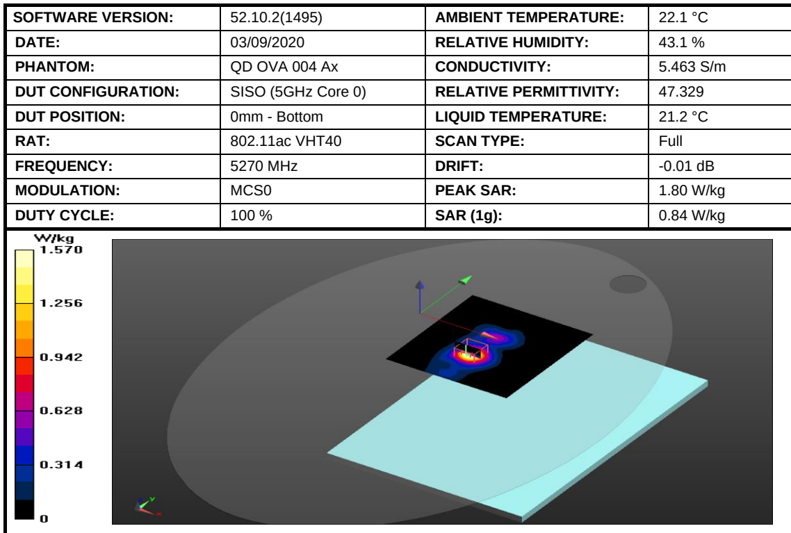
Figure 12: SAR Body Testing Results for the A2337 at 5270 MHz.
