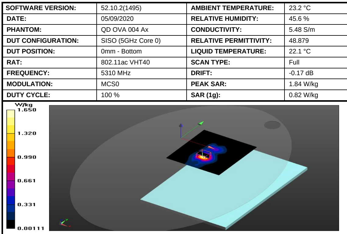
Figure 14: SAR Body Testing Results for the A2337 at 5310 MHz
