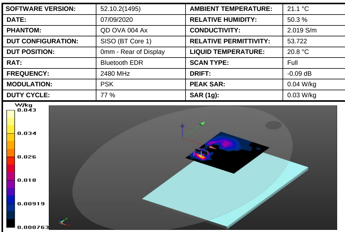
Figure 6: SAR Body Testing Results for the A2337 at 2480 MHz.
