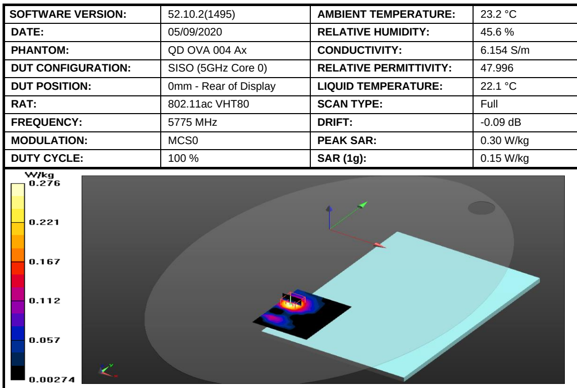
Figure 31: SAR Body Testing Results for the A2337 at 5775 MHz.
