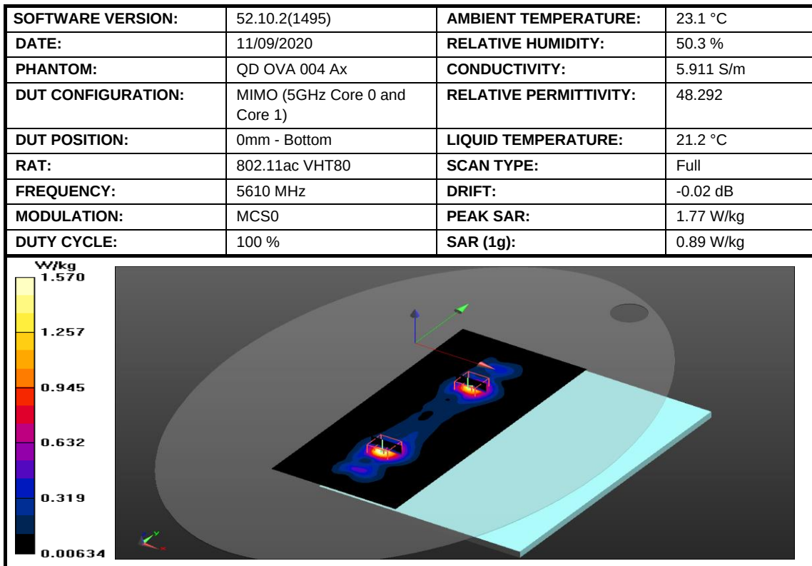
Figure 28: SAR Body Testing Results for the A2337 at 5610 MHz.
