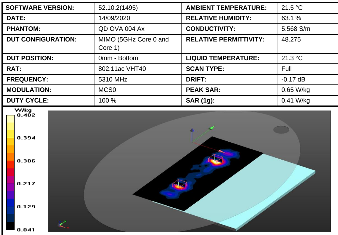
Figure 18: SAR Body Testing Results for the A2337 at 5310 MHz.
