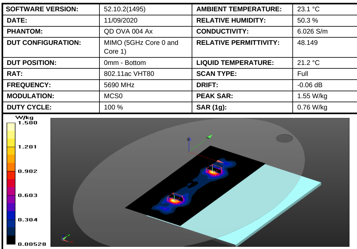
Figure 27: SAR Body Testing Results for the A2337 at 5690 MHz.
