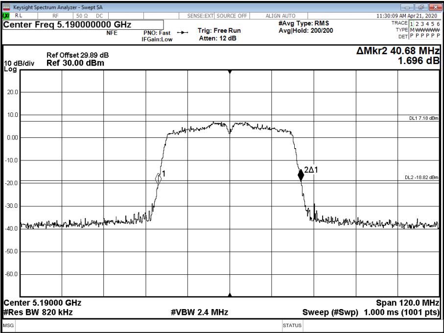
Figure 333 - 5190 MHz - 26 dB Emission Bandwidth
