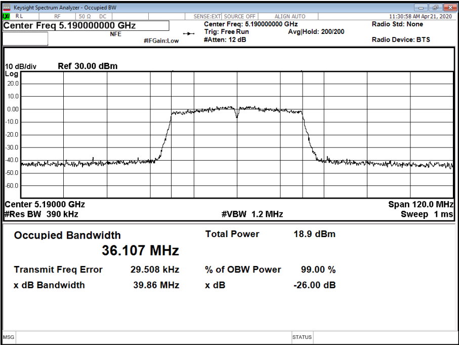
Figure 334 - 5190 MHz - 99% Occupied Bandwidth
