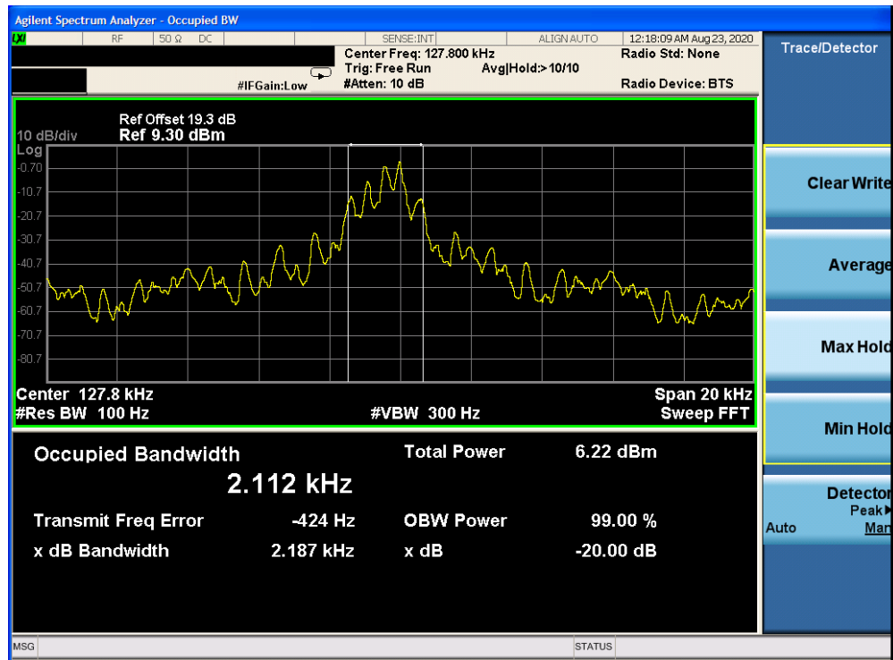
Plot 6-1. Occupied Bandwidth Plot (Charging Rate 10C)
