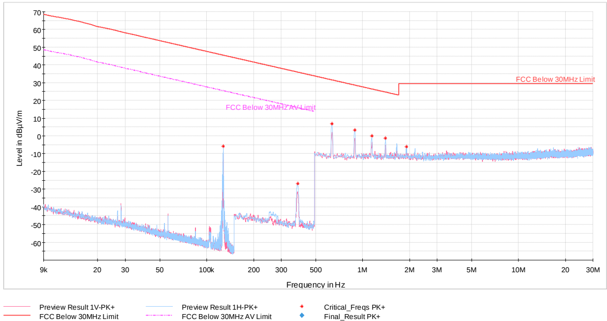
Plot 6-3. Radiated Spurious Emissions 9kHz-30MHz (Charging Rate 10C, with AC/DC Adapter)
