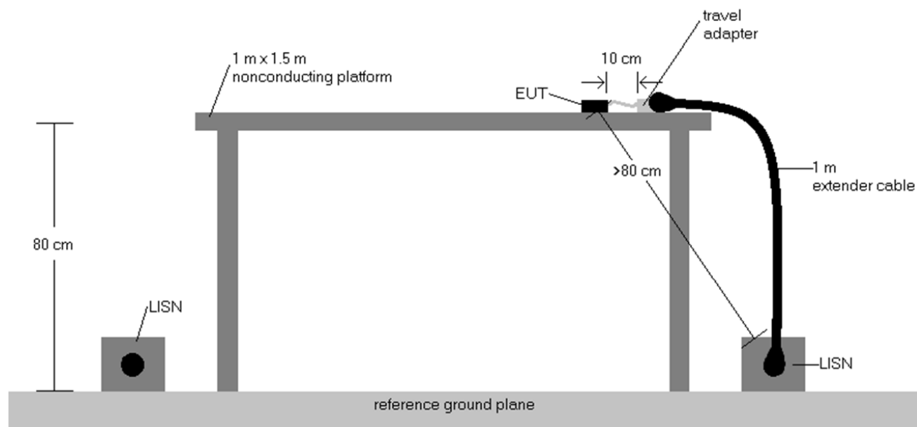
Figure 6-4. Test Instrument & Measurement Setup
