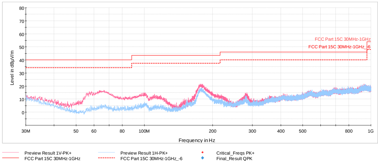
Plot 6-4. Radiated Spurious Emissions 30MHz-1000MHz (Charging Rate 10C, with AC/DC Adapter)
