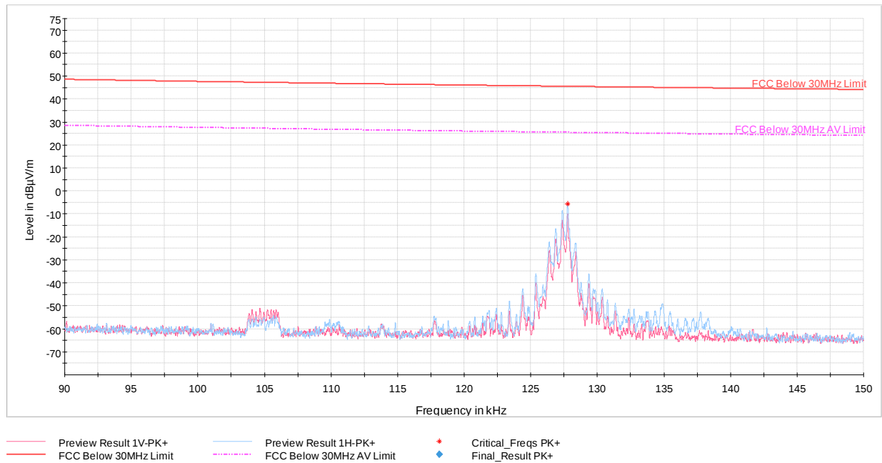
Plot 6-2. Radiated Restricted Lower Band Edge Peak Measurement (Charging Rate 10C)
