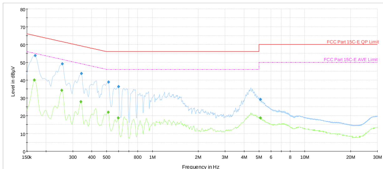
Plot 6-6. AC Line Conducted Plot (N, Charging Rate 10C, with AC/DC Adapter)
