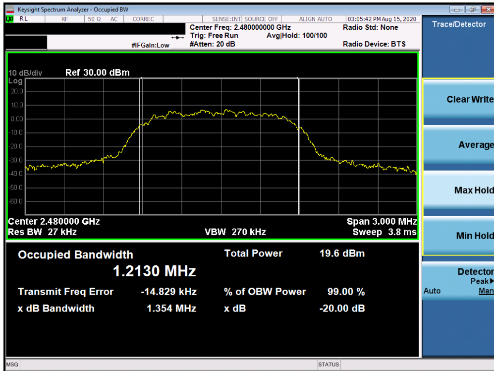
Plot 7-6. 20dB Bandwidth Plot Antenna 3a (Bluetooth, 8DPSK, ePA – Ch. 78)
