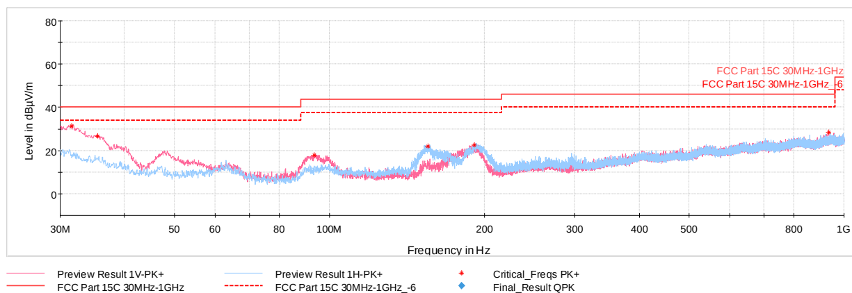
Plot 7-80. Radiated Spurious Emissions below 1GHz TxBF (GFSK ePA – Ch.0, with AC/DC Adapter)
