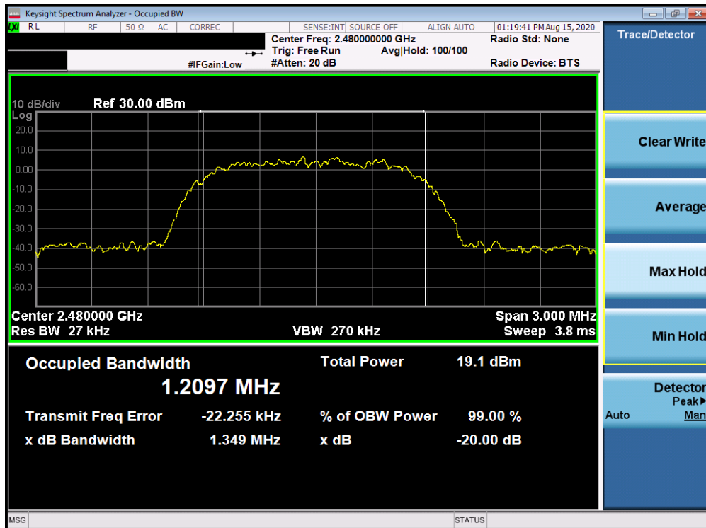
Plot 7-12. 20dB Bandwidth Plot Antenna 1a (Bluetooth, 8DPSK, ePA – Ch. 78)
