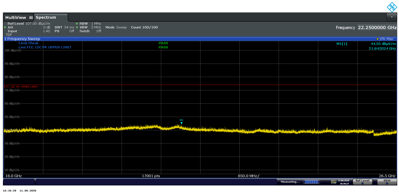
Plot 7-67. Radiated Spurious Emissions above 18GHz TxBF (GFSK ePA – Ch.0, Pol. V)
