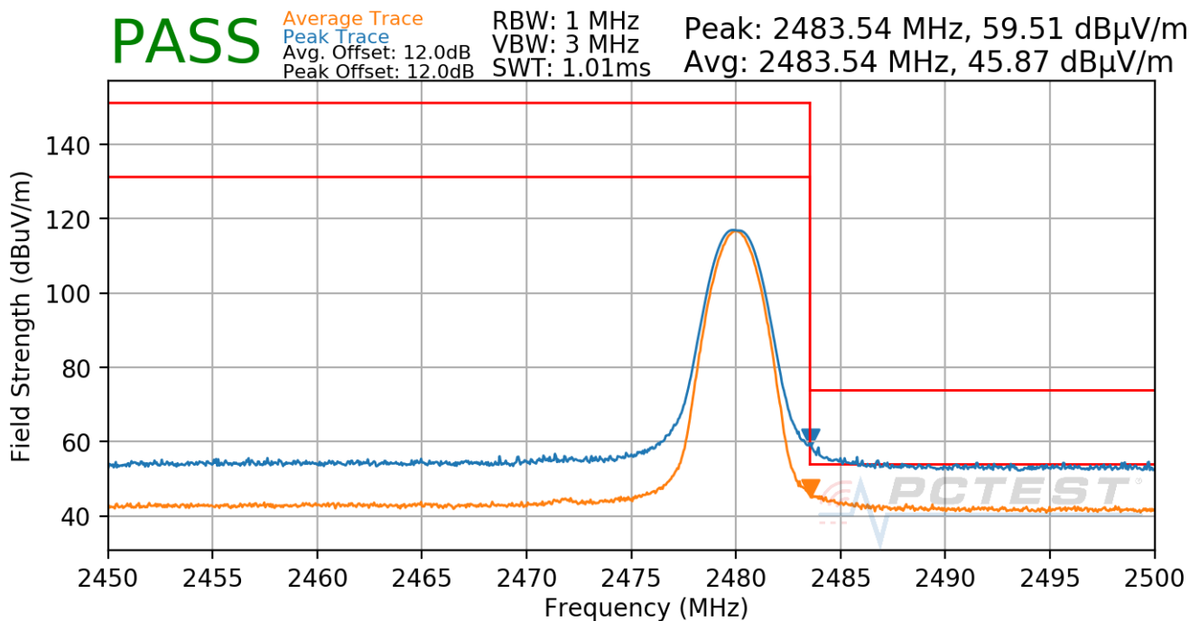
Plot 7-70. Radiated Restricted Upper Band Edge Measurement Antenna 3a (Average & Peak)
