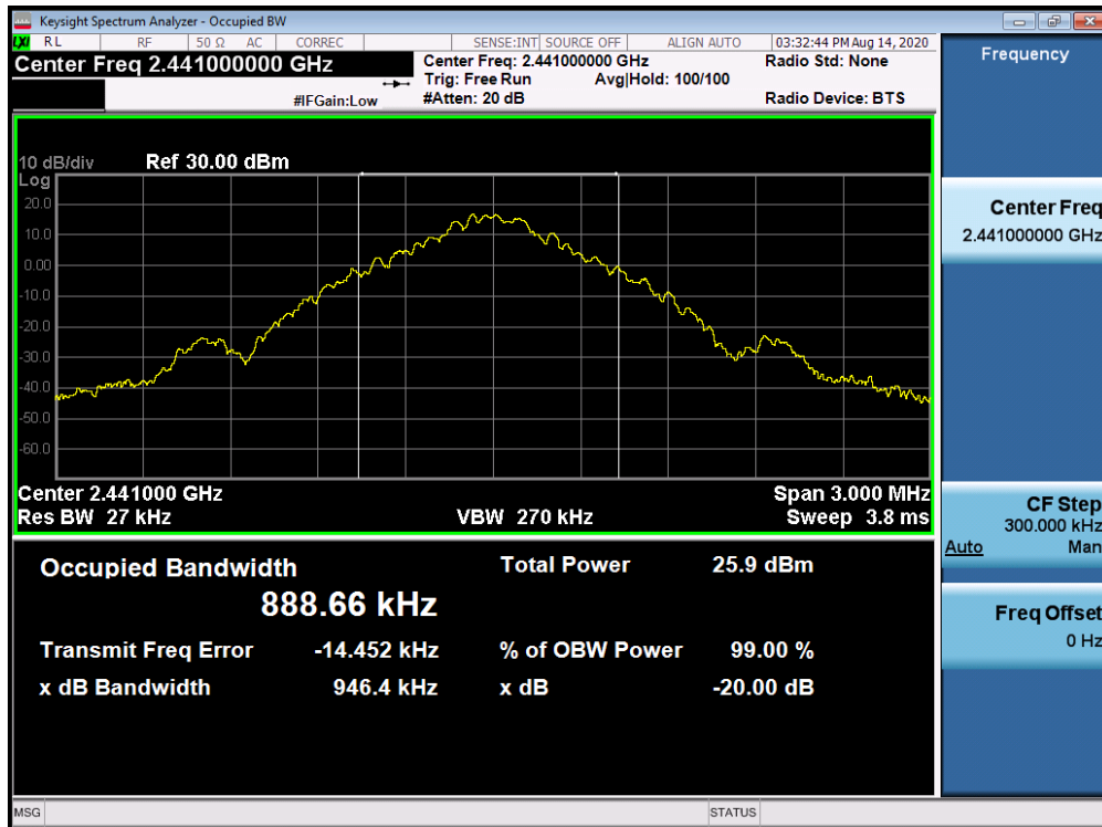
Plot 7-2. 20dB Bandwidth Plot Antenna 3a (Bluetooth, GFSK, ePA – Ch. 39)
