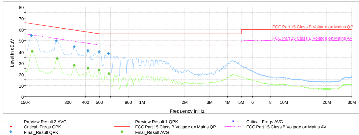
Plot 7-82. AC Line-Conducted Test Plot TxBF (N, GFSK ePA – Ch.0, with AC/DC Adapter)
