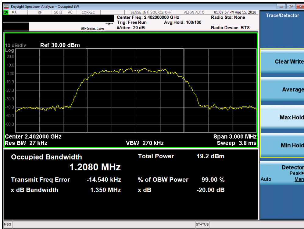
Plot 7-10. 20dB Bandwidth Plot Antenna 1a (Bluetooth, 8DPSK, ePA – Ch. 0)
