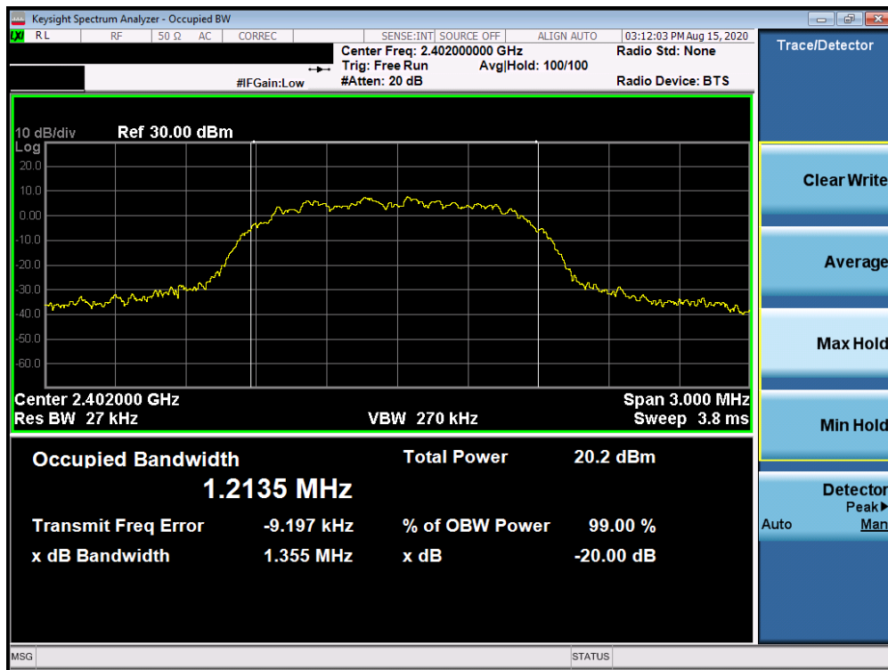
Plot 7-4. 20dB Bandwidth Plot Antenna 3a (Bluetooth, 8DPSK, ePA – Ch. 0)
