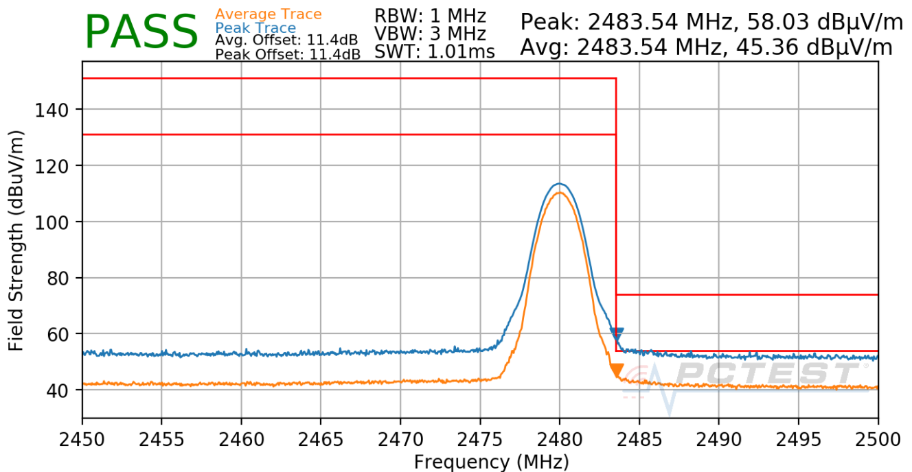
Plot 7-75. Radiated Restricted Upper Band Edge Measurement Antenna 1a (Average & Peak)
