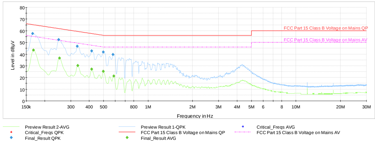
Plot 7-81. AC Line-Conducted Test Plot TxBF (L1, GFSK ePA – Ch.0, with AC/DC Adapter)
