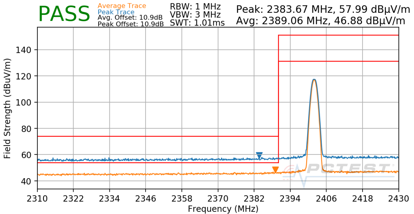
Plot 7-72. Radiated Restricted Lower Band Edge Measurement Antenna 1a (Average & Peak)
