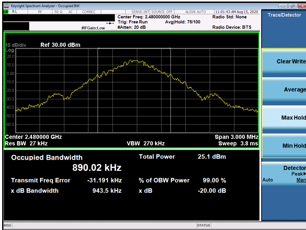
Plot 7-3. 20dB Bandwidth Plot Antenna 3a (Bluetooth, GFSK, ePA – Ch. 78)
