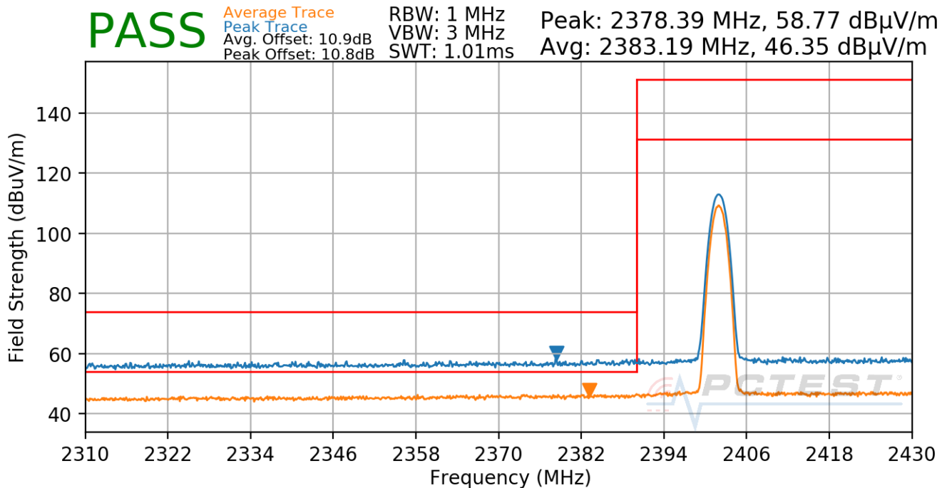
Plot 7-73. Radiated Restricted Lower Band Edge Measurement Antenna 1a (Average & Peak)
