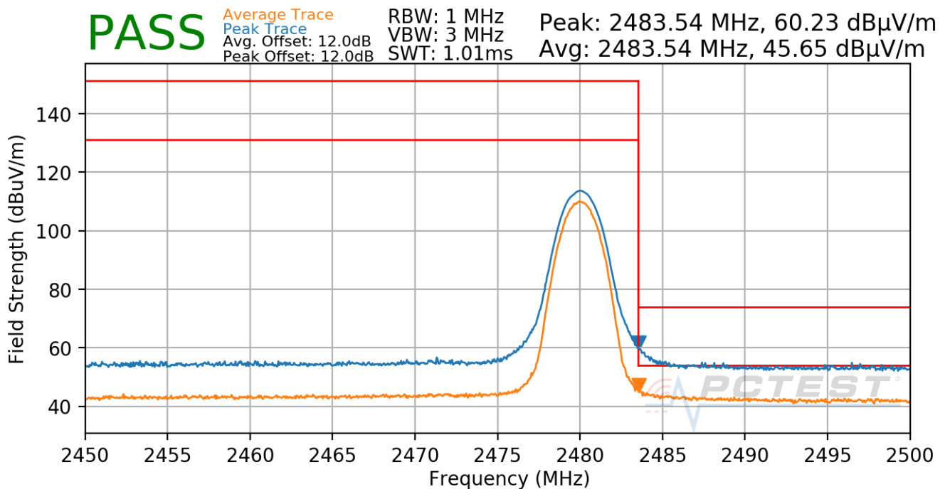
Plot 7-71. Radiated Restricted Upper Band Edge Measurement Antenna 3a (Average & Peak)
