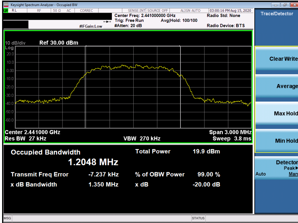
Plot 7-5. 20dB Bandwidth Plot Antenna 3a (Bluetooth, 8DPSK, ePA – Ch. 39)
