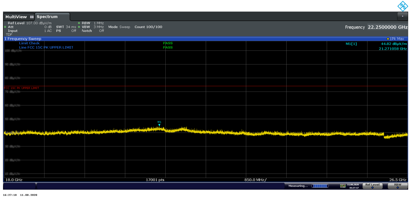
Plot 7-66. Radiated Spurious Emissions above 18GHz TxBF (GFSK ePA – Ch.0, Pol. H)
