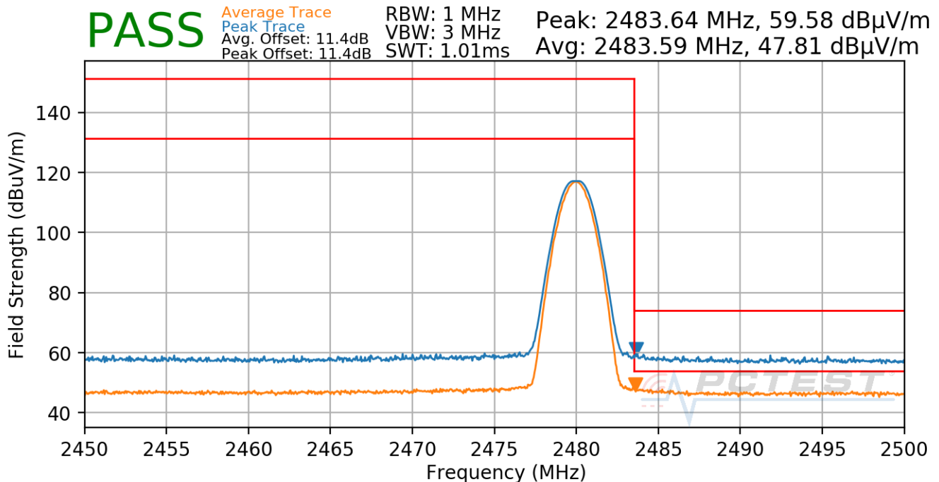
Plot 7-74. Radiated Restricted Upper Band Edge Measurement Antenna 1a (Average & Peak)
