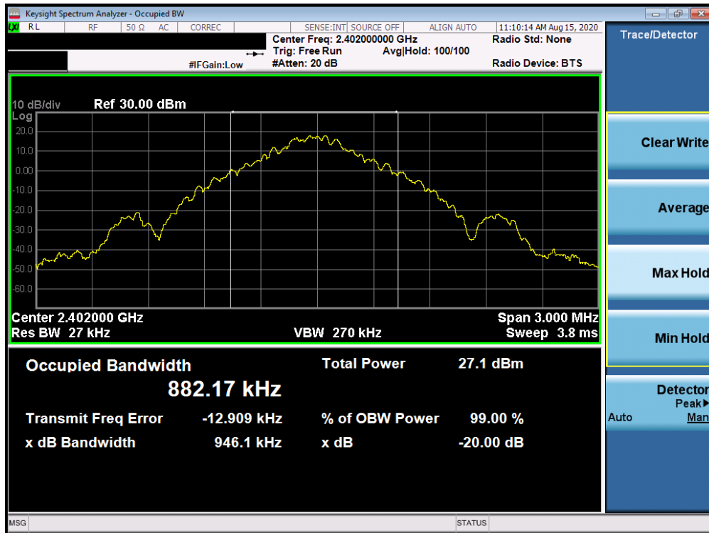
Plot 7-7. 20dB Bandwidth Plot Antenna 1a (Bluetooth, GFSK, ePA – Ch. 0)
