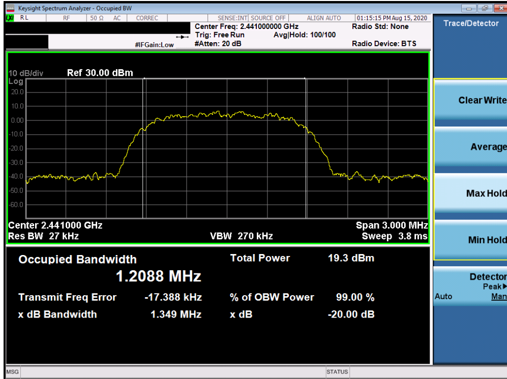
Plot 7-11. 20dB Bandwidth Plot Antenna 1a (Bluetooth, 8DPSK, ePA – Ch. 39)
