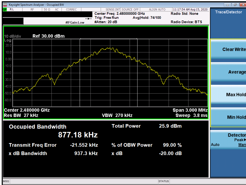
Plot 7-9. 20dB Bandwidth Plot Antenna 1a (Bluetooth, GFSK, ePA – Ch. 78)
