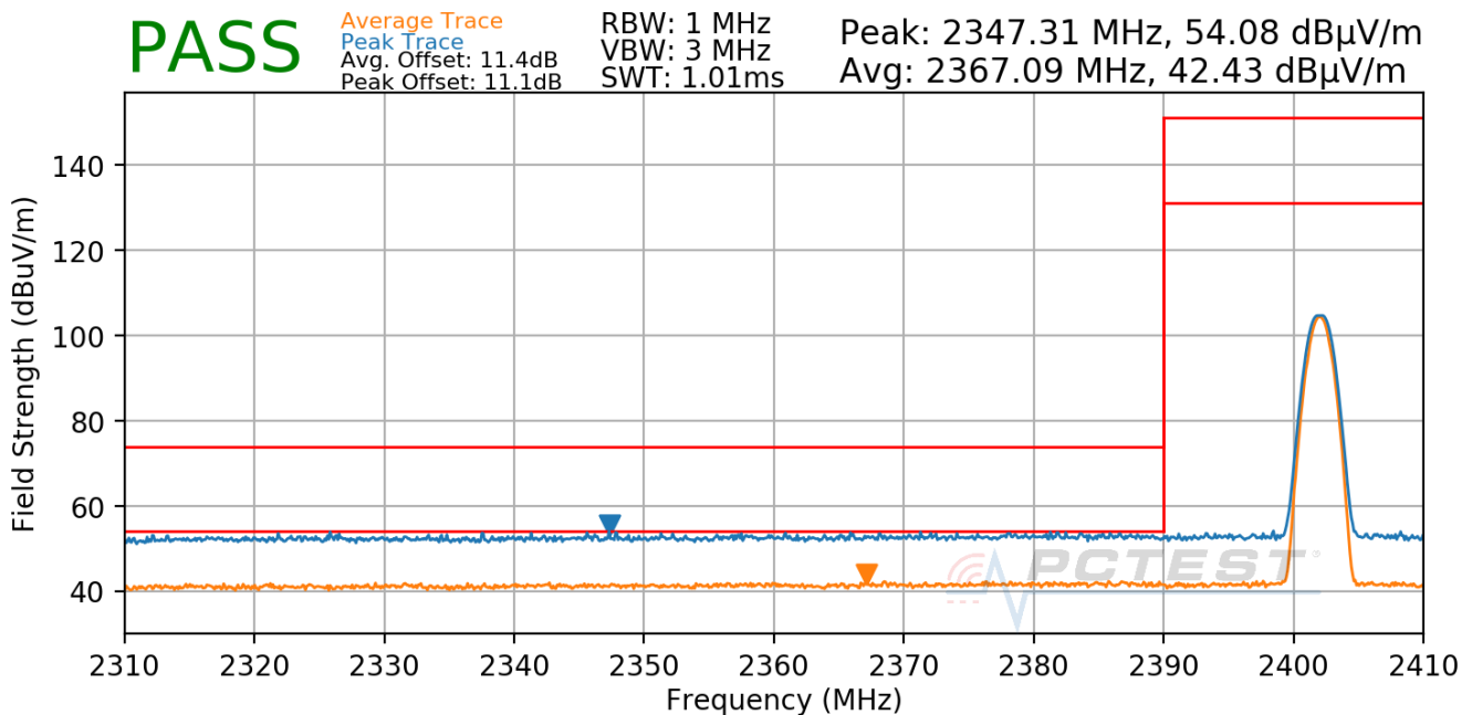
Plot 7-68. Radiated Restricted Lower Band Edge Measurement Antenna 3a (Average & Peak)
