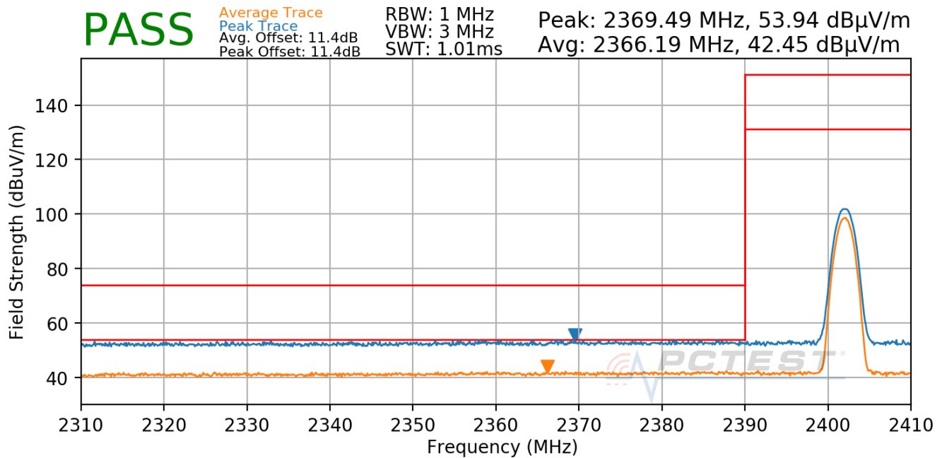
Plot 7-69. Radiated Restricted Lower Band Edge Measurement Antenna 3a (Average & Peak)
