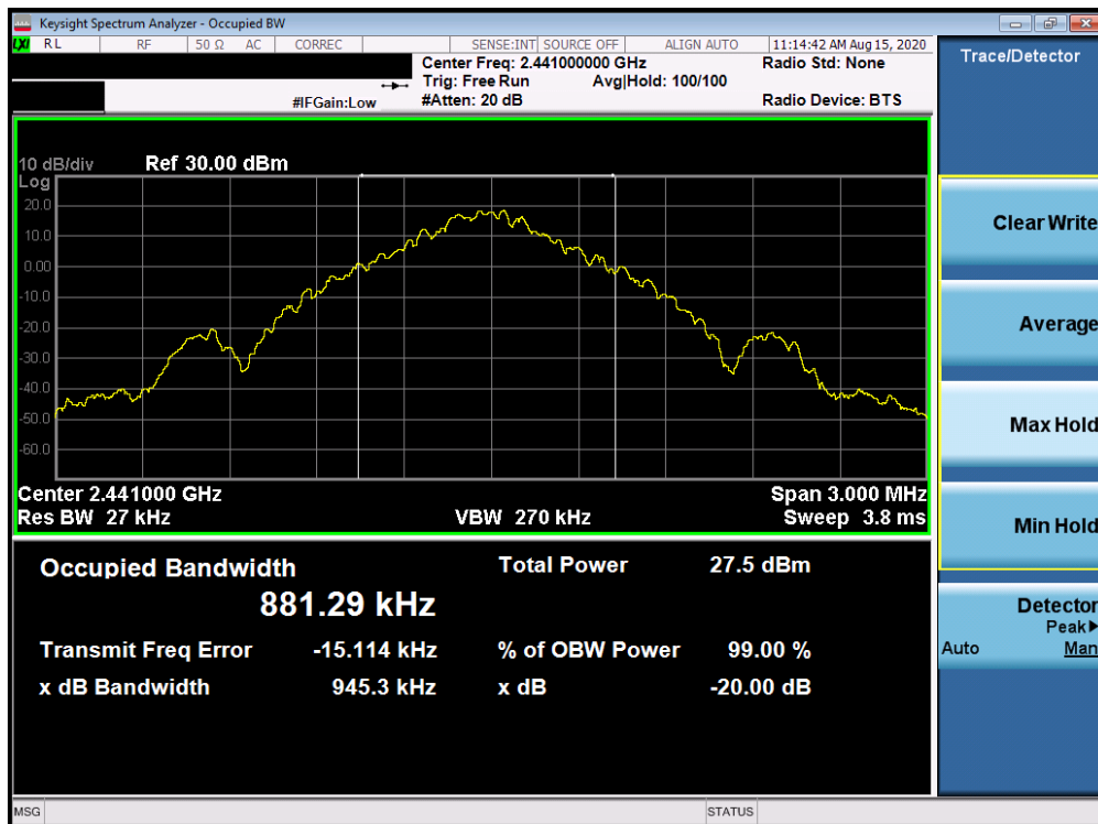
Plot 7-8. 20dB Bandwidth Plot Antenna 1a (Bluetooth, GFSK, ePA – Ch. 39)
