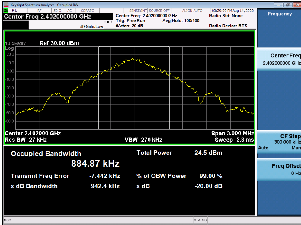
Plot 7-1. 20dB Bandwidth Plot Antenna 3a (Bluetooth, GFSK, ePA – Ch. 0)
