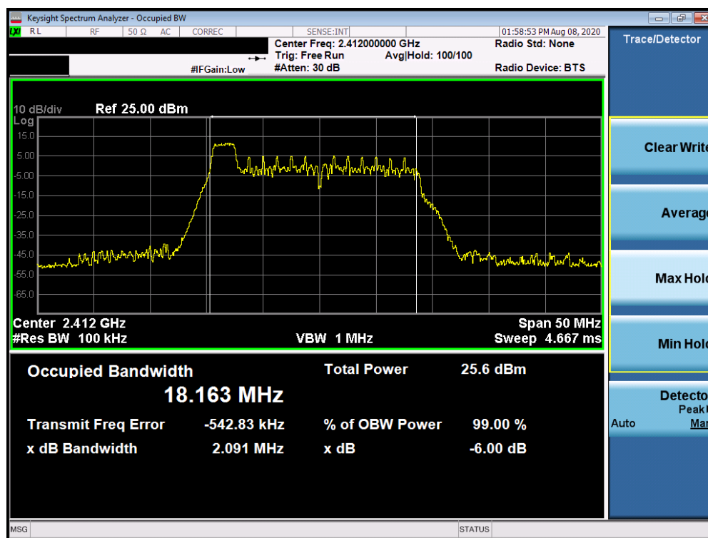
Plot 7-13. 6dB Bandwidth Plot Antenna 1a (802.11ax OFDMA – RU26 Index 0 – Ch. 1)
