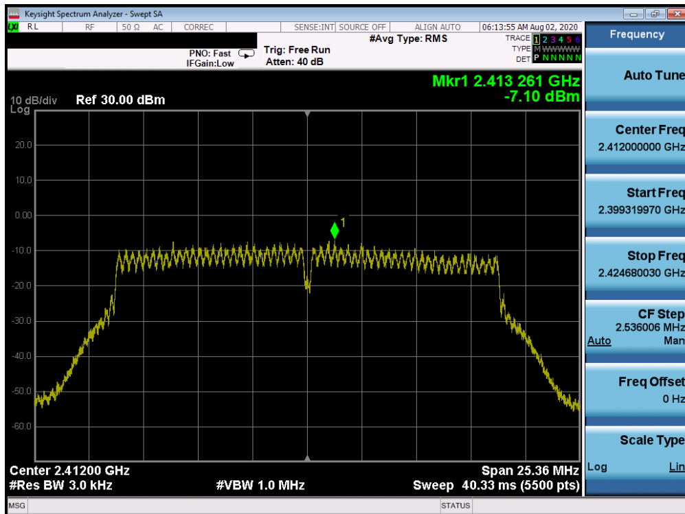
Plot 7-25. Power Spectral Density Plot ANT 3a (802.11n (2.4GHz) – Ch. 1)
