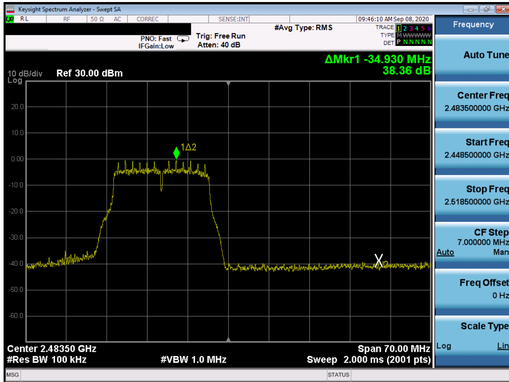
Plot 7-65. Band Edge Plot ANT 3a (802.11g – Ch. 13)
