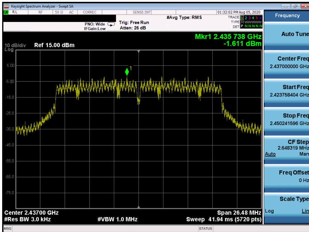
Plot 7-46. Power Spectral Density Plot CDD ANT 1a (802.11n (2.4GHz) – Ch. 6)
