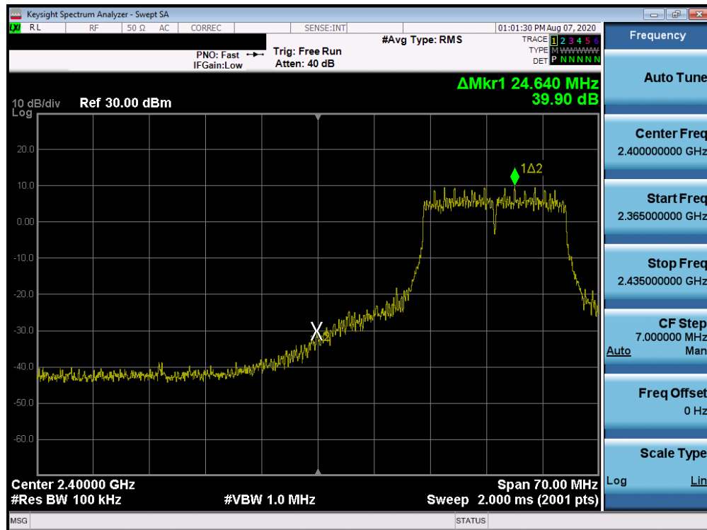
Plot 7-68. Band Edge Plot ANT 3a (802.11n (2.4GHz) – Ch. 3)
