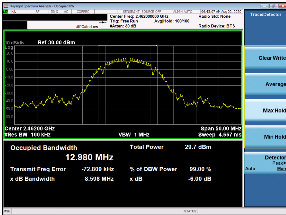
Plot 7-3. 6dB Bandwidth Plot ANT 3a (802.11b – Ch. 11)
