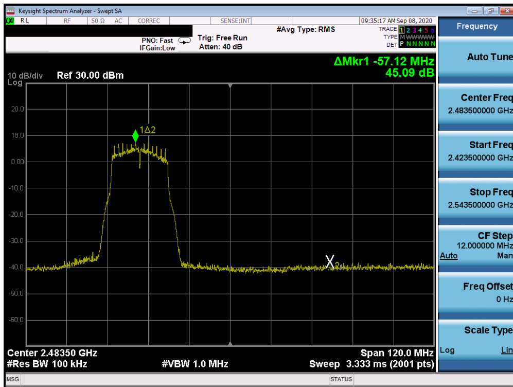
Plot 7-62. Band Edge Plot ANT 3a (802.11g – Ch. 10)
