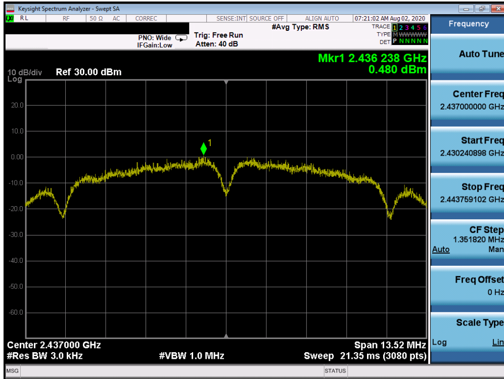
Plot 7-29. Power Spectral Density Plot ANT 1a (802.11b – Ch. 6)
