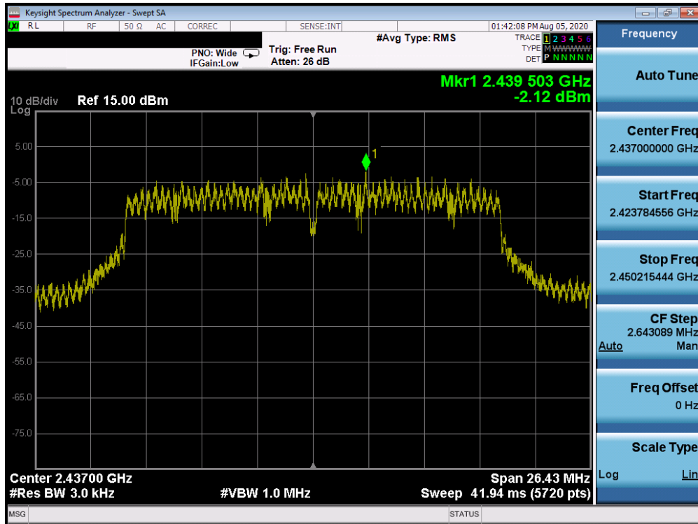
Plot 7-45. Power Spectral Density Plot CDD ANT 3a (802.11n (2.4GHz) – Ch. 6)
