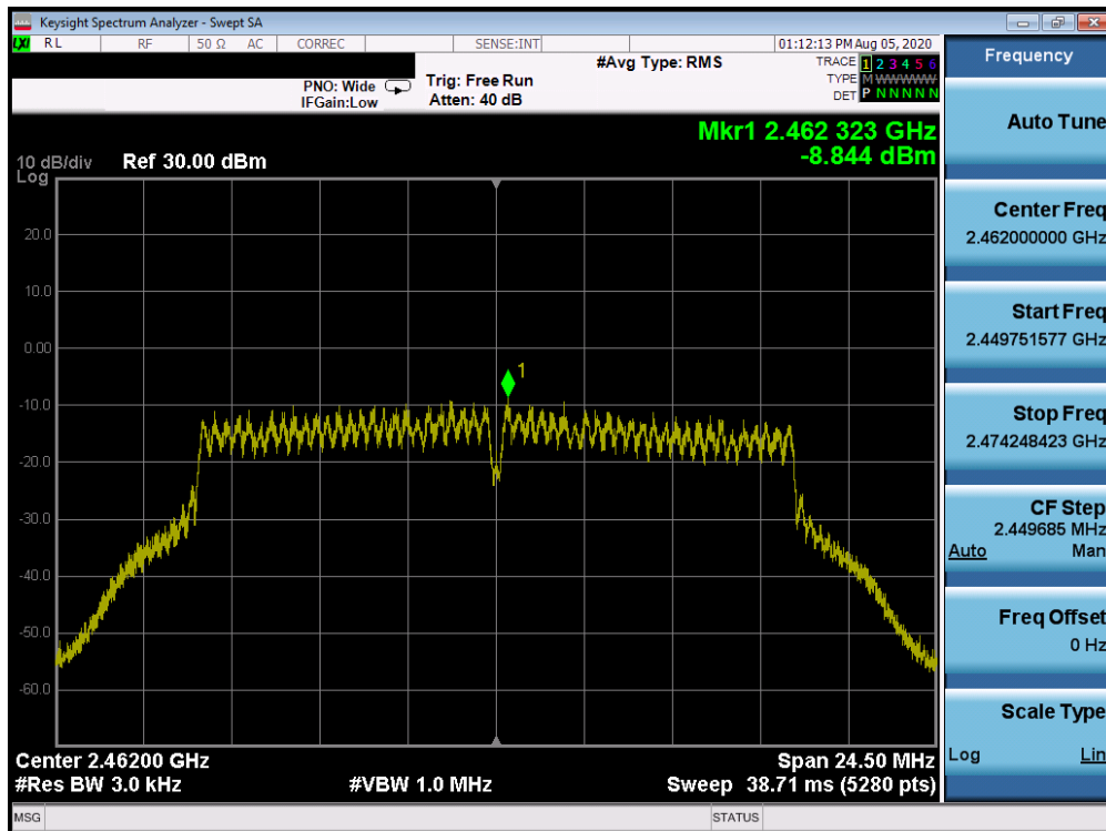
Plot 7-42. Power Spectral Density Plot CDD ANT 1a (802.11g – Ch. 11)
