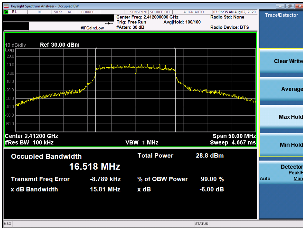
Plot 7-13. 6dB Bandwidth Plot ANT 1a (802.11g – Ch. 1)
