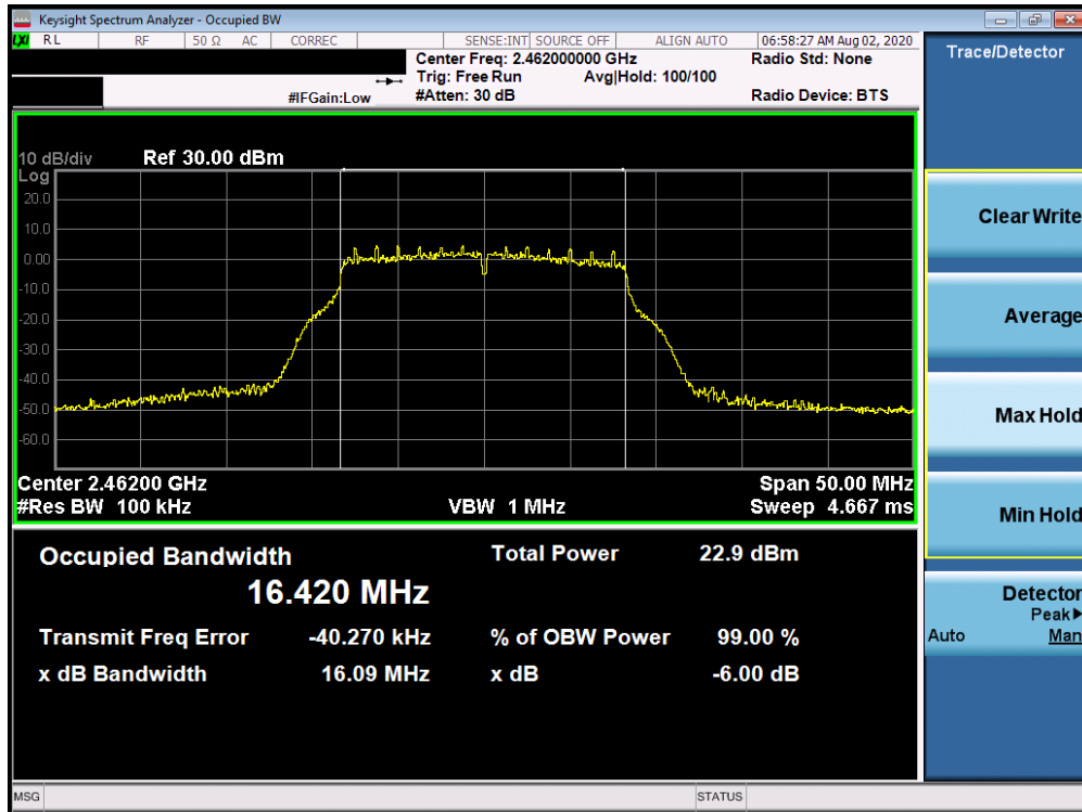
Plot 7-6. 6dB Bandwidth Plot ANT 3a (802.11g – Ch. 11)
