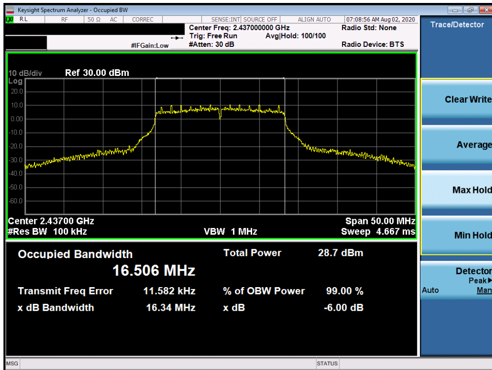
Plot 7-14. 6dB Bandwidth Plot ANT 1a (802.11g – Ch. 6)
