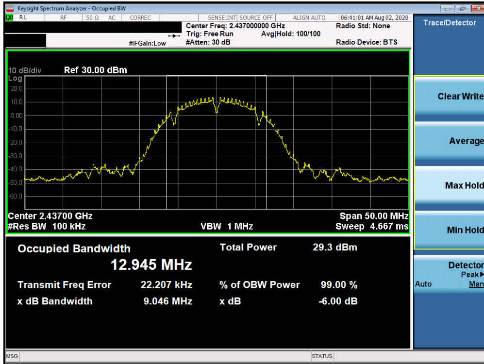
Plot 7-2. 6dB Bandwidth Plot ANT 3a (802.11b – Ch. 6)
