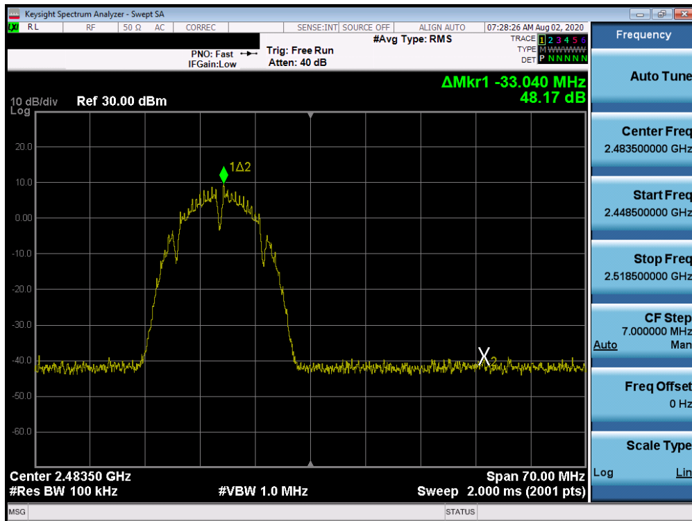
Plot 7-82. Band Edge Plot ANT 1a (802.11b – Ch. 13)
