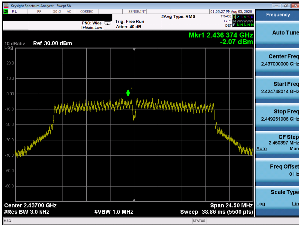
Plot 7-39. Power Spectral Density Plot CDD ANT 3a (802.11g – Ch. 6)
