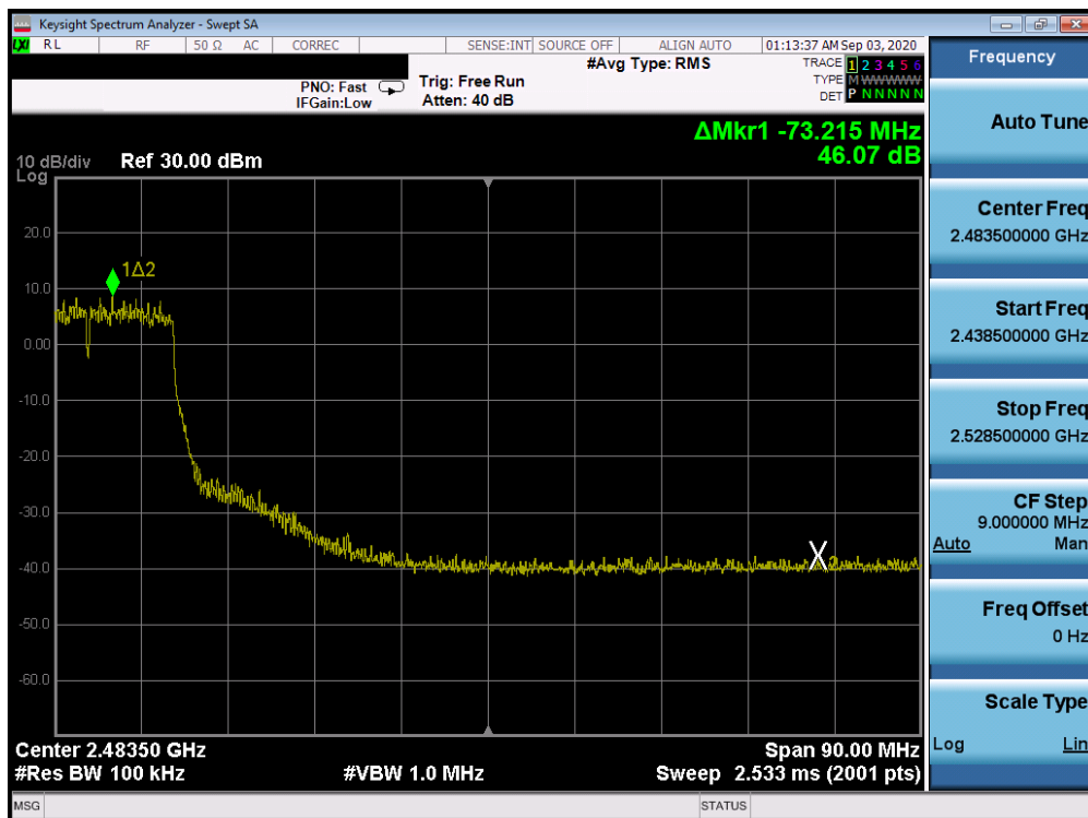
Plot 7-70. Band Edge Plot ANT 3a (802.11n (2.4GHz) – Ch. 7)
