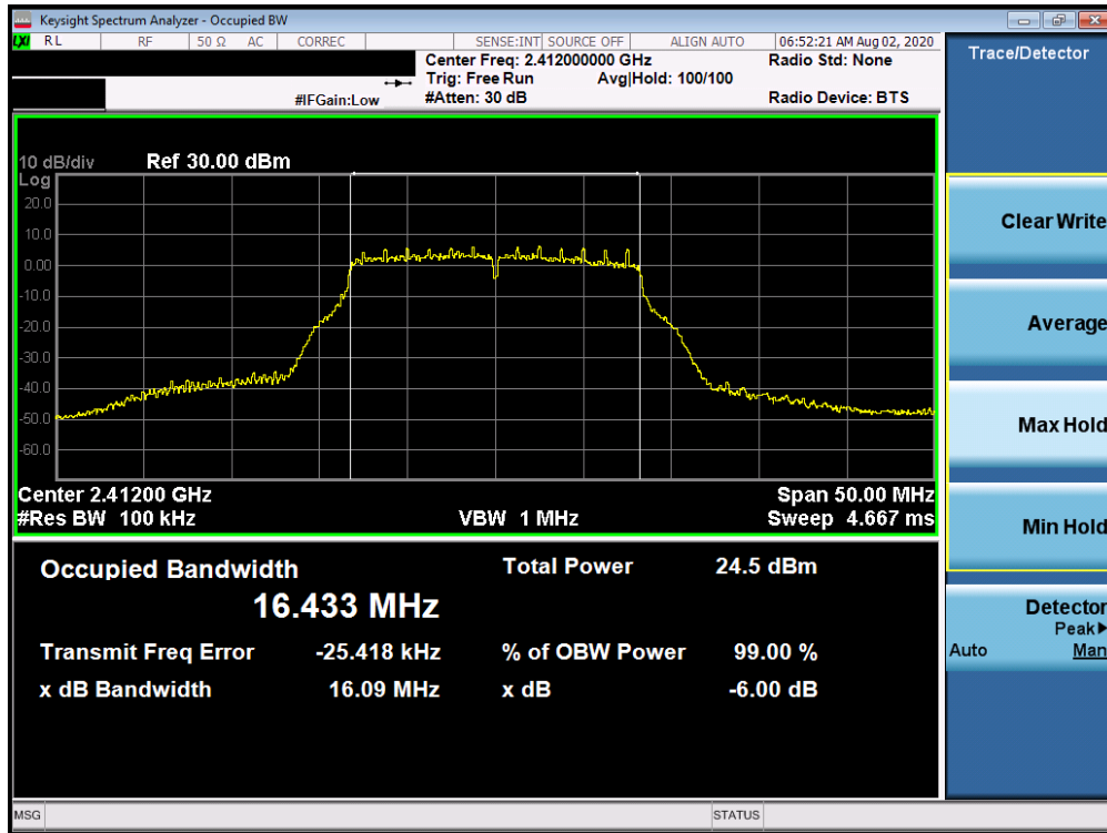
Plot 7-4. 6dB Bandwidth Plot ANT 3a (802.11g – Ch. 1)
