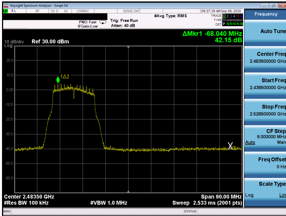
Plot 7-63. Band Edge Plot ANT 3a (802.11g - Ch. 11)
