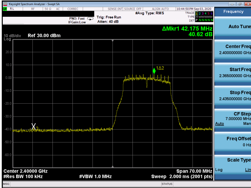
Plot 7-83. Band Edge Plot ANT 1a (802.11g- Ch. 1)
