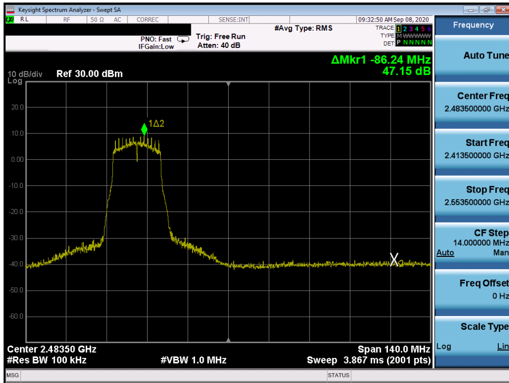
Plot 7-61. Band Edge Plot ANT 3a (802.11g – Ch. 9)
