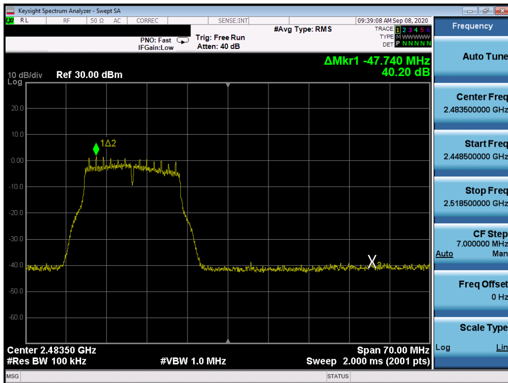
Plot 7-64. Band Edge Plot ANT 3a (802.11g - Ch. 12)
