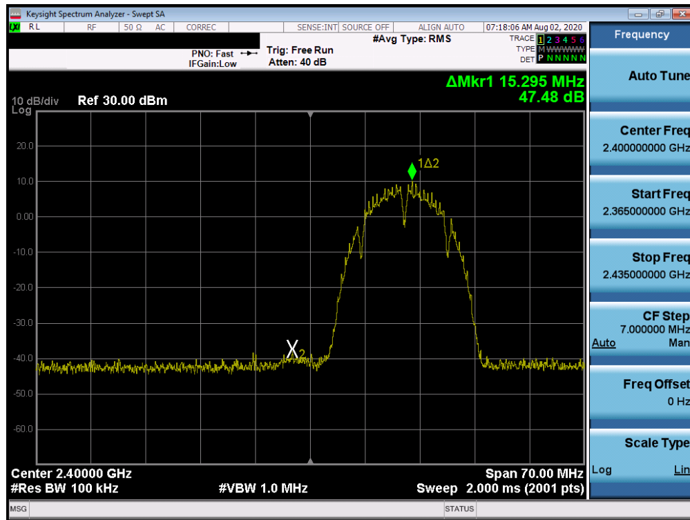
Plot 7-77. Band Edge Plot ANT 1a (802.11b – Ch. 1)
