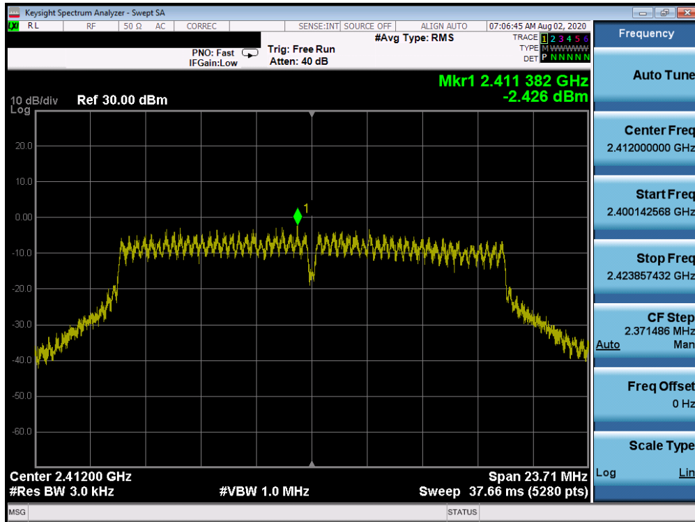
Plot 7-31. Power Spectral Density Plot ANT 1a (802.11g – Ch. 1)
