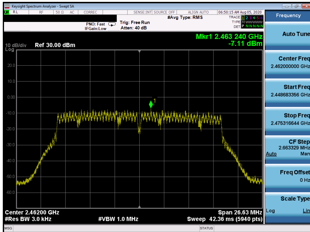
Plot 7-36. Power Spectral Density Plot ANT 1a (802.11n (2.4GHz) – Ch. 11)
