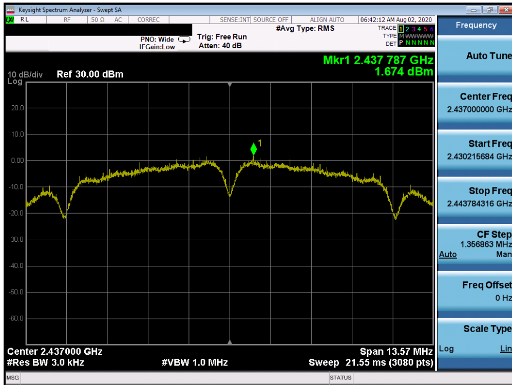
Plot 7-20. Power Spectral Density Plot ANT 3a (802.11b – Ch. 6)
