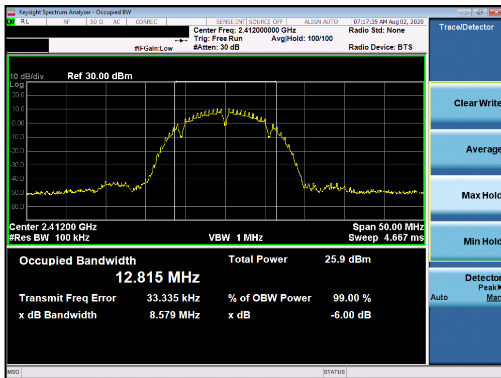
Plot 7-10. 6dB Bandwidth Plot ANT 1a (802.11b – Ch. 1)
