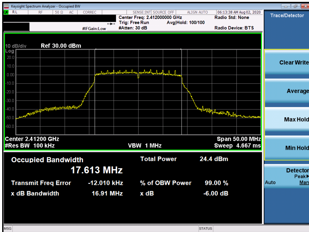
Plot 7-7. 6dB Bandwidth Plot ANT 3a (802.11n (2.4GHz) – Ch. 1)
