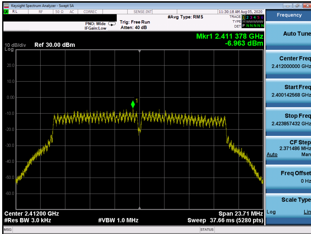
Plot 7-37. Power Spectral Density Plot CDD ANT 3a (802.11g – Ch. 1)
