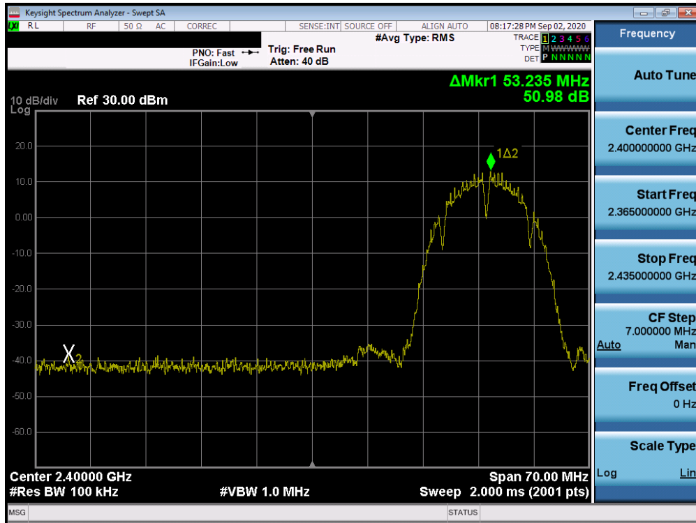
Plot 7-51. Band Edge Plot ANT 3a (802.11b – Ch. 3)
