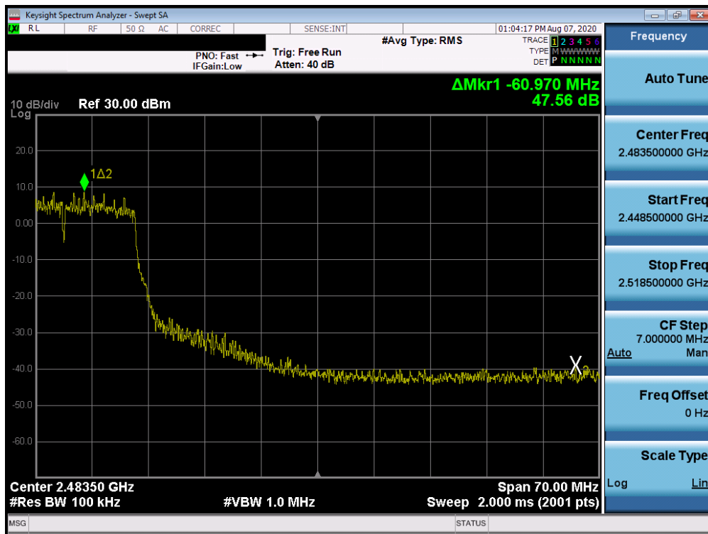
Plot 7-72. Band Edge Plot ANT 3a (802.11n (2.4GHz) – Ch. 9)
