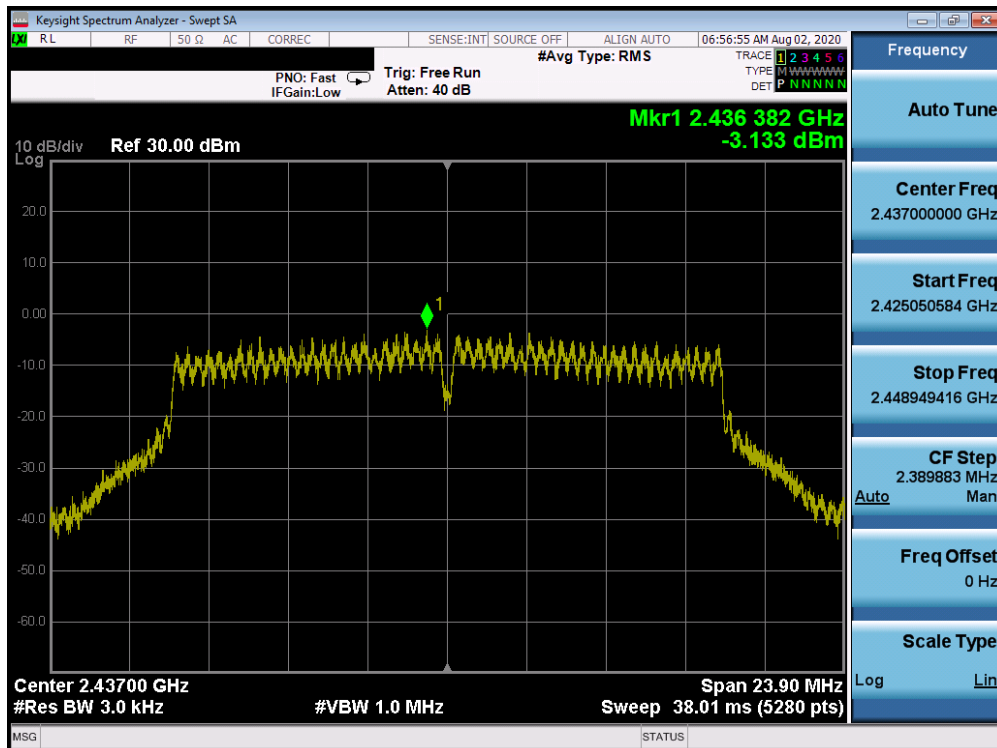
Plot 7-23. Power Spectral Density Plot ANT 3a (802.11g – Ch. 6)
