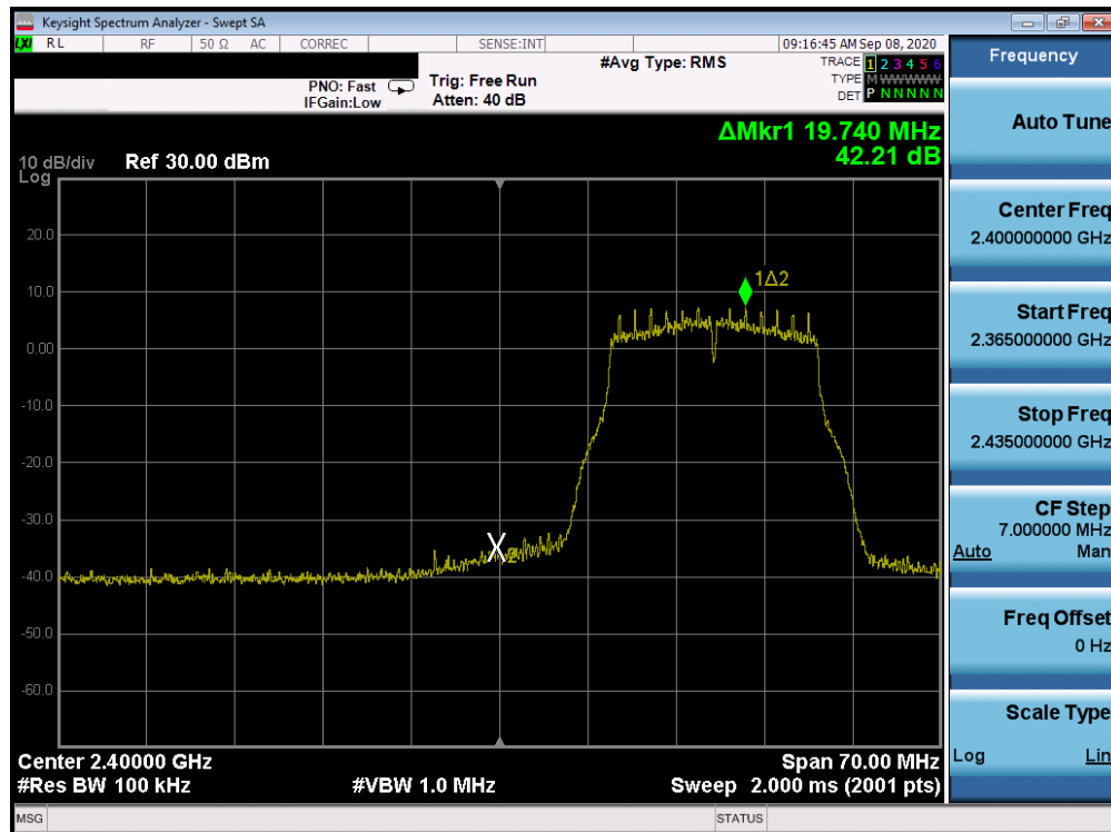
Plot 7-56. Band Edge Plot ANT 3a (802.11g- Ch. 2)
