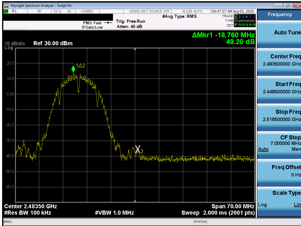
Plot 7-53. Band Edge Plot ANT 3a (802.11b - Ch. 12)
