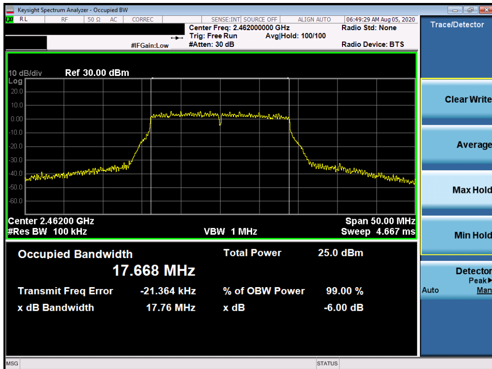
Plot 7-18. 6dB Bandwidth Plot ANT 1a (802.11n (2.4GHz) – Ch. 11)
