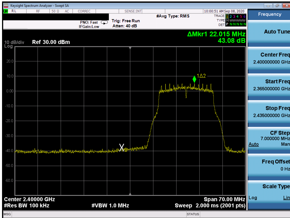
Plot 7-84. Band Edge Plot ANT 1a (802.11g- Ch. 2)
