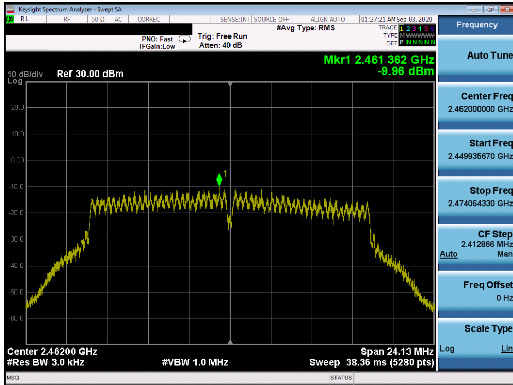
Plot 7-41. Power Spectral Density Plot CDD ANT 3a (802.11g – Ch. 11)
