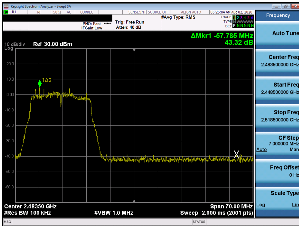
Plot 7-74. Band Edge Plot ANT 3a (802.11n (2.4GHz) – Ch. 11)
