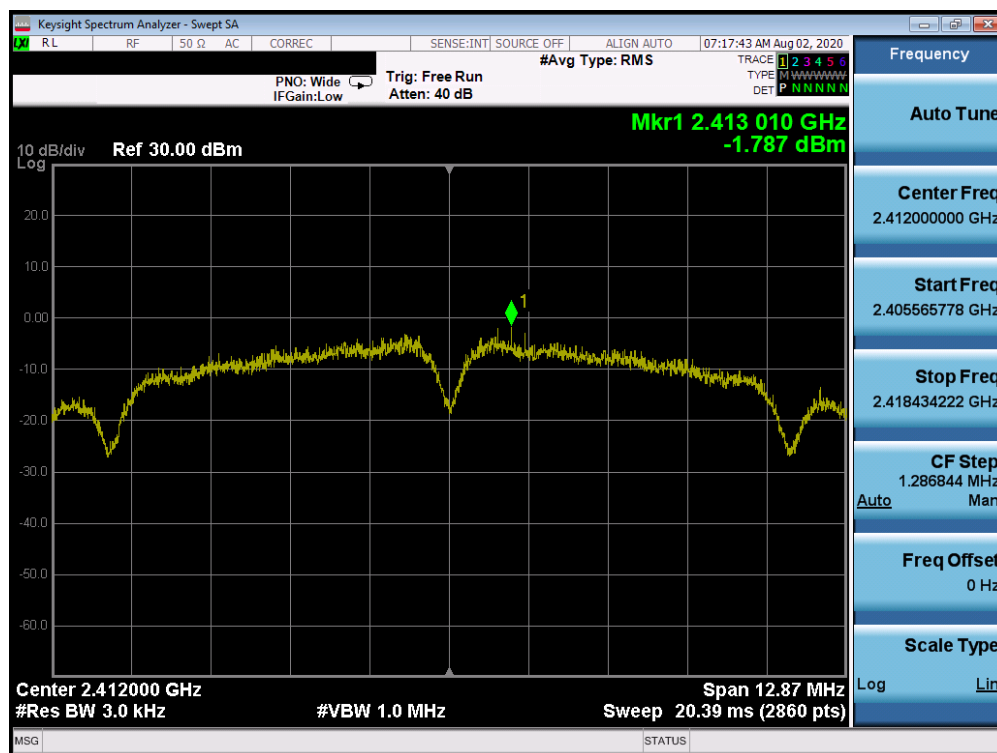
Plot 7-28. Power Spectral Density Plot ANT 1a (802.11b – Ch. 1)
