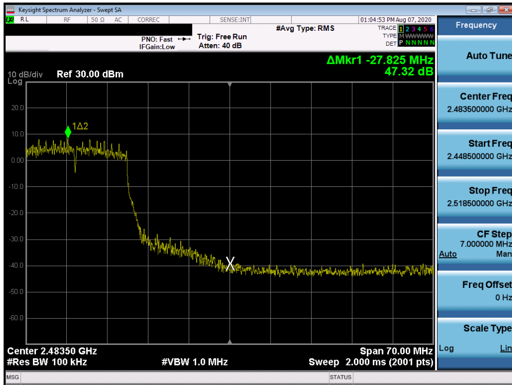
Plot 7-73. Band Edge Plot ANT 3a (802.11n (2.4GHz) – Ch. 10)
