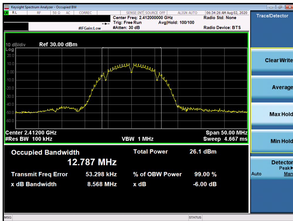
Plot 7-1. 6dB Bandwidth Plot ANT 3a (802.11b – Ch. 1)
