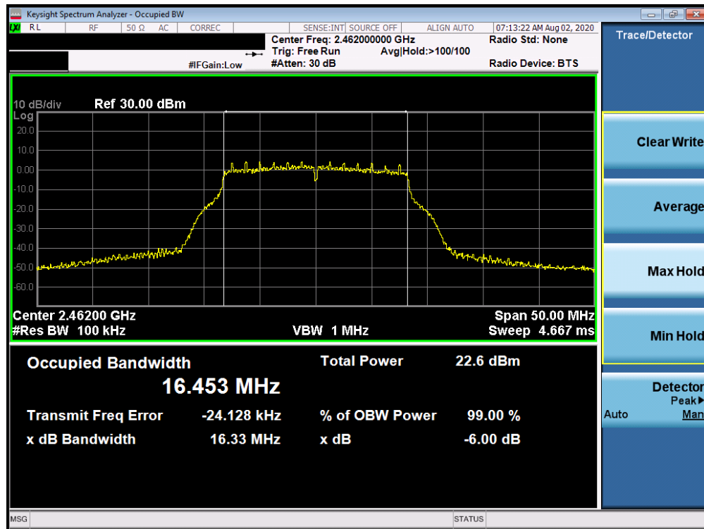
Plot 7-15. 6dB Bandwidth Plot ANT 1a (802.11g – Ch. 11)
