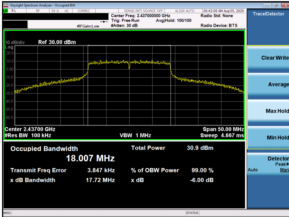
Plot 7-17. 6dB Bandwidth Plot ANT 1a (802.11n (2.4GHz) – Ch. 6)
