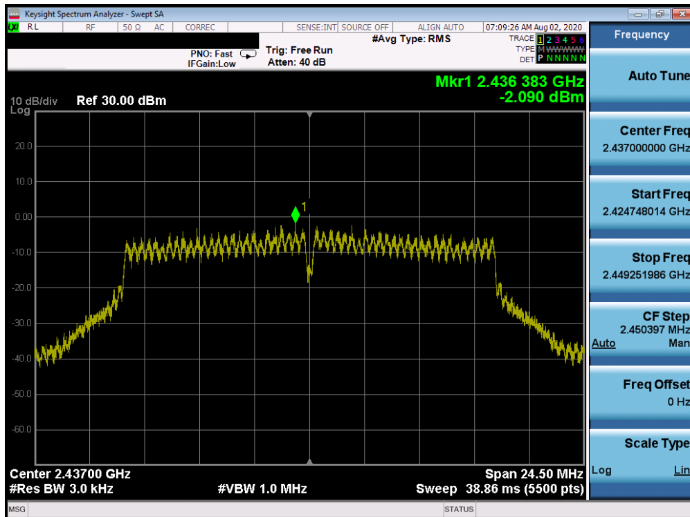
Plot 7-32. Power Spectral Density Plot ANT 1a (802.11g – Ch. 6)
