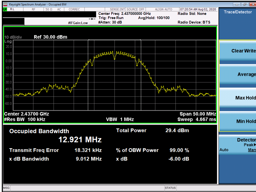
Plot 7-11. 6dB Bandwidth Plot ANT 1a (802.11b – Ch. 6)
