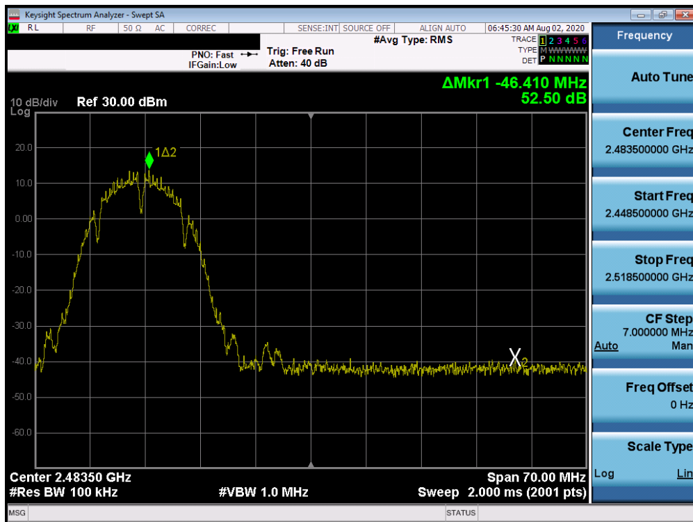
Plot 7-52. Band Edge Plot ANT 3a (802.11b – Ch. 11)
