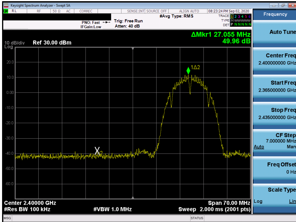
Plot 7-50. Band Edge Plot ANT 3a (802.11b – Ch. 2)
