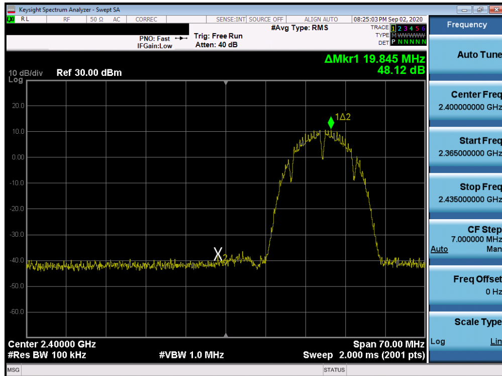
Plot 7-78. Band Edge Plot ANT 1a (802.11b – Ch. 2)
