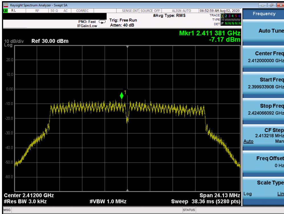
Plot 7-22. Power Spectral Density Plot ANT 3a (802.11g – Ch. 1)
