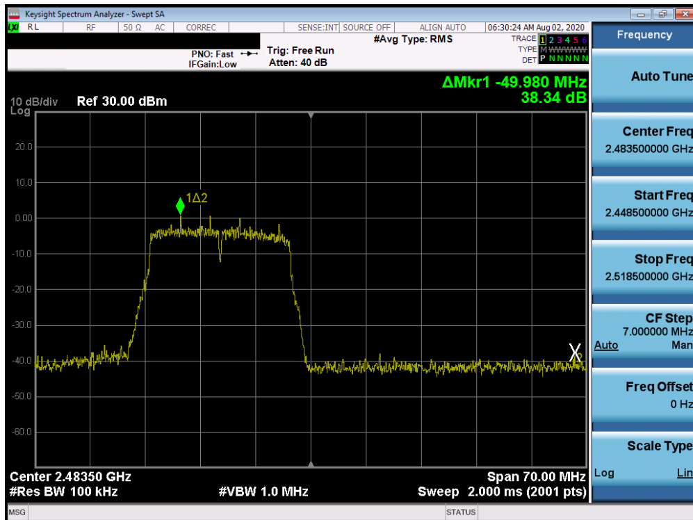
Plot 7-76. Band Edge Plot ANT 3a (802.11n (2.4GHz) – Ch. 13)
