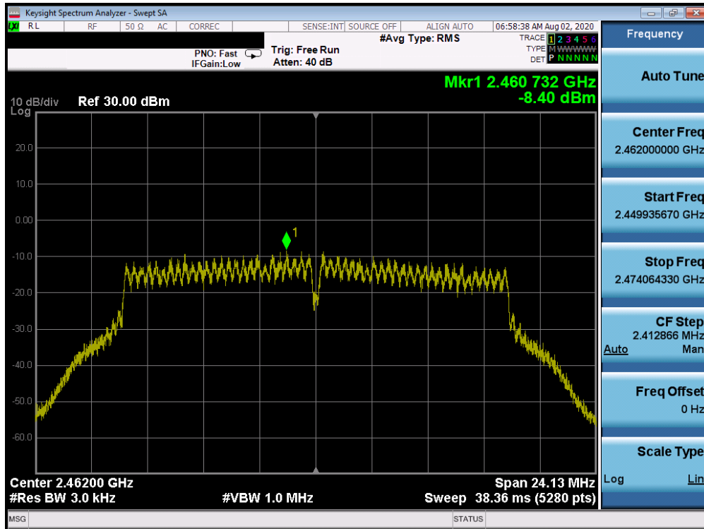
Plot 7-24. Power Spectral Density Plot ANT 3a (802.11g – Ch. 11)
