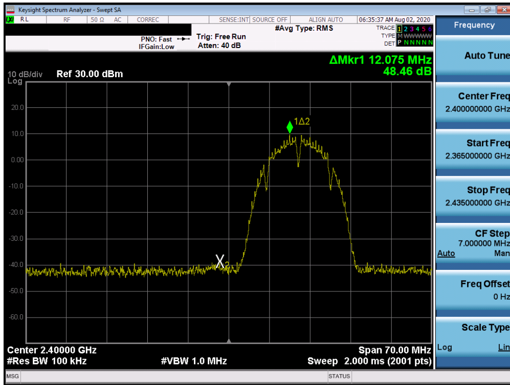
Plot 7-49. Band Edge Plot ANT 3a (802.11b – Ch. 1)
