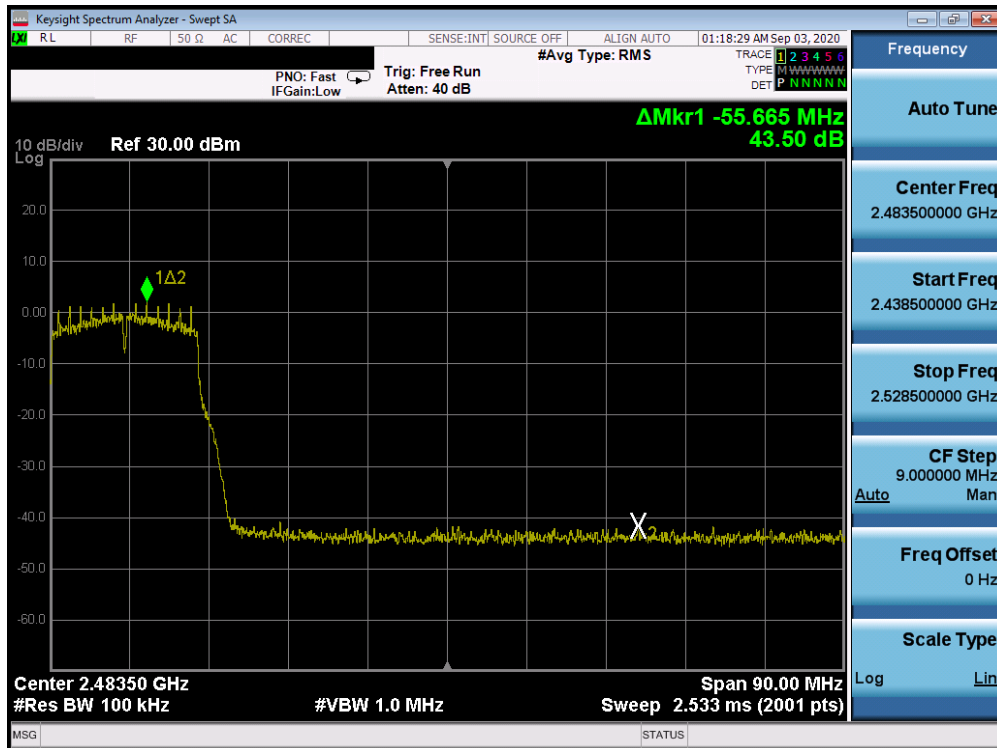
Plot 7-60. Band Edge Plot ANT 3a (802.11g – Ch. 8)
