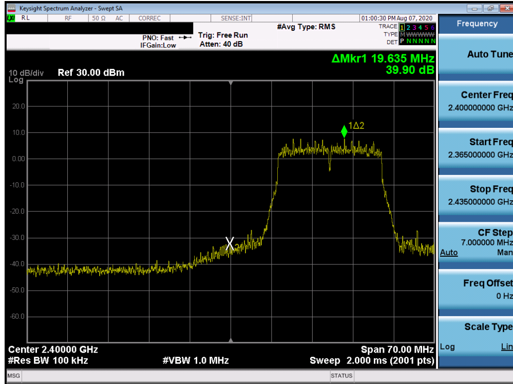
Plot 7-67. Band Edge Plot ANT 3a (802.11n (2.4GHz) – Ch. 2)
