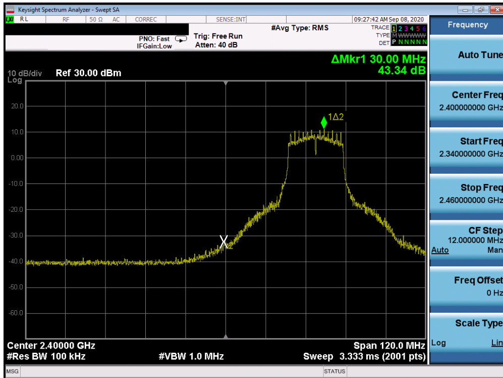
Plot 7-58. Band Edge Plot ANT 3a (802.11g- Ch. 4)
