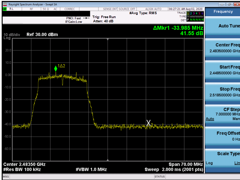
Plot 7-75. Band Edge Plot ANT 3a (802.11n (2.4GHz) – Ch. 12)
