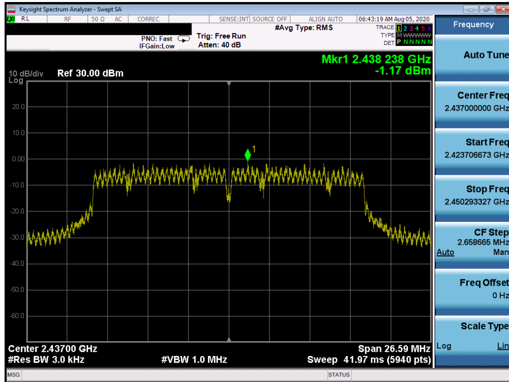
Plot 7-35. Power Spectral Density Plot ANT 1a (802.11n (2.4GHz) – Ch. 6)
