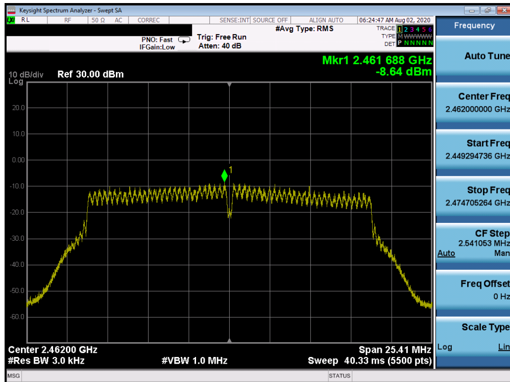
Plot 7-27. Power Spectral Density Plot ANT 3a (802.11n (2.4GHz) – Ch. 11)
