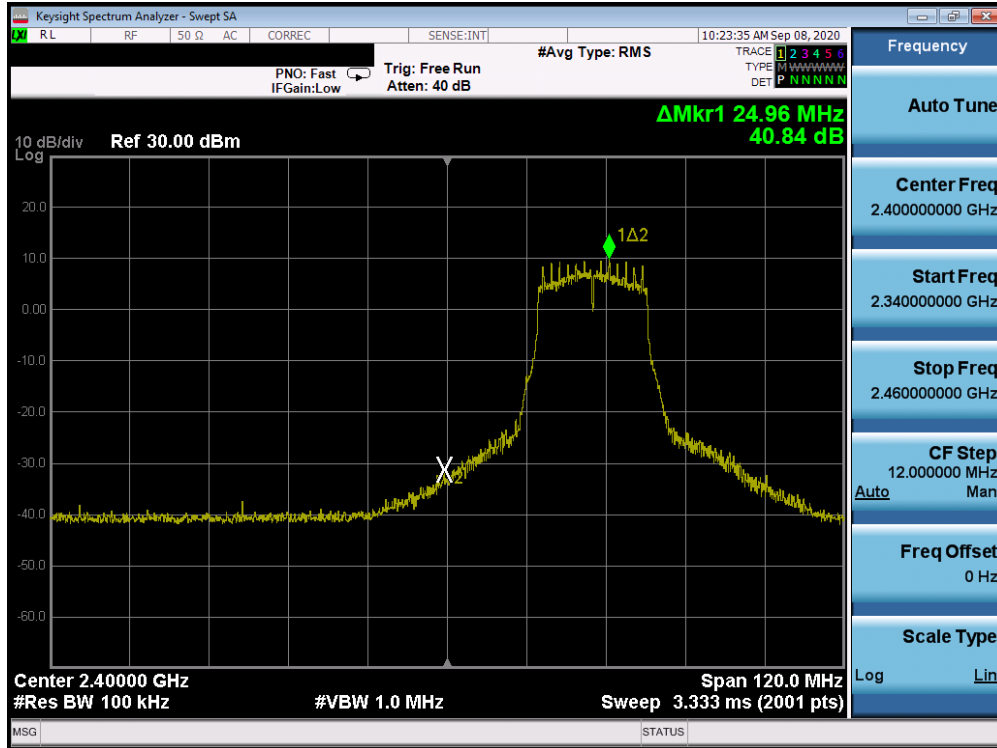
Plot 7-57. Band Edge Plot ANT 3a (802.11g- Ch. 3)
