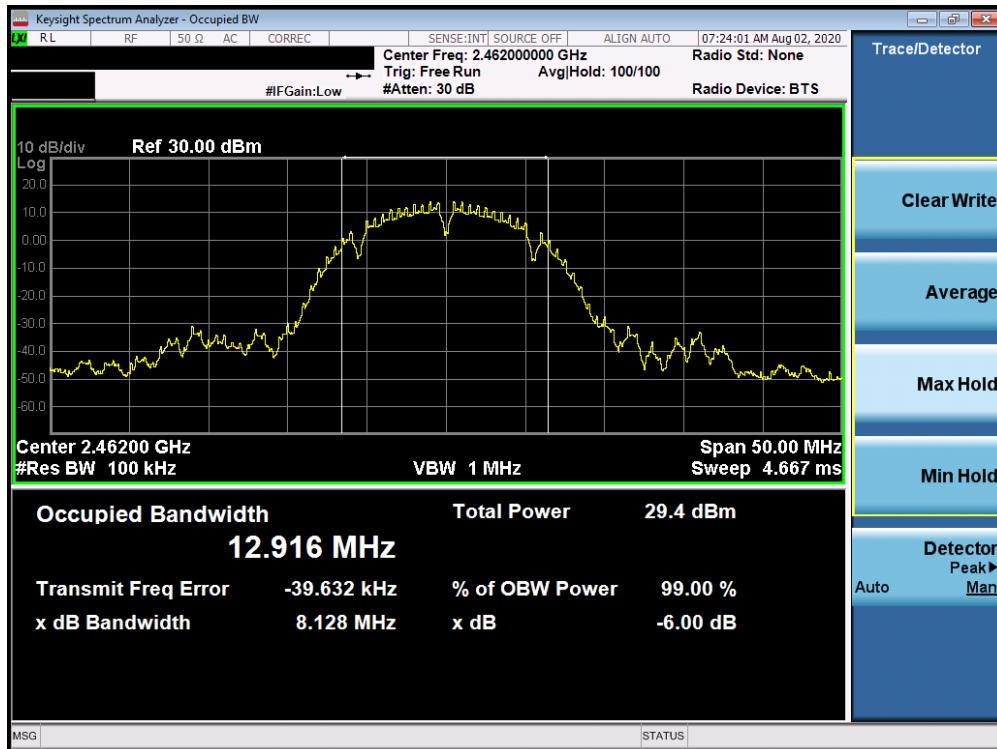
Plot 7-12. 6dB Bandwidth Plot ANT 1a (802.11b – Ch. 11)
