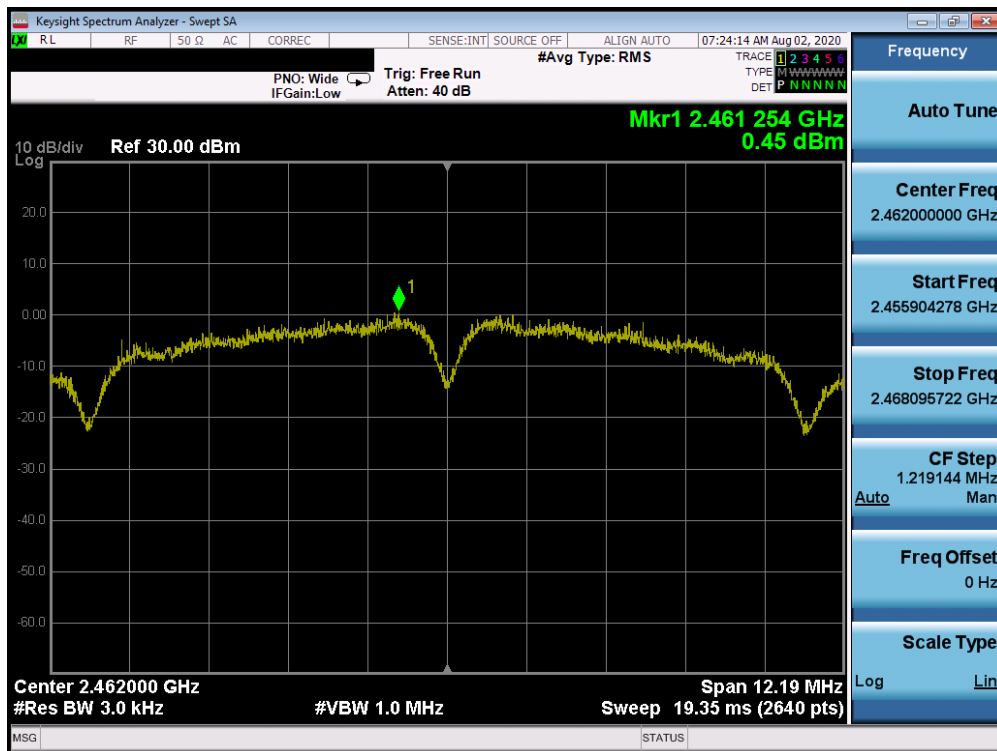
Plot 7-30. Power Spectral Density Plot ANT 1a (802.11b – Ch. 11)
