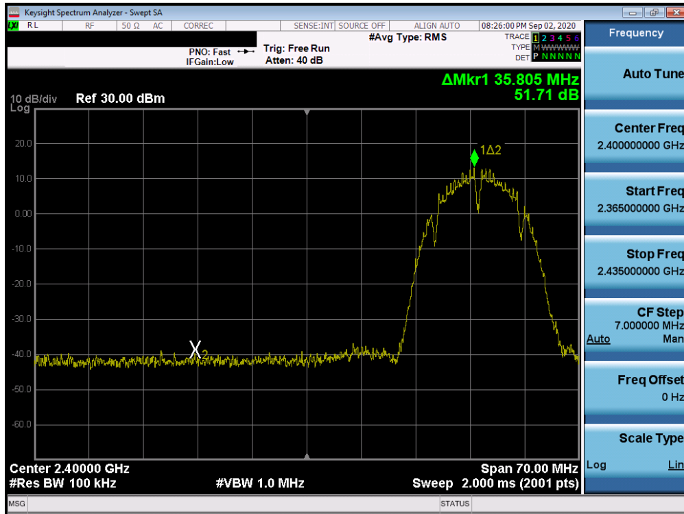
Plot 7-79. Band Edge Plot ANT 1a (802.11b – Ch. 3)
