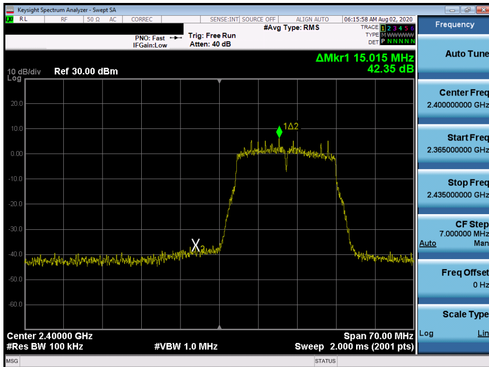
Plot 7-66. Band Edge Plot ANT 3a (802.11n (2.4GHz) – Ch. 1)
