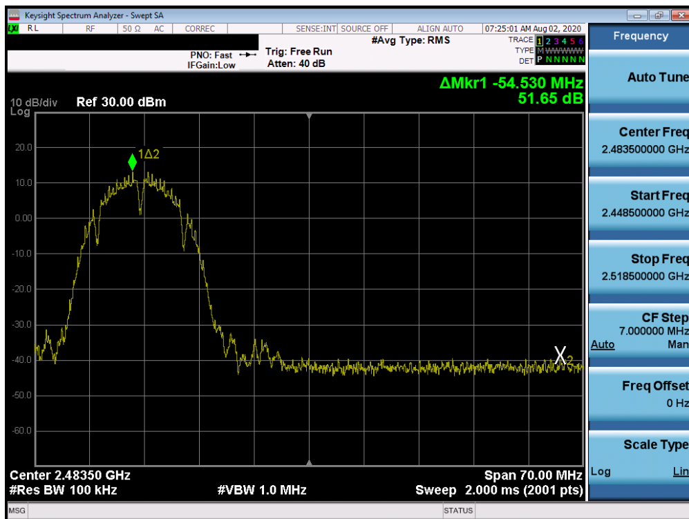
Plot 7-80. Band Edge Plot ANT 1a (802.11b – Ch. 11)
