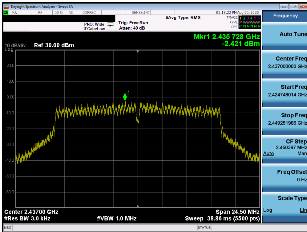
Plot 7-40. Power Spectral Density Plot CDD ANT 1a (802.11g – Ch. 6)
