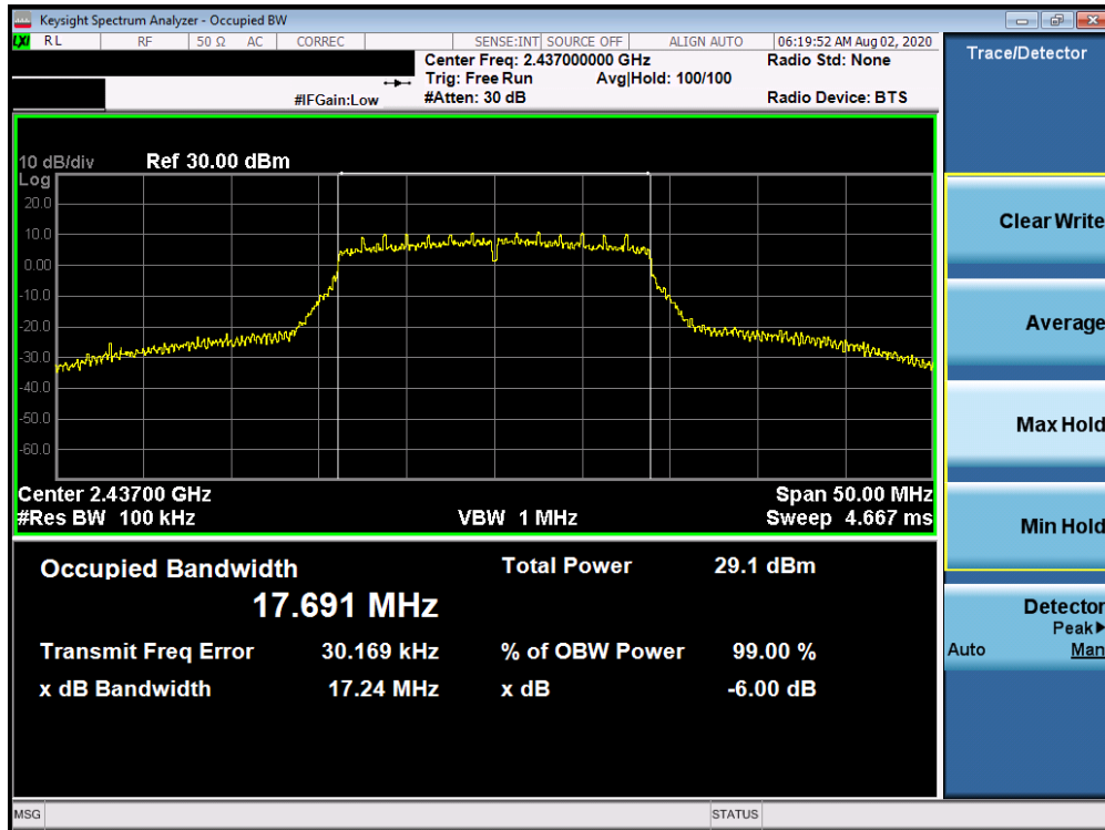
Plot 7-8. 6dB Bandwidth Plot ANT 3a (802.11n (2.4GHz) – Ch. 6)
