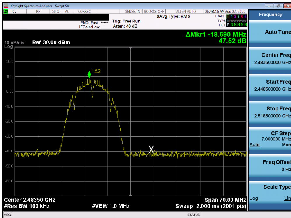
Plot 7-54. Band Edge Plot ANT 3a (802.11b - Ch. 13)
