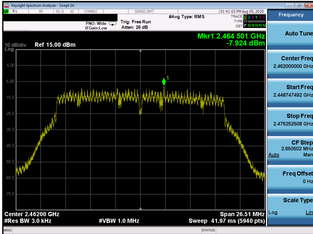
Plot 7-47. Power Spectral Density Plot CDD ANT 3a (802.11n (2.4GHz) – Ch. 11)
