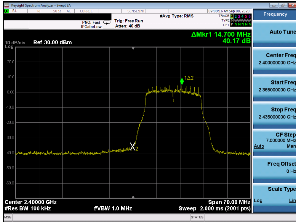
Plot 7-55. Band Edge Plot ANT 3a (802.11g- Ch. 1)
