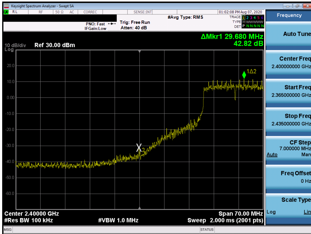
Plot 7-69. Band Edge Plot ANT 3a (802.11n (2.4GHz) – Ch. 4)
