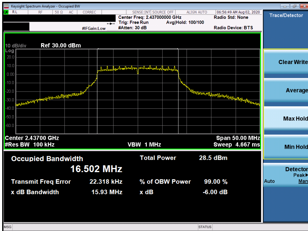
Plot 7-5. 6dB Bandwidth Plot ANT 3a (802.11g – Ch. 6)
