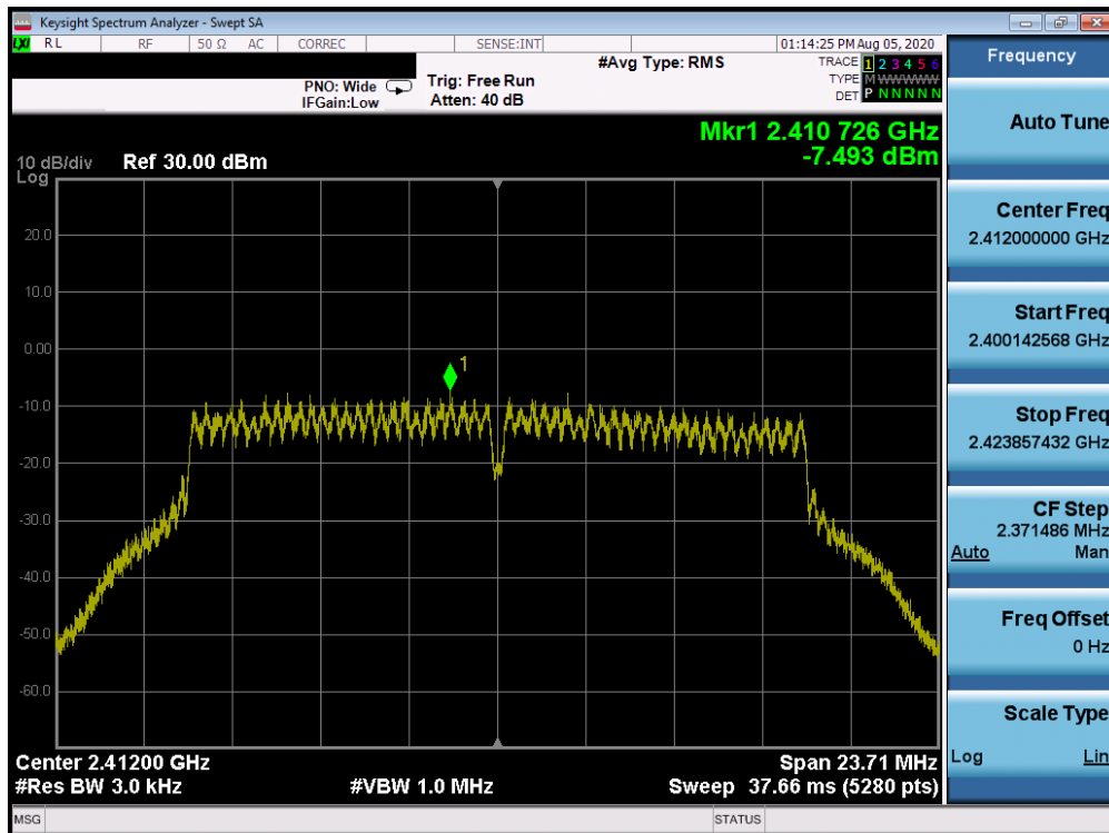
Plot 7-38. Power Spectral Density Plot CDD ANT 1a (802.11g – Ch. 1)
