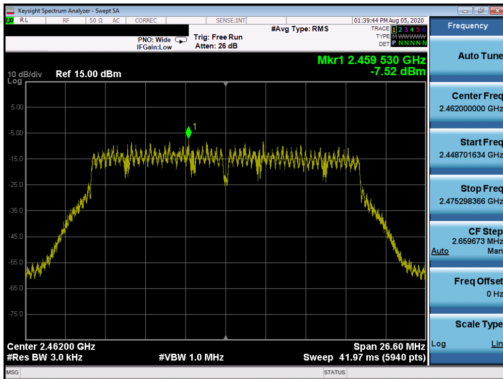
Plot 7-48. Power Spectral Density Plot CDD ANT 1a (802.11n (2.4GHz) – Ch. 11)
