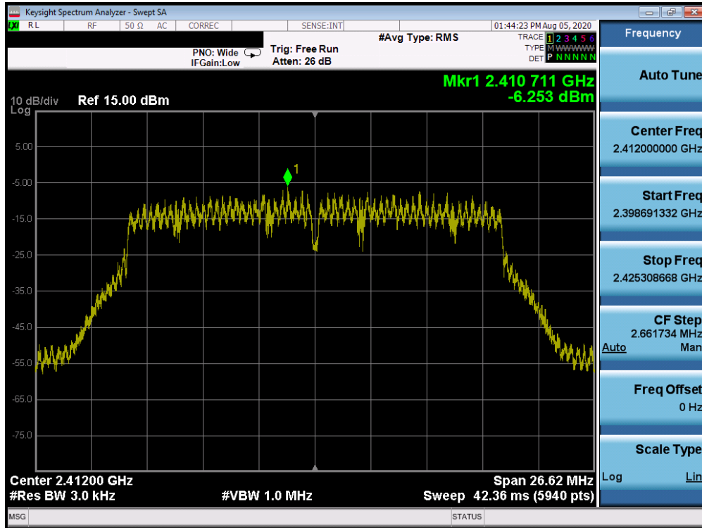
Plot 7-43. Power Spectral Density Plot CDD ANT 3a (802.11n (2.4GHz) – Ch. 1)
