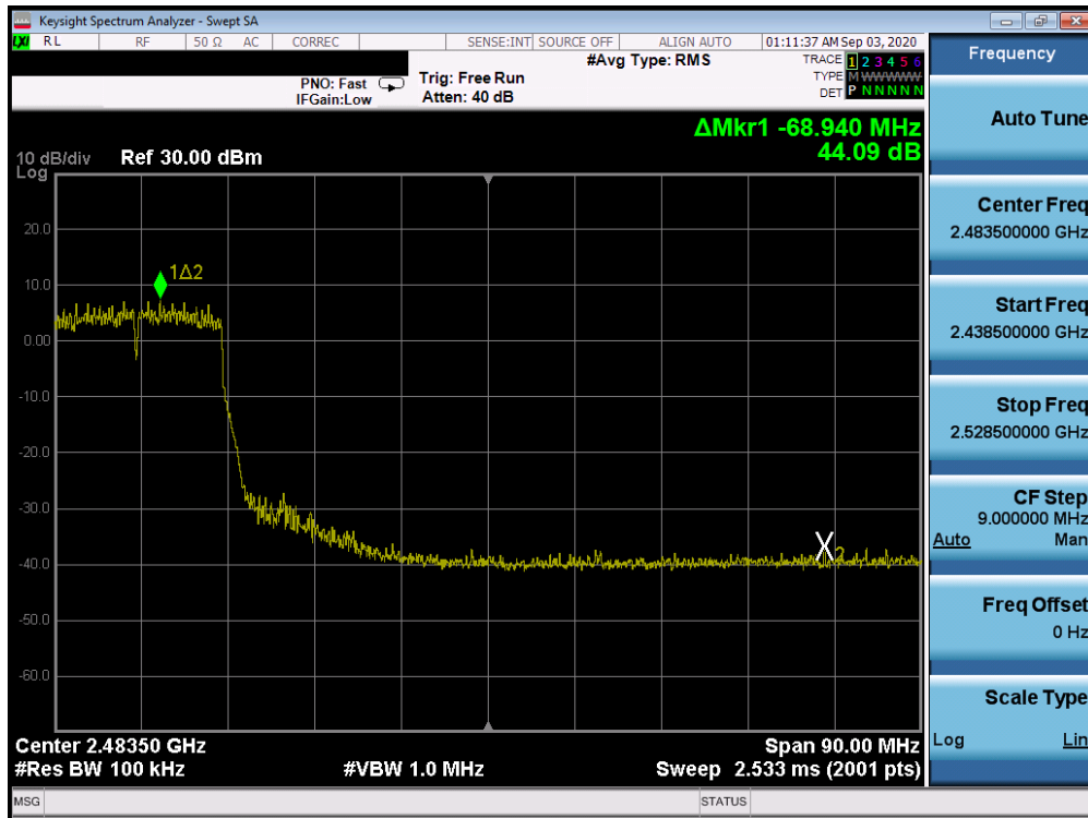
Plot 7-71. Band Edge Plot ANT 3a (802.11n (2.4GHz) – Ch. 8)
