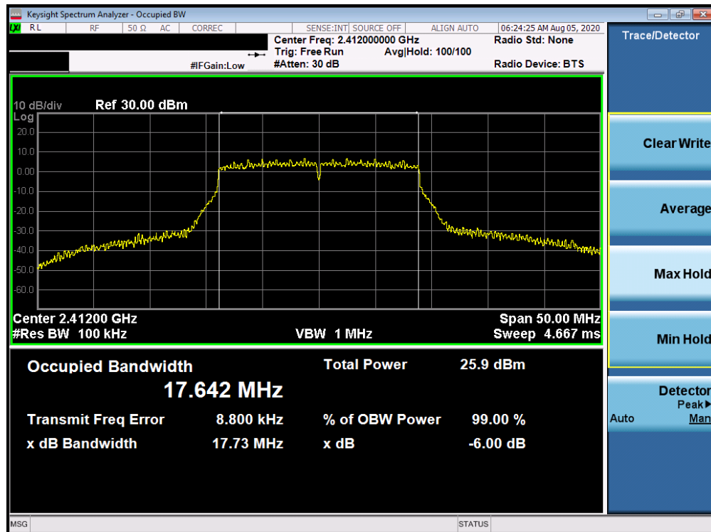
Plot 7-16. 6dB Bandwidth Plot ANT 1a (802.11n (2.4GHz) – Ch. 1)
