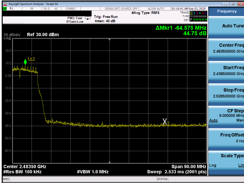
Plot 7-59. Band Edge Plot ANT 3a (802.11g – Ch. 7)
