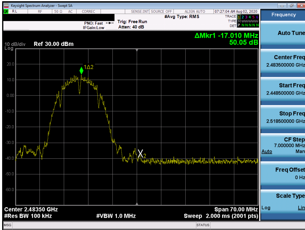
Plot 7-81. Band Edge Plot ANT 1a (802.11b – Ch. 12)
