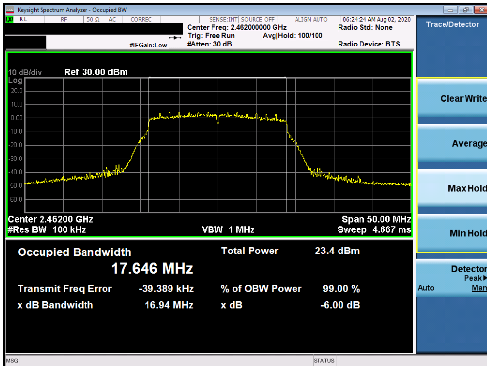
Plot 7-9. 6dB Bandwidth Plot ANT 3a (802.11n (2.4GHz) – Ch. 11)
