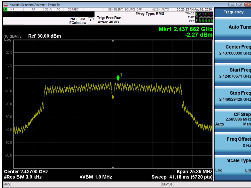
Plot 7-26. Power Spectral Density Plot ANT 3a (802.11n (2.4GHz) – Ch. 6)
