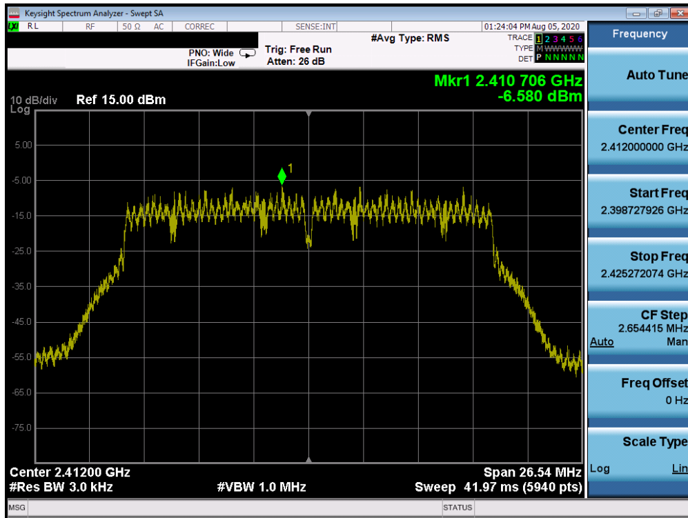
Plot 7-44. Power Spectral Density Plot CDD ANT 1a (802.11n (2.4GHz) – Ch. 1)
