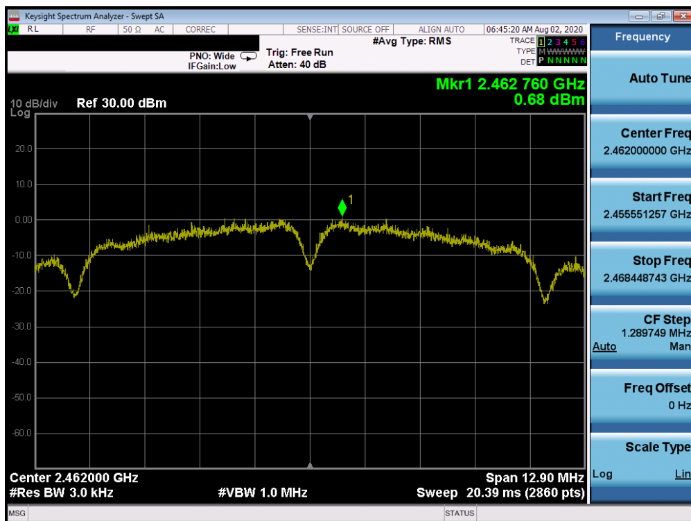
Plot 7-21. Power Spectral Density Plot ANT 3a (802.11b – Ch. 11)
