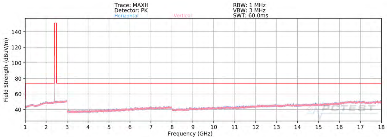
Plot 7-81. Radiated Spurious Emissions Above 1GHz Antenna 3a (4Mbps, HDR4, ePA – Ch. 1)
