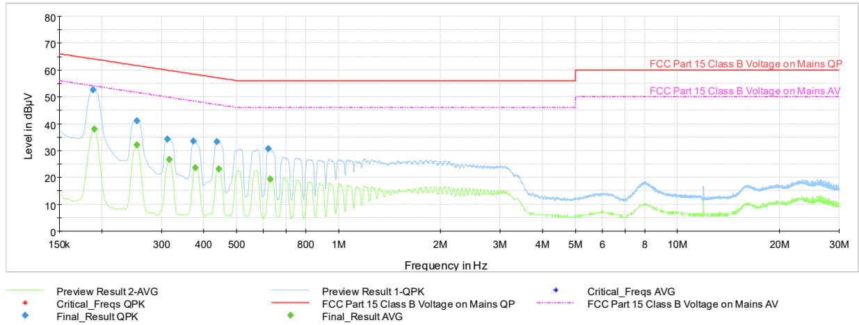
Plot 7-106. AC Line Conducted Plot with Bluetooth HDR (N, 4Mbps ePA - Ch.1 with Laptop)
