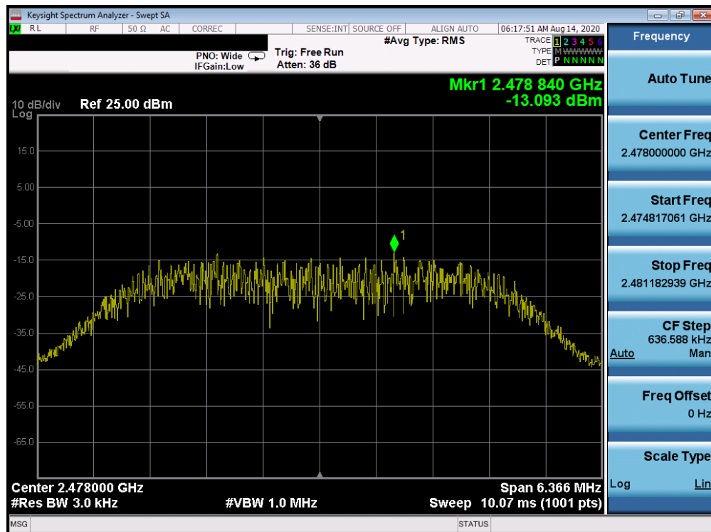
Plot 7-24. Power Spectral Density Plot Antenna 3a (Bluetooth (HDR8), 8Mbps, iPA – Ch. 75)
