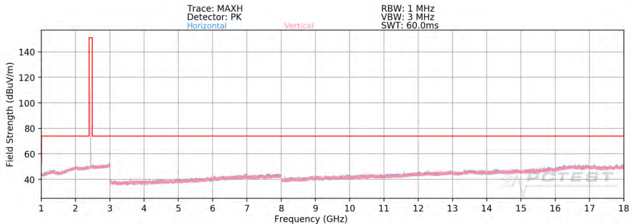
Plot 7-85. Radiated Spurious Emissions Above 1GHz Antenna 1a (4Mbps, HDR4, ePA – Ch. 38)
