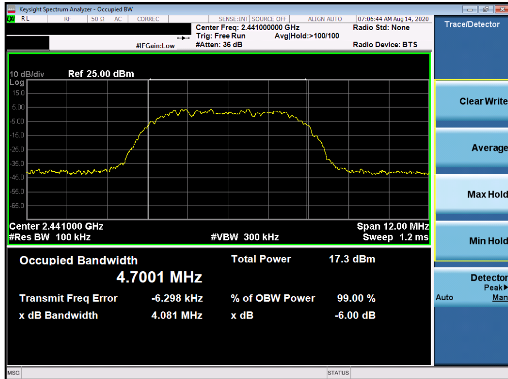
Plot 7-11. 6dB Bandwidth Plot Antenna 1a (Bluetooth (HDR8), 8Mbps, ePA – Ch. 38)
