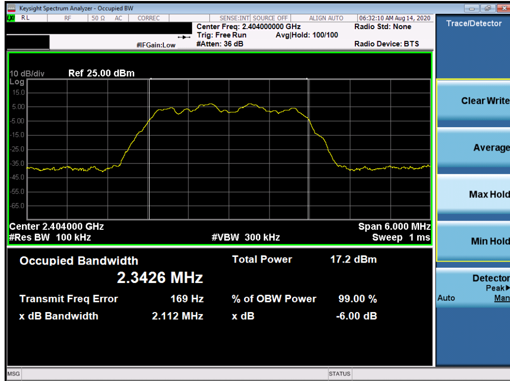
Plot 7-7. 6dB Bandwidth Plot Antenna 1a (Bluetooth (HDR4), 4Mbps, ePA – Ch. 1)
