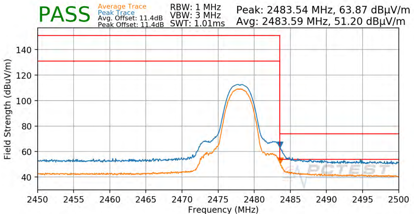
Plot 7-98. Radiated Restricted Upper Band Edge Measurement Antenna 1a (Average & Peak)
