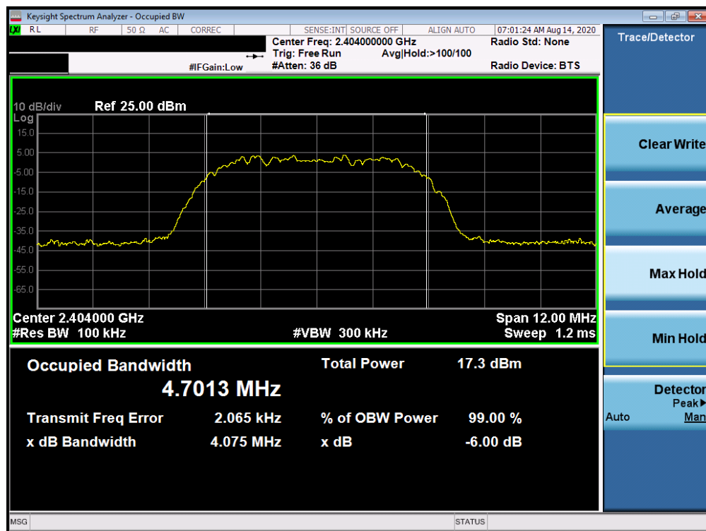
Plot 7-10. 6dB Bandwidth Plot Antenna 1a (Bluetooth (HDR8), 8Mbps, ePA – Ch. 1)
