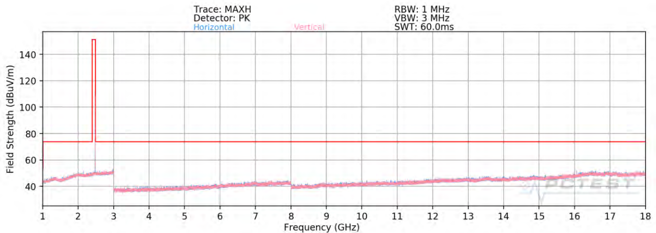
Plot 7-89. Radiated Spurious Emissions Above 1GHz TxBF (4Mbps, HDR4, ePA – Ch. 75)
