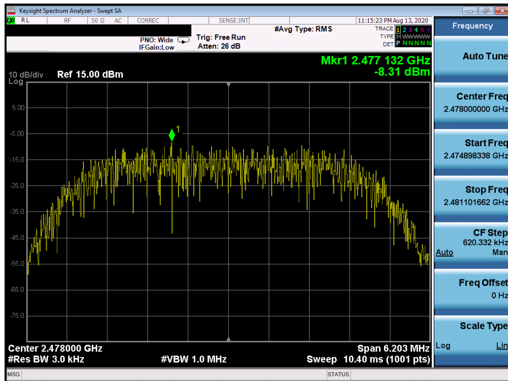
Plot 7-53. Power Spectral Density Plot TxBF Antenna 3a (Bluetooth (HDR8), 8Mbps, ePA – Ch. 75)
