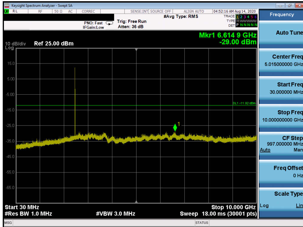
Plot 7-73. Conducted Spurious Plot Antenna 3a (Bluetooth (HDR4), 4 Mbps, ePA – Ch. 75)
