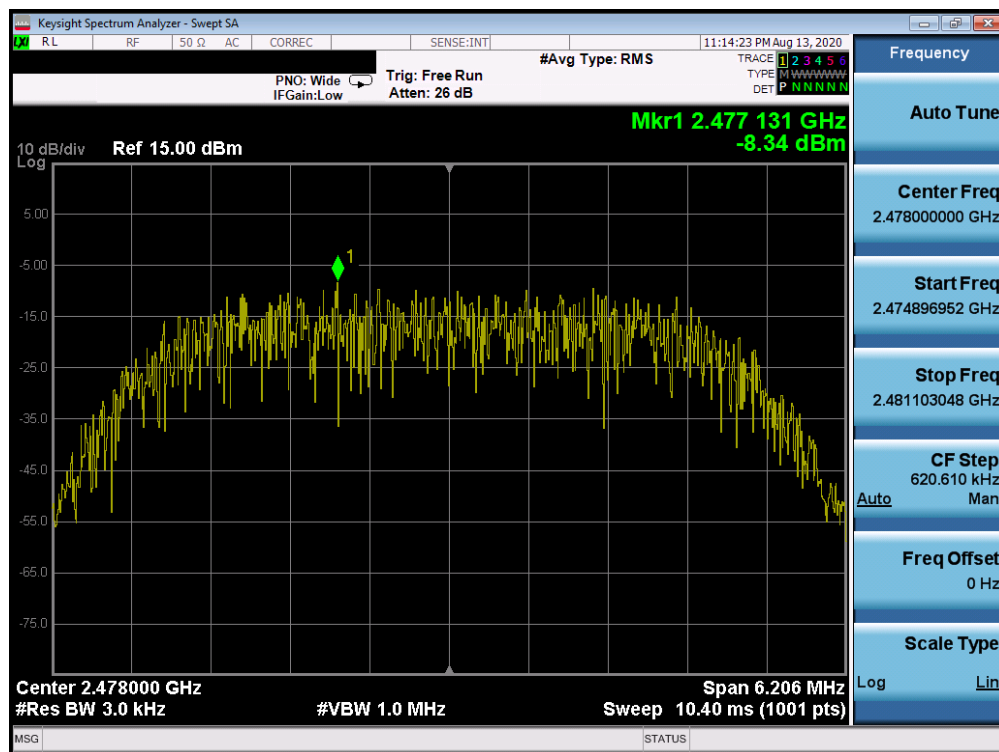
Plot 7-54. Power Spectral Density Plot TxBF Antenna 1a (Bluetooth (HDR8), 8Mbps, ePA – Ch. 75)
