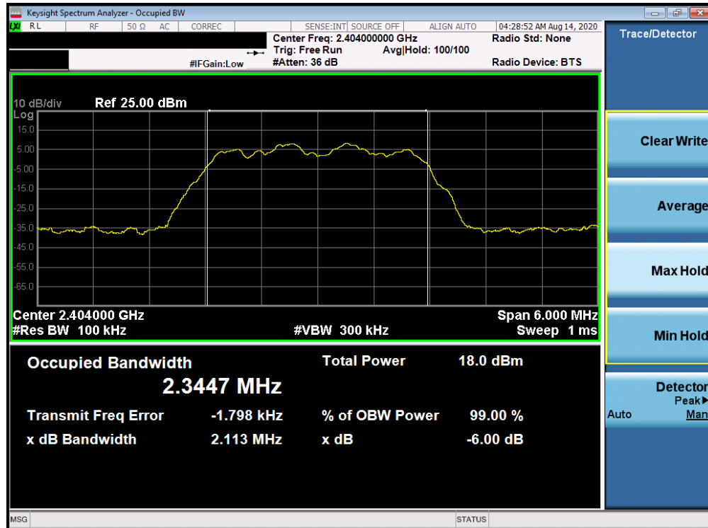
Plot 7-1. 6dB Bandwidth Plot Antenna 3a (Bluetooth (HDR4), 4Mbps, ePA – Ch. 1)
