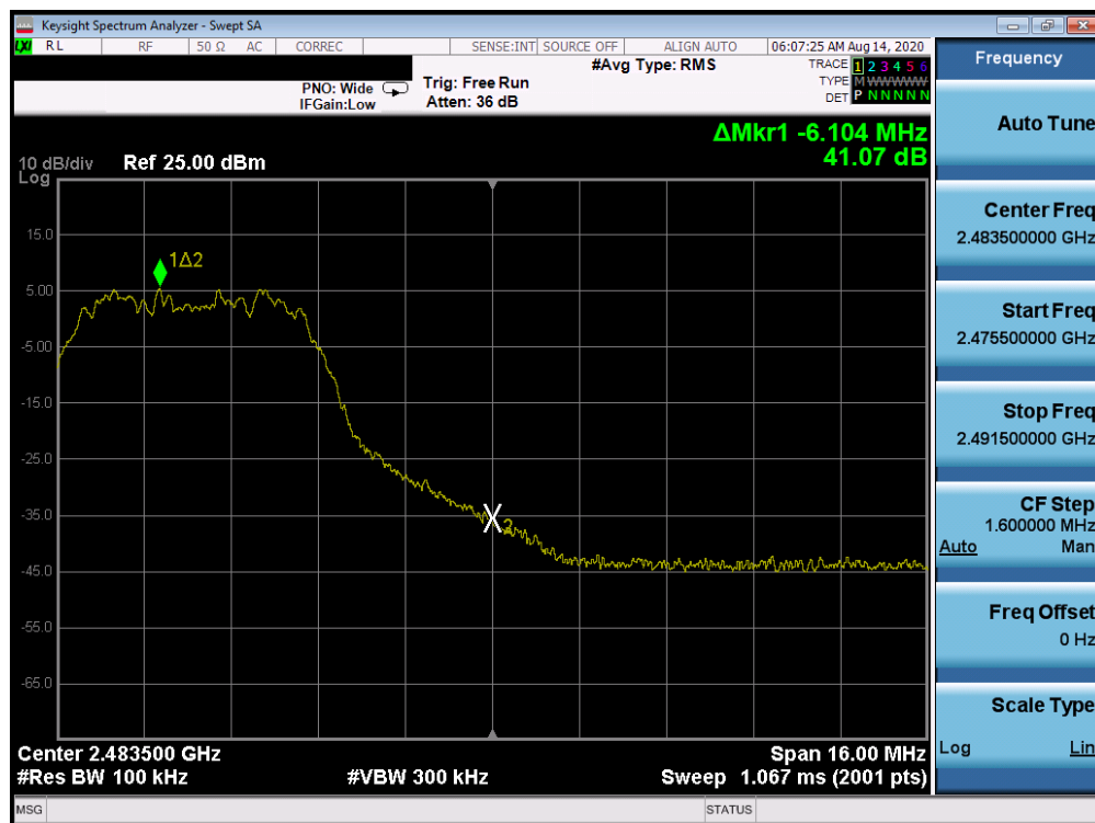
Plot 7-64. Band Edge Plot Antenna 3a (Bluetooth (HDR8), ePA – Ch. 75)
