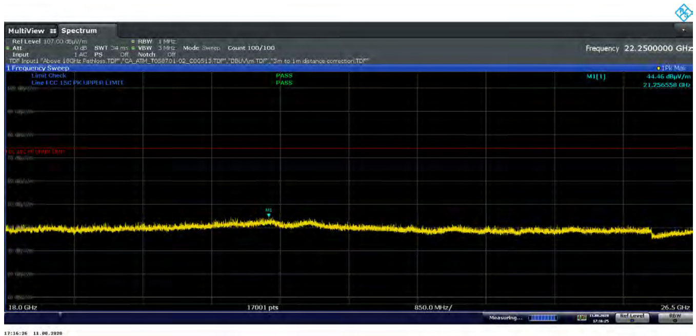
Plot 7-90. Radiated Spurious Emissions Above 18GHz TxBF (4Mbps – Ch.38, ePA, Ant. Pol. H)
