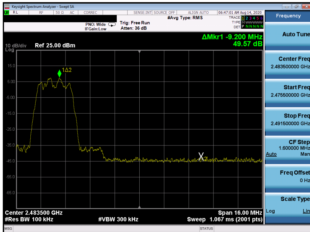
Plot 7-66. Band Edge Plot Antenna 1a (Bluetooth (HDR4), ePA – Ch. 75)
