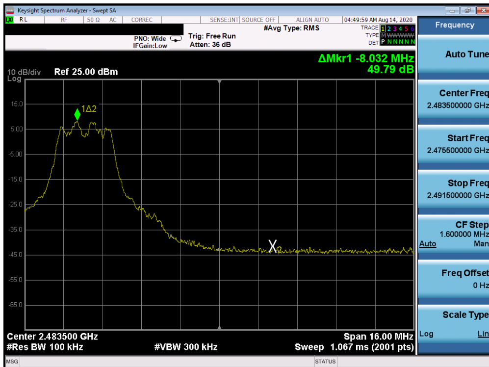
Plot 7-62. Band Edge Plot Antenna 3a (Bluetooth (HDR4), ePA – Ch. 75)
