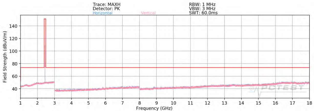
Plot 7-82. Radiated Spurious Emissions Above 1GHz Antenna 3a (4Mbps, HDR4, ePA – Ch. 38)
