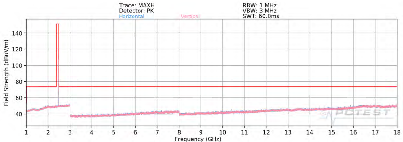
Plot 7-83. Radiated Spurious Emissions Above 1GHz Antenna 3a (4Mbps, HDR4, ePA – Ch. 75)
