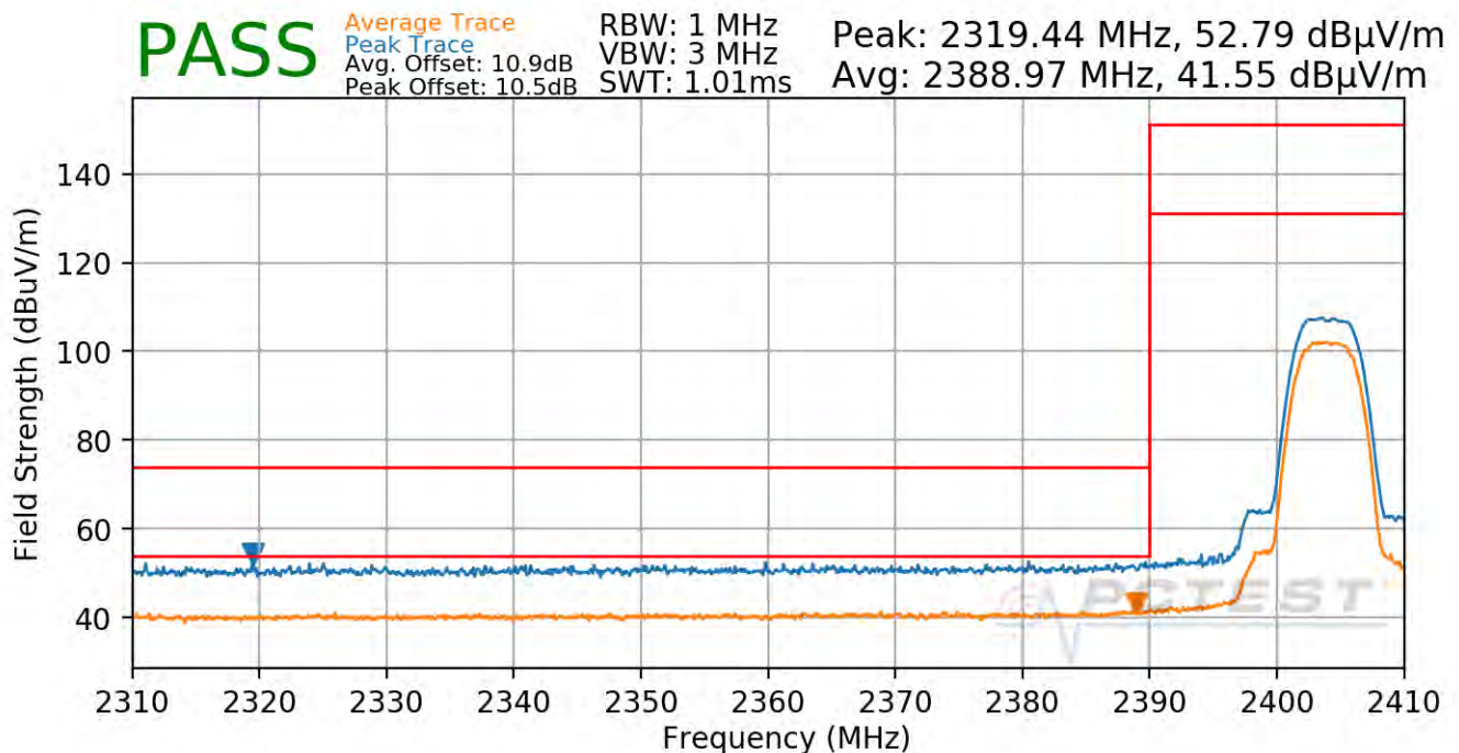
Plot 7-97. Radiated Restricted Lower Band Edge Measurement Antenna 1a (Average & Peak)
