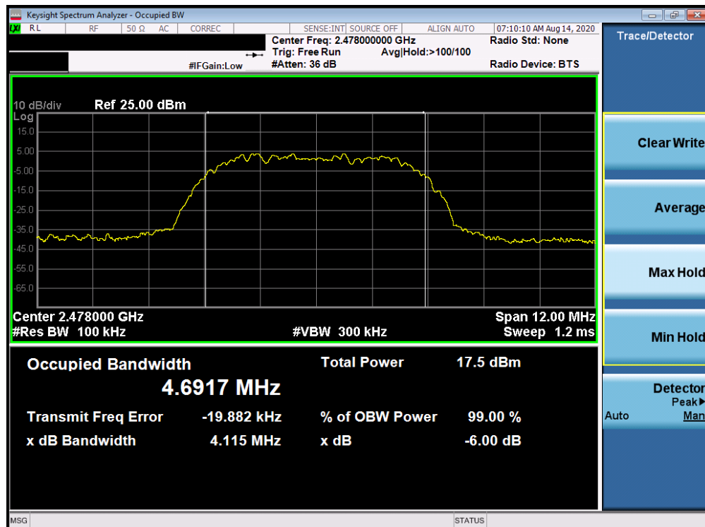
Plot 7-12. 6dB Bandwidth Plot Antenna 1a (Bluetooth (HDR8), 8Mbps, ePA – Ch. 75)
