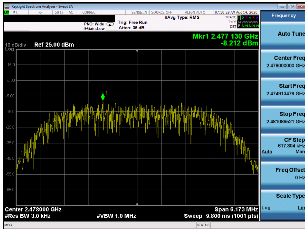
Plot 7-33. Power Spectral Density Plot Antenna 1a (Bluetooth (HDR8), 8Mbps, ePA – Ch. 75)
