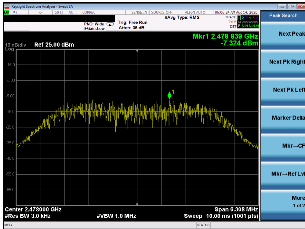
Plot 7-21. Power Spectral Density Plot Antenna 3a (Bluetooth (HDR8), 8Mbps, ePA – Ch. 75)
