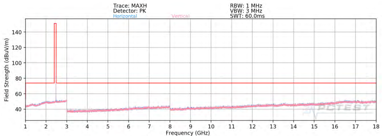
Plot 7-86. Radiated Spurious Emissions Above 1GHz Antenna 1a (4Mbps, HDR4, ePA – Ch. 75)
