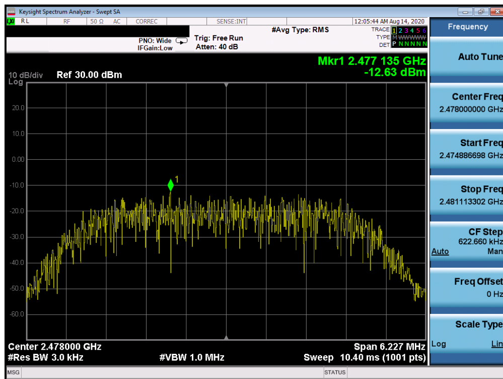
Plot 7-60. Power Spectral Density Plot TxBF Antenna 1a (Bluetooth (HDR8), 8Mbps, iPA – Ch. 75)
