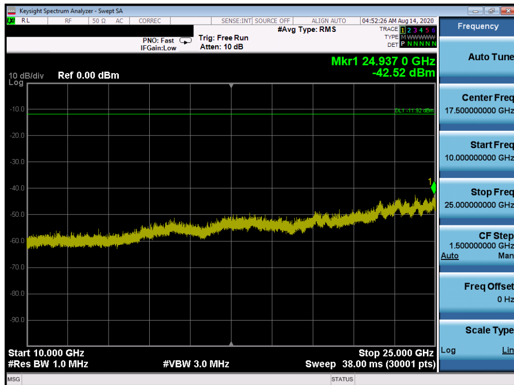
Plot 7-74. Conducted Spurious Plot Antenna 3a (Bluetooth (HDR4), 4 Mbps, ePA – Ch. 75)
