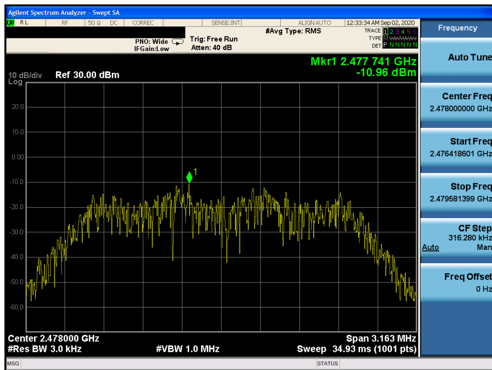
Plot 7-48. Power Spectral Density Plot Tx BF Antenna 1a (Bluetooth (HDR4), 4Mbps, iPA – Ch. 75)
