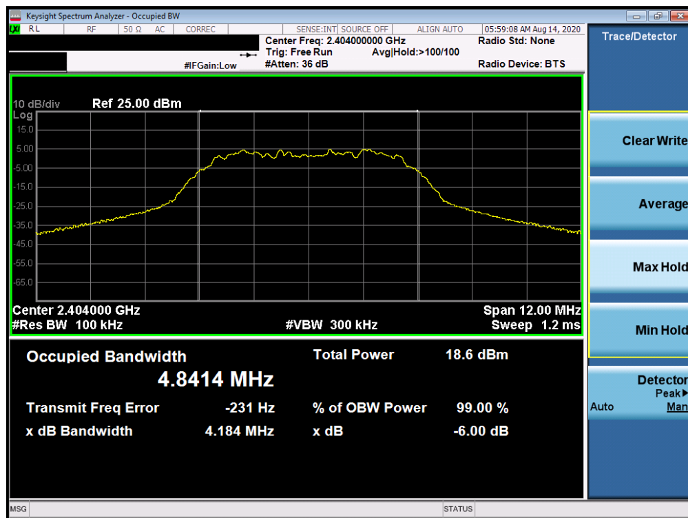
Plot 7-4. 6dB Bandwidth Plot Antenna 3a (Bluetooth (HDR8), 8Mbps, ePA – Ch. 1)
