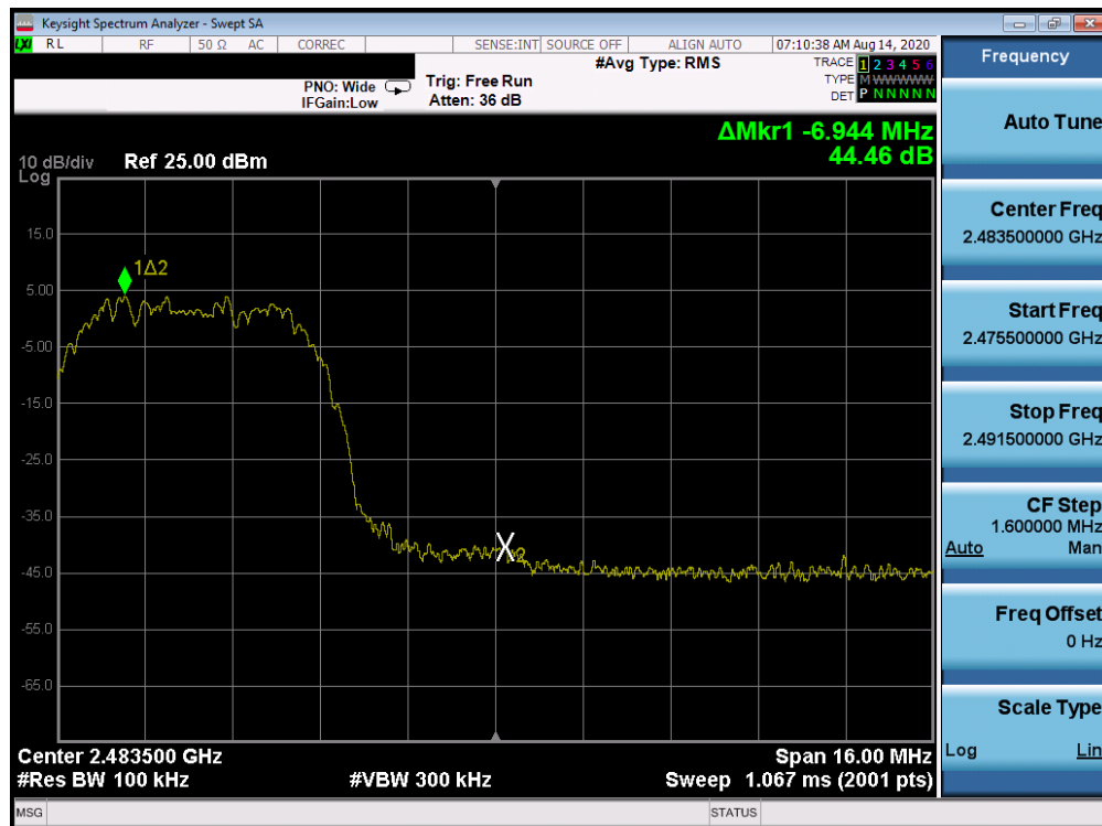
Plot 7-68. Band Edge Plot Antenna 1a (Bluetooth (HDR8), ePA – Ch. 75)
