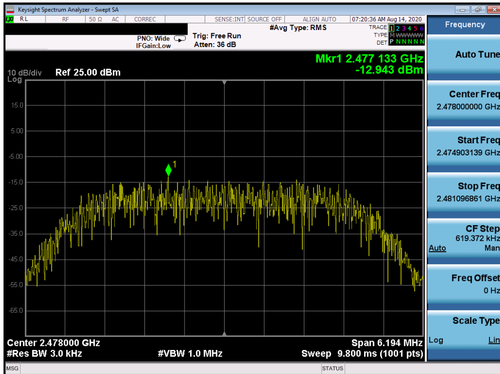
Plot 7-36. Power Spectral Density Plot Antenna 1a (Bluetooth (HDR8), 8Mbps, iPA – Ch. 75)
