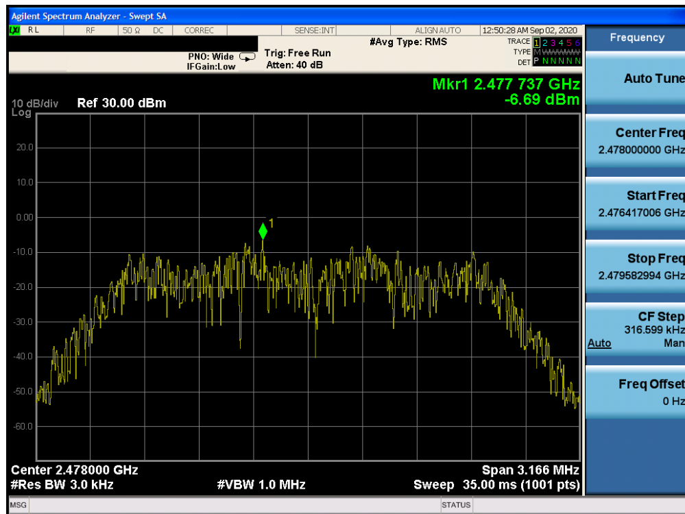
Plot 7-41. Power Spectral Density Plot TxBF Antenna 3a (Bluetooth (HDR4), 4Mbps, ePA – Ch. 75)
