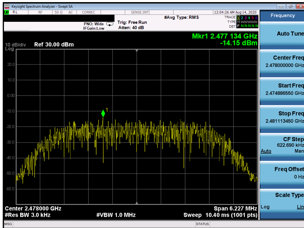
Plot 7-59. Power Spectral Density Plot TxBF Antenna 3a (Bluetooth (HDR8), 8Mbps, iPA – Ch. 75)
