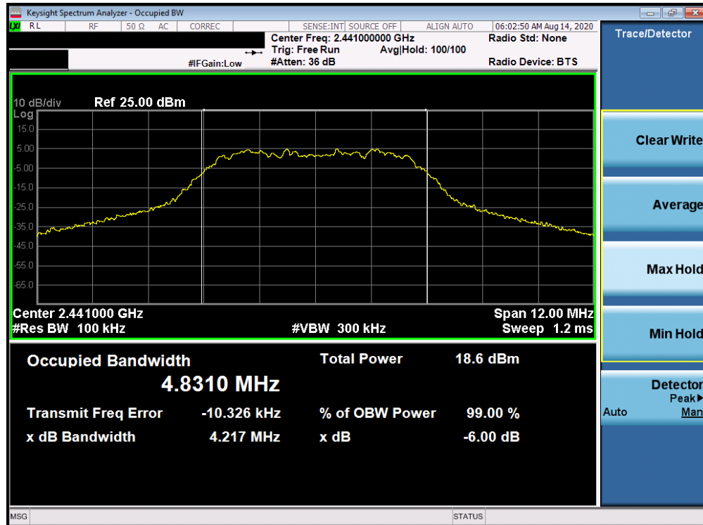
Plot 7-5. 6dB Bandwidth Plot Antenna 3a (Bluetooth (HDR8), 8Mbps, ePA – Ch. 38)
