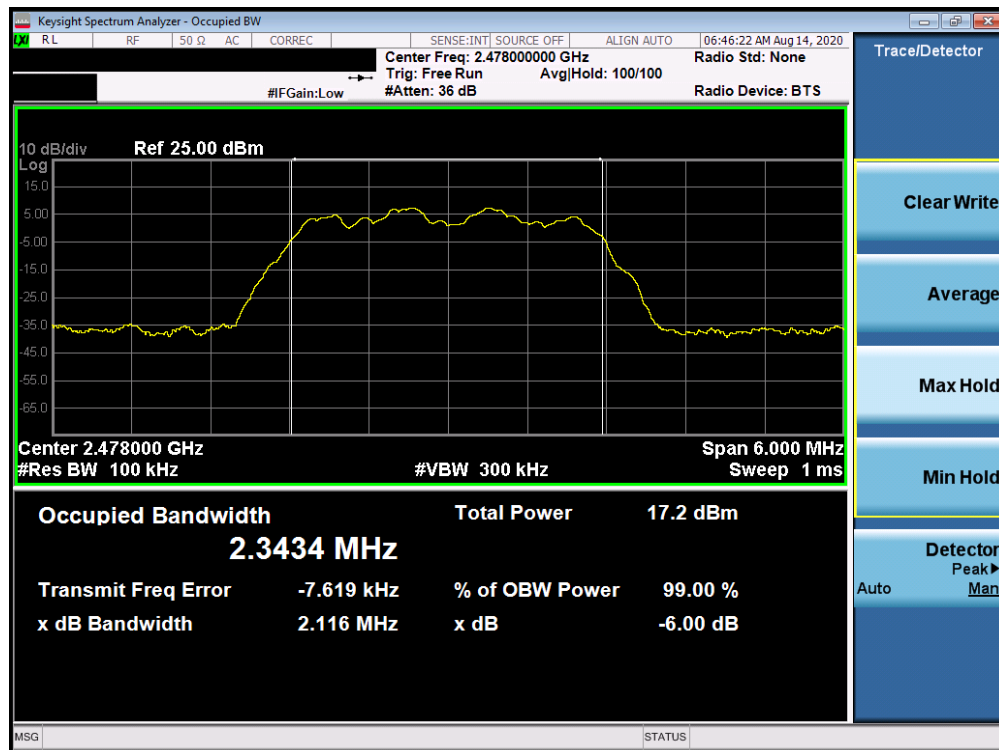
Plot 7-9. 6dB Bandwidth Plot Antenna 1a (Bluetooth (HDR4), 4Mbps, ePA – Ch. 75)
