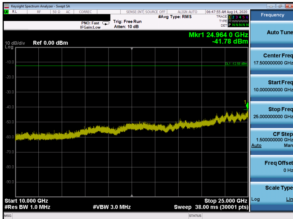
Plot 7-80. Conducted Spurious Plot Antenna 1a (Bluetooth (HDR4), 4 Mbps, ePA – Ch. 75)
