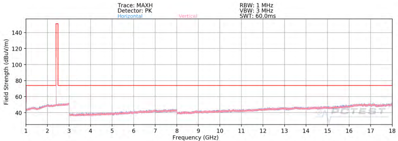
Plot 7-84. Radiated Spurious Emissions Above 1GHz Antenna 1a (4Mbps, HDR4, ePA – Ch. 1)
