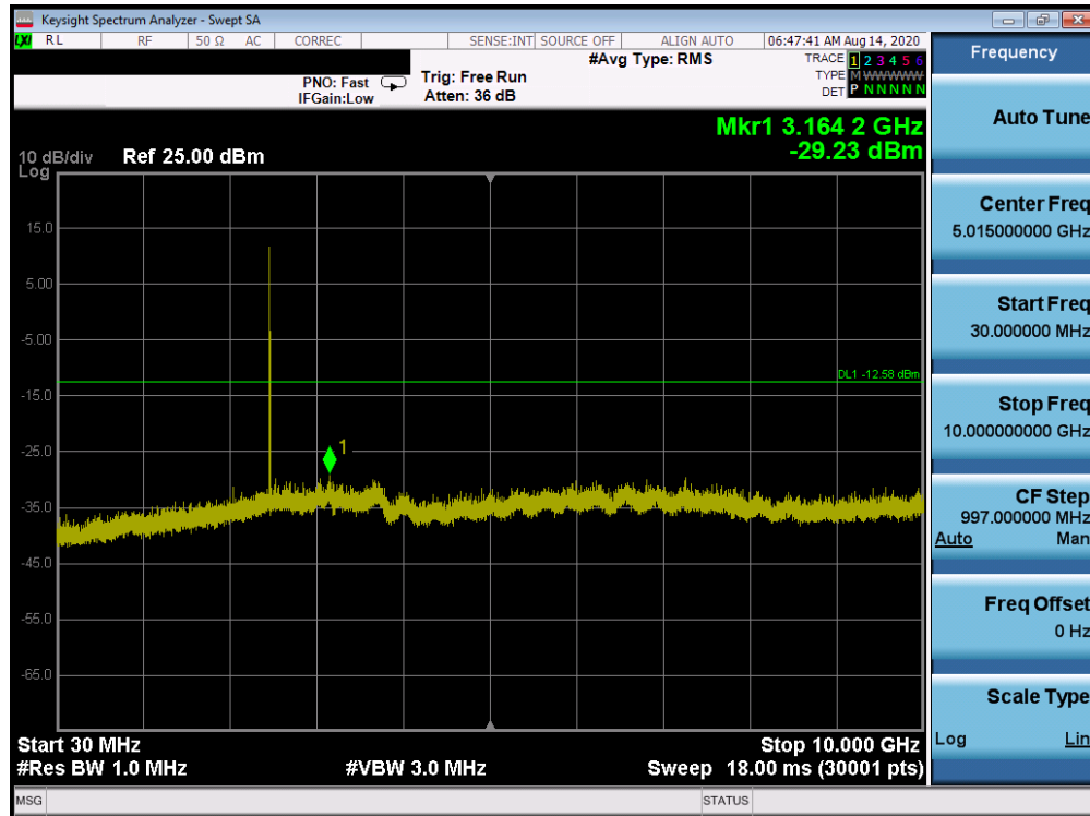
Plot 7-79. Conducted Spurious Plot Antenna 1a (Bluetooth (HDR4), 4 Mbps, ePA – Ch. 75)
