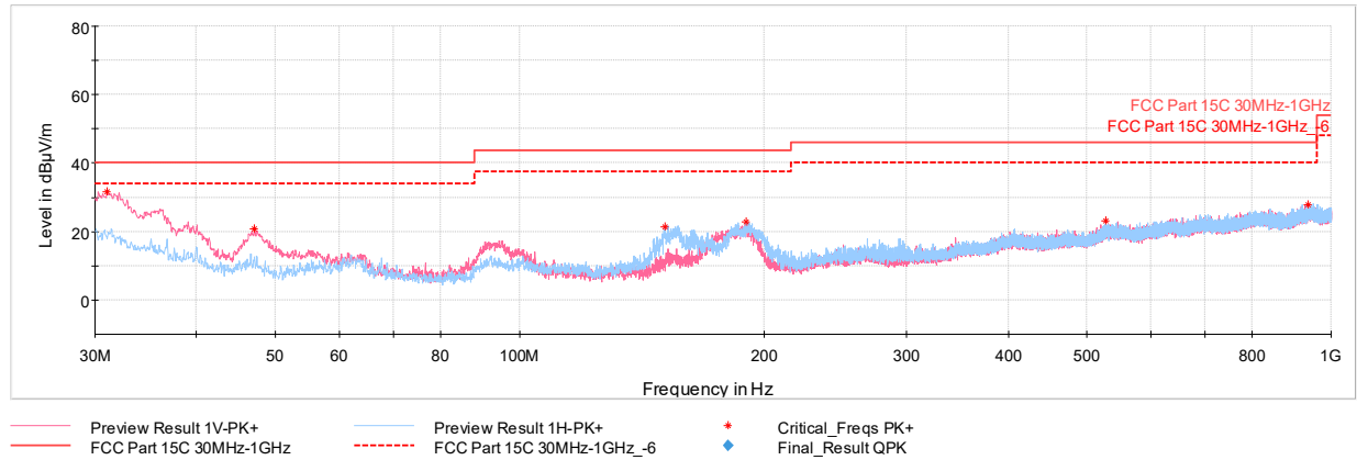
Plot 7-104. Radiated Spurious Emissions below 1GHz TxBF (4Mbps, ePA – Ch.1 with AC/DC Adapter)
