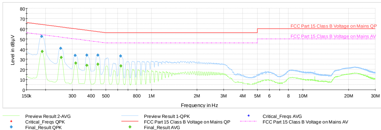
Plot 7-1585. AC Line Conducted Plot with 802.11ax UNII Band 1 – RU26 – Ch. 36 (L1) with Laptop
