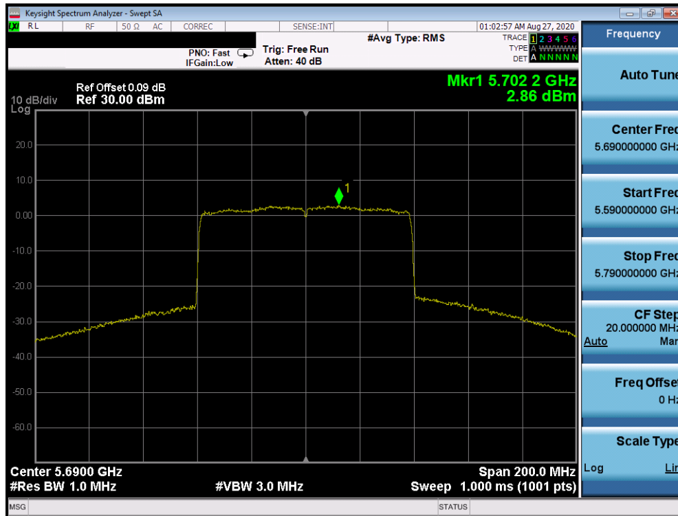
Plot 7-1125. Power Spectral Density Plot CDD Diversity Antenna 2b (80MHz BW 802.11ax – RU996 (UNII Band 2C) – Ch. 138)
