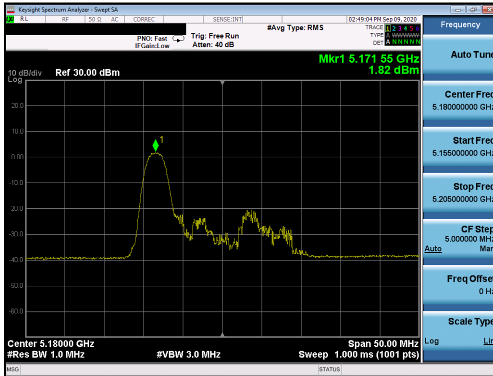
Plot 7-1175. ISED Power Spectral Density Plot SDM Antenna 2b (20MHz BW 802.11ax Index 0 – RU26 (UNII Band 1) – Ch. 36)
