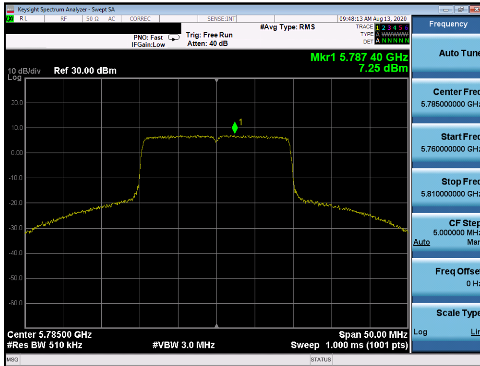
Plot 7-1147. Power Spectral Density Plot CDD Diversity Antenna 2b (20MHz BW 802.11ax– RU242 (UNII Band 3) – Ch. 157)
