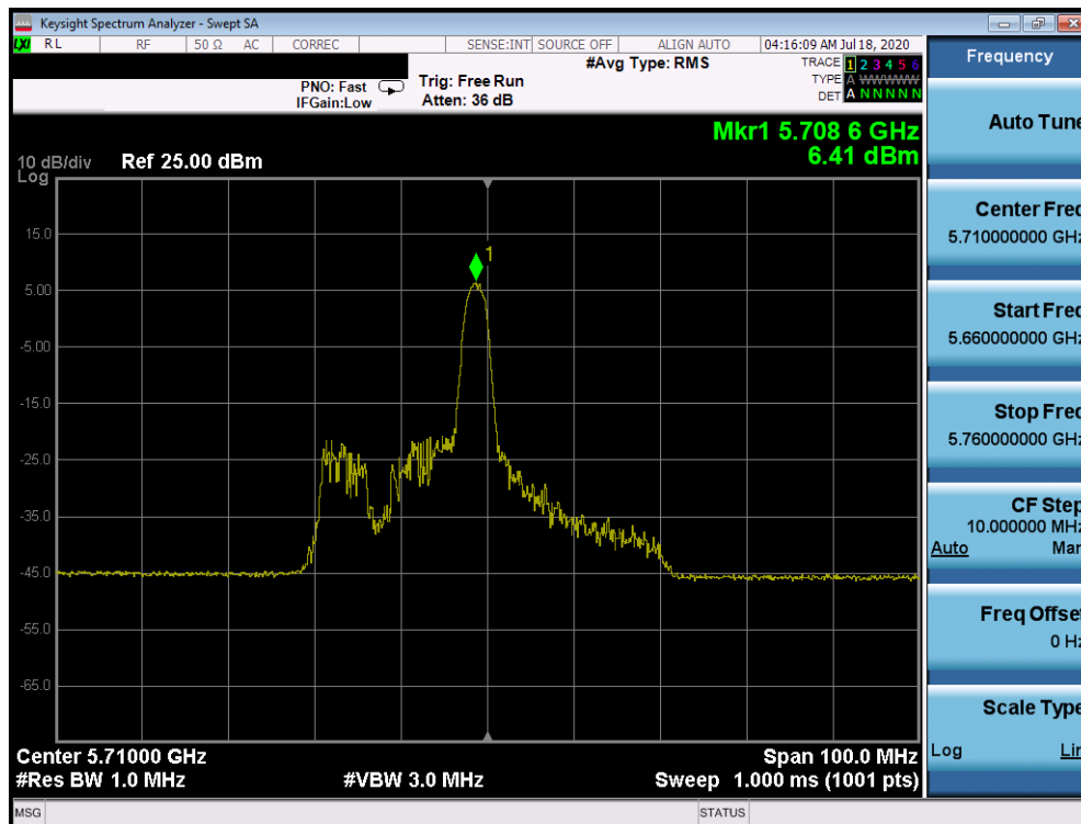
Plot 7-1098. Power Spectral Density Plot CDD Diversity Antenna 1b (40MHz BW 802.11ax Index 8 – RU26 (UNII Band 2C) – Ch. 142)
