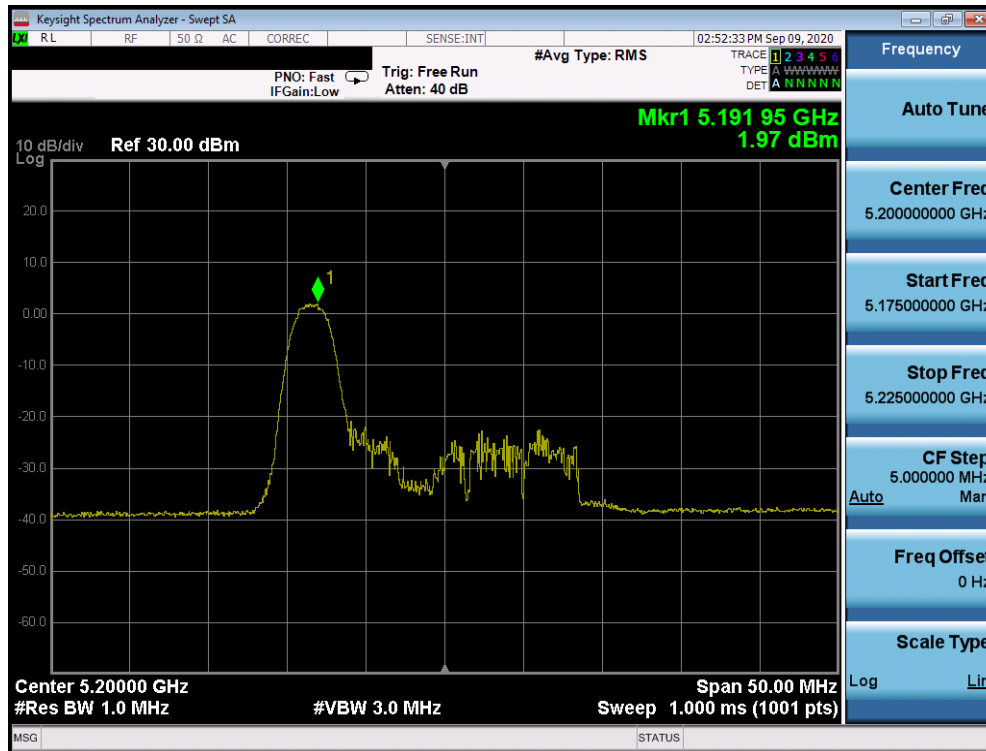
Plot 7-1181. ISED Power Spectral Density Plot SDM Antenna 2b (20MHz BW 802.11ax Index 0 – RU26 (UNII Band 1) – Ch. 40)
