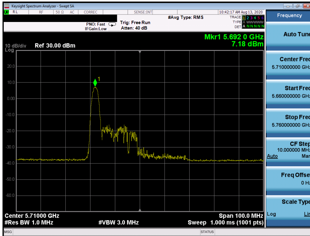
Plot 7-1095. Power Spectral Density Plot CDD Diversity Antenna 2b (40MHz BW 802.11ax Index 0 – RU26 (UNII Band 2C) – Ch. 142)
