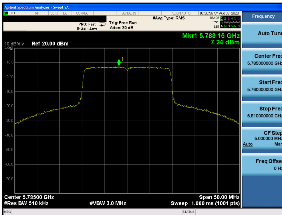
Plot 7-1148. Power Spectral Density Plot CDD Diversity Antenna 1b (20MHz BW 802.11ax– RU242 (UNII Band 3) – Ch. 157)
