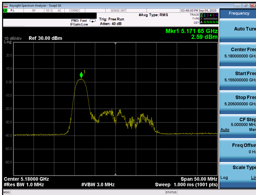
Plot 7-1176. ISED Power Spectral Density Plot SDM Antenna 1b (20MHz BW 802.11ax Index 0 – RU26 (UNII Band 1) – Ch. 36)
