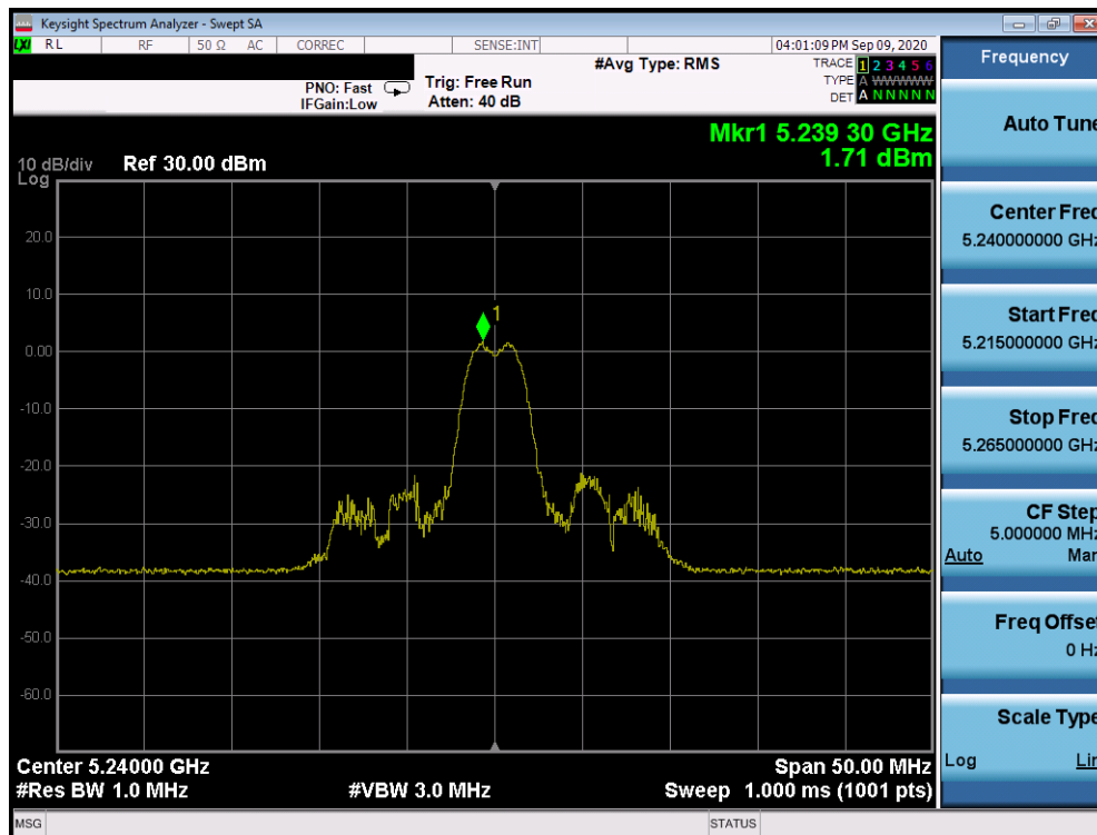
Plot 7-1190. ISED Power Spectral Density Plot SDM Antenna 1b (20MHz BW 802.11ax Index 4 – RU26 (UNII Band 1) – Ch. 48)
