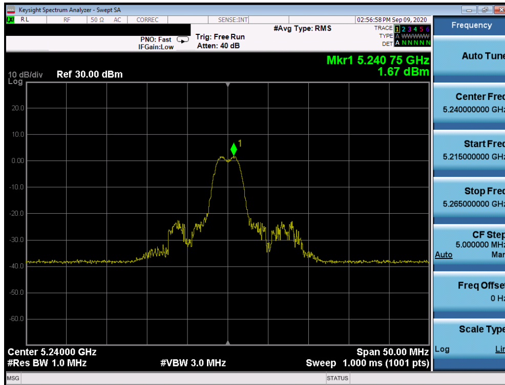
Plot 7-1189. ISED Power Spectral Density Plot SDM Antenna 2b (20MHz BW 802.11ax Index 4 – RU26 (UNII Band 1) – Ch. 48)
