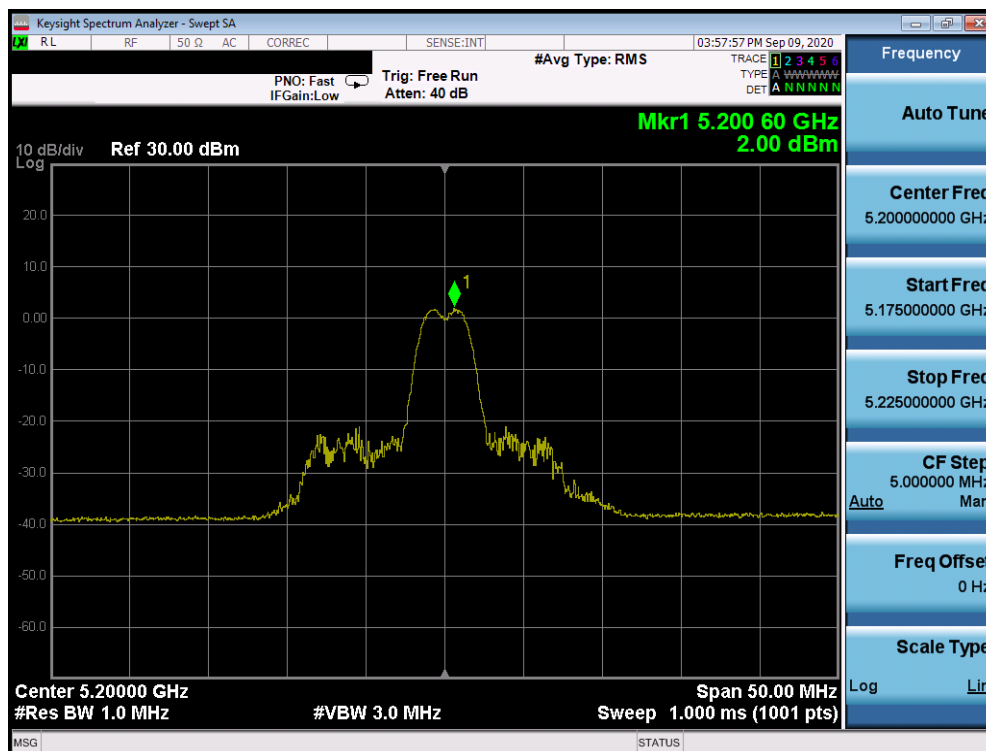
Plot 7-1184. ISED Power Spectral Density Plot SDM Antenna 1b (20MHz BW 802.11ax Index 4 – RU26 (UNII Band 1) – Ch. 40)
