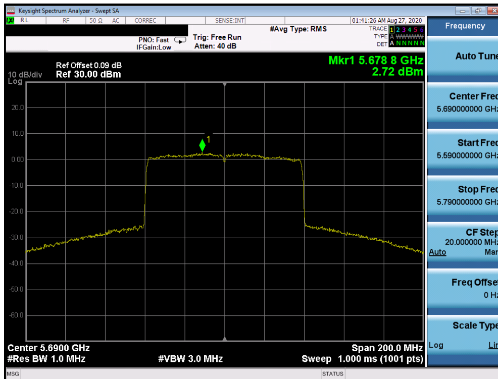
Plot 7-1126. Power Spectral Density Plot CDD Diversity Antenna 1b (80MHz BW 802.11ax – RU996 (UNII Band 2C) – Ch. 138)
