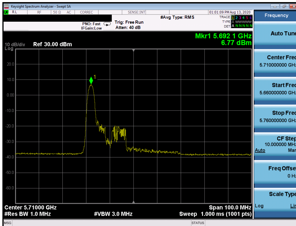
Plot 7-1096. Power Spectral Density Plot CDD Diversity Antenna 1b (40MHz BW 802.11ax Index 0 – RU26 (UNII Band 2C) – Ch. 142)
