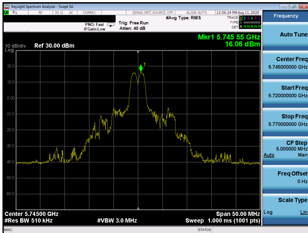
Plot 7-1130. Power Spectral Density Plot CDD Diversity Antenna 1b (20MHz BW 802.11ax Index 4 – RU26 (UNII Band 3) – Ch. 149)
