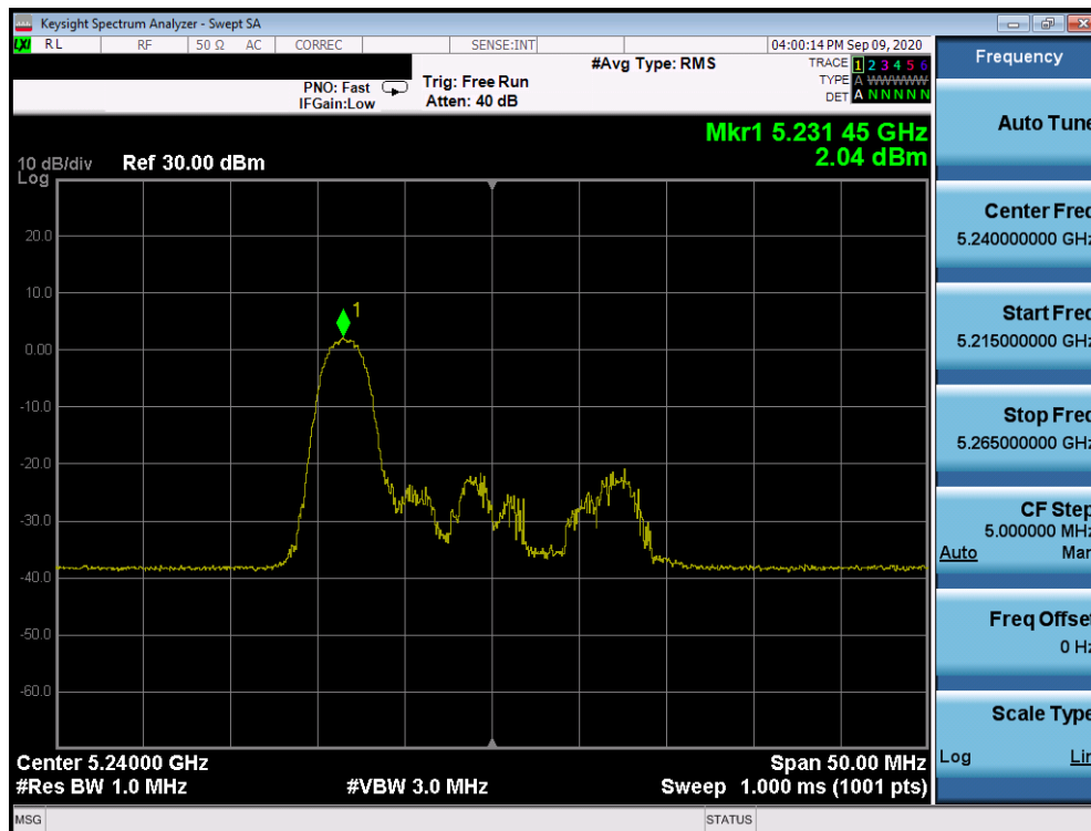
Plot 7-1188. ISED Power Spectral Density Plot SDM Antenna 1b (20MHz BW 802.11ax Index 0 – RU26 (UNII Band 1) – Ch. 48)
