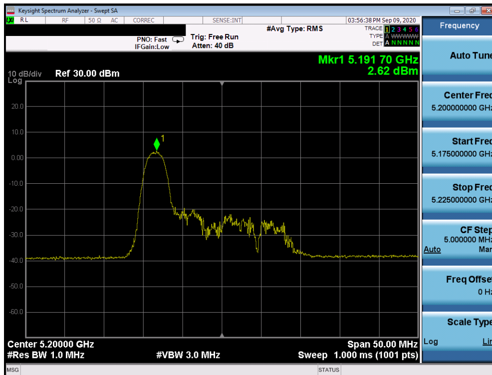
Plot 7-1182. ISED Power Spectral Density Plot SDM Antenna 1b (20MHz BW 802.11ax Index 0 – RU26 (UNII Band 1) – Ch. 40)
