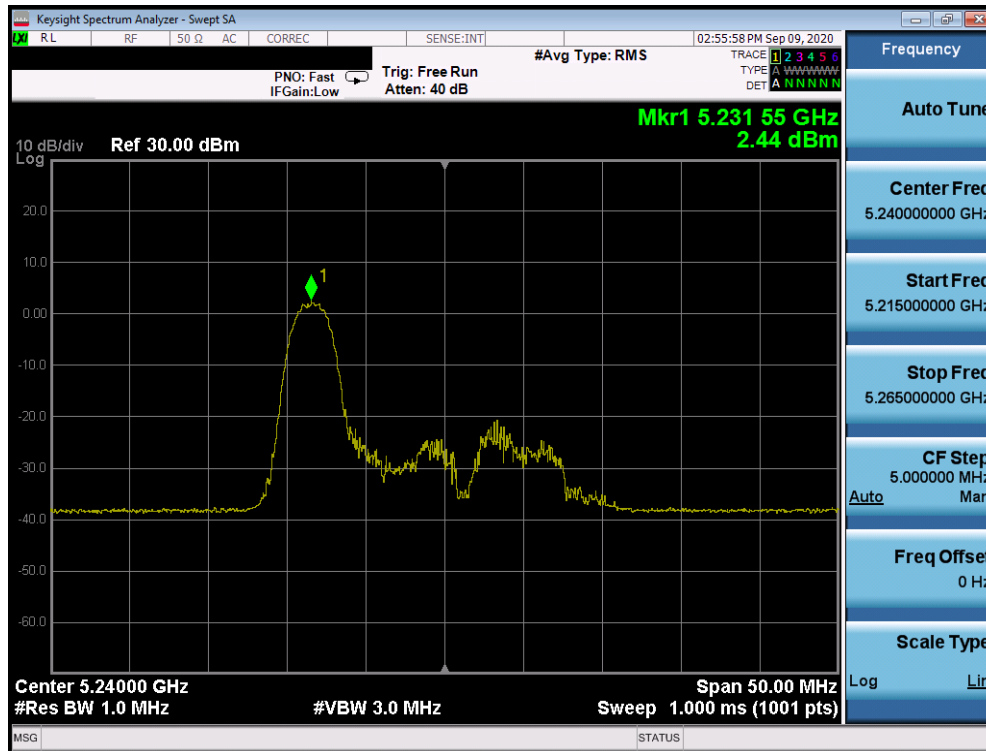
Plot 7-1187. ISED Power Spectral Density Plot SDM Antenna 2b (20MHz BW 802.11ax Index 0 – RU26 (UNII Band 1) – Ch. 48)
