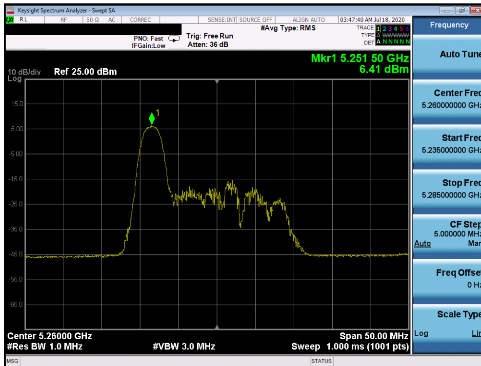
Plot 7-1012. Power Spectral Density Plot CDD Diversity Antenna 1b (20MHz BW 802.11ax Index 0 – RU26 (UNII Band 2A) – Ch. 52)
