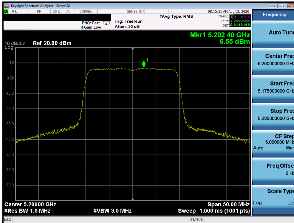
Plot 7-983. Power Spectral Density Plot CDD Diversity Antenna 2b (20MHz BW 802.11ax– RU242 (UNII Band 1) – Ch. 40)
