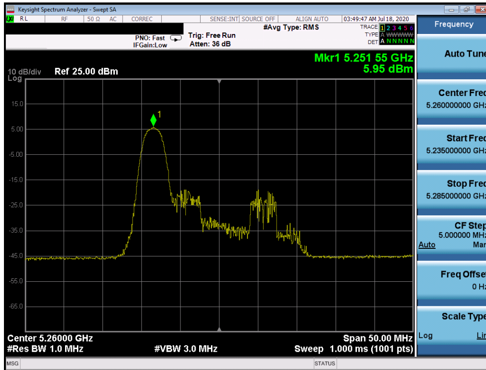
Plot 7-1011. Power Spectral Density Plot CDD Diversity Antenna 2b (20MHz BW 802.11ax Index 0 – RU26 (UNII Band 2A) – Ch. 52)
