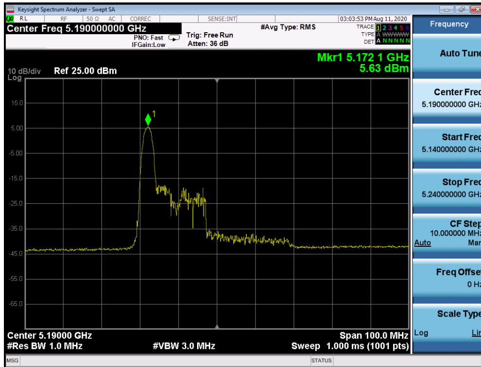
Plot 7-987. Power Spectral Density Plot CDD Diversity Antenna 2b (40MHz BW 802.11ax Index 0 – RU26 (UNII Band 1) – Ch. 38)
