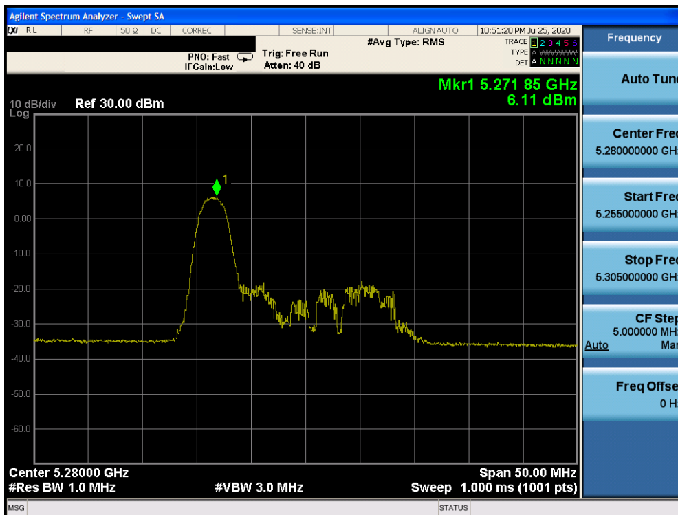
Plot 7-1018. Power Spectral Density Plot CDD Diversity Antenna 1b (20MHz BW 802.11ax Index 0 – RU26 (UNII Band 2A) – Ch. 56)
