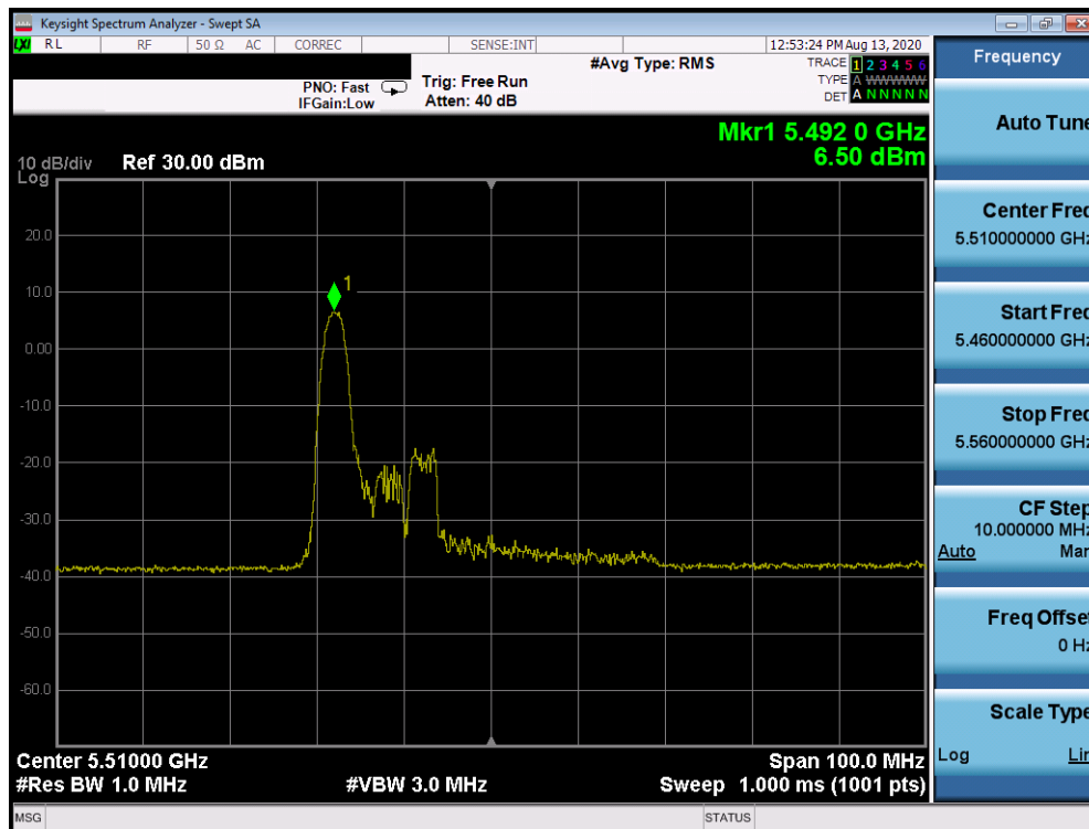
Plot 7-1084. Power Spectral Density Plot CDD Diversity Antenna 1b (40MHz BW 802.11ax Index 0 – RU26 (UNII Band 2C) – Ch. 102)
