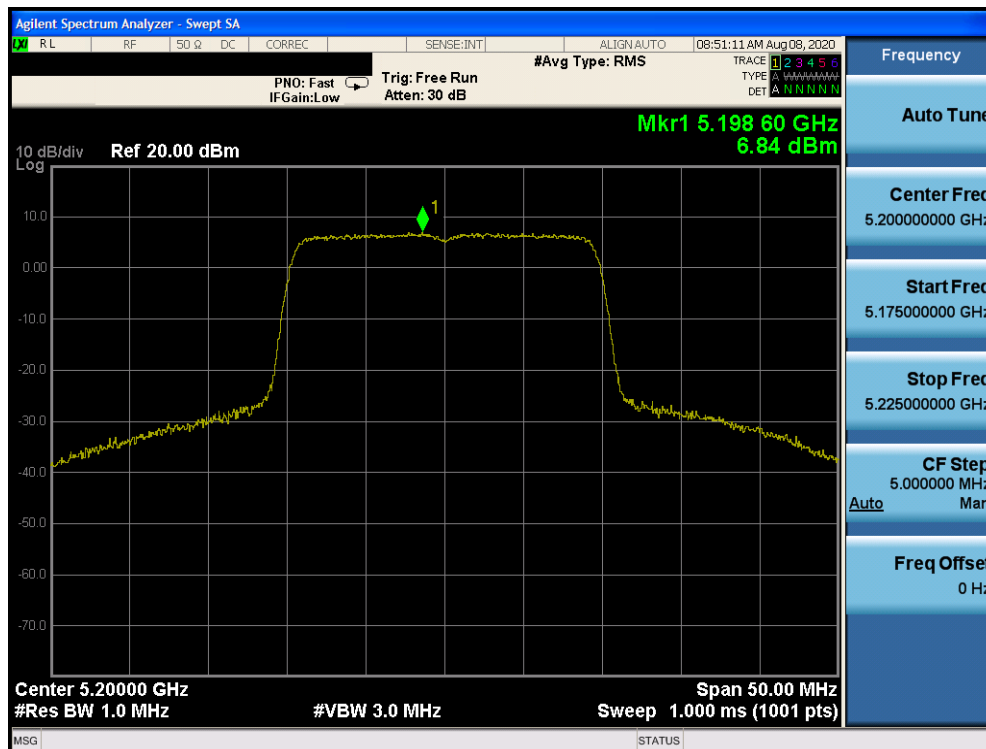
Plot 7-984. Power Spectral Density Plot CDD Diversity Antenna 1b (20MHz BW 802.11ax– RU242 (UNII Band 1) – Ch. 40)
