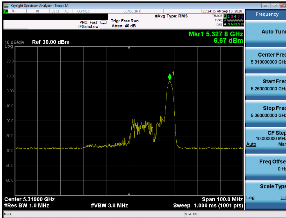
Plot 7-1045. Power Spectral Density Plot CDD Diversity Antenna 2b (40MHz BW 802.11ax Index 17 – RU26 (UNII Band 2A) – Ch. 62)
