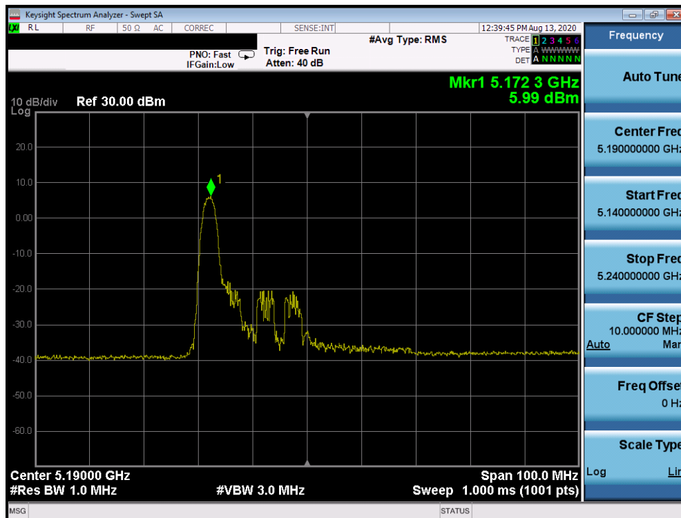
Plot 7-988. Power Spectral Density Plot CDD Diversity Antenna 1b (40MHz BW 802.11ax Index 0 – RU26 (UNII Band 1) – Ch. 38)
