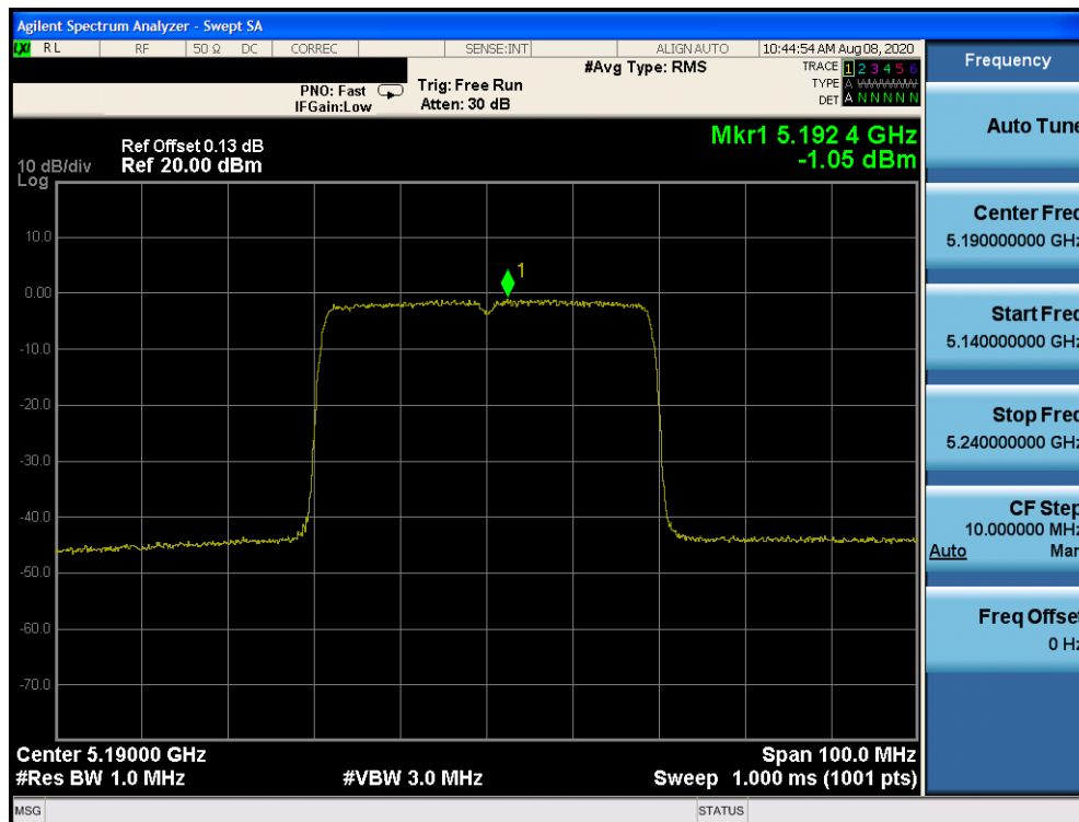
Plot 7-1000. Power Spectral Density Plot CDD Diversity Antenna 1b (40MHz BW 802.11ax – RU484 (UNII Band 1) – Ch. 38)
