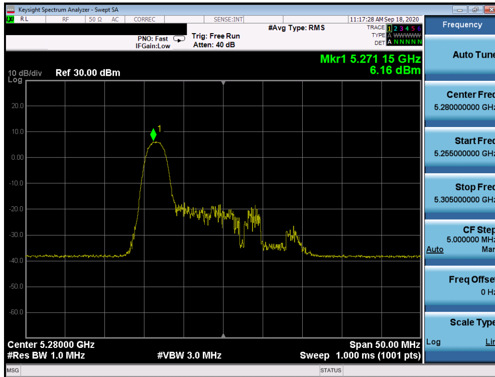
Plot 7-1017. Power Spectral Density Plot CDD Diversity Antenna 2b (20MHz BW 802.11ax Index 0 – RU26 (UNII Band 2A) – Ch. 56)
