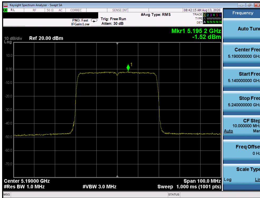
Plot 7-999. Power Spectral Density Plot CDD Diversity Antenna 2b (40MHz BW 802.11ax – RU484 (UNII Band 1) – Ch. 38)
