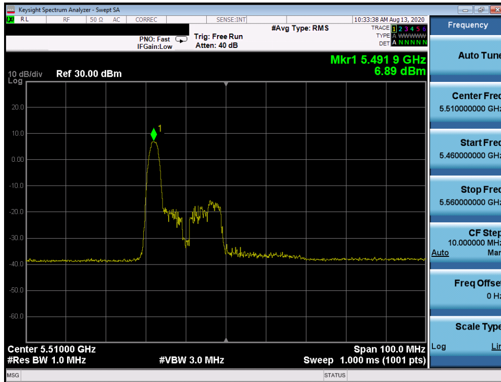
Plot 7-1083. Power Spectral Density Plot CDD Diversity Antenna 2b (40MHz BW 802.11ax Index 0 – RU26 (UNII Band 2C) – Ch. 102)
