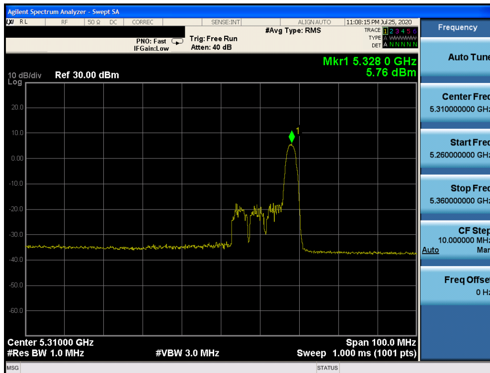
Plot 7-1046. Power Spectral Density Plot CDD Diversity Antenna 1b (40MHz BW 802.11ax Index 17 – RU26 (UNII Band 2A) – Ch. 62)
