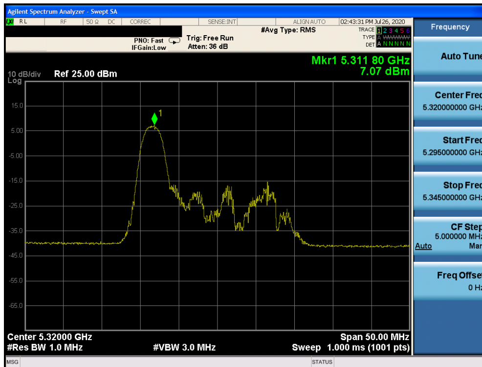
Plot 7-1024. Power Spectral Density Plot CDD Diversity Antenna 1b (20MHz BW 802.11ax Index 0 – RU26 (UNII Band 2A) – Ch. 64)
