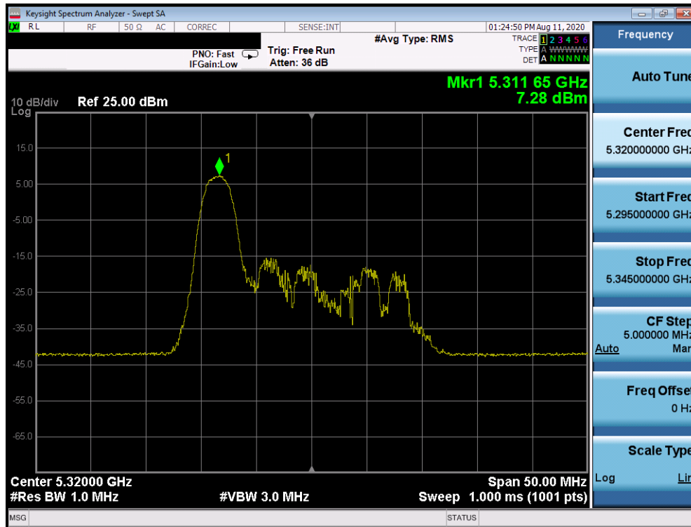
Plot 7-1023. Power Spectral Density Plot CDD Diversity Antenna 2b (20MHz BW 802.11ax Index 0 – RU26 (UNII Band 2A) – Ch. 64)
