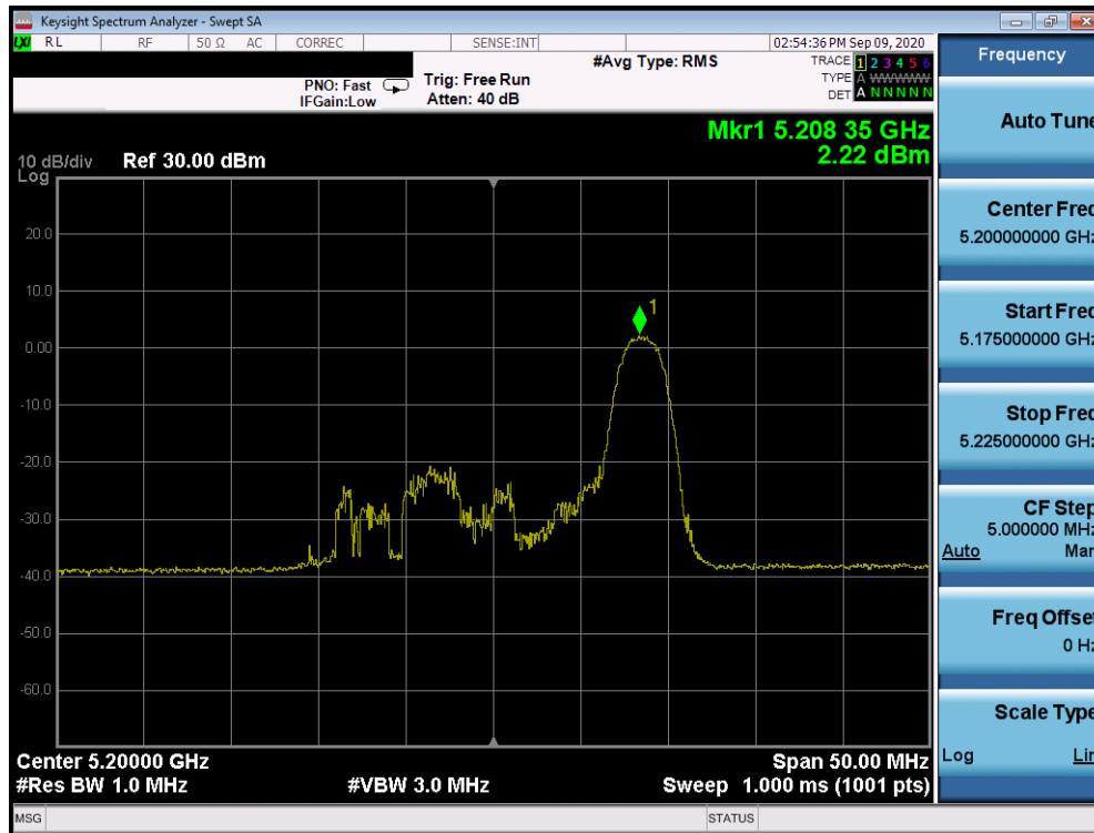
Plot 7-925. ISED Power Spectral Density Plot SDM Antenna 2b (20MHz BW 802.11ax Index 8– RU26 (UNII Band 1) – Ch. 40)
