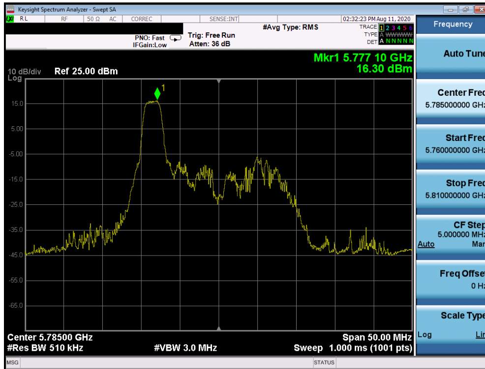
Plot 7-873. Power Spectral Density Plot CDD Primary Antenna 2b (20MHz BW 802.11ax Index 0 – RU26 (UNII Band 3) – Ch. 157)
