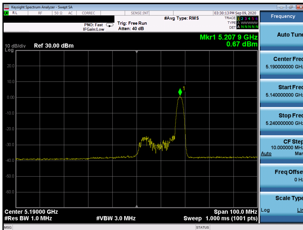
Plot 7-944. ISED Power Spectral Density Plot SDM Antenna 2a (40MHz BW 802.11ax Index 17 – RU26 (UNII Band 1) – Ch. 38)
