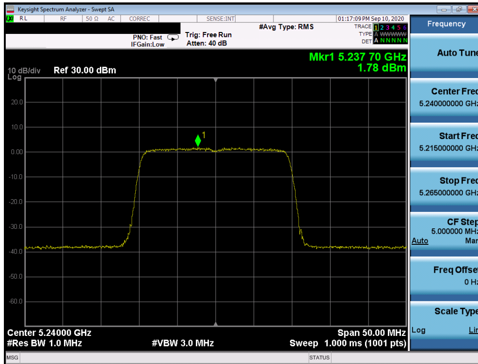
Plot 7-937. ISED Power Spectral Density Plot SDM Antenna 2b (20MHz BW 802.11ax- RU242 (UNII Band 1) – Ch. 48)
