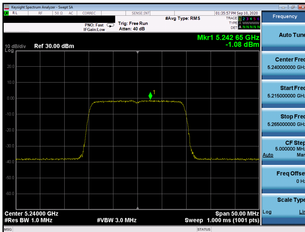
Plot 7-938. ISED Power Spectral Density Plot SDM Antenna 2a (20MHz BW 802.11ax- RU242 (UNII Band 1) – Ch. 48)
