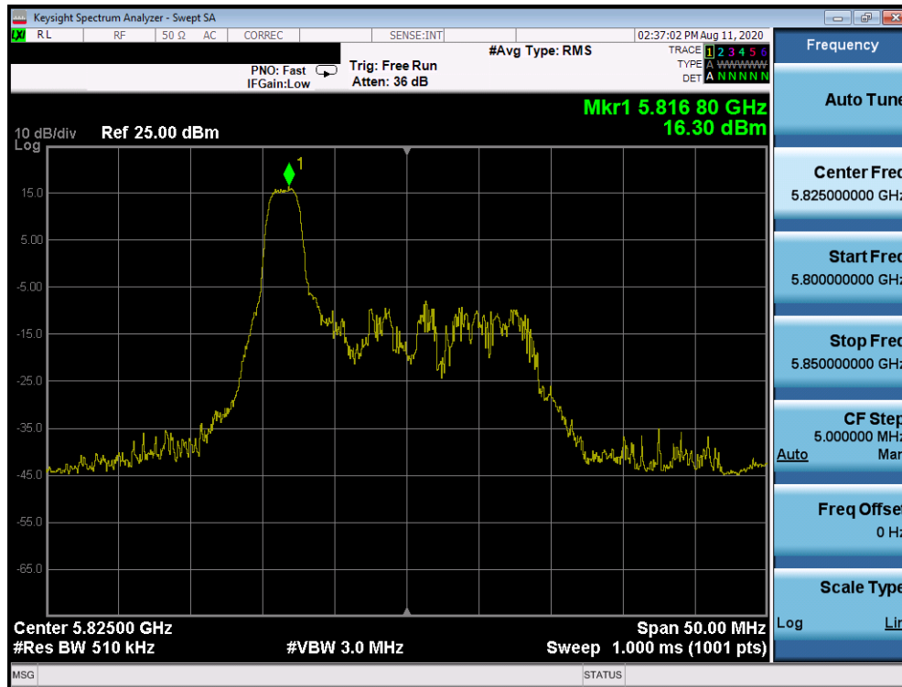
Plot 7-879. Power Spectral Density Plot CDD Primary Antenna 2b (20MHz BW 802.11ax Index 0 – RU26 (UNII Band 3) – Ch. 165)
