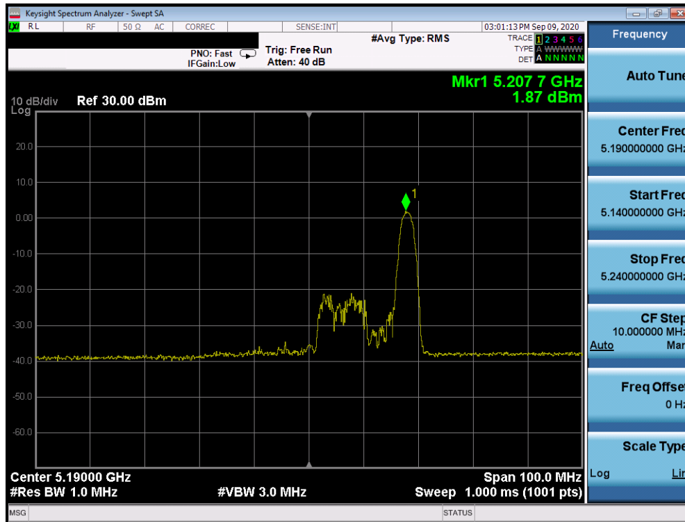
Plot 7-943. ISED Power Spectral Density Plot SDM Antenna 2b (40MHz BW 802.11ax Index 17 – RU26 (UNII Band 1) – Ch. 38)
