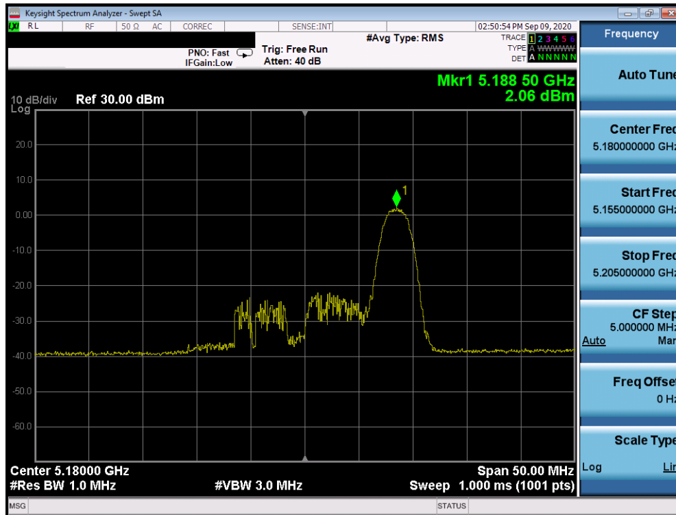
Plot 7-919. ISED Power Spectral Density Plot SDM Antenna 2b (20MHz BW 802.11ax Index 8 – RU26 (UNII Band 1) – Ch. 36)
