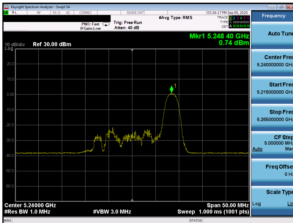
Plot 7-932. ISD Power Spectral Density Plot SDM Antenna 2a (20MHz BW 802.11ax Index 8 – RU26 (UNII Band 1) – Ch. 48)
