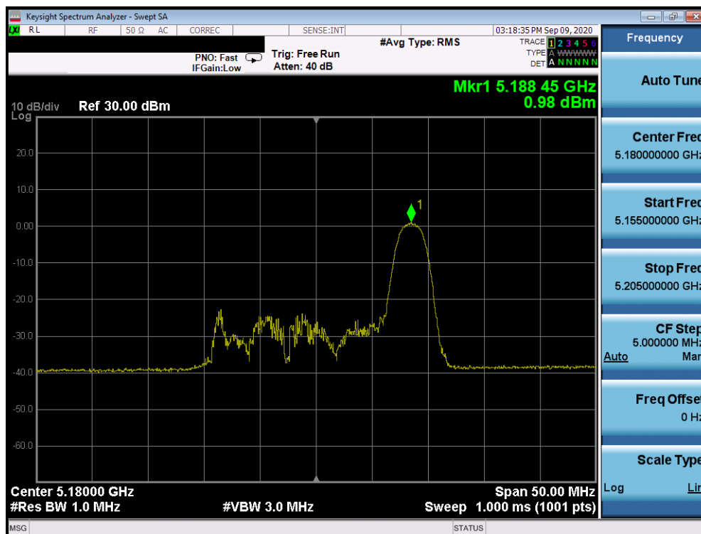
Plot 7-920. ISED Power Spectral Density Plot SDM Antenna 2a (20MHz BW 802.11ax Index 8 – RU26 (UNII Band 1) – Ch. 36)
