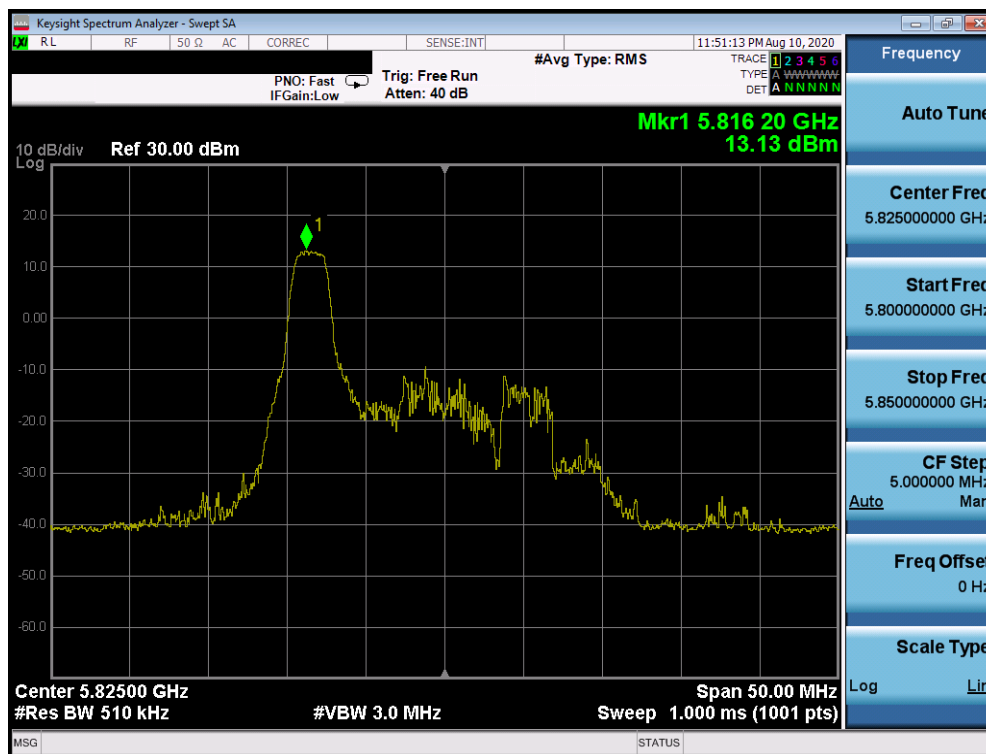
Plot 7-880. Power Spectral Density Plot CDD Primary Antenna 2a (20MHz BW 802.11ax Index 0 – RU26 (UNII Band 3) – Ch. 165)
