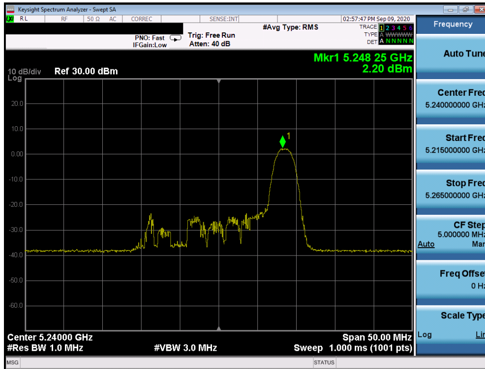
Plot 7-931. ISD Power Spectral Density Plot SDM Antenna 2b (20MHz BW 802.11ax Index 8 – RU26 (UNII Band 1) – Ch. 48)
