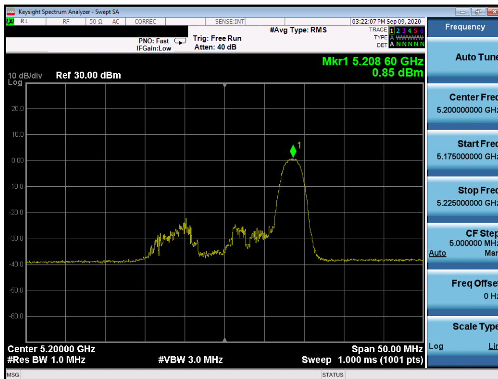
Plot 7-926. ISED Power Spectral Density Plot SDM Antenna 2a (20MHz BW 802.11ax Index 8– RU26 (UNII Band 1) – Ch. 40)
