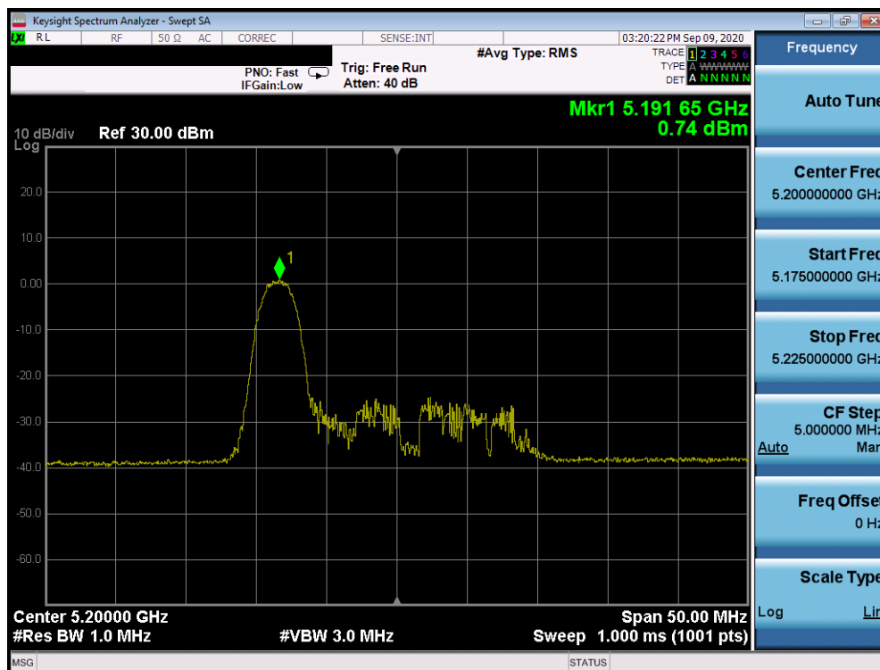
Plot 7-922. ISED Power Spectral Density Plot SDM Antenna 2a (20MHz BW 802.11ax Index 0 – RU26 (UNII Band 1) – Ch. 40)
