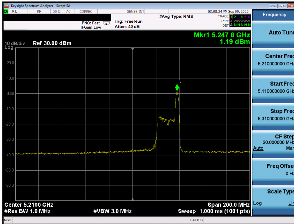
Plot 7-959. ISED Power Spectral Density Plot CDD Antenna 2b (80MHz BW 802.11ax Index 36 – RU26 (UNII Band 1) – Ch. 42)
