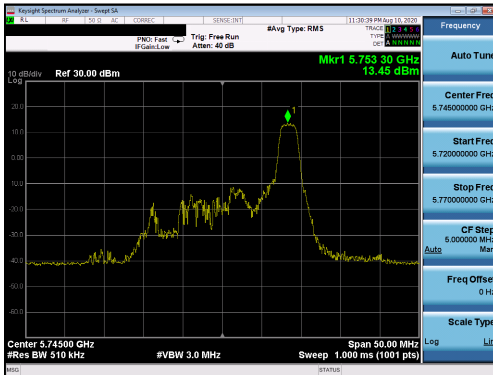
Plot 7-872. Power Spectral Density Plot CDD Primary Antenna 2a (20MHz BW 802.11ax Index 8 – RU26 (UNII Band 3) – Ch. 149)
