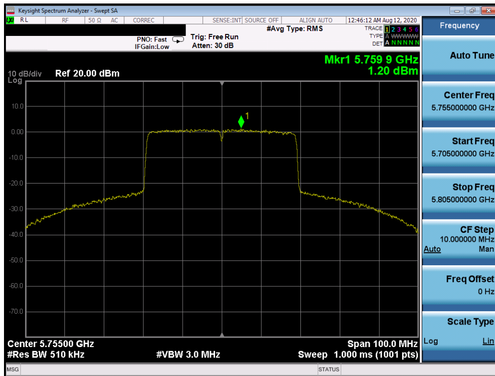
Plot 7-904. Power Spectral Density Plot CDD Primary Antenna 2a (40MHz BW 802.11ax – RU484 (UNII Band 3) – Ch. 151)
