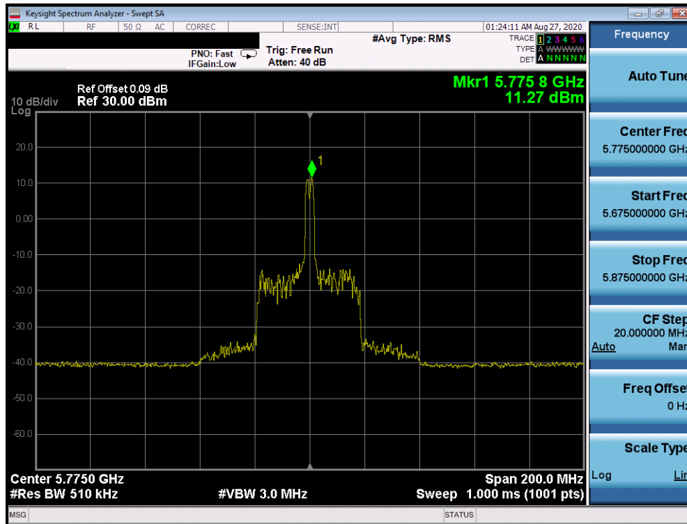
Plot 7-909. Power Spectral Density Plot CDD Primary Antenna 2b (80MHz BW 802.11ax Index 18 – RU26 (UNII Band 3) – Ch. 155)
