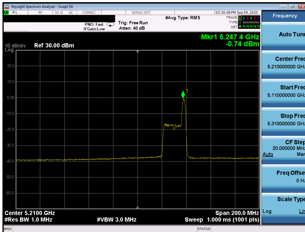
Plot 7-960. ISED Power Spectral Density Plot CDD Antenna 2a (80MHz BW 802.11ax Index 36 – RU26 (UNII Band 1) – Ch. 42)
