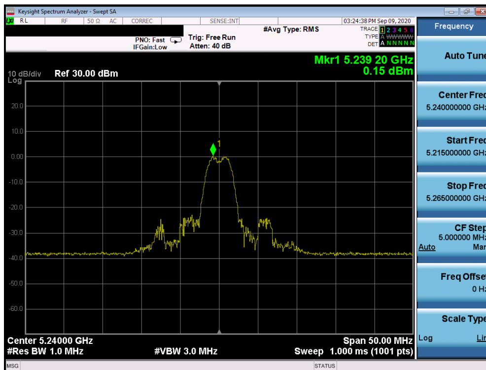
Plot 7-930. ISED Power Spectral Density Plot SDM Antenna 2a (20MHz BW 802.11ax Index 4 – RU26 (UNII Band 1) – Ch. 48)
