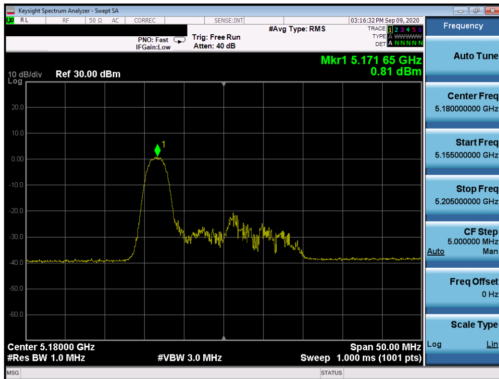
Plot 7-916. ISD Power Spectral Density Plot SDM Antenna 2a (20MHz BW 802.11ax Index 0 – RU26 (UNII Band 1) – Ch. 36)
