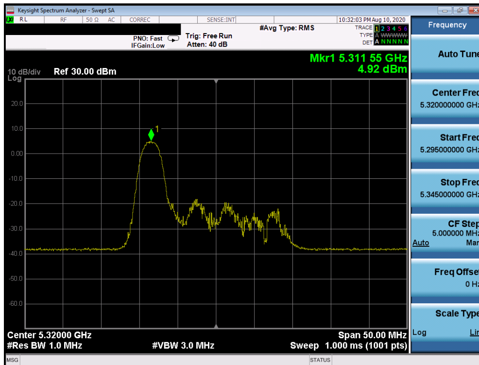
Plot 7-764. Power Spectral Density Plot CDD Primary Antenna 2a (20MHz BW 802.11ax Index 0 – RU26 (UNII Band 2A) – Ch. 64)
