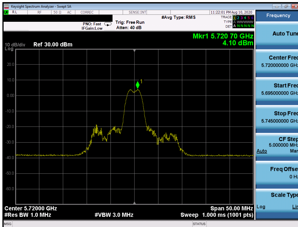
Plot 7-814. Power Spectral Density Plot CDD Primary Antenna 2a (20MHz BW 802.11ax Index 4 – RU26 (UNII Band 2C) – Ch. 144)
