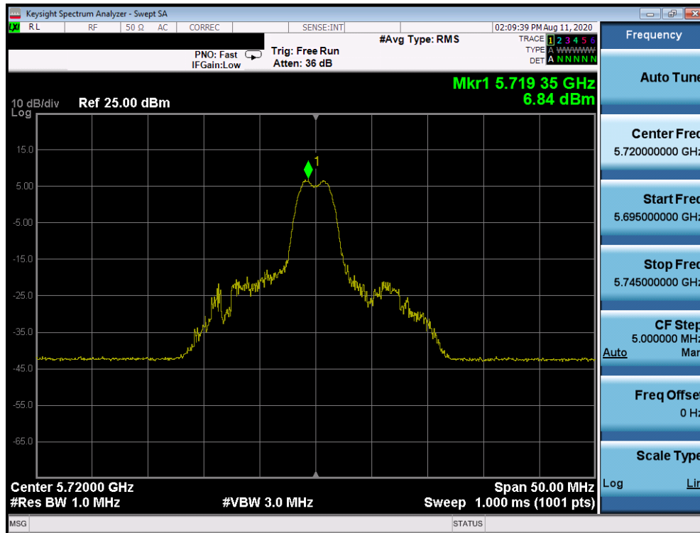
Plot 7-813. Power Spectral Density Plot CDD Primary Antenna 2b (20MHz BW 802.11ax Index 4 – RU26 (UNII Band 2C) – Ch. 144)
