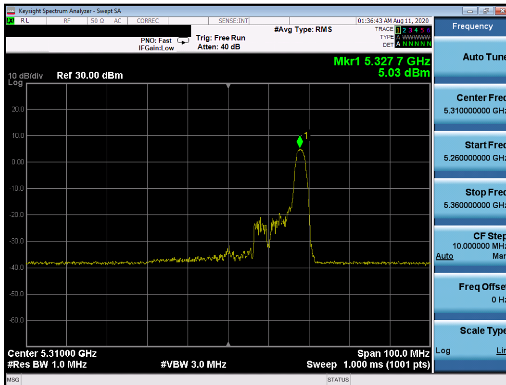
Plot 7-786. Power Spectral Density Plot CDD Primary Antenna 2a (40MHz BW 802.11ax Index 17 – RU26 (UNII Band 2A) – Ch. 62)
