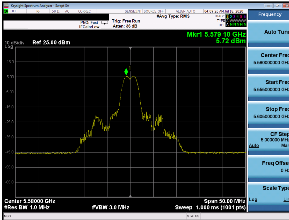
Plot 7-807. Power Spectral Density Plot CDD Primary Antenna 2b (20MHz BW 802.11ax Index 4 – RU26 (UNII Band 2C) – Ch. 116)
