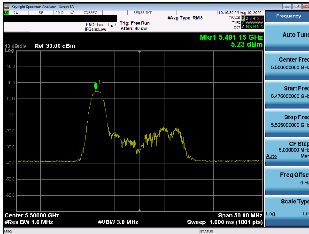
Plot 7-800. Power Spectral Density Plot CDD Primary Antenna 2a (20MHz BW 802.11ax Index 0 – RU26 (UNII Band 2C) – Ch. 100)
