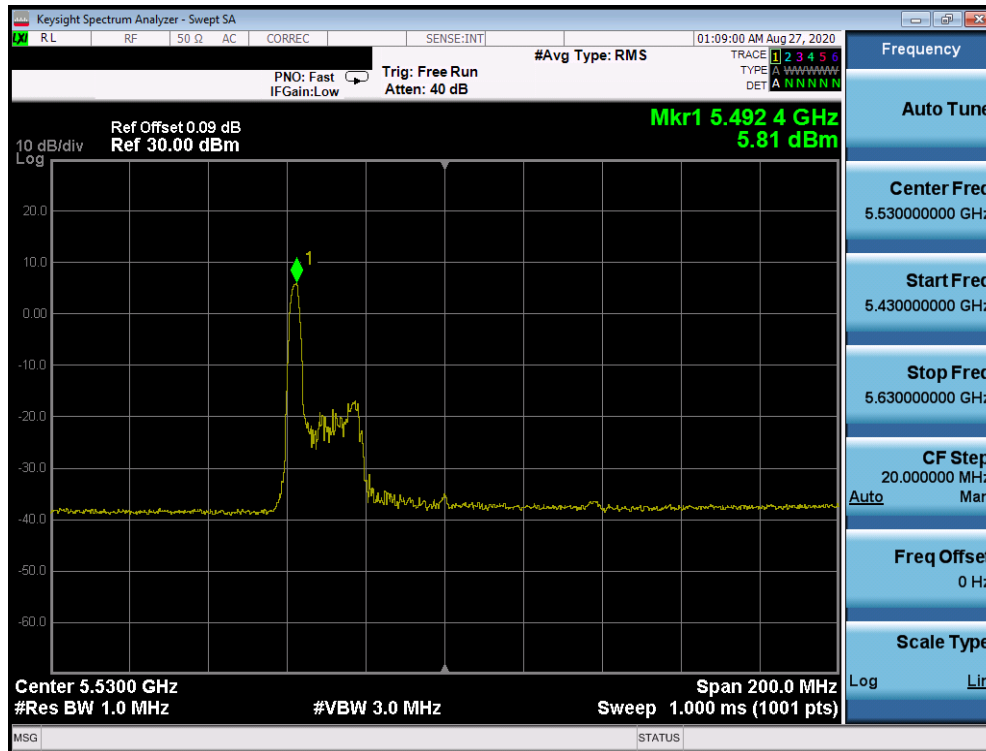
Plot 7-849. Power Spectral Density Plot CDD Primary Antenna 2b (80MHz BW 802.11ax Index 0 – RU26 (UNII Band 2C) – Ch. 106)
