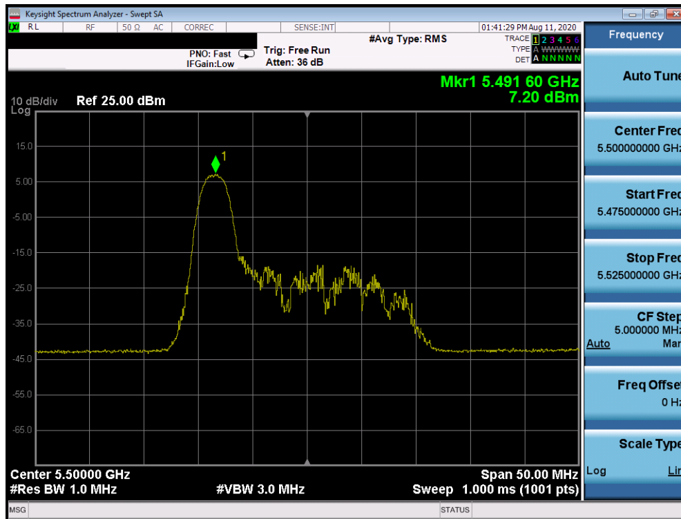
Plot 7-799. Power Spectral Density Plot CDD Primary Antenna 2b (20MHz BW 802.11ax Index 0 – RU26 (UNII Band 2C) – Ch. 100)
