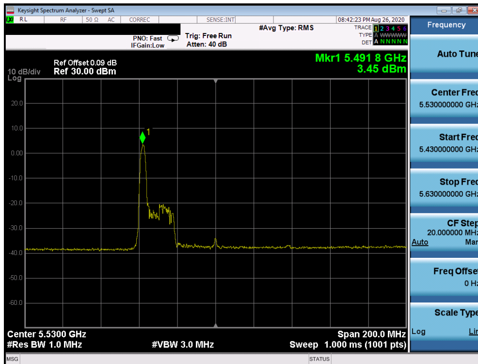
Plot 7-850. Power Spectral Density Plot CDD Primary Antenna 2a (80MHz BW 802.11ax Index 0 – RU26 (UNII Band 2C) – Ch. 106)
