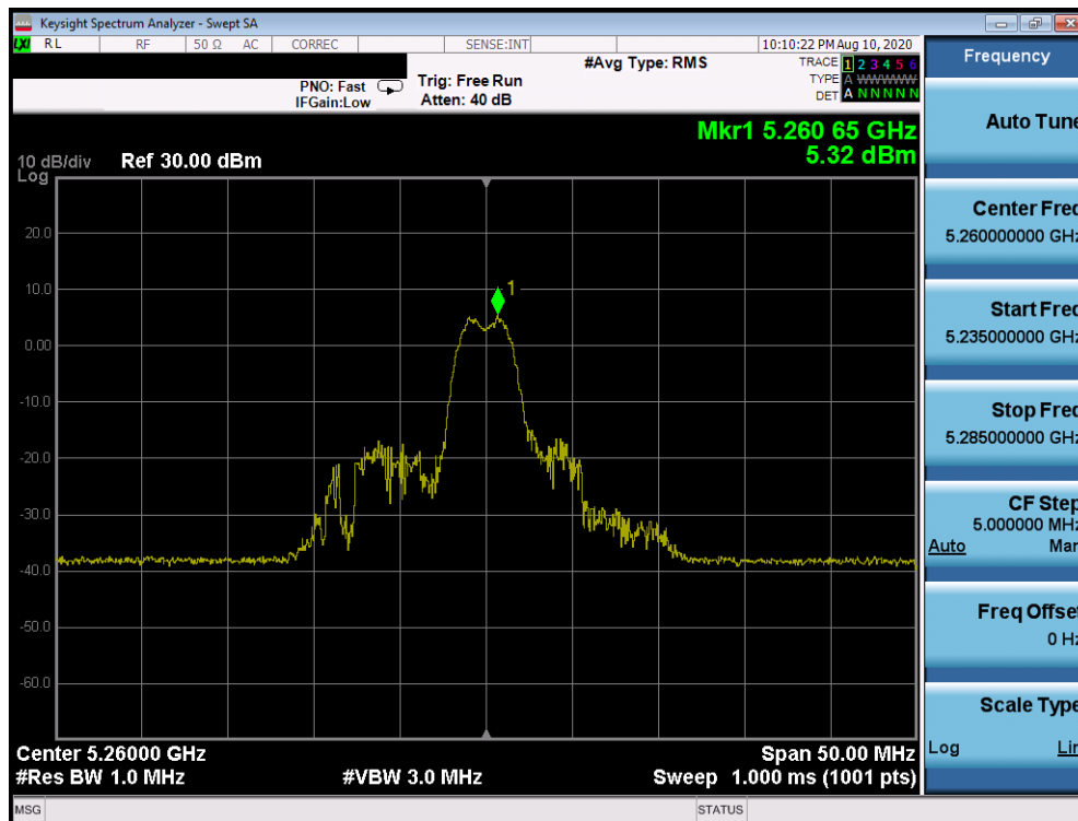
Plot 7-754. Power Spectral Density Plot CDD Primary Antenna 2a (20MHz BW 802.11ax Index 4 – RU26 (UNII Band 2A) – Ch. 52)
