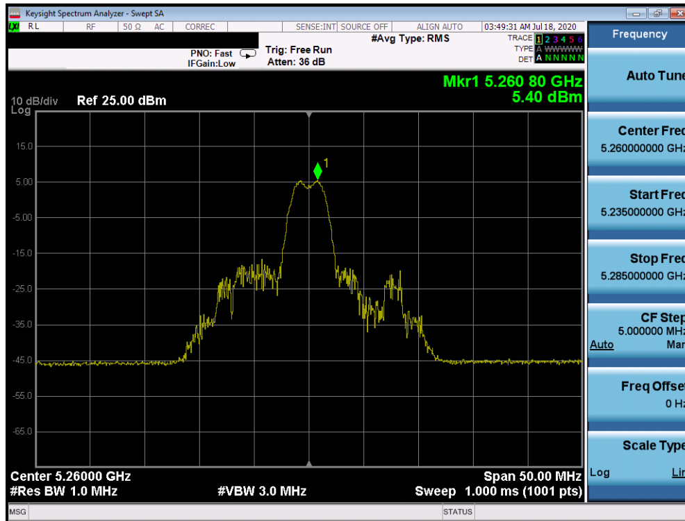
Plot 7-753. Power Spectral Density Plot CDD Primary Antenna 2b (20MHz BW 802.11ax Index 4 – RU26 (UNII Band 2A) – Ch. 52)
