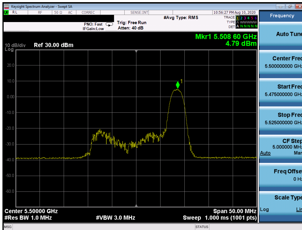
Plot 7-804. Power Spectral Density Plot CDD Primary Antenna 2a (20MHz BW 802.11ax Index 8 – RU26 (UNII Band 2C) – Ch. 100)
