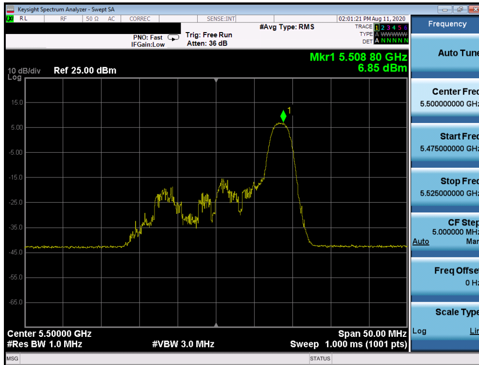
Plot 7-803. Power Spectral Density Plot CDD Primary Antenna 2b (20MHz BW 802.11ax Index 8 – RU26 (UNII Band 2C) – Ch. 100)
