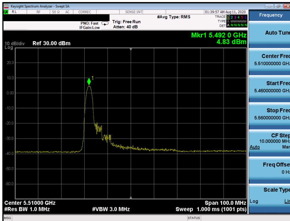
Plot 7-824. Power Spectral Density Plot CDD Primary Antenna 2a (40MHz BW 802.11ax Index 0 – RU26 (UNII Band 2C) – Ch. 102)
