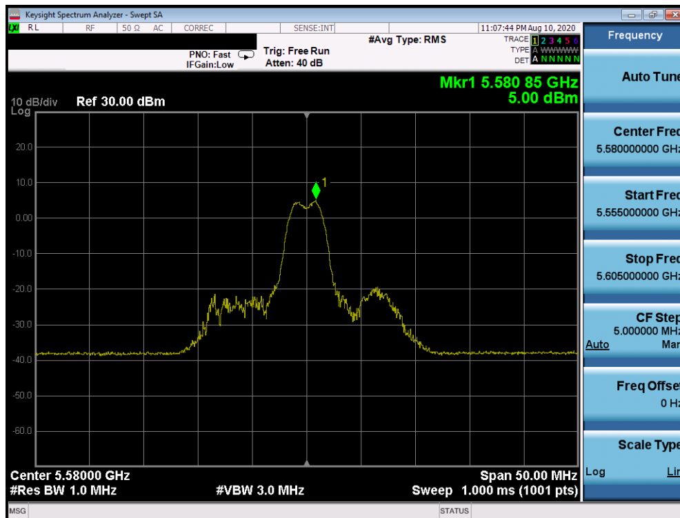
Plot 7-808. Power Spectral Density Plot CDD Primary Antenna 2a (20MHz BW 802.11ax Index 4 – RU26 (UNII Band 2C) – Ch. 116)
