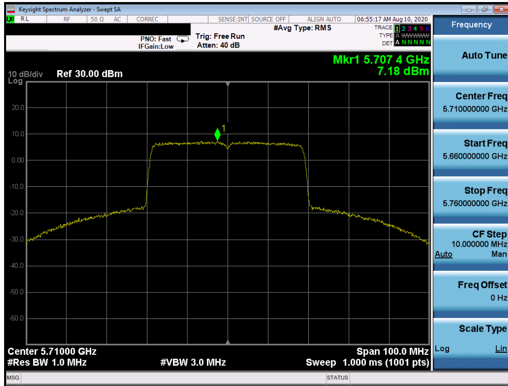
Plot 7-645. Power Spectral Density Plot Antenna 1b (40MHz BW 802.11ax – RU484 (UNII Band 2C) – Ch. 142)
