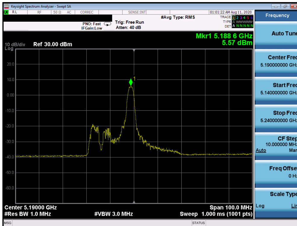
Plot 7-730. Power Spectral Density Plot CDD Primary Antenna 2a (40MHz BW 802.11ax Index 8 – RU26 (UNII Band 1) – Ch. 38)
