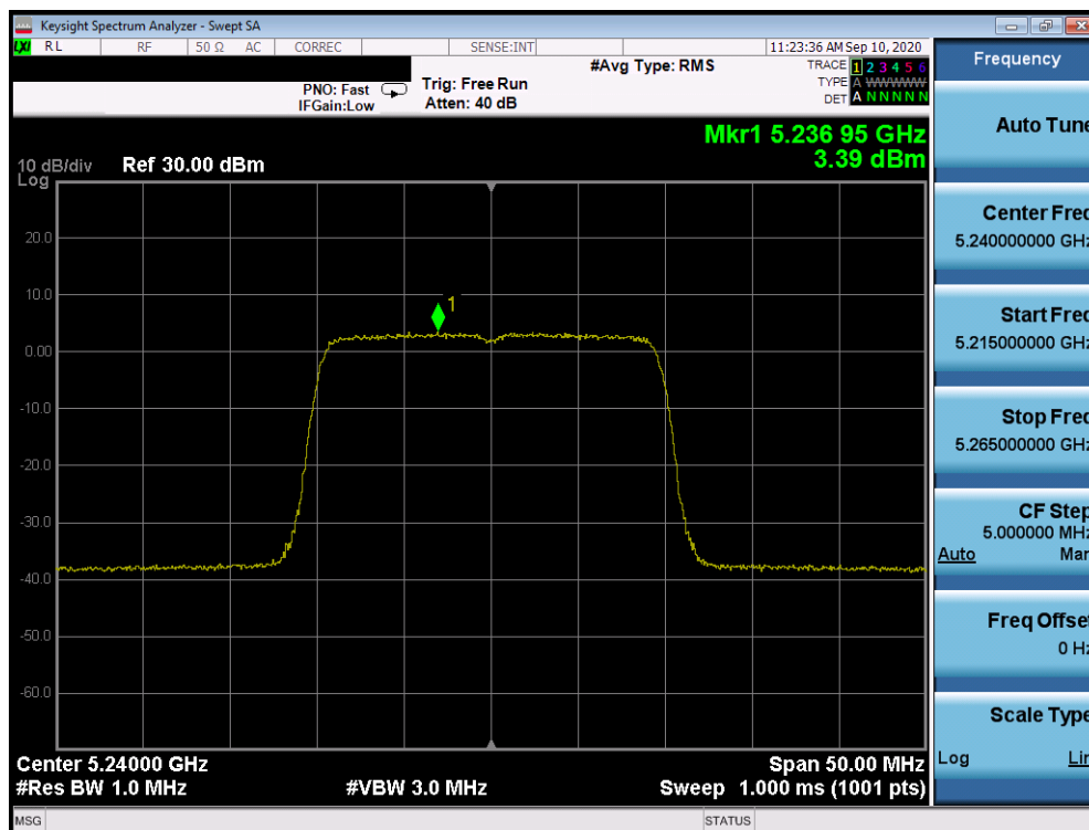
Plot 7-690. ISD Power Spectral Density Plot Antenna 1b (20MHz BW 802.11ax– RU242 (UNII Band 1) – Ch. 48)
