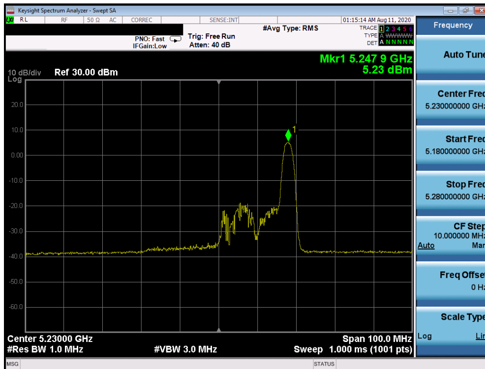
Plot 7-738. Power Spectral Density Plot CDD Primary Antenna 2a (40MHz BW 802.11ax Index 17 – RU26 (UNII Band 1) – Ch. 46)
