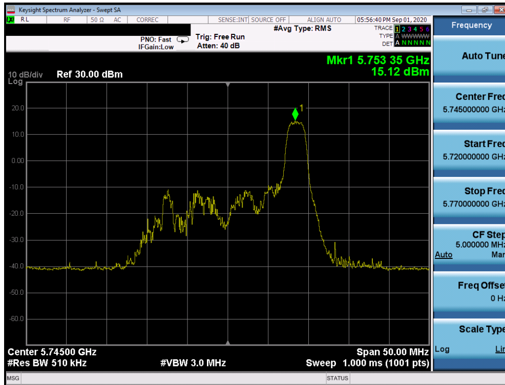
Plot 7-657. Power Spectral Density Plot Antenna 1b (20MHz BW 802.11ax Index 8 – RU26 (UNII Band 3) – Ch. 149)
