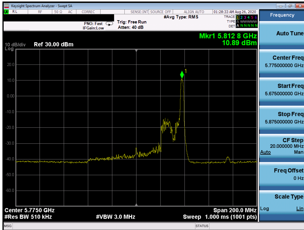
Plot 7-677. Power Spectral Density Plot Antenna 1b (80MHz BW 802.11ax Index 36 – RU26 (UNII Band 3) – Ch. 155)
