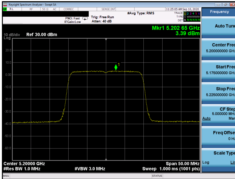
Plot 7-689. ISD Power Spectral Density Plot Antenna 1b (20MHz BW 802.11ax– RU242 (UNII Band 1) – Ch. 40)
