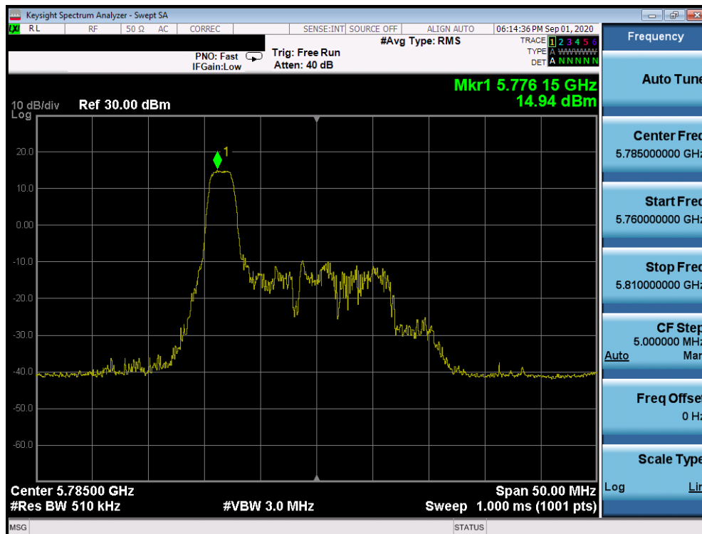
Plot 7-658. Power Spectral Density Plot Antenna 1b (20MHz BW 802.11ax Index 0 – RU26 (UNII Band 3) – Ch. 157)
