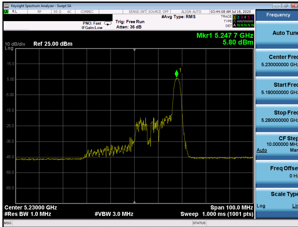
Plot 7-737. Power Spectral Density Plot CDD Primary Antenna 2b (40MHz BW 802.11ax Index 17 – RU26 (UNII Band 1) – Ch. 46)
