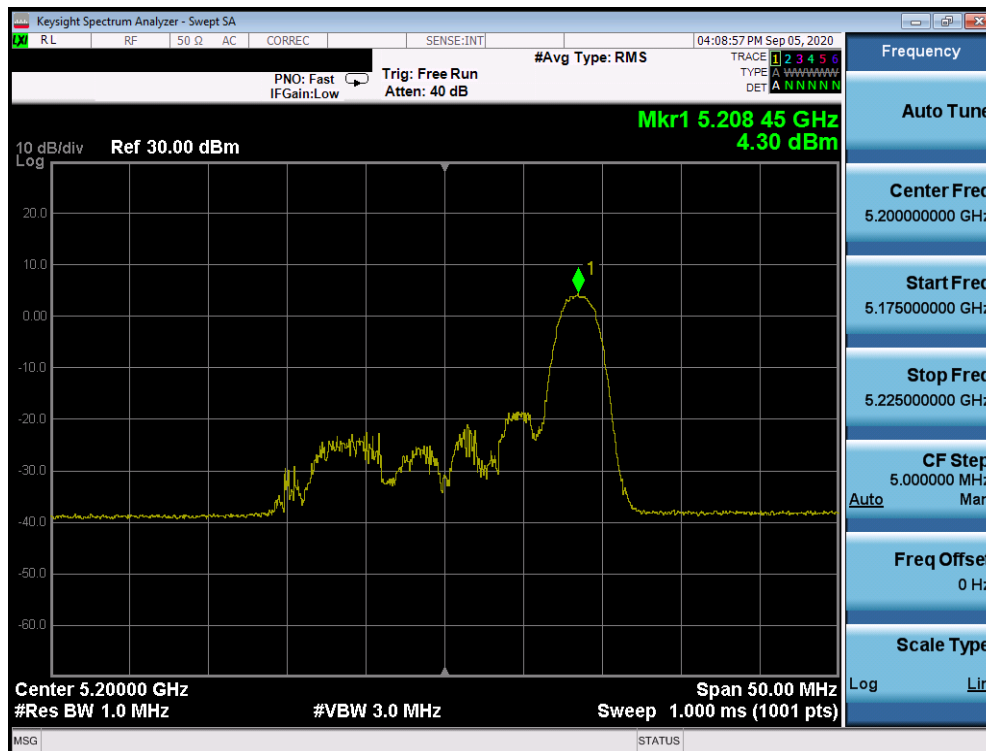
Plot 7-684. ISD Power Spectral Density Plot Antenna 1b (20MHz BW 802.11ax Index 8– RU26 (UNII Band 1) – Ch. 40)
