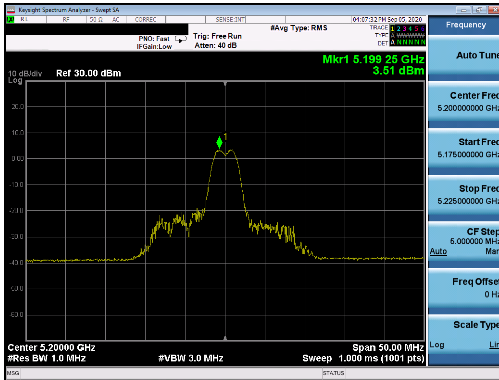
Plot 7-683. ISD Power Spectral Density Plot Antenna 1b (20MHz BW 802.11ax Index 4 – RU26 (UNII Band 1) – Ch. 40)
