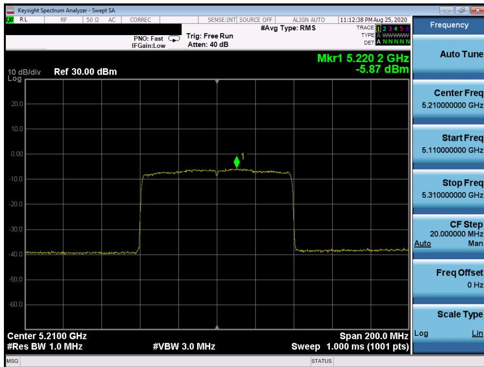
Plot 7-572. ISD Power Spectral Density Plot Antenna 2a (80MHz BW 802.11ax – RU996 (UNII Band 1) – Ch. 42)
