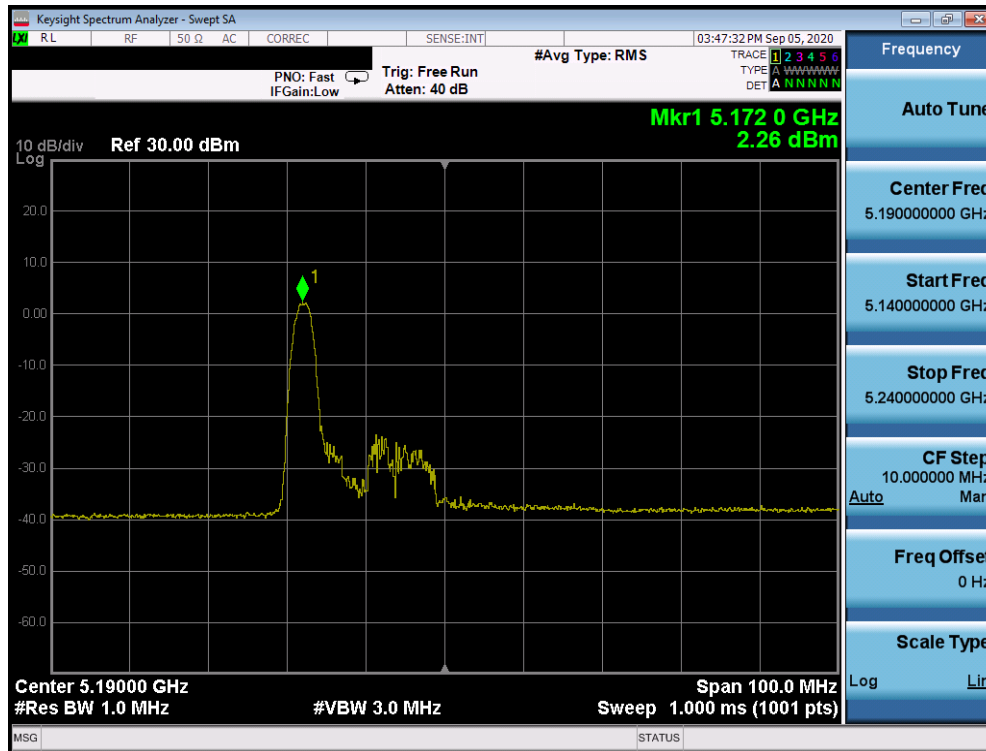
Plot 7-561. ISED Power Spectral Density Plot Antenna 2a (40MHz BW 802.11ax Index 0 – RU26 (UNII Band 1) – Ch. 38)
