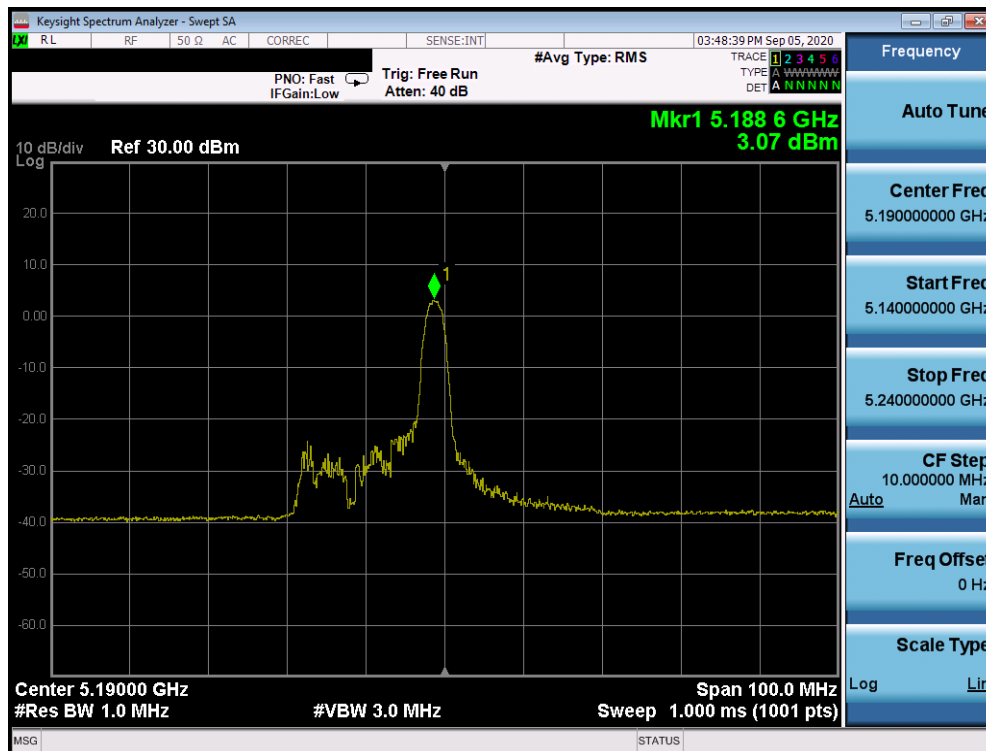
Plot 7-562. ISED Power Spectral Density Plot Antenna 2a (40MHz BW 802.11ax Index 8 – RU26 (UNII Band 1) – Ch. 38)
