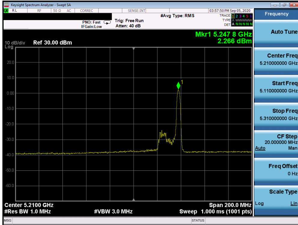
Plot 7-571. ISD Power Spectral Density Plot Antenna 2a (80MHz BW 802.11ax Index 36 – RU26 (UNII Band 1) – Ch. 42)
