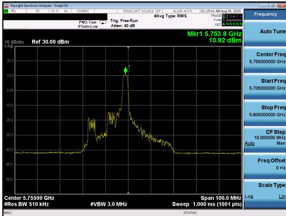
Plot 7-538. Power Spectral Density Plot Antenna 2a (40MHz BW 802.11ax Index 8 – RU26 (UNII Band 3) – Ch. 151)
