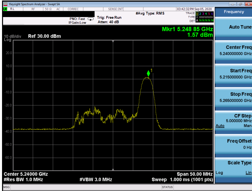
Plot 7-557. ISD Power Spectral Density Plot Antenna 2a (20MHz BW 802.11ax Index 8 – RU26 (UNII Band 1) – Ch. 48)
