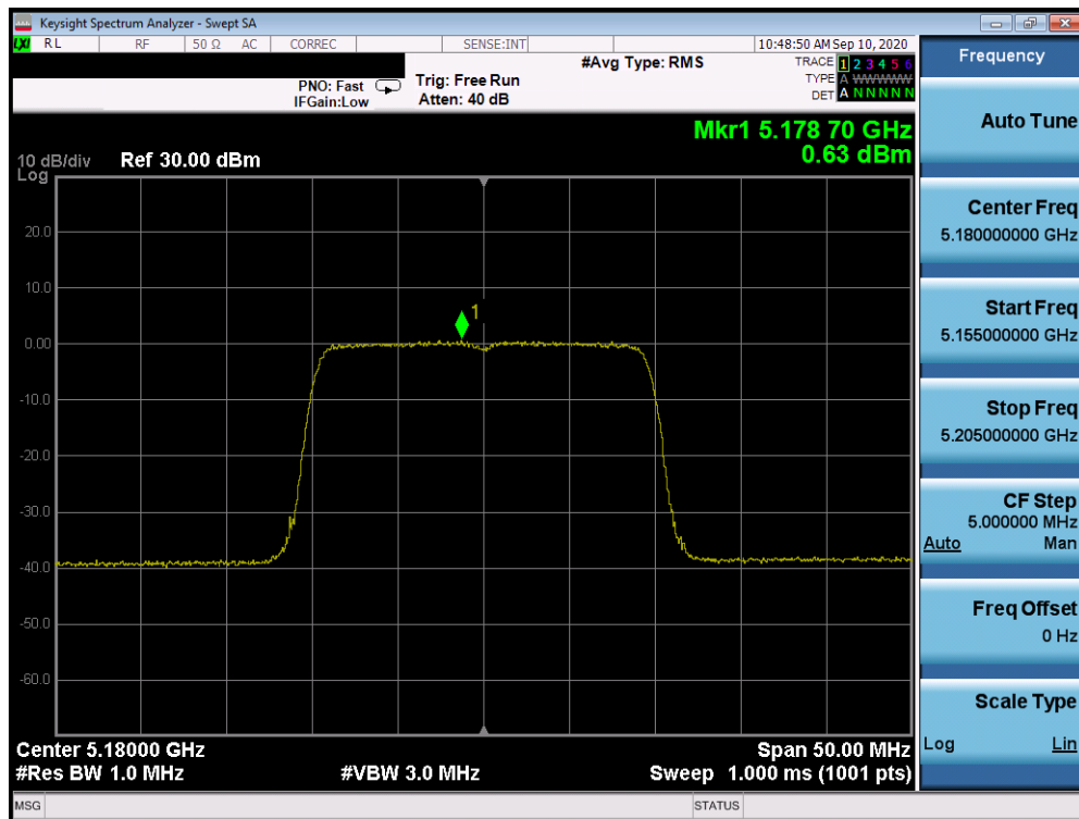
Plot 7-558. ISD Power Spectral Density Plot Antenna 2a (20MHz BW 802.11ax– RU242 (UNII Band 1) – Ch. 36)
