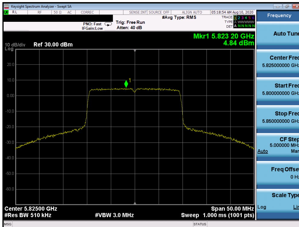
Plot 7-536. Power Spectral Density Plot Antenna 2a (20MHz BW 802.11ax– RU242 (UNII Band 3) – Ch. 165)
