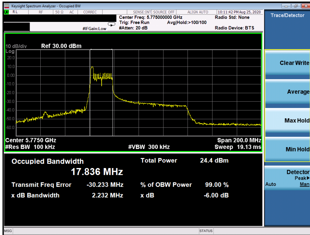
Plot 7-285. 6dB Bandwidth Plot Antenna 2a (80MHz BW 802.11ax Index 0 – RU26 (UNII Band 3) – Ch. 155)
