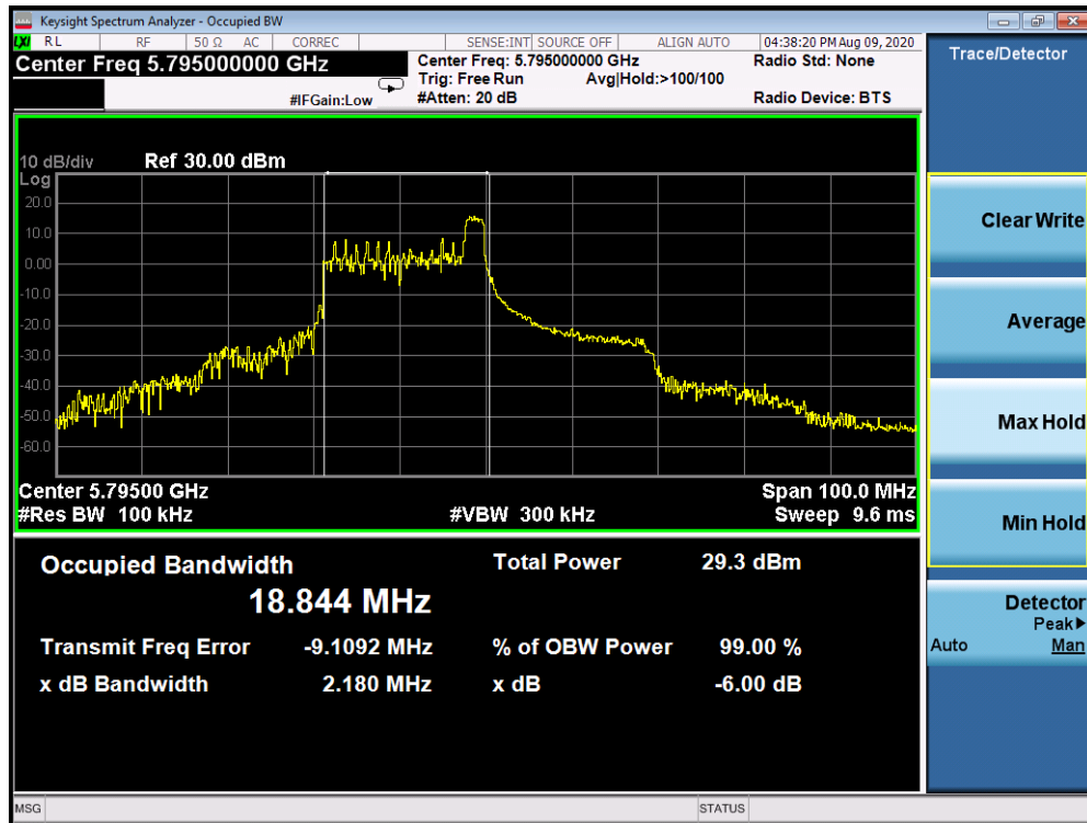
Plot 7-305. 6dB Bandwidth Plot Antenna 1b (40MHz BW 802.11ax Index 8 – RU26 (UNII Band 3) – Ch. 159)
