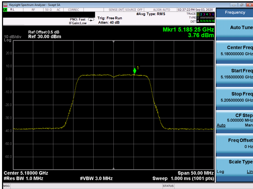
Plot 7-80. ISD Power Spectral Density Plot Antenna 2b (20MHz BW 802.11n (UNII Band 1) – Ch. 36)
