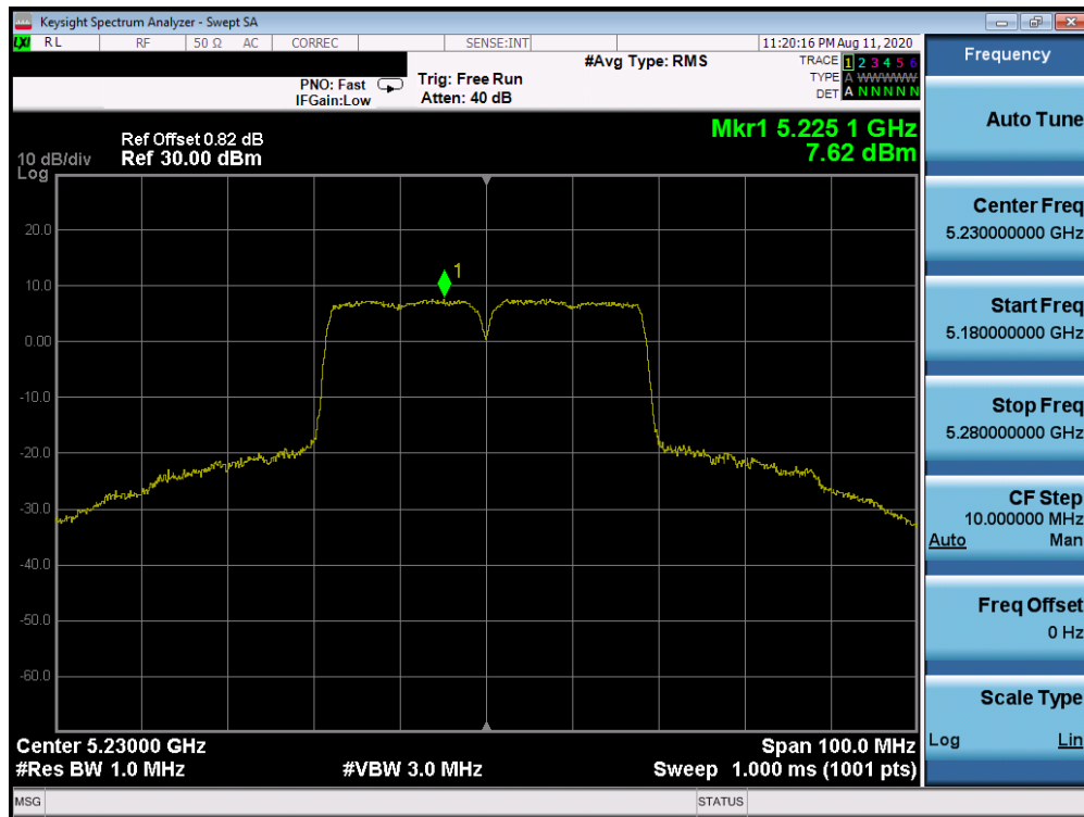
Plot 7-86. Power Spectral Density Plot Antenna 2b (40MHz BW 802.11n (UNII Band 1) – Ch. 46)
