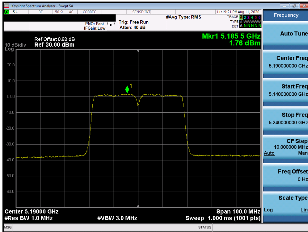
Plot 7-85. Power Spectral Density Plot Antenna 2b (40MHz BW 802.11n (UNII Band 1) – Ch. 38)
