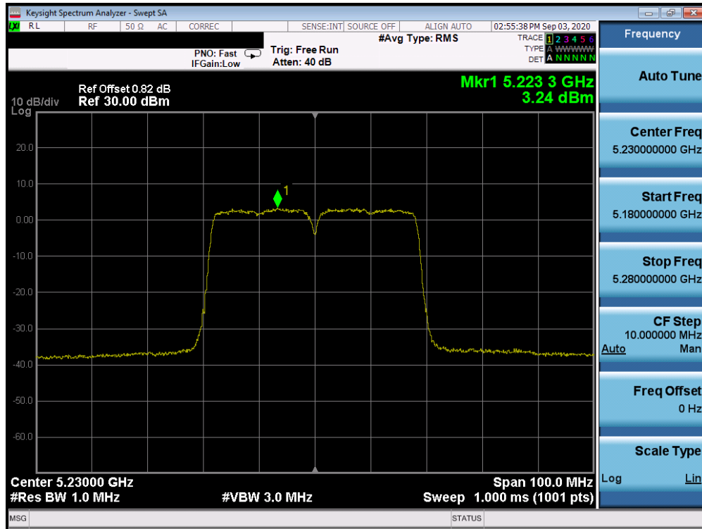
Plot 7-87. ISD Power Spectral Density Plot Antenna 2b (40MHz BW 802.11n (UNII Band 1) – Ch. 46)
