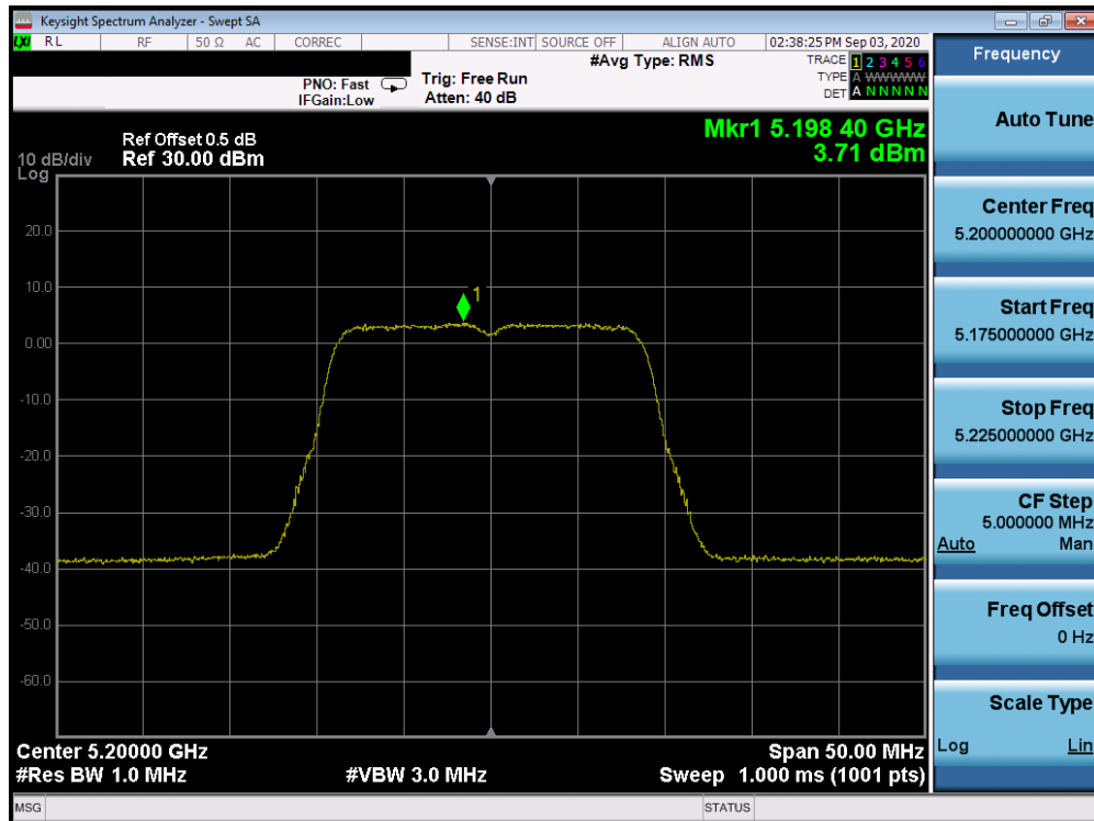
Plot 7-82. ISD Power Spectral Density Plot Antenna 2b (20MHz BW 802.11n (UNII Band 1) – Ch. 40)
