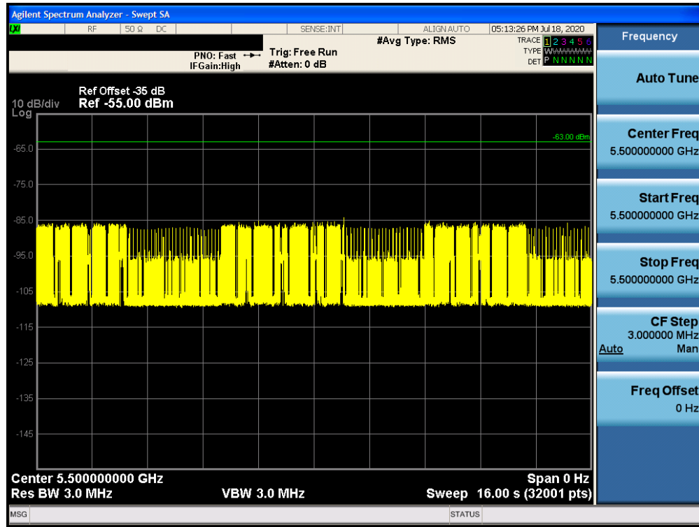
Figure 9-7. 5500MHz - Channel Loading - Mode 2 (20MHz)
