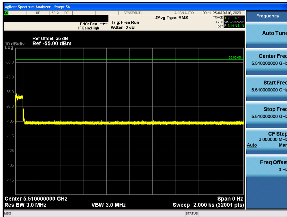
Figure 9-41. 5510MHz - Non-Occupancy Period (30 Minutes) - Mode 2 (40MHz)
