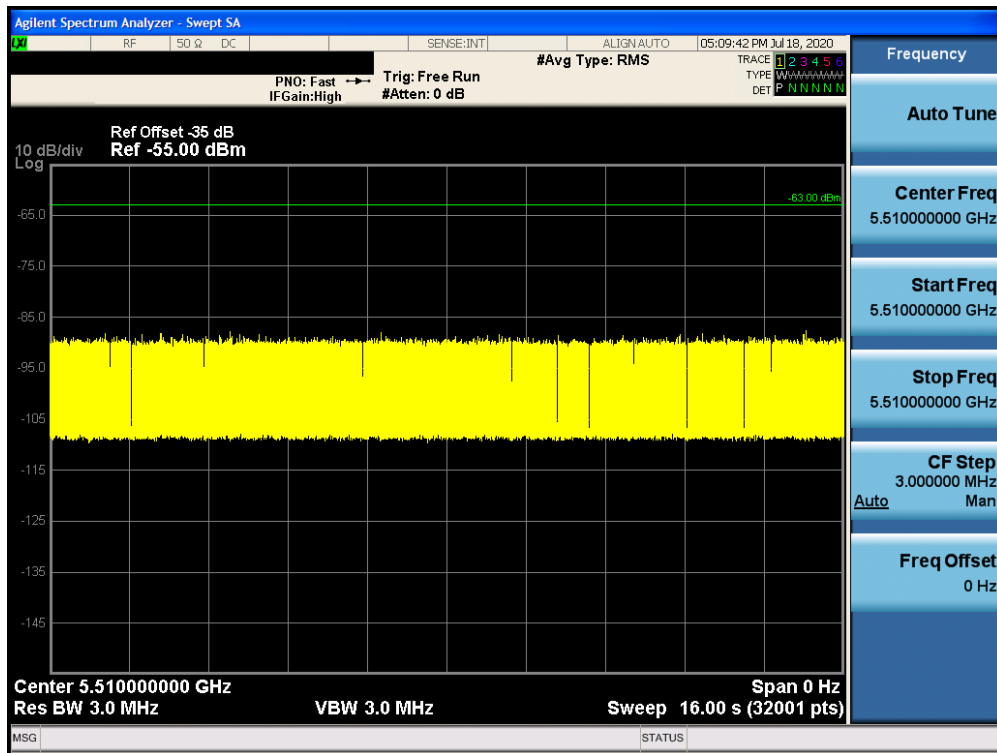
Figure 9-3. 5510MHz - Channel Loading - Mode 1 (40MHz)
