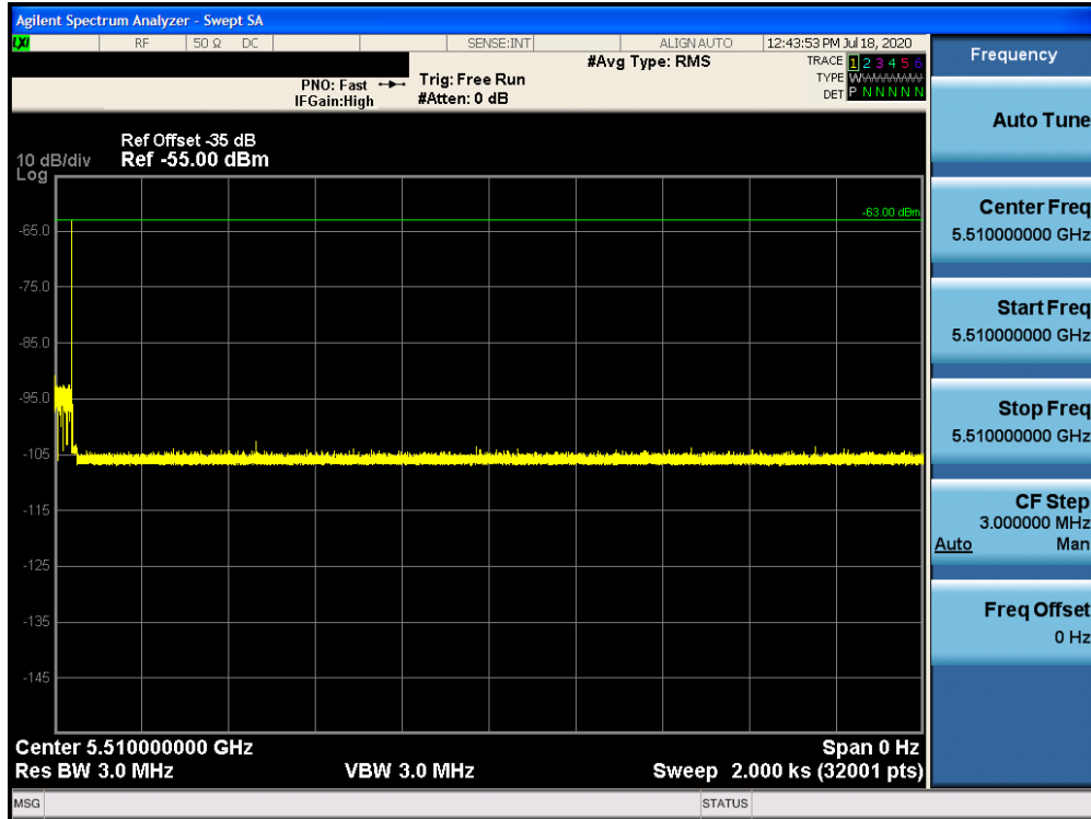
Figure 9-44. 5510MHz - Non-Occupancy Period (30 Minutes) - Mode 3 (40MHz)
