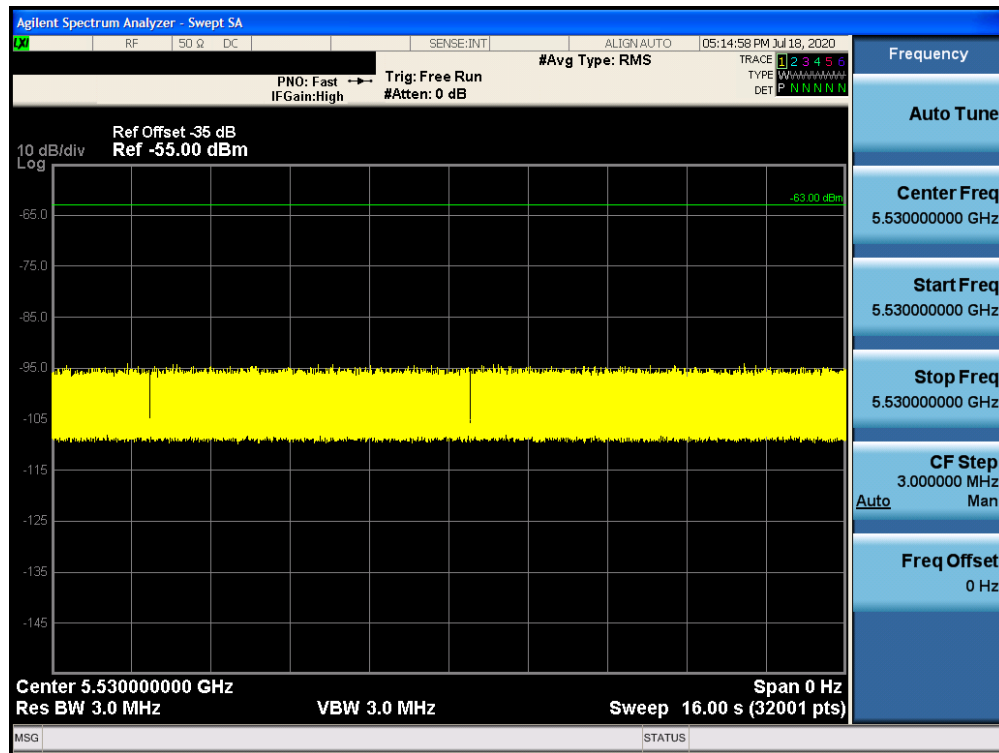
Figure 9-5. 5530MHz - Channel Loading - Mode 1 (80MHz)
