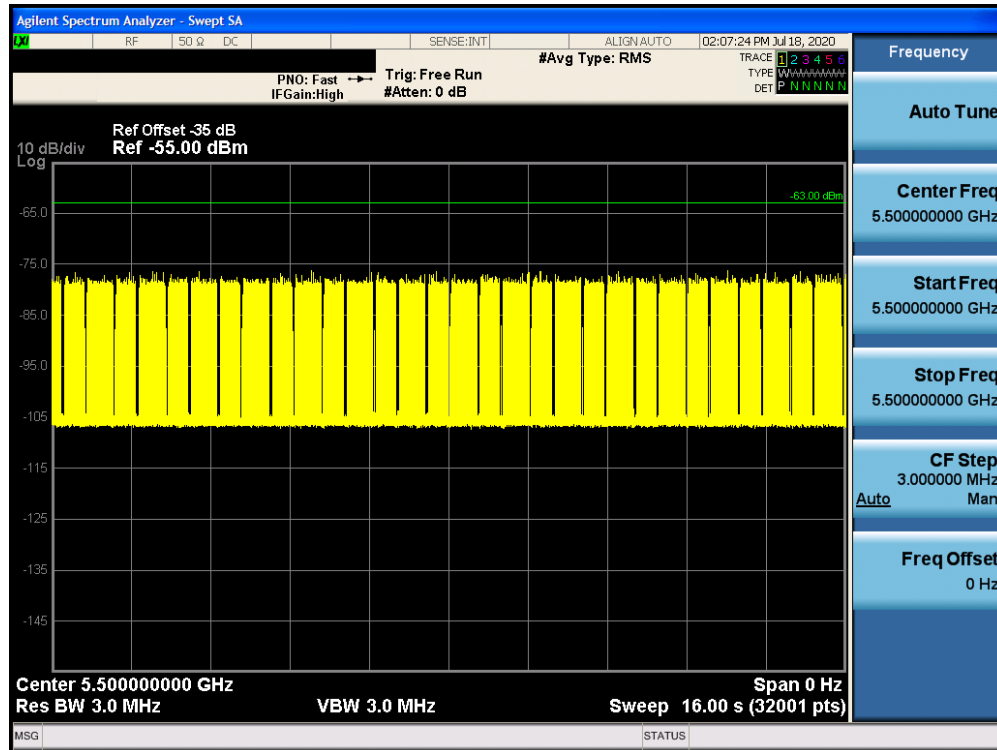
Figure 9-19. 5500 MHz - Channel Loading - Mode 4 (20MHz)
