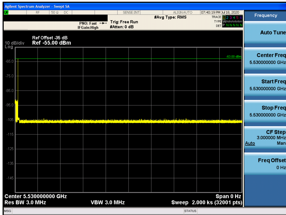
Figure 9-42. 5530MHz - Non-Occupancy Period (30 Minutes) - Mode 2 (80MHz)
