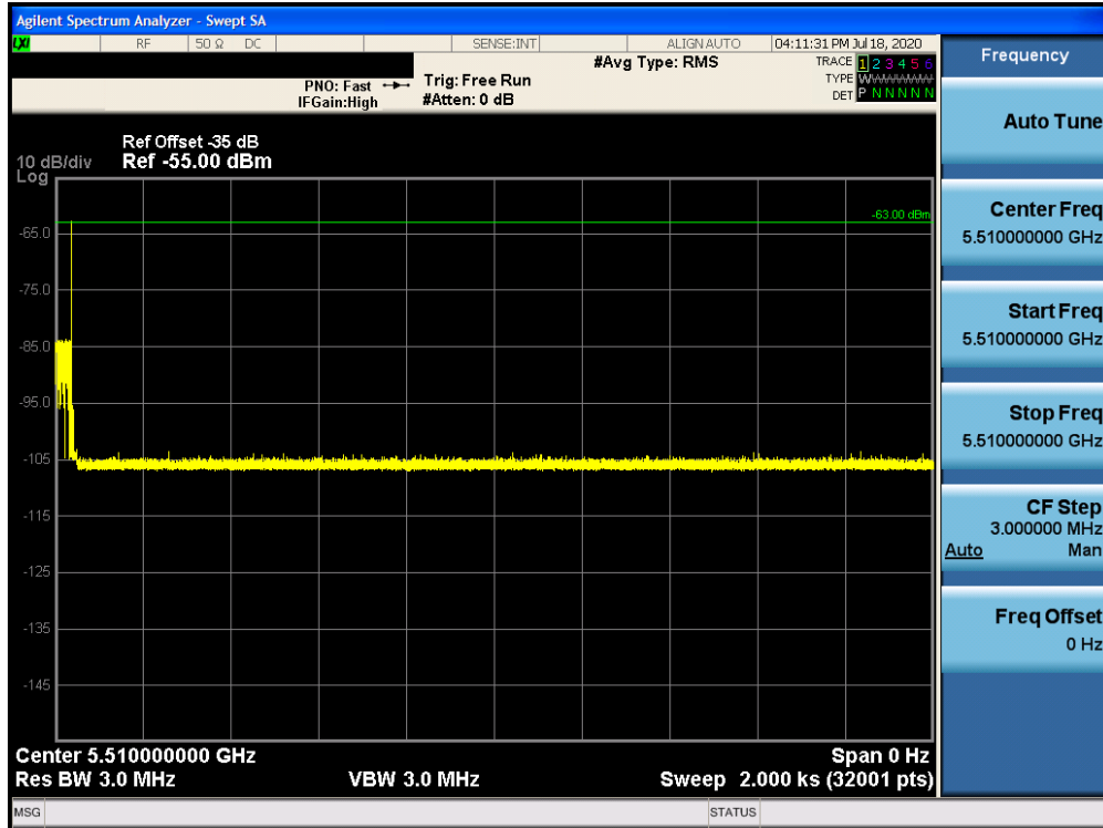
Figure 9-47. 5510MHz - Non-Occupancy Period (30 Minutes) - Mode 4 (40MHz)
