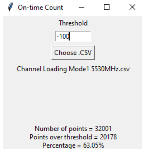
Figure 9-6. 5530MHz - Channel Loading Calculation - Mode 1 (80MHz)
