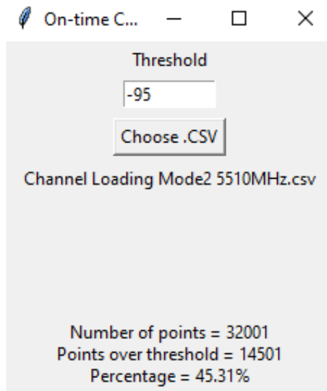
Figure 9-10 5510MHz - Channel Loading Calculation - Mode 2 (40MHz)
