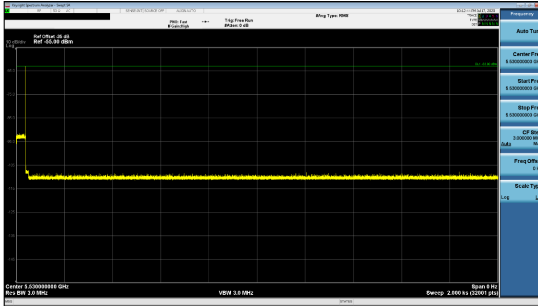
Figure 9-39. 5530MHz - Non-Occupancy Period (30 Minutes) - Mode 1 (80MHz)
