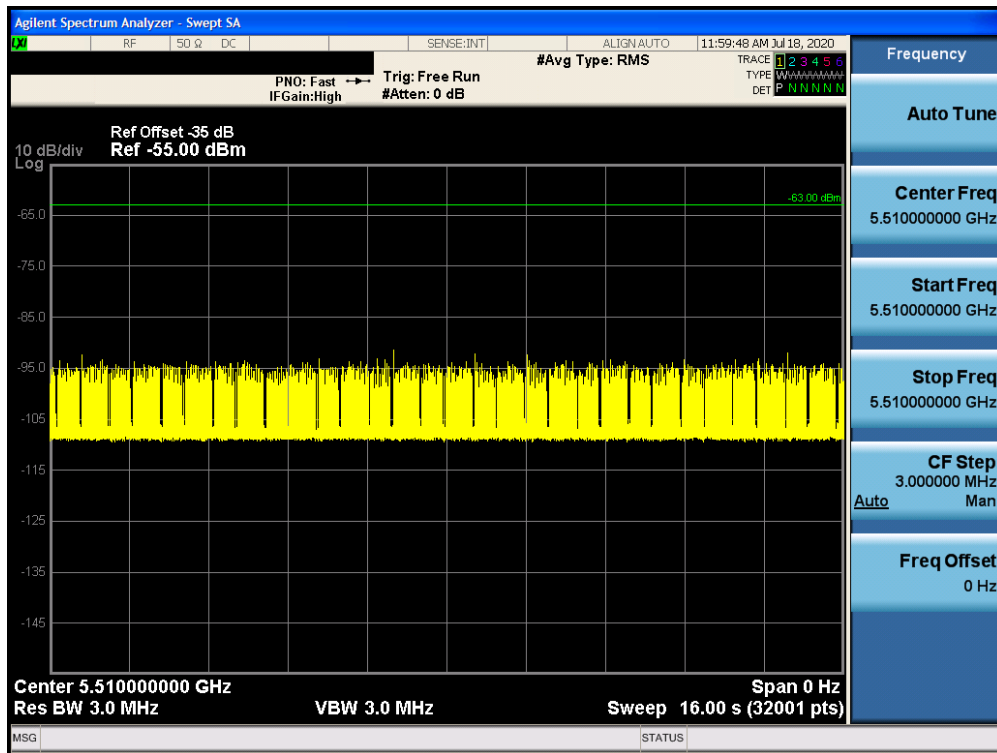
Figure 9-15. 5510MHz - Channel Loading - Mode 3 (40MHz)
