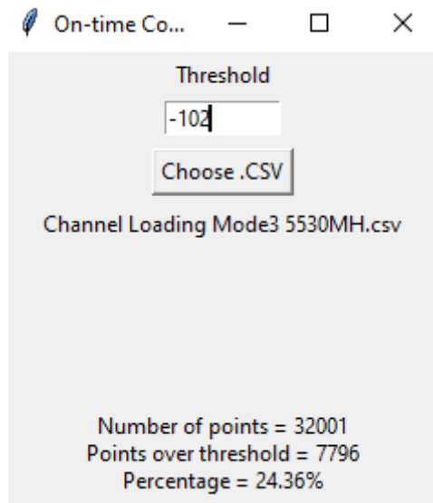
Figure 9-18. 5530MHz - Channel Loading Calculation - Mode 3 (80MHz)
