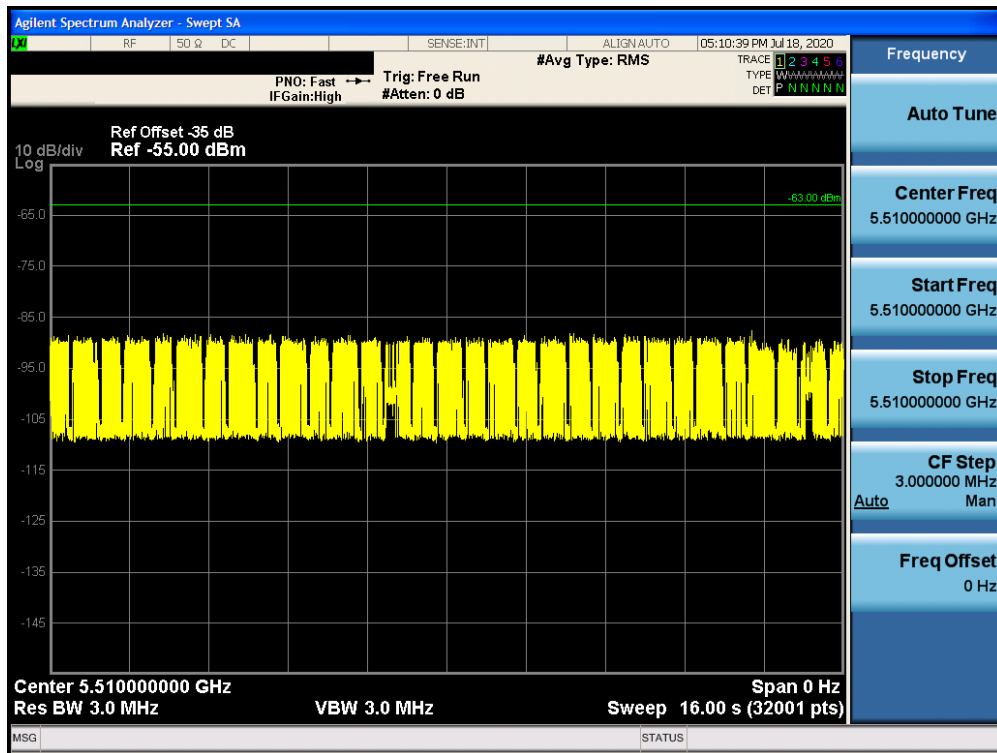
Figure 9-9. 5510MHz - Channel Loading - Mode 2 (40MHz)
