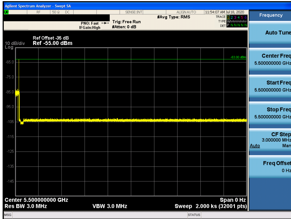
Figure 9-43. 5500MHz - Non-Occupancy Period (30 Minutes) - Mode 3 (20MHz)
