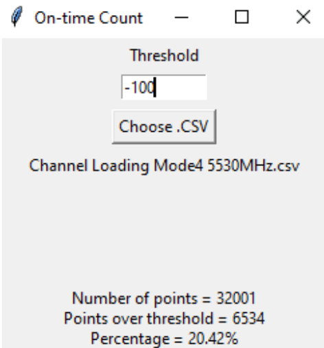
Figure 9-24. 5530MHz - Channel Loading Calculation - Mode 4 (80MHz)
