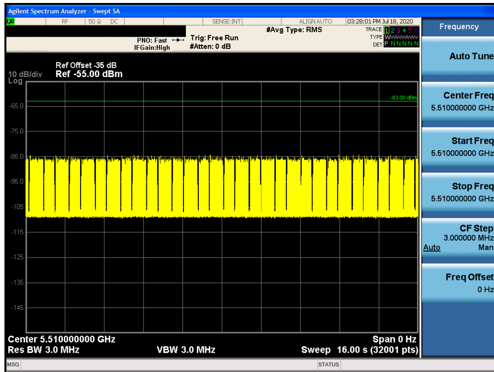
Figure 9-21. 5510MHz - Channel Loading - Mode 4 (40MHz)
