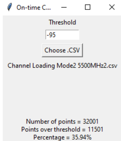
Figure 9-8. 5500MHz - Channel Loading Calculation - Mode 2 (20MHz)
