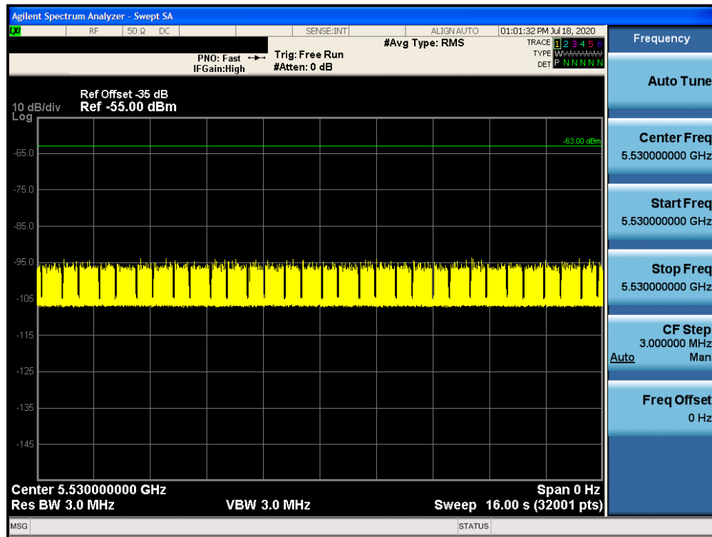
Figure 9-17. 5530MHz - Channel Loading - Mode 3 (80MHz)
