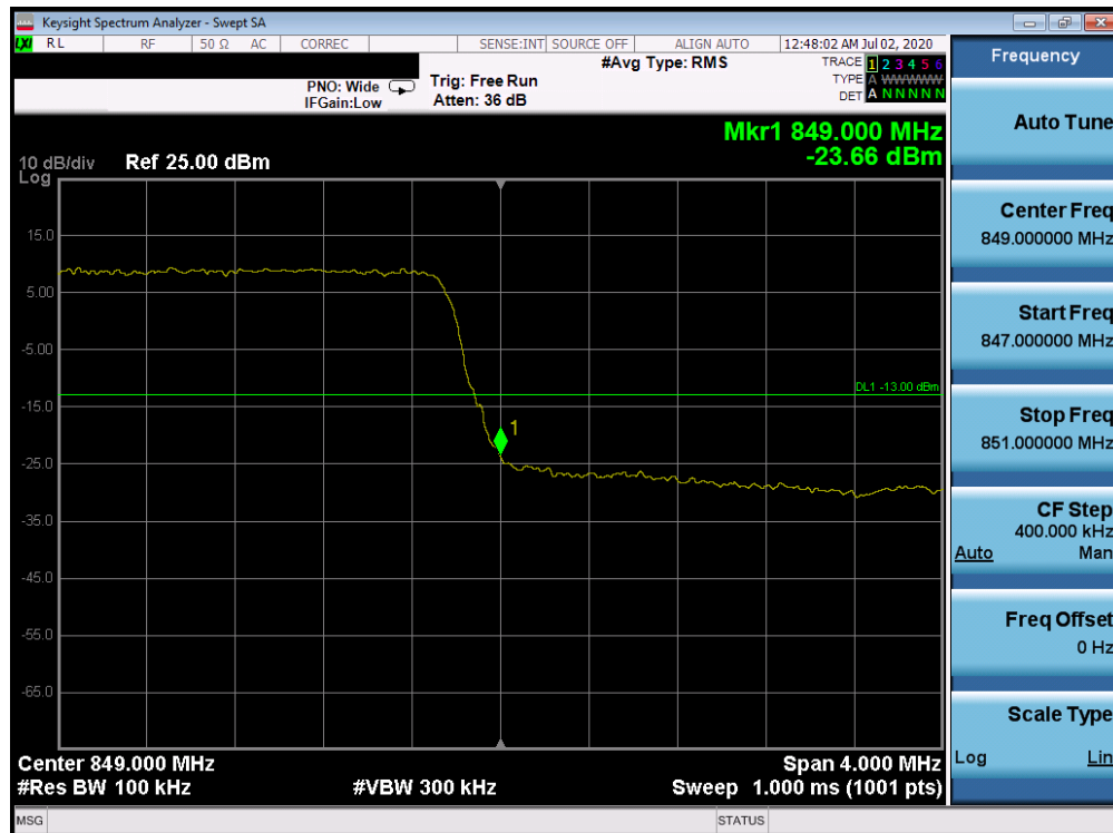
Plot 7-223. Upper Band Edge Plot (Band 26 - 5.0MHz QPSK - Full RB Configuration)
