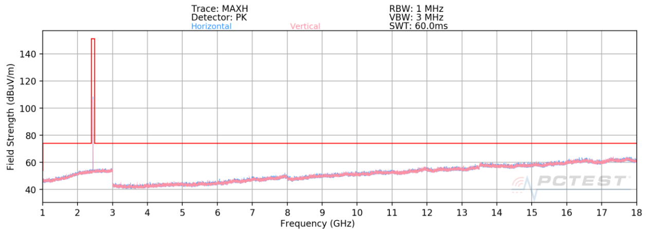
Plot 7-85. Radiated Spurious Emissions Above 1GHz Antenna WF7b (4Mbps, HDR4, ePA – Ch. 38)
