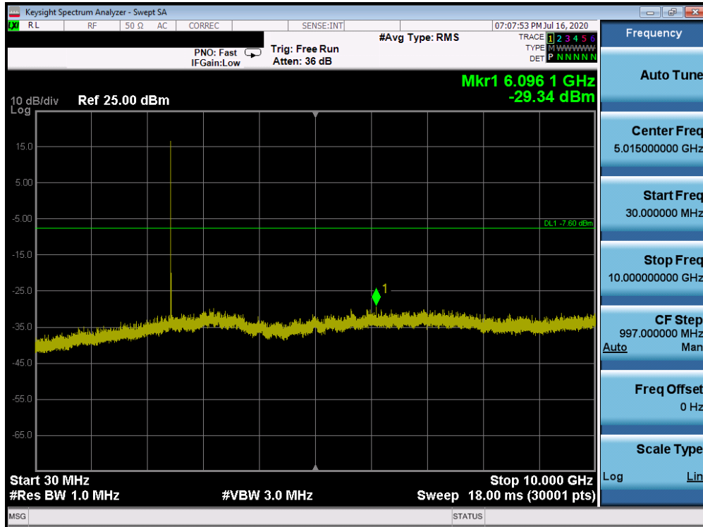
Plot 7-77. Conducted Spurious Plot Antenna WF7b (Bluetooth (HDR4), 4 Mbps, ePA – Ch. 38)
