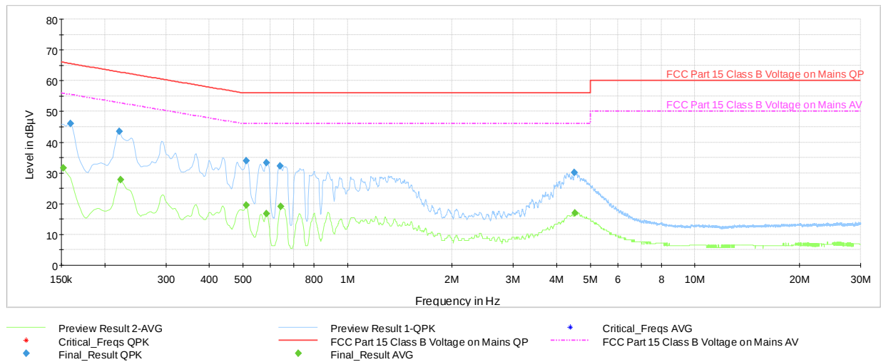
Plot 7-106. AC Line Conducted Plot with Bluetooth HDR (N, 4Mbps ePA - Ch.38 with AC/DC Adapter)
