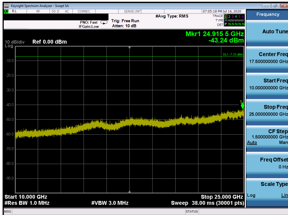
Plot 7-76. Conducted Spurious Plot Antenna WF7b (Bluetooth (HDR4), 4 Mbps, ePA – Ch. 1)
