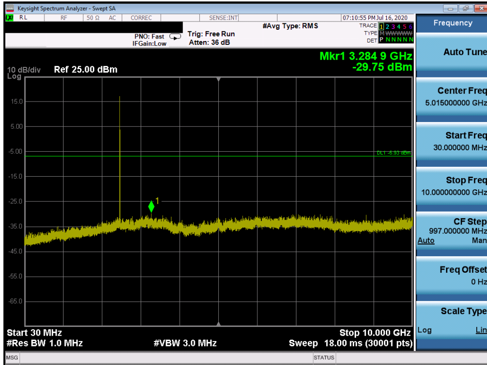
Plot 7-79. Conducted Spurious Plot Antenna WF7b (Bluetooth (HDR4), 4 Mbps, ePA – Ch. 75)
