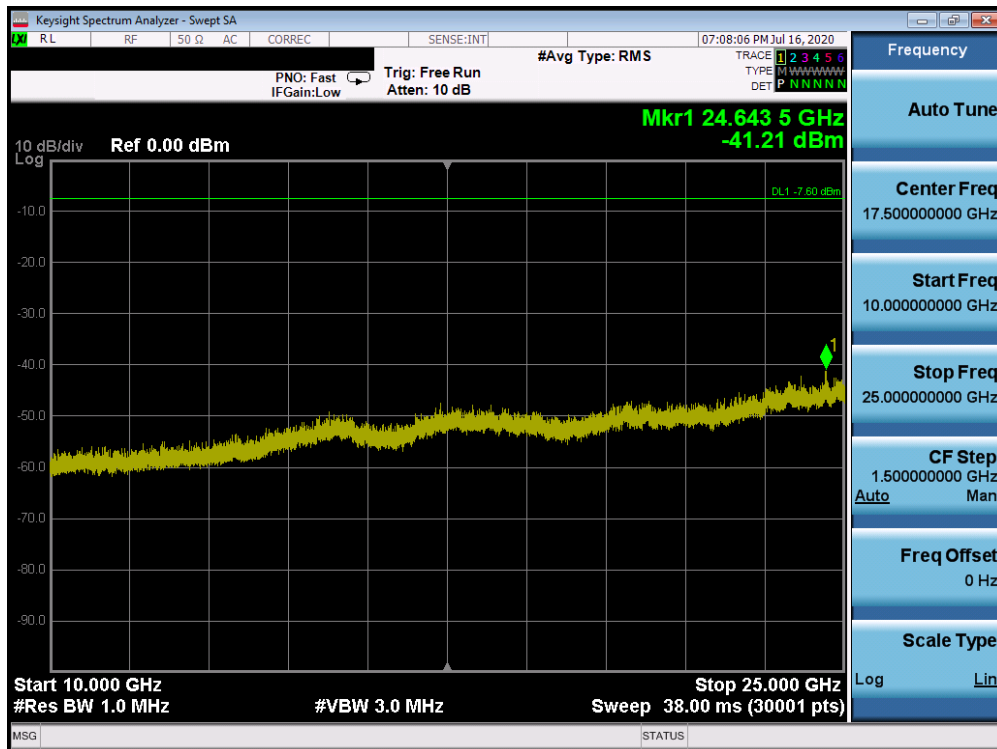
Plot 7-78. Conducted Spurious Plot Antenna WF7b (Bluetooth (HDR4), 4 Mbps, ePA – Ch. 38)
