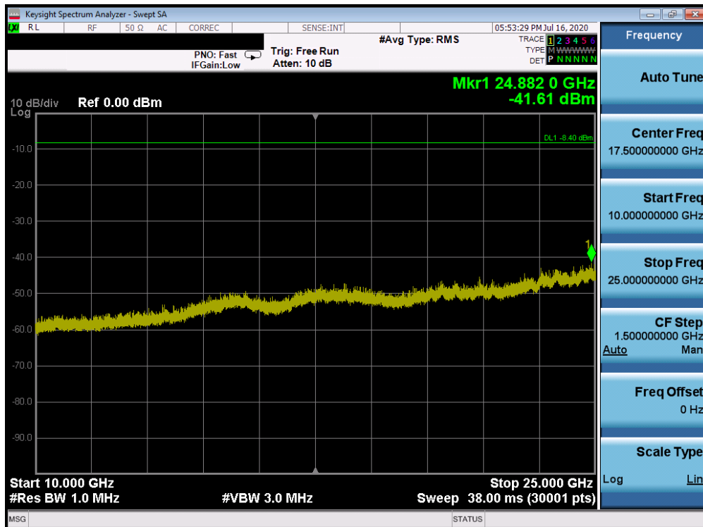
Plot 7-74. Conducted Spurious Plot Antenna WF8 (Bluetooth (HDR4), 4 Mbps, ePA – Ch. 75)
