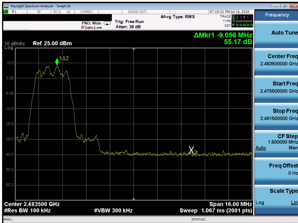
Plot 7-66. Band Edge Plot Antenna WF7b (Bluetooth (HDR4), ePA – Ch. 75)
