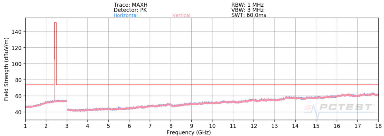
Plot 7-84. Radiated Spurious Emissions Above 1GHz Antenna WF7b (4Mbps, HDR4, ePA – Ch. 1)
