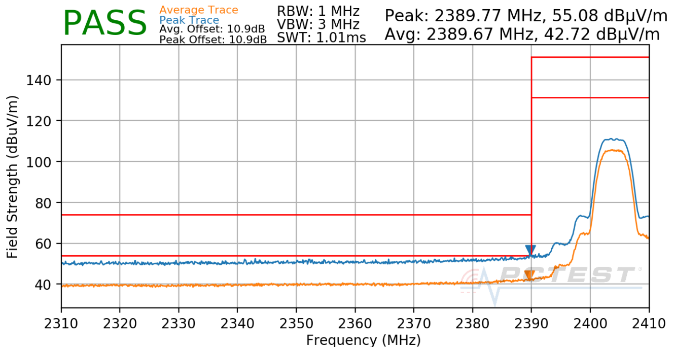
Plot 7-97. Radiated Restricted Lower Band Edge Measurement Antenna WF7b (Average & Peak)
