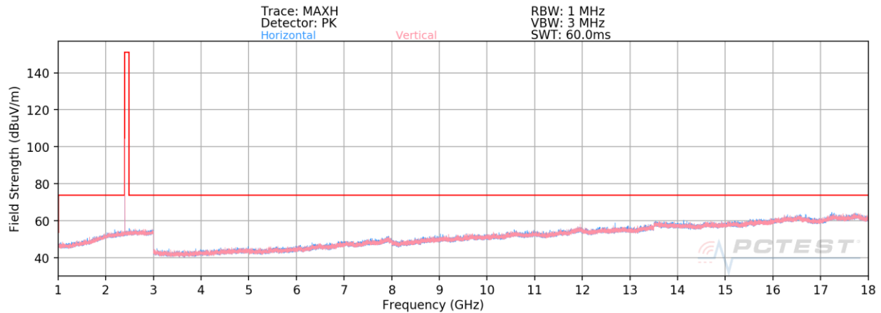
Plot 7-81. Radiated Spurious Emissions Above 1GHz Antenna WF8 (4Mbps, HDR4, ePA – Ch. 1)
