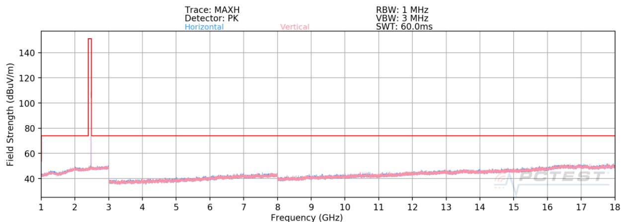
Plot 7-86. Radiated Spurious Emissions Above 1GHz Antenna WF7b (4Mbps, HDR4, ePA – Ch. 75)
