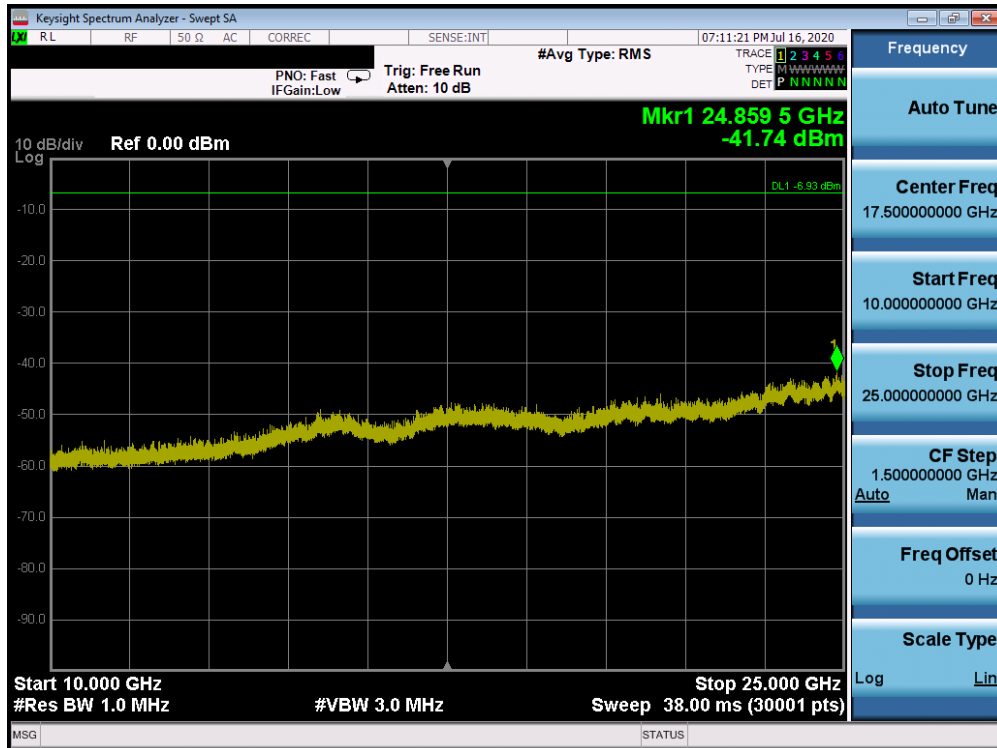
Plot 7-80. Conducted Spurious Plot Antenna WF7b (Bluetooth (HDR4), 4 Mbps, ePA – Ch. 75)
