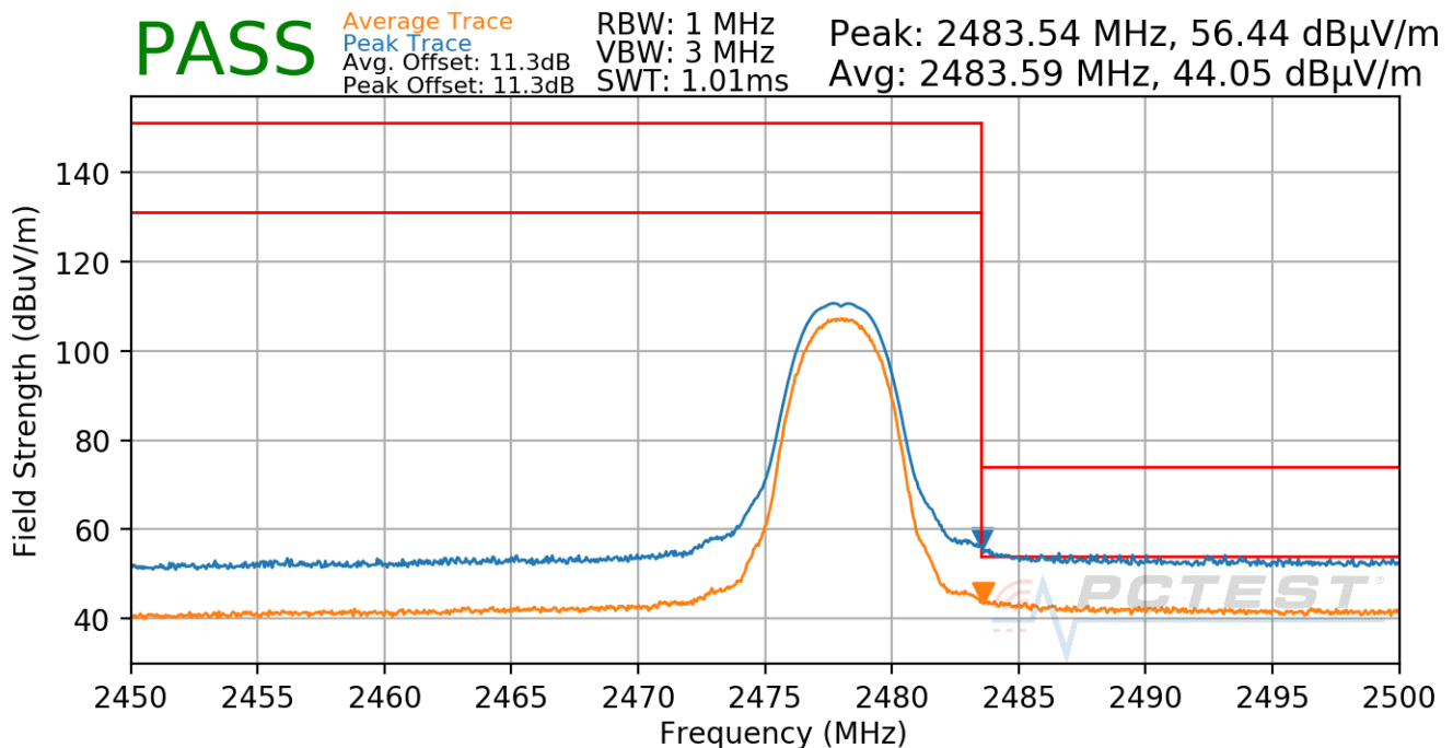
Plot 7-98. Radiated Restricted Upper Band Edge Measurement Antenna WF7b (Average & Peak)
