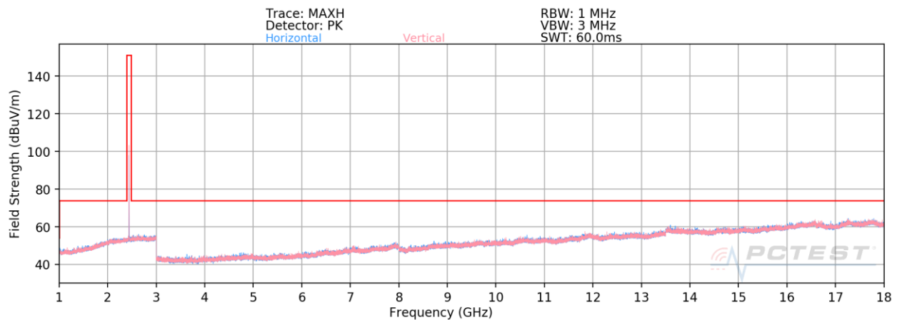
Plot 7-82. Radiated Spurious Emissions Above 1GHz Antenna WF8 (4Mbps, HDR4, ePA – Ch. 38)
