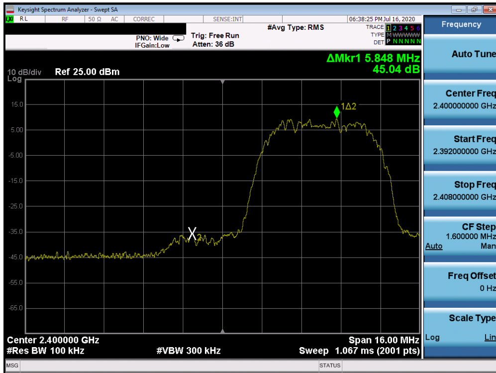
Plot 7-67. Band Edge Plot Antenna WF7b (Bluetooth (HDR8), ePA – Ch. 1)
