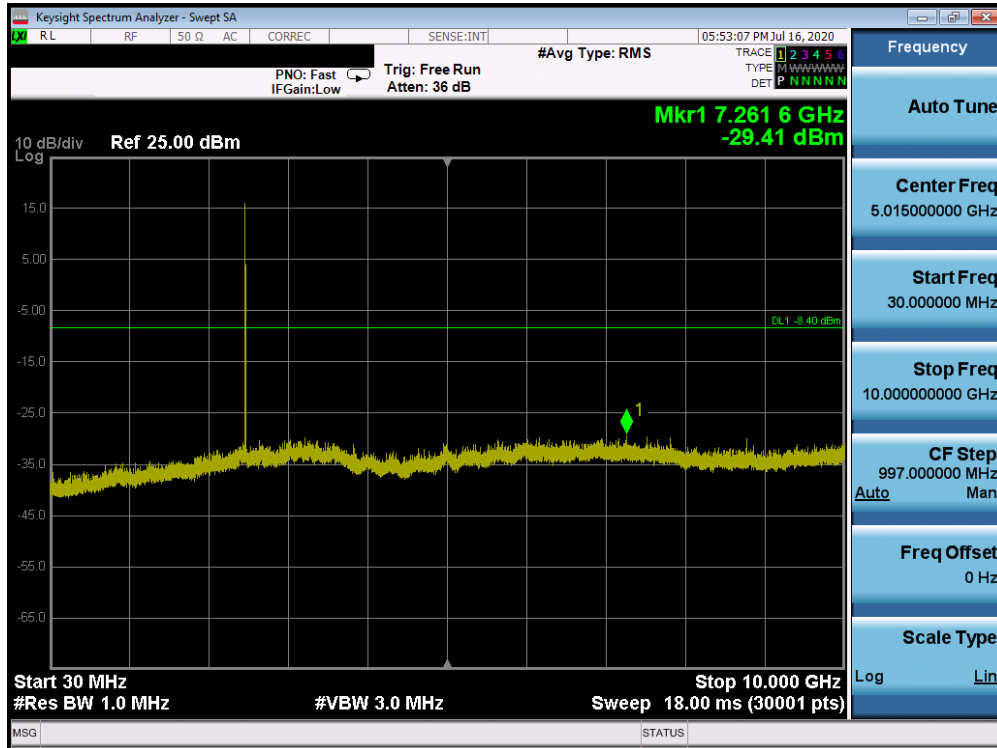
Plot 7-73. Conducted Spurious Plot Antenna WF8 (Bluetooth (HDR4), 4 Mbps, ePA – Ch. 75)
