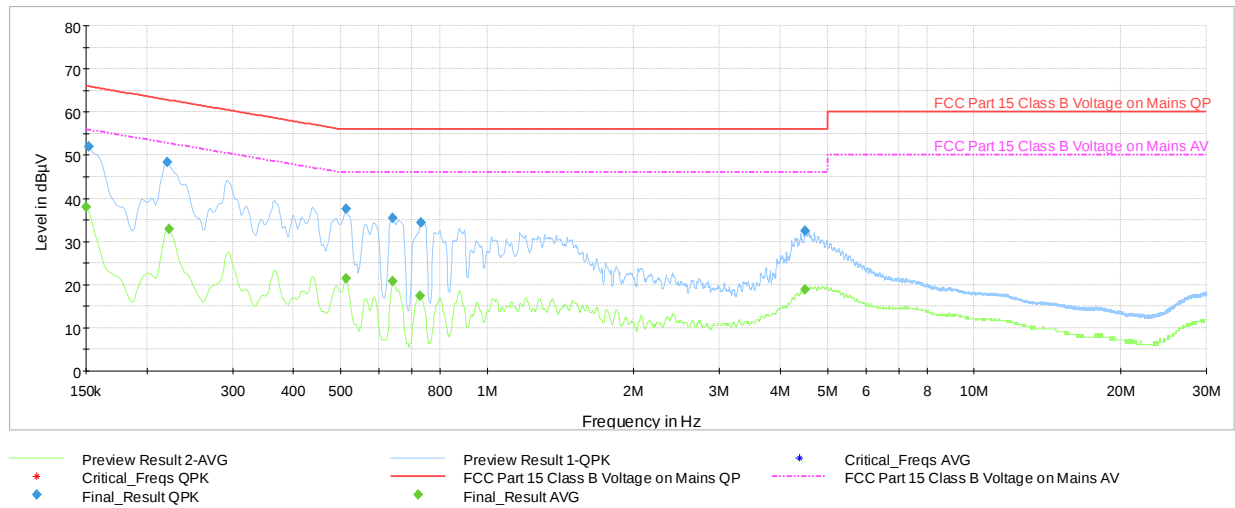
Plot 7-105. AC Line Conducted Plot with Bluetooth HDR (L1, 4Mbps ePA - Ch.38 with AC/DC Adapter)
