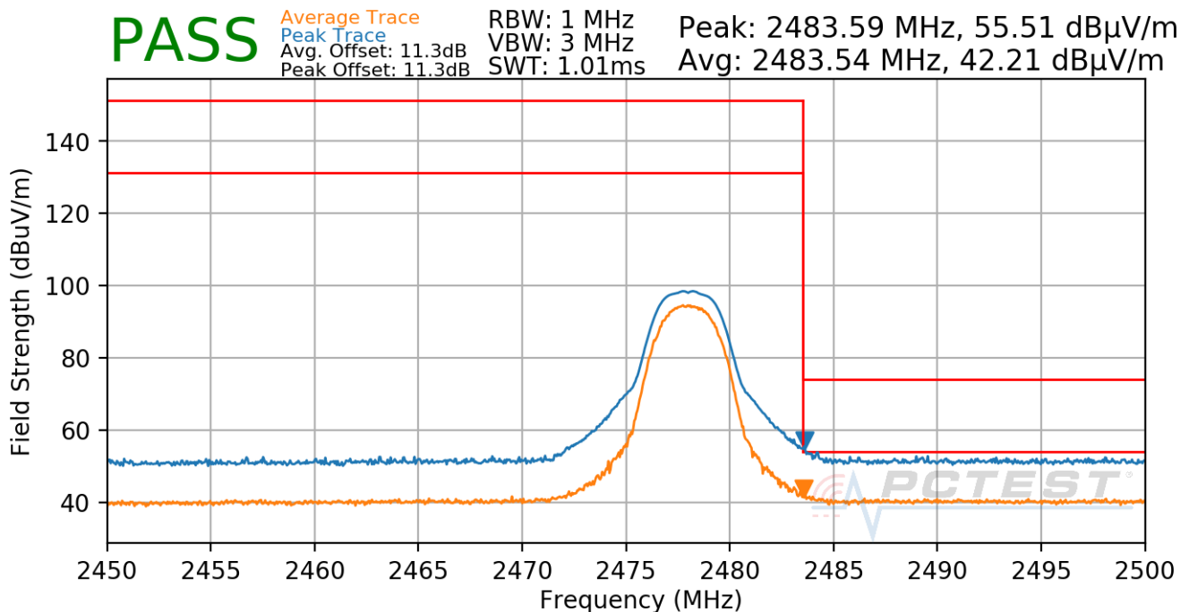
Plot 7-94. Radiated Restricted Upper Band Edge Measurement Antenna WF8 (Average & Peak)
