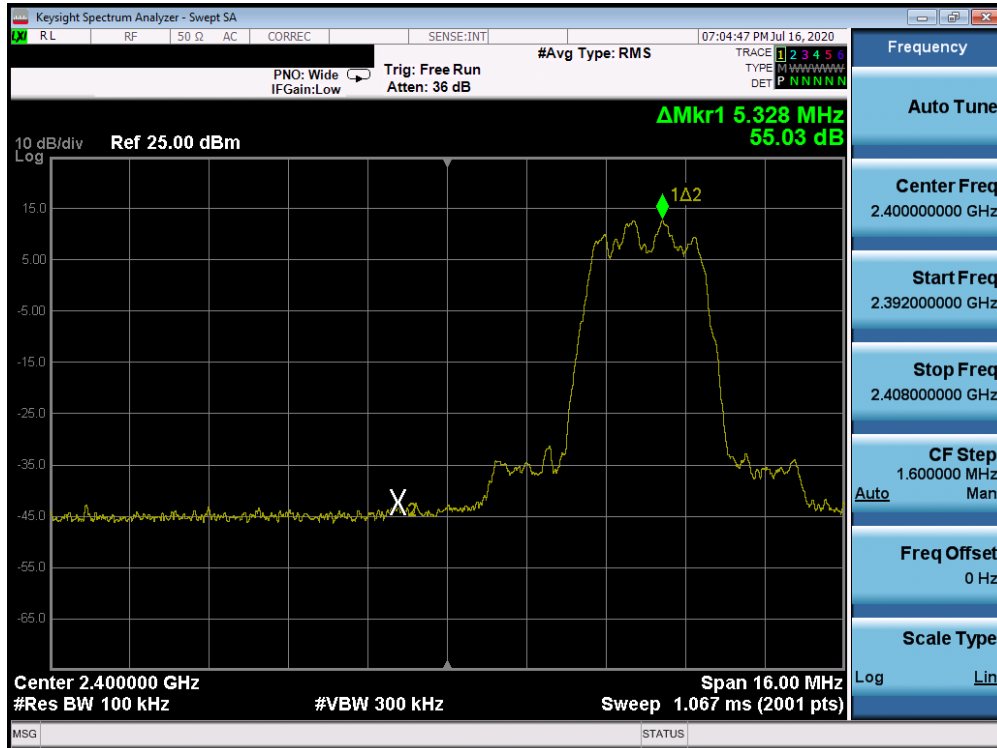
Plot 7-65. Band Edge Plot Antenna WF7b (Bluetooth (HDR4), ePA – Ch. 1)
