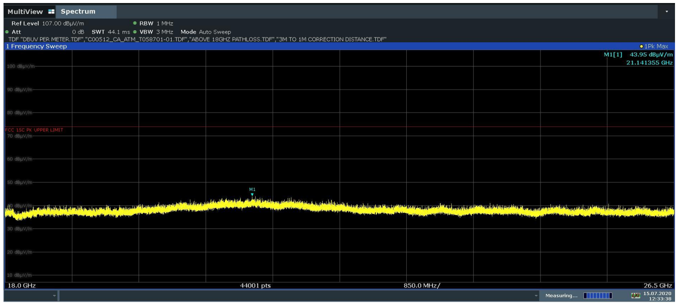
Plot 7-90. Radiated Spurious Emissions Above 18GHz TxBF (4Mbps – Ch.38, ePA, Ant. Pol. H)
