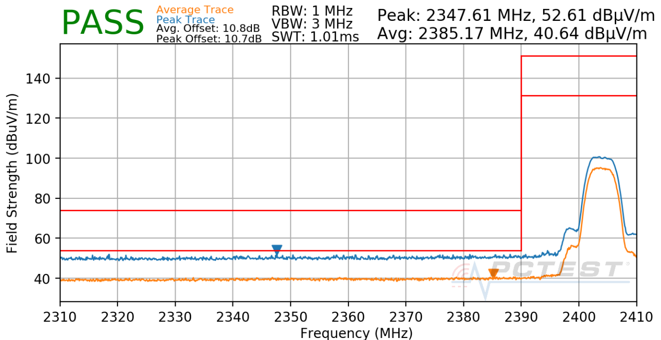
Plot 7-93. Radiated Restricted Lower Band Edge Measurement Antenna WF8 (Average & Peak)
