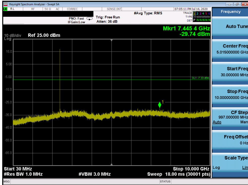
Plot 7-75. Conducted Spurious Plot Antenna WF7b (Bluetooth (HDR4), 4 Mbps, ePA – Ch. 1)
