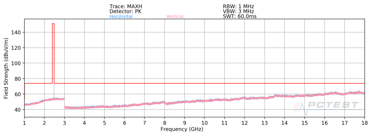
Plot 7-83. Radiated Spurious Emissions Above 1GHz Antenna WF8 (4Mbps, HDR4, ePA – Ch. 75)
