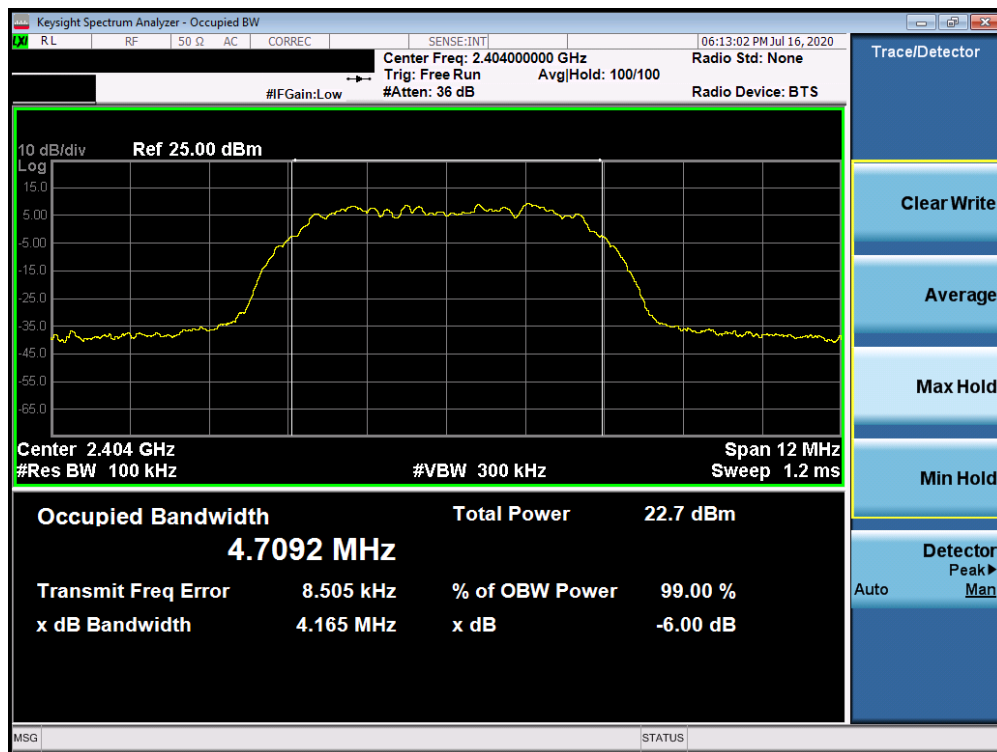
Plot 7-4. 6dB Bandwidth Plot Antenna WF8 (Bluetooth (HDR8), 8Mbps, ePA – Ch. 1)
