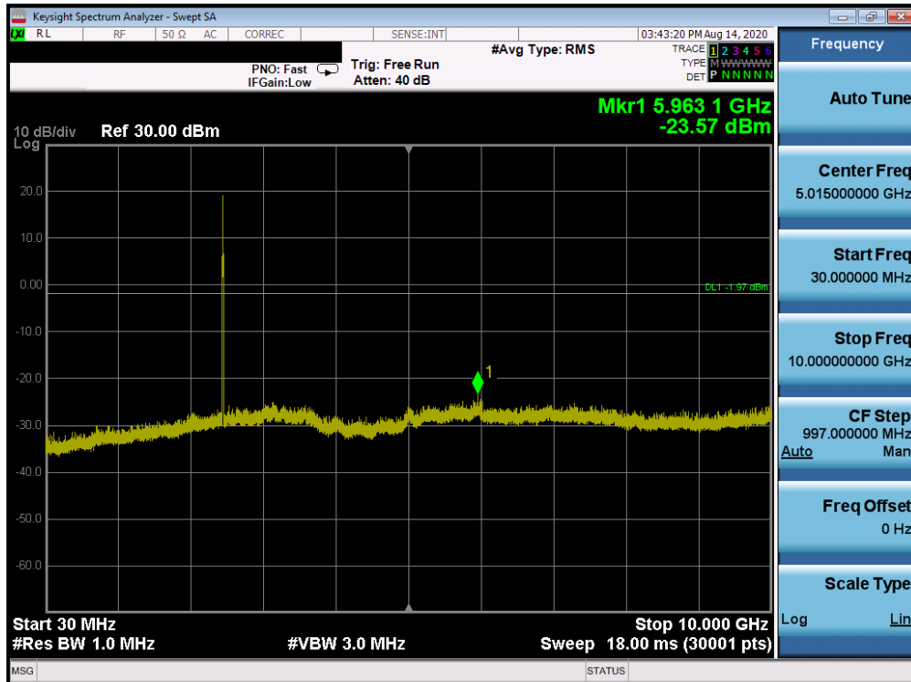
Plot 7-133. Conducted Spurious Plot ANT WF7b (802.11ax OFDMA – RU26 – Ch. 11)
