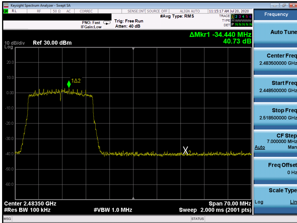
Plot 7-93. Band Edge ANT WF8 (802.11ax OFDMA – RU242 – Ch. 11)
