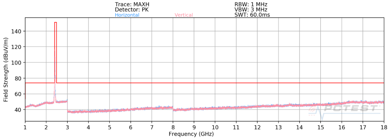
Plot 7-147. Radiated Spurious Emissions above 1GHz ANT WF7b (802.11ax OFDMA – RU26 – Ch. 1)
