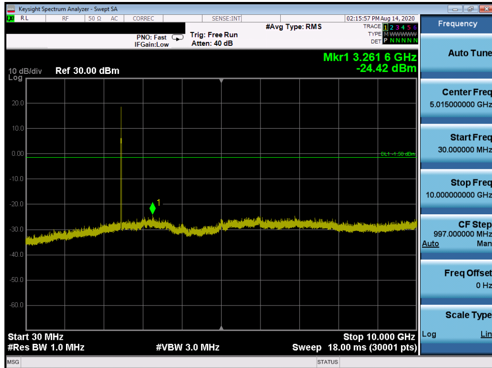
Plot 7-121. Conducted Spurious Plot ANT WF8 (802.11ax OFDMA – RU26 – Ch. 11)
