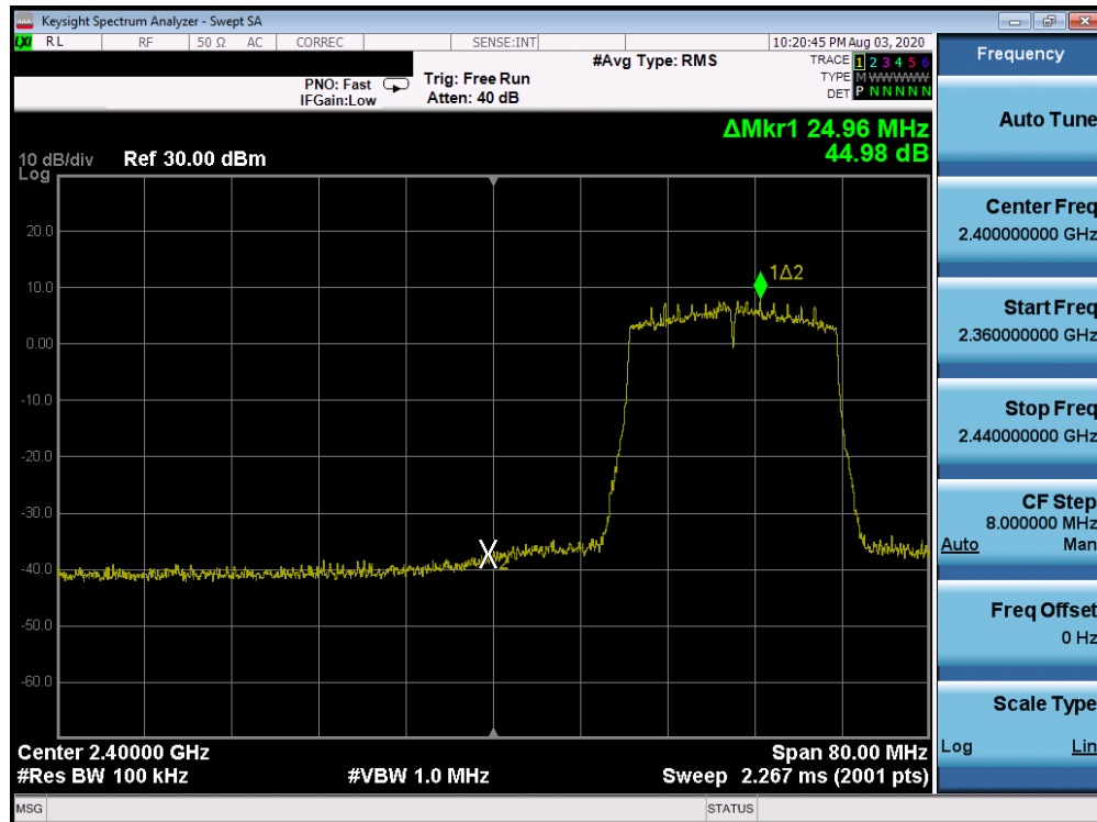
Plot 7-86. Band Edge ANT WF8 (802.11ax OFDMA – RU242 – Ch. 3)
