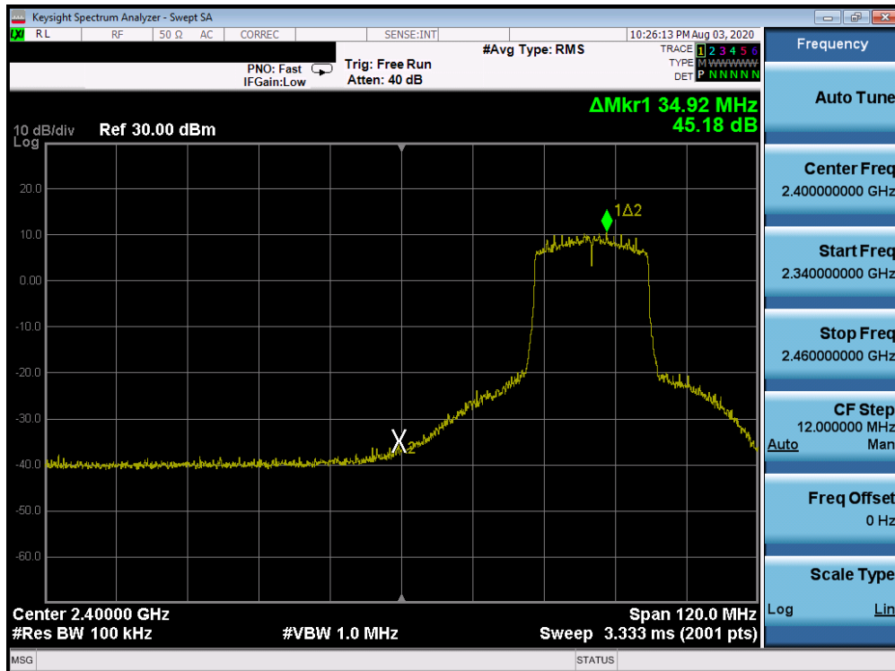
Plot 7-88. Band Edge ANT WF8 (802.11ax OFDMA – RU242 – Ch. 5)
