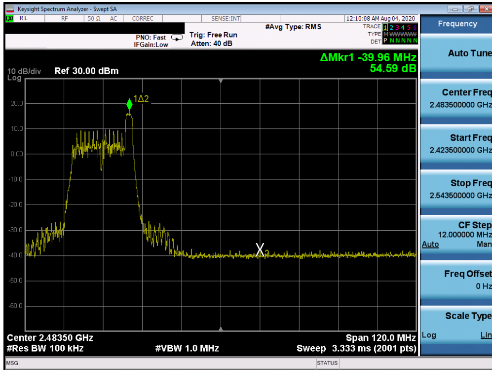
Plot 7-101. Band Edge ANT WF7b (802.11ax OFDMA – RU26 Index 8 – Ch. 8)
