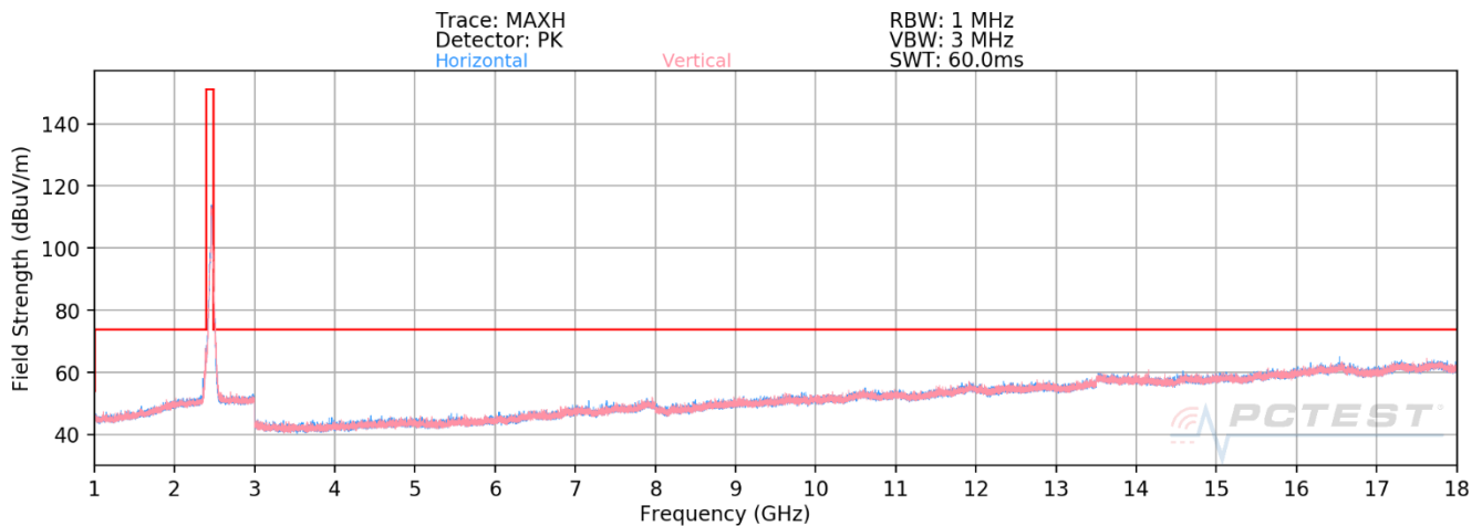
Plot 7-152. Radiated Spurious Emissions above 1GHz ANT WF7b (802.11ax OFDMA – RU242 – Ch. 11)
