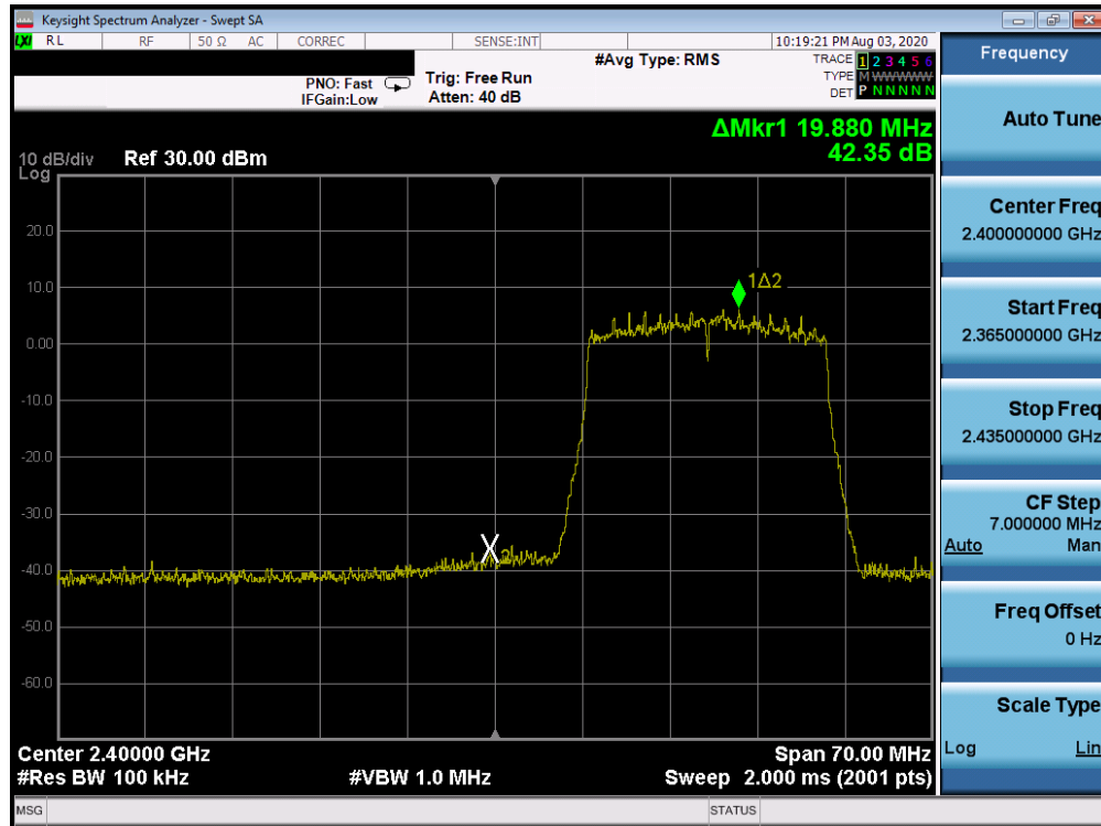
Plot 7-85. Band Edge ANT WF8 (802.11ax OFDMA – RU242 – Ch. 2)
