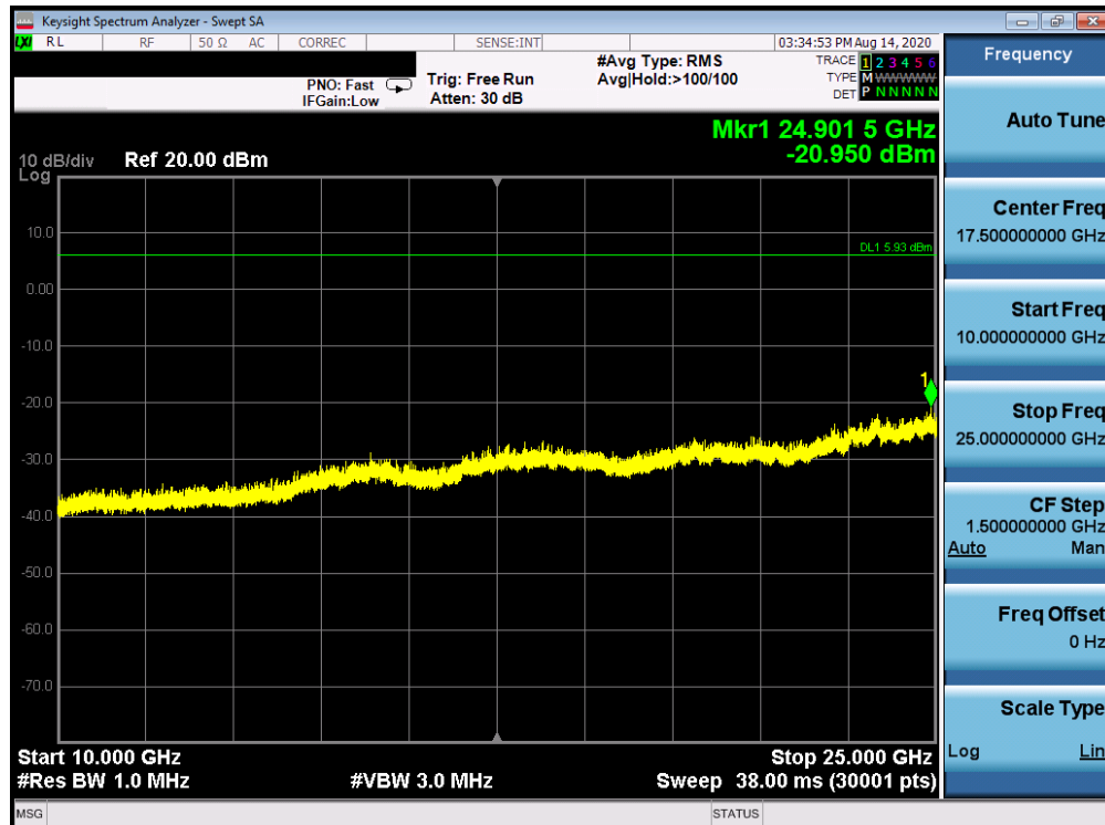
Plot 7-132. Conducted Spurious Plot ANT WF7b (802.11ax OFDMA – RU26 – Ch. 6)
