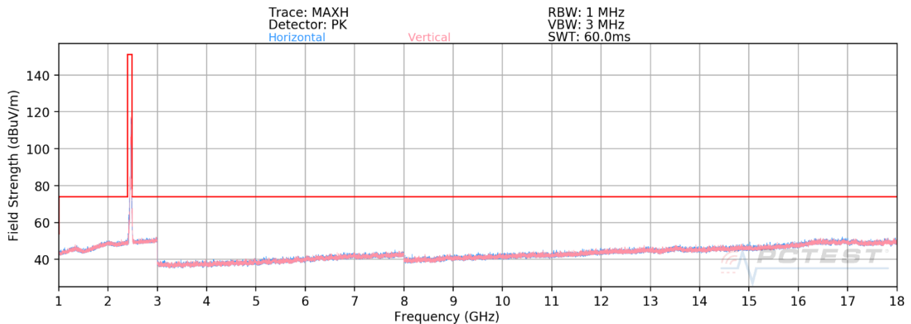
Plot 7-149. Radiated Spurious Emissions above 1GHz ANT WF7b (802.11ax OFDMA – RU26 – Ch. 11)
