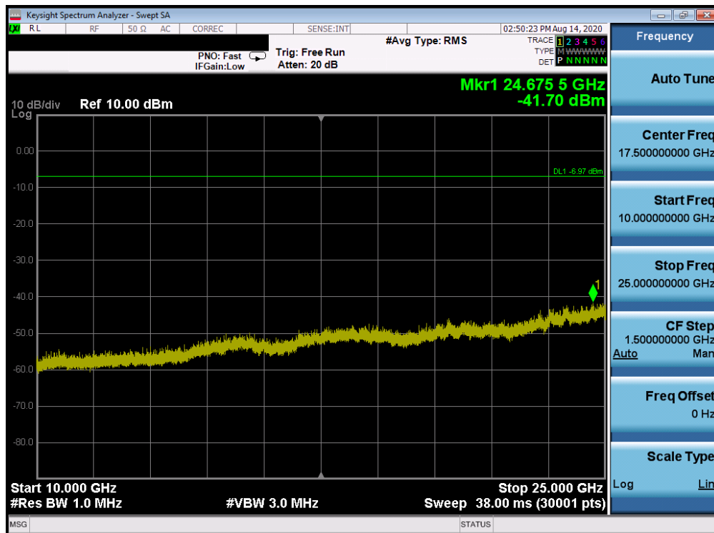
Plot 7-124. Conducted Spurious Plot ANT WF8 (802.11ax OFDMA – RU242 – Ch. 1)
