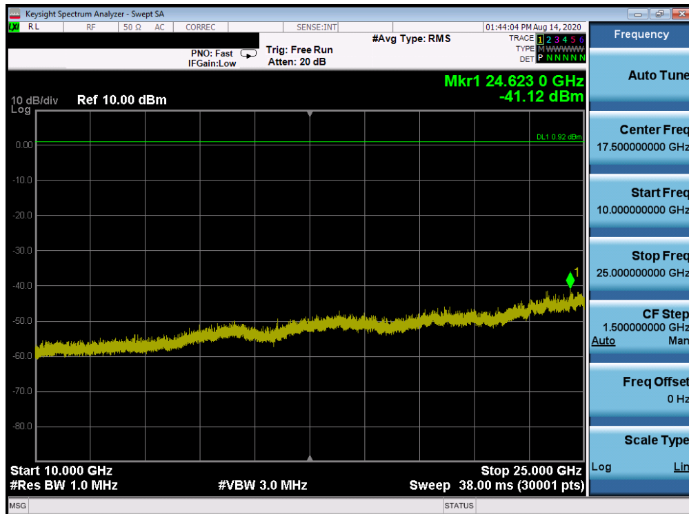
Plot 7-118. Conducted Spurious Plot ANT WF8 (802.11ax OFDMA – RU26 – Ch. 1)
