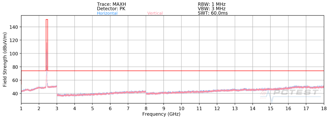
Plot 7-148. Radiated Spurious Emissions above 1GHz ANT WF7b (802.11ax OFDMA – RU26 – Ch. 6)
