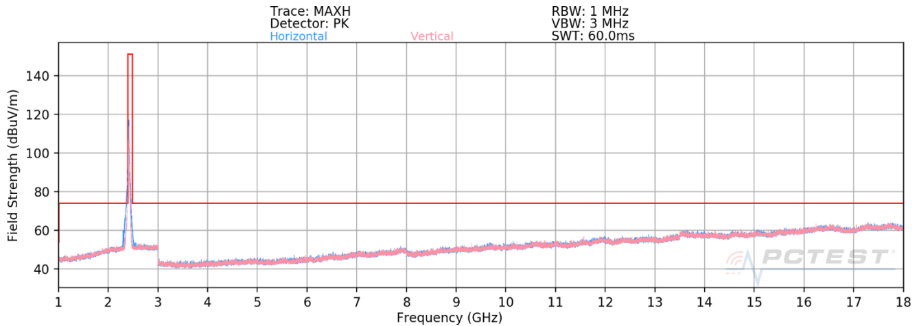
Plot 7-144. Radiated Spurious Emissions above 1GHz ANT WF8 (802.11ax OFDMA – RU242 – Ch. 1)
