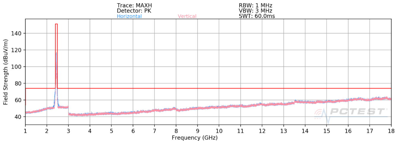
Plot 7-145. Radiated Spurious Emissions above 1GHz ANT WF8 (802.11ax OFDMA – RU242 – Ch. 6)
