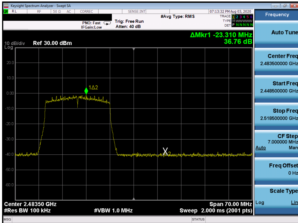
Plot 7-94. Band Edge ANT WF8 (802.11ax OFDMA – RU242 – Ch. 12)
