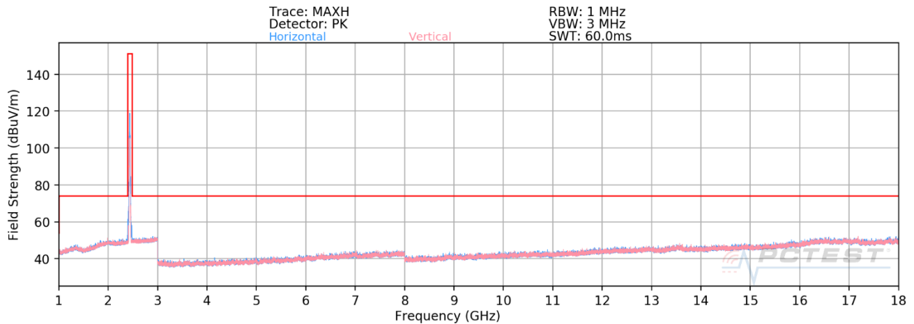
Plot 7-142. Radiated Spurious Emissions above 1GHz ANT WF8 (802.11ax OFDMA – RU26 – Ch. 6)
