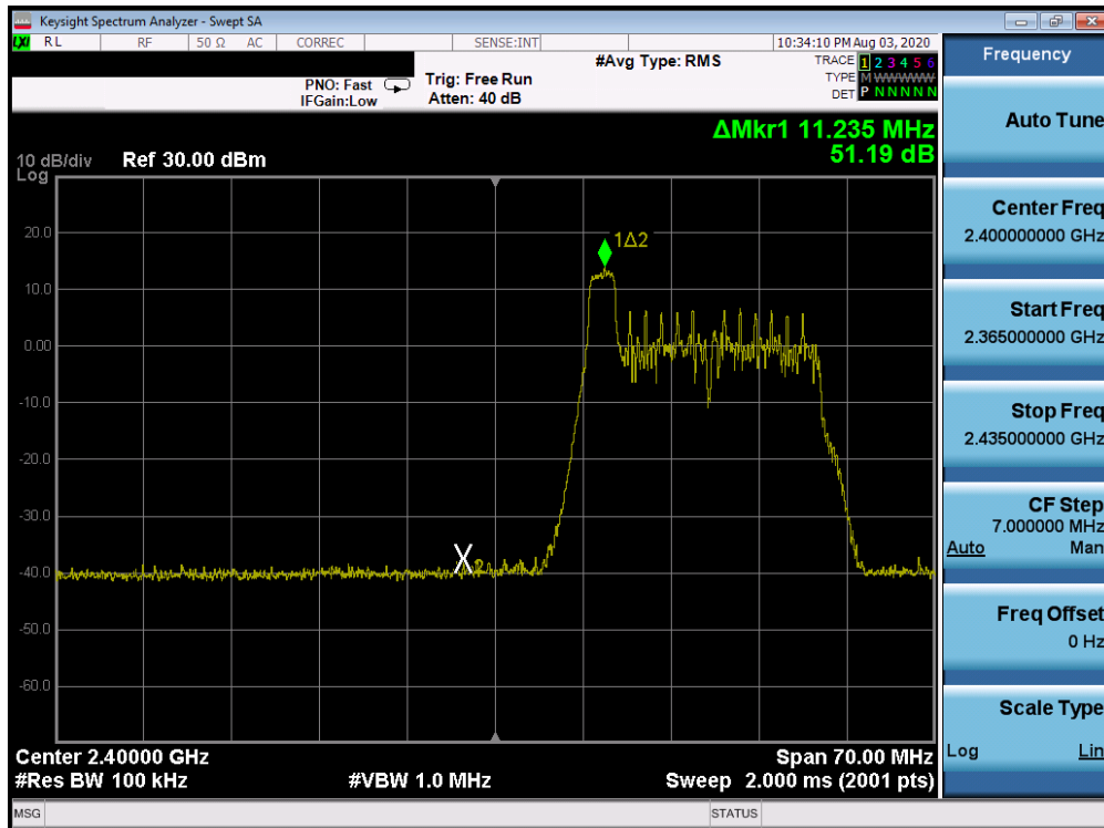
Plot 7-96. Band Edge ANT WF7b (802.11ax OFDMA – RU26 Index 0 – Ch. 2)
