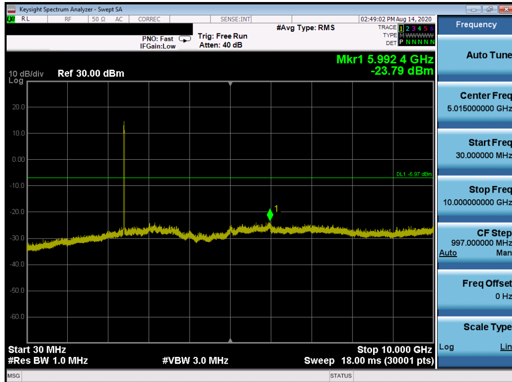
Plot 7-123. Conducted Spurious Plot ANT WF8 (802.11ax OFDMA – RU242 – Ch. 1)
