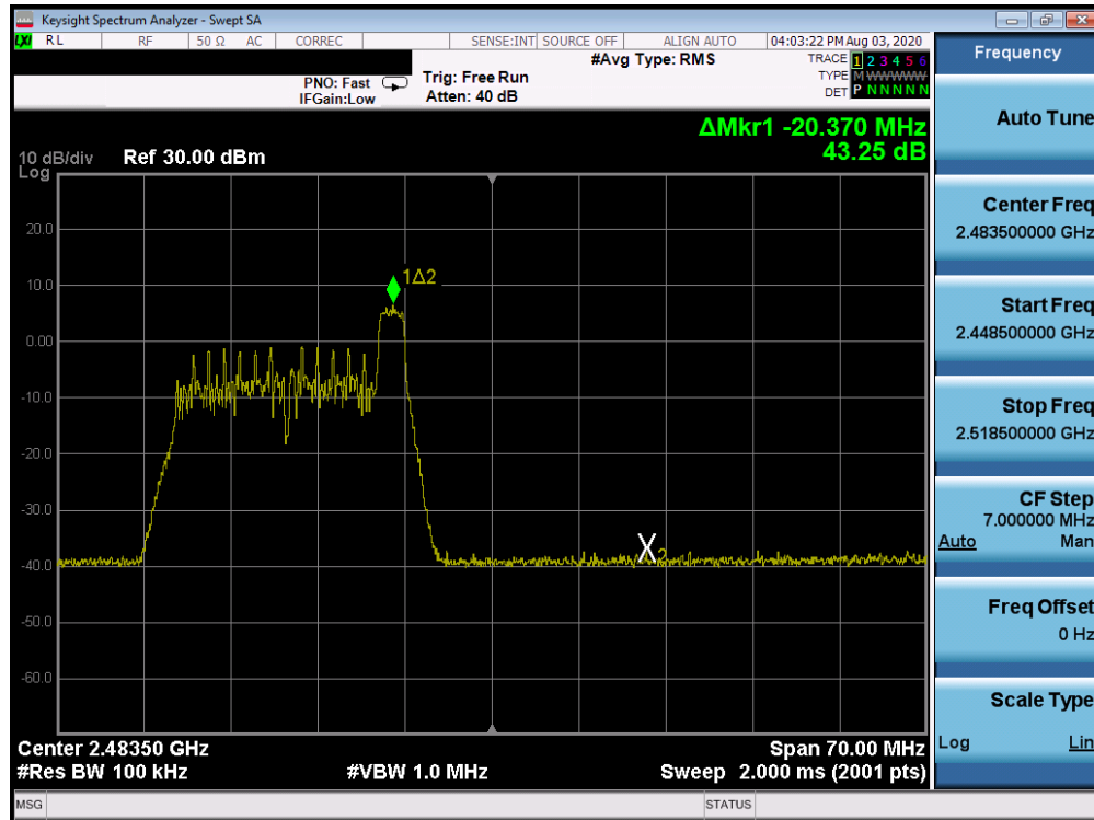
Plot 7-83. Band Edge ANT WF8 (802.11ax OFDMA – RU26 Index 8 – Ch. 12)
