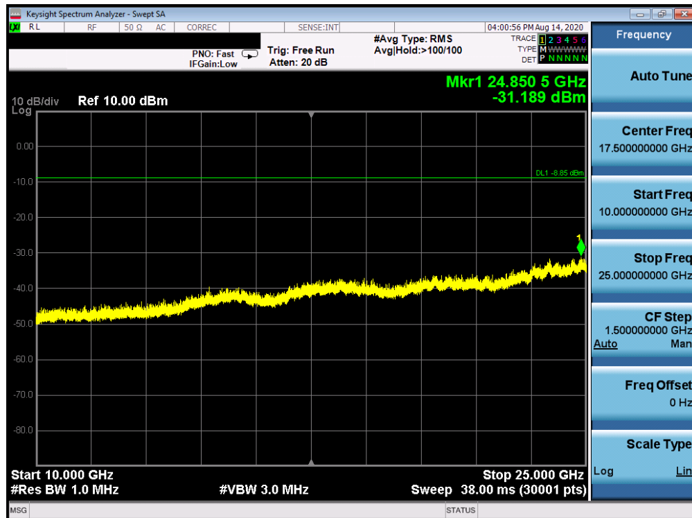
Plot 7-140. Conducted Spurious Plot ANT WF7b (802.11ax OFDMA – RU242 – Ch. 11)
