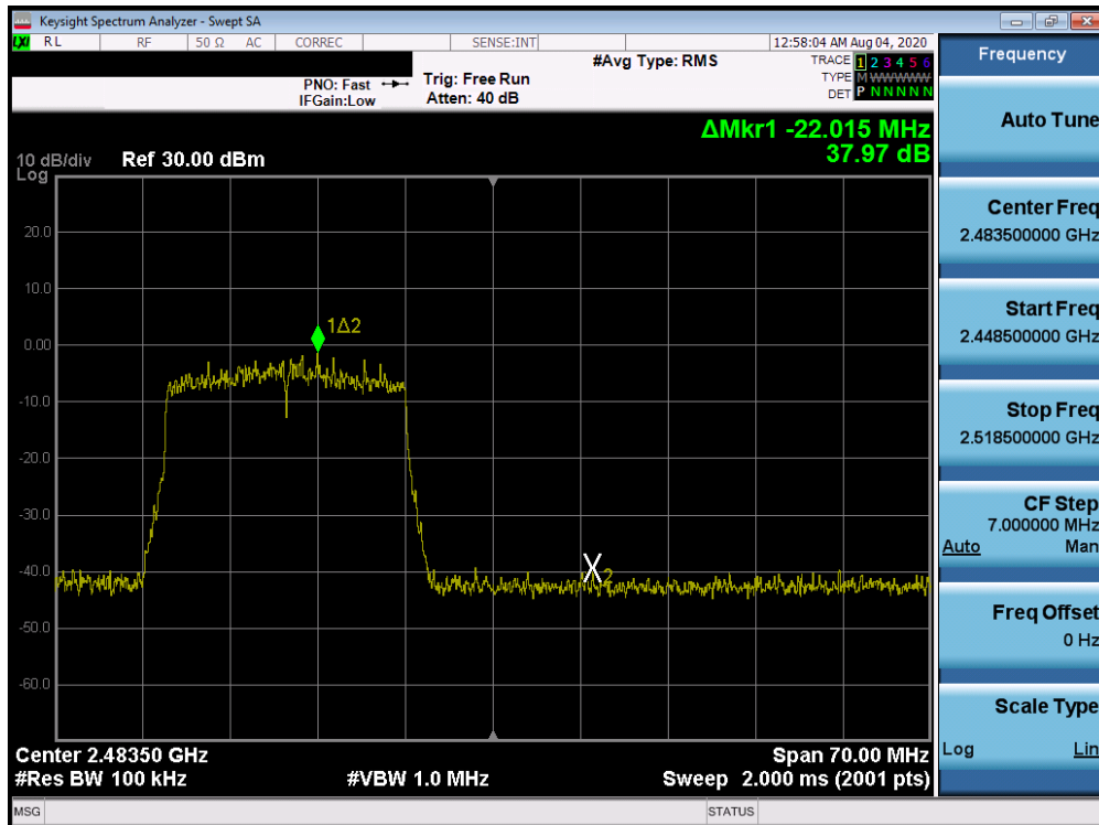
Plot 7-116. Band Edge ANT WF7b (802.11ax OFDMA – RU242 – Ch. 12)
