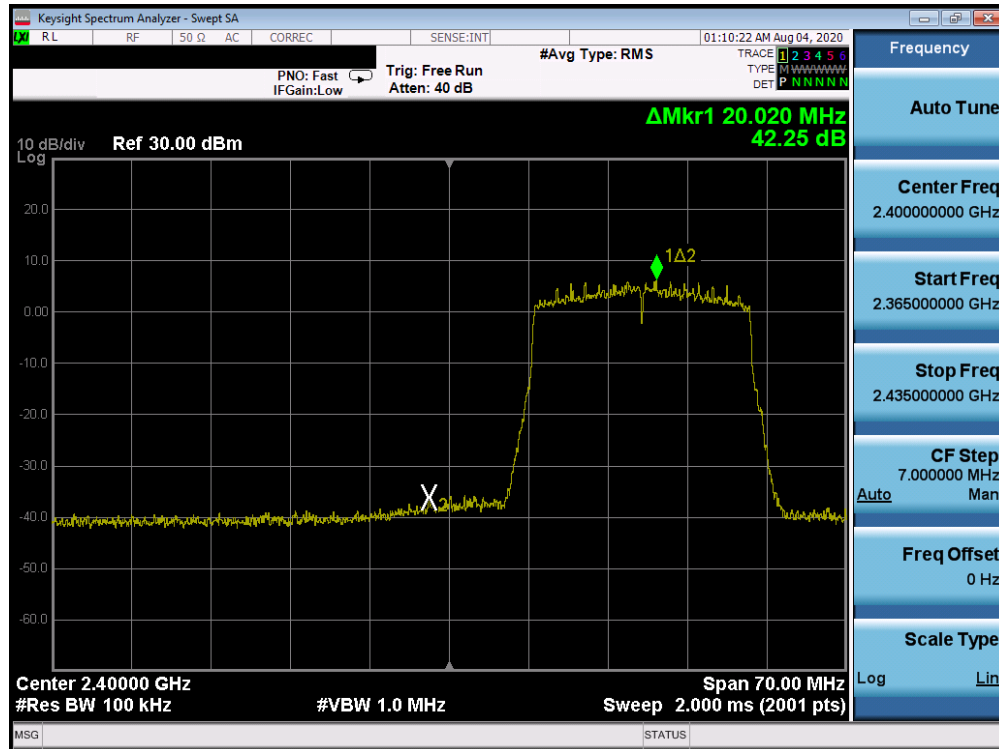
Plot 7-107. Band Edge ANT WF7b (802.11ax OFDMA – RU242 – Ch. 2)
