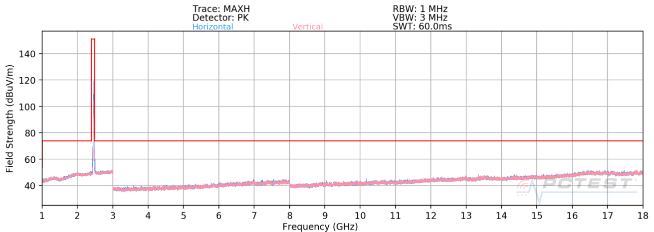
Plot 7-143. Radiated Spurious Emissions above 1GHz ANT WF8 (802.11ax OFDMA – RU26 – Ch. 11)
