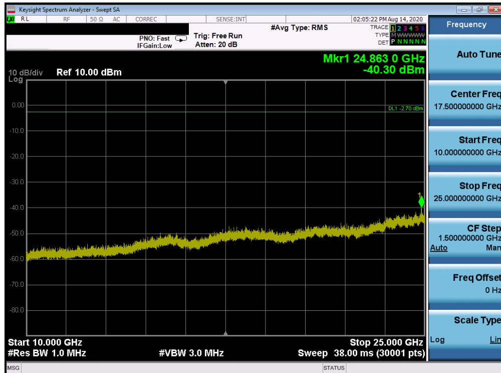
Plot 7-120. Conducted Spurious Plot ANT WF8 (802.11ax OFDMA – RU26 – Ch. 6)
