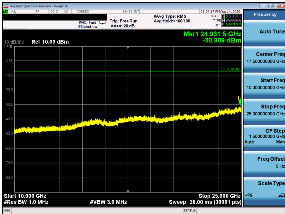
Plot 7-136. Conducted Spurious Plot ANT WF7b (802.11ax OFDMA – RU242 – Ch. 1)
