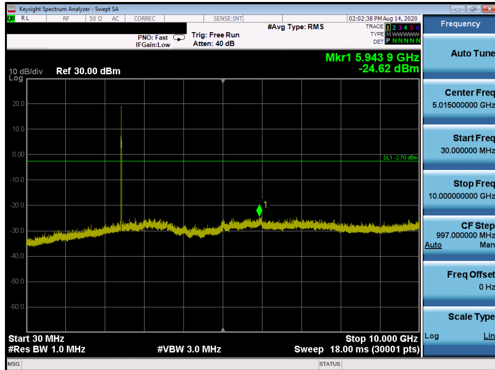
Plot 7-119. Conducted Spurious Plot ANT WF8 (802.11ax OFDMA – RU26 – Ch. 6)
