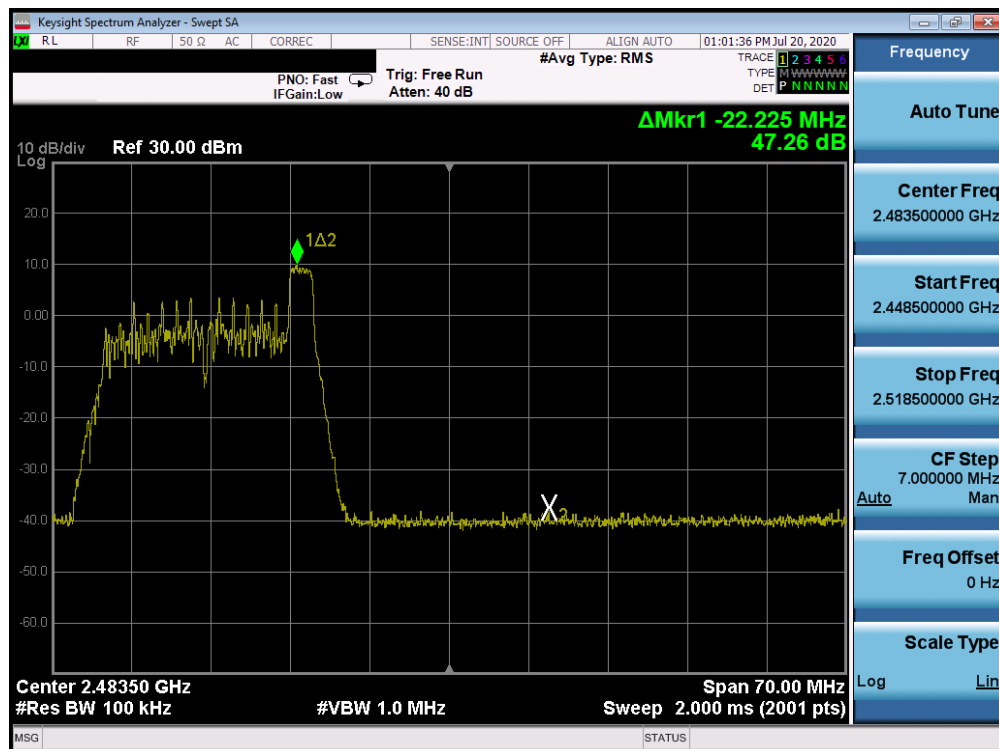
Plot 7-104. Band Edge ANT WF7b (802.11ax OFDMA – RU26 Index 8 – Ch. 11)
