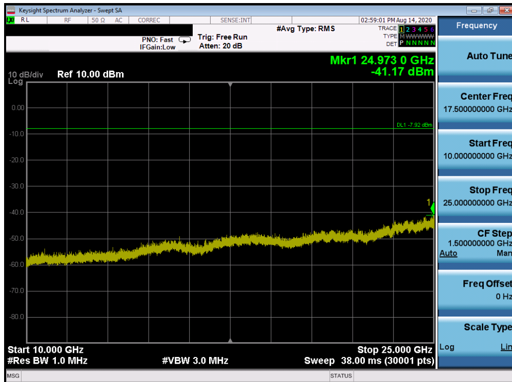
Plot 7-128. Conducted Spurious Plot ANT WF8 (802.11ax OFDMA – RU242 – Ch. 11)
