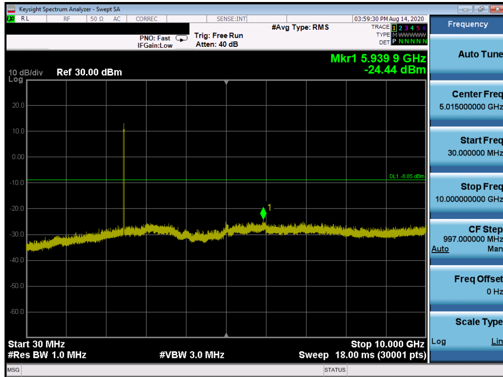
Plot 7-139. Conducted Spurious Plot ANT WF7b (802.11ax OFDMA – RU242 – Ch. 11)
