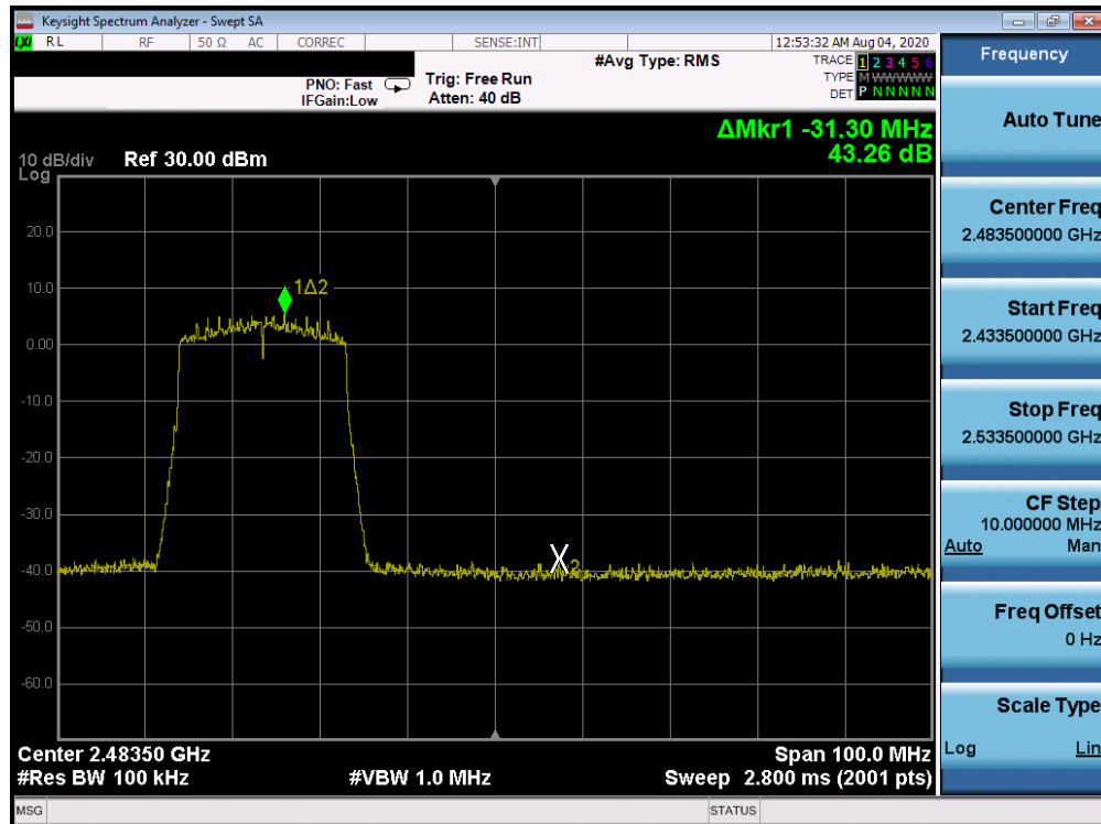
Plot 7-114. Band Edge ANT WF7b (802.11ax OFDMA – RU242 – Ch. 10)
