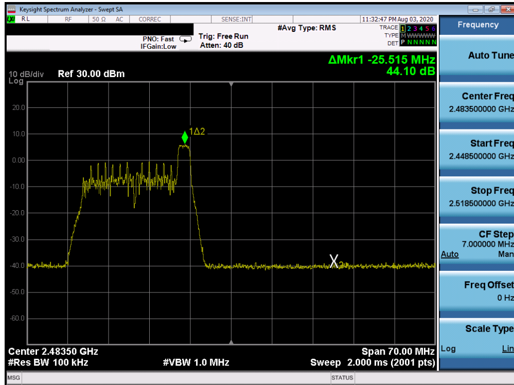
Plot 7-105. Band Edge ANT WF7b (802.11ax OFDMA – RU26 Index 8 – Ch. 12)
