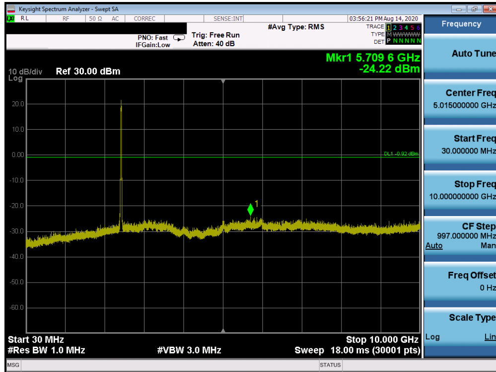
Plot 7-137. Conducted Spurious Plot ANT WF7b (802.11ax OFDMA – RU242 – Ch. 6)
