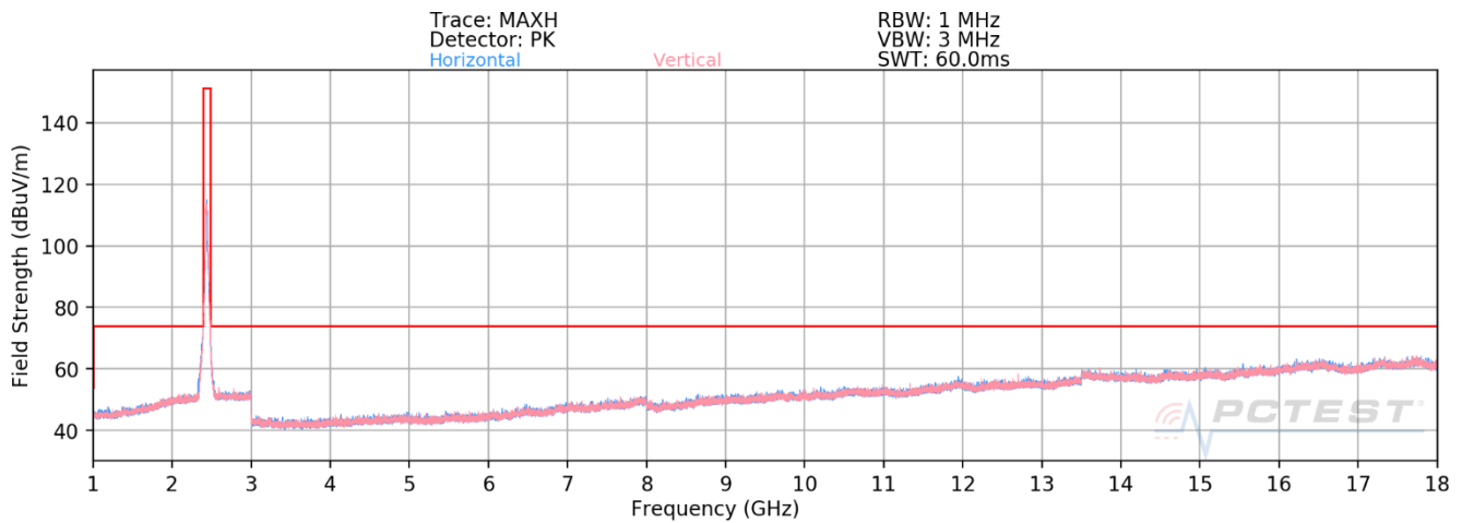
Plot 7-151. Radiated Spurious Emissions above 1GHz ANT WF7b (802.11ax OFDMA – RU242 – Ch. 6)
