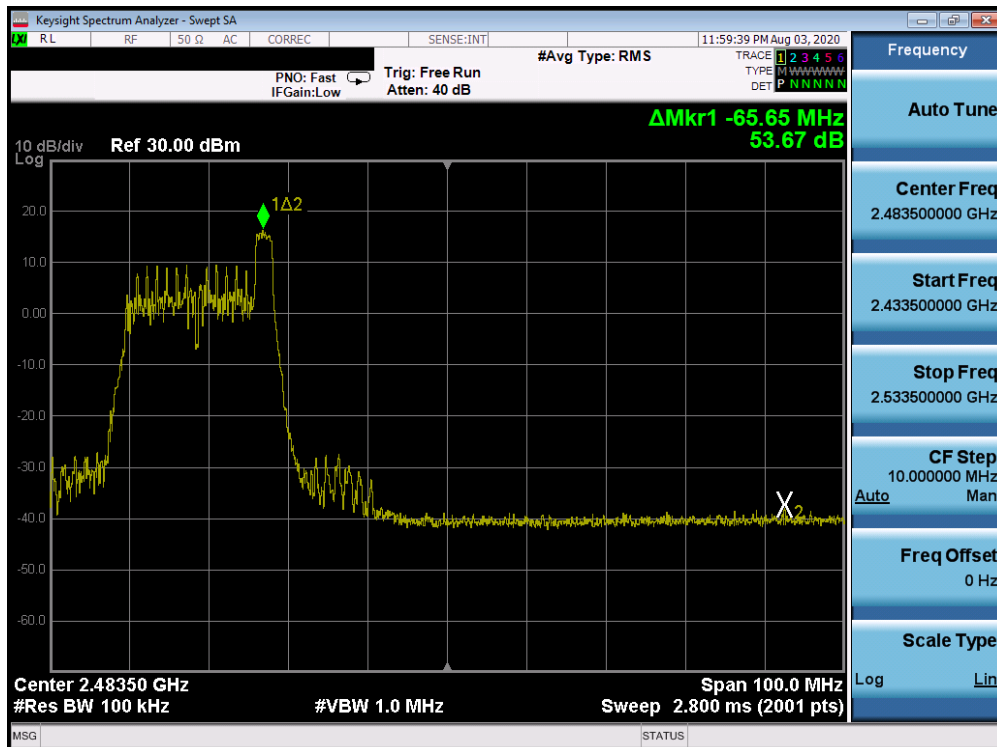
Plot 7-102. Band Edge ANT WF7b (802.11ax OFDMA – RU26 Index 8 – Ch. 9)
