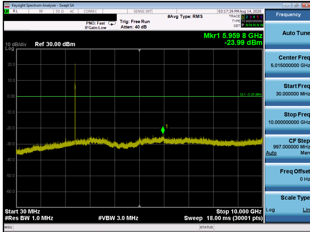
Plot 7-129. Conducted Spurious Plot ANT WF7b (802.11ax OFDMA – RU26 – Ch. 1)
