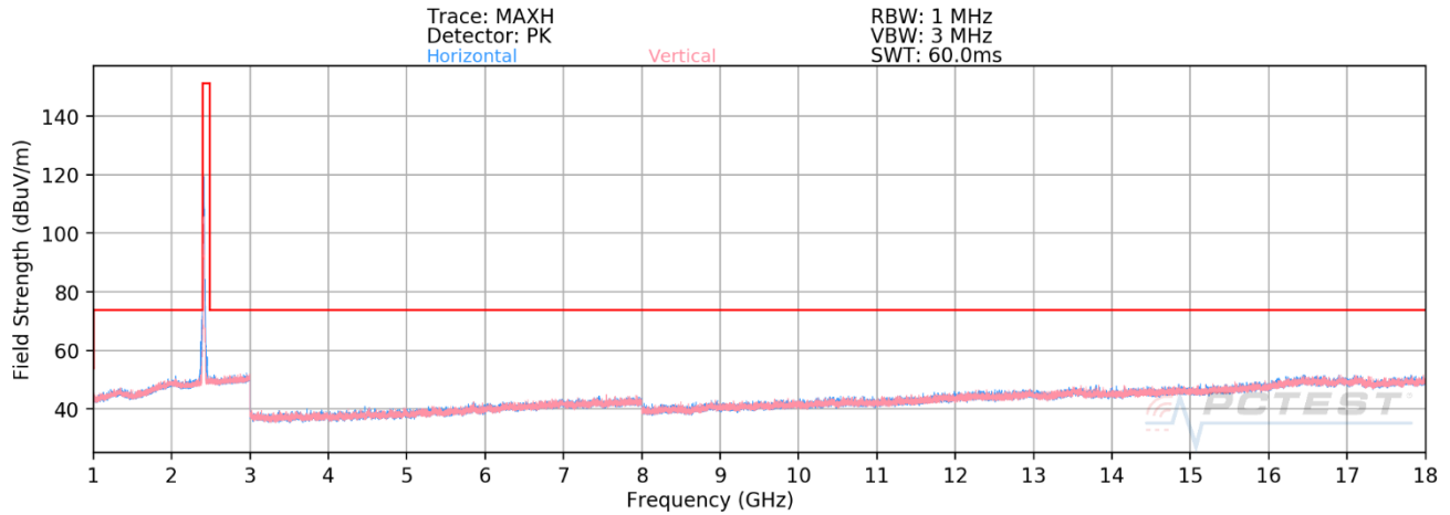
Plot 7-141. Radiated Spurious Emissions above 1GHz ANT WF8 (802.11ax OFDMA – RU26 – Ch. 1)
