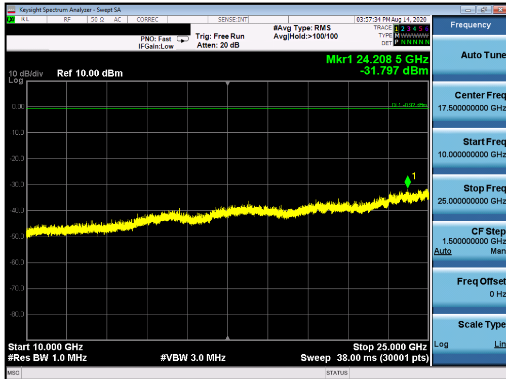
Plot 7-138. Conducted Spurious Plot ANT WF7b (802.11ax OFDMA – RU242 – Ch. 6)
