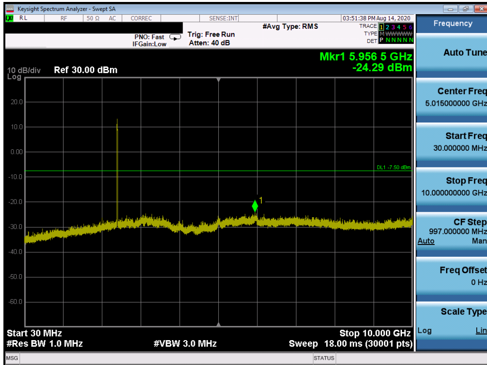
Plot 7-135. Conducted Spurious Plot ANT WF7b (802.11ax OFDMA – RU242 – Ch. 1)
