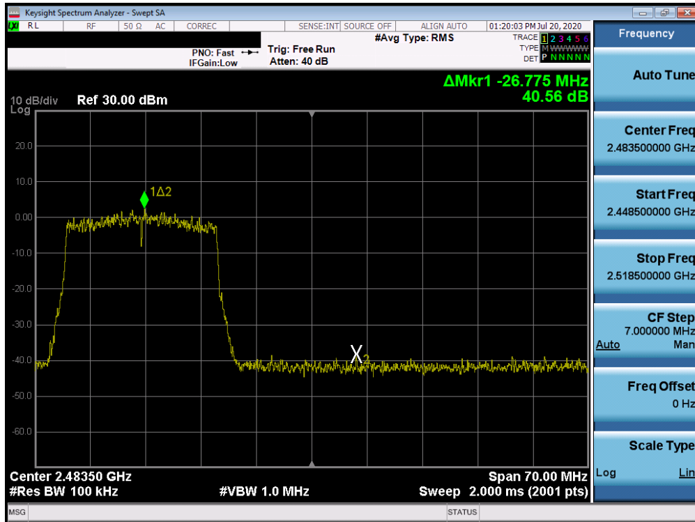
Plot 7-115. Band Edge ANT WF7b (802.11ax OFDMA – RU242 – Ch. 11)
