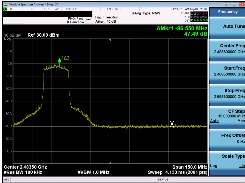
Plot 7-111. Band Edge ANT WF7b (802.11ax OFDMA – RU242 – Ch. 7)
