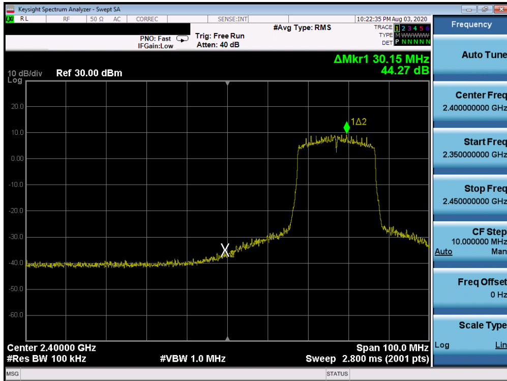
Plot 7-87. Band Edge ANT WF8 (802.11ax OFDMA – RU242 – Ch. 4)
