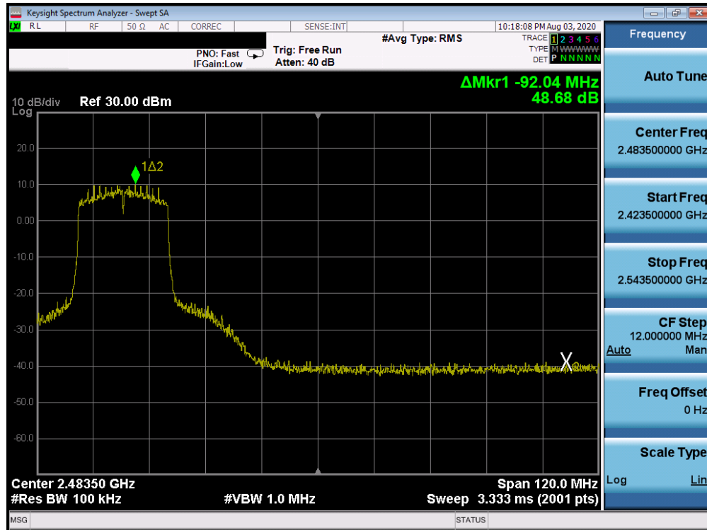
Plot 7-89. Band Edge ANT WF8 (802.11ax OFDMA – RU242 – Ch. 7)
