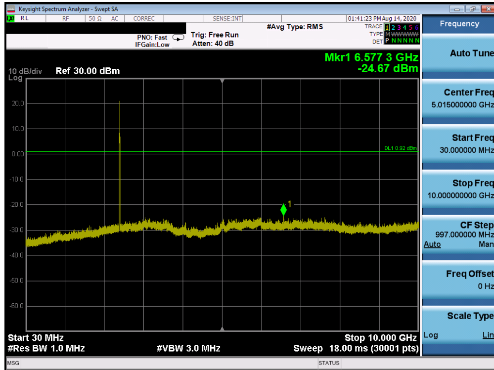
Plot 7-117. Conducted Spurious Plot ANT WF8 (802.11ax OFDMA – RU26 – Ch. 1)
