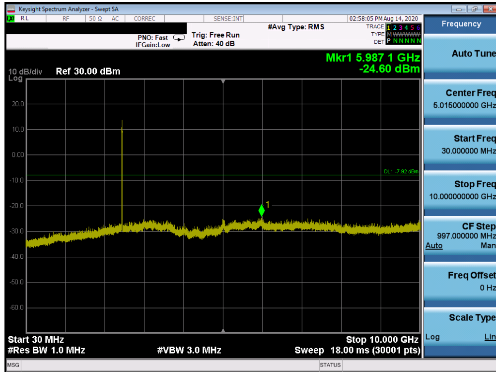
Plot 7-127. Conducted Spurious Plot ANT WF8 (802.11ax OFDMA – RU242 – Ch. 11)
