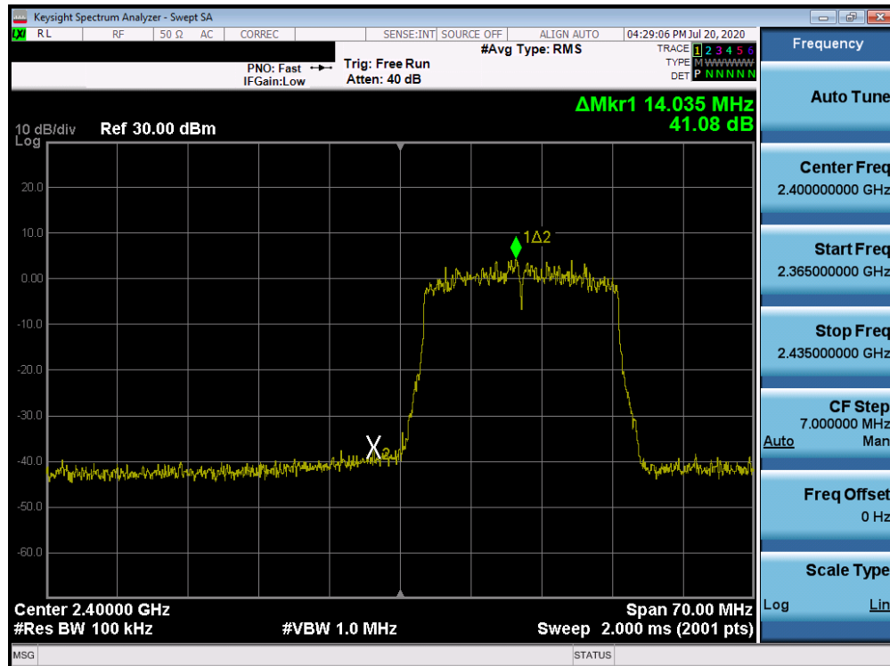
Plot 7-84. Band Edge ANT WF8 (802.11ax OFDMA – RU242 – Ch. 1)
