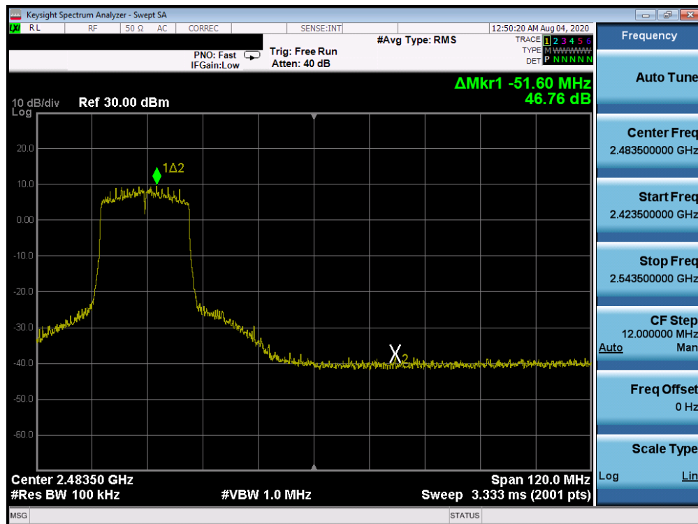
Plot 7-112. Band Edge ANT WF7b (802.11ax OFDMA – RU242 – Ch. 8)
