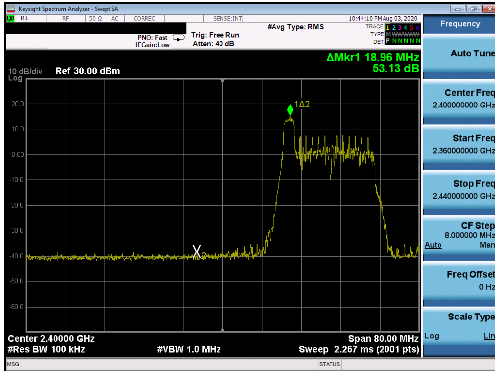
Plot 7-97. Band Edge ANT WF7b (802.11ax OFDMA – RU26 Index 0 – Ch. 3)
