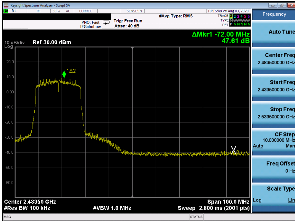
Plot 7-91. Band Edge ANT WF8 (802.11ax OFDMA – RU242 – Ch. 9)
