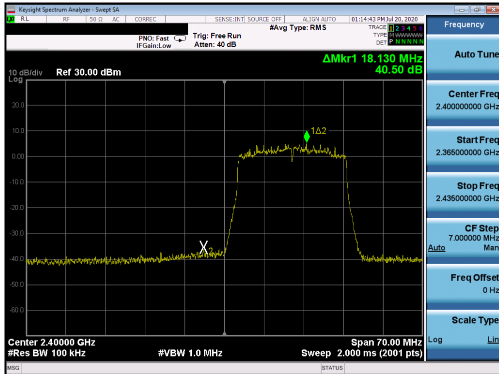
Plot 7-106. Band Edge ANT WF7b (802.11ax OFDMA – RU242 – Ch. 1)
