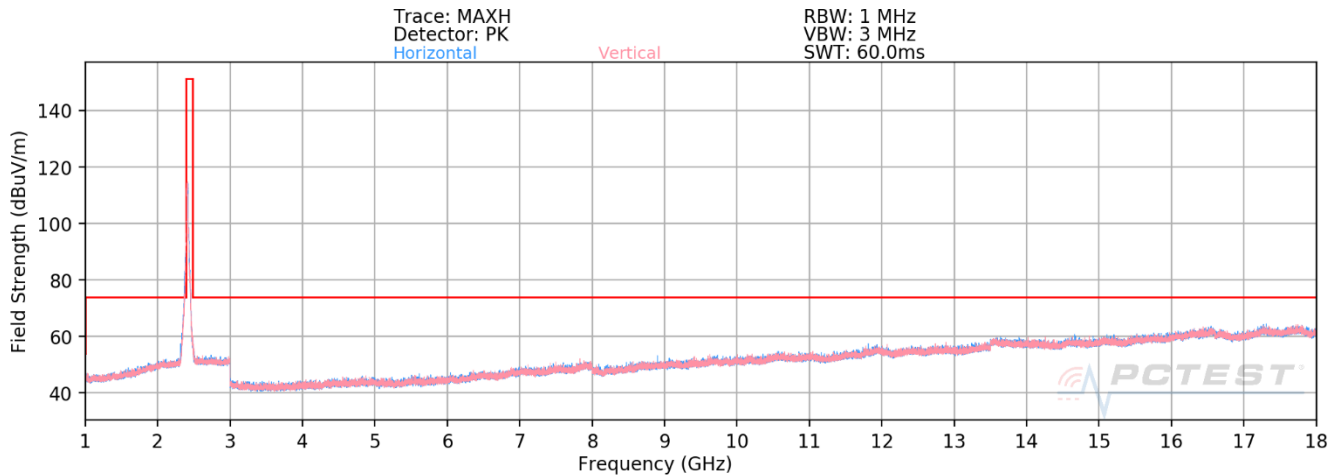
Plot 7-150. Radiated Spurious Emissions above 1GHz ANT WF7b (802.11ax OFDMA – RU242 – Ch. 1)
