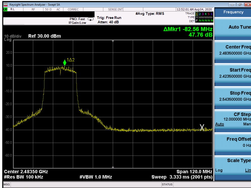
Plot 7-113. Band Edge ANT WF7b (802.11ax OFDMA – RU242 – Ch. 9)
