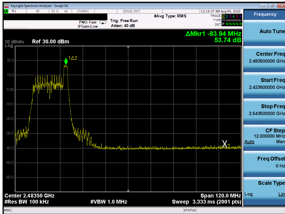
Plot 7-100. Band Edge ANT WF7b (802.11ax OFDMA – RU26 Index 8 – Ch. 7)
