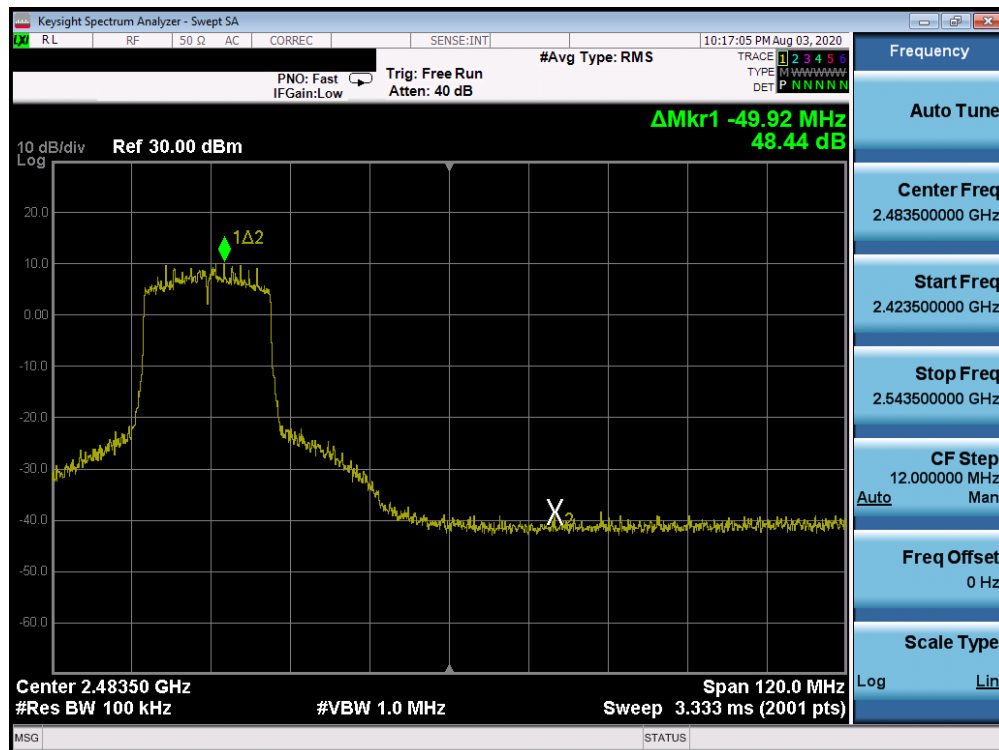
Plot 7-90. Band Edge ANT WF8 (802.11ax OFDMA – RU242 – Ch. 8)
