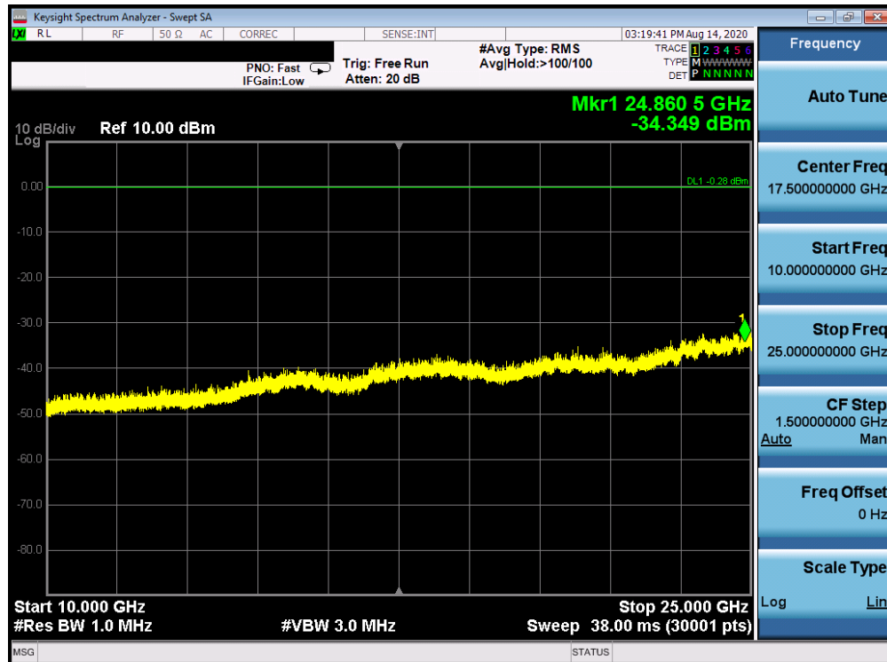
Plot 7-130. Conducted Spurious Plot ANT WF7b (802.11ax OFDMA – RU26 – Ch. 1)
