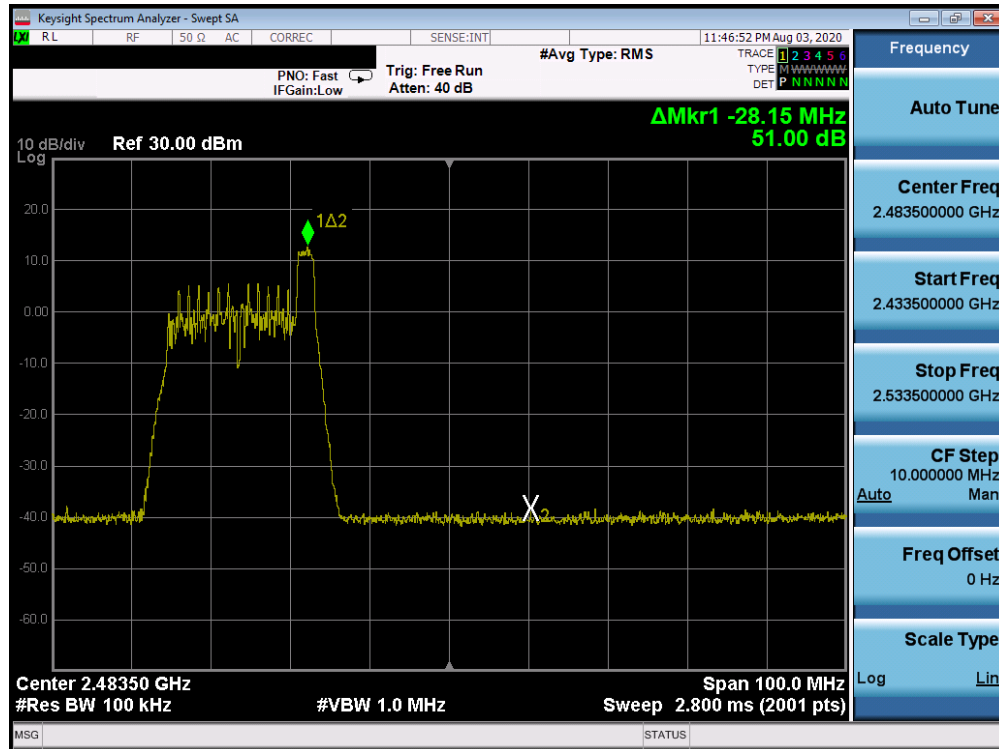
Plot 7-103. Band Edge ANT WF7b (802.11ax OFDMA – RU26 Index 8 – Ch. 10)
