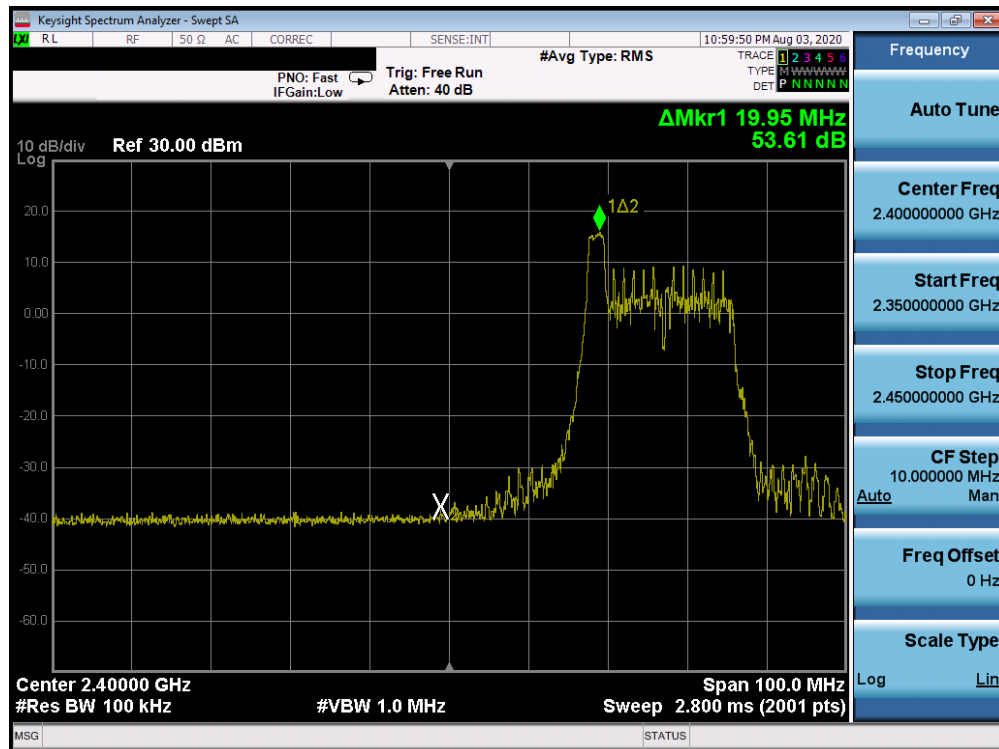
Plot 7-98. Band Edge ANT WF7b (802.11ax OFDMA – RU26 Index 0 – Ch. 4)
