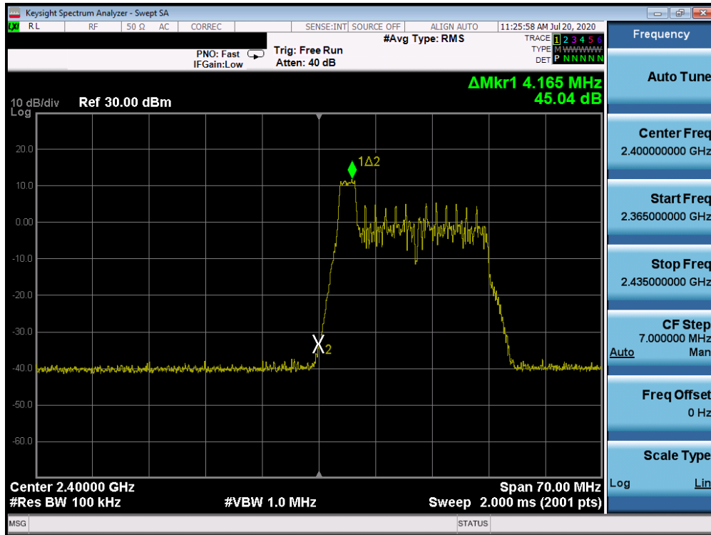
Plot 7-95. Band Edge ANT WF7b (802.11ax OFDMA – RU26 Index 0 – Ch. 1)
