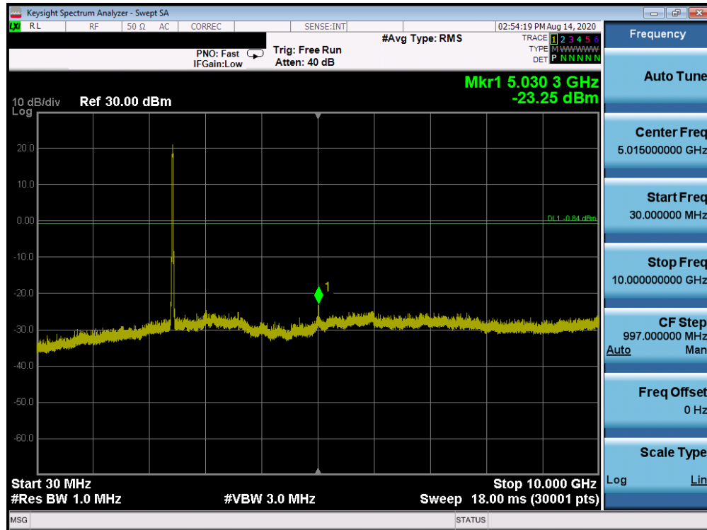
Plot 7-125. Conducted Spurious Plot ANT WF8 (802.11ax OFDMA – RU242 – Ch. 6)
