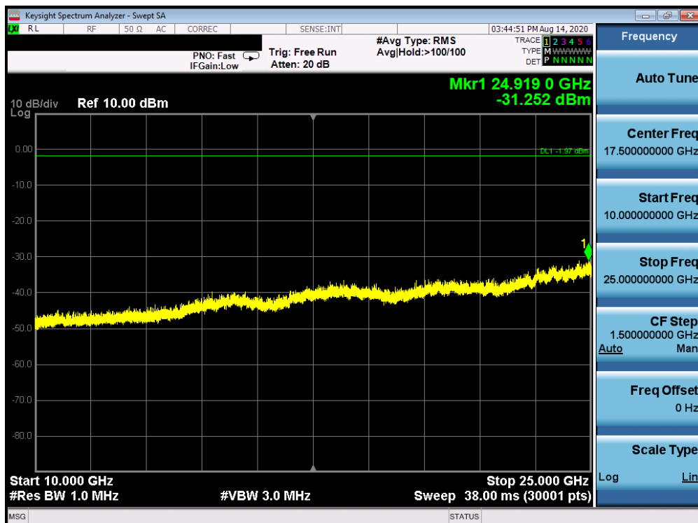
Plot 7-134. Conducted Spurious Plot ANT WF7b (802.11ax OFDMA – RU26 – Ch. 11)
