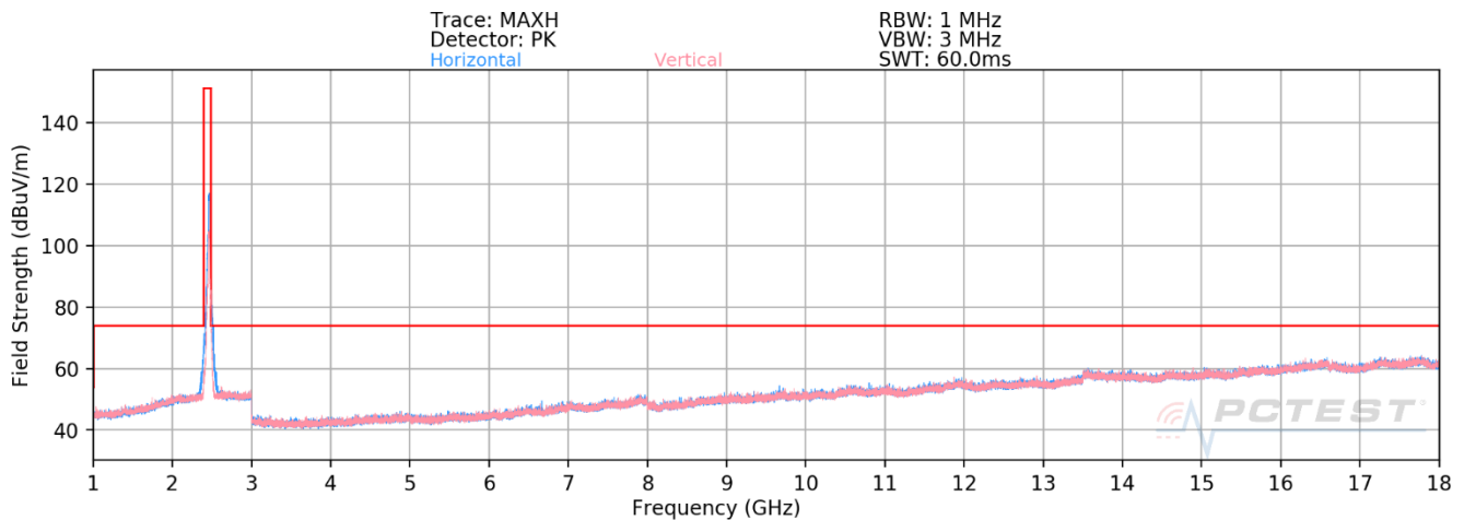
Plot 7-146. Radiated Spurious Emissions above 1GHz ANT WF8 (802.11ax OFDMA – RU242 – Ch. 11)
