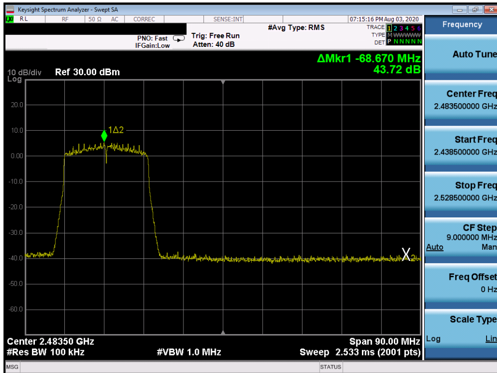
Plot 7-92. Band Edge ANT WF8 (802.11ax OFDMA – RU242 – Ch. 10)
