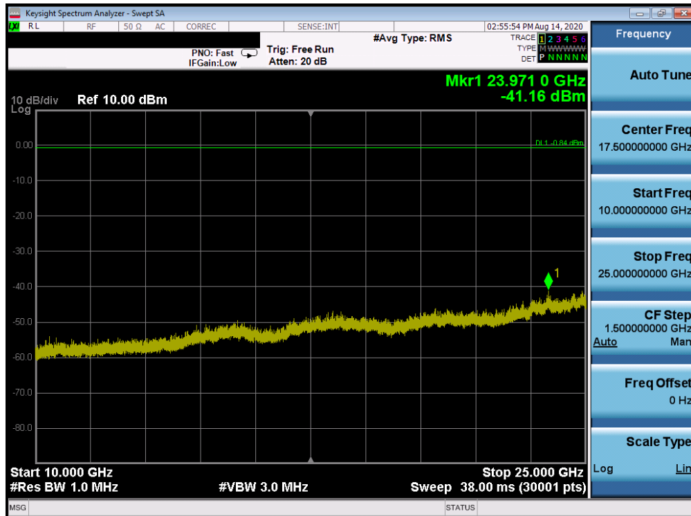
Plot 7-126. Conducted Spurious Plot ANT WF8 (802.11ax OFDMA – RU242 – Ch. 6)
