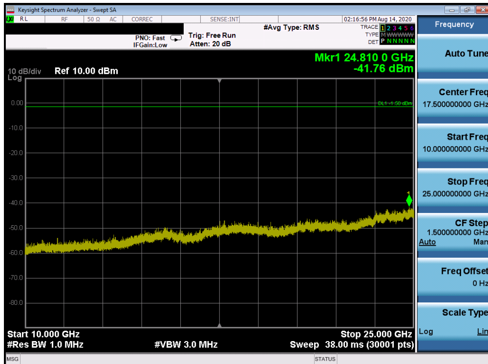
Plot 7-122. Conducted Spurious Plot ANT WF8 (802.11ax OFDMA – RU26 – Ch. 11)
