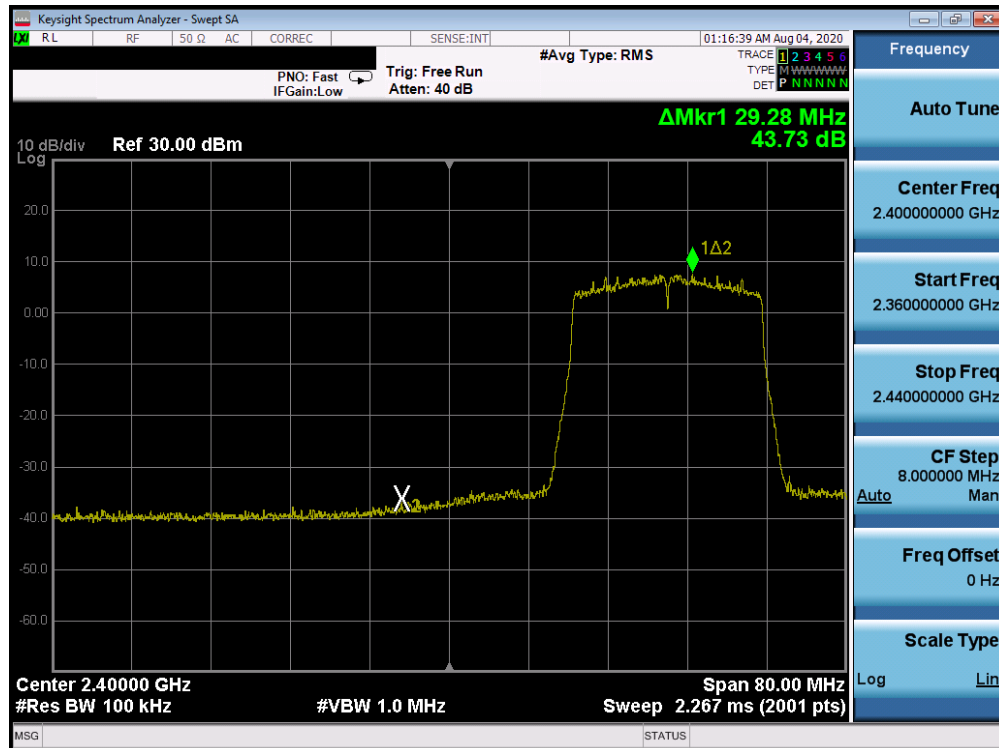
Plot 7-108. Band Edge ANT WF7b (802.11ax OFDMA – RU242 – Ch. 3)
