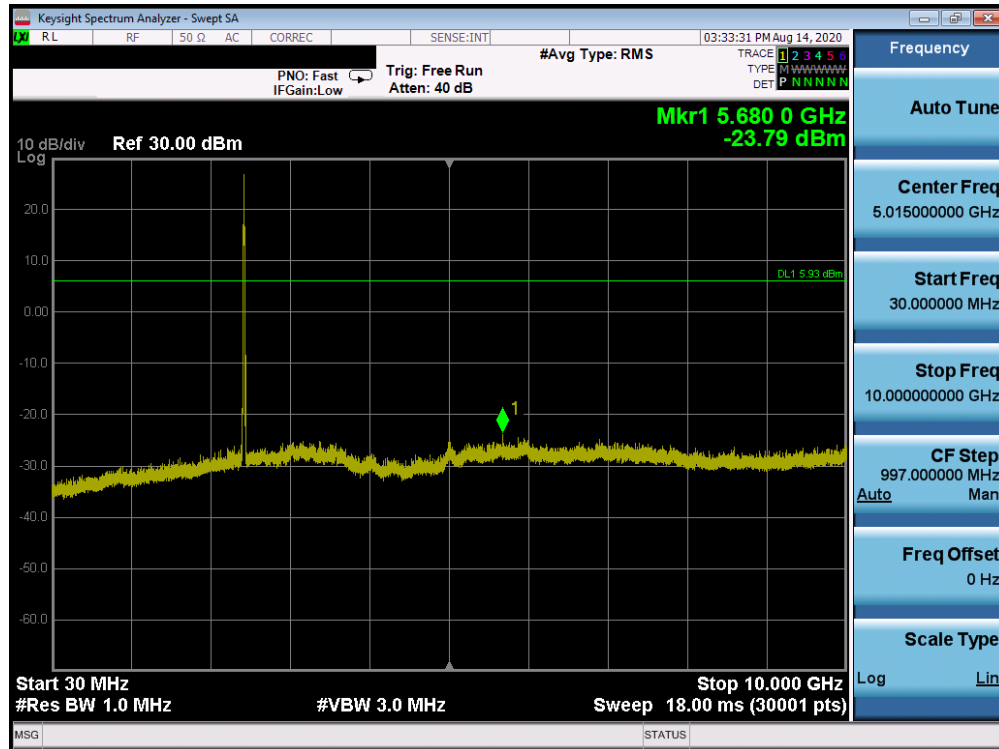
Plot 7-131. Conducted Spurious Plot ANT WF7b (802.11ax OFDMA – RU26 – Ch. 6)
