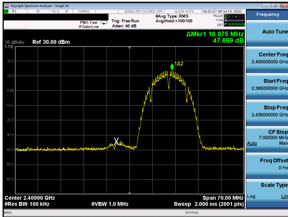
Plot 7-80. Band Edge Plot ANT WF7b (802.11b – Ch. 1)
