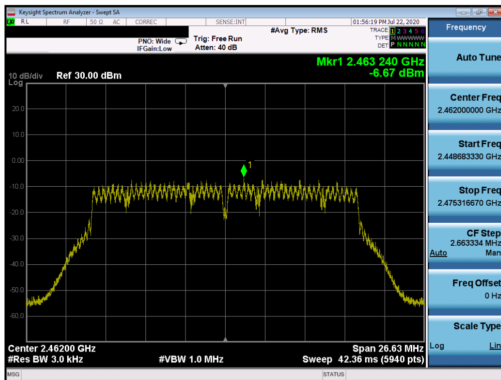
Plot 7-36. Power Spectral Density Plot ANT WF7b (802.11n (2.4GHz) – Ch. 11)
