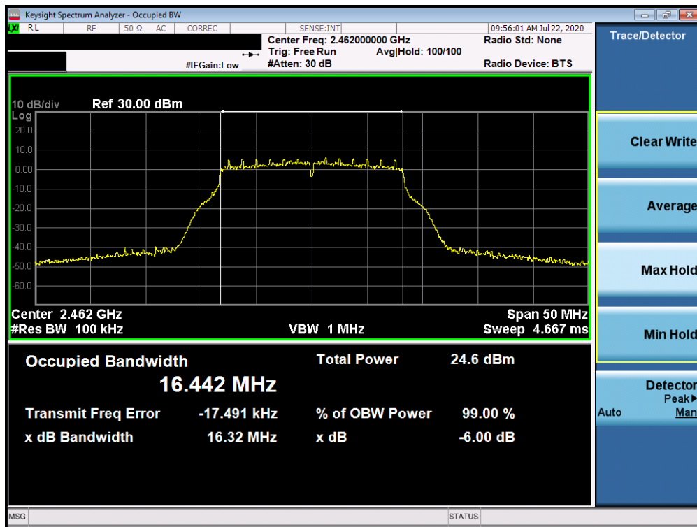
Plot 7-15. 6dB Bandwidth Plot ANT WF7b (802.11g – Ch. 11)
