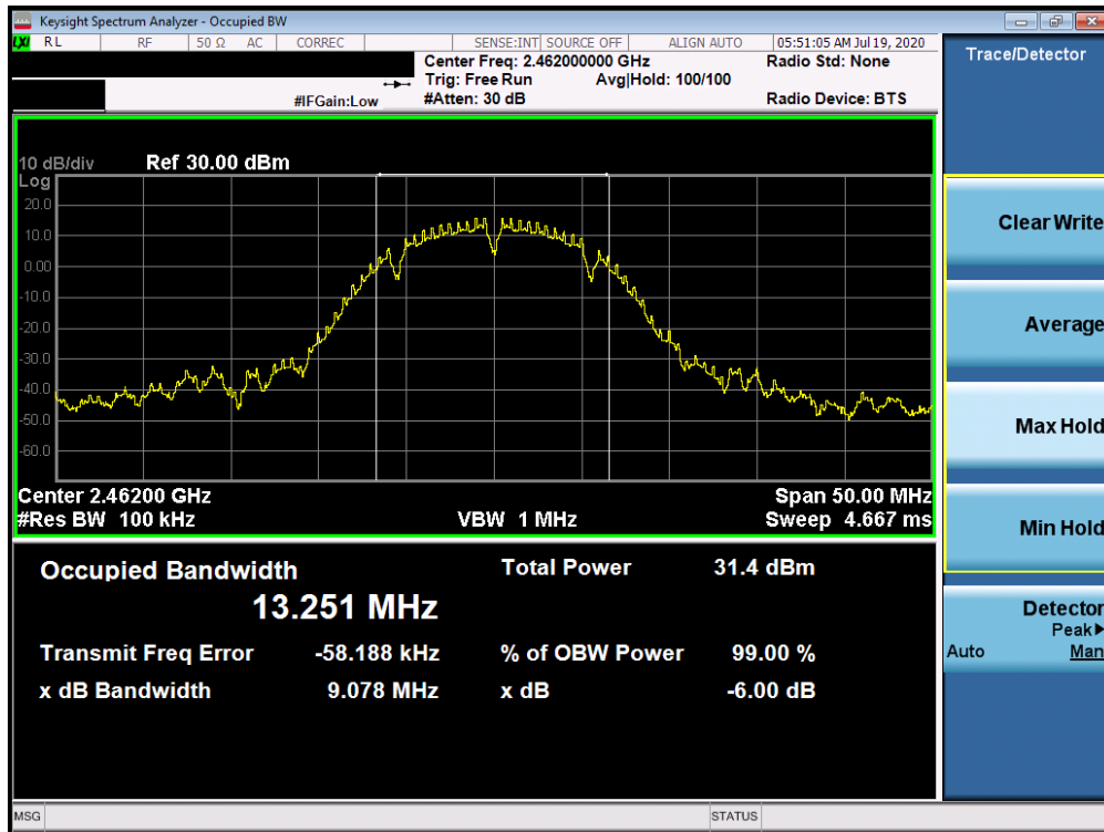
Plot 7-12. 6dB Bandwidth Plot ANT WF7b (802.11b – Ch. 11)
