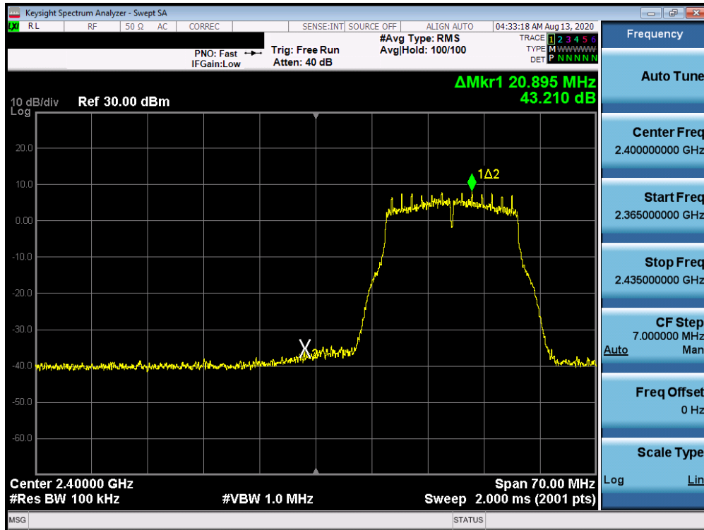
Plot 7-57. Band Edge Plot ANT WF8 (802.11g– Ch. 2)
