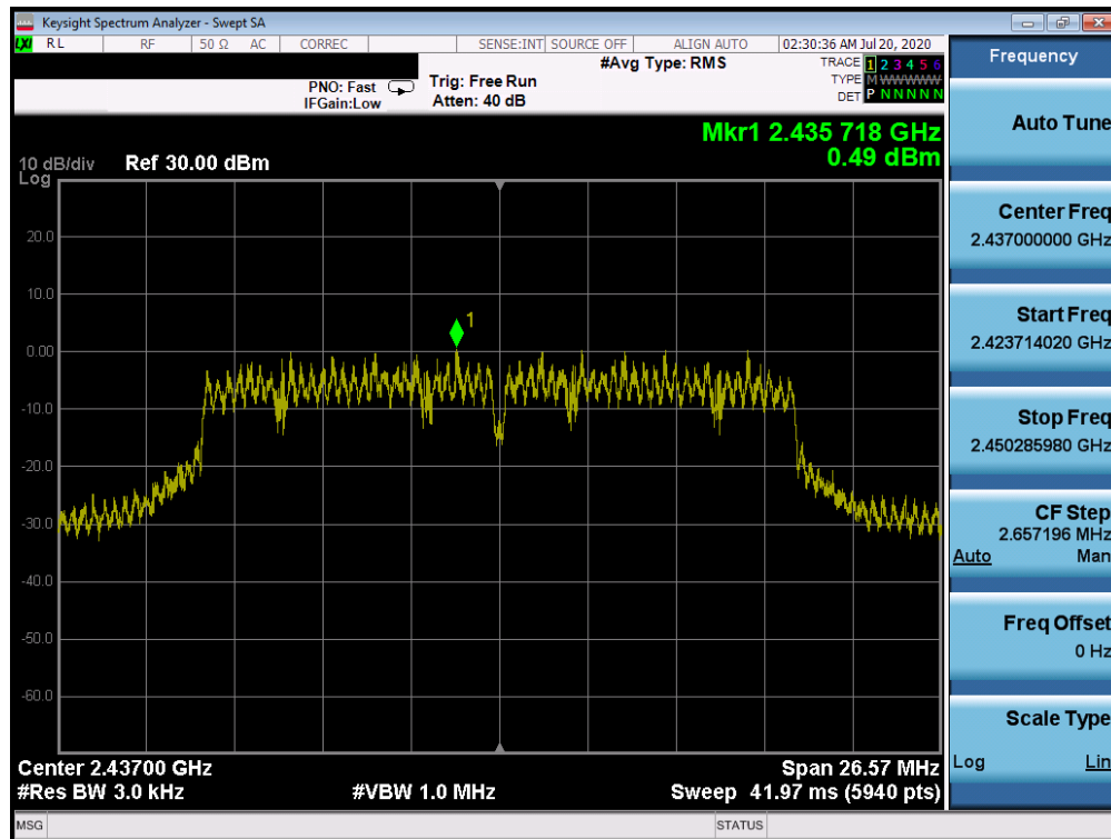
Plot 7-46. Power Spectral Density Plot CDD ANT WF7b (802.11n (2.4GHz) – Ch. 6)
