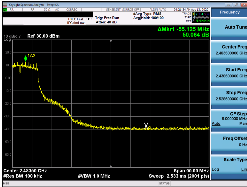
Plot 7-61. Band Edge Plot ANT WF8 (802.11g – Ch. 7)
