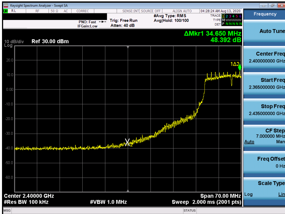
Plot 7-60. Band Edge Plot ANT WF8 (802.11g– Ch. 5)
