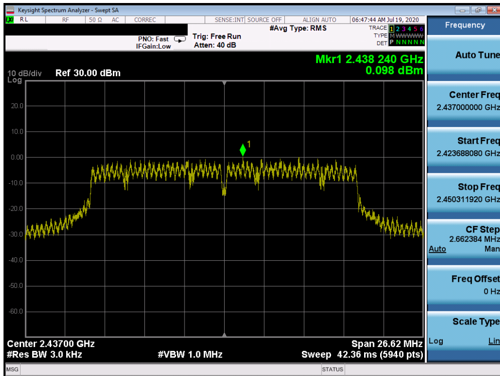
Plot 7-35. Power Spectral Density Plot ANT WF7b (802.11n (2.4GHz) – Ch. 6)
