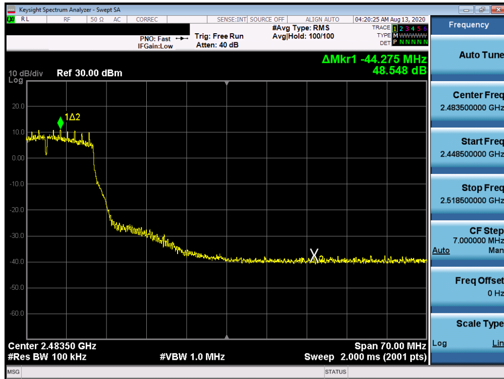
Plot 7-63. Band Edge Plot ANT WF8 (802.11g - Ch. 9)
