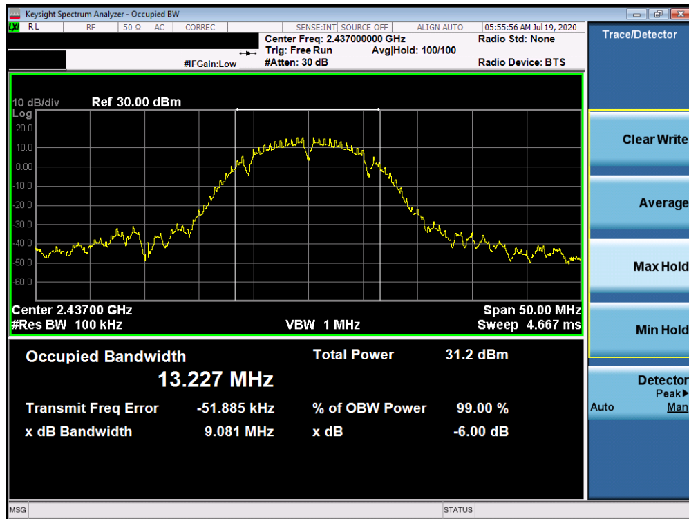
Plot 7-11. 6dB Bandwidth Plot ANT WF7b (802.11b – Ch. 6)
