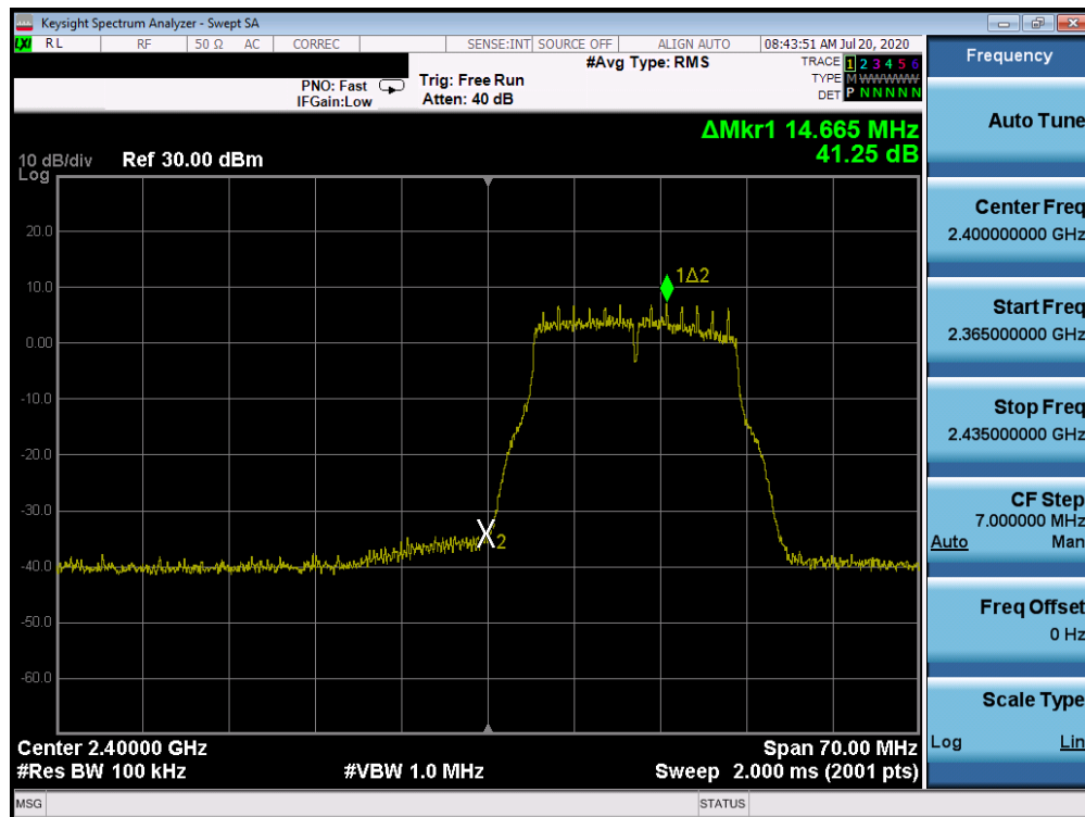
Plot 7-56. Band Edge Plot ANT WF8 (802.11g– Ch. 1)
