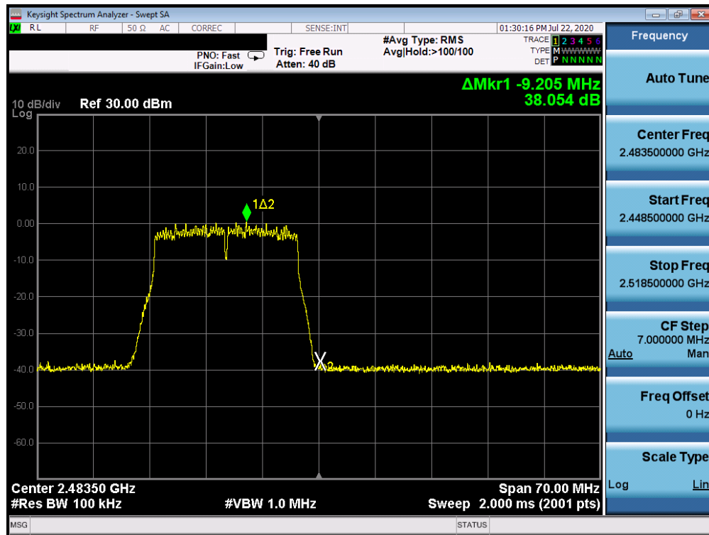
Plot 7-79. Band Edge Plot ANT WF8 (802.11n (2.4GHz) – Ch. 13)
