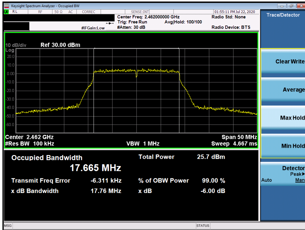
Plot 7-18. 6dB Bandwidth Plot ANT WF7b (802.11n (2.4GHz) – Ch. 11)
