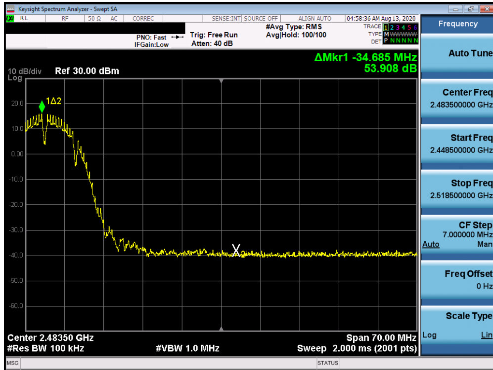
Plot 7-51. Band Edge Plot ANT WF8 (802.11b – Ch. 9)
