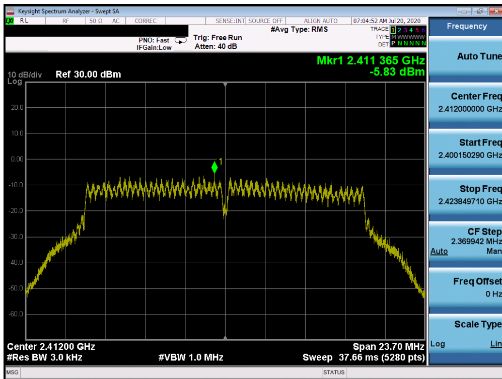
Plot 7-31. Power Spectral Density Plot ANT WF7b (802.11g – Ch. 1)
