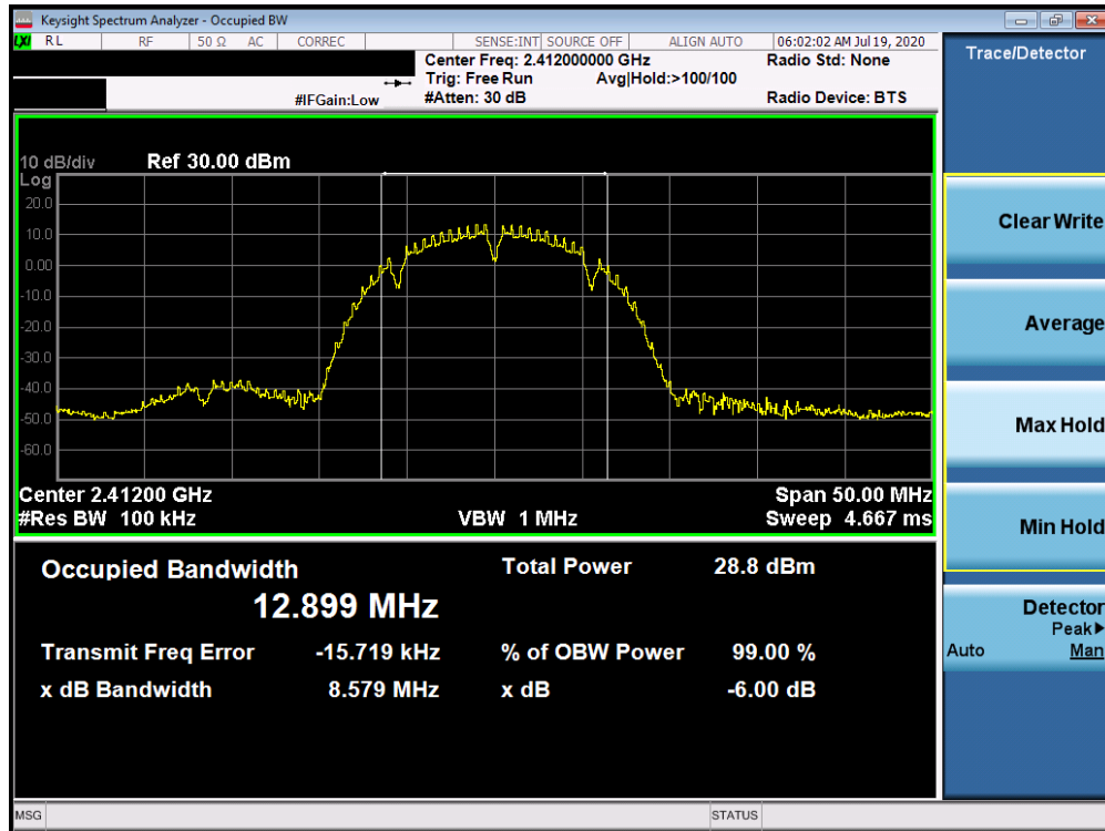
Plot 7-10. 6dB Bandwidth Plot ANT WF7b (802.11b – Ch. 1)
