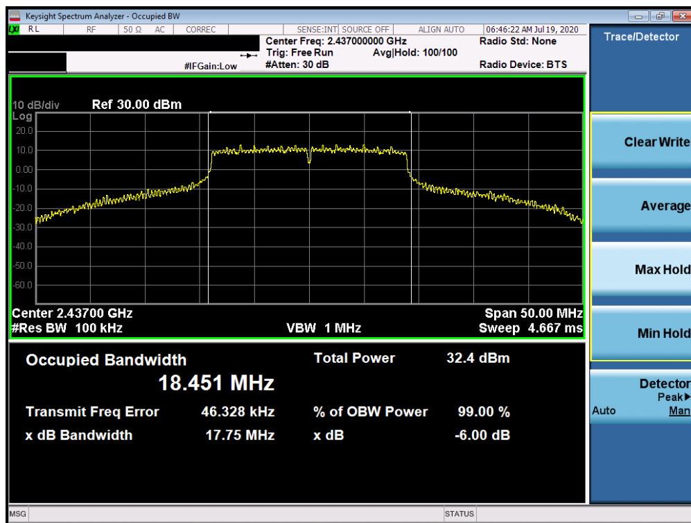
Plot 7-17. 6dB Bandwidth Plot ANT WF7b (802.11n (2.4GHz) – Ch. 6)
