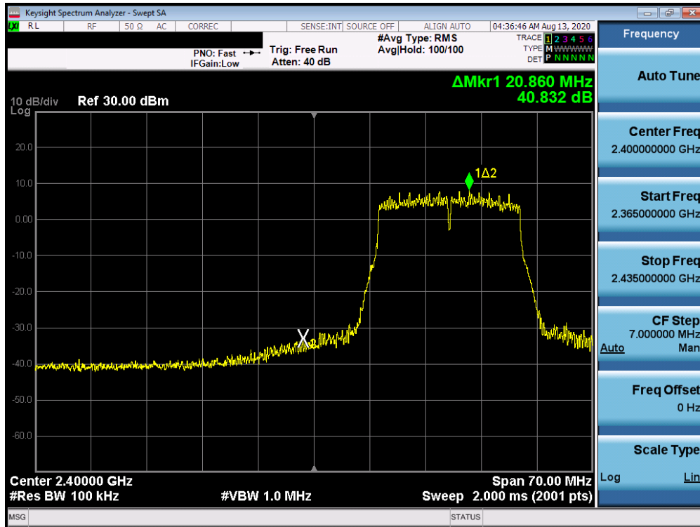
Plot 7-69. Band Edge Plot ANT WF8 (802.11n (2.4GHz) – Ch. 2)
