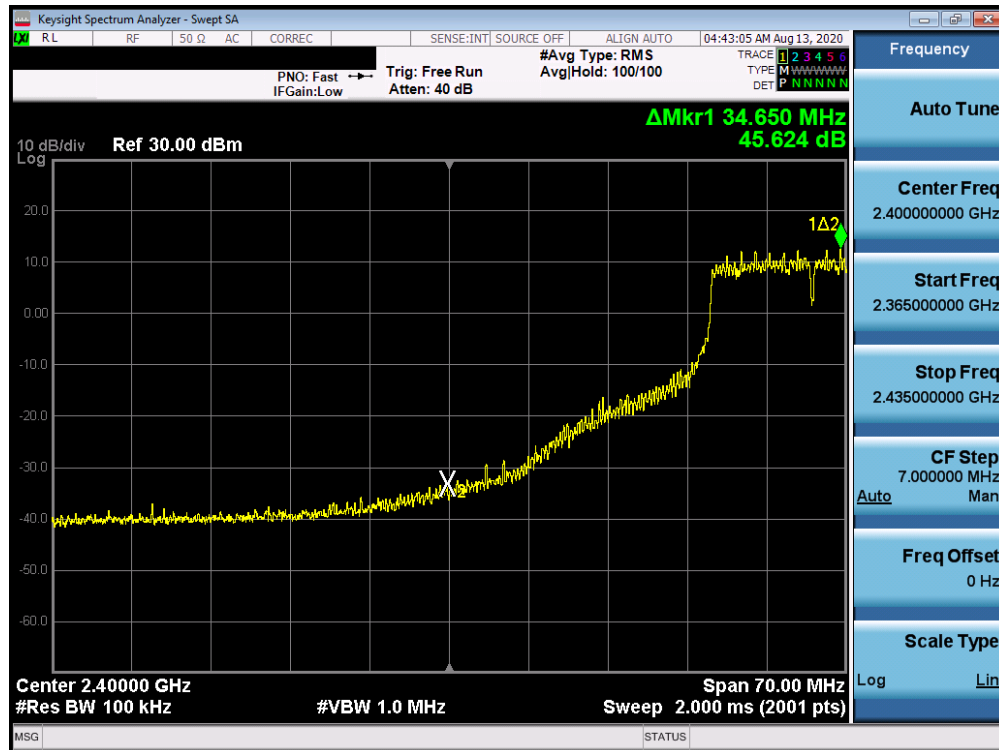
Plot 7-72. Band Edge Plot ANT WF8 (802.11n (2.4GHz) – Ch. 5)
