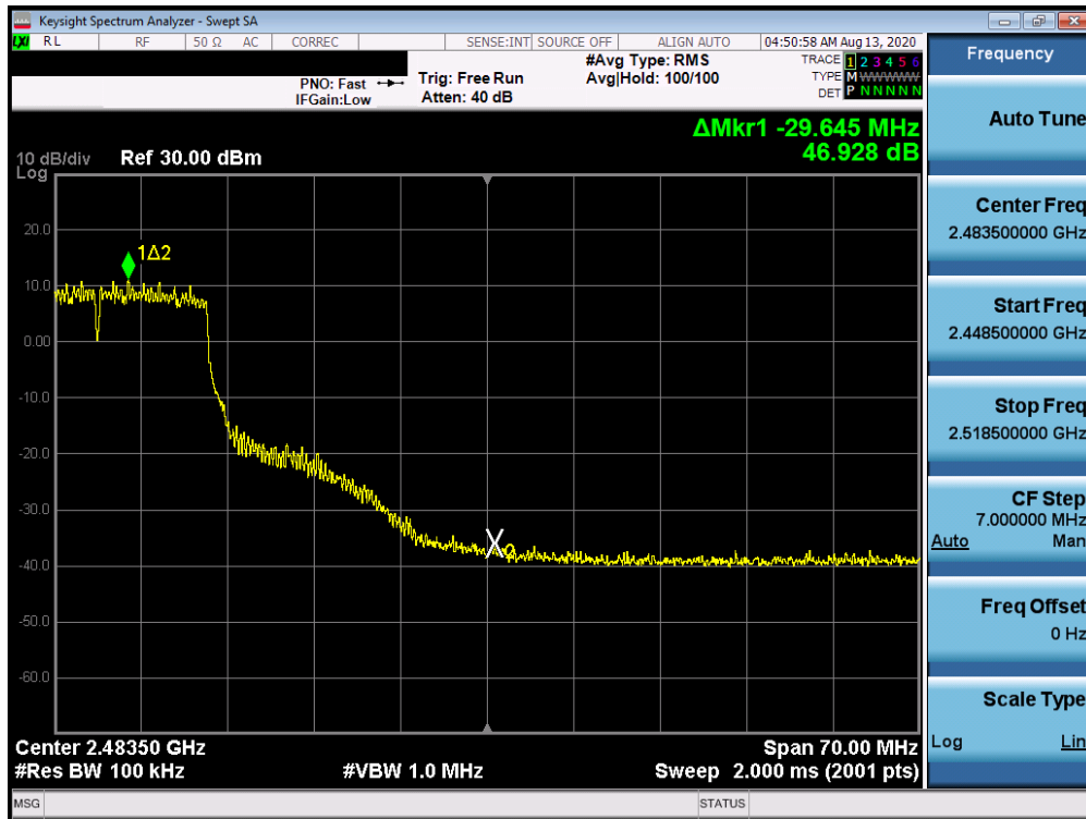
Plot 7-75. Band Edge Plot ANT WF8 (802.11n (2.4GHz) – Ch. 9)
