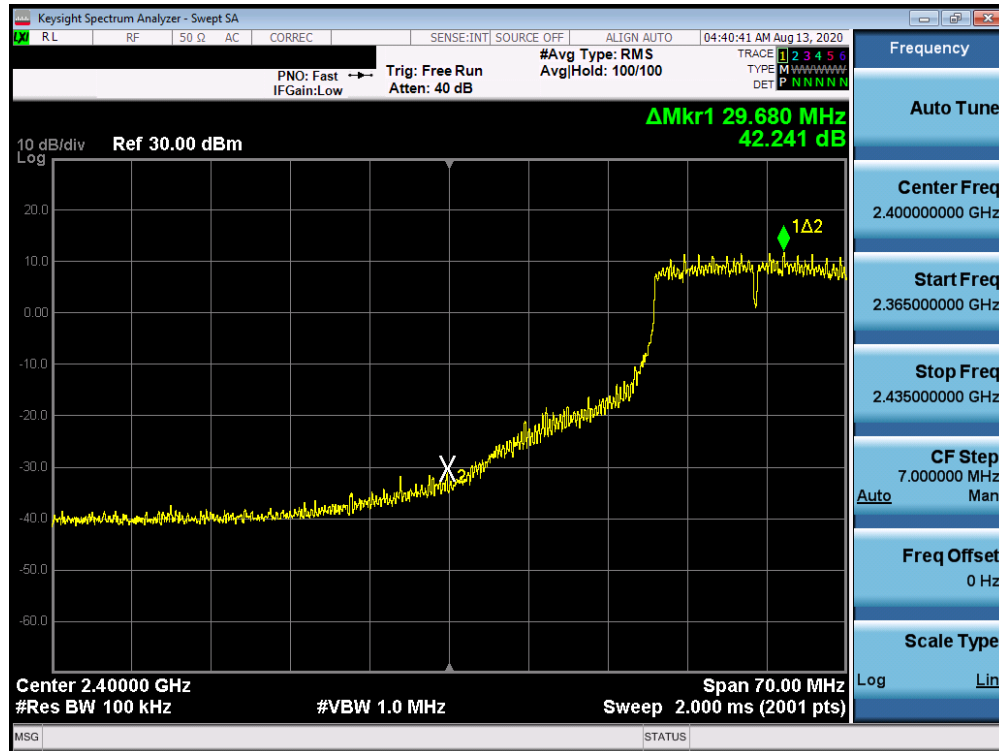
Plot 7-71. Band Edge Plot ANT WF8 (802.11n (2.4GHz) – Ch. 4)
