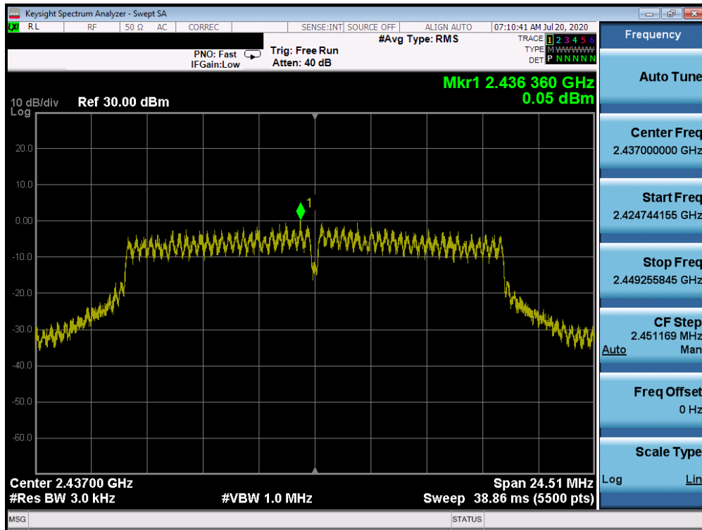
Plot 7-32. Power Spectral Density Plot ANT WF7b (802.11g – Ch. 6)
