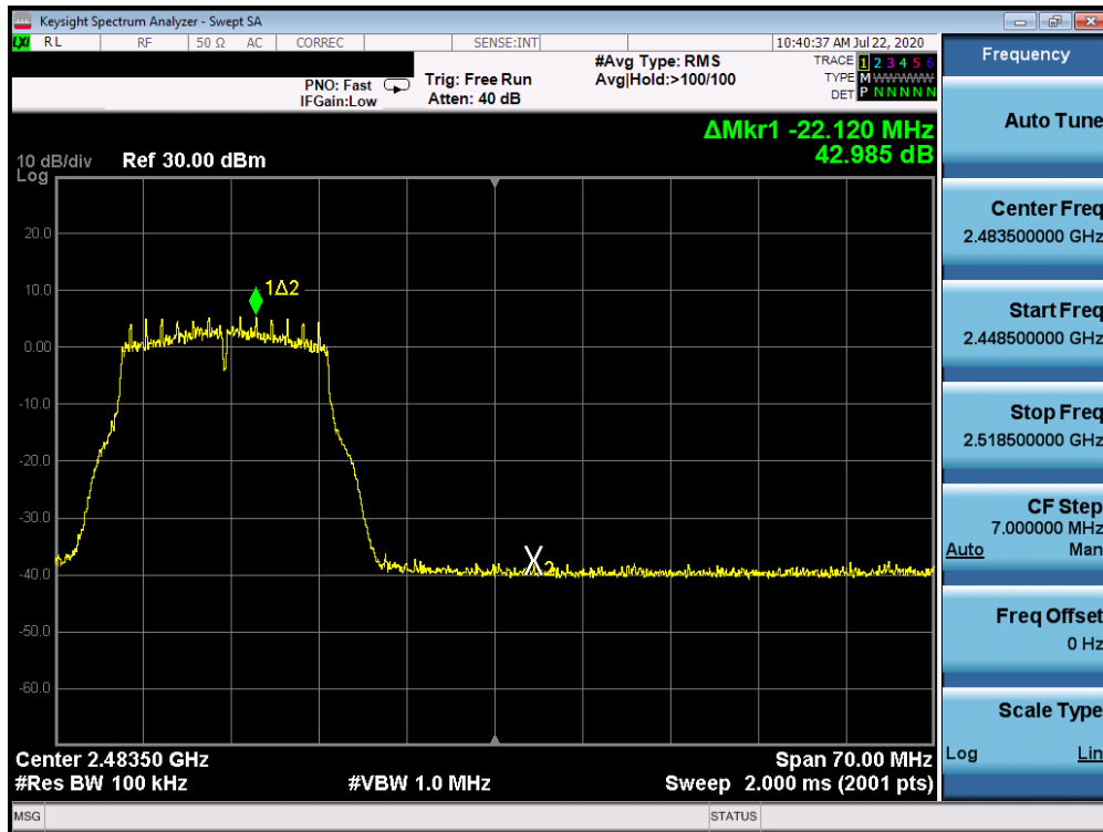
Plot 7-65. Band Edge Plot ANT WF8 (802.11g – Ch. 11)
