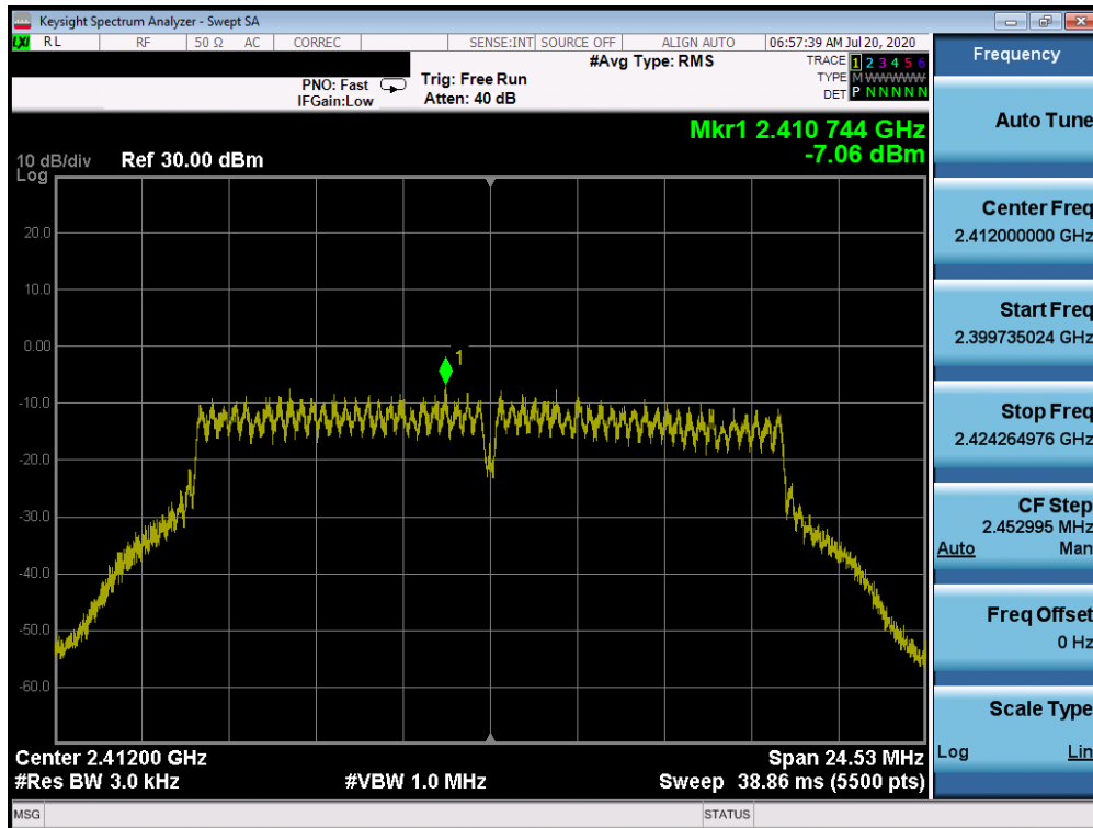
Plot 7-38. Power Spectral Density Plot CDD ANT WF7b (802.11g – Ch. 1)
