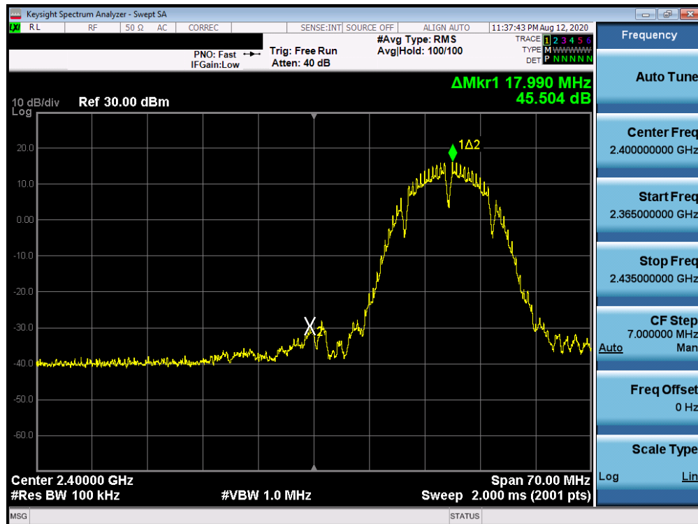
Plot 7-81. Band Edge Plot ANT WF7b (802.11b – Ch. 2)
