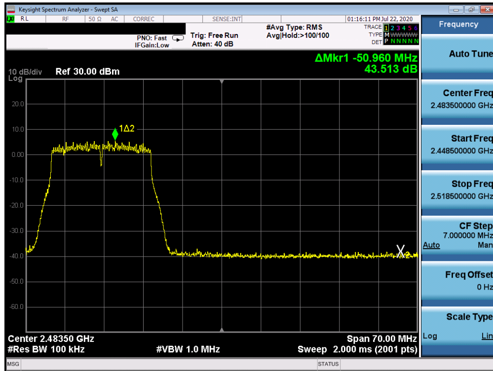
Plot 7-77. Band Edge Plot ANT WF8 (802.11n (2.4GHz) – Ch. 11)
