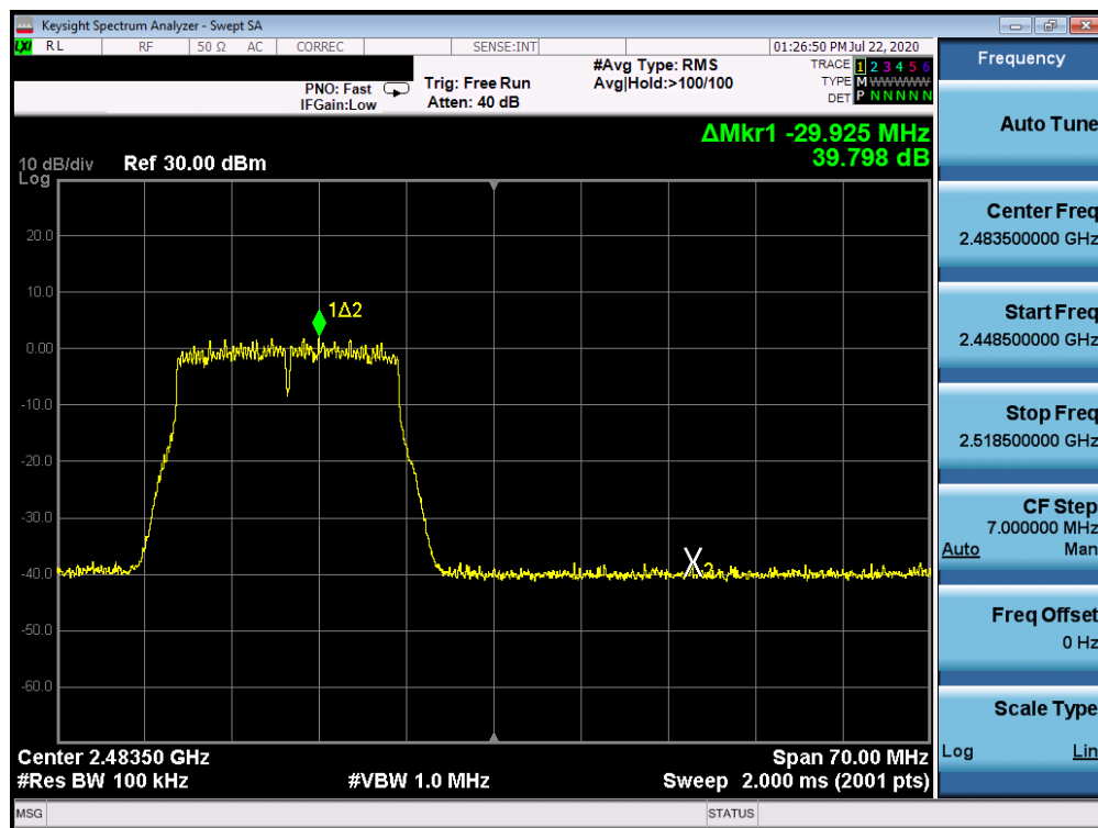
Plot 7-78. Band Edge Plot ANT WF8 (802.11n (2.4GHz) – Ch. 12)
