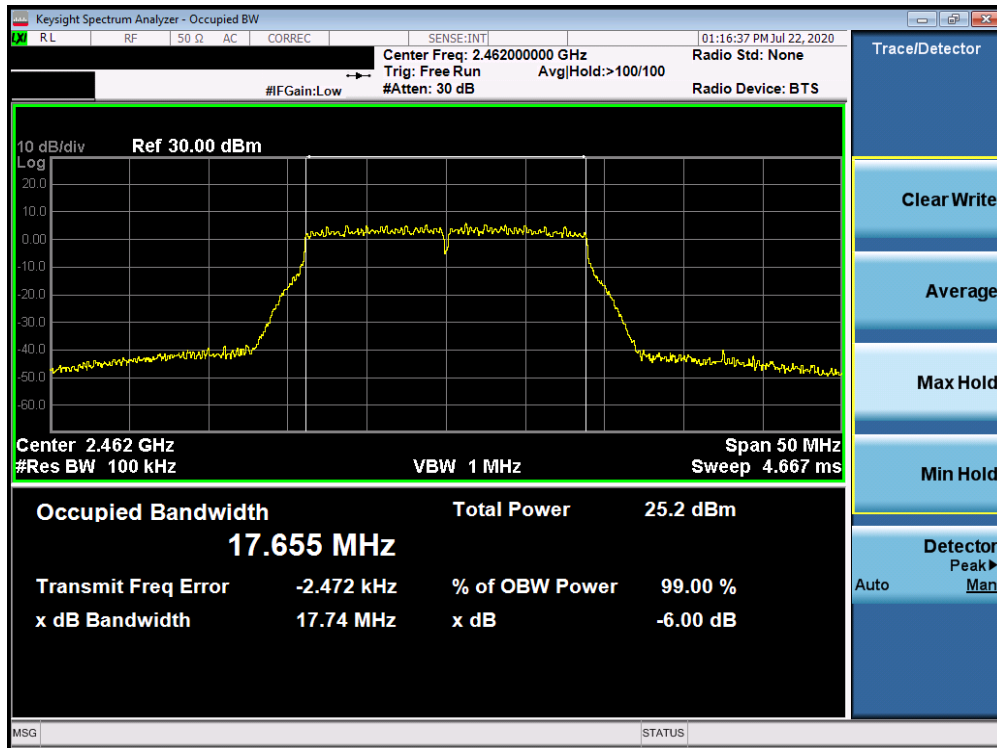
Plot 7-9. 6dB Bandwidth Plot ANT WF8 (802.11n (2.4GHz) – Ch. 11)
