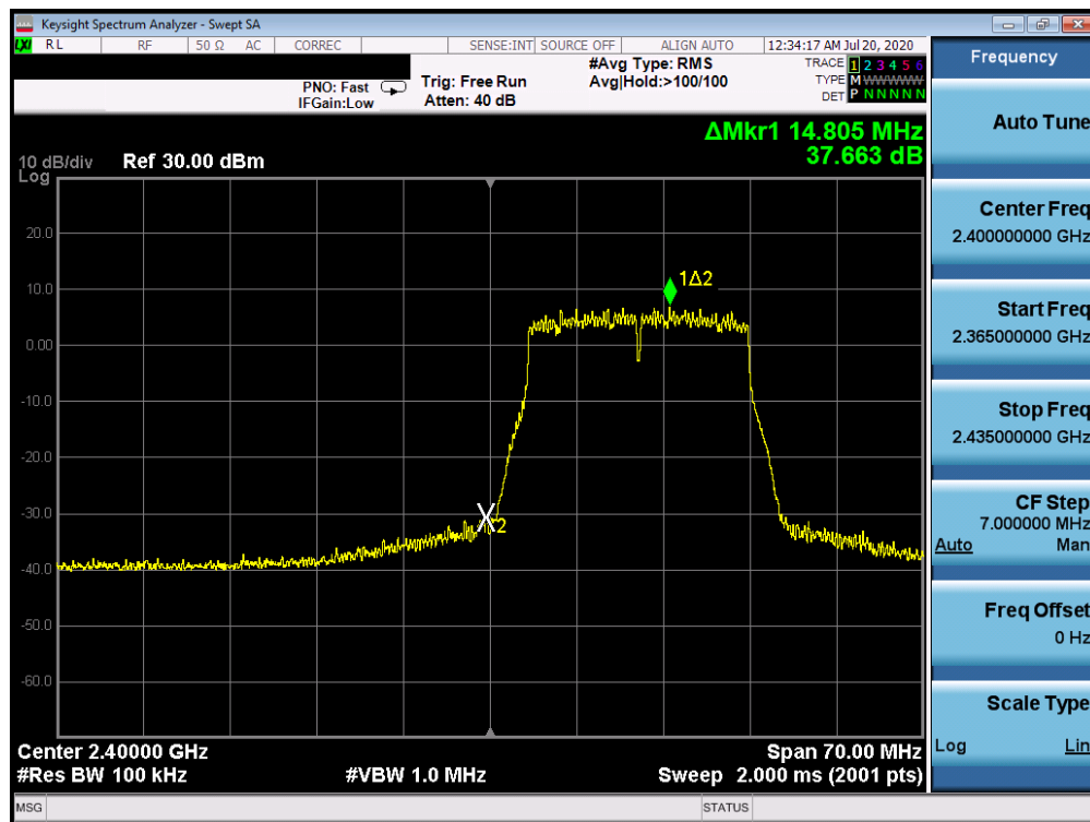
Plot 7-68. Band Edge Plot ANT WF8 (802.11n (2.4GHz) – Ch. 1)
