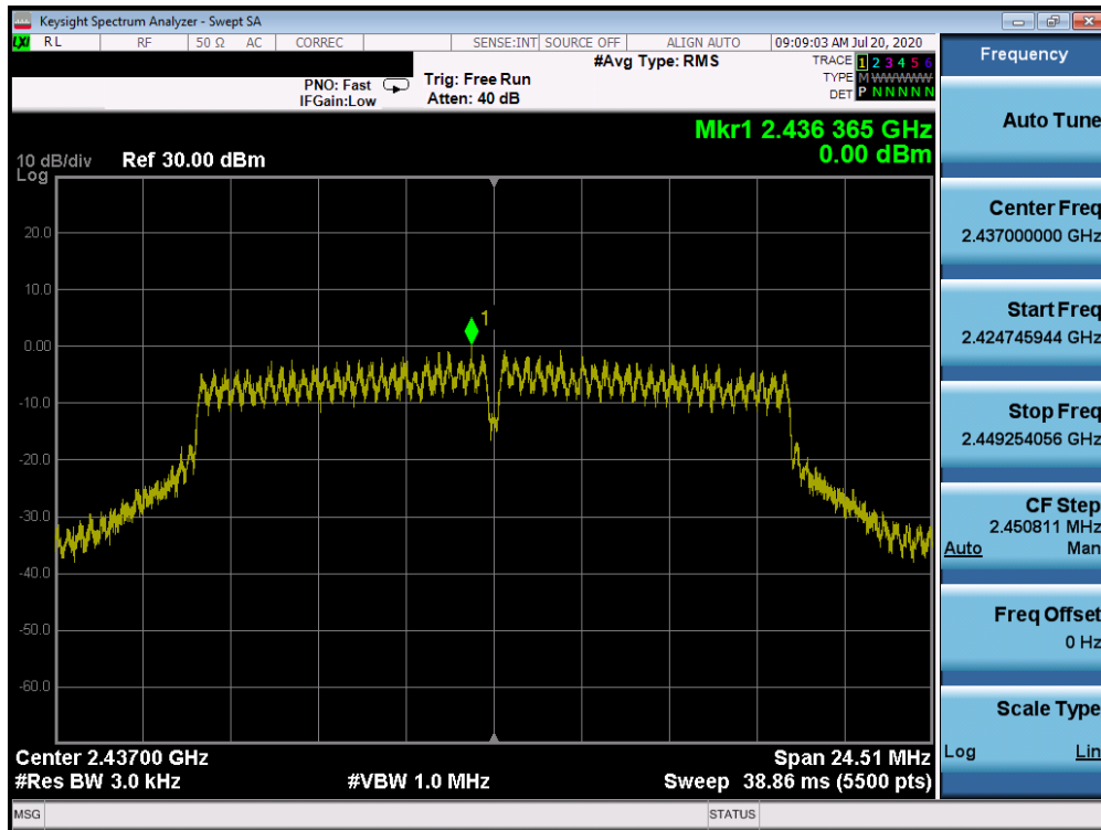
Plot 7-23. Power Spectral Density Plot ANT WF8 (802.11g – Ch. 6)
