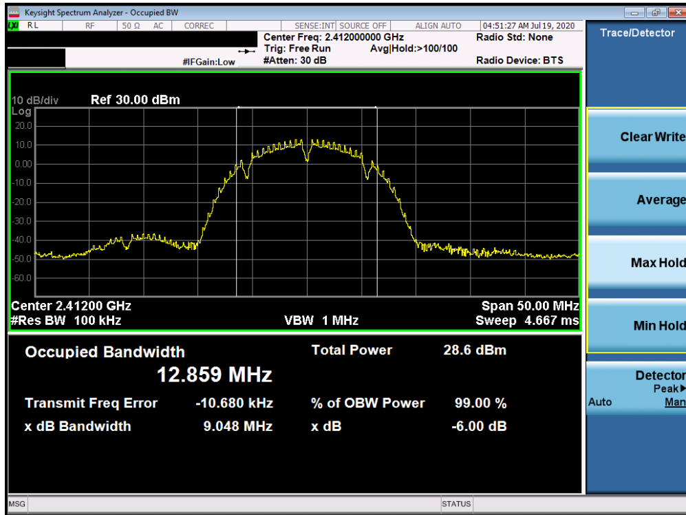
Plot 7-1. 6dB Bandwidth Plot ANT WF8 (802.11b – Ch. 1)
