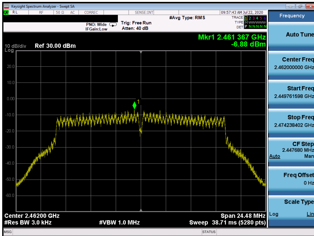
Plot 7-33. Power Spectral Density Plot ANT WF7b (802.11g – Ch. 11)
