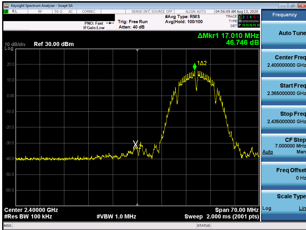
Plot 7-50. Band Edge Plot ANT WF8 (802.11b – Ch. 2)
