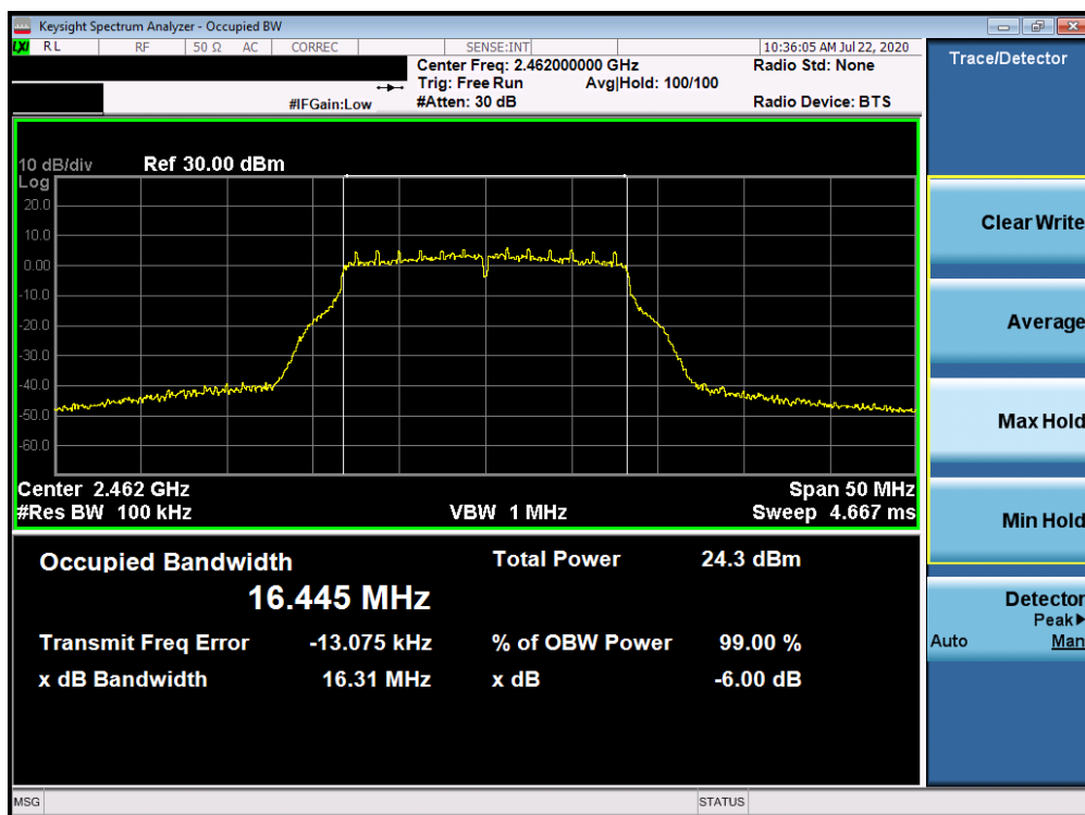
Plot 7-6. 6dB Bandwidth Plot ANT WF8 (802.11g – Ch. 11)
