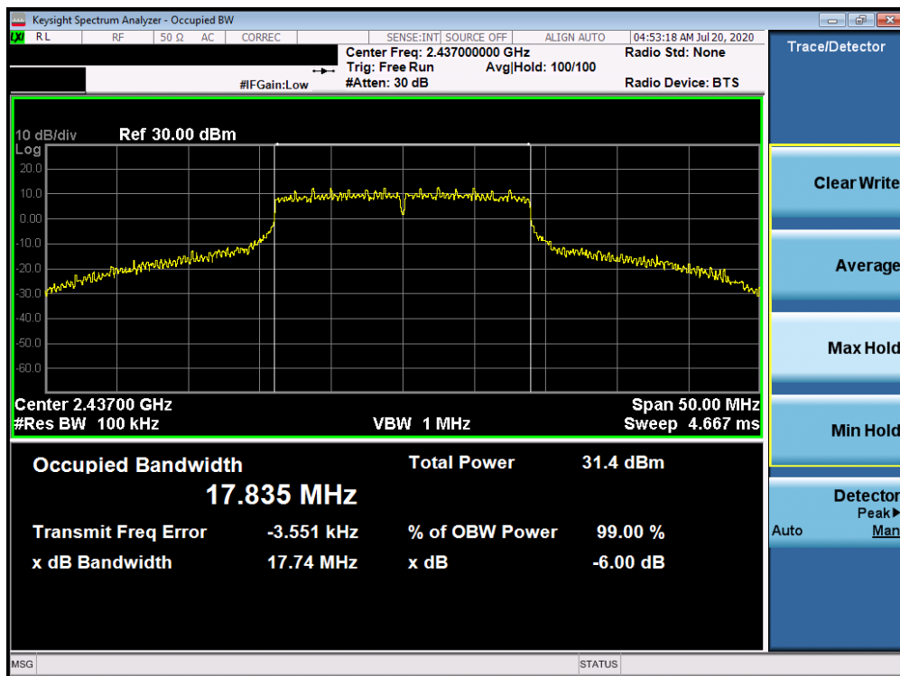
Plot 7-8. 6dB Bandwidth Plot ANT WF8 (802.11n (2.4GHz) – Ch. 6)
