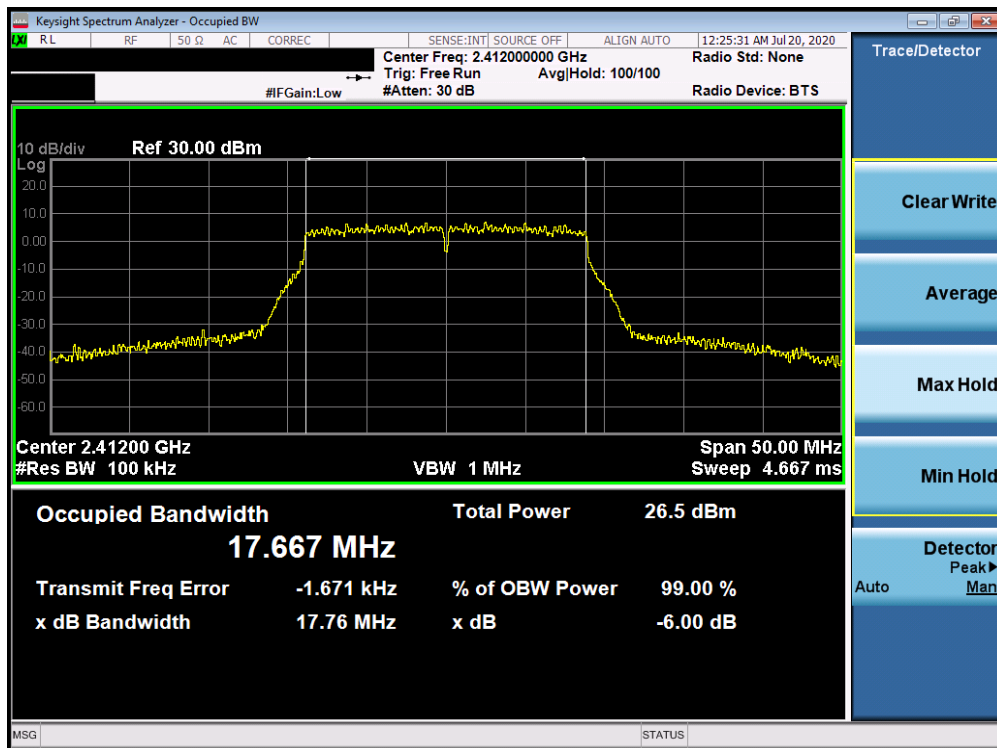
Plot 7-7. 6dB Bandwidth Plot ANT WF8 (802.11n (2.4GHz) – Ch. 1)
