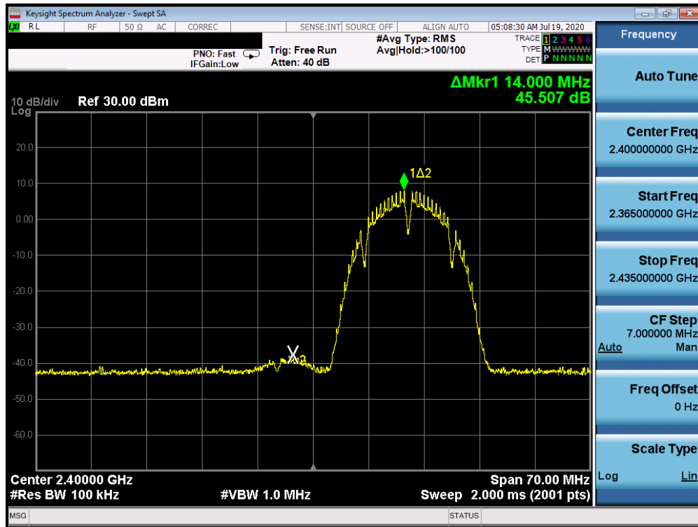
Plot 7-49. Band Edge Plot ANT WF8 (802.11b – Ch. 1)
