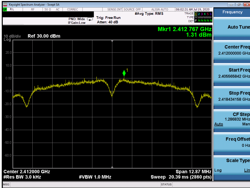
Plot 7-28. Power Spectral Density Plot ANT WF7b (802.11b – Ch. 1)
