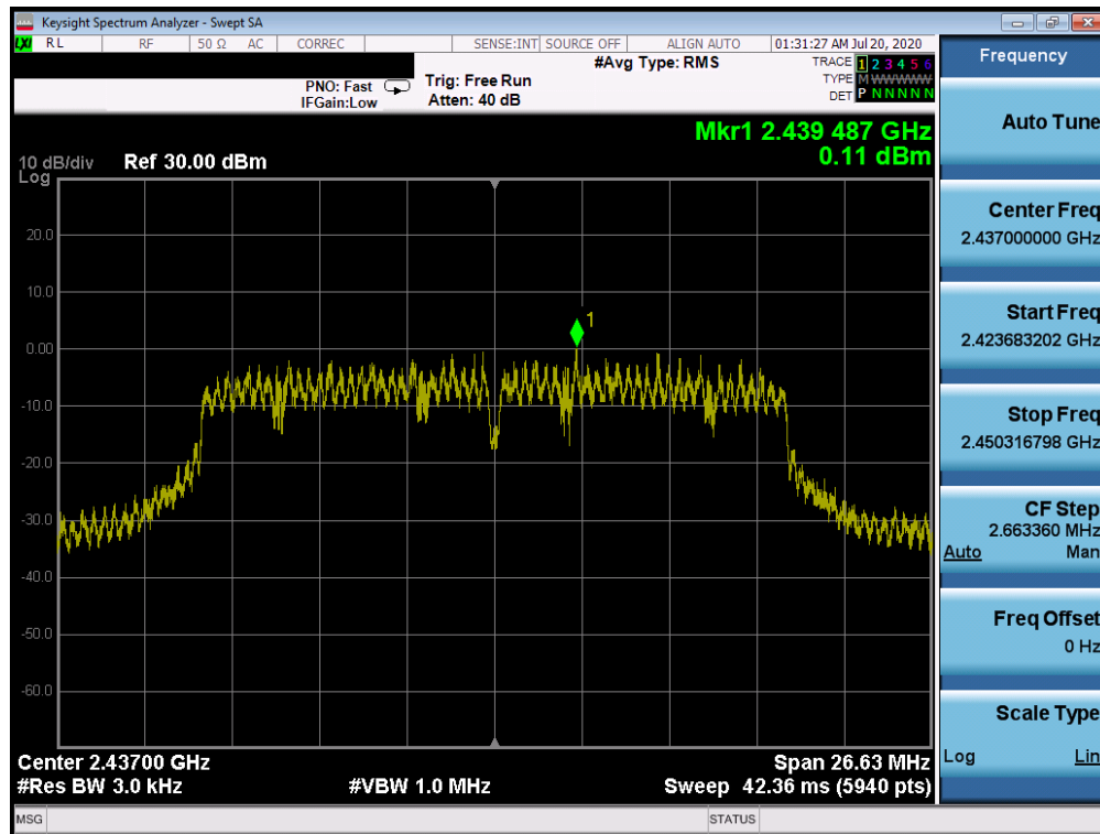
Plot 7-45. Power Spectral Density Plot CDD ANT WF8 (802.11n (2.4GHz) – Ch. 6)
