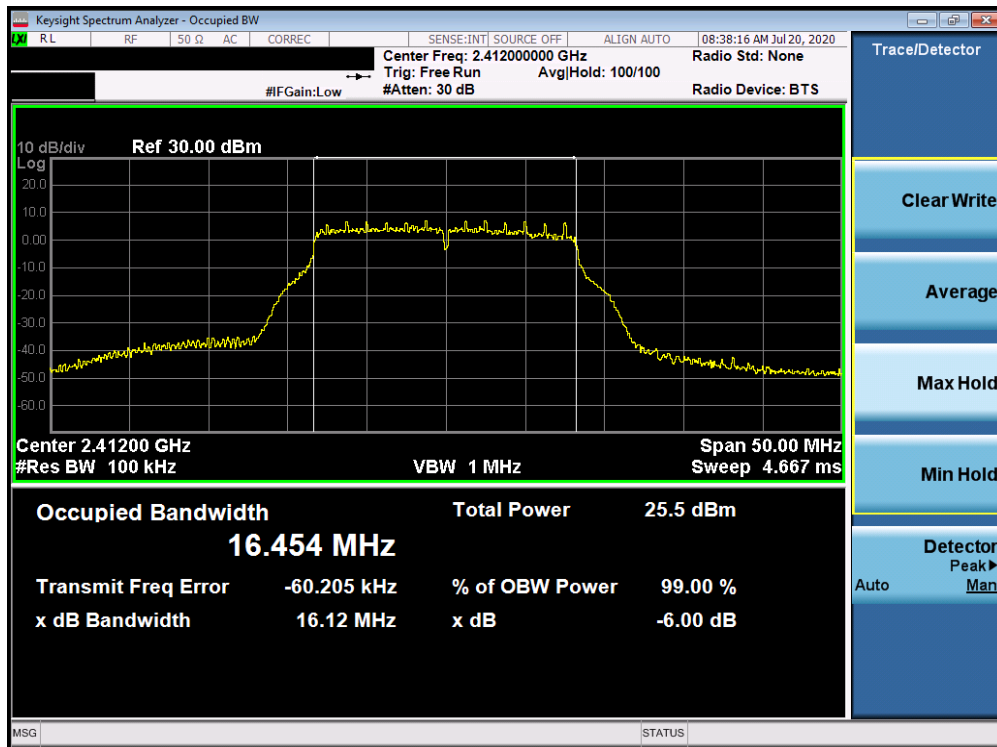
Plot 7-4. 6dB Bandwidth Plot ANT WF8 (802.11g – Ch. 1)
