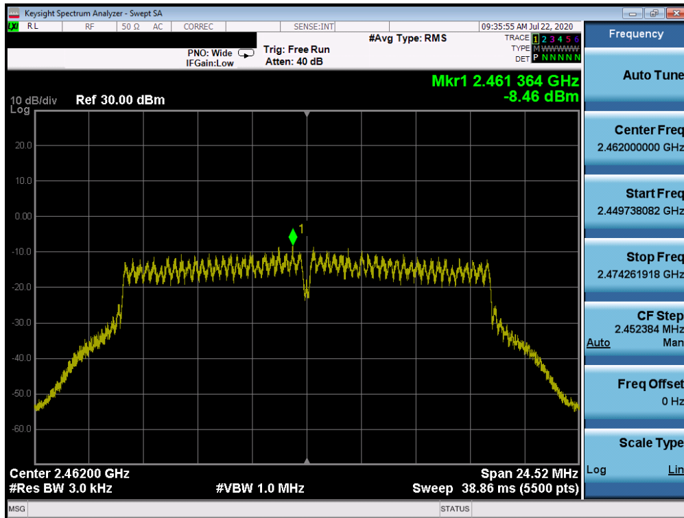
Plot 7-42. Power Spectral Density Plot CDD ANT WF7b (802.11g – Ch. 11)
