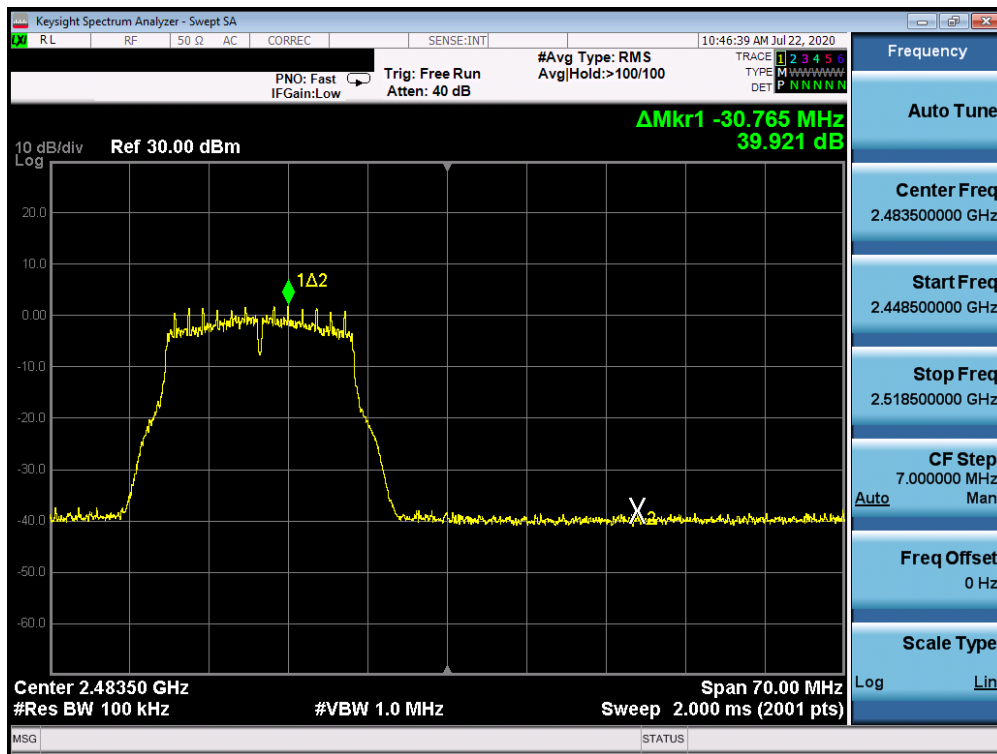
Plot 7-66. Band Edge Plot ANT WF8 (802.11g – Ch. 12)
