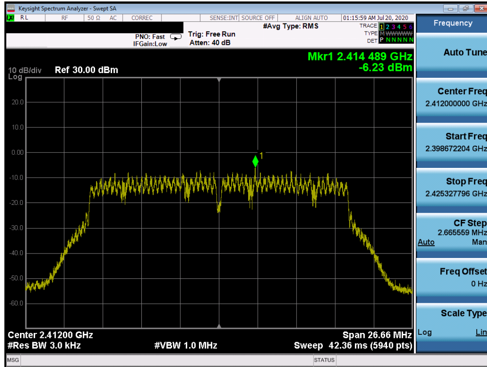
Plot 7-43. Power Spectral Density Plot CDD ANT WF8 (802.11n (2.4GHz) – Ch. 1)
