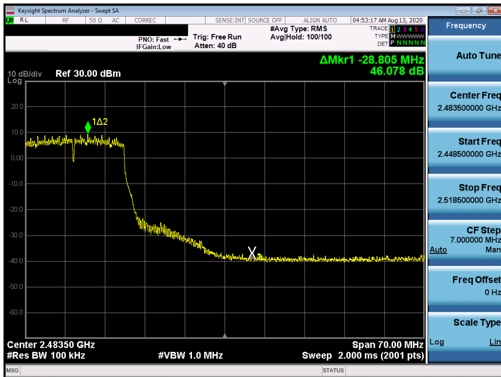
Plot 7-76. Band Edge Plot ANT WF8 (802.11n (2.4GHz) – Ch. 10)
