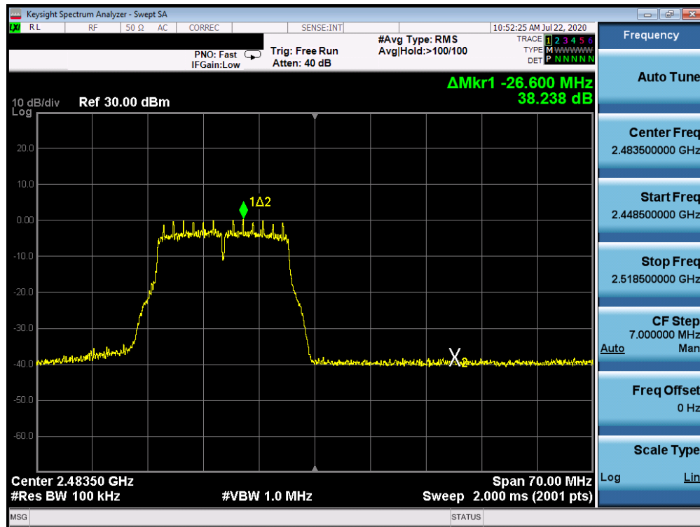
Plot 7-67. Band Edge Plot ANT WF8 (802.11g – Ch. 13)
