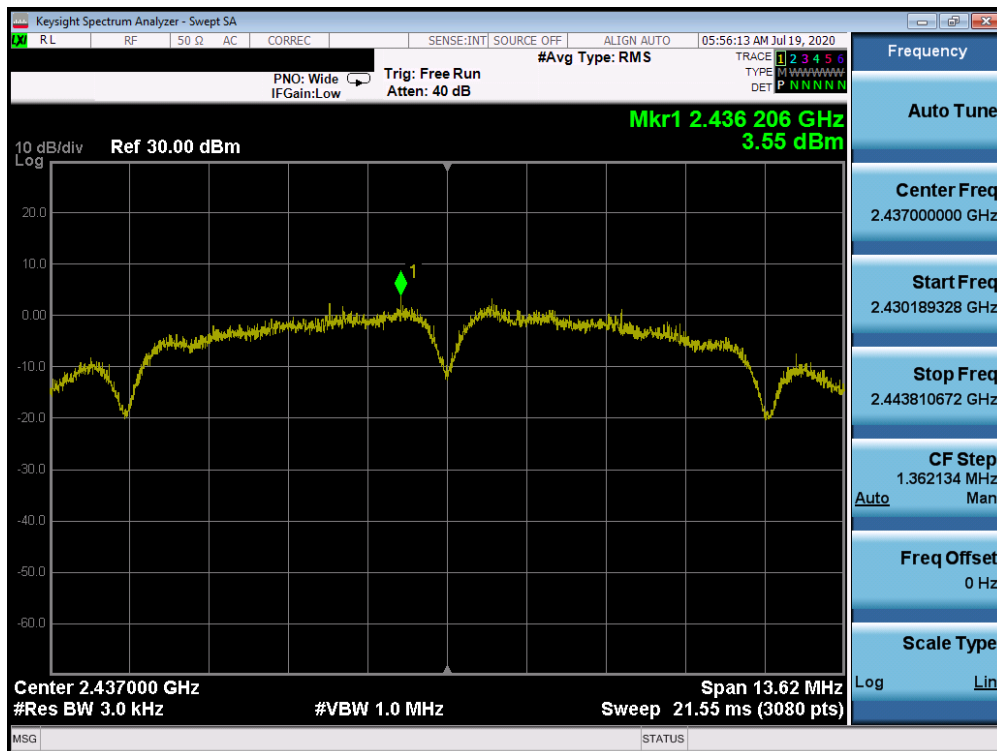
Plot 7-29. Power Spectral Density Plot ANT WF7b (802.11b – Ch. 6)
