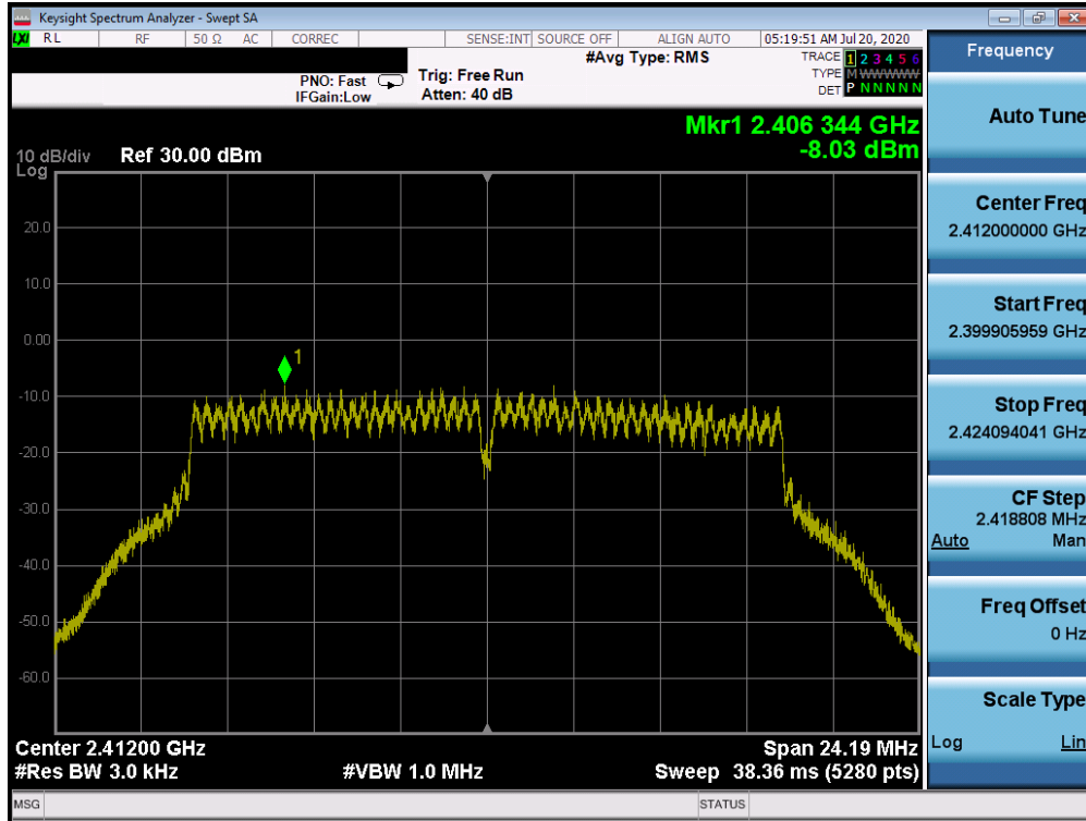
Plot 7-37. Power Spectral Density Plot CDD ANT WF8 (802.11g – Ch. 1)
