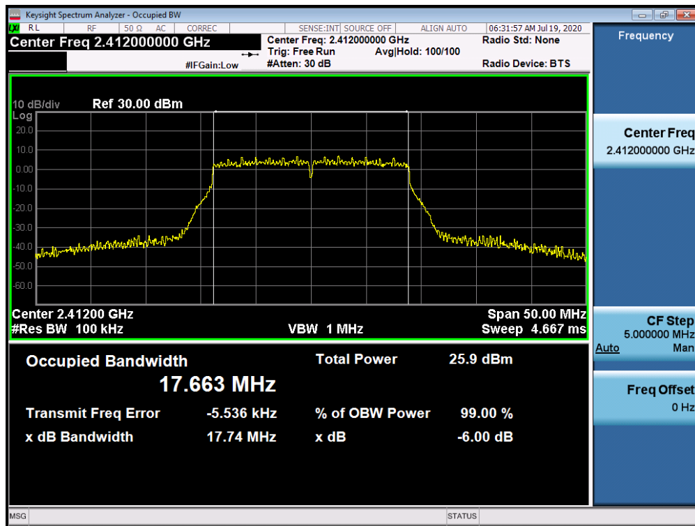
Plot 7-16. 6dB Bandwidth Plot ANT WF7b (802.11n (2.4GHz) – Ch. 1)
