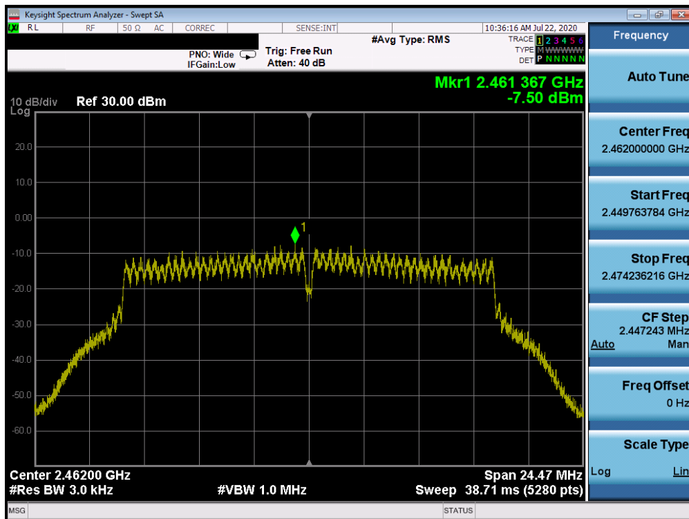
Plot 7-24. Power Spectral Density Plot ANT WF8 (802.11g – Ch. 11)
