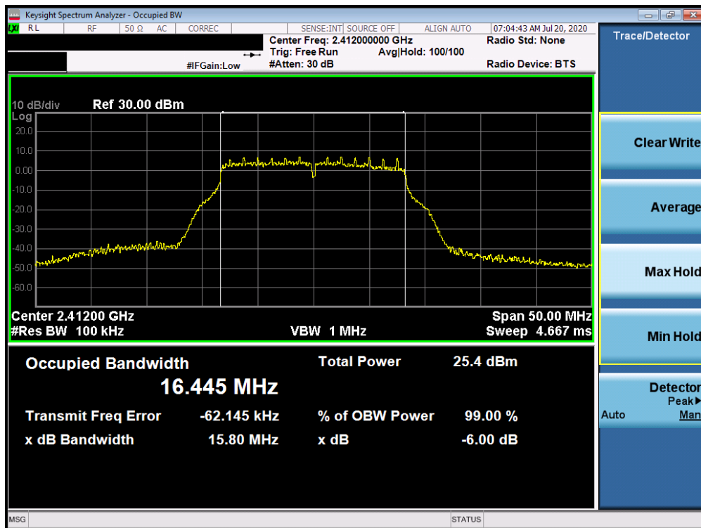
Plot 7-13. 6dB Bandwidth Plot ANT WF7b (802.11g – Ch. 1)
