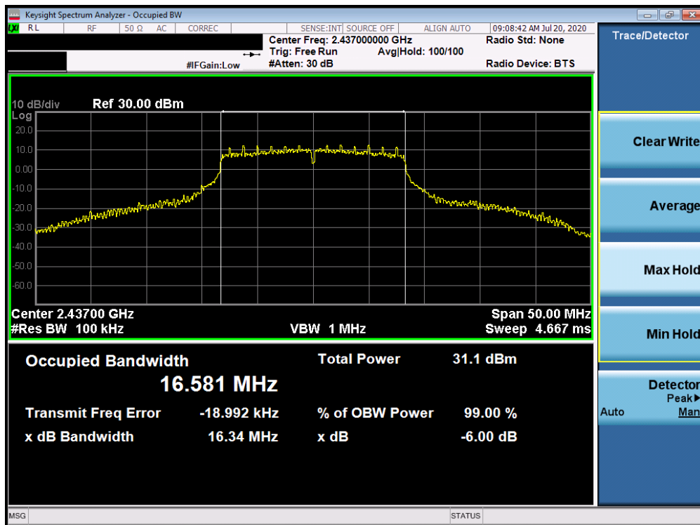
Plot 7-5. 6dB Bandwidth Plot ANT WF8 (802.11g – Ch. 6)
