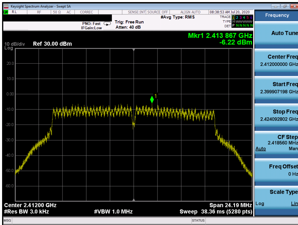
Plot 7-22. Power Spectral Density Plot ANT WF8 (802.11g – Ch. 1)
