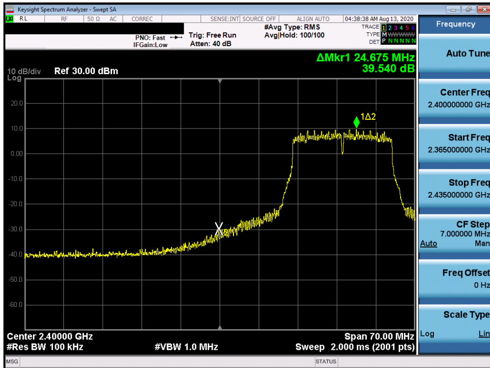
Plot 7-70. Band Edge Plot ANT WF8 (802.11n (2.4GHz) – Ch. 3)
