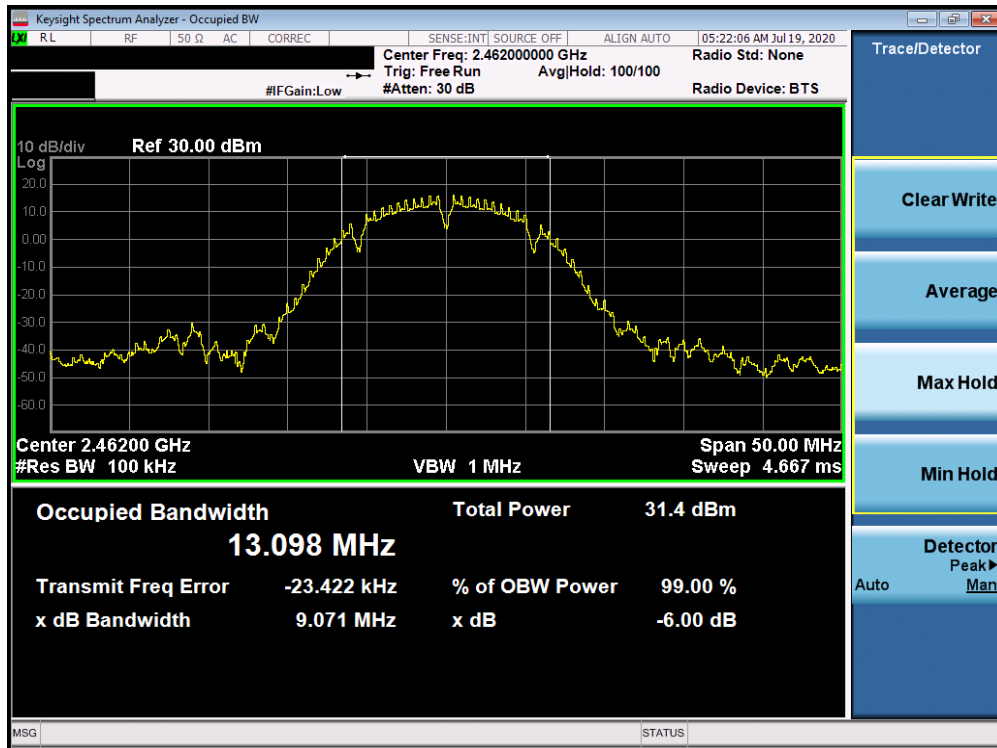
Plot 7-3. 6dB Bandwidth Plot ANT WF8 (802.11b – Ch. 11)
