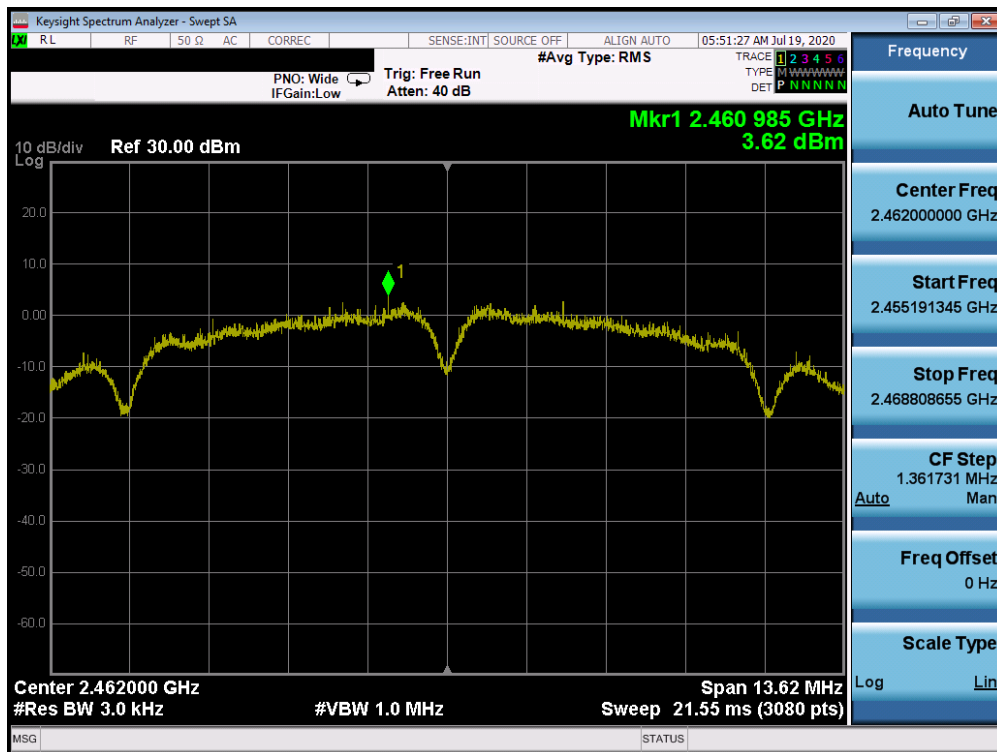
Plot 7-30. Power Spectral Density Plot ANT WF7b (802.11b – Ch. 11)
