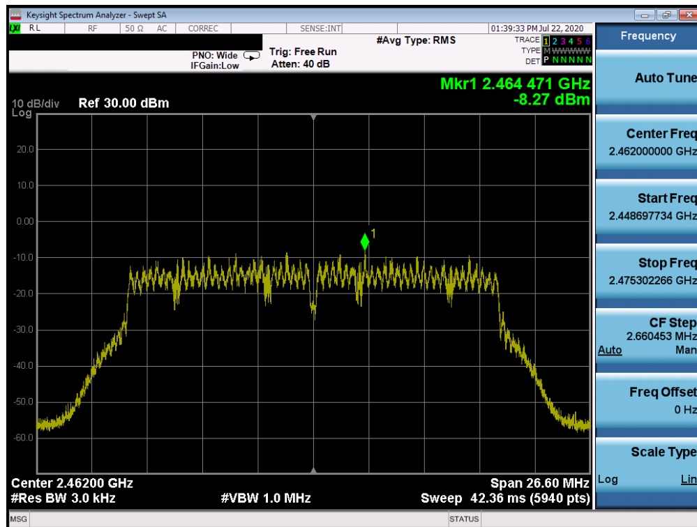
Plot 7-48. Power Spectral Density Plot CDD ANT WF7b (802.11n (2.4GHz) – Ch. 11)
