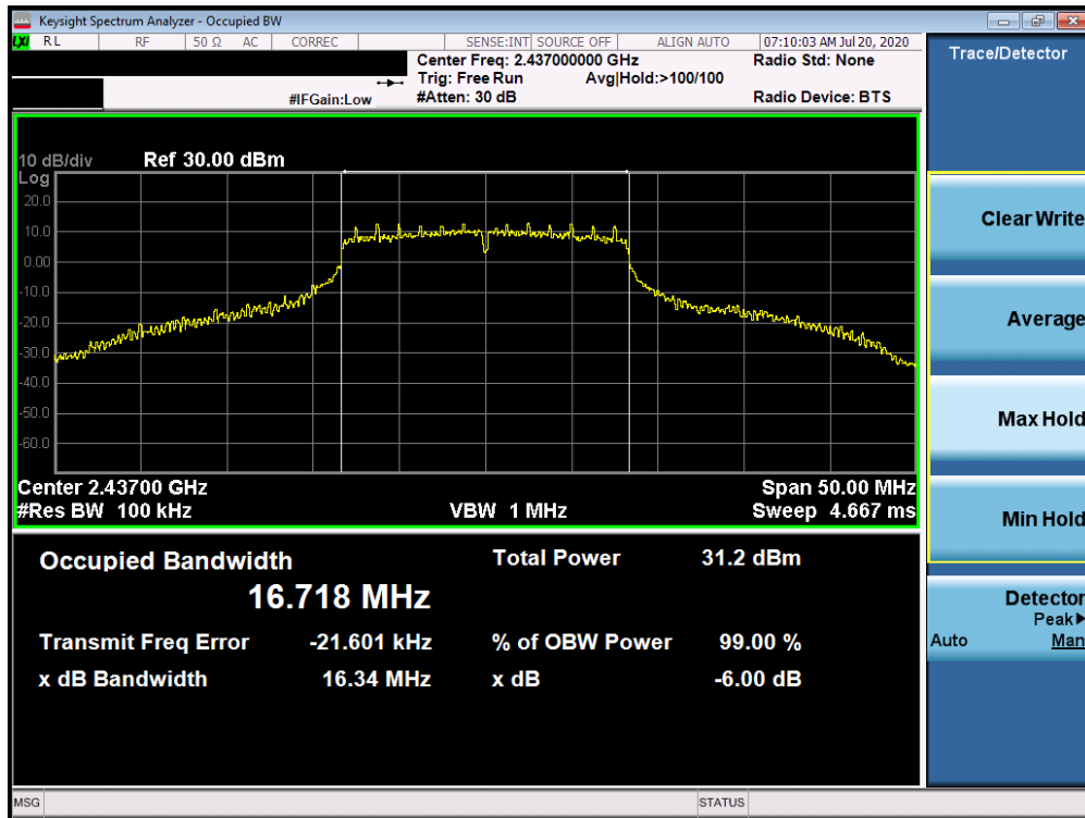
Plot 7-14. 6dB Bandwidth Plot ANT WF7b (802.11g – Ch. 6)
