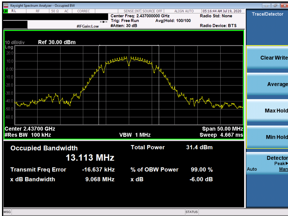
Plot 7-2. 6dB Bandwidth Plot ANT WF8 (802.11b – Ch. 6)
