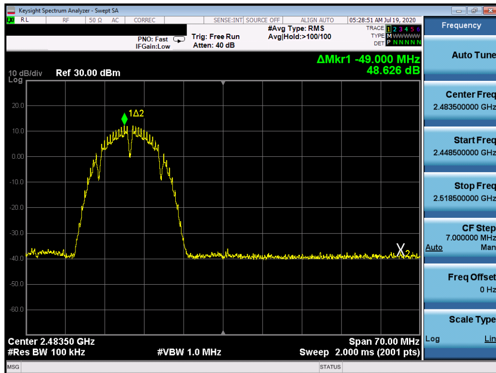
Plot 7-54. Band Edge Plot ANT WF8 (802.11b – Ch. 12)
