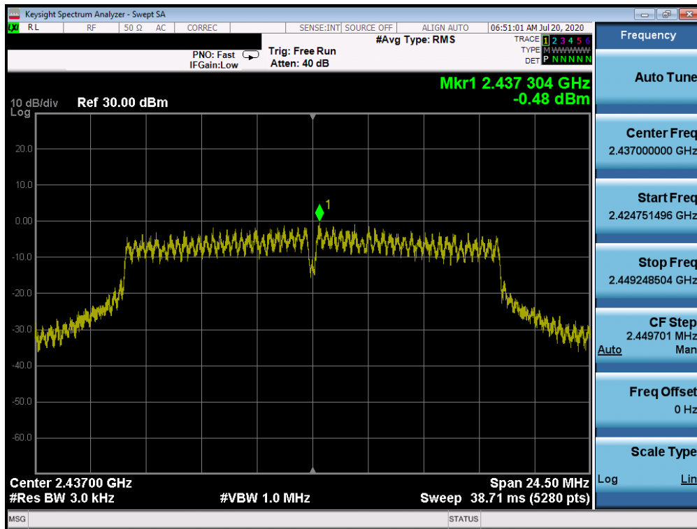
Plot 7-40. Power Spectral Density Plot CDD ANT WF7b (802.11g – Ch. 6)
