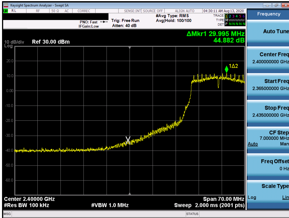
Plot 7-59. Band Edge Plot ANT WF8 (802.11g– Ch. 4)
