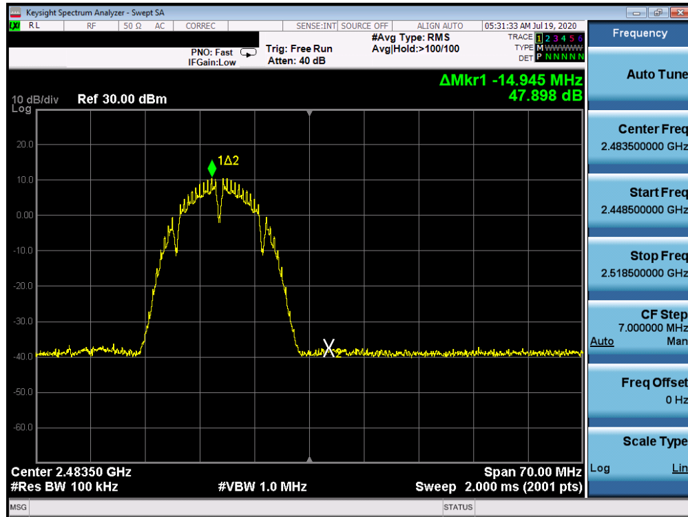
Plot 7-55. Band Edge Plot ANT WF8 (802.11b – Ch. 13)
