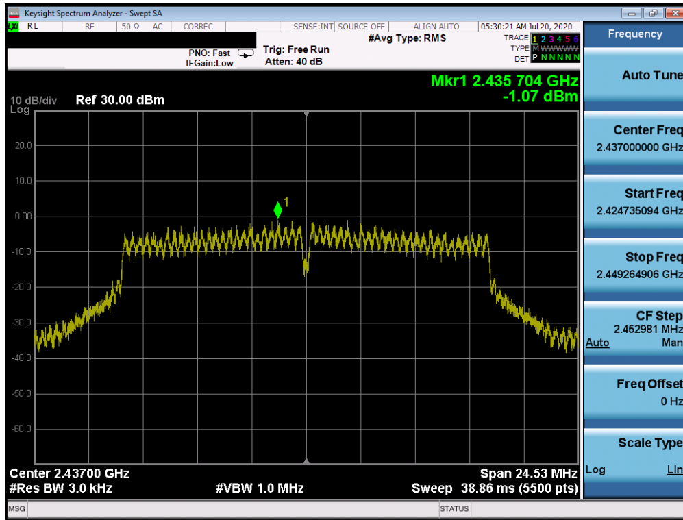
Plot 7-39. Power Spectral Density Plot CDD ANT WF8 (802.11g – Ch. 6)
