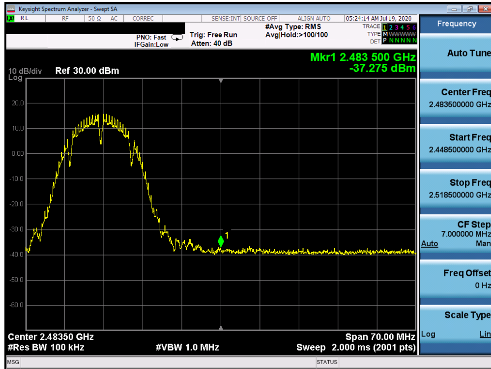
Plot 7-53. Band Edge Plot ANT WF8 (802.11b – Ch. 11)
