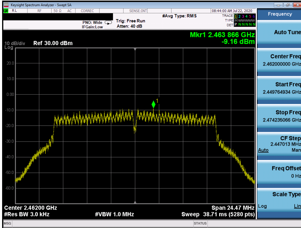
Plot 7-41. Power Spectral Density Plot CDD ANT WF8 (802.11g – Ch. 11)
