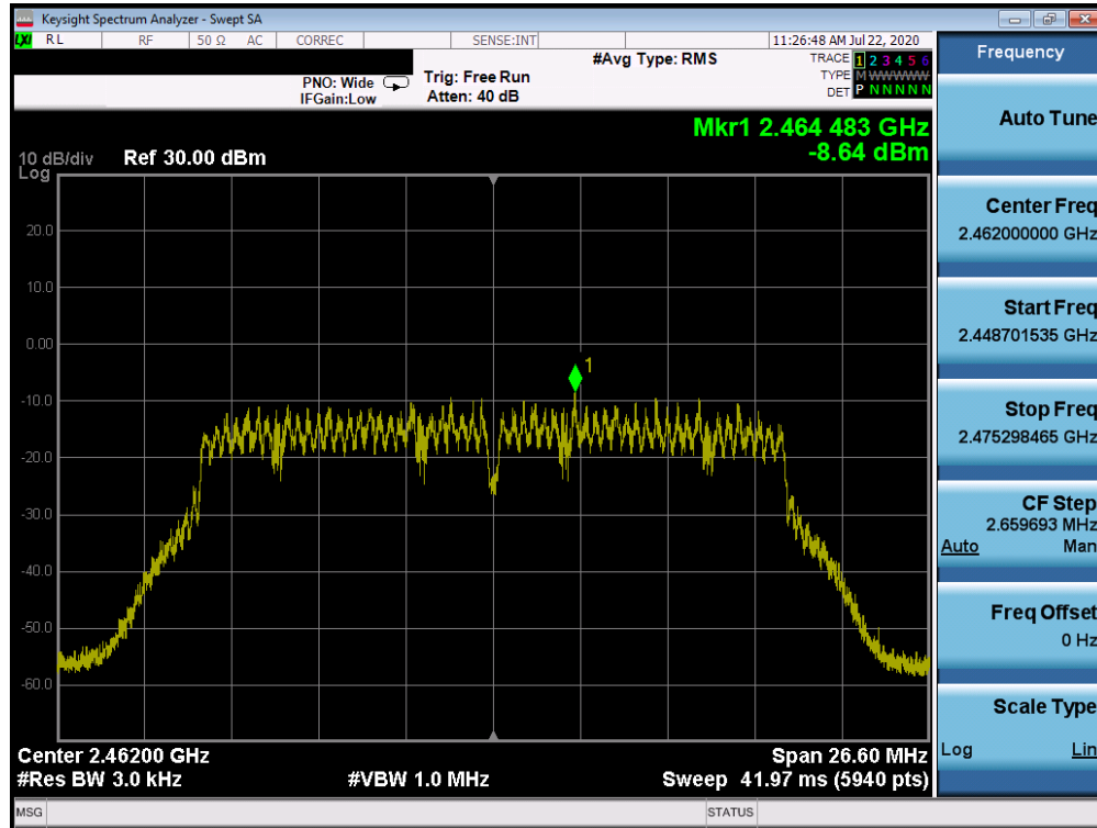
Plot 7-47. Power Spectral Density Plot CDD ANT WF8 (802.11n (2.4GHz) – Ch. 11)
