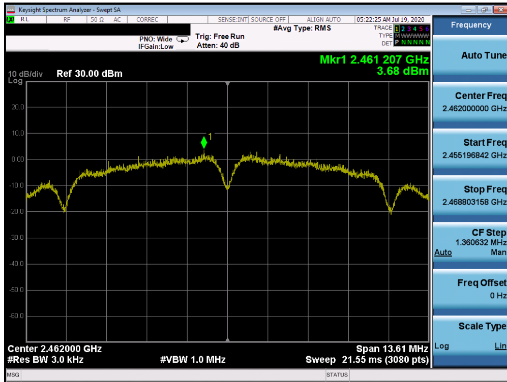
Plot 7-21. Power Spectral Density Plot ANT WF8 (802.11b – Ch. 11)
