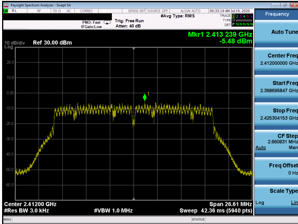
Plot 7-34. Power Spectral Density Plot ANT WF7b (802.11n (2.4GHz) – Ch. 1)
