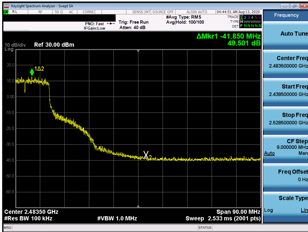
Plot 7-73. Band Edge Plot ANT WF8 (802.11n (2.4GHz) – Ch. 7)
