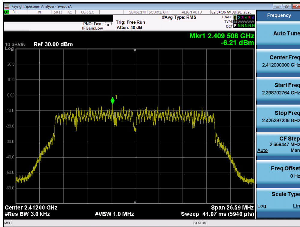
Plot 7-44. Power Spectral Density Plot CDD ANT WF7b (802.11n (2.4GHz) – Ch. 1)
