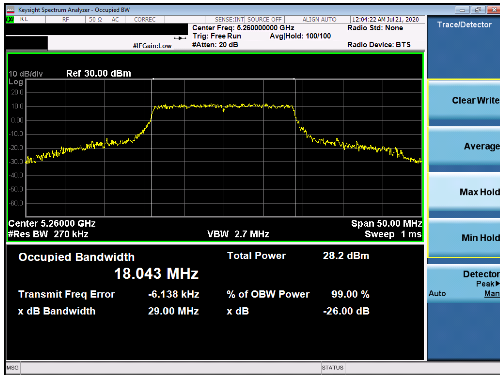
Plot 7-7. 26dB Bandwidth Plot ANT WF8 (20MHz BW 802.11n (UNII Band 2A) – Ch. 52)
