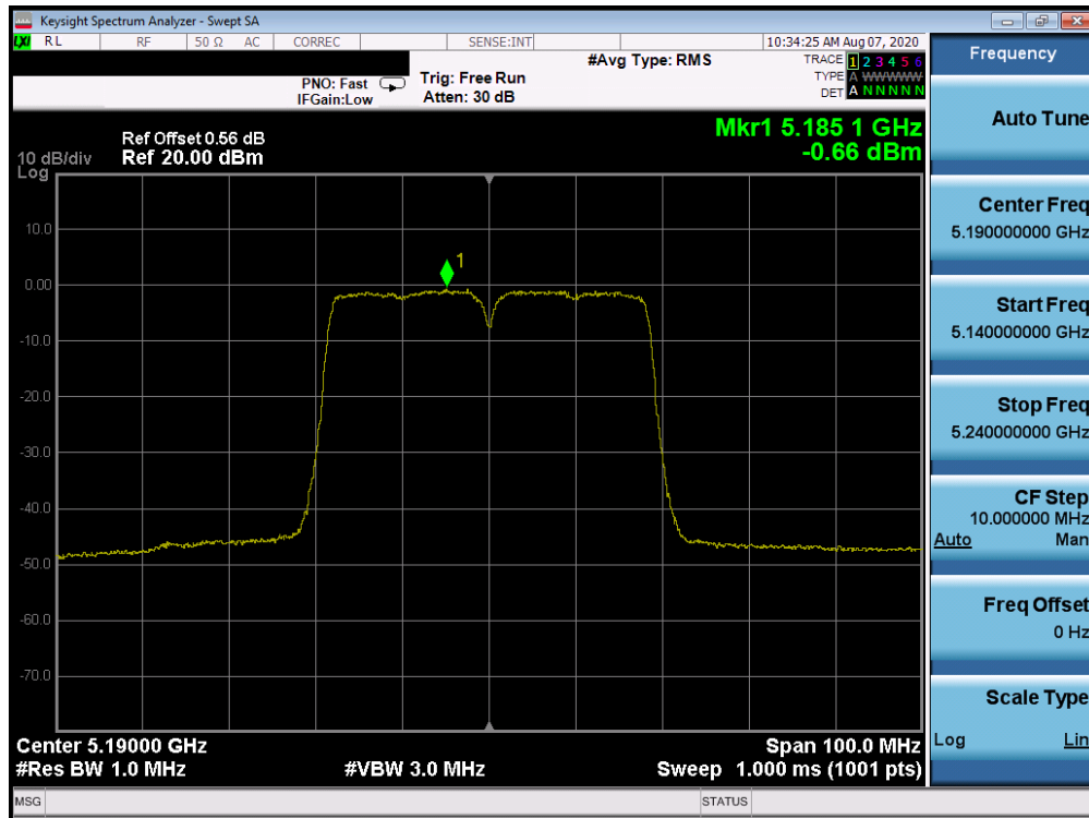
Plot 7-88. Power Spectral Density Plot ANT WF7a (40MHz BW 802.11n (UNII Band 1) – Ch. 38)
