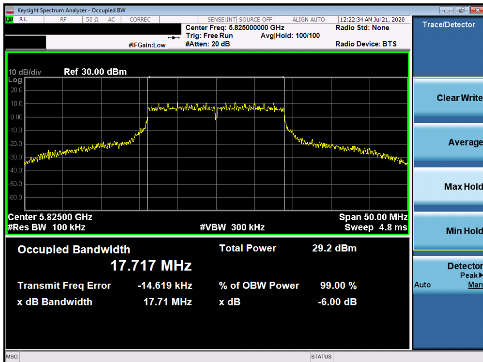
Plot 7-43. 6dB Bandwidth Plot ANT WF8 (20MHz BW 802.11n (UNII Band 3) – Ch. 165)
