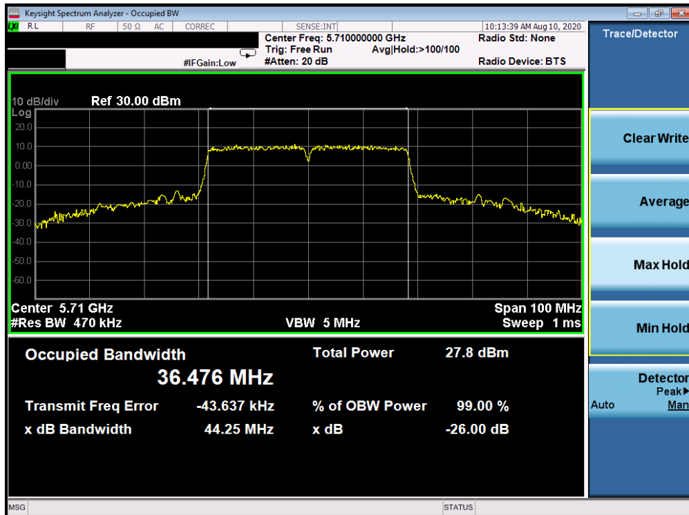
Plot 7-38. 26dB Bandwidth Plot ANT WF7a (40MHz BW 802.11n (UNII Band 2C) – Ch. 142)
