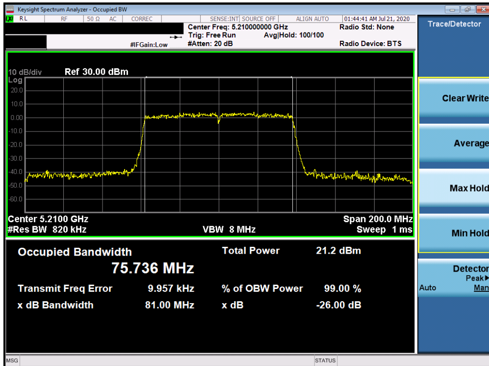
Plot 7-6. 26dB Bandwidth Plot ANT WF8 (80MHz BW 802.11ac (UNII Band 1) – Ch. 42)
