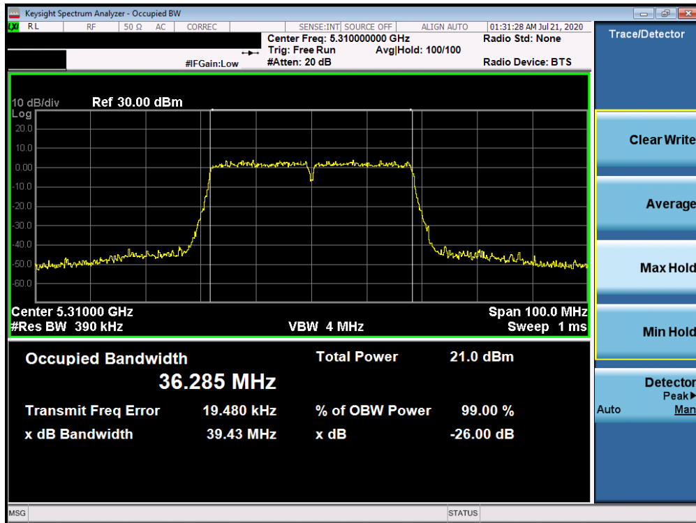
Plot 7-11. 26dB Bandwidth Plot ANT WF8 (40MHz BW 802.11n (UNII Band 2A) – Ch. 62)
