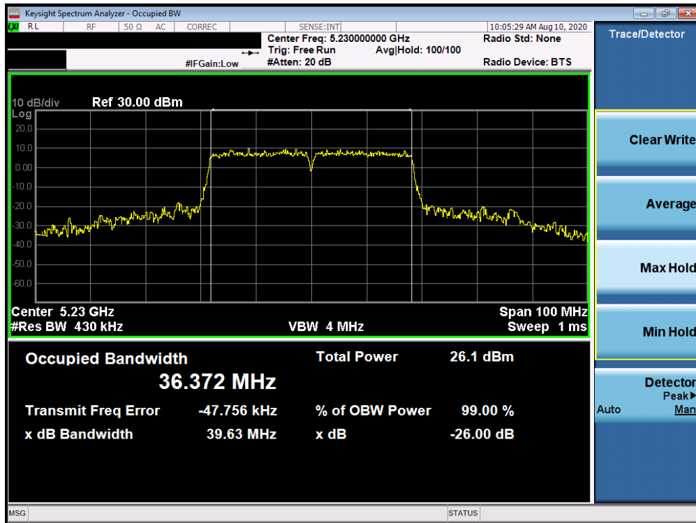
Plot 7-25. 26dB Bandwidth Plot ANT WF7a (40MHz BW 802.11n (UNII Band 1) – Ch. 46)
