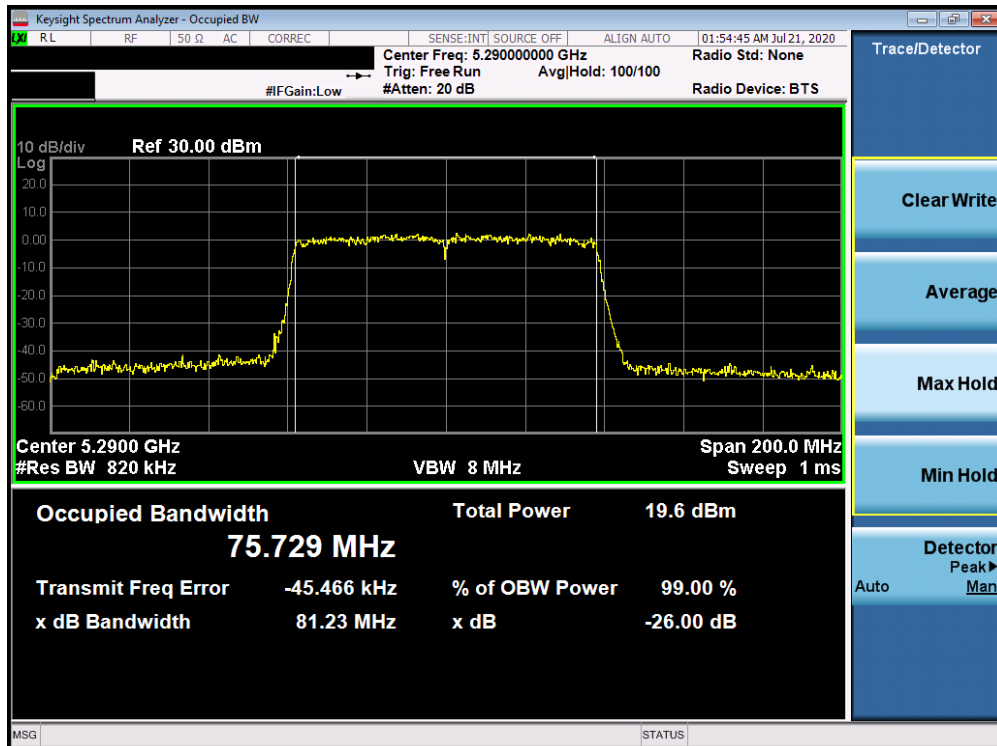
Plot 7-32. 26dB Bandwidth Plot ANT WF7a (80MHz BW 802.11ac (UNII Band 2A) – Ch. 58)
