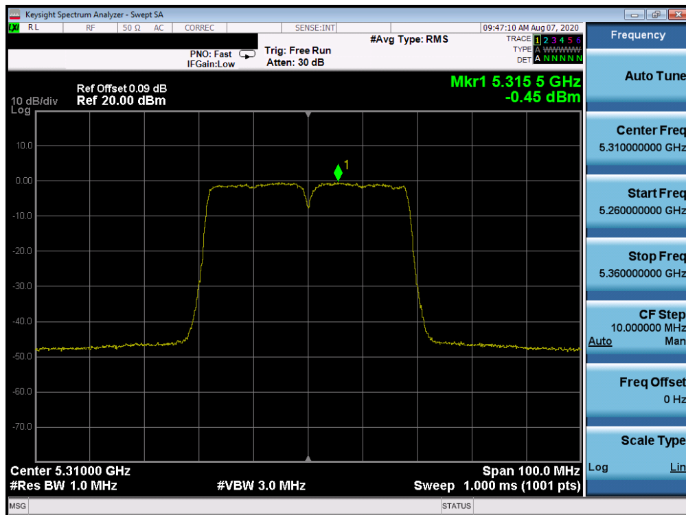
Plot 7-66. Power Spectral Density Plot ANT WF8 (40MHz BW 802.11n (UNII Band 2A) – Ch. 62)
