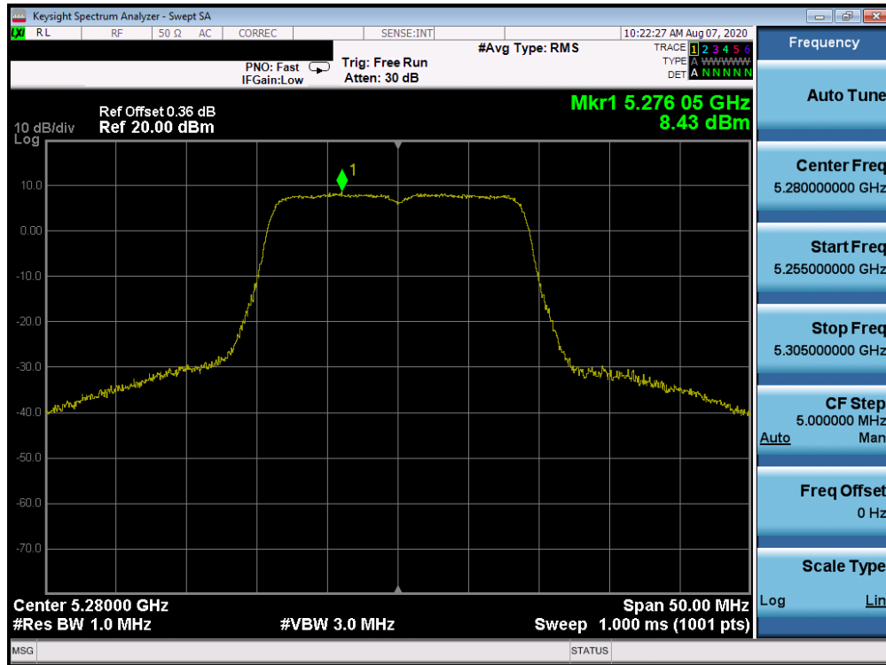
Plot 7-92. Power Spectral Density Plot ANT WF7a (20MHz BW 802.11n (UNII Band 2A) – Ch. 56)
