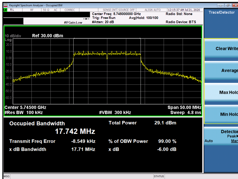
Plot 7-41. 6dB Bandwidth Plot ANT WF8 (20MHz BW 802.11n (UNII Band 3) – Ch. 149)
