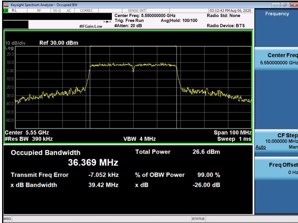
Plot 7-37. 26dB Bandwidth Plot ANT WF7a (40MHz BW 802.11n (UNII Band 2C) – Ch. 110)
