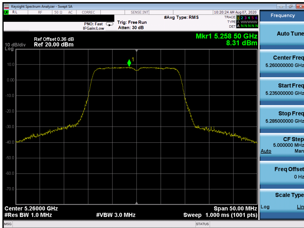
Plot 7-91. Power Spectral Density Plot ANT WF7a (20MHz BW 802.11n (UNII Band 2A) – Ch. 52)
