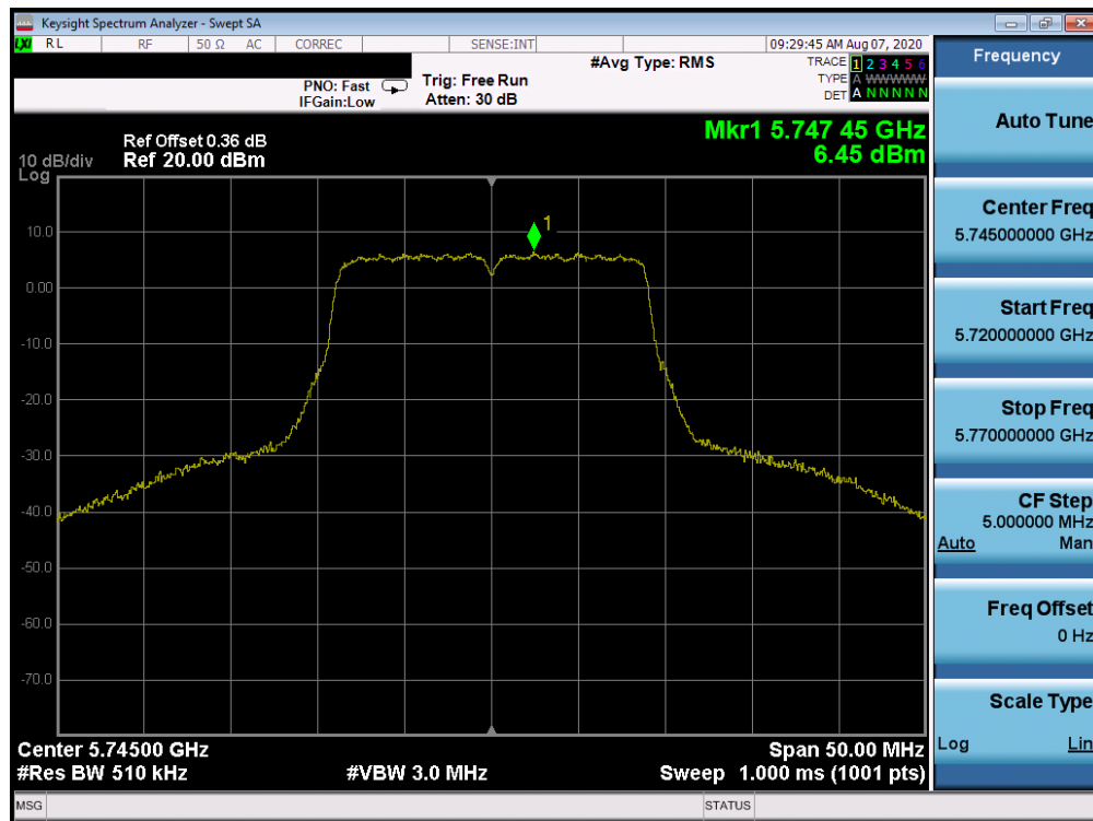
Plot 7-76. Power Spectral Density Plot ANT WF8 (20MHz BW 802.11n (UNII Band 3) – Ch. 149)
