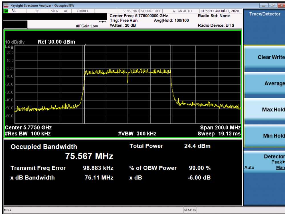
Plot 7-52. 6dB Bandwidth Plot ANT WF7a (80MHz BW 802.11ac (UNII Band 3) – Ch. 155)
