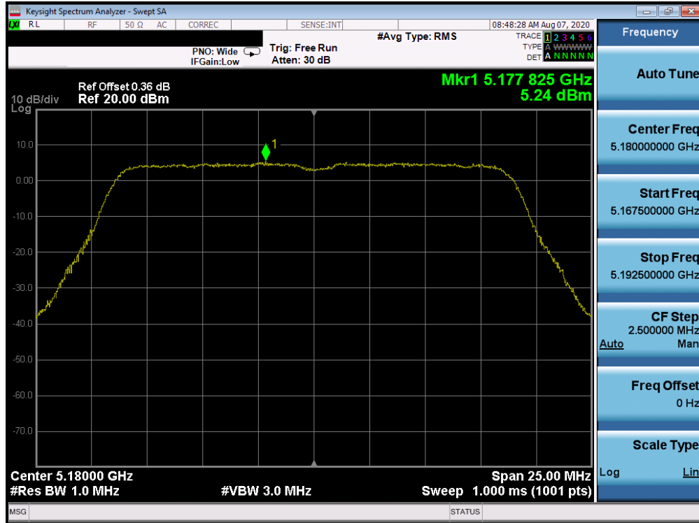
Plot 7-53. Power Spectral Density Plot ANT WF8 (20MHz BW 802.11n (UNII Band 1) – Ch. 36)
