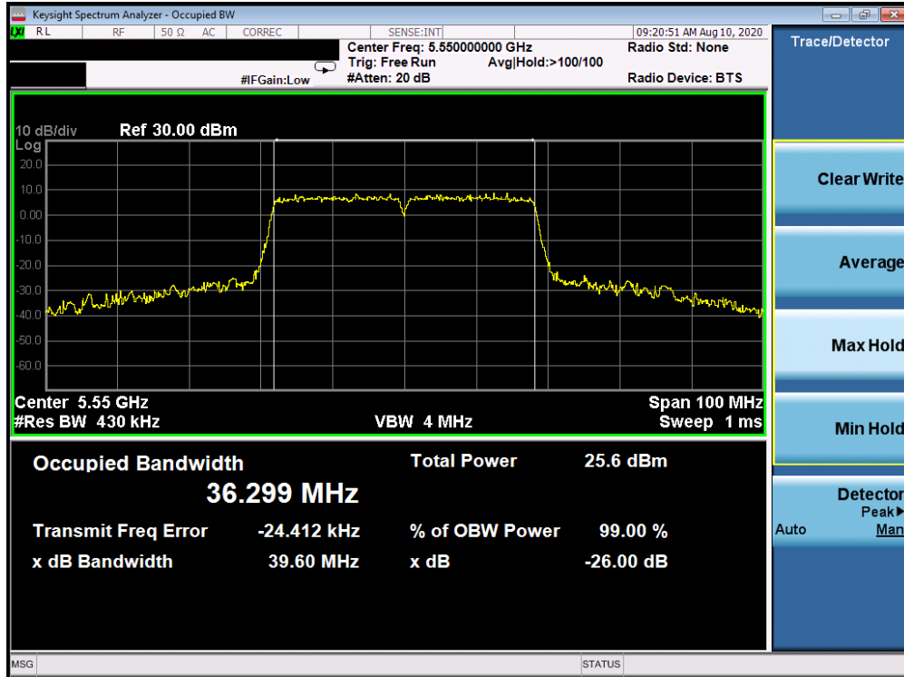
Plot 7-17. 26dB Bandwidth Plot ANT WF8 (40MHz BW 802.11n (UNII Band 2C) – Ch. 110)
