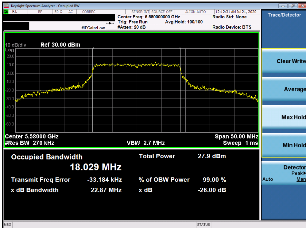
Plot 7-14. 26dB Bandwidth Plot ANT WF8 (20MHz BW 802.11n (UNII Band 2C) – Ch. 116)
