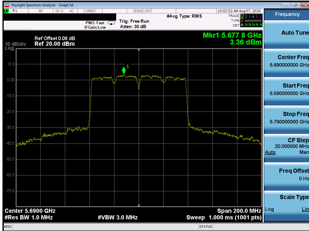
Plot 7-75. Power Spectral Density Plot ANT WF8 (80MHz BW 802.11ac (UNII Band 2C) – Ch. 138)
