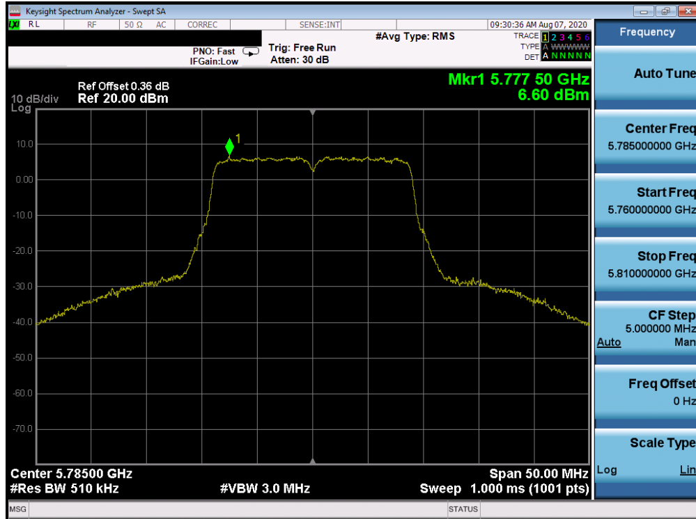
Plot 7-77. Power Spectral Density Plot ANT WF8 (20MHz BW 802.11n (UNII Band 3) – Ch. 157)
