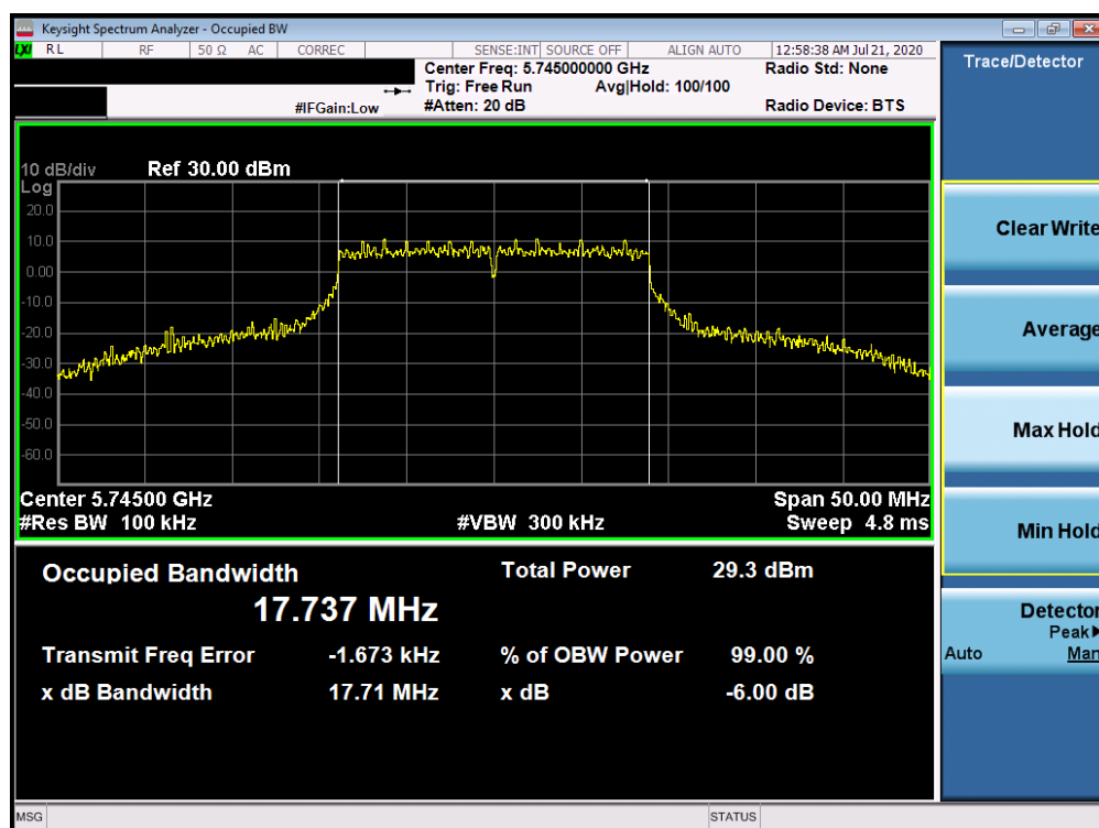
Plot 7-47. 6dB Bandwidth Plot ANT WF7a (20MHz BW 802.11n (UNII Band 3) – Ch. 149)
