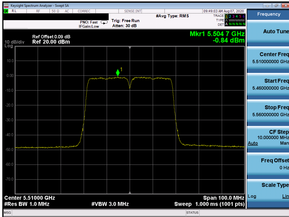
Plot 7-71. Power Spectral Density Plot ANT WF8 (40MHz BW 802.11n (UNII Band 2C) – Ch. 102)
