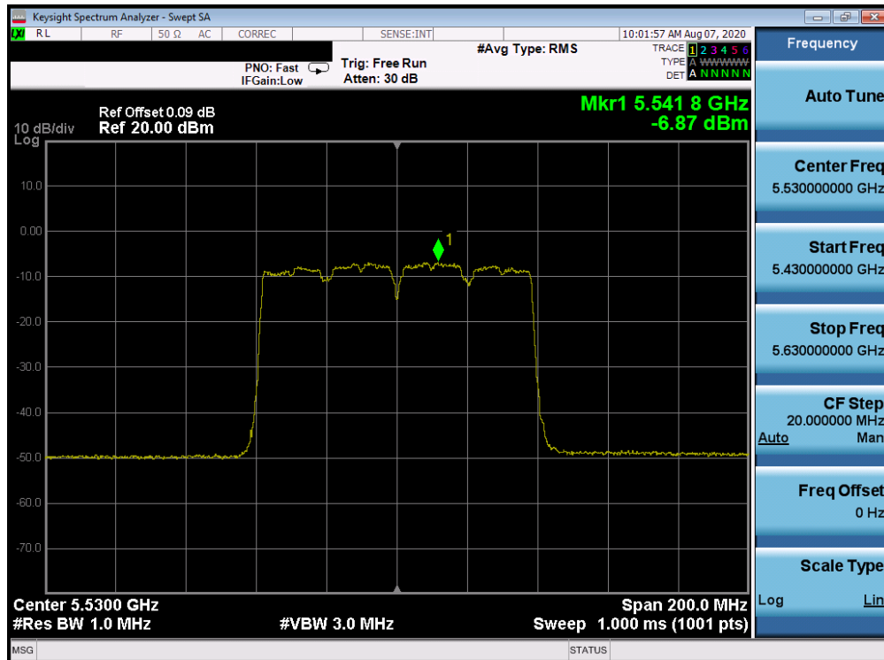
Plot 7-74. Power Spectral Density Plot ANT WF8 (80MHz BW 802.11ac (UNII Band 2C) – Ch. 106)
