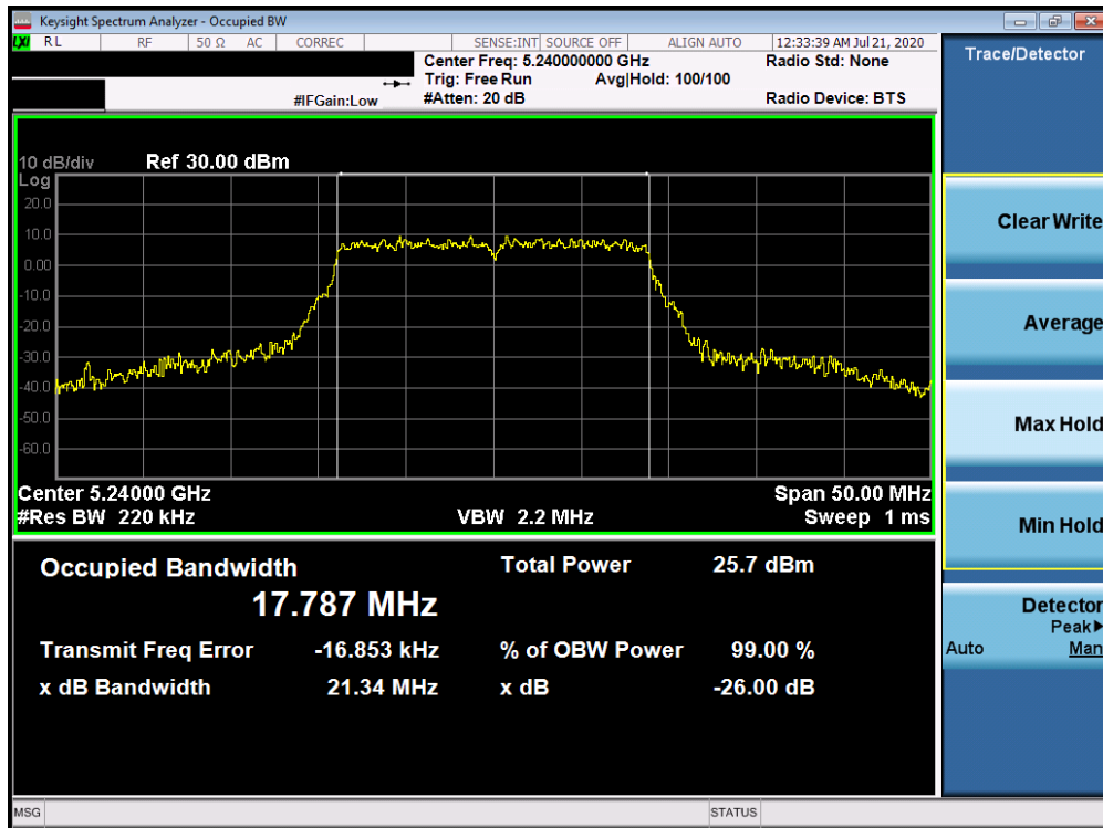
Plot 7-23. 26dB Bandwidth Plot ANT WF7a (20MHz BW 802.11n (UNII Band 1) – Ch. 48)
