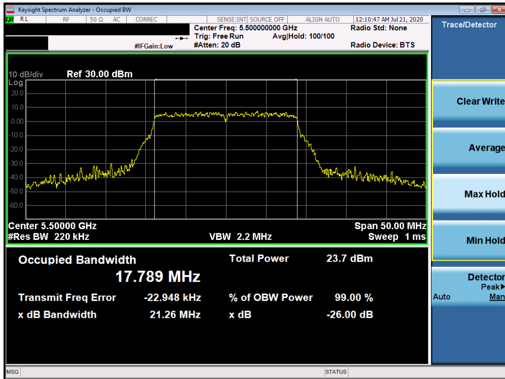
Plot 7-13. 26dB Bandwidth Plot ANT WF8 (20MHz BW 802.11n (UNII Band 2C) – Ch. 100)
