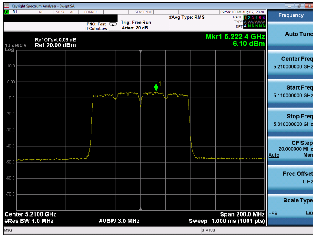
Plot 7-61. Power Spectral Density Plot ANT WF8 (80MHz BW 802.11ac (UNII Band 1) – Ch. 42)
