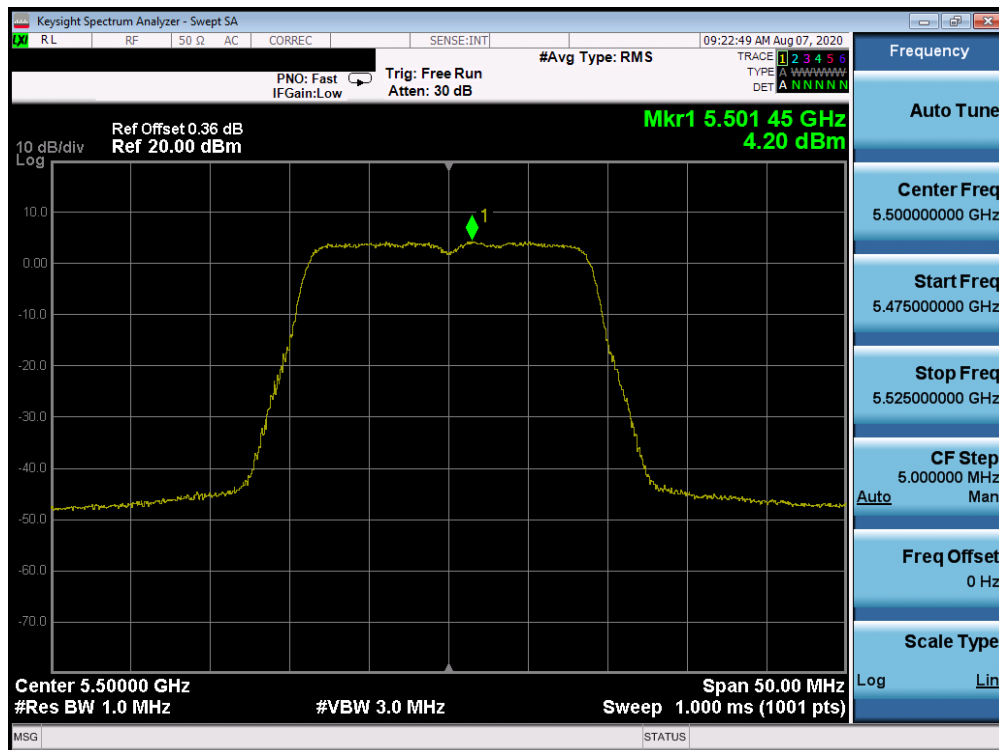
Plot 7-68. Power Spectral Density Plot ANT WF8 (20MHz BW 802.11n (UNII Band 2C) – Ch. 100)
