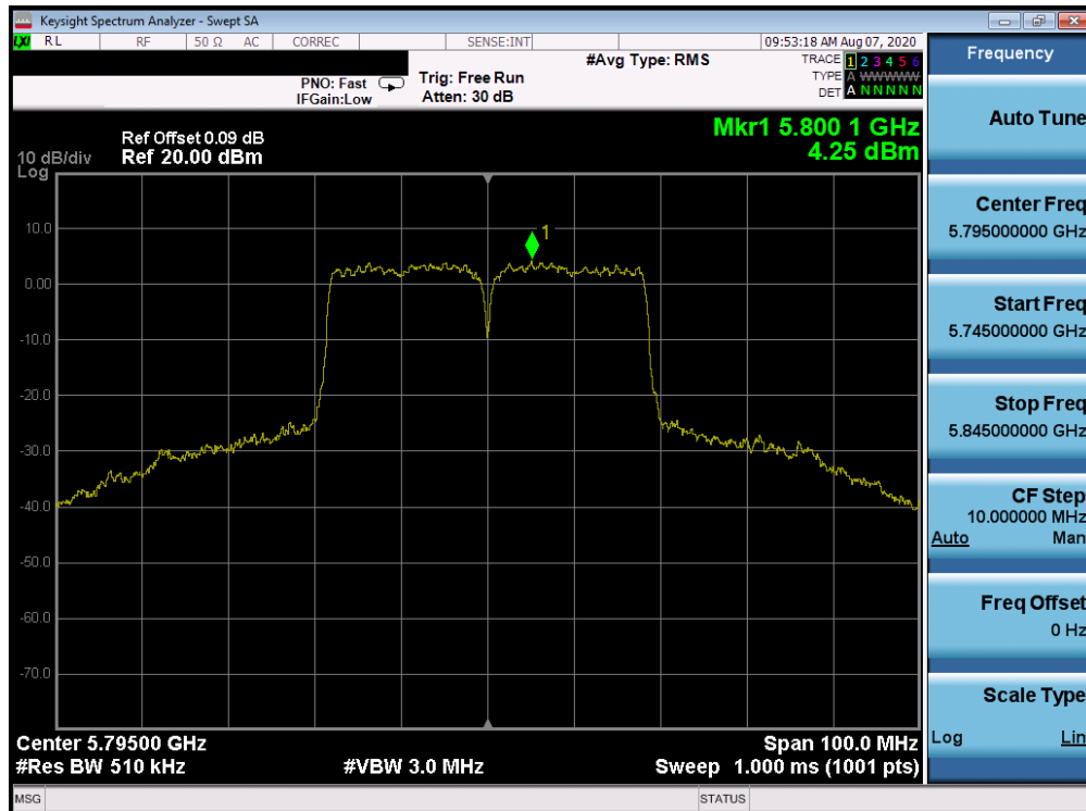
Plot 7-80. Power Spectral Density Plot ANT WF8 (40MHz BW 802.11n (UNII Band 3) – Ch. 159)
