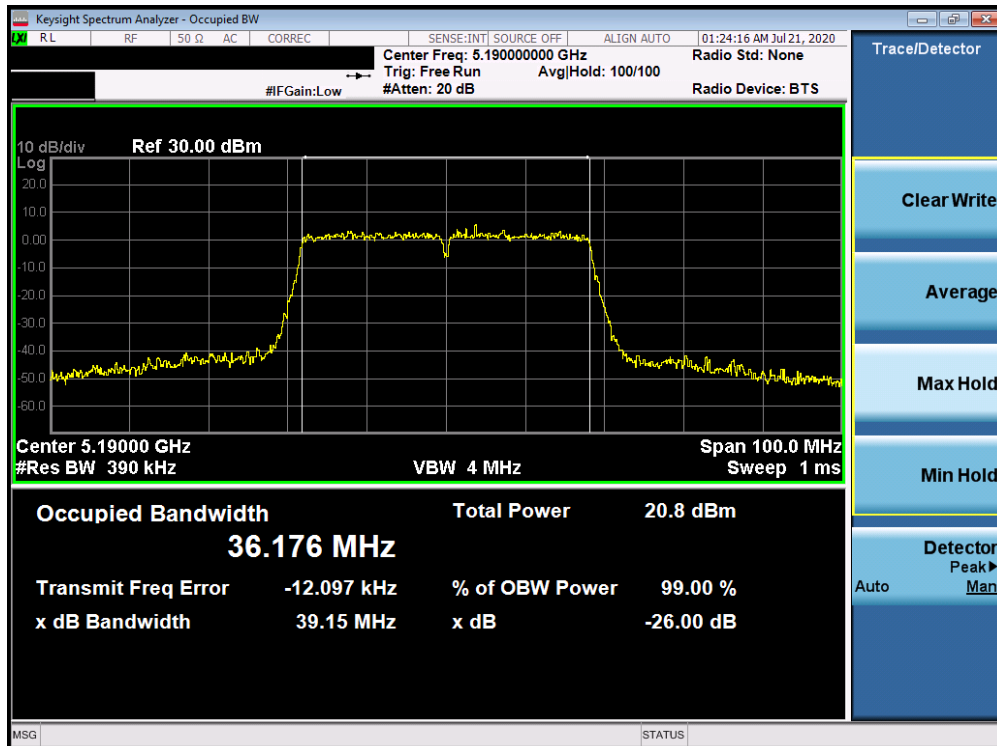
Plot 7-4. 26dB Bandwidth Plot ANT WF8 (40MHz BW 802.11n (UNII Band 1) – Ch. 38)
