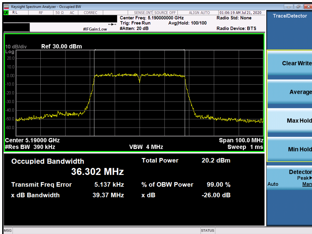
Plot 7-24. 26dB Bandwidth Plot ANT WF7a (40MHz BW 802.11n (UNII Band 1) – Ch. 38)
