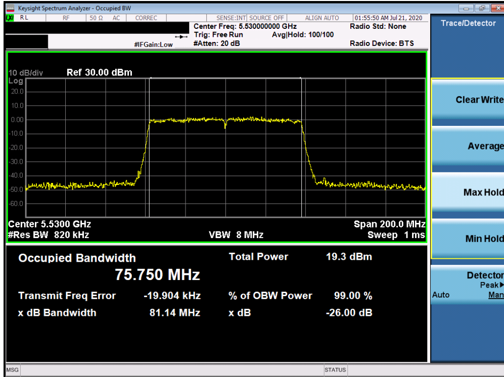
Plot 7-39. 26dB Bandwidth Plot ANT WF7a (80MHz BW 802.11ac (UNII Band 2C) – Ch. 106)
