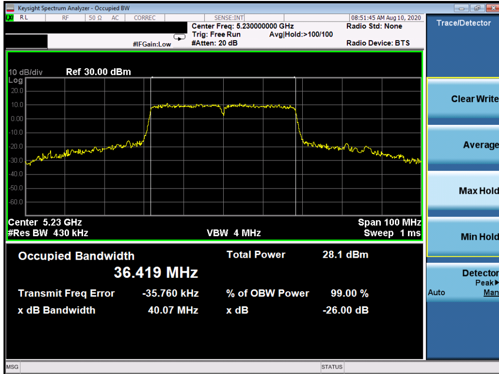
Plot 7-5. 26dB Bandwidth Plot ANT WF8 (40MHz BW 802.11n (UNII Band 1) – Ch. 46)
