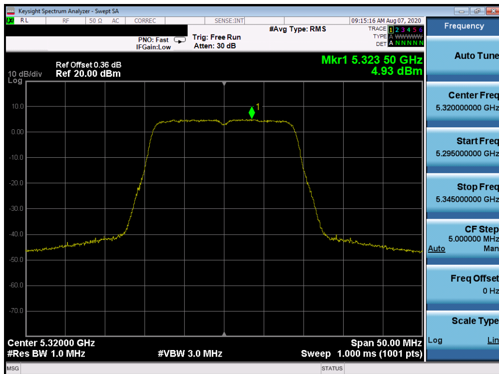
Plot 7-64. Power Spectral Density Plot ANT WF8 (20MHz BW 802.11n (UNII Band 2A) – Ch. 64)
