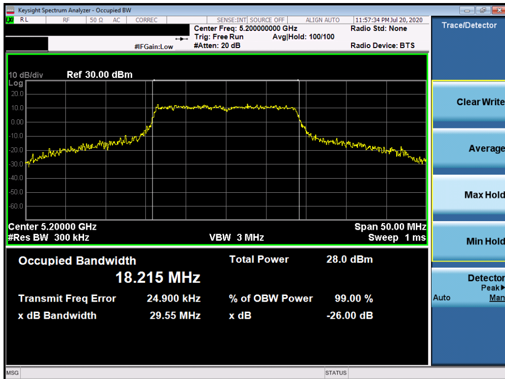
Plot 7-2. 26dB Bandwidth Plot ANT WF8 (20MHz BW 802.11n (UNII Band 1) – Ch. 40)
