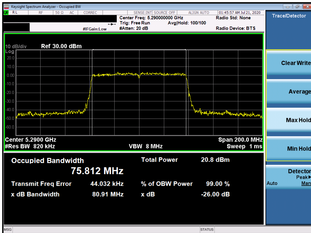
Plot 7-12. 26dB Bandwidth Plot ANT WF8 (80MHz BW 802.11ac (UNII Band 2A) – Ch. 58)
