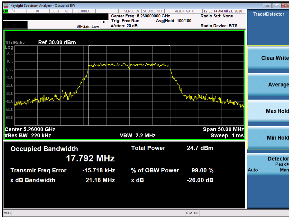
Plot 7-27. 26dB Bandwidth Plot ANT WF7a (20MHz BW 802.11n (UNII Band 2A) – Ch. 52)
