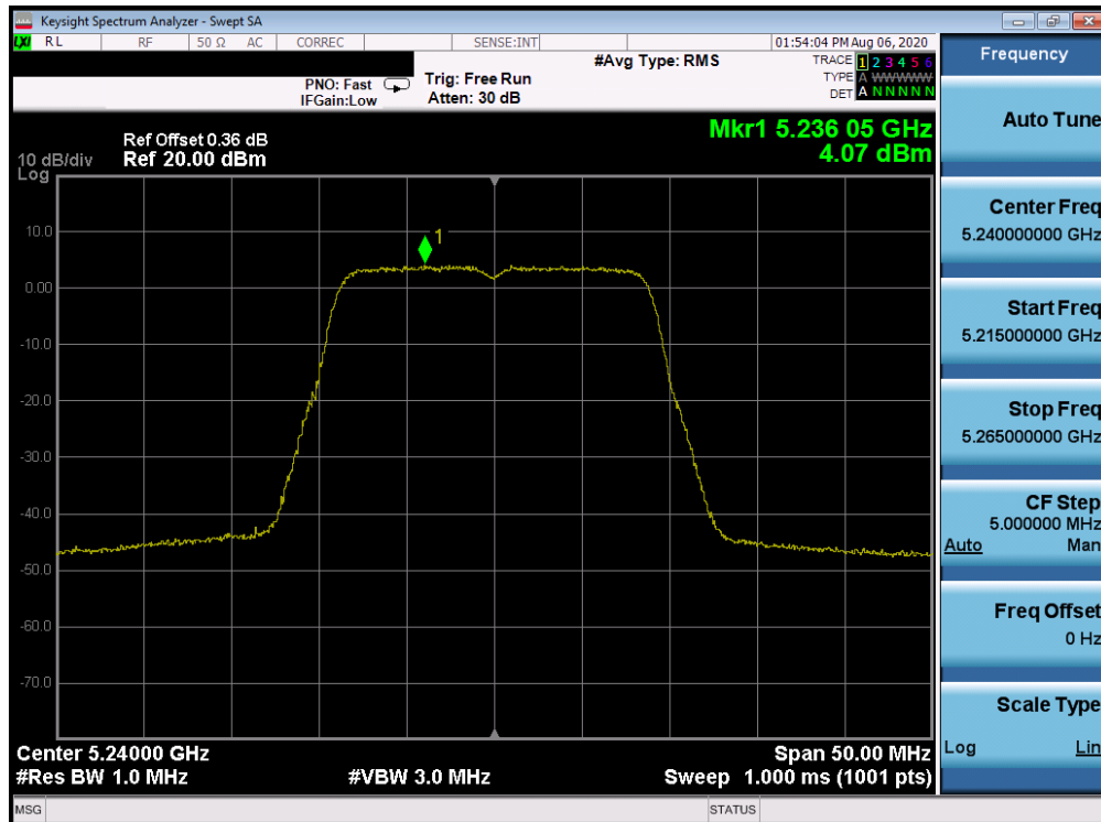
Plot 7-58. ISSED Power Spectral Density Plot ANT WF8 (20MHz BW 802.11n (UNII Band 1) – Ch. 48)
