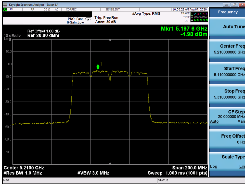
Plot 7-90. Power Spectral Density Plot ANT WF7a (80MHz BW 802.11ac (UNII Band 1) – Ch. 42)
