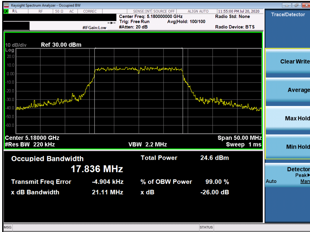
Plot 7-1. 26dB Bandwidth Plot ANT WF8 (20MHz BW 802.11n (UNII Band 1) – Ch. 36)
