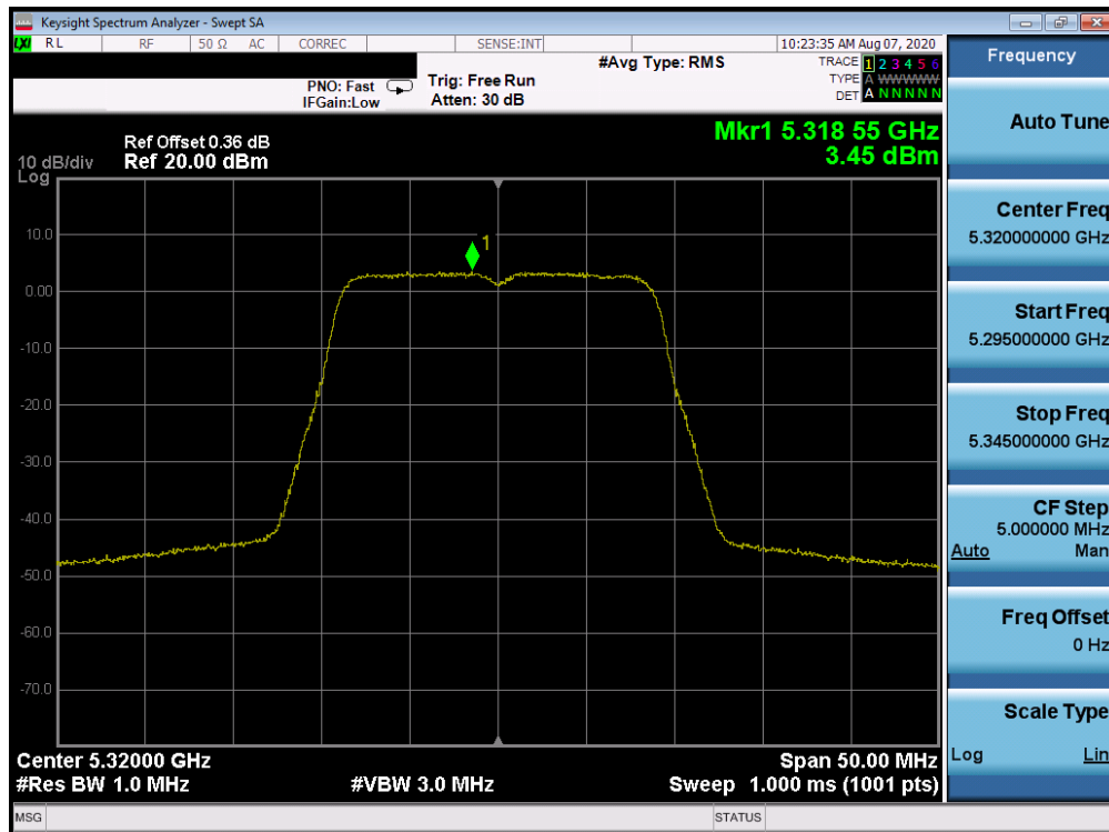
Plot 7-93. Power Spectral Density Plot ANT WF7a (20MHz BW 802.11n (UNII Band 2A) – Ch. 64)
