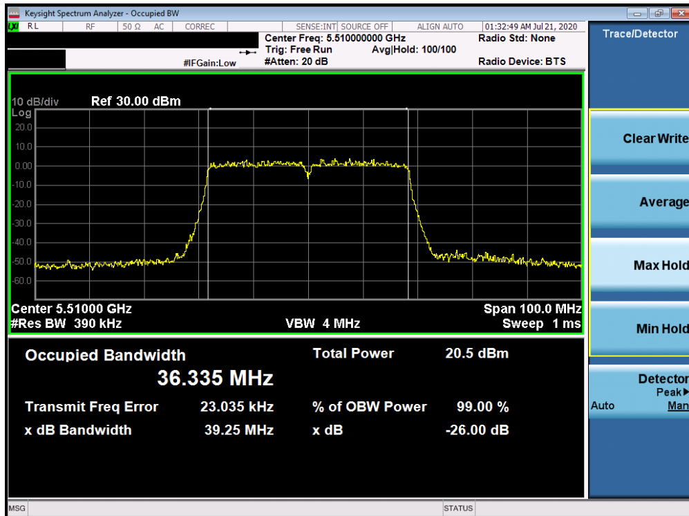
Plot 7-16. 26dB Bandwidth Plot ANT WF8 (40MHz BW 802.11n (UNII Band 2C) – Ch. 102)
