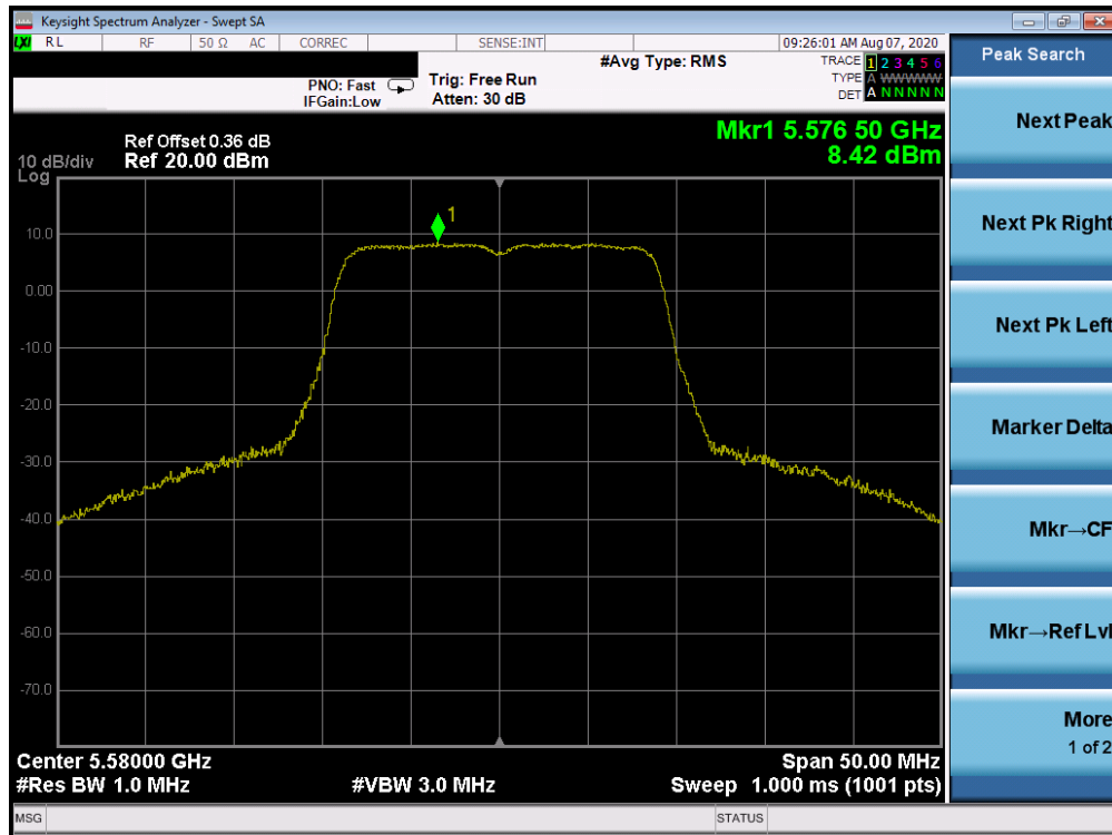
Plot 7-69. Power Spectral Density Plot ANT WF8 (20MHz BW 802.11n (UNII Band 2C) – Ch. 116
