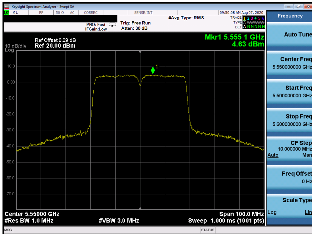
Plot 7-72. Power Spectral Density Plot ANT WF8 (40MHz BW 802.11n (UNII Band 2C) – Ch. 110)
