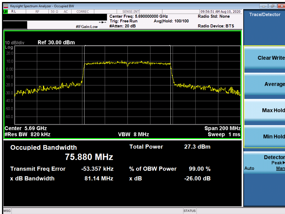
Plot 7-20. 26dB Bandwidth Plot ANT WF8 (80MHz BW 802.11ac (UNII Band 2C) – Ch. 138)
