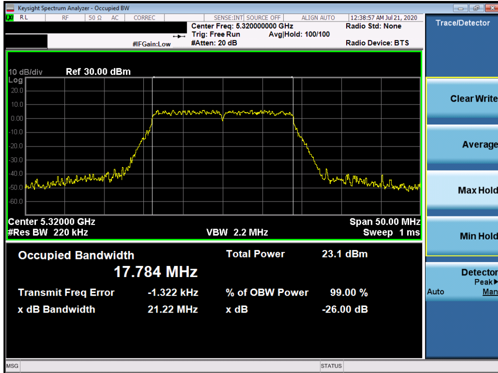
Plot 7-29. 26dB Bandwidth Plot ANT WF7a (20MHz BW 802.11n (UNII Band 2A) – Ch. 64)
