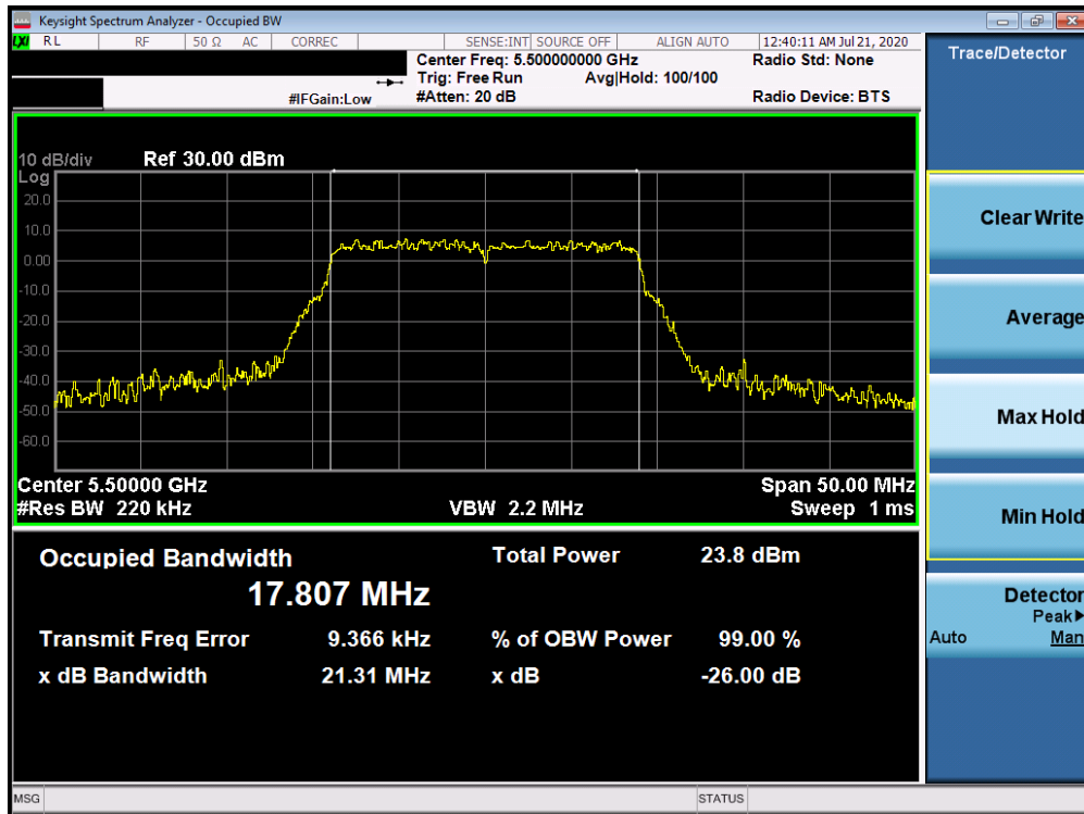
Plot 7-33. 26dB Bandwidth Plot ANT WF7a (20MHz BW 802.11n (UNII Band 2C) – Ch. 100)
