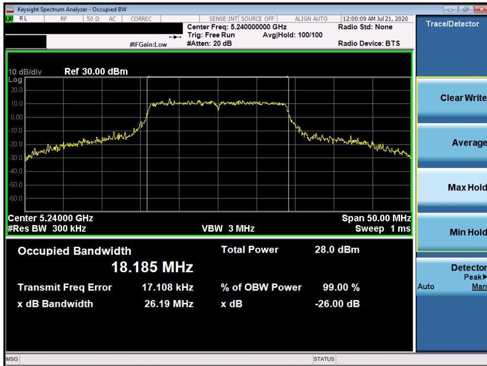
Plot 7-3. 26dB Bandwidth Plot ANT WF8 (20MHz BW 802.11n (UNII Band 1) – Ch. 48)
