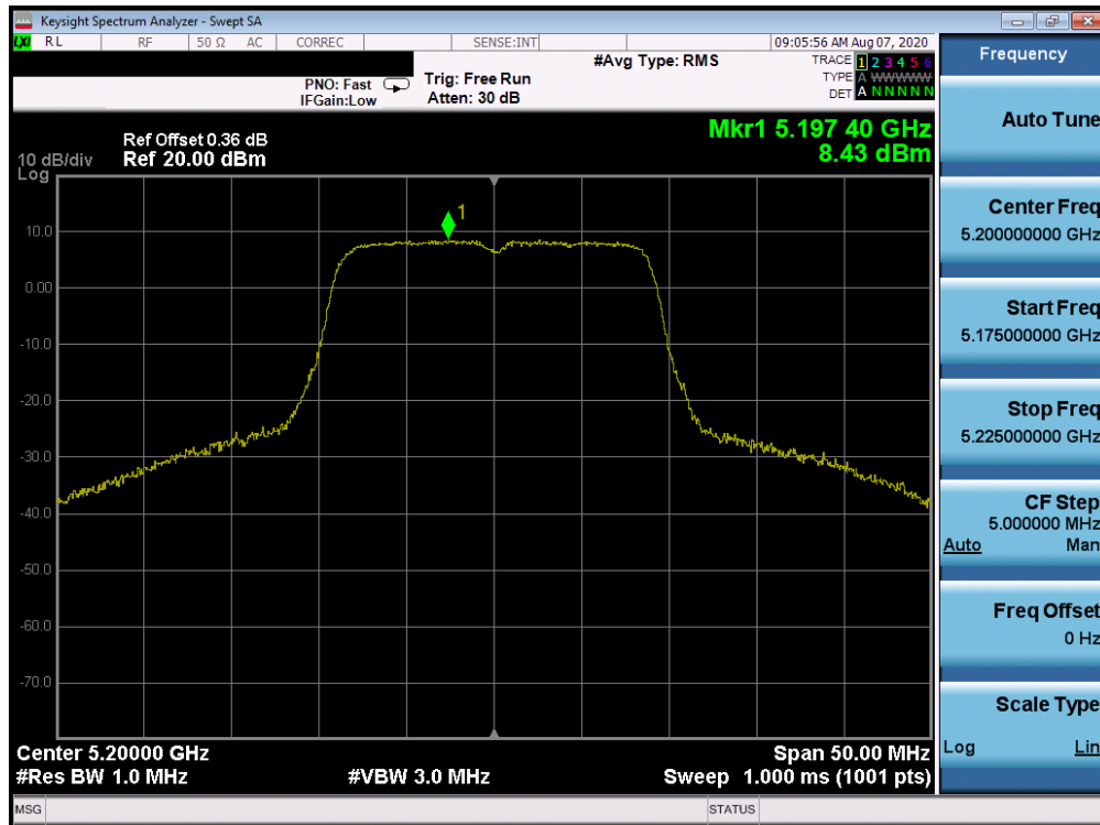
Plot 7-55. Power Spectral Density Plot ANT WF8 (20MHz BW 802.11n (UNII Band 1) – Ch. 40)
