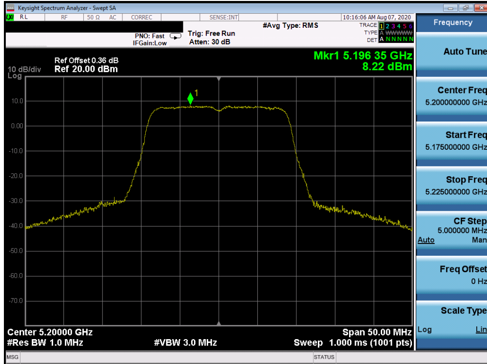
Plot 7-84. Power Spectral Density Plot ANT WF7a (20MHz BW 802.11n (UNII Band 1) – Ch. 40)
