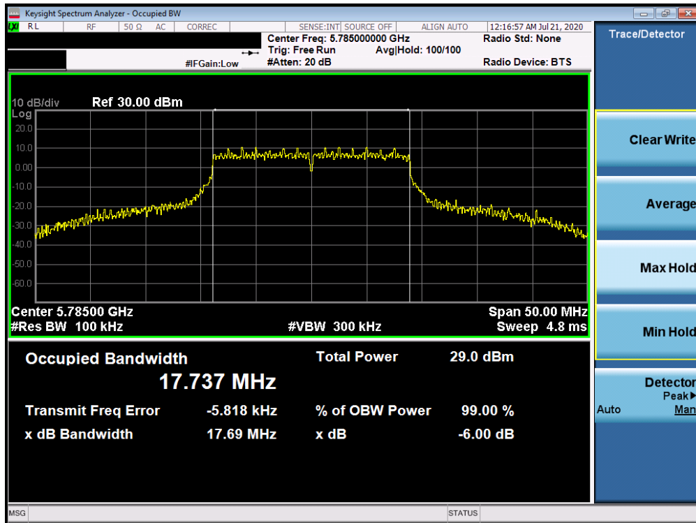
Plot 7-42. 6dB Bandwidth Plot ANT WF8 (20MHz BW 802.11n (UNII Band 3) – Ch. 157)
