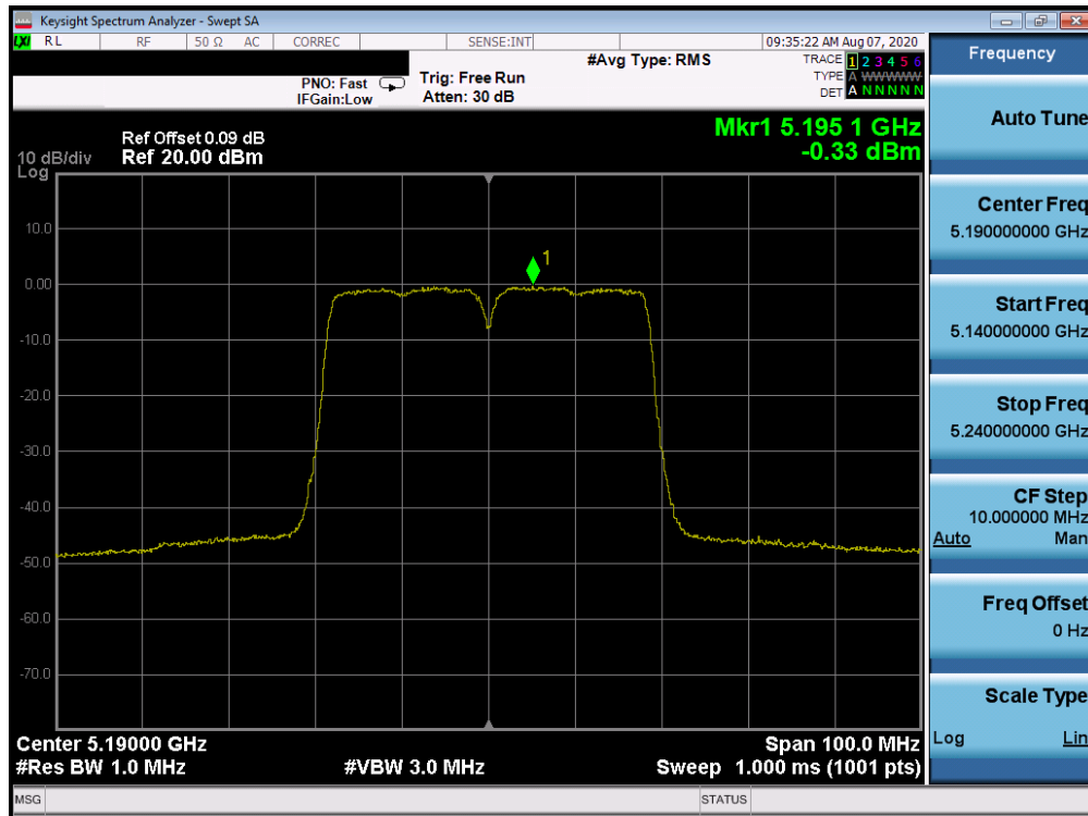
Plot 7-59. Power Spectral Density Plot ANT WF8 (40MHz BW 802.11n (UNII Band 1) – Ch. 38)
