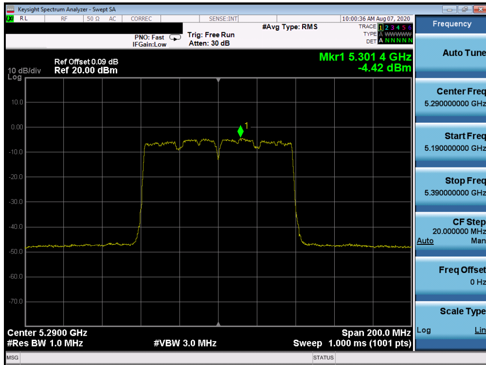
Plot 7-67. Power Spectral Density Plot ANT WF8 (80MHz BW 802.11ac (UNII Band 2A) – Ch. 58)
