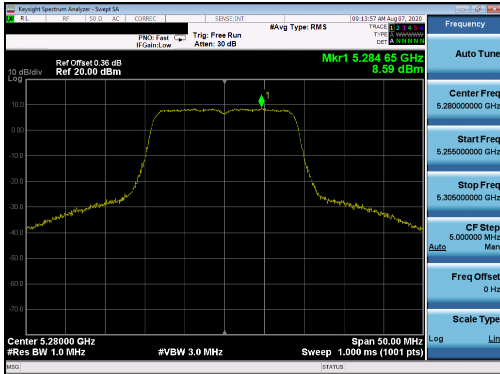
Plot 7-63. Power Spectral Density Plot ANT WF8 (20MHz BW 802.11n (UNII Band 2A) – Ch. 56)
