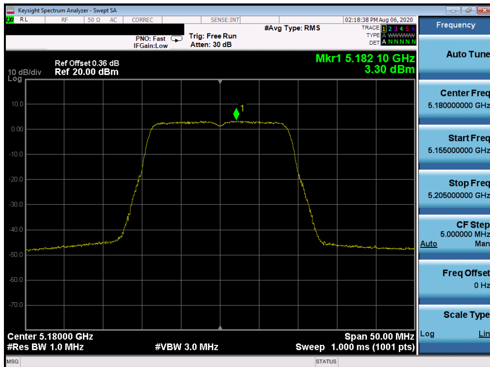
Plot 7-83. ISD Power Spectral Density Plot ANT WF7a (20MHz BW 802.11n (UNII Band 1) – Ch. 36)
