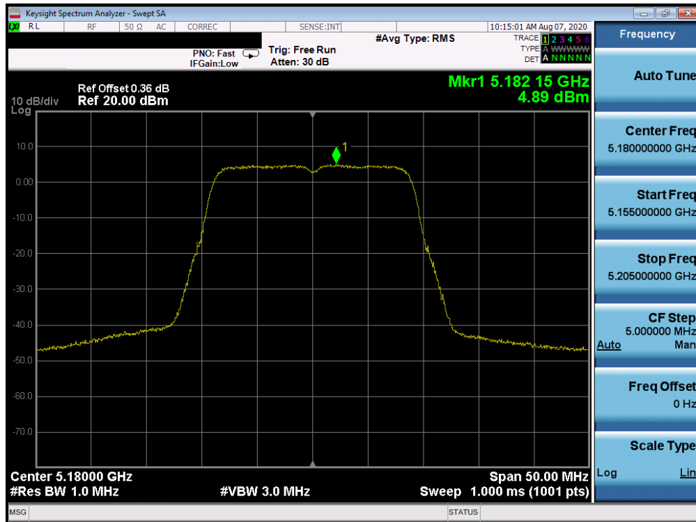
Plot 7-82. Power Spectral Density Plot ANT WF7a (20MHz BW 802.11n (UNII Band 1) – Ch. 36)
