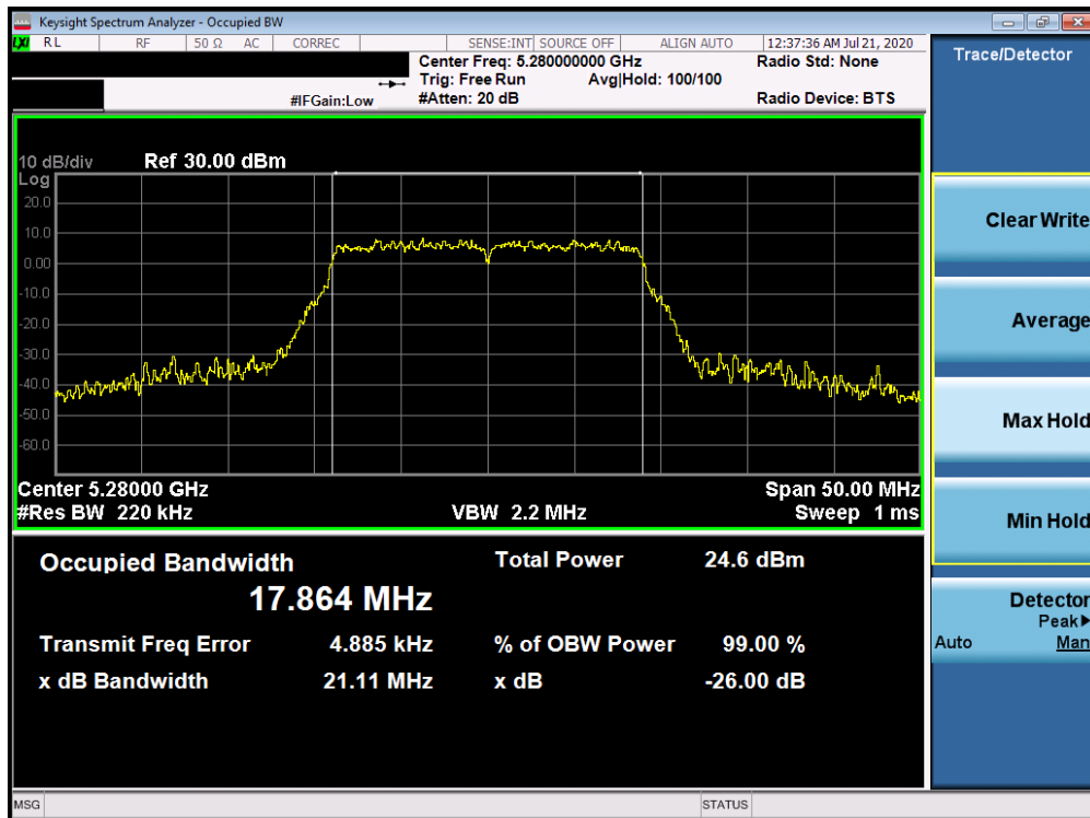
Plot 7-28. 26dB Bandwidth Plot ANT WF7a (20MHz BW 802.11n (UNII Band 2A) – Ch. 56)
