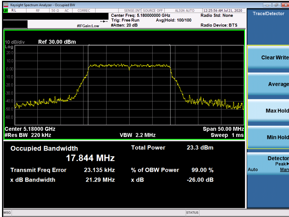
Plot 7-21. 26dB Bandwidth Plot ANT WF7a (20MHz BW 802.11n (UNII Band 1) – Ch. 36)
