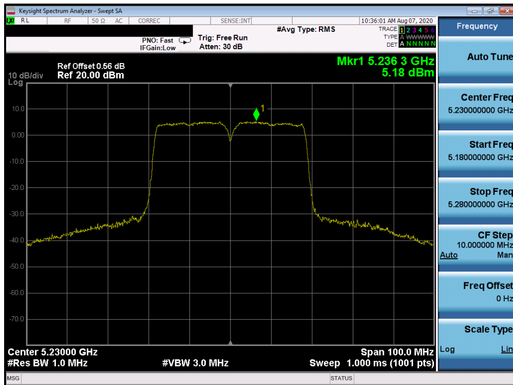
Plot 7-89. Power Spectral Density Plot ANT WF7a (40MHz BW 802.11n (UNII Band 1) – Ch. 46)
