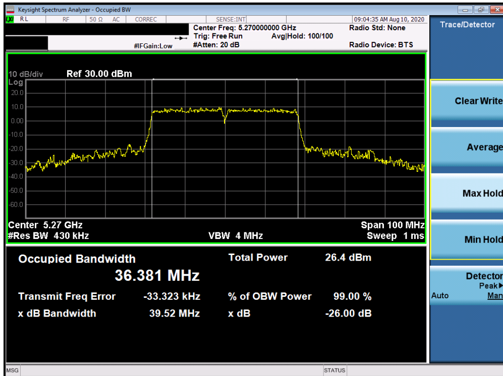
Plot 7-10. 26dB Bandwidth Plot ANT WF8 (40MHz BW 802.11n (UNII Band 2A) – Ch. 54)
