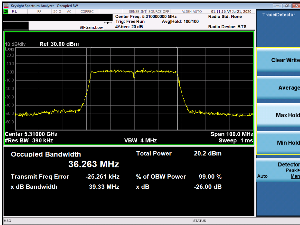
Plot 7-31. 26dB Bandwidth Plot ANT WF7a (40MHz BW 802.11n (UNII Band 2A) – Ch. 62)
