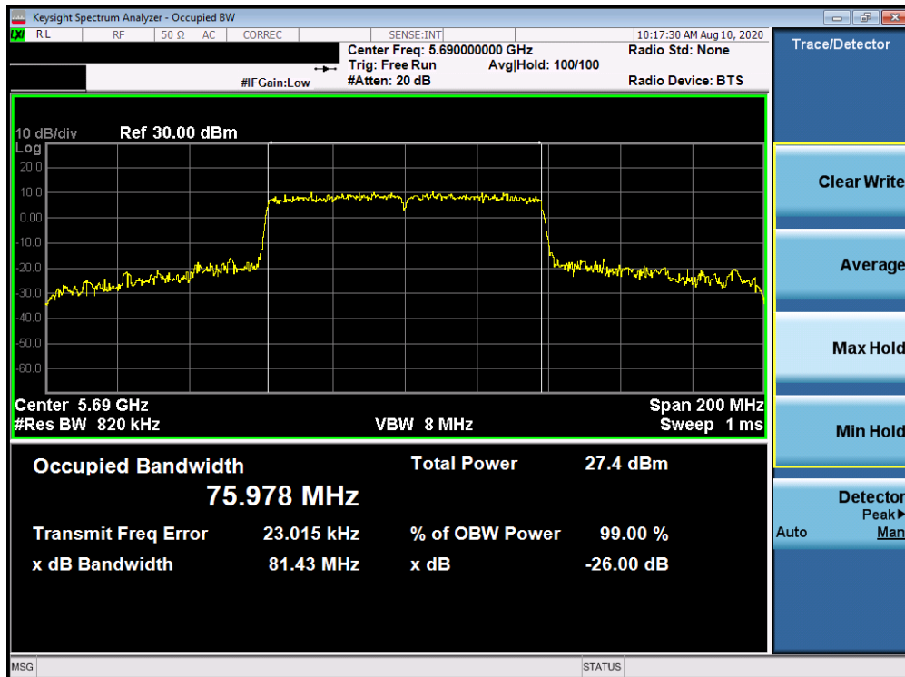
Plot 7-40. 26dB Bandwidth Plot ANT WF7a (80MHz BW 802.11ac (UNII Band 2C) – Ch. 138)
