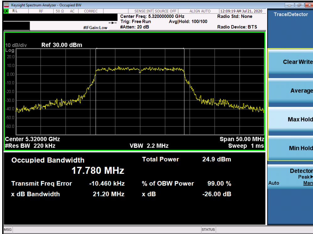
Plot 7-9. 26dB Bandwidth Plot ANT WF8 (20MHz BW 802.11n (UNII Band 2A) – Ch. 64)
