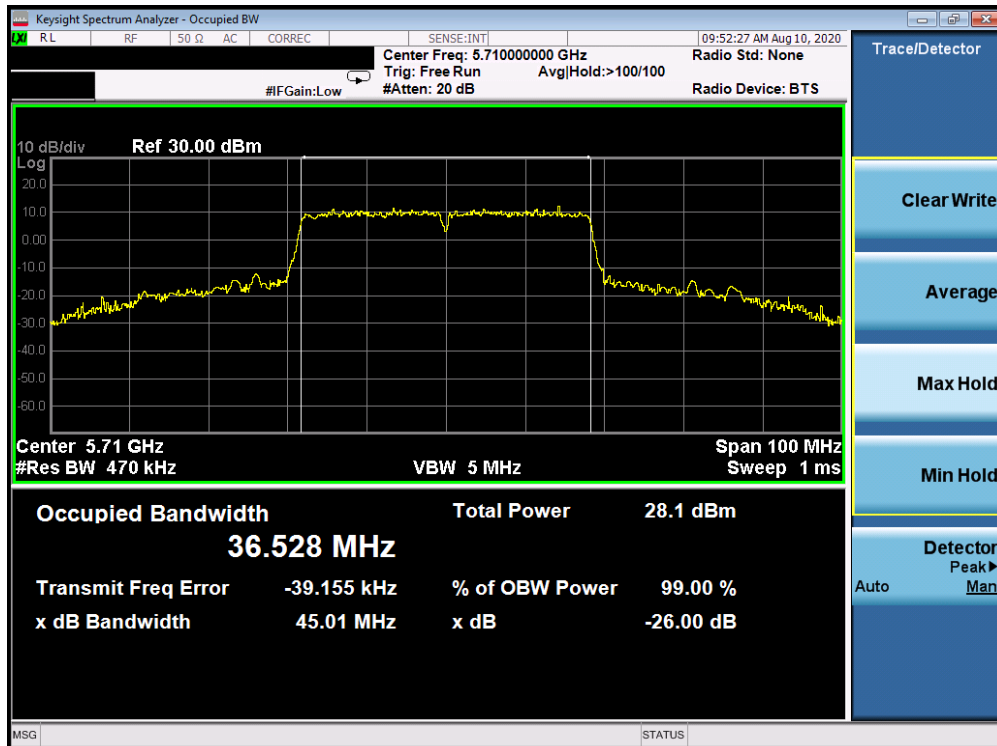
Plot 7-18. 26dB Bandwidth Plot ANT WF8 (40MHz BW 802.11n (UNII Band 2C) – Ch. 142)
