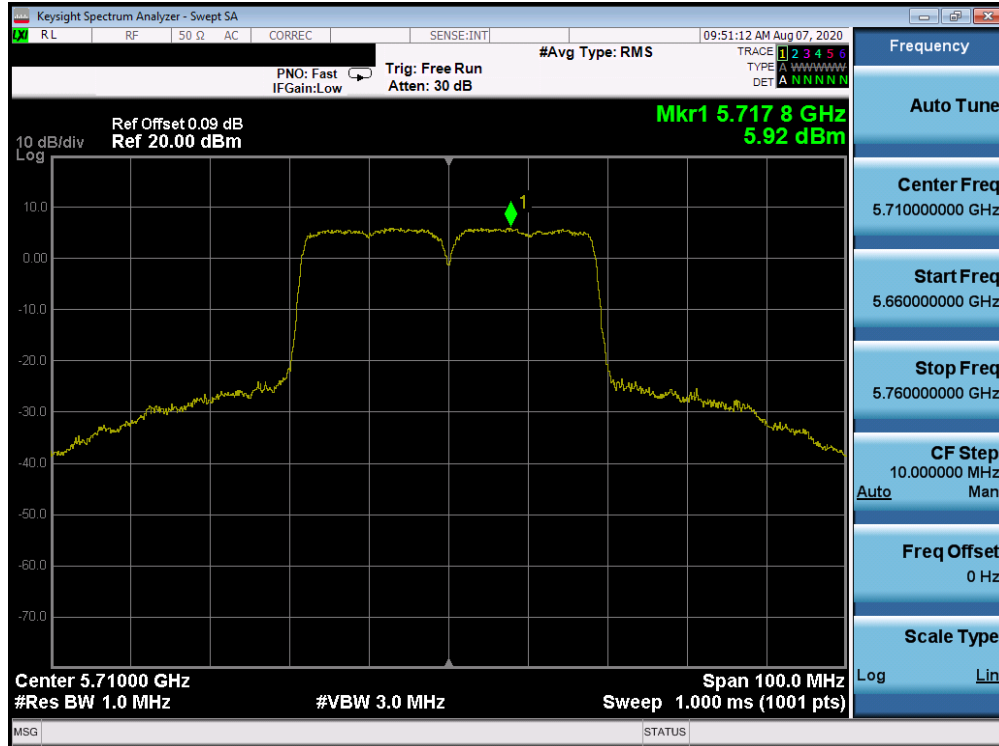
Plot 7-73. Power Spectral Density Plot ANT WF8 (40MHz BW 802.11n (UNII Band 2C) – Ch. 142)
