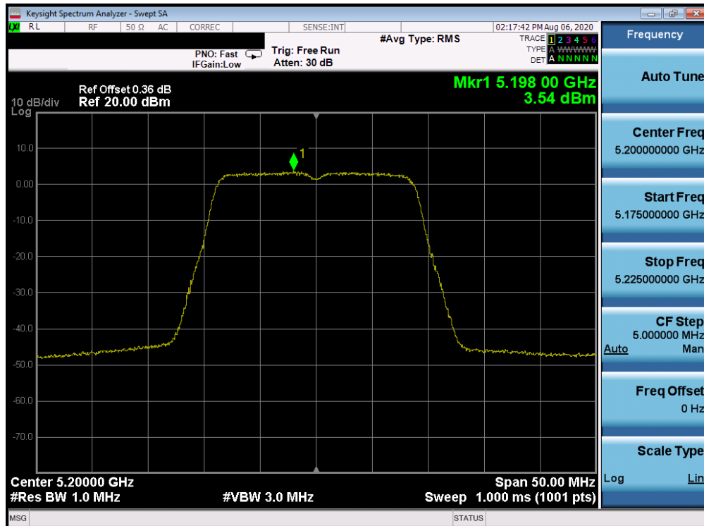
Plot 7-85. ISD Power Spectral Density Plot ANT WF7a (20MHz BW 802.11n (UNII Band 1) – Ch. 40)
