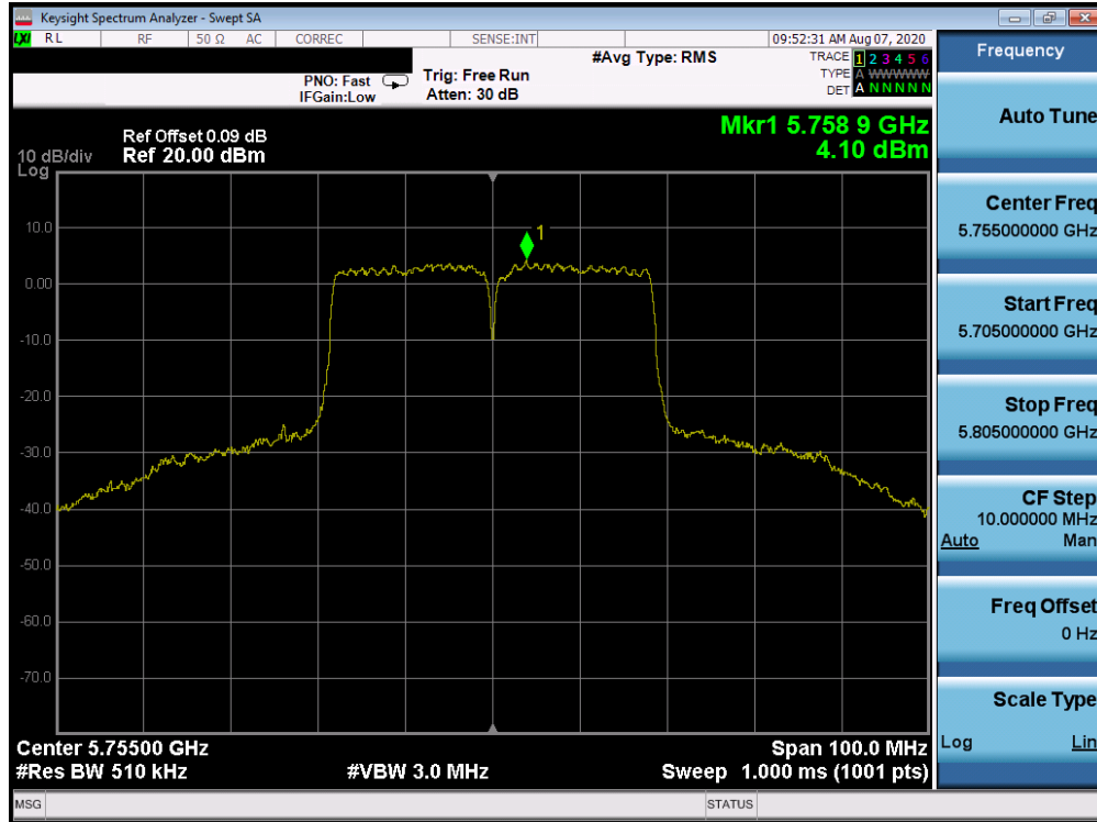
Plot 7-79. Power Spectral Density Plot ANT WF8 (40MHz BW 802.11n (UNII Band 3) – Ch. 151)
