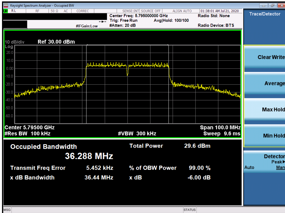
Plot 7-45. 6dB Bandwidth Plot ANT WF8 (40MHz BW 802.11n (UNII Band 3) – Ch. 159)
