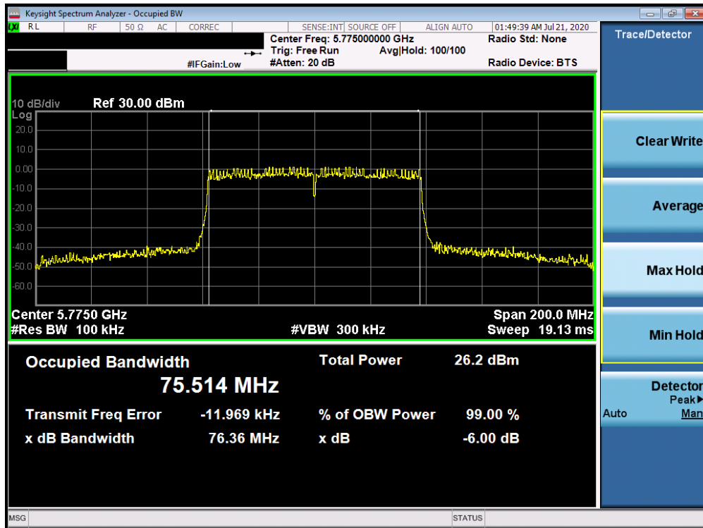
Plot 7-46. 6dB Bandwidth Plot ANT WF8 (80MHz BW 802.11ac (UNII Band 3) – Ch. 155)
