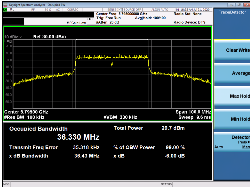
Plot 7-51. 6dB Bandwidth Plot ANT WF7a (40MHz BW 802.11n (UNII Band 3) – Ch. 159)
