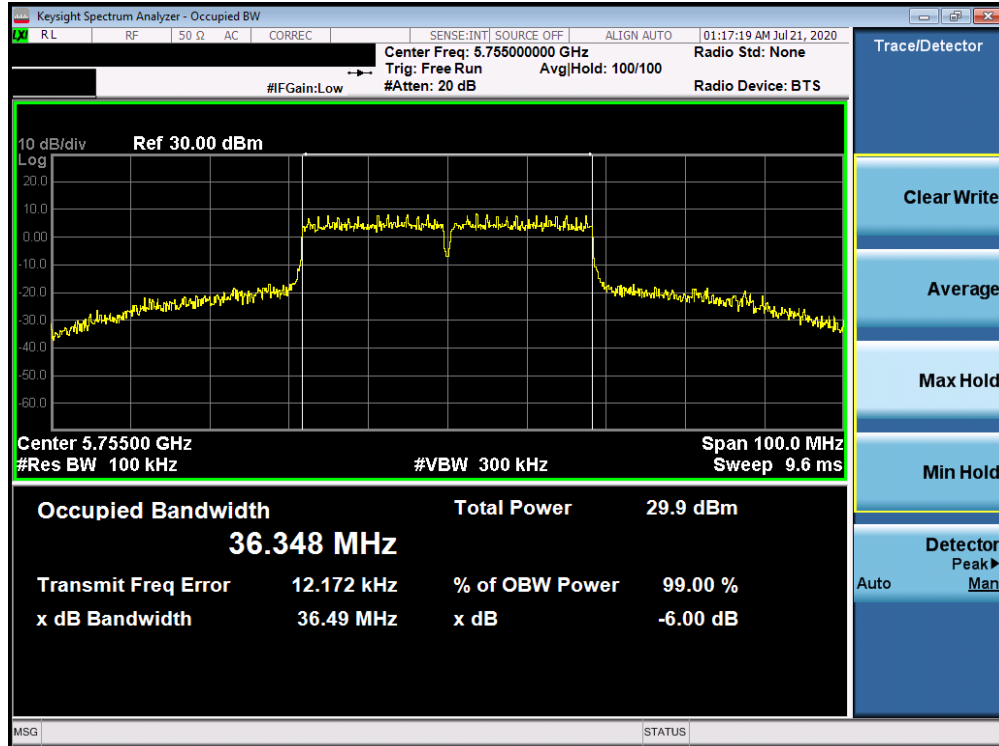
Plot 7-50. 6dB Bandwidth Plot ANT WF7a (40MHz BW 802.11n (UNII Band 3) – Ch. 151)
