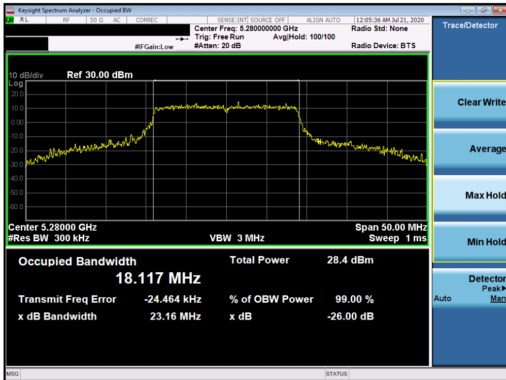
Plot 7-8. 26dB Bandwidth Plot ANT WF8 (20MHz BW 802.11n (UNII Band 2A) – Ch. 56)
