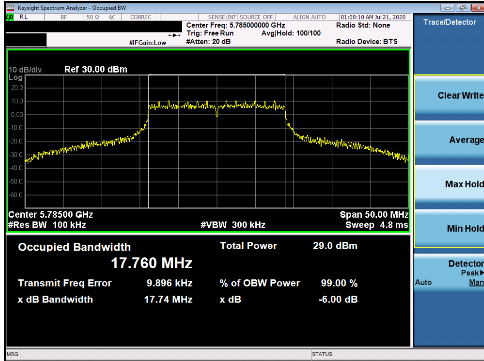
Plot 7-48. 6dB Bandwidth Plot ANT WF7a (20MHz BW 802.11n (UNII Band 3) – Ch. 157)
