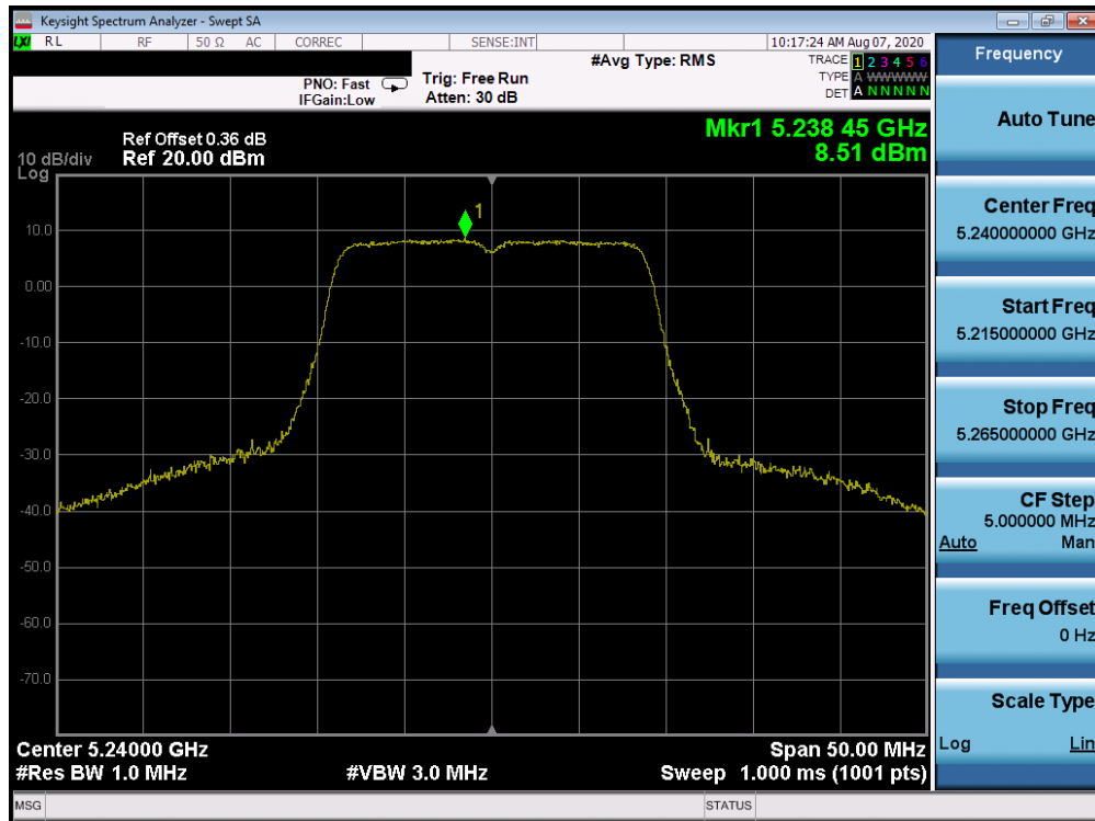
Plot 7-86. Power Spectral Density Plot ANT WF7a (20MHz BW 802.11n (UNII Band 1) – Ch. 48)
