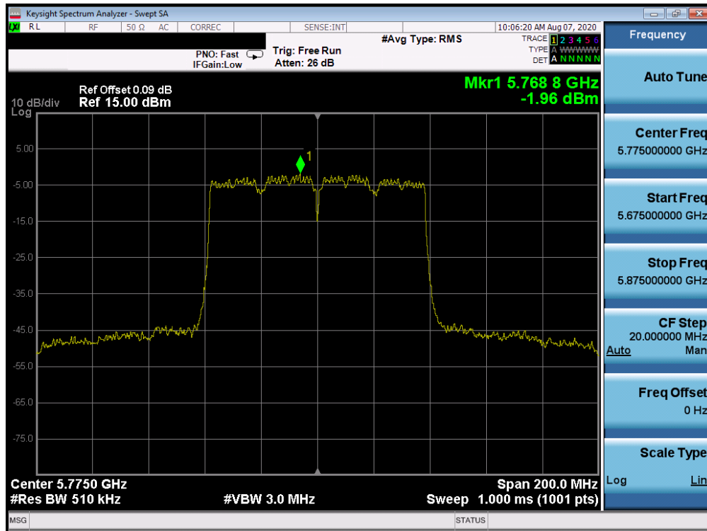
Plot 7-81. Power Spectral Density Plot ANT WF8 (80MHz BW 802.11ac (UNII Band 3) – Ch. 155)
