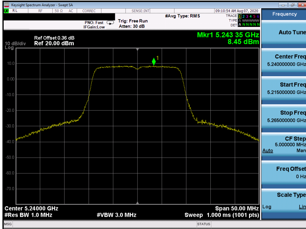
Plot 7-57. Power Spectral Density Plot ANT WF8 (20MHz BW 802.11n (UNII Band 1) – Ch. 48)
