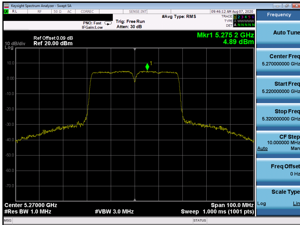
Plot 7-65. Power Spectral Density Plot ANT WF8 (40MHz BW 802.11n (UNII Band 2A) – Ch. 54)
