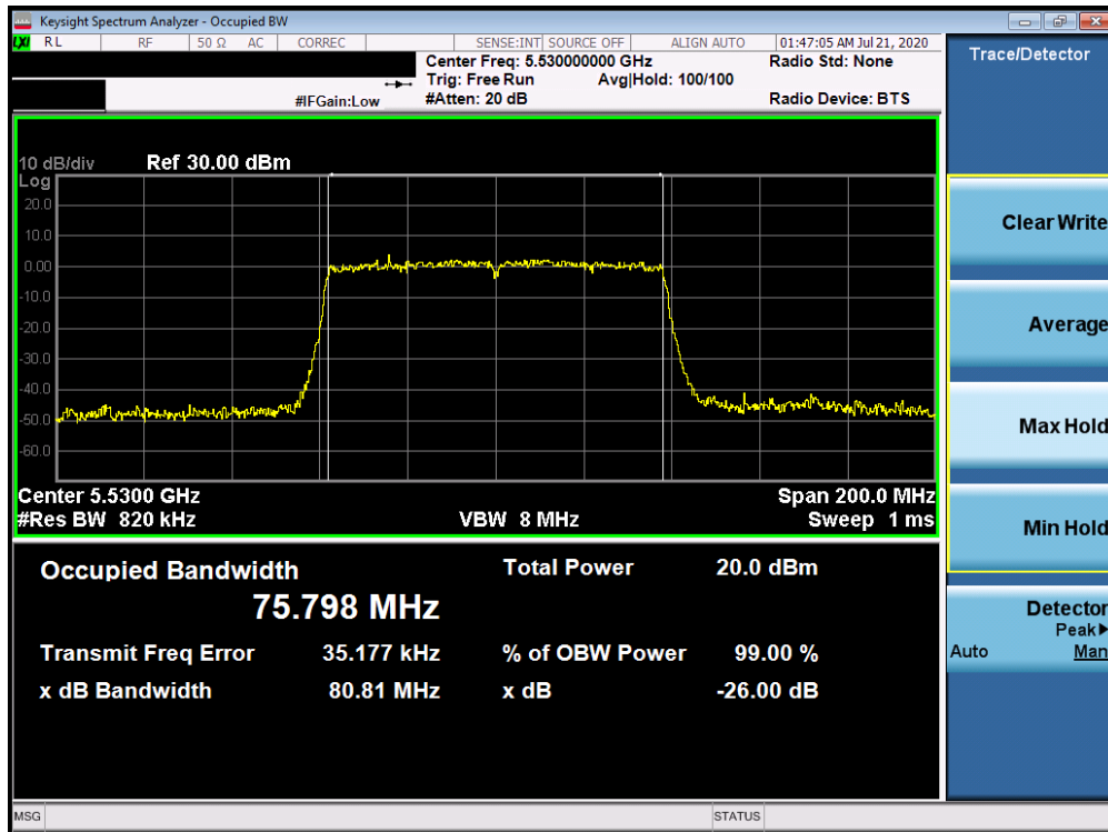
Plot 7-19. 26dB Bandwidth Plot ANT WF8 (80MHz BW 802.11ac (UNII Band 2C) – Ch. 106)
