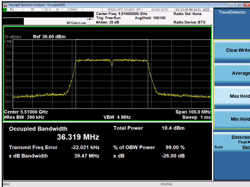
Plot 7-36. 26dB Bandwidth Plot ANT WF7a (40MHz BW 802.11n (UNII Band 2C) – Ch. 102)
