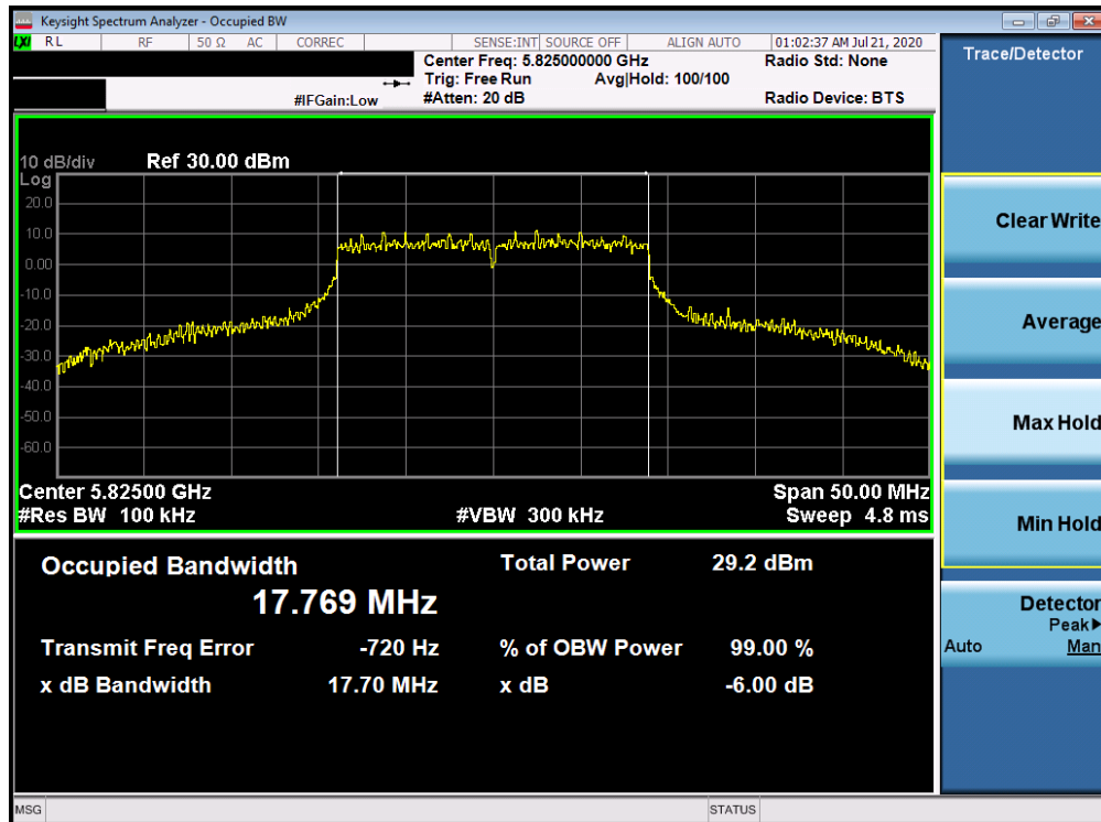
Plot 7-49. 6dB Bandwidth Plot ANT WF7a (20MHz BW 802.11n (UNII Band 3) – Ch. 165)
