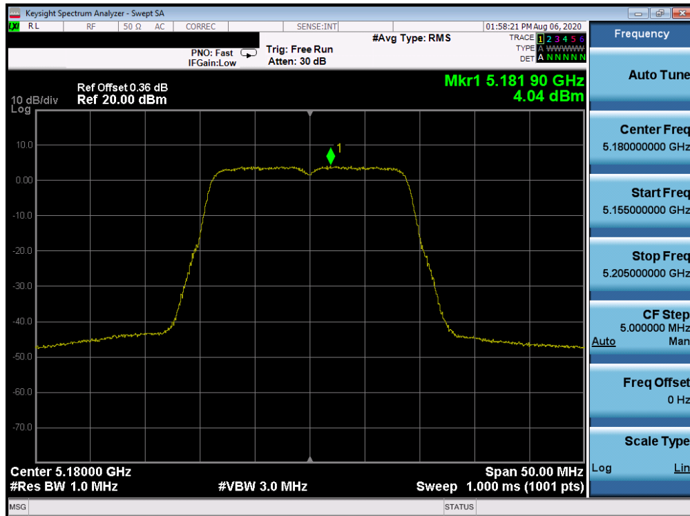
Plot 7-54. ISSED Power Spectral Density Plot ANT WF8 (20MHz BW 802.11n (UNII Band 1) – Ch. 36)
