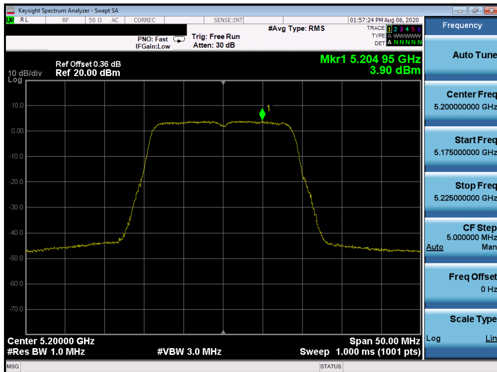
Plot 7-56. ISD Power Spectral Density Plot ANT WF8 (20MHz BW 802.11n (UNII Band 1) – Ch. 40)
