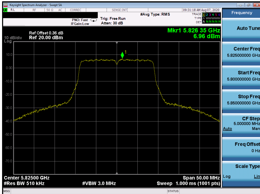
Plot 7-78. Power Spectral Density Plot ANT WF8 (20MHz BW 802.11n (UNII Band 3) – Ch. 165)
