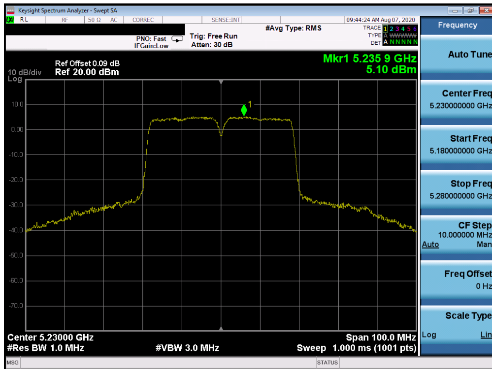
Plot 7-60. Power Spectral Density Plot ANT WF8 (40MHz BW 802.11n (UNII Band 1) – Ch. 46)
