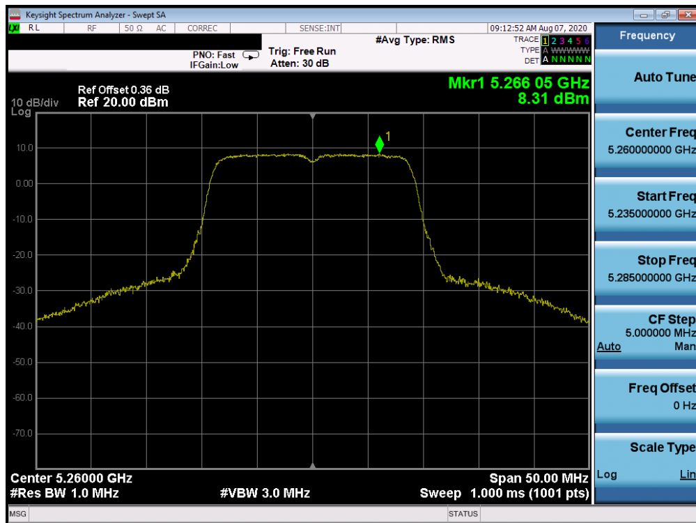
Plot 7-62. Power Spectral Density Plot ANT WF8 (20MHz BW 802.11n (UNII Band 2A) – Ch. 52)
