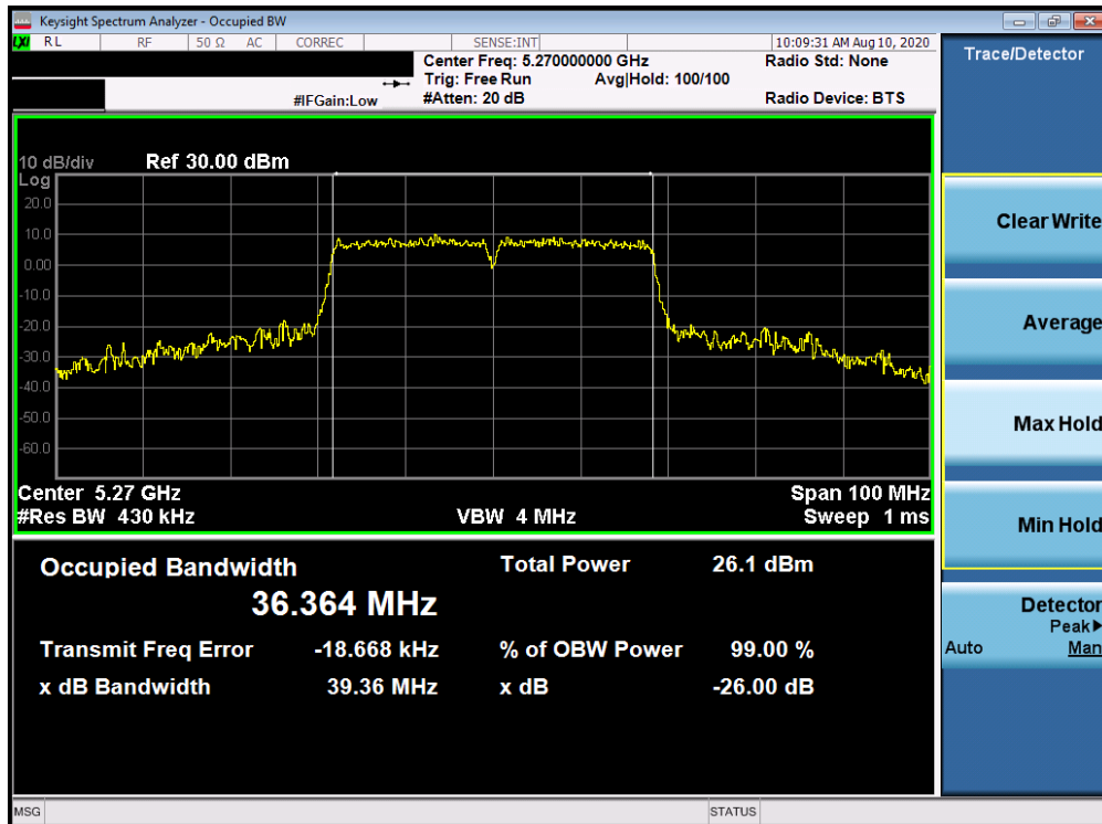
Plot 7-30. 26dB Bandwidth Plot ANT WF7a (40MHz BW 802.11n (UNII Band 2A) – Ch. 54)
