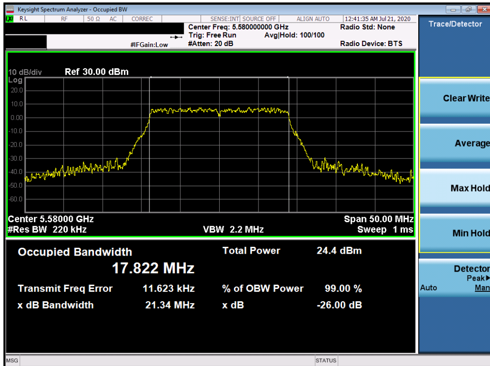
Plot 7-34. 26dB Bandwidth Plot ANT WF7a (20MHz BW 802.11n (UNII Band 2C) – Ch. 116)
