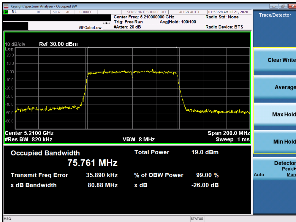
Plot 7-26. 26dB Bandwidth Plot ANT WF7a (80MHz BW 802.11ac (UNII Band 1) – Ch. 42)
