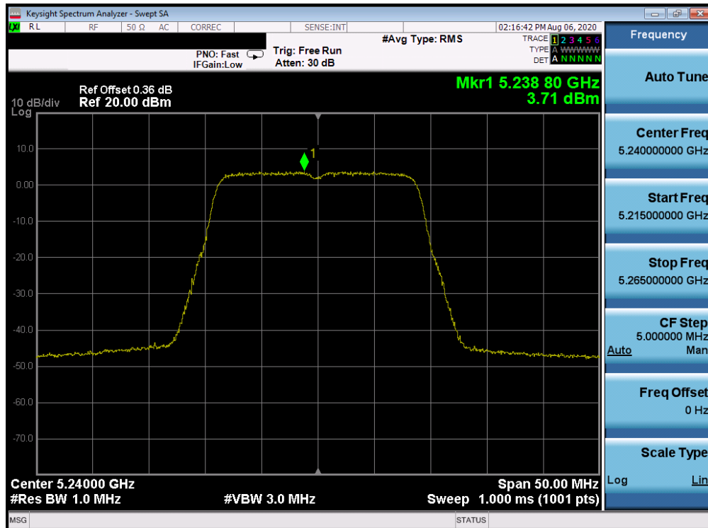
Plot 7-87. ISSED Power Spectral Density Plot ANT WF7a (20MHz BW 802.11n (UNII Band 1) – Ch. 48)
