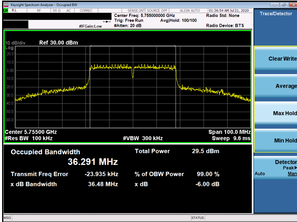
Plot 7-44. 6dB Bandwidth Plot ANT WF8 (40MHz BW 802.11n (UNII Band 3) – Ch. 151)
