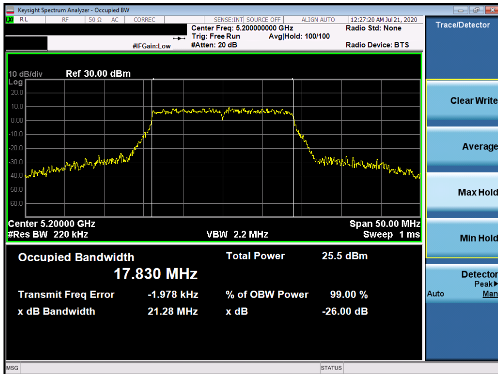
Plot 7-22. 26dB Bandwidth Plot ANT WF7a (20MHz BW 802.11n (UNII Band 1) – Ch. 40)
