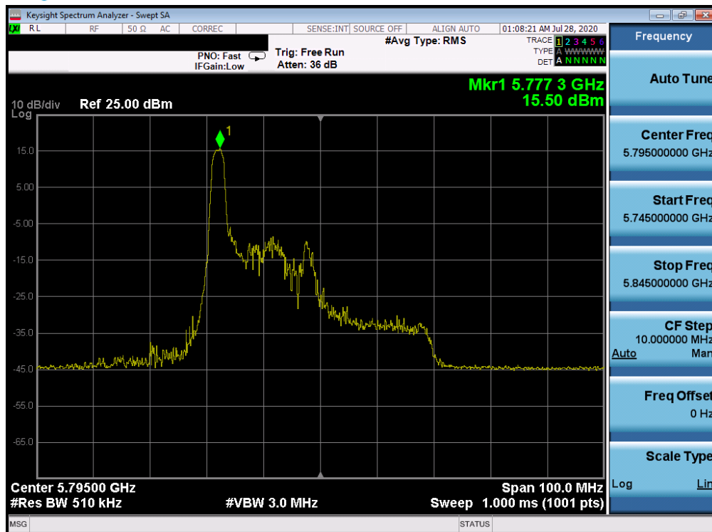
Plot 7-655. Power Spectral Density Plot CDD ANT WF8 (40MHz BW 802.11ax Index 0 – RU26 (UNII Band 3) – Ch. 159)
