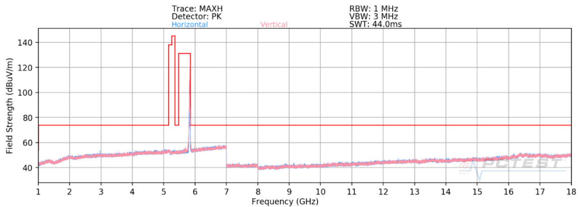
Plot 7-732. Radiated Spurious Emissions above 1GHz ANT WF8 (802.11ax – UNII Band 3, Ch. 165 – RU26)
