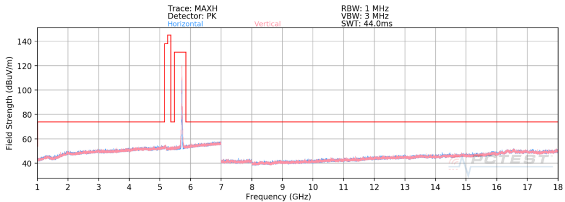
Plot 7-729. Radiated Spurious Emissions above 1GHz ANT WF8 (802.11ax – UNII Band 2C, Ch. 144 – RU26)
