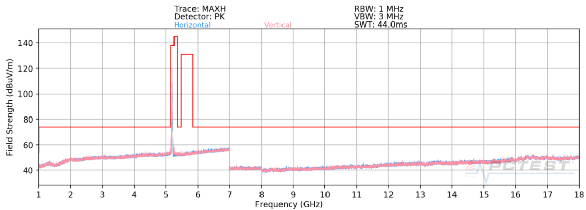
Plot 7-722. Radiated Spurious Emissions above 1GHz ANT WF8 (802.11ax – UNII Band 1, Ch. 40 – RU26)
