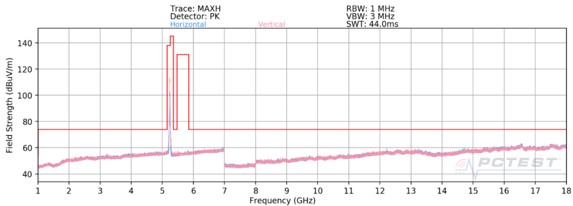
Plot 7-735. Radiated Spurious Emissions above 1GHz ANT WF8 (802.11ax – UNII Band 1, Ch. 48 – RU242)
