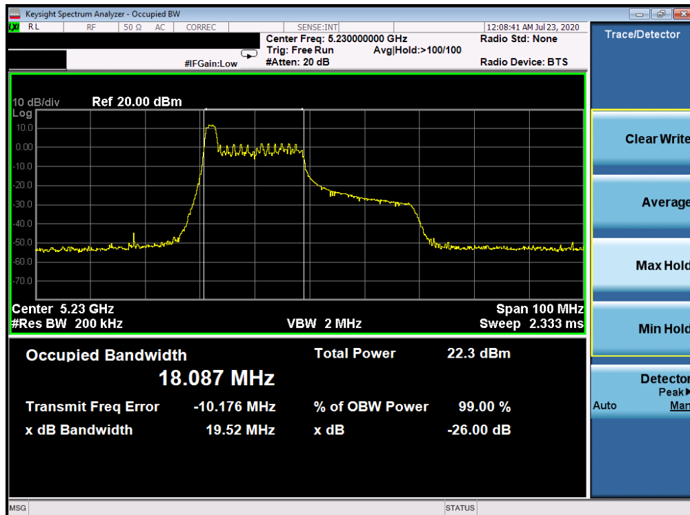
Plot 7-16. 26dB Bandwidth Plot ANT WF8 (40MHz BW 802.11ax Index 0 – RU26 (UNII Band 1) – Ch. 46)
