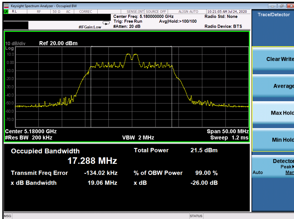
Plot 7-82. 26dB Bandwidth Plot ANT WF7a (20MHz BW 802.11ax Index 4 – RU26 (UNII Band 1) – Ch. 36)
