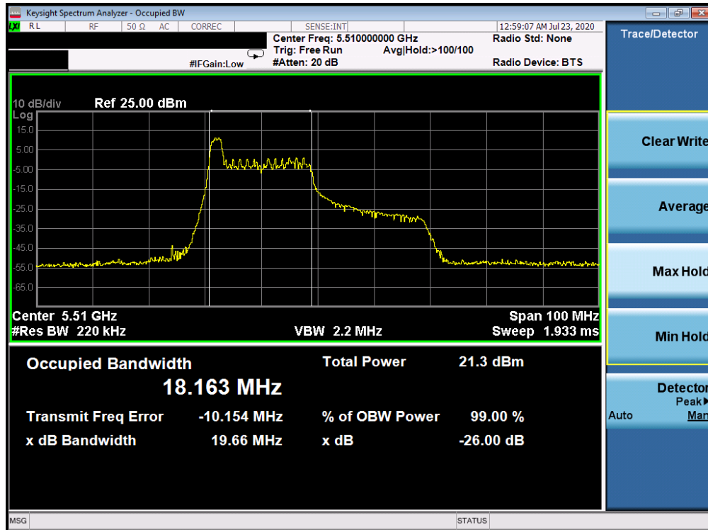
Plot 7-61. 26dB Bandwidth Plot ANT WF8 (40MHz BW 802.11ax Index 0 – RU26 (UNII Band 2C) – Ch. 102)
