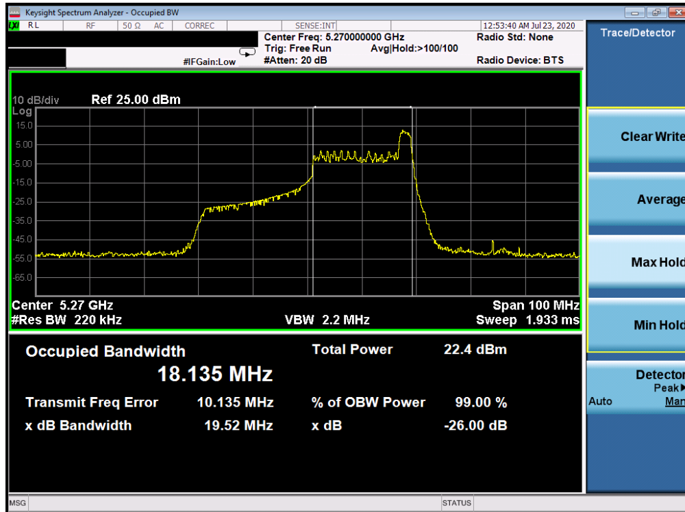
Plot 7-39. 26dB Bandwidth Plot ANT WF8 (40MHz BW 802.11ax Index 17 – RU26 (UNII Band 2A) – Ch. 54)
