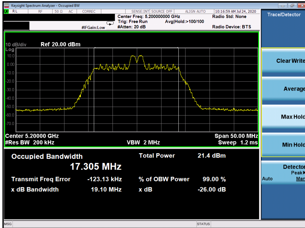
Plot 7-85. 26dB Bandwidth Plot ANT WF7a (20MHz BW 802.11ax Index 4 – RU26 (UNII Band 1) – Ch. 40)
