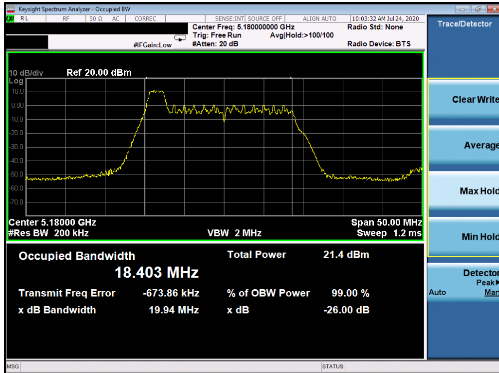
Plot 7-81. 26dB Bandwidth Plot ANT WF7a (20MHz BW 802.11ax Index 0 – RU26 (UNII Band 1) – Ch. 36)
