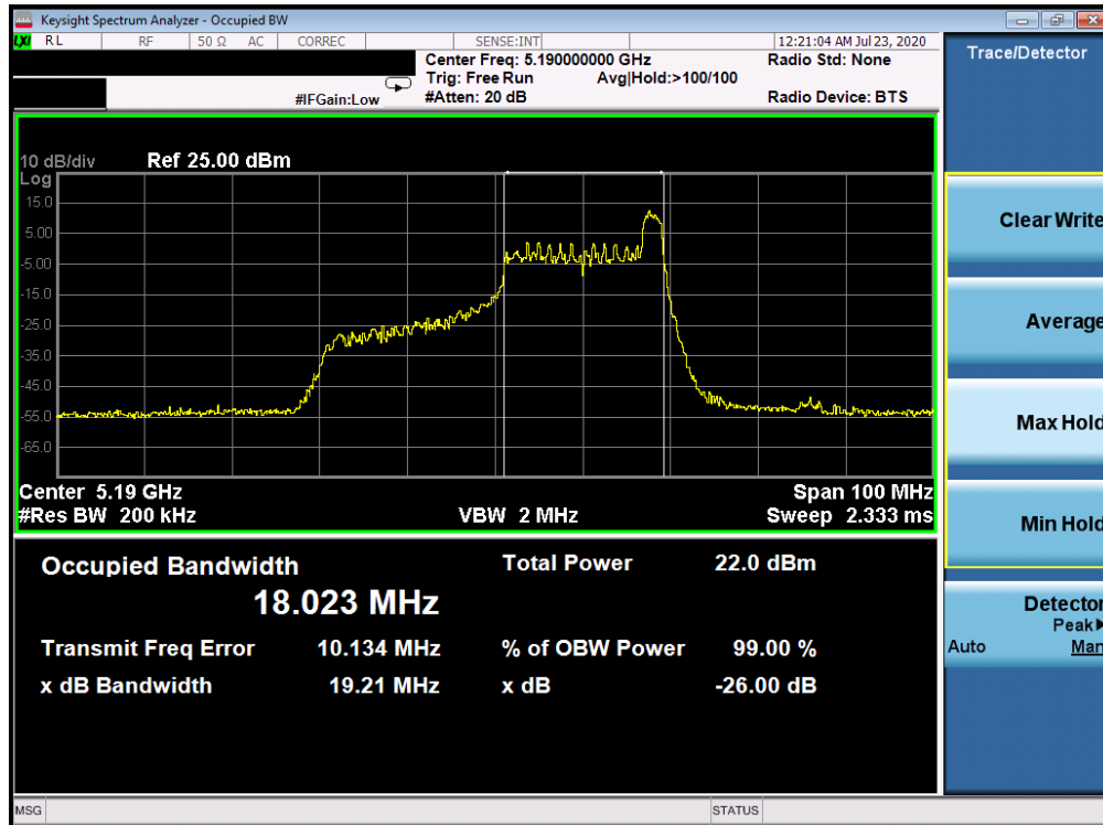
Plot 7-15. 26dB Bandwidth Plot ANT WF8 (40MHz BW 802.11ax Index 17 – RU26 (UNII Band 1) – Ch. 38)
