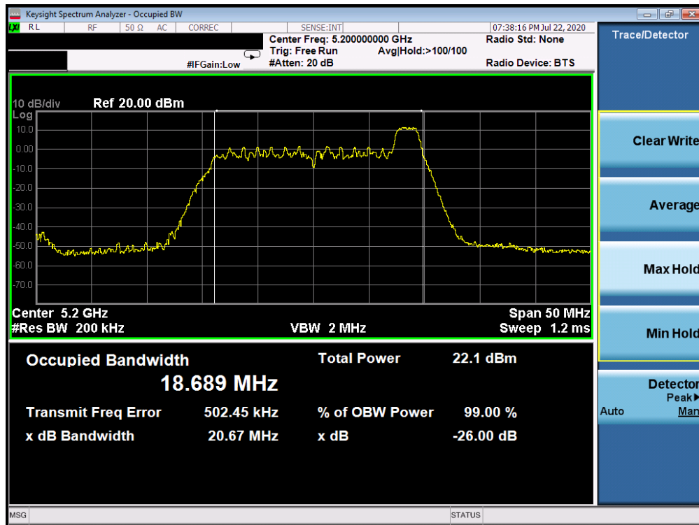
Plot 7-6. 26dB Bandwidth Plot ANT WF8 (20MHz BW 802.11ax Index 8– RU26 (UNII Band 1) – Ch. 40)
