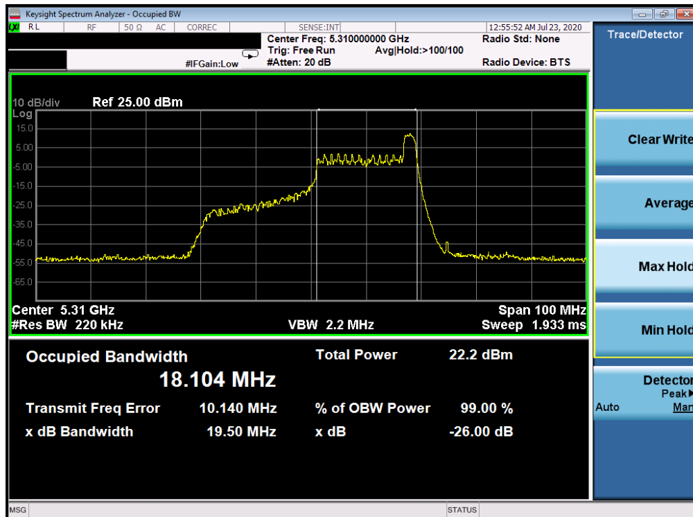
Plot 7-42. 26dB Bandwidth Plot ANT WF8 (40MHz BW 802.11ax Index 17 – RU26 (UNII Band 2A) – Ch. 62)
