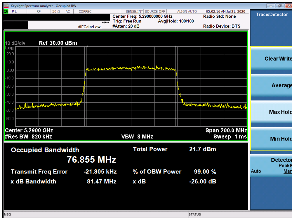
Plot 7-48. 26dB Bandwidth Plot ANT WF8 (80MHz BW 802.11ax - RU996 (UNII Band 2A) – Ch. 58)
