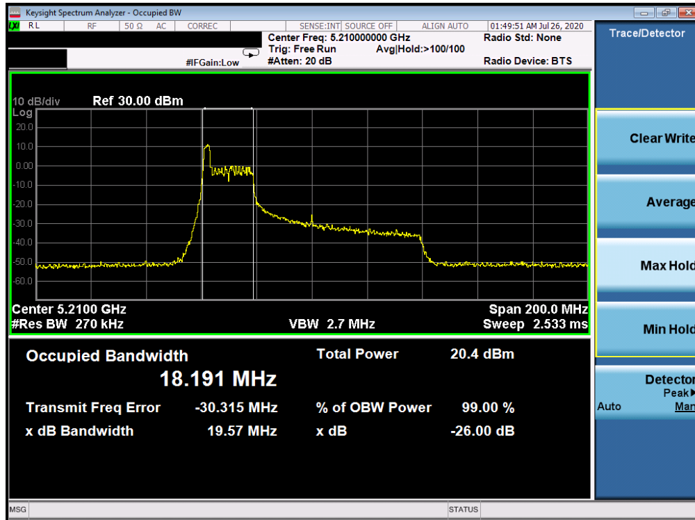
Plot 7-101. 26dB Bandwidth Plot ANT WF7a (80MHz BW 802.11ax Index 0 – RU26 (UNII Band 1) – Ch. 42)
