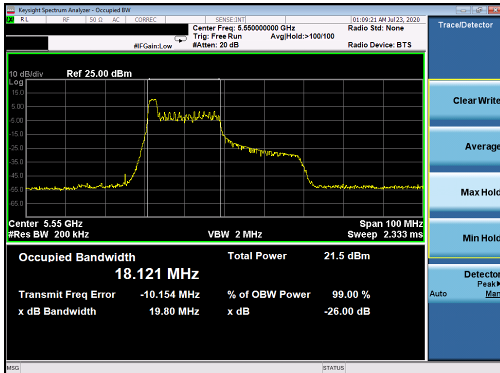
Plot 7-64. 26dB Bandwidth Plot ANT WF8 (40MHz BW 802.11ax Index 0 – RU26 (UNII Band 2C) – Ch. 110)
