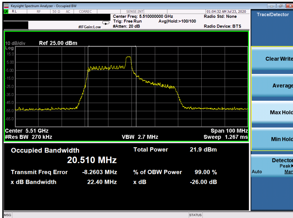
Plot 7-62. 26dB Bandwidth Plot ANT WF8 (40MHz BW 802.11ax Index 8 – RU26 (UNII Band 2C) – Ch. 102)
