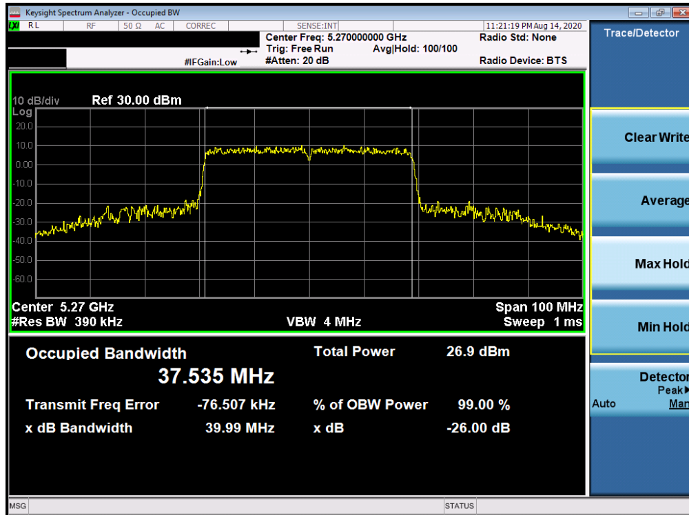
Plot 7-43. 26dB Bandwidth Plot ANT WF8 (40MHz BW 802.11ax – RU484 (UNII Band 2A) – Ch. 54)
