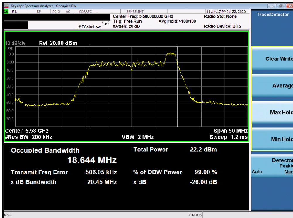
Plot 7-54. 26dB Bandwidth Plot ANT WF8 (20MHz BW 802.11ax Index 8– RU26 (UNII Band 2C) – Ch. 116)
