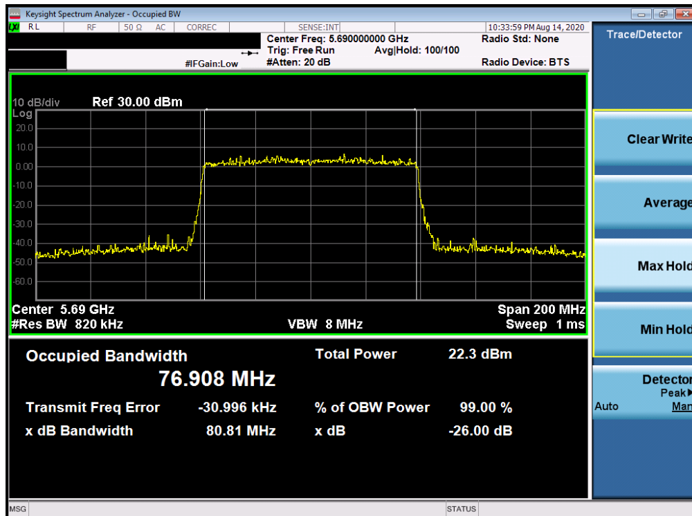
Plot 7-80. 26dB Bandwidth Plot ANT WF8 (80MHz BW 802.11ax – RU996 (UNII Band 2C) – Ch. 138)
