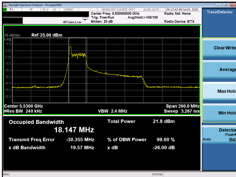
Plot 7-73. 26dB Bandwidth Plot ANT WF8 (80MHz BW 802.11ax Index 0 – RU26 (UNII Band 2C) – Ch. 106)
