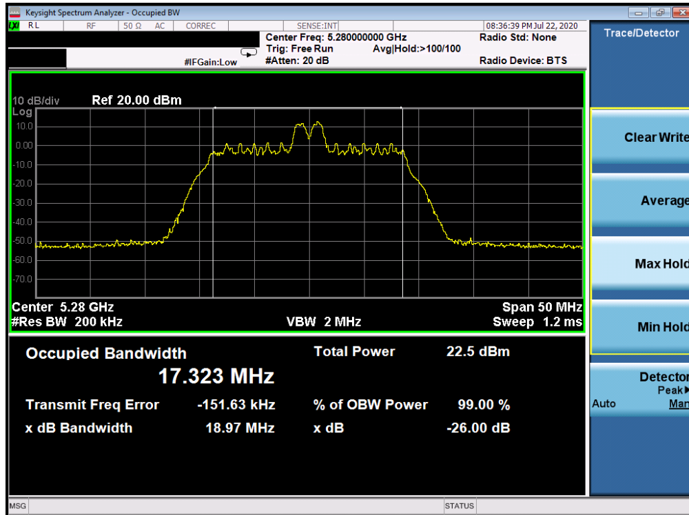
Plot 7-29. 26dB Bandwidth Plot ANT WF8 (20MHz BW 802.11ax Index 4 – RU26 (UNII Band 2A) – Ch. 56)
