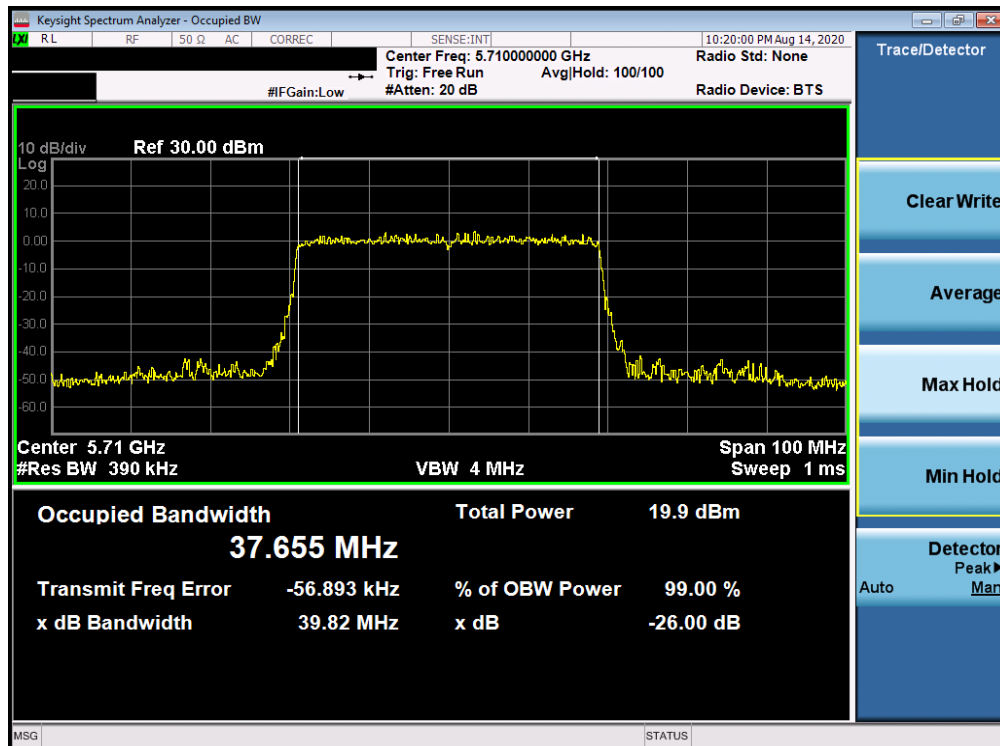
Plot 7-72. 26dB Bandwidth Plot ANT WF8 (40MHz BW 802.11ax – RU484 (UNII Band 2C) – Ch. 142)
