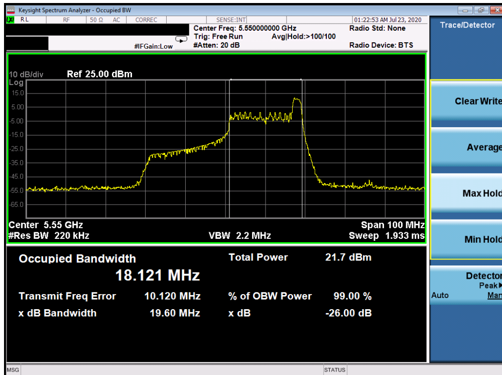
Plot 7-66. 26dB Bandwidth Plot ANT WF8 (40MHz BW 802.11ax Index 17 – RU26 (UNII Band 2C) – Ch. 110)
