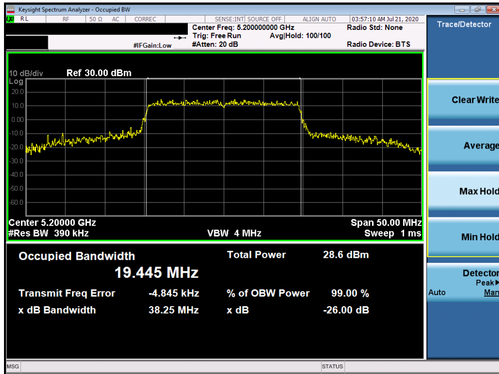
Plot 7-11. 26dB Bandwidth Plot ANT WF8 (20MHz BW 802.11ax- RU242 (UNII Band 1) – Ch. 40)
