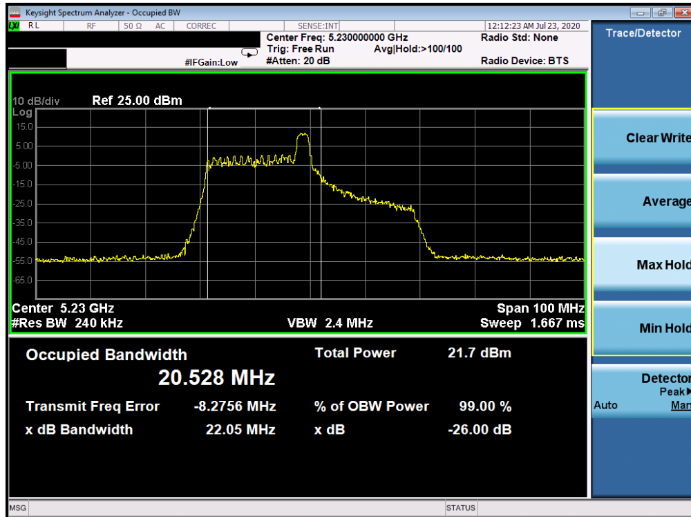
Plot 7-17. 26dB Bandwidth Plot ANT WF8 (40MHz BW 802.11ax Index 8 – RU26 (UNII Band 1) – Ch. 46)
