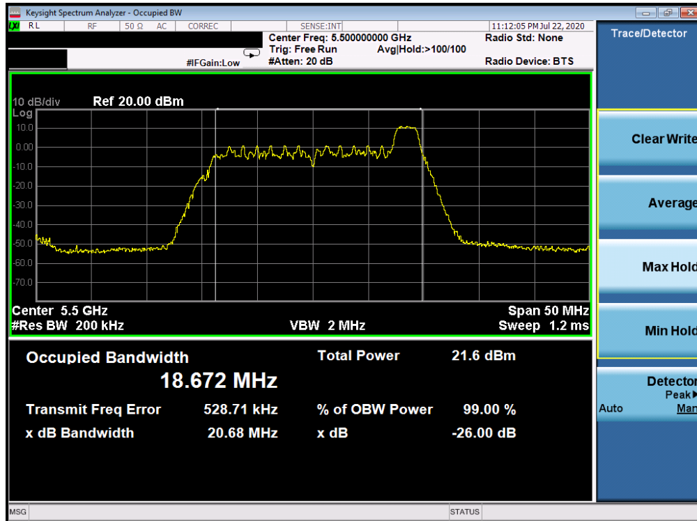
Plot 7-51. 26dB Bandwidth Plot ANT WF8 (20MHz BW 802.11ax Index 8 – RU26 (UNII Band 2C) – Ch. 100)
