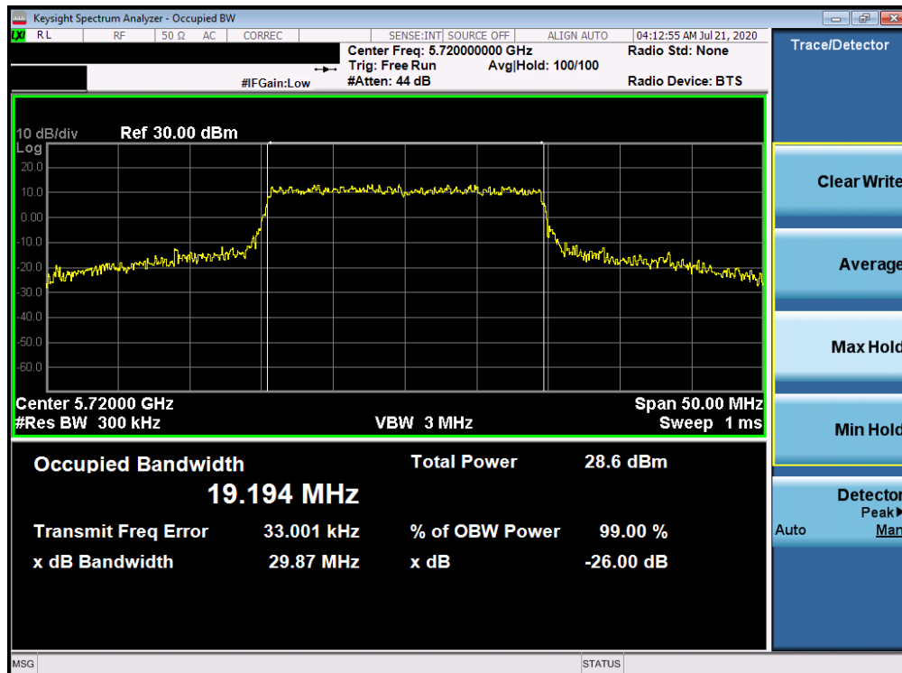
Plot 7-60. 26dB Bandwidth Plot ANT WF8 (20MHz BW 802.11ax- RU242 (UNII Band 2C) - Ch. 144)
