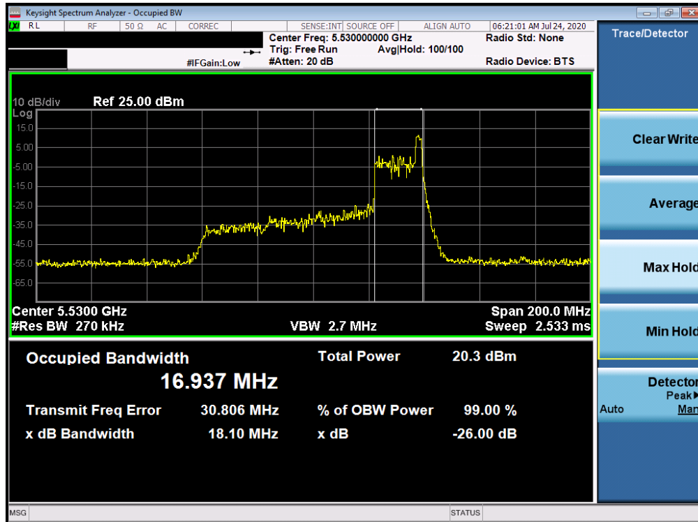
Plot 7-75. 26dB Bandwidth Plot ANT WF8 (80MHz BW 802.11ax Index 36 – RU26 (UNII Band 2C) – Ch. 106)
