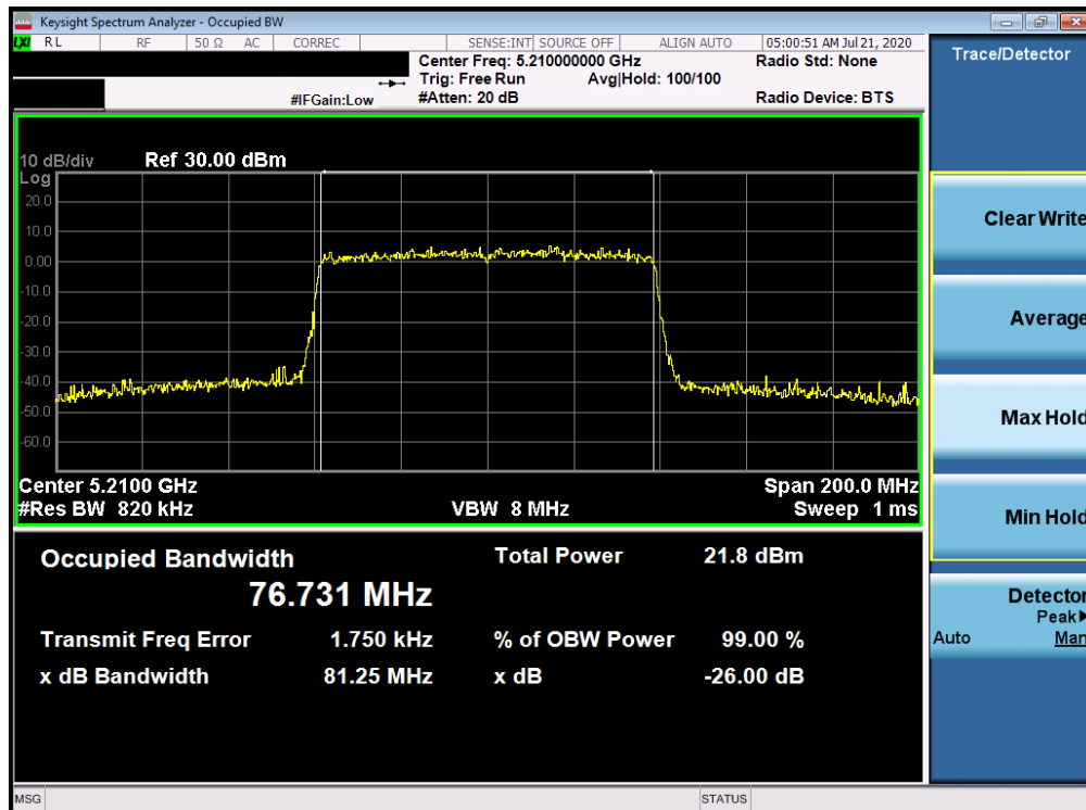
Plot 7-24. 26dB Bandwidth Plot ANT WF8 (80MHz BW 802.11ax – RU996 (UNII Band 1) – Ch. 42)
