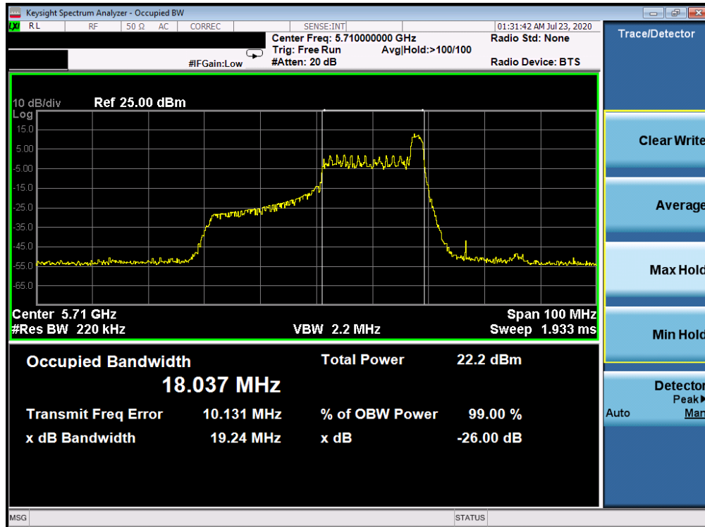
Plot 7-69. 26dB Bandwidth Plot ANT WF8 (40MHz BW 802.11ax Index 17 – RU26 (UNII Band 2C) – Ch. 142)
