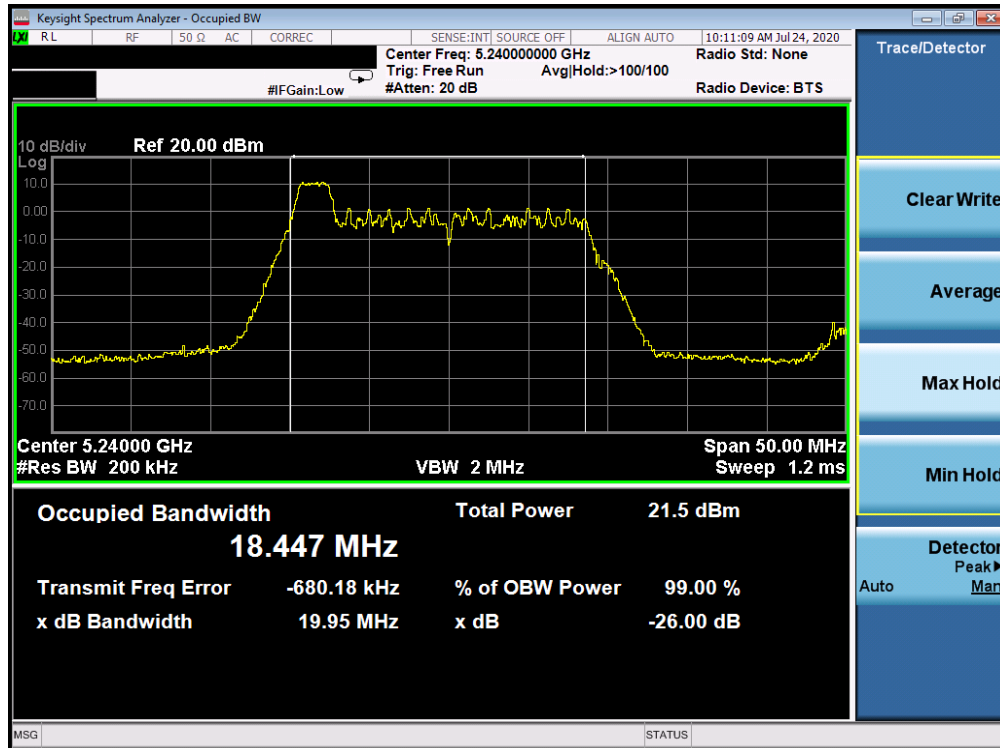
Plot 7-87. 26dB Bandwidth Plot ANT WF7a (20MHz BW 802.11ax Index 0 – RU26 (UNII Band 1) – Ch. 48)
