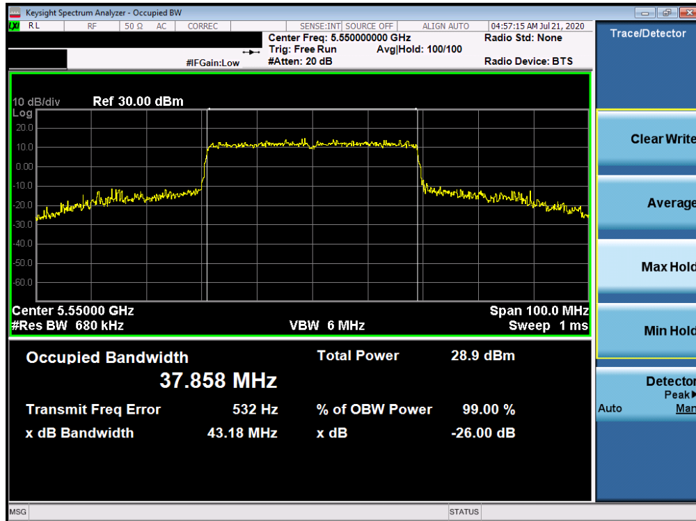
Plot 7-71. 26dB Bandwidth Plot ANT WF8 (40MHz BW 802.11ax – RU484 (UNII Band 2C) – Ch. 110)
