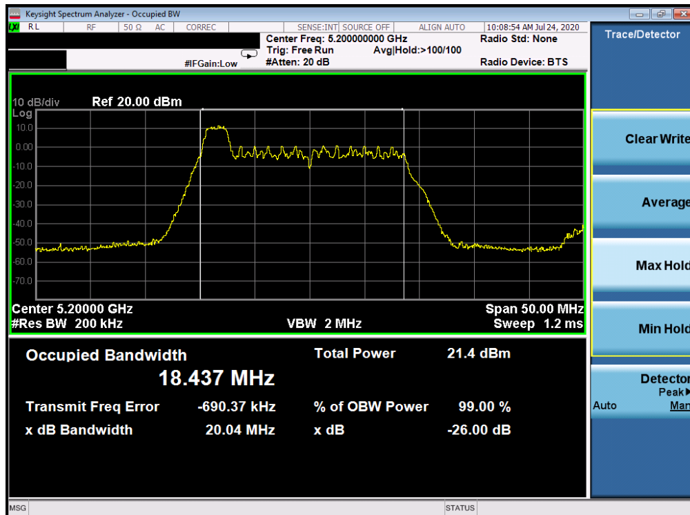
Plot 7-84. 26dB Bandwidth Plot ANT WF7a (20MHz BW 802.11ax Index 0 – RU26 (UNII Band 1) – Ch. 40)
