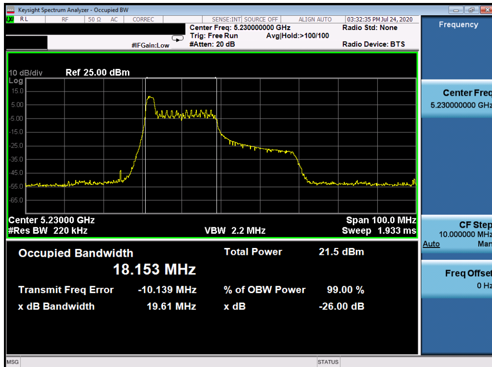
Plot 7-96. 26dB Bandwidth Plot ANT WF7a (40MHz BW 802.11ax Index 0 – RU26 (UNII Band 1) – Ch. 46)
