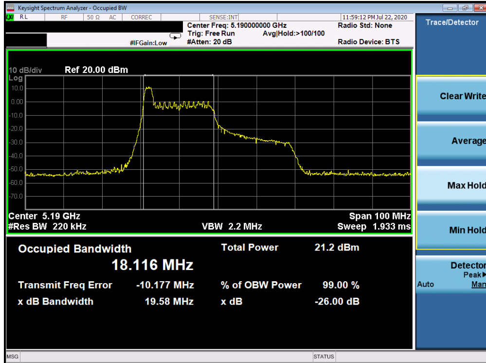
Plot 7-13. 26dB Bandwidth Plot ANT WF8 (40MHz BW 802.11ax Index 0 – RU26 (UNII Band 1) – Ch. 38)
