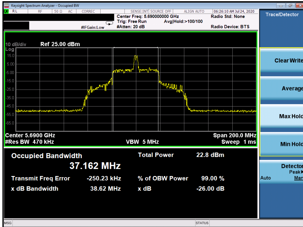
Plot 7-77. 26dB Bandwidth Plot ANT WF8 (80MHz BW 802.11ax Index 18 – RU26 (UNII Band 2C) – Ch. 138)
