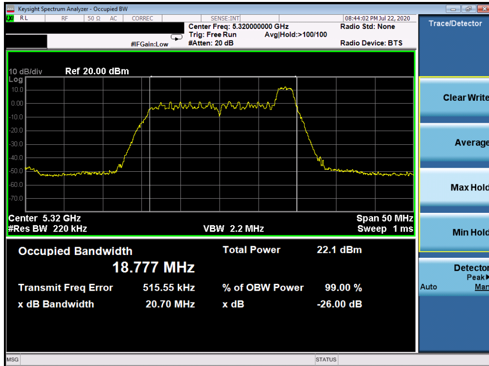
Plot 7-33. 26dB Bandwidth Plot ANT WF8 (20MHz BW 802.11ax Index 8 – RU26 (UNII Band 2A) – Ch. 64)
