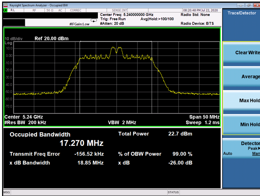
Plot 7-8. 26dB Bandwidth Plot ANT WF8 (20MHz BW 802.11ax Index 4 – RU26 (UNII Band 1) – Ch. 48)
