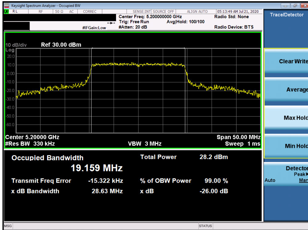
Plot 7-91. 26dB Bandwidth Plot ANT WF7a (20MHz BW 802.11ax- RU242 (UNII Band 1) – Ch. 40)
