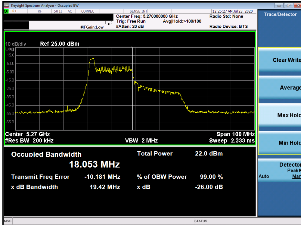
Plot 7-37. 26dB Bandwidth Plot ANT WF8 (40MHz BW 802.11ax Index 0 – RU26 (UNII Band 2A) – Ch. 54)
