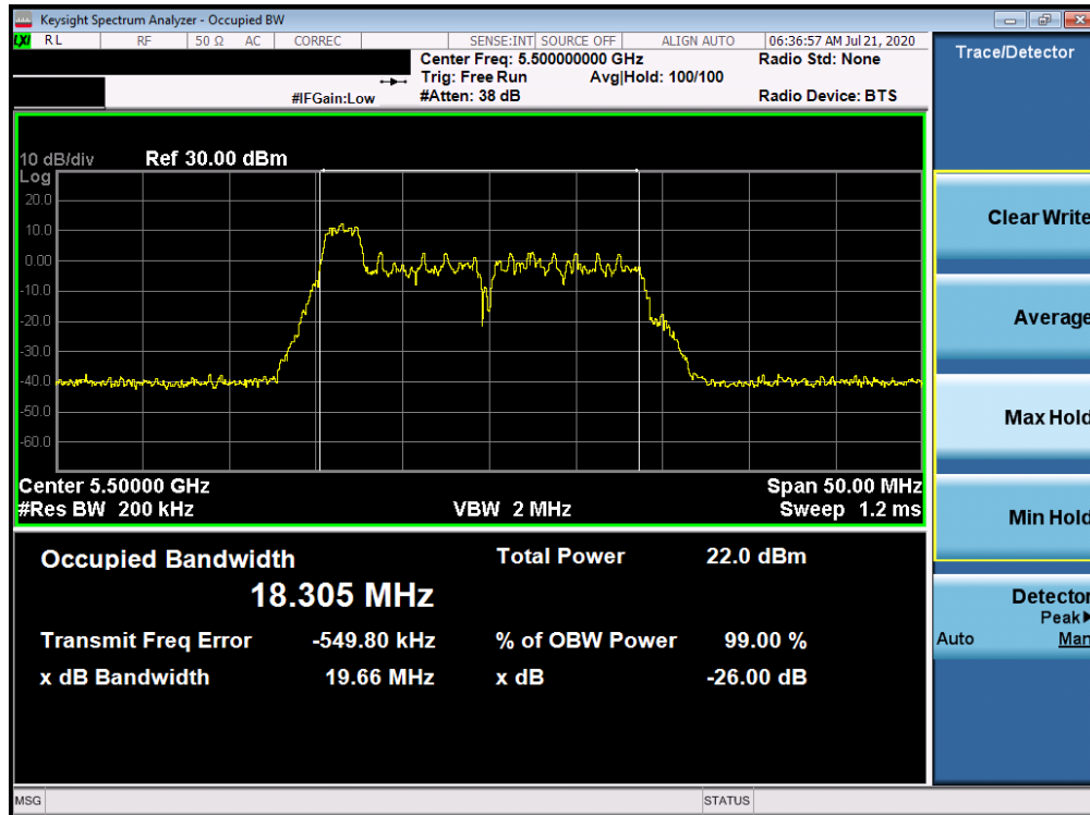
Plot 7-49. 26dB Bandwidth Plot ANT WF8 (20MHz BW 802.11ax Index 0 – RU26 (UNII Band 2C) – Ch. 100)
