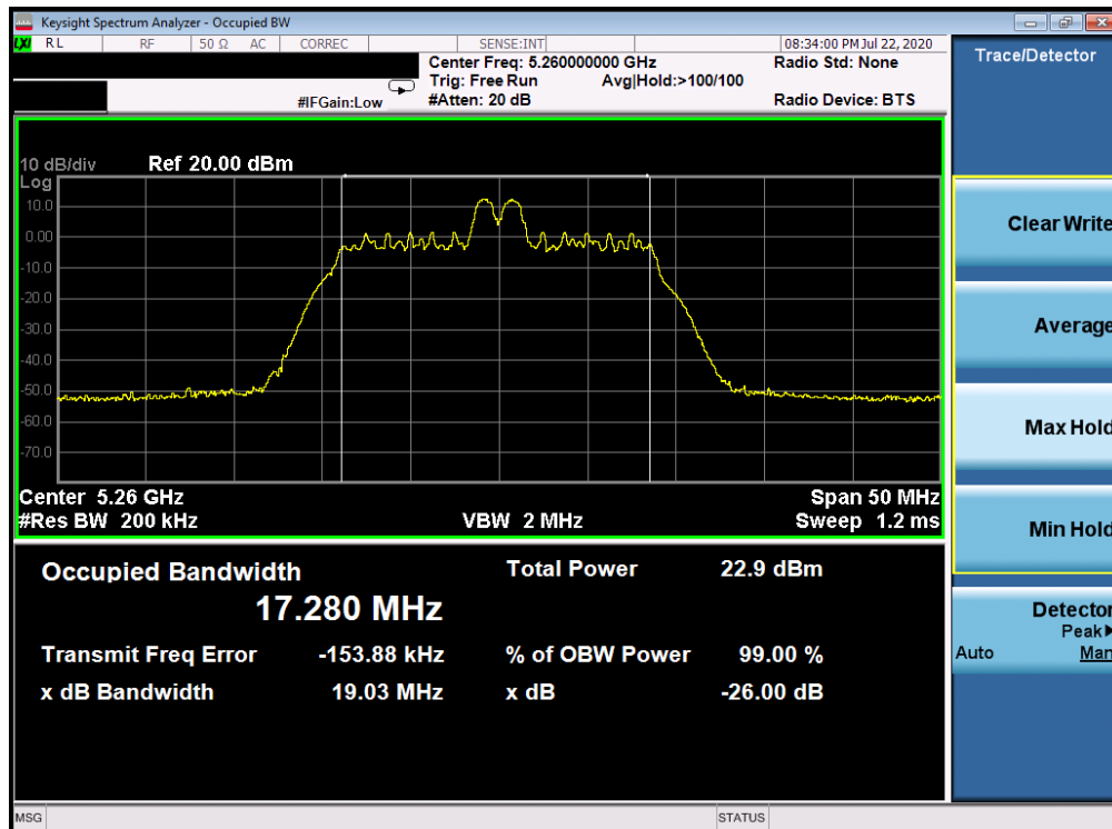
Plot 7-26. 26dB Bandwidth Plot ANT WF8 (20MHz BW 802.11ax Index 4 – RU26 (UNII Band 2A) – Ch. 52)
