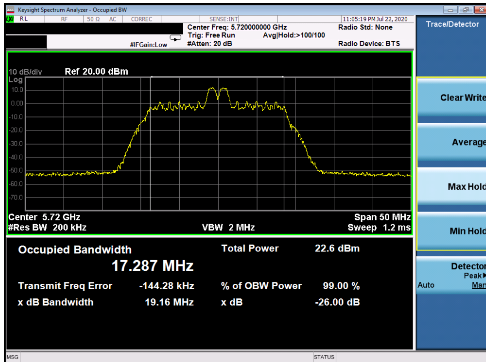
Plot 7-56. 26dB Bandwidth Plot ANT WF8 (20MHz BW 802.11ax Index 4 – RU26 (UNII Band 2C) – Ch. 144)
