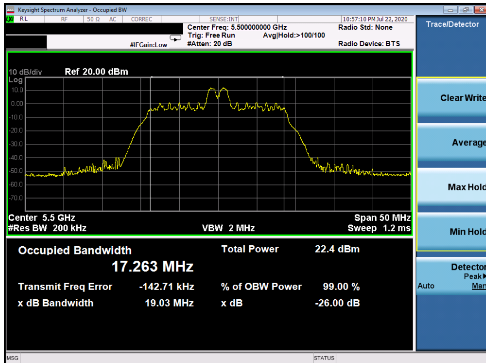
Plot 7-50. 26dB Bandwidth Plot ANT WF8 (20MHz BW 802.11ax Index 4 – RU26 (UNII Band 2C) – Ch. 100)
