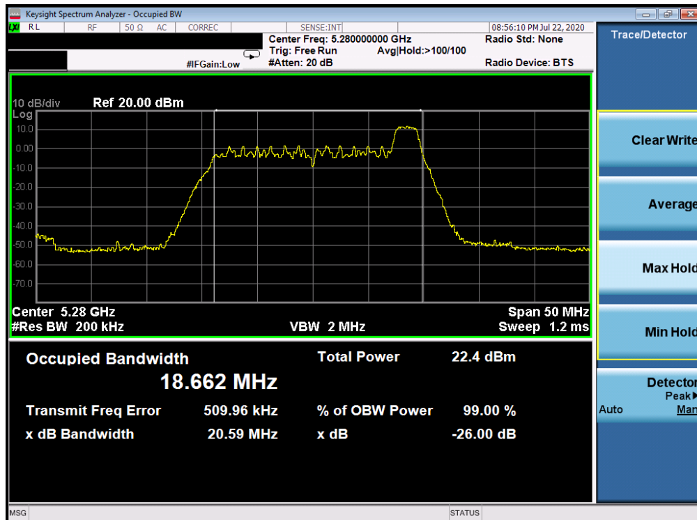
Plot 7-30. 26dB Bandwidth Plot ANT WF8 (20MHz BW 802.11ax Index 8– RU26 (UNII Band 2A) – Ch. 56)
