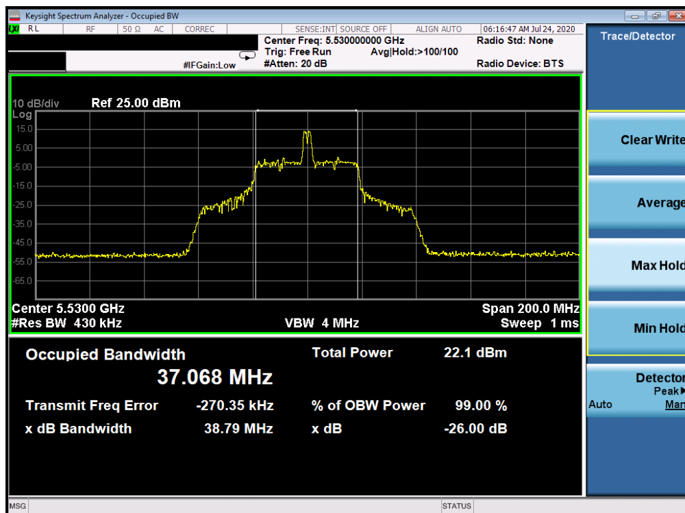
Plot 7-74. 26dB Bandwidth Plot ANT WF8 (80MHz BW 802.11ax Index 18 – RU26 (UNII Band 2C) – Ch. 106)
