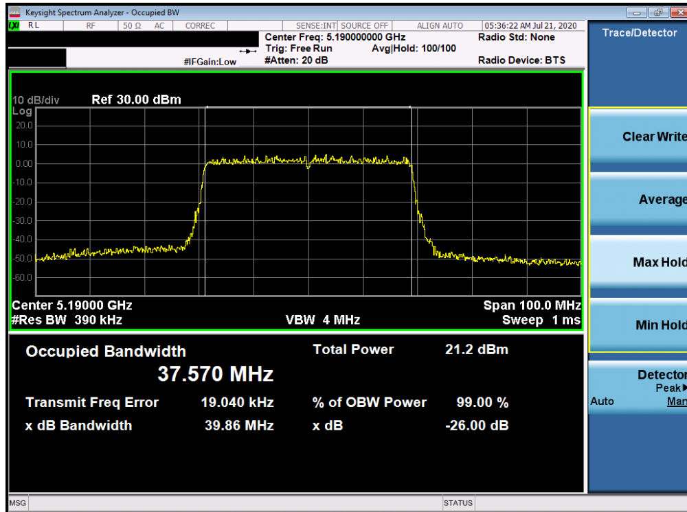
Plot 7-99. 26dB Bandwidth Plot ANT WF7a (40MHz BW 802.11ax – RU484 (UNII Band 1) – Ch. 38)
