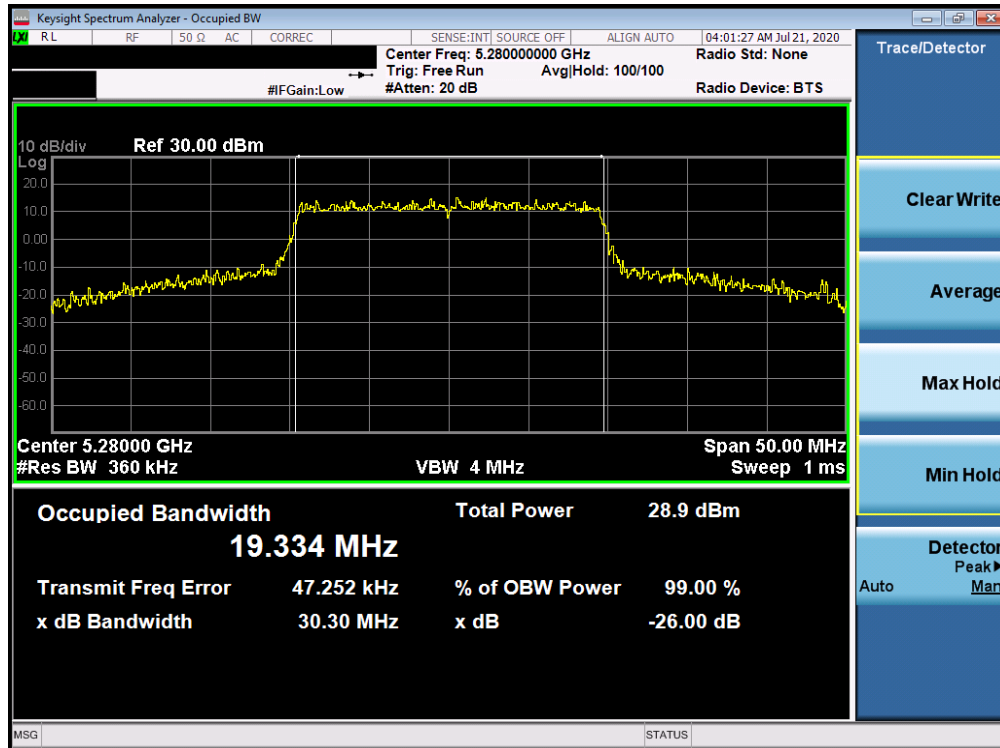
Plot 7-35. 26dB Bandwidth Plot ANT WF8 (20MHz BW 802.11ax– RU242 (UNII Band 2A) – Ch. 56)
