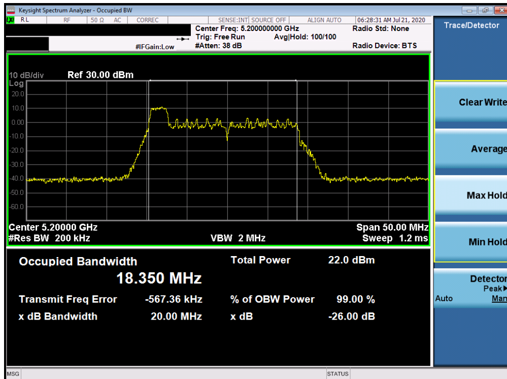
Plot 7-4. 26dB Bandwidth Plot ANT WF8 (20MHz BW 802.11ax Index 0 – RU26 (UNII Band 1) – Ch. 40)
