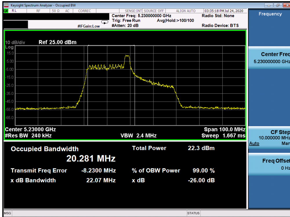
Plot 7-97. 26dB Bandwidth Plot ANT WF7a (40MHz BW 802.11ax Index 8 – RU26 (UNII Band 1) – Ch. 46)
