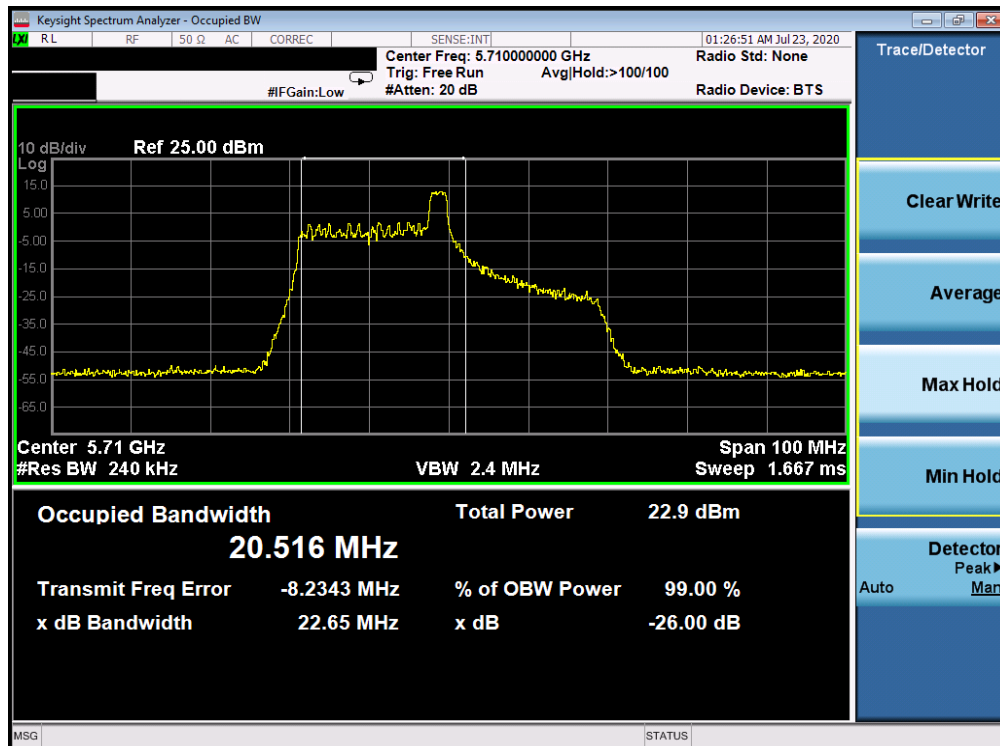
Plot 7-68. 26dB Bandwidth Plot ANT WF8 (40MHz BW 802.11ax Index 8 – RU26 (UNII Band 2C) – Ch. 142)
