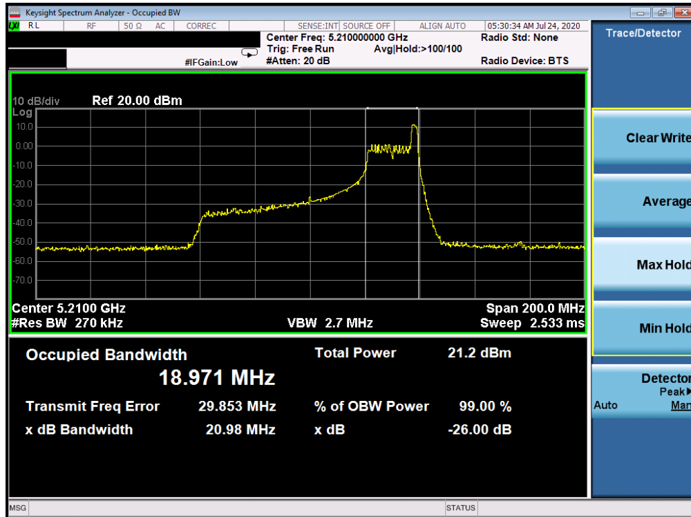
Plot 7-23. 26dB Bandwidth Plot ANT WF8 (80MHz BW 802.11ax Index 36 – RU26 (UNII Band 1) – Ch. 42)
