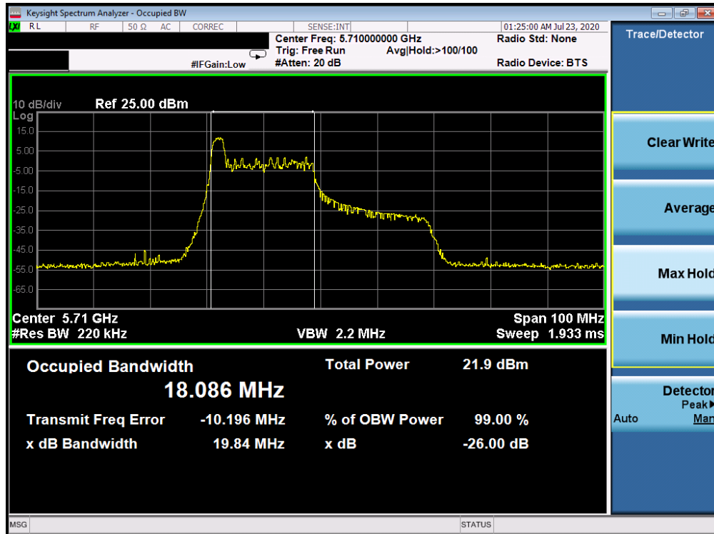
Plot 7-67. 26dB Bandwidth Plot ANT WF8 (40MHz BW 802.11ax Index 0 – RU26 (UNII Band 2C) – Ch. 142)
