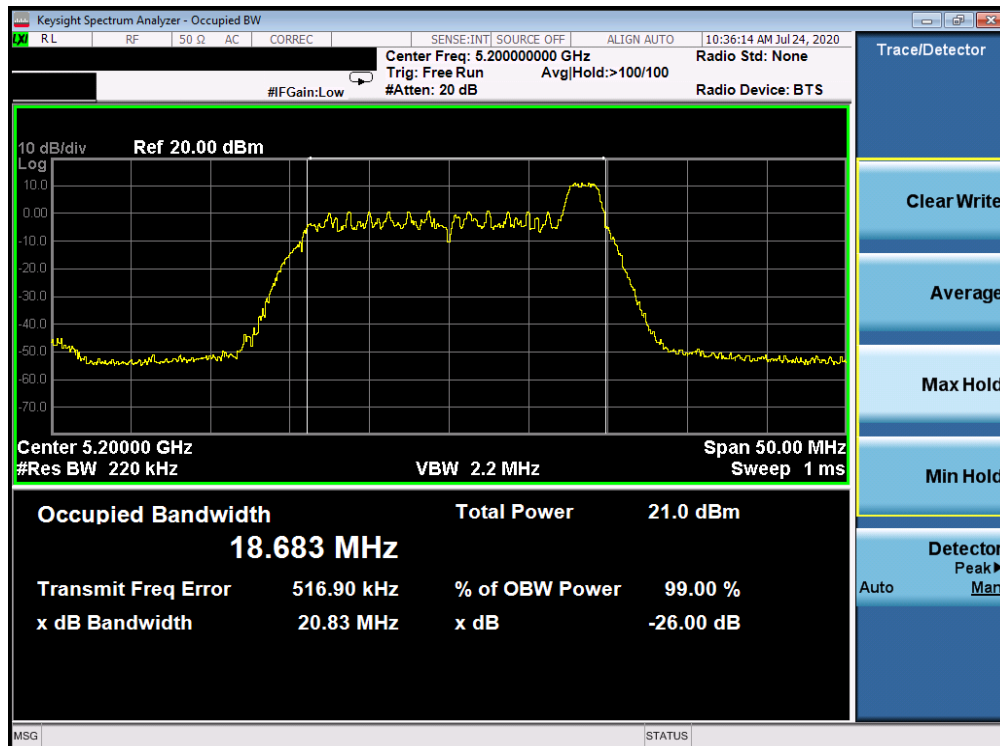
Plot 7-86. 26dB Bandwidth Plot ANT WF7a (20MHz BW 802.11ax Index 8– RU26 (UNII Band 1) – Ch. 40)
