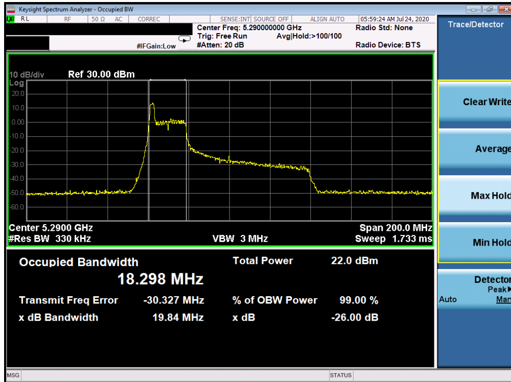
Plot 7-45. 26dB Bandwidth Plot ANT WF8 (80MHz BW 802.11ax Index 0 – RU26 (UNII Band 2A) – Ch. 58)
