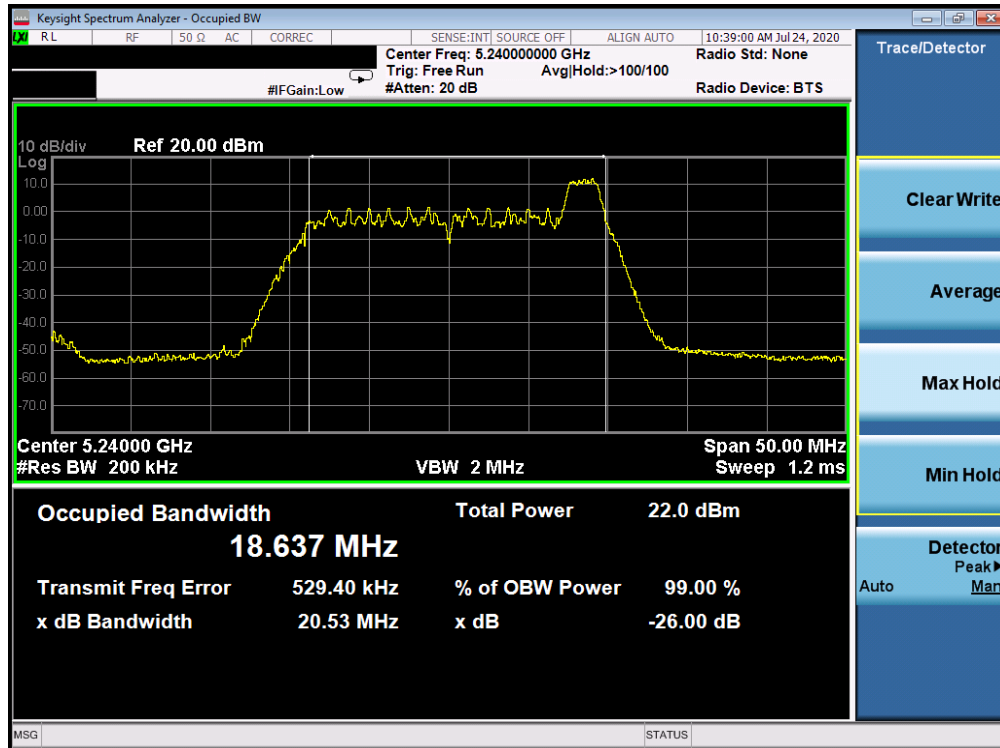
Plot 7-89. 26dB Bandwidth Plot ANT WF7a (20MHz BW 802.11ax Index 8 – RU26 (UNII Band 1) – Ch. 48)
