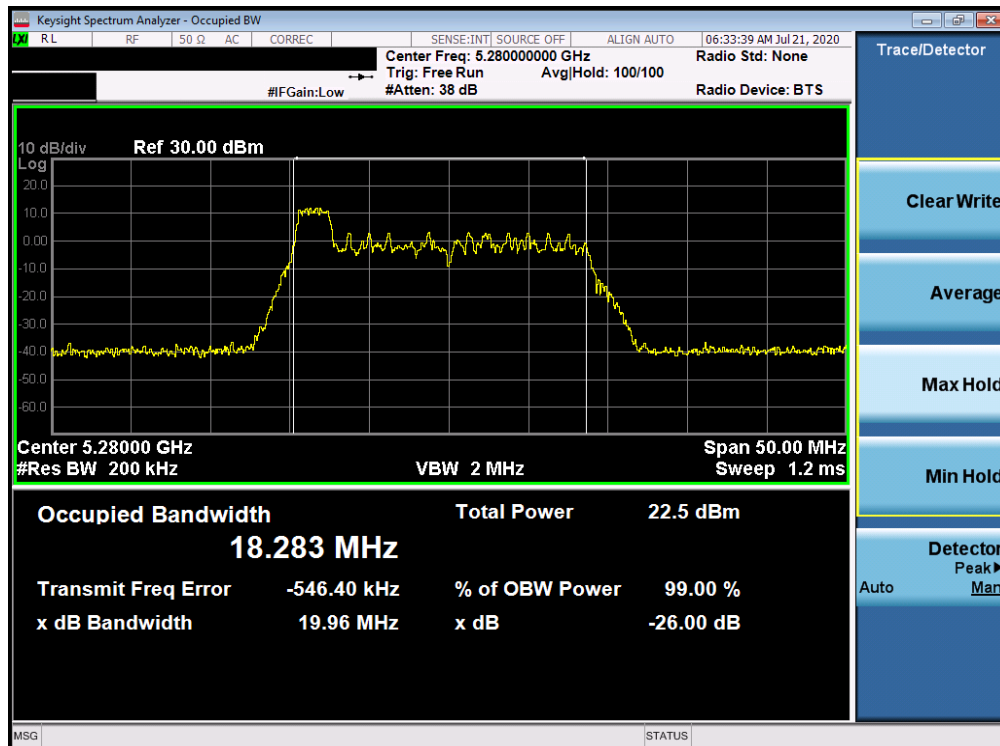
Plot 7-28. 26dB Bandwidth Plot ANT WF8 (20MHz BW 802.11ax Index 0 – RU26 (UNII Band 2A) – Ch. 56)
