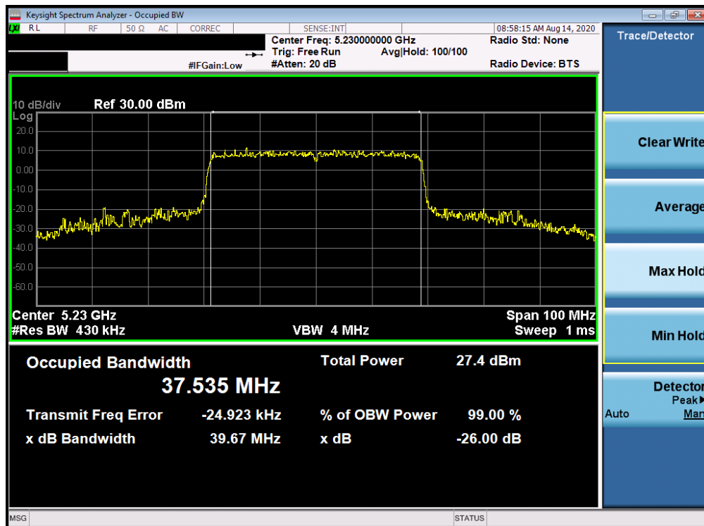
Plot 7-100. 26dB Bandwidth Plot ANT WF7a (40MHz BW 802.11ax – RU484 (UNII Band 1) – Ch. 46)
