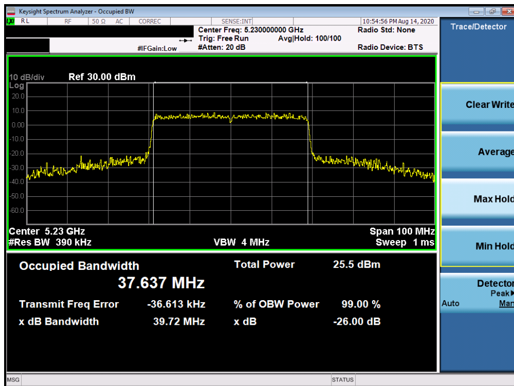
Plot 7-20. 26dB Bandwidth Plot ANT WF8 (40MHz BW 802.11ax – RU484 (UNII Band 1) – Ch. 46)
