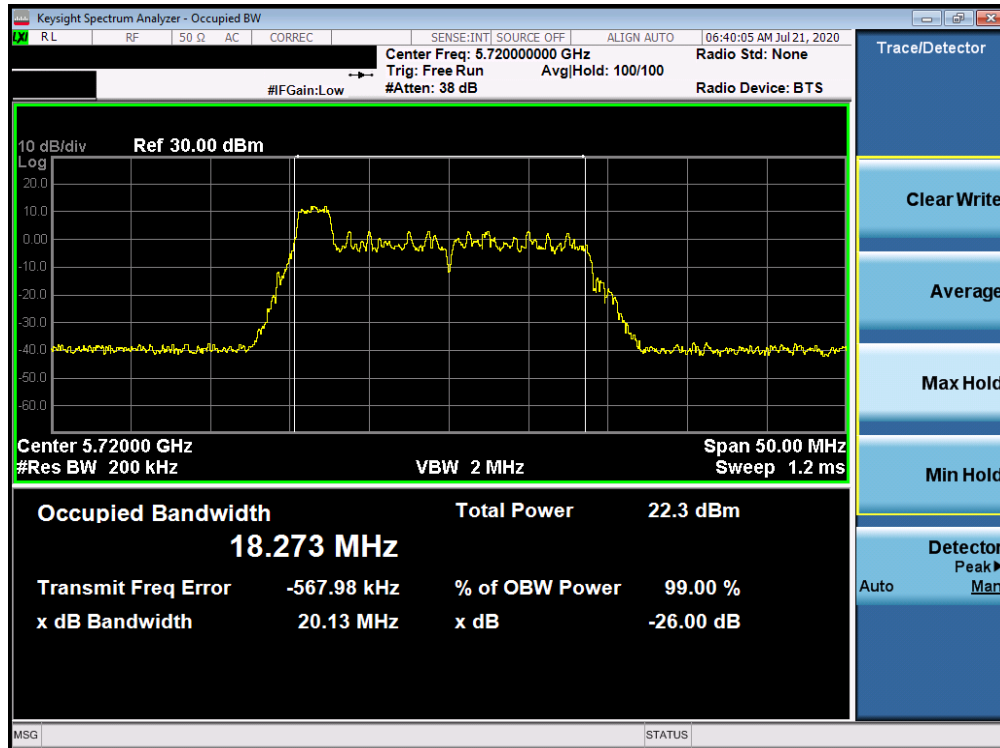
Plot 7-55. 26dB Bandwidth Plot ANT WF8 (20MHz BW 802.11ax Index 0 – RU26 (UNII Band 2C) – Ch. 144)
