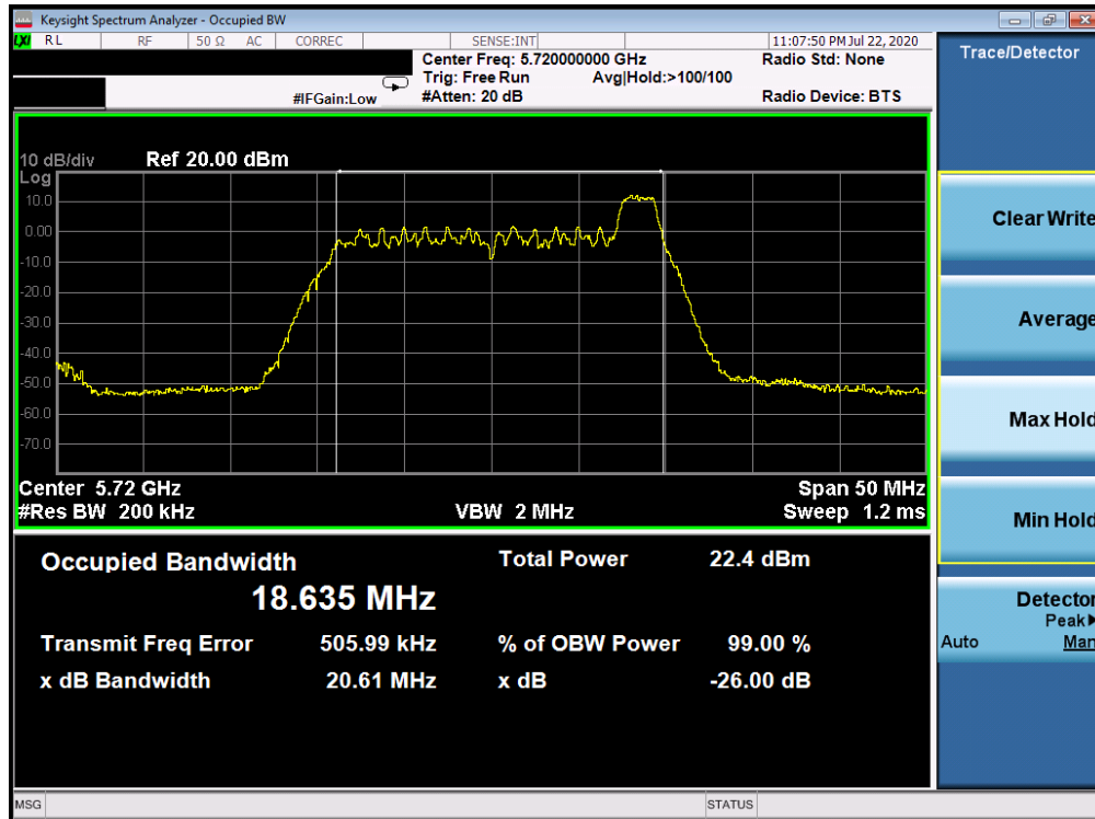
Plot 7-57. 26dB Bandwidth Plot ANT WF8 (20MHz BW 802.11ax Index 8 – RU26 (UNII Band 2C) – Ch. 144)
