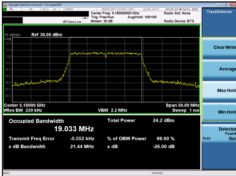
Plot 7-10. 26dB Bandwidth Plot ANT WF8 (20MHz BW 802.11ax– RU242 (UNII Band 1) – Ch. 36)
