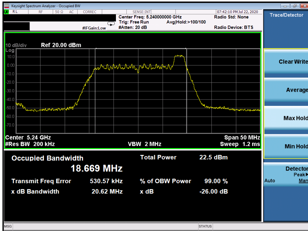
Plot 7-9. 26dB Bandwidth Plot ANT WF8 (20MHz BW 802.11ax Index 8 – RU26 (UNII Band 1) – Ch. 48)
