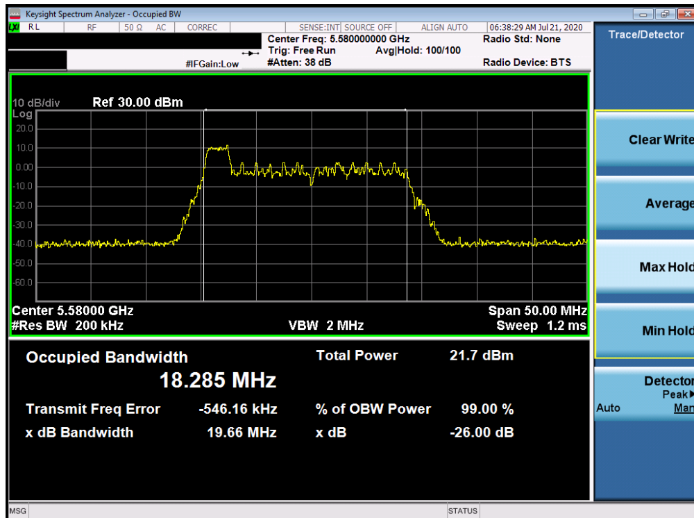
Plot 7-52. 26dB Bandwidth Plot ANT WF8 (20MHz BW 802.11ax Index 0 – RU26 (UNII Band 2C) – Ch. 116)
