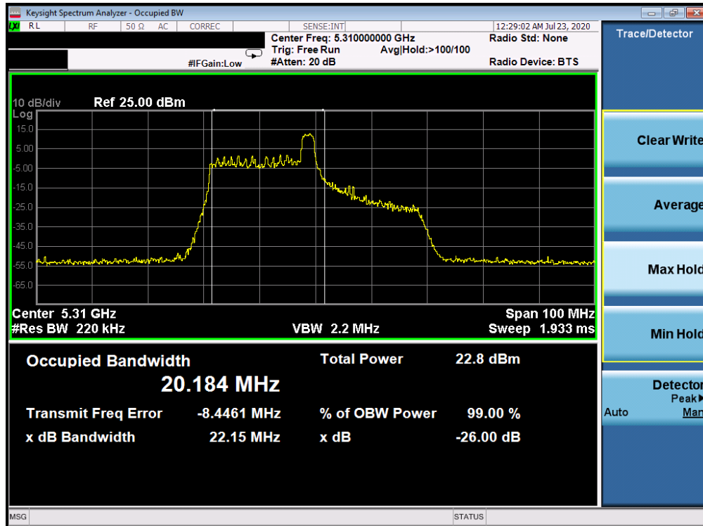
Plot 7-41. 26dB Bandwidth Plot ANT WF8 (40MHz BW 802.11ax Index 8 – RU26 (UNII Band 2A) – Ch. 62)
