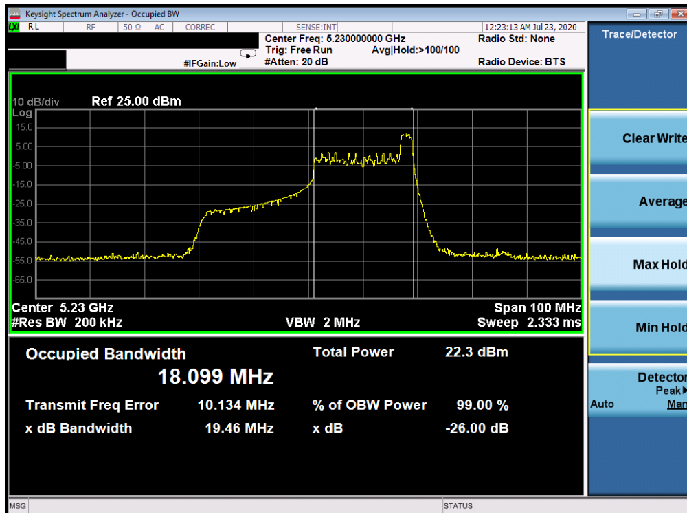
Plot 7-18. 26dB Bandwidth Plot ANT WF8 (40MHz BW 802.11ax Index 17 – RU26 (UNII Band 1) – Ch. 46)
