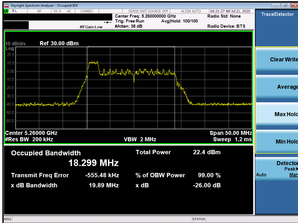
Plot 7-25. 26dB Bandwidth Plot ANT WF8 (20MHz BW 802.11ax Index 0 – RU26 (UNII Band 2A) – Ch. 52)
