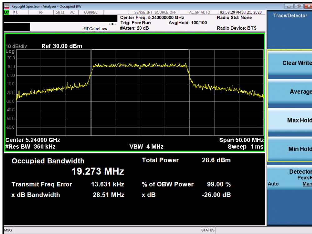
Plot 7-12. 26dB Bandwidth Plot ANT WF8 (20MHz BW 802.11ax- RU242 (UNII Band 1) – Ch. 48)
