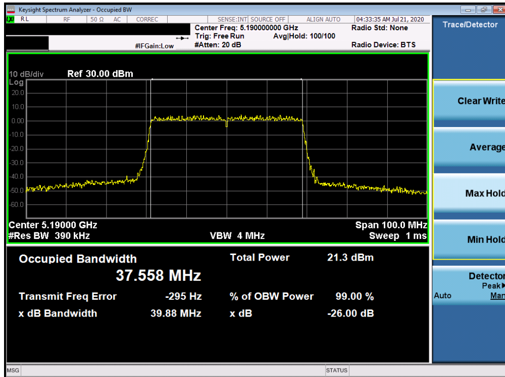
Plot 7-19. 26dB Bandwidth Plot ANT WF8 (40MHz BW 802.11ax – RU484 (UNII Band 1) – Ch. 38)
