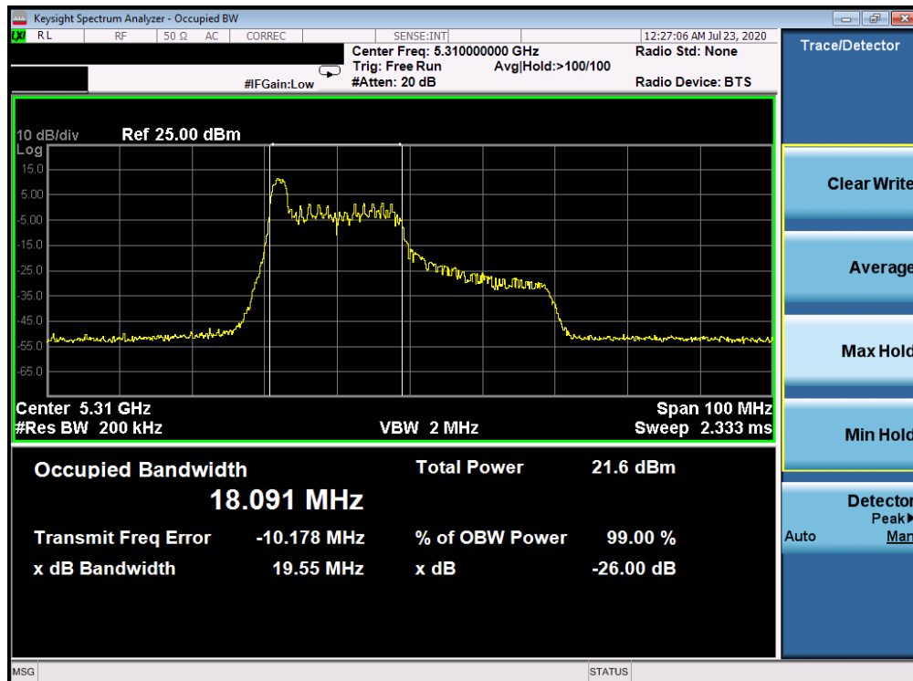
Plot 7-40. 26dB Bandwidth Plot ANT WF8 (40MHz BW 802.11ax Index 0 – RU26 (UNII Band 2A) – Ch. 62)
