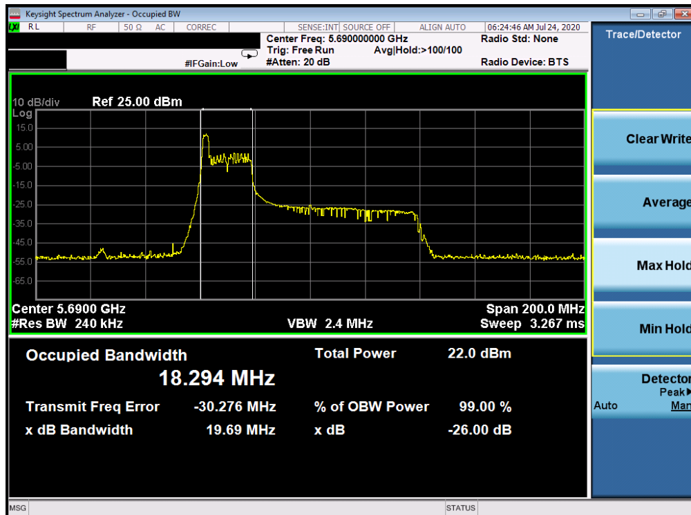
Plot 7-76. 26dB Bandwidth Plot ANT WF8 (80MHz BW 802.11ax Index 0 – RU26 (UNII Band 2C) – Ch. 138)
