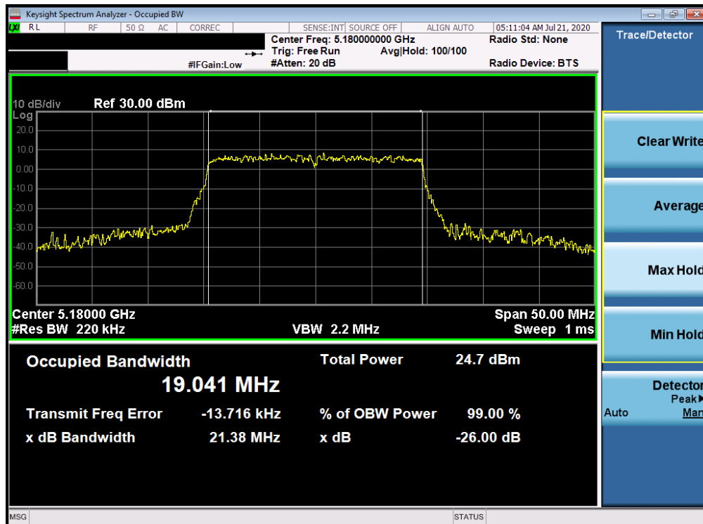
Plot 7-90. 26dB Bandwidth Plot ANT WF7a (20MHz BW 802.11ax– RU242 (UNII Band 1) – Ch. 36)
