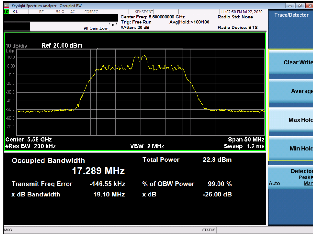
Plot 7-53. 26dB Bandwidth Plot ANT WF8 (20MHz BW 802.11ax Index 4 – RU26 (UNII Band 2C) – Ch. 116)
