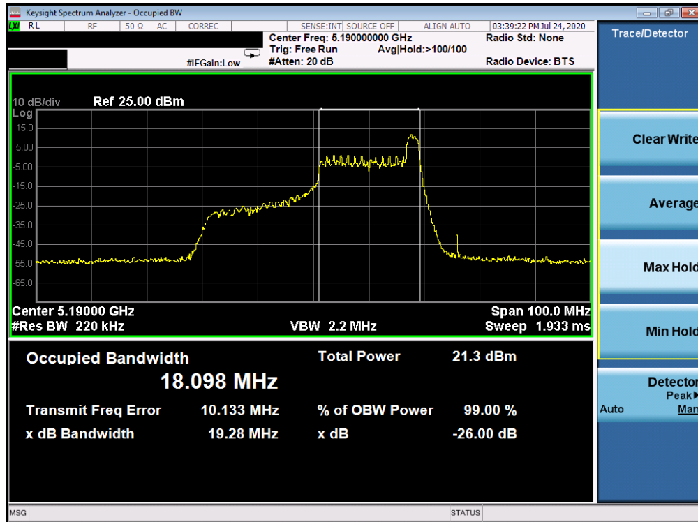
Plot 7-95. 26dB Bandwidth Plot ANT WF7a (40MHz BW 802.11ax Index 17 – RU26 (UNII Band 1) – Ch. 38)
