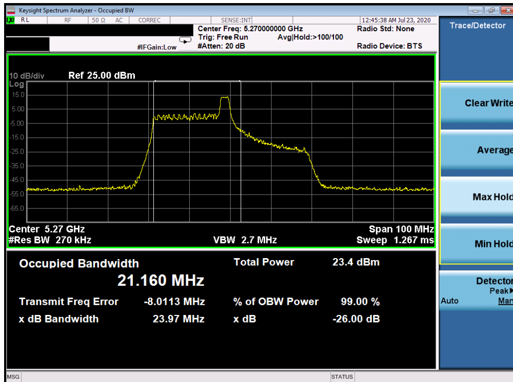
Plot 7-38. 26dB Bandwidth Plot ANT WF8 (40MHz BW 802.11ax Index 8 – RU26 (UNII Band 2A) – Ch. 54)
