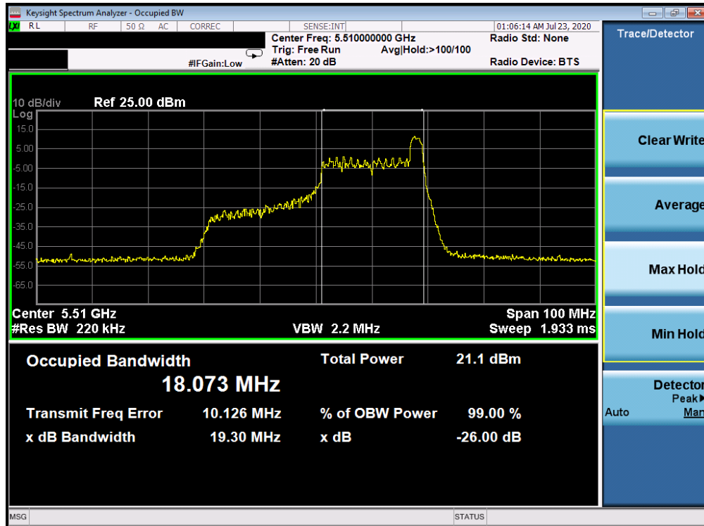
Plot 7-63. 26dB Bandwidth Plot ANT WF8 (40MHz BW 802.11ax Index 17 – RU26 (UNII Band 2C) – Ch. 102)
