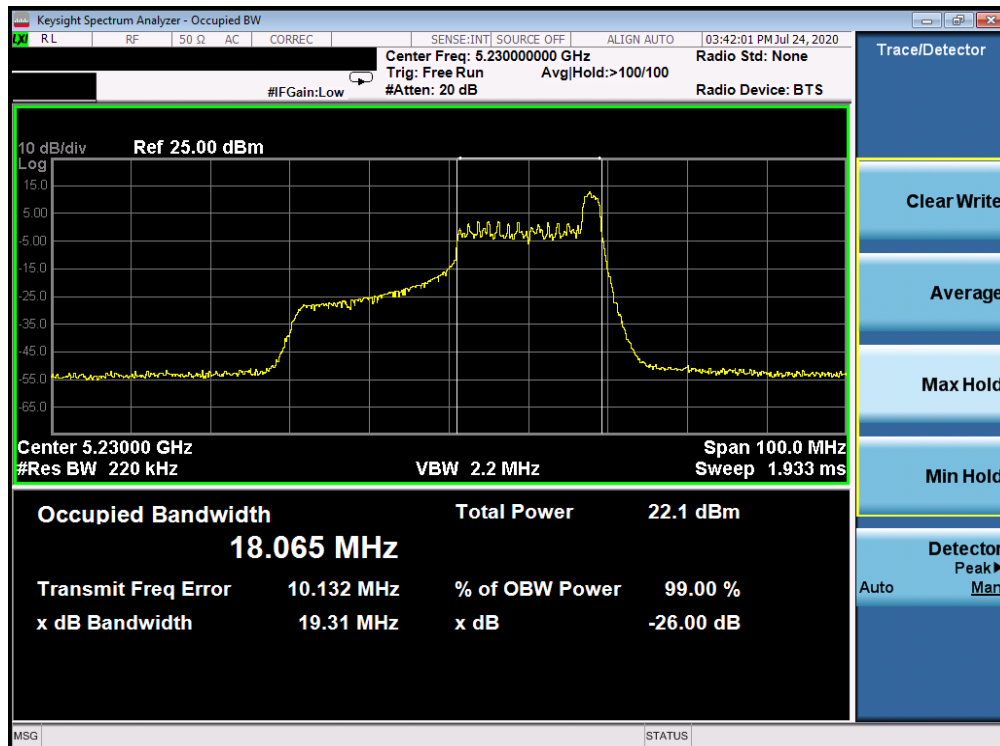
Plot 7-98. 26dB Bandwidth Plot ANT WF7a (40MHz BW 802.11ax Index 17 – RU26 (UNII Band 1) – Ch. 46)
