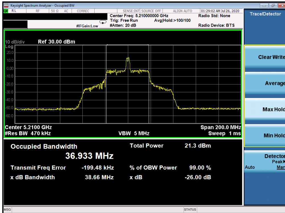
Plot 7-102. 26dB Bandwidth Plot ANT WF7a (80MHz BW 802.11ax Index 18 – RU26 (UNII Band 1) – Ch. 42)
