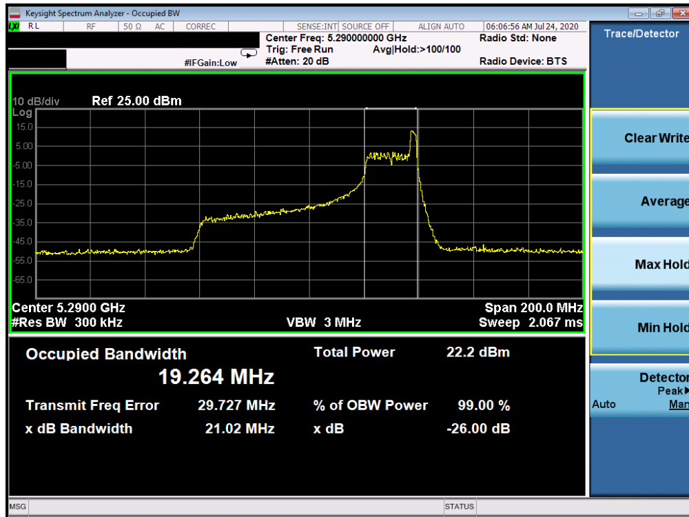
Plot 7-47. 26dB Bandwidth Plot ANT WF8 (80MHz BW 802.11ax Index 36 – RU26 (UNII Band 2A) – Ch. 58)
