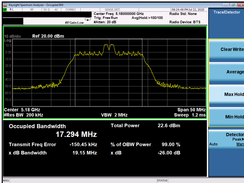
Plot 7-2. 26dB Bandwidth Plot ANT WF8 (20MHz BW 802.11ax Index 4 – RU26 (UNII Band 1) – Ch. 36)
