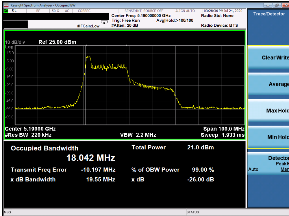
Plot 7-93. 26dB Bandwidth Plot ANT WF7a (40MHz BW 802.11ax Index 0 – RU26 (UNII Band 1) – Ch. 38)
