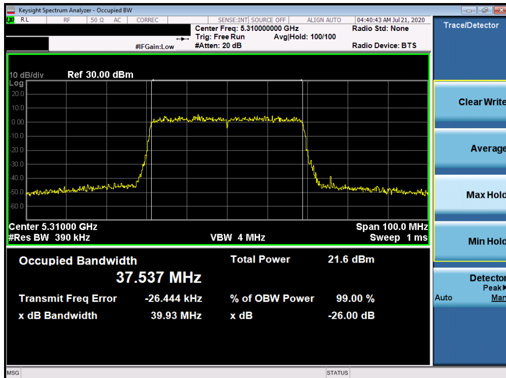
Plot 7-44. 26dB Bandwidth Plot ANT WF8 (40MHz BW 802.11ax – RU484 (UNII Band 2A) – Ch. 62)
