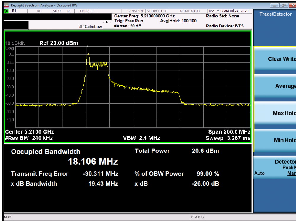
Plot 7-21. 26dB Bandwidth Plot ANT WF8 (80MHz BW 802.11ax Index 0 – RU26 (UNII Band 1) – Ch. 42)
