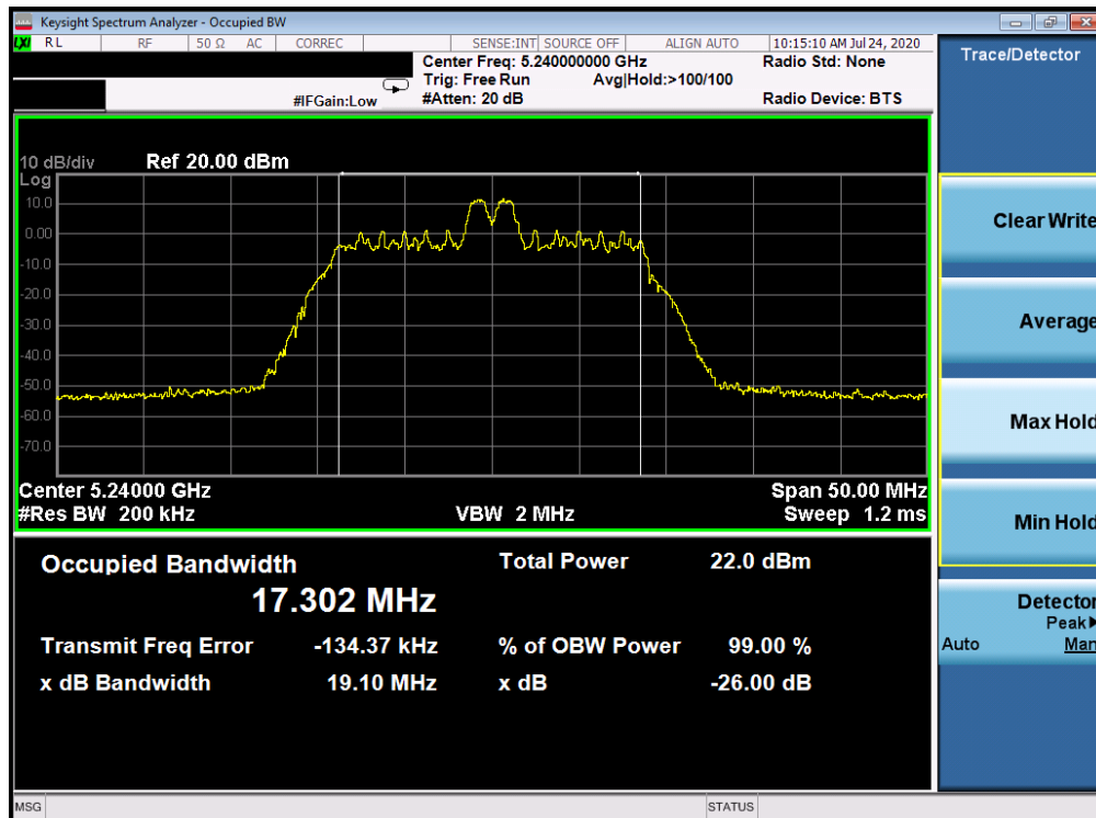
Plot 7-88. 26dB Bandwidth Plot ANT WF7a (20MHz BW 802.11ax Index 4 – RU26 (UNII Band 1) – Ch. 48)
