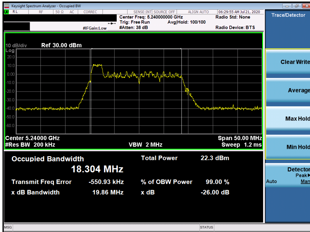
Plot 7-7. 26dB Bandwidth Plot ANT WF8 (20MHz BW 802.11ax Index 0 – RU26 (UNII Band 1) – Ch. 48)
