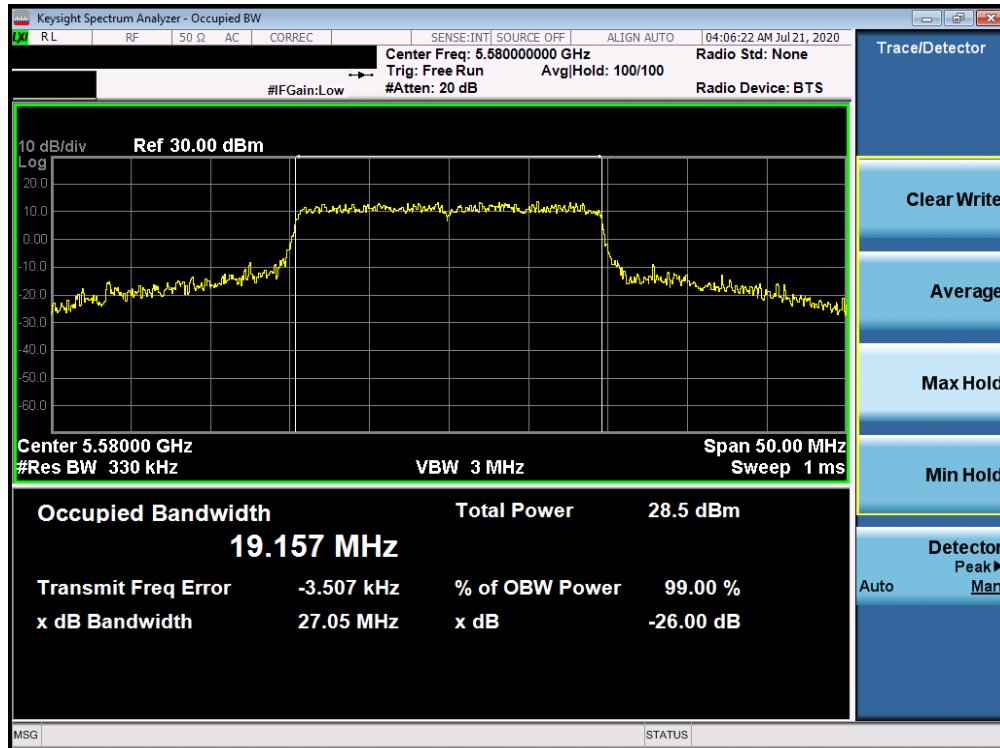
Plot 7-59. 26dB Bandwidth Plot ANT WF8 (20MHz BW 802.11ax- RU242 (UNII Band 2C) - Ch. 116)
