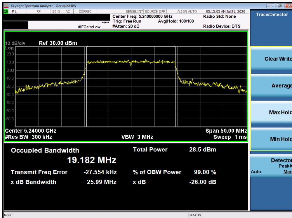
Plot 7-92. 26dB Bandwidth Plot ANT WF7a (20MHz BW 802.11ax- RU242 (UNII Band 1) – Ch. 48)
