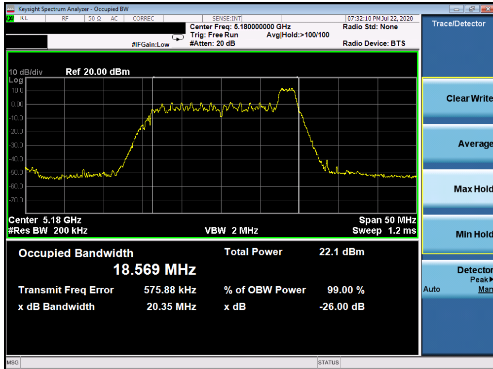
Plot 7-3. 26dB Bandwidth Plot ANT WF8 (20MHz BW 802.11ax Index 8 – RU26 (UNII Band 1) – Ch. 36)
