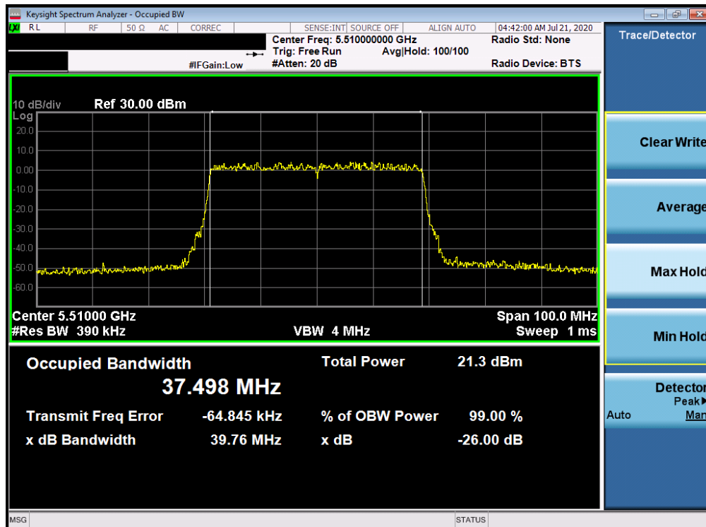
Plot 7-70. 26dB Bandwidth Plot ANT WF8 (40MHz BW 802.11ax – RU484 (UNII Band 2C) – Ch. 102)
