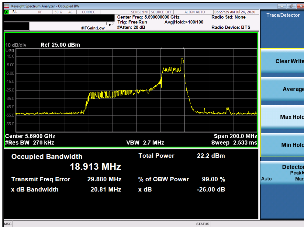
Plot 7-78. 26dB Bandwidth Plot ANT WF8 (80MHz BW 802.11ax Index 36 – RU26 (UNII Band 2C) – Ch. 138)
