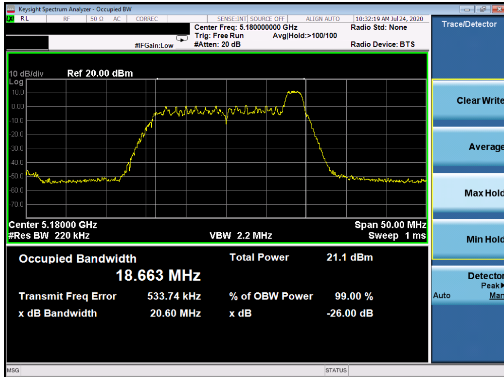
Plot 7-83. 26dB Bandwidth Plot ANT WF7a (20MHz BW 802.11ax Index 8 – RU26 (UNII Band 1) – Ch. 36)
