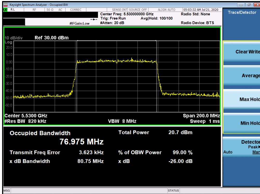
Plot 7-79. 26dB Bandwidth Plot ANT WF8 (80MHz BW 802.11ax – RU996 (UNII Band 2C) – Ch. 106)
