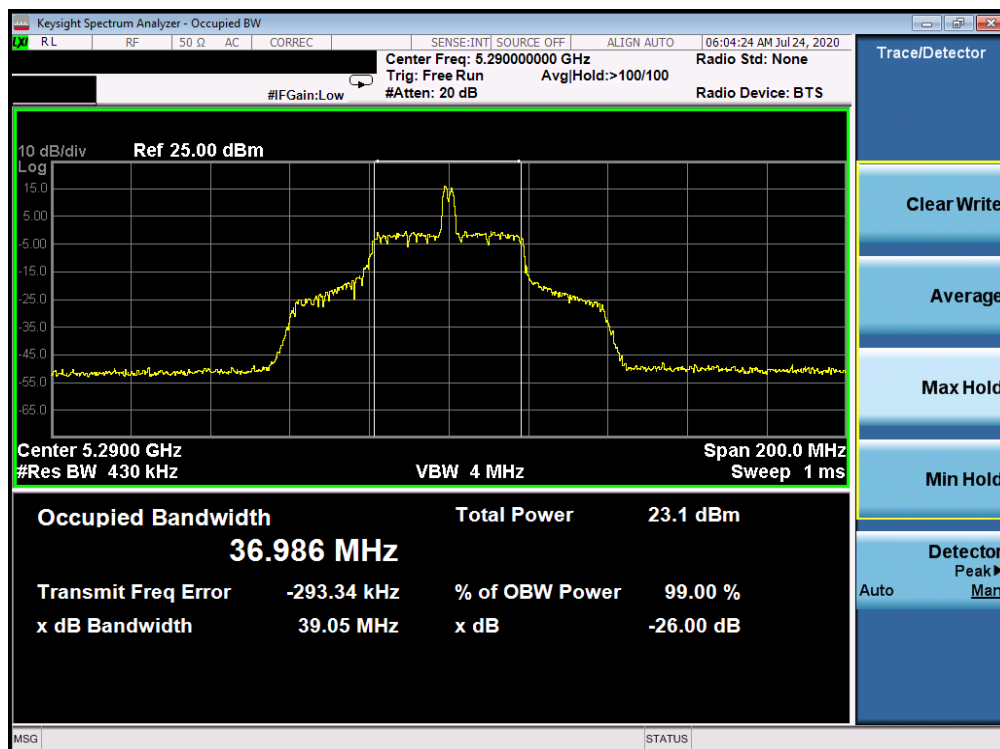
Plot 7-46. 26dB Bandwidth Plot ANT WF8 (80MHz BW 802.11ax Index 18 – RU26 (UNII Band 2A) – Ch. 58)
