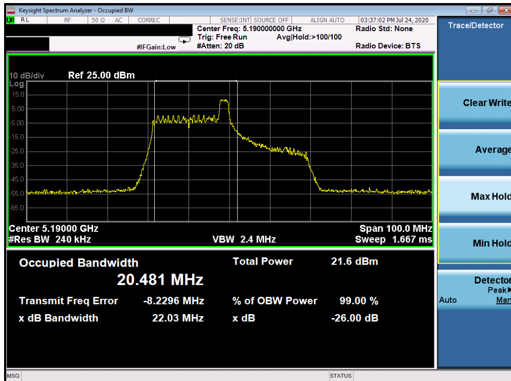
Plot 7-94. 26dB Bandwidth Plot ANT WF7a (40MHz BW 802.11ax Index 8 – RU26 (UNII Band 1) – Ch. 38)
