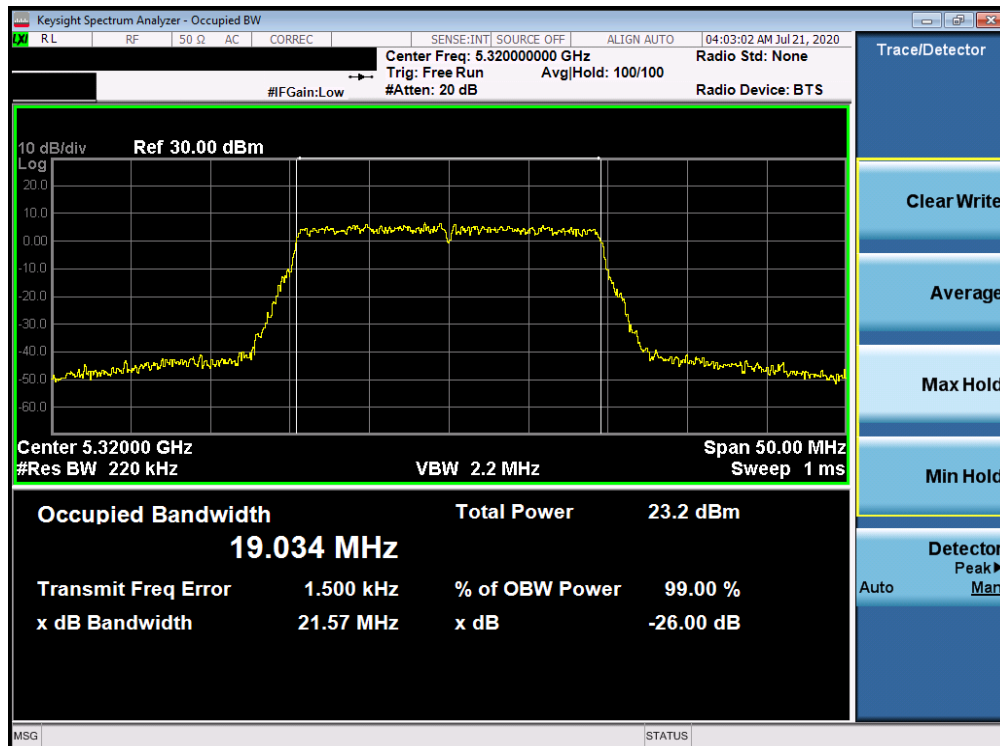
Plot 7-36. 26dB Bandwidth Plot ANT WF8 (20MHz BW 802.11ax– RU242 (UNII Band 2A) – Ch. 64)
