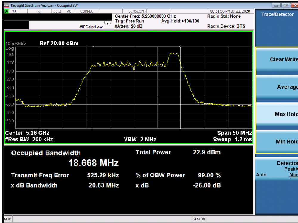
Plot 7-27. 26dB Bandwidth Plot ANT WF8 (20MHz BW 802.11ax Index 8 – RU26 (UNII Band 2A) – Ch. 52)
