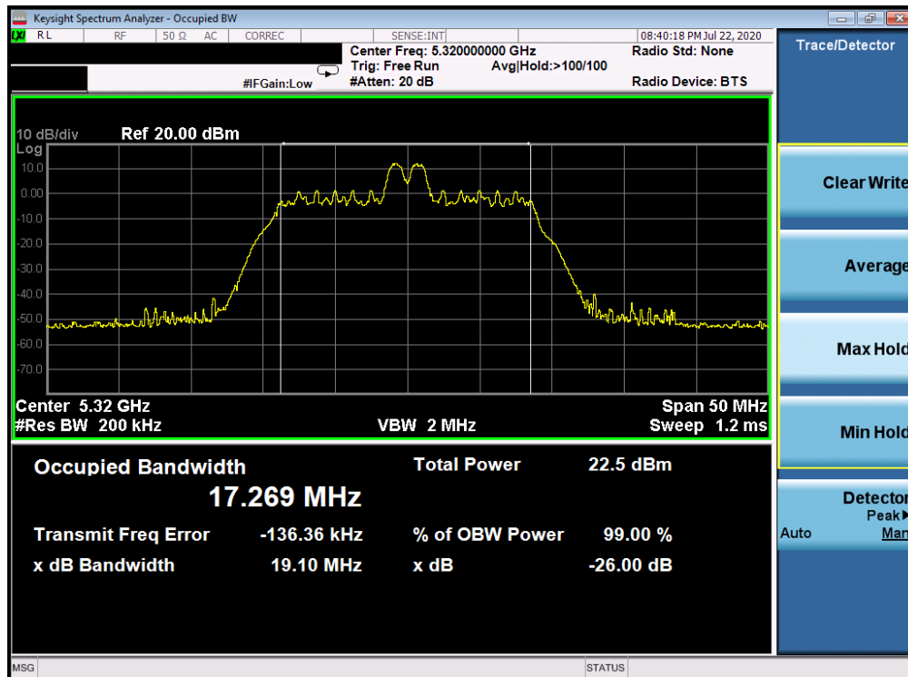
Plot 7-32. 26dB Bandwidth Plot ANT WF8 (20MHz BW 802.11ax Index 4 – RU26 (UNII Band 2A) – Ch. 64)
