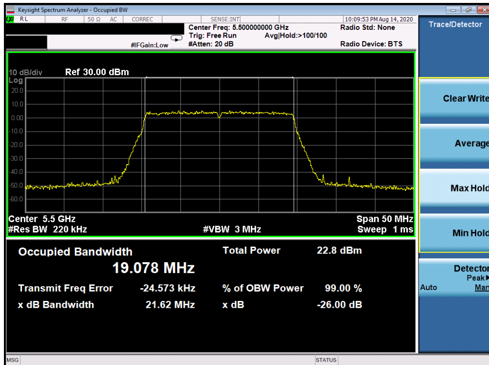
Plot 7-58. 26dB Bandwidth Plot ANT WF8 (20MHz BW 802.11ax– RU242 (UNII Band 2C) – Ch. 100)
