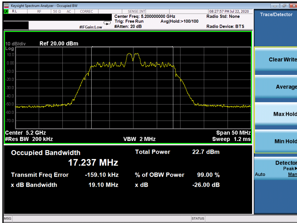
Plot 7-5. 26dB Bandwidth Plot ANT WF8 (20MHz BW 802.11ax Index 4 – RU26 (UNII Band 1) – Ch. 40)
