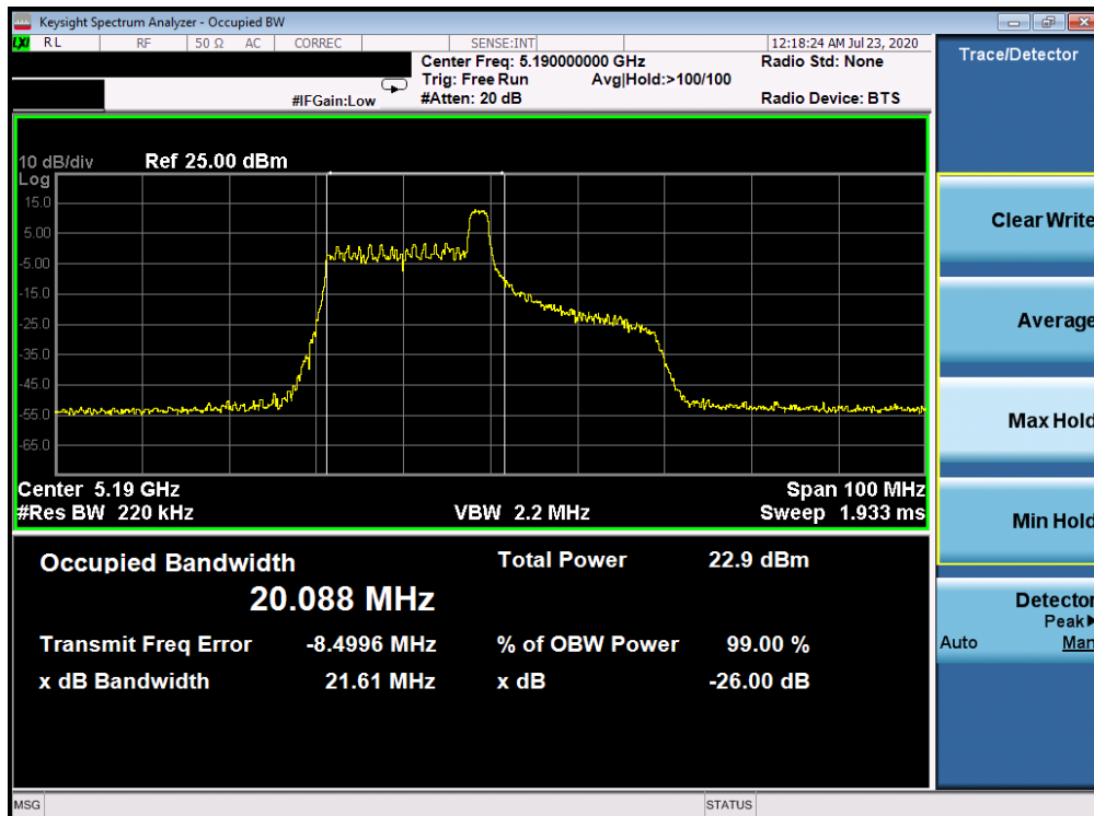
Plot 7-14. 26dB Bandwidth Plot ANT WF8 (40MHz BW 802.11ax Index 8 – RU26 (UNII Band 1) – Ch. 38)
