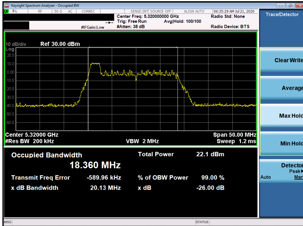
Plot 7-31. 26dB Bandwidth Plot ANT WF8 (20MHz BW 802.11ax Index 0 – RU26 (UNII Band 2A) – Ch. 64)
