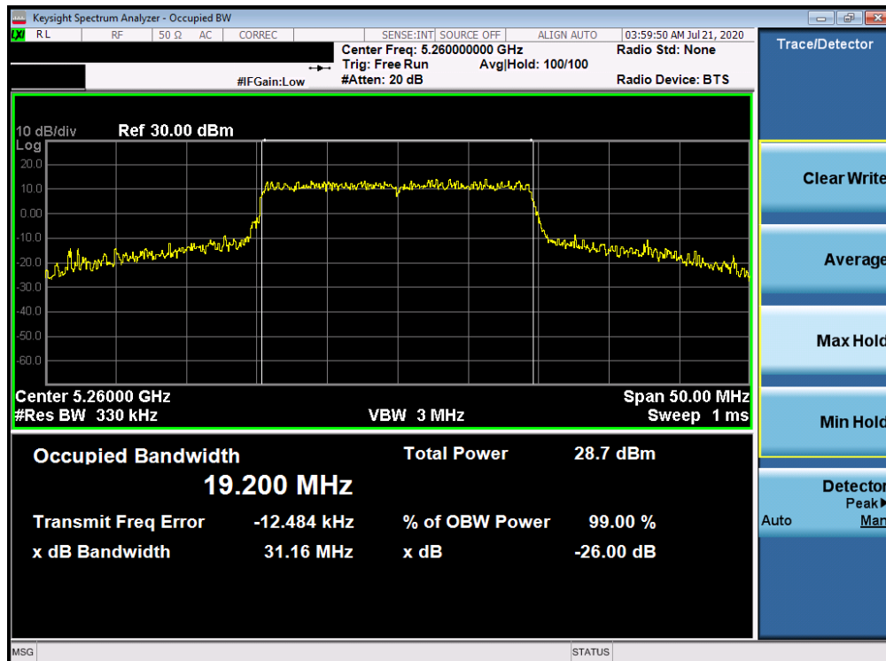
Plot 7-34. 26dB Bandwidth Plot ANT WF8 (20MHz BW 802.11ax – RU242 (UNII Band 2A) – Ch. 52)
