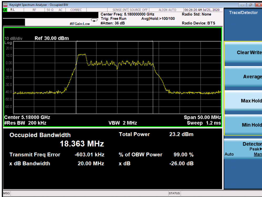
Plot 7-1. 26dB Bandwidth Plot ANT WF8 (20MHz BW 802.11ax Index 0 – RU26 (UNII Band 1) – Ch. 36)
