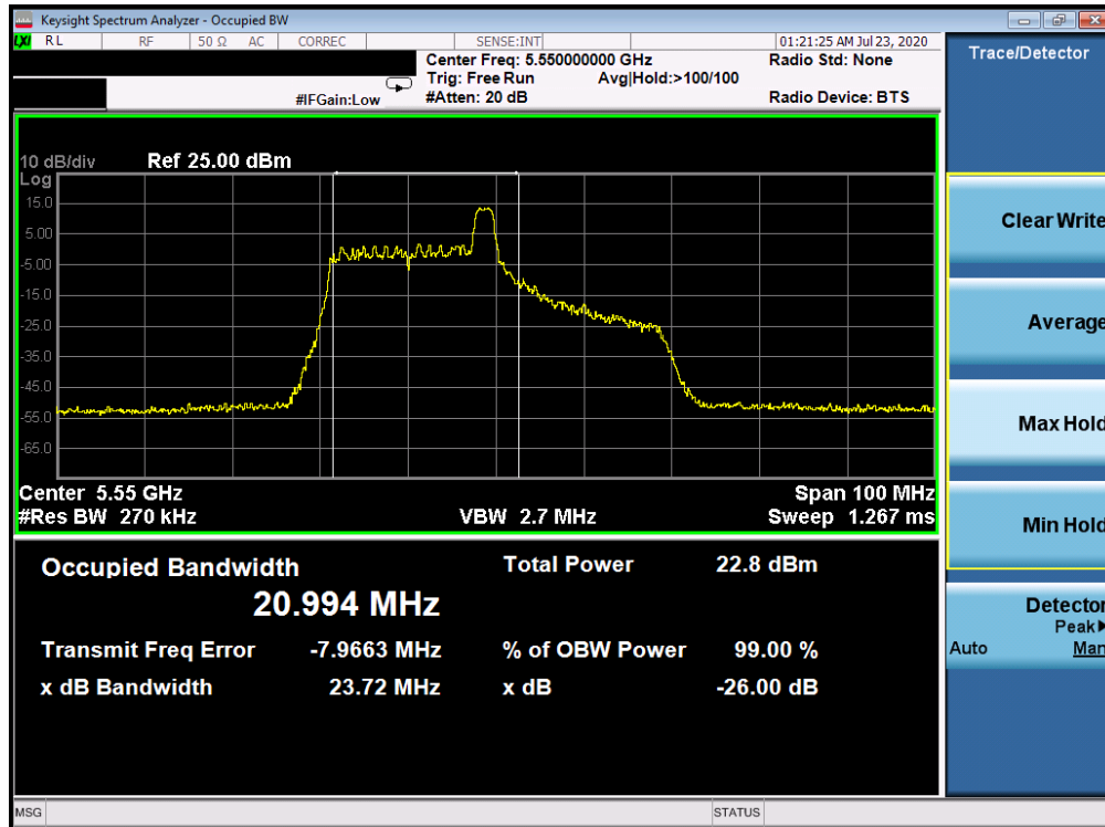
Plot 7-65. 26dB Bandwidth Plot ANT WF8 (40MHz BW 802.11ax Index 8 – RU26 (UNII Band 2C) – Ch. 110)
