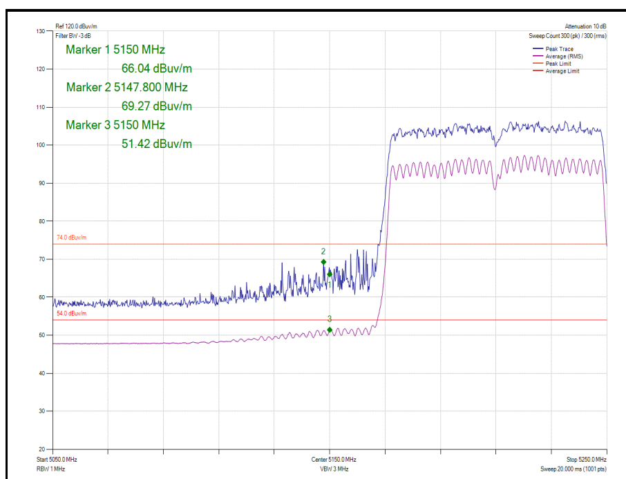
Figure 885 - 802.11ac VHT80 CDD Cores 1-2- 5210 MHz Band Edge Frequency 5150 MHz
