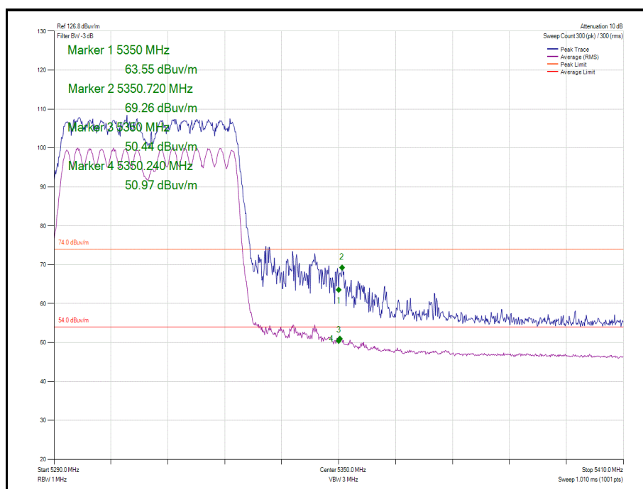
Figure 869 - 802.11n HT40 CDD Cores 1-2 - 5310 MHz Band Edge Frequency 5350 MHz
