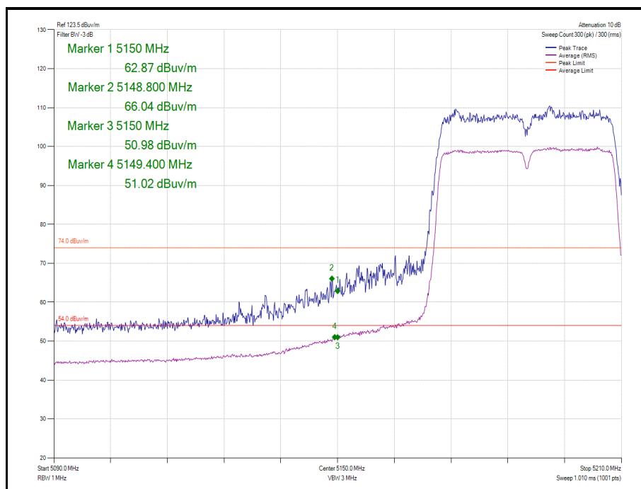
Figure 868 - 802.11n HT40 SDM Cores 1-2 - 5190 MHz Band Edge Frequency 5150 MHz
