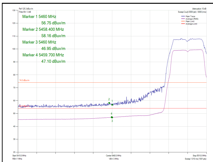
Figure 847 - 802.11a Core Aux - 5500 MHz Band Edge Frequency 5460 MHz
