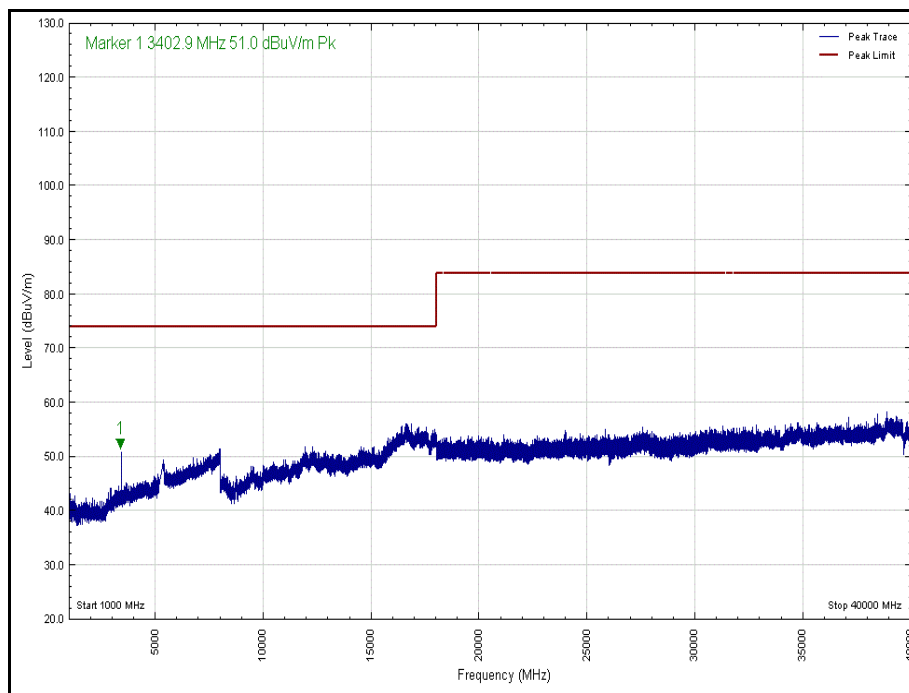
Figure 906 - U-NII 2a - 5320 MHz - 1 GHz to 40 GHz - Polarisation: Vertical (Peak)
