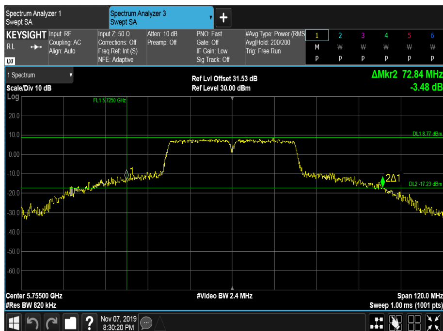
Figure 662 - 5755 MHz - 26 dB Emission Bandwidth
