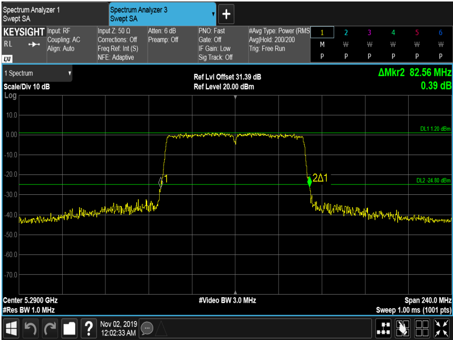
Figure 323 - 5290 MHz - 26 dB Emission Bandwidth
