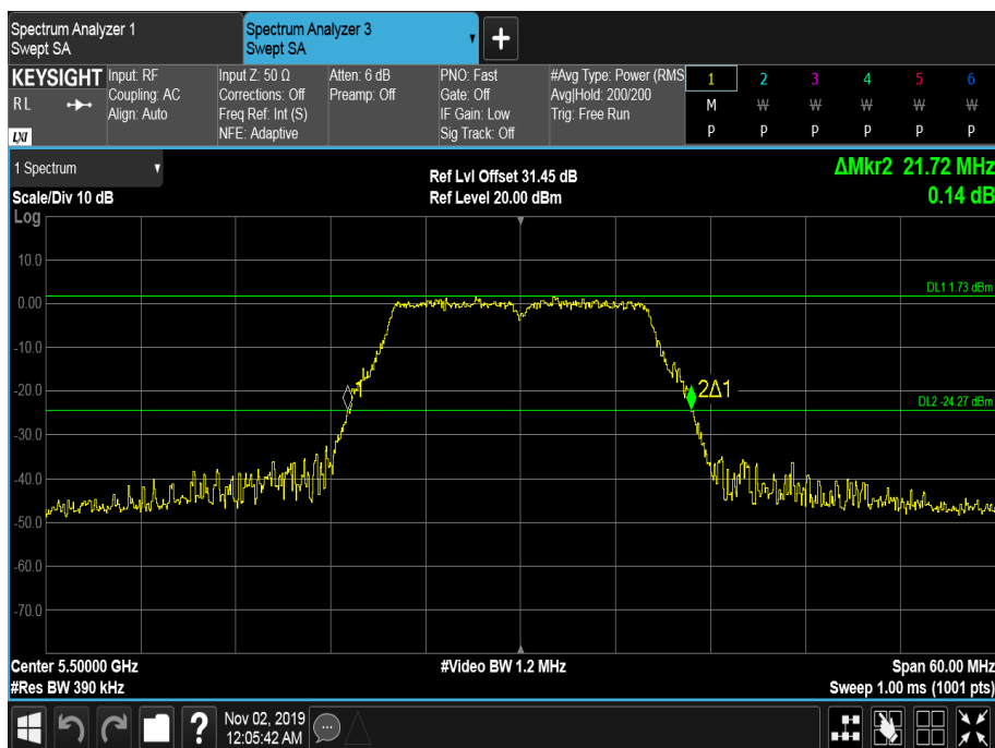
Figure 333 - 5500 MHz - 26 dB Emission Bandwidth
