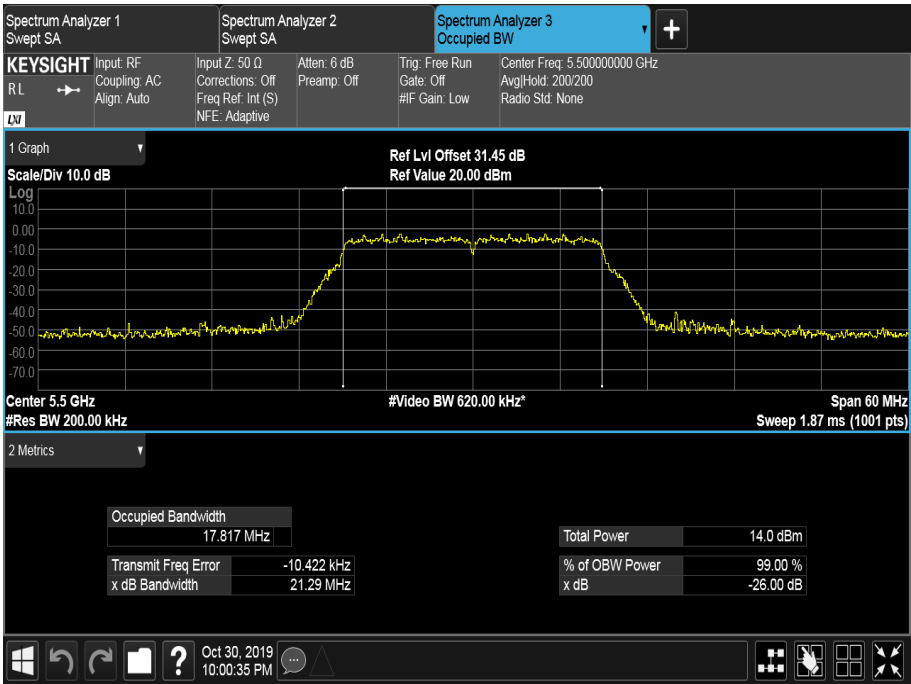
Figure 358 - 5500 MHz - 99% Occupied Bandwidth
