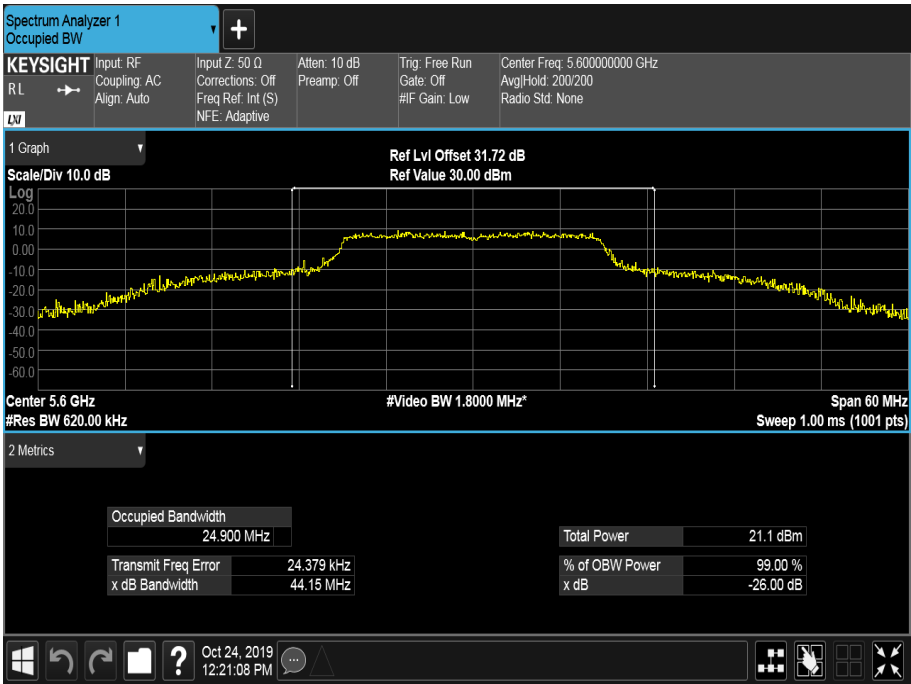
Figure 376 - 5600 MHz - 99% Occupied Bandwidth
