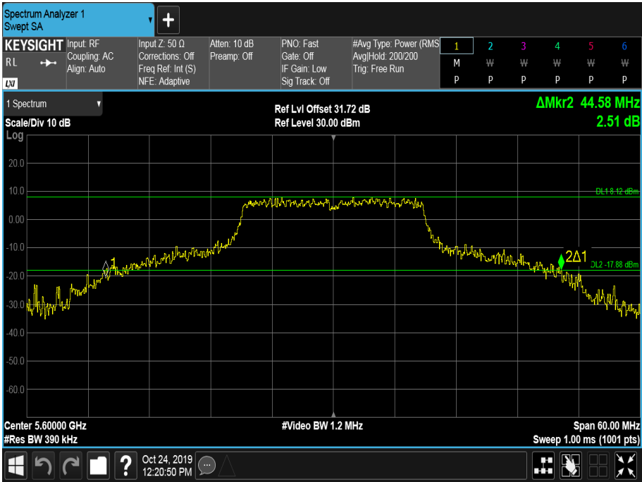
Figure 375 - 5600 MHz - 26 dB Emission Bandwidth
