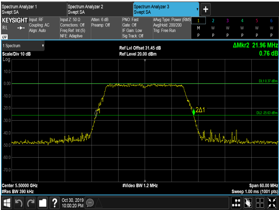
Figure 357 - 5500 MHz - 26 dB Emission Bandwidth
