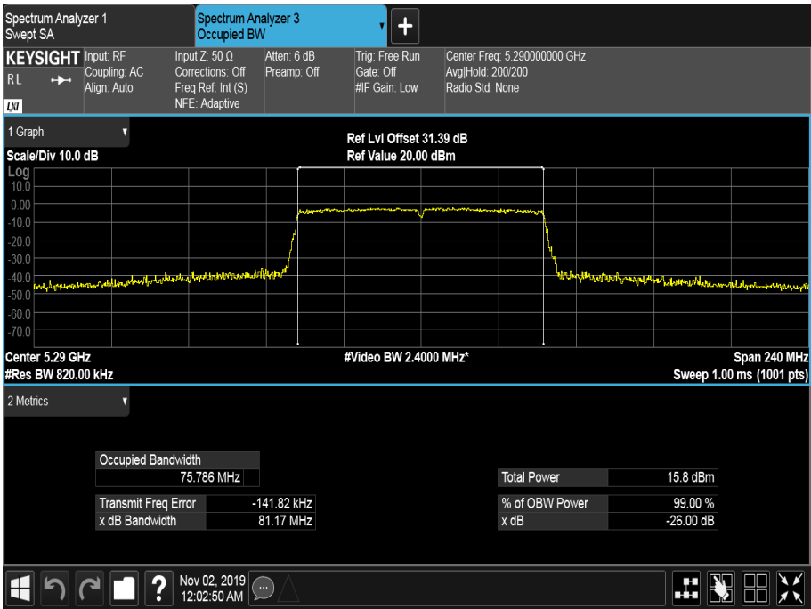
Figure 324 - 5290 MHz - 99% Occupied Bandwidth
