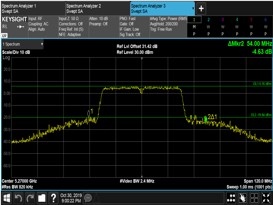
Figure 277 - 5270 MHz - 26 dB Emission Bandwidth
