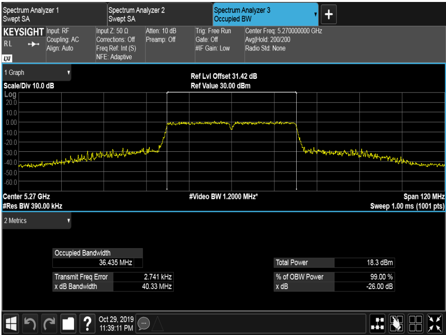
Figure 278 - 5270 MHz - 99% Occupied Bandwidth
