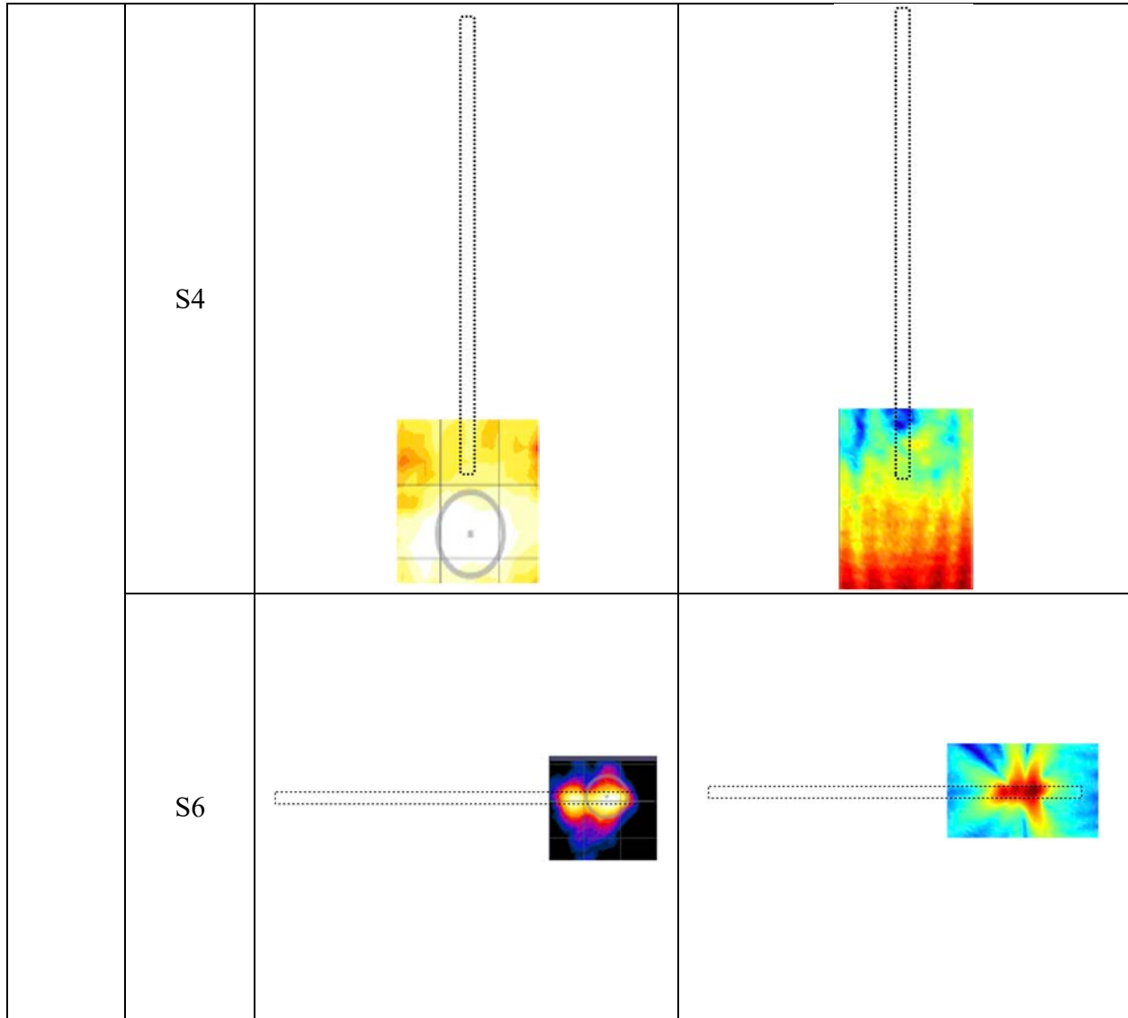
Figure 15. Bottom array: simulated and measured power density at 2 mm away from DUT. Measured max MPE for measurement is 4.56 mW/cm 2 , and simulation is 5.5 mW/cm 2 (scale: dB).
