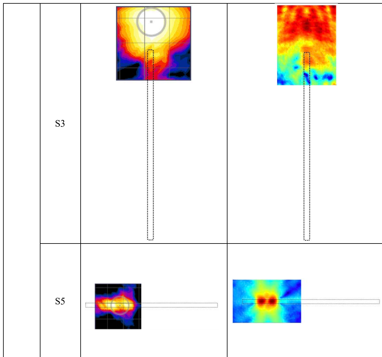
Figure 14. Top array: simulated and measured power density at 2 mm away from DUT. Measured max MPE from measurement is 6.59 mW/cm 2 , and from simulation is 7.4 mW/cm 2 (scale: dB)
