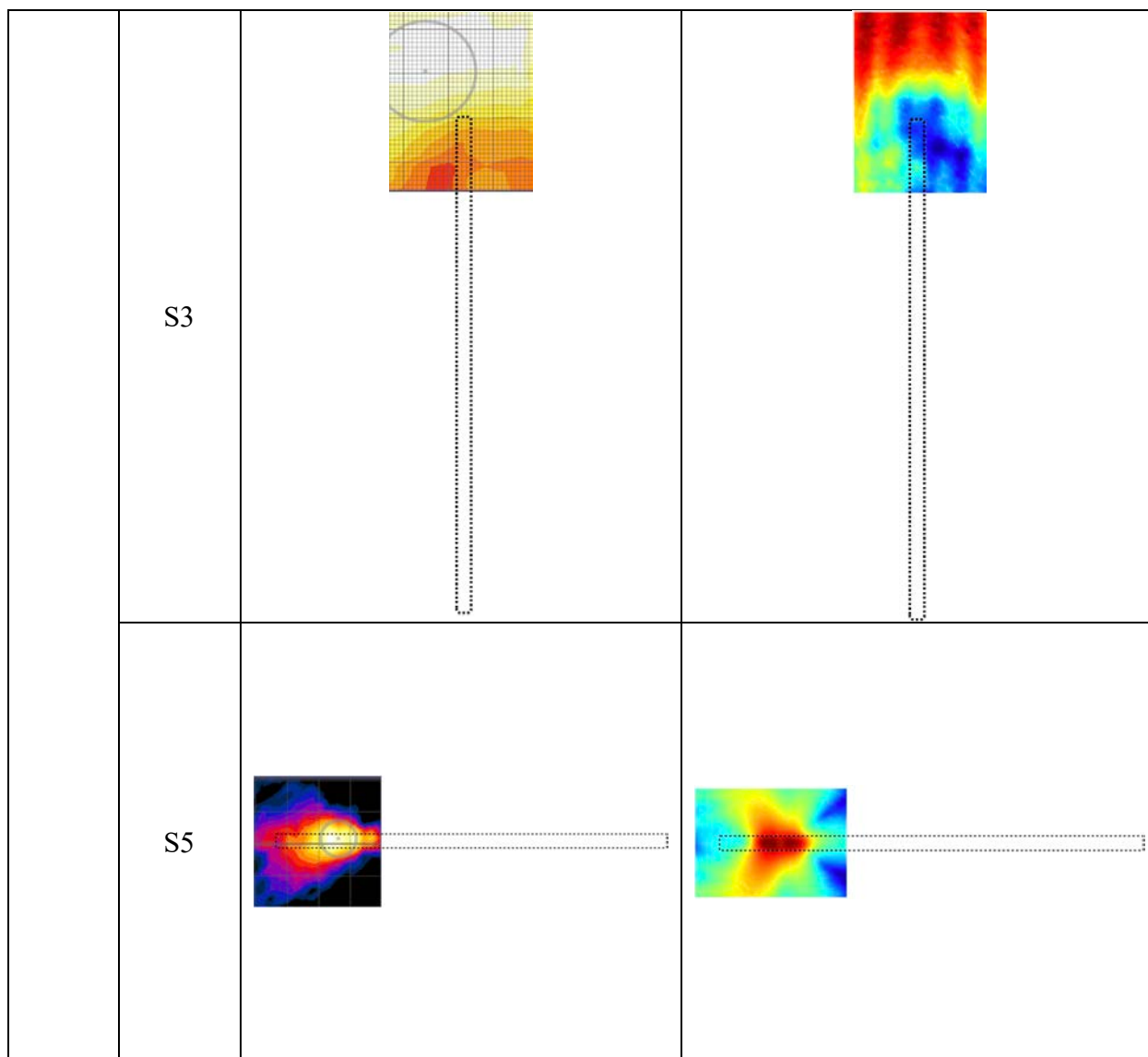
Figure 10. Top array: simulated and measured power density at 2 mm away from DUT. Measured max MPE from measurement is 6.28 mW/cm 2 , and from simulation is 7.91 mW/cm 2 (scale: dB)
