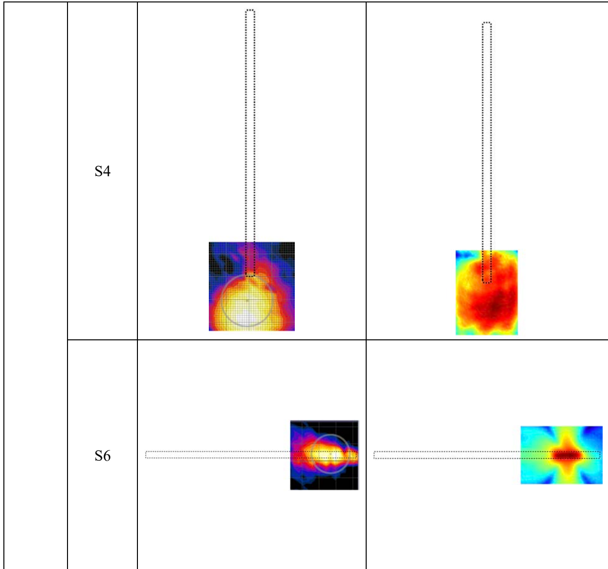
Figure 11. Bottom array: simulated and measured power density at 2 mm away from DUT. Measured max MPE for measurement is 5.63 mW/cm 2 , and simulation is 8.17 mW/cm 2 (scale: dB).
