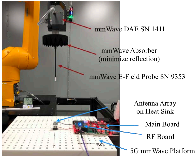
Figure 2. A representation of the MPE measurement setup.
