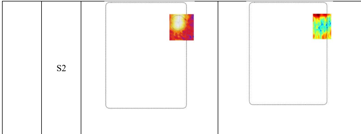
Figure 12. Front array: simulated and measured power density at 2 mm away from DUT. Measured max MPE for measurement is 6.45 mW/cm 2 , and simulation is 4.12 mW/cm 2 (scale: dB).
