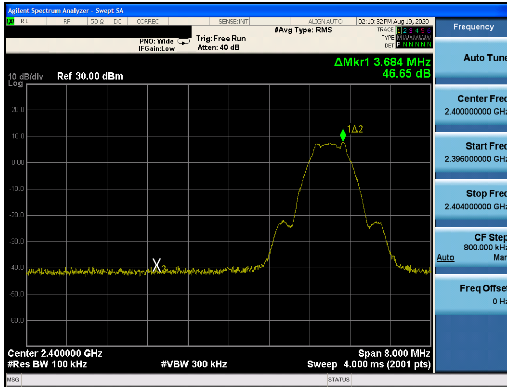
Plot 7-7. Band Edge Plot (Bluetooth (LE), 1Mbps, iPA - Ch. 0)
