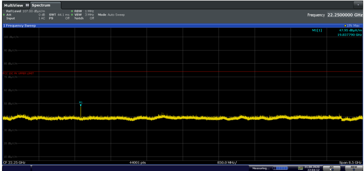
Plot 7-22. Radiated Spurious Plot Above 18GHz (1Mbps, iPA – Ch.39, Pol. H)
