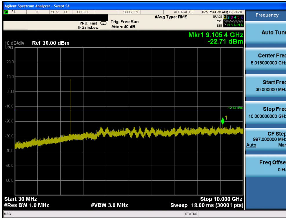
Plot 7-13. Conducted Spurious Plot (Bluetooth (LE), 1Mbps, iPA – Ch. 39)
