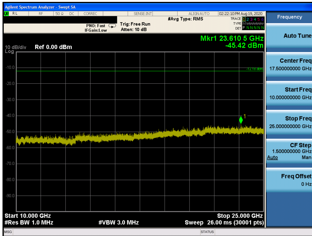
Plot 7-12. Conducted Spurious Plot (Bluetooth (LE), 1Mbps, iPA – Ch. 19)
