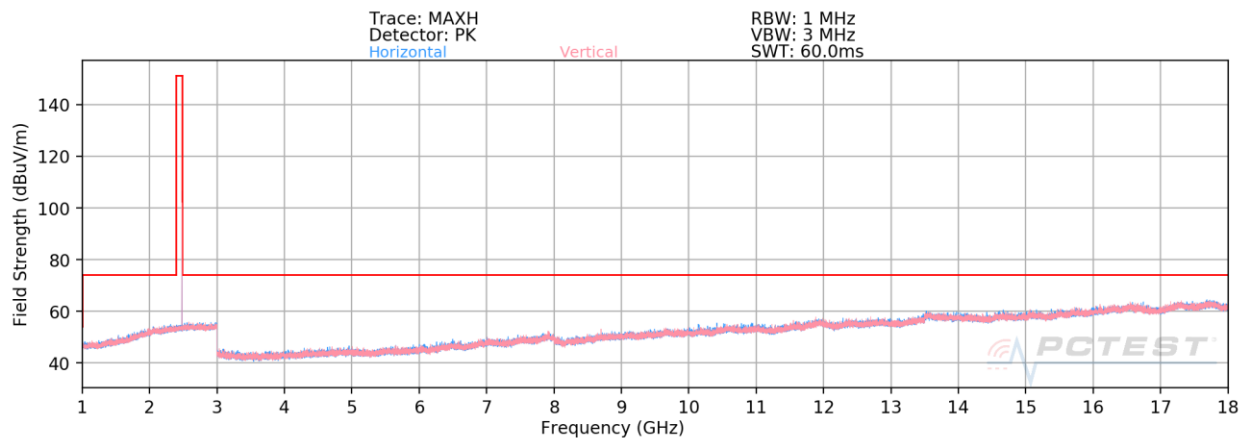
Plot 7-17. Radiated Spurious Emissions 1-18GHz (1Mbps iPA – Ch. 39)
