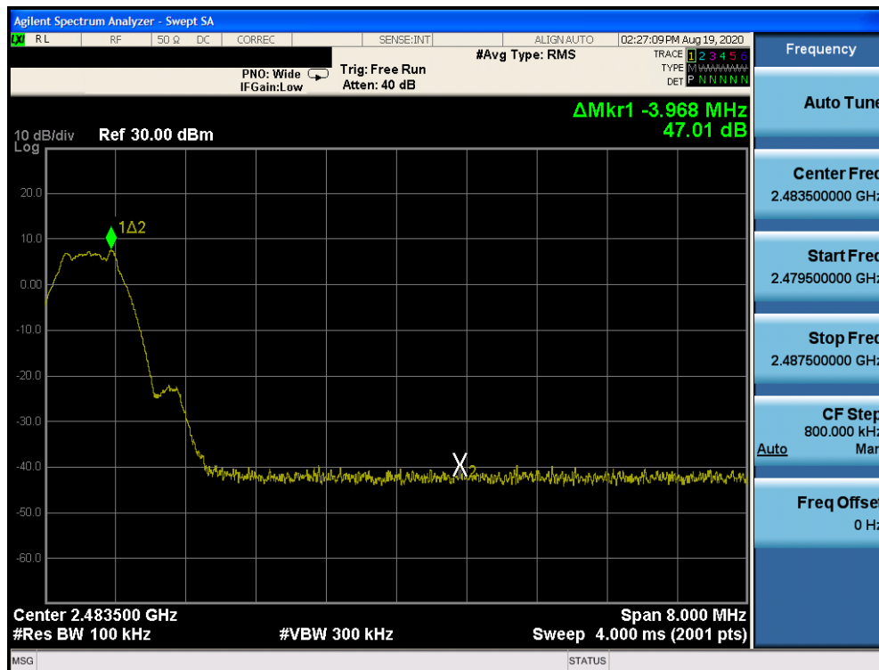
Plot 7-8. Band Edge Plot (Bluetooth (LE), 1Mbps, iPA - Ch. 39)
