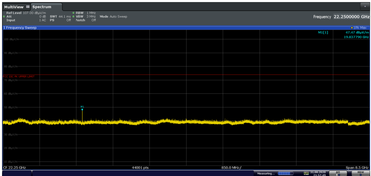
Plot 7-23. Radiated Spurious Plot Above 18GHz (1Mbps, iPA – Ch.39, Pol. V)
