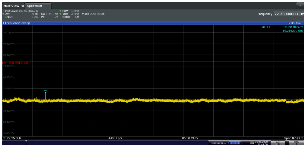
Plot 7-19. Radiated Spurious Plot Above 18GHz (1Mbps, iPA – Ch.0, Pol. V)
