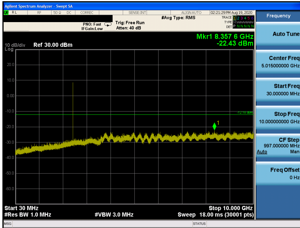
Plot 7-11. Conducted Spurious Plot (Bluetooth (LE), 1Mbps, iPA – Ch. 19)
