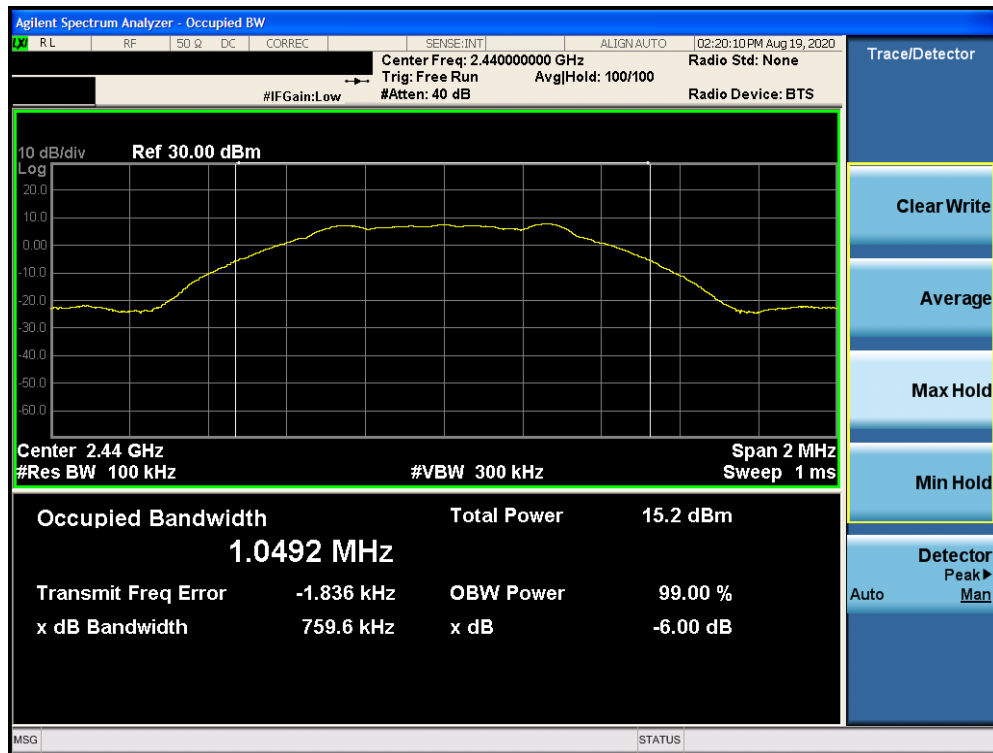
Plot 7-2. 6dB Bandwidth Plot (Bluetooth (LE), 1Mbps, iPA – Ch. 19)
