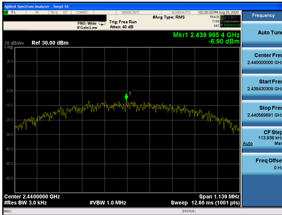
Plot 7-5. Power Spectral Density Plot (Bluetooth (LE), 1Mbps, iPA – Ch. 19)
