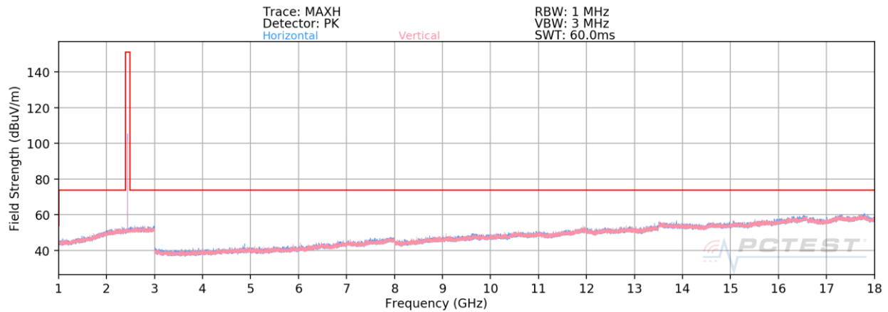
Plot 7-16. Radiated Spurious Emissions 1-18GHz (1Mbps, iPA – Ch. 19)
