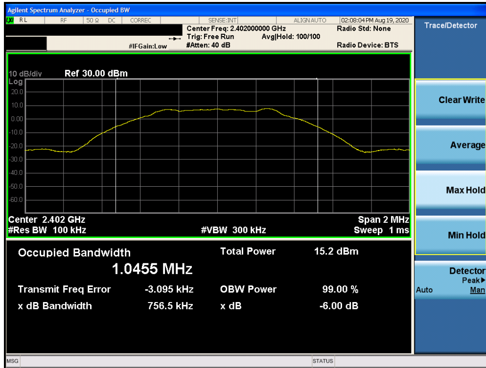
Plot 7-1. 6dB Bandwidth Plot (Bluetooth (LE), 1Mbps, iPA – Ch. 0)
