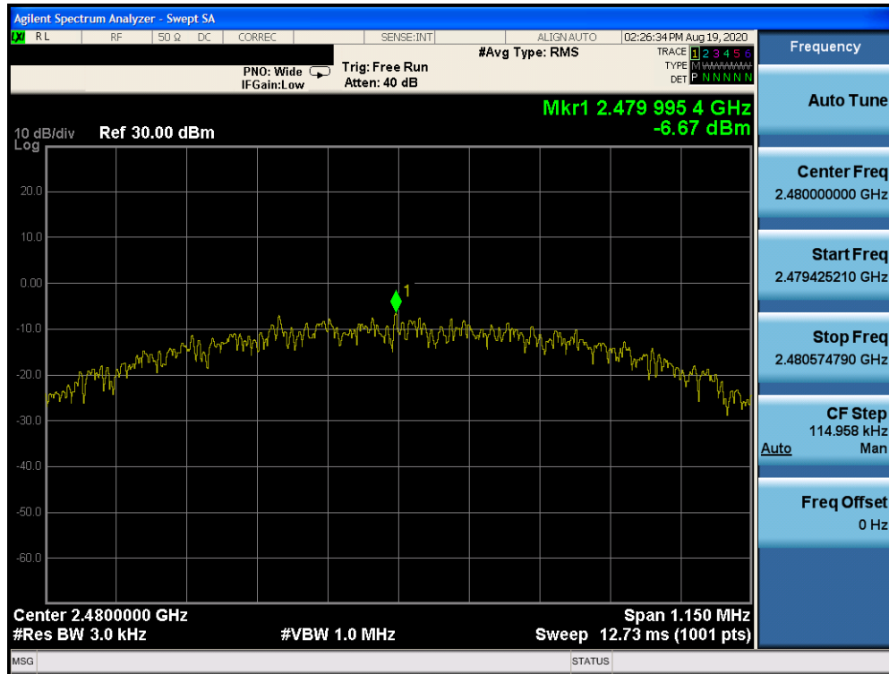
Plot 7-6. Power Spectral Density Plot (Bluetooth (LE), 1Mbps, iPA – Ch. 39)
