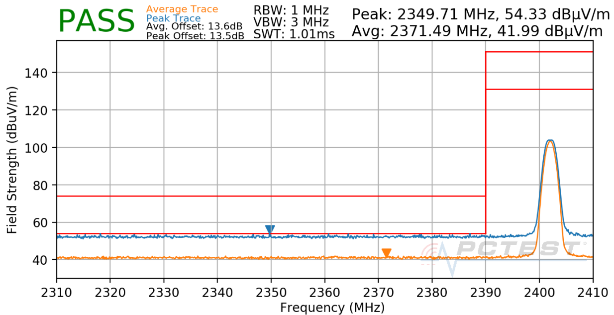
Plot 7-24. Radiated Restricted Lower Band Edge Measurement
