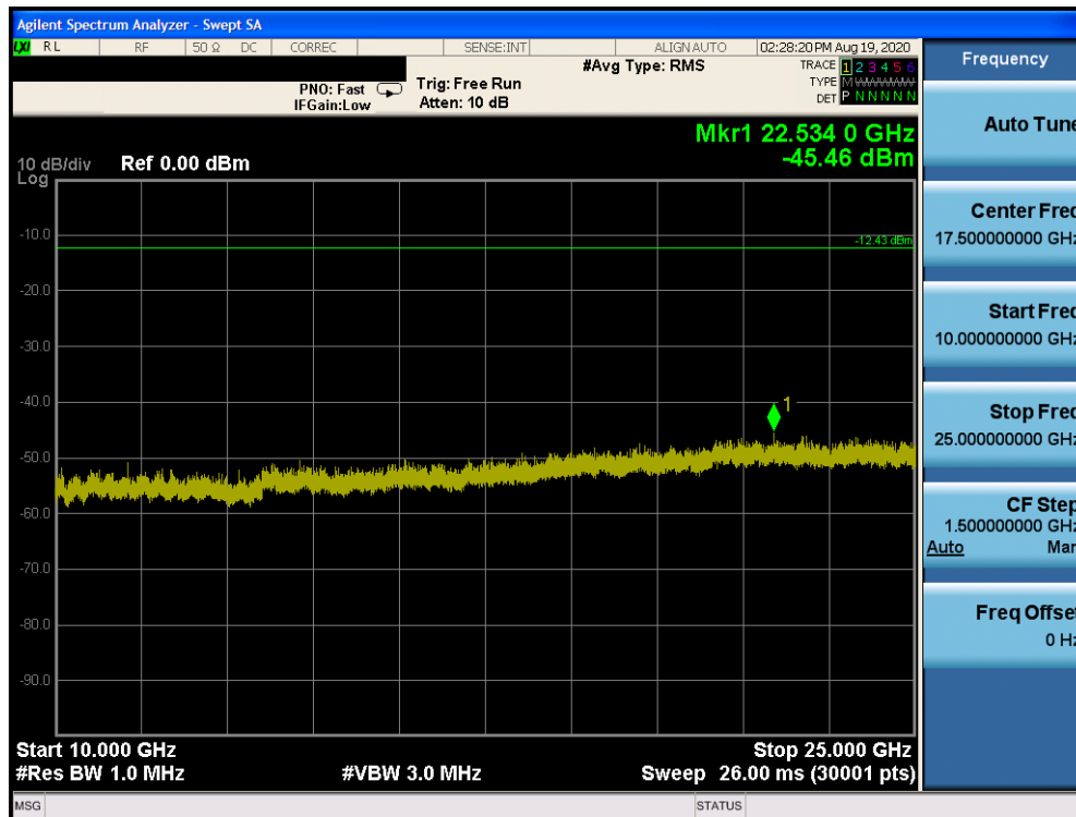
Plot 7-14. Conducted Spurious Plot (Bluetooth (LE), 1Mbps, iPA – Ch. 39)
