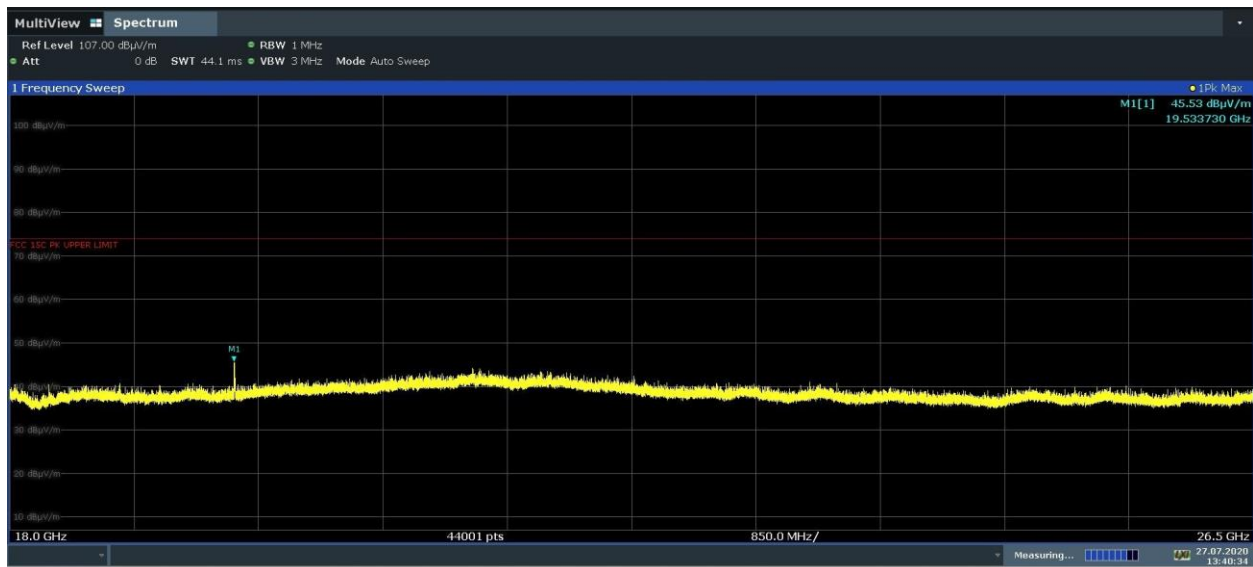
Plot 7-21. Radiated Spurious Plot Above 18GHz (1Mbps, iPA – Ch.19, Pol. V)
