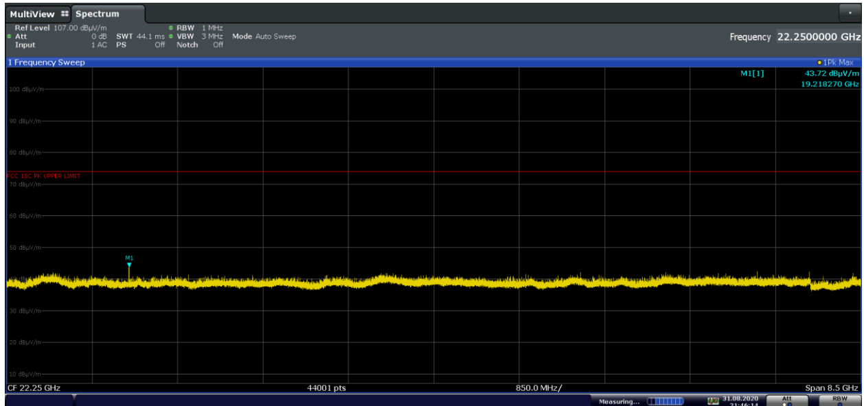
Plot 7-18. Radiated Spurious Plot Above 18GHz (1Mbps, iPA – Ch.0, Pol. H)
