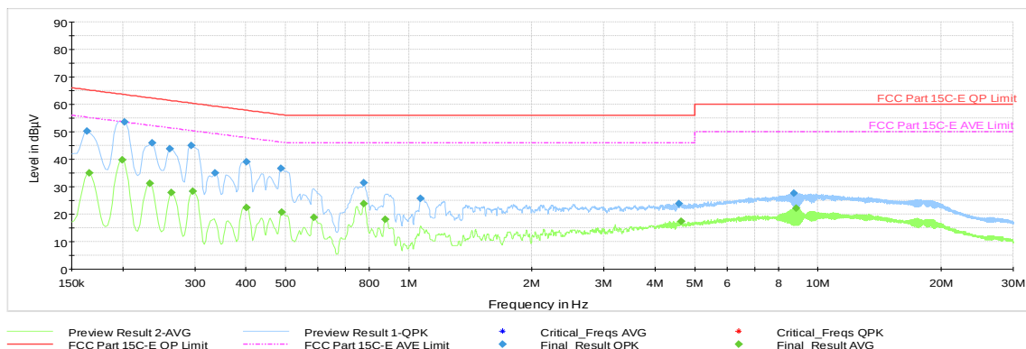
Plot 7-27. AC Line Conducted Plot with Bluetooth LE (L1 – 1Mbps, iPA, Ch.19, with Laptop)
