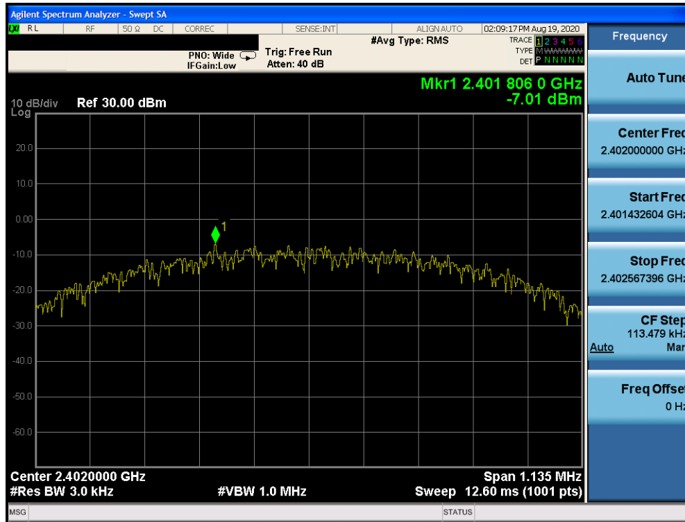
Plot 7-4. Power Spectral Density Plot (Bluetooth (LE), 1Mbps, iPA – Ch. 0)
