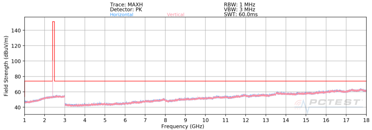
Plot 7-15. Radiated Spurious Emissions 1-18GHz (1Mbps, iPA – Ch. 0)
