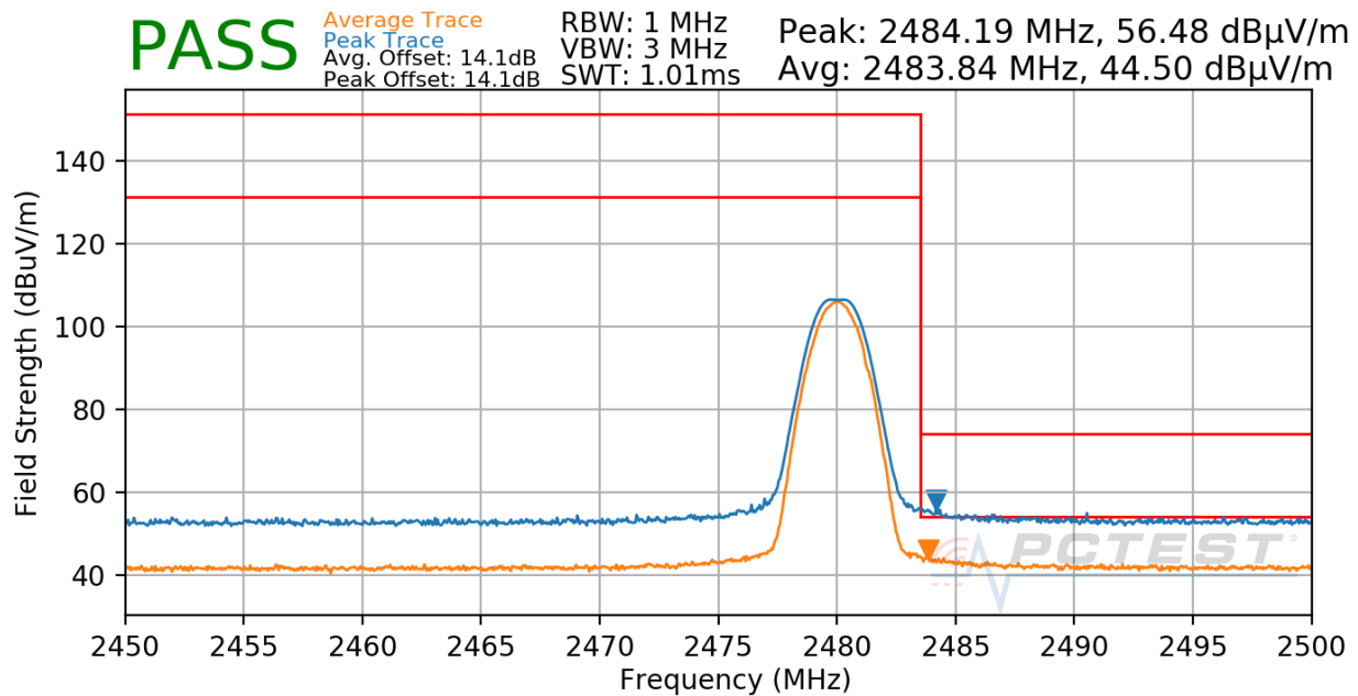
Plot 7-25. Radiated Restricted Upper Band Edge Measurement
