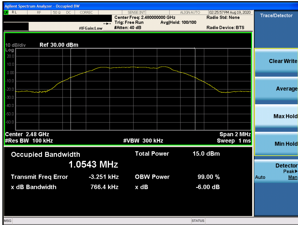
Plot 7-3. 6dB Bandwidth Plot (Bluetooth (LE), 1Mbps, iPA – Ch. 39)
