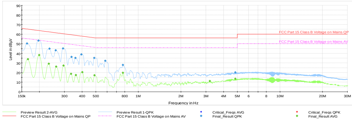
Plot 7-28. AC Line Conducted Plot with Bluetooth LE (N – 1Mbps, iPA, Ch.19, with Laptop)
