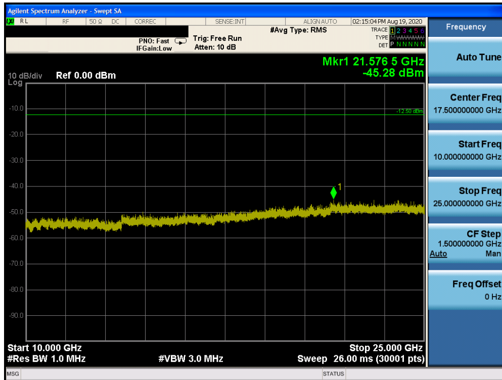
Plot 7-10. Conducted Spurious Plot (Bluetooth (LE), 1Mbps, iPA – Ch. 0)
