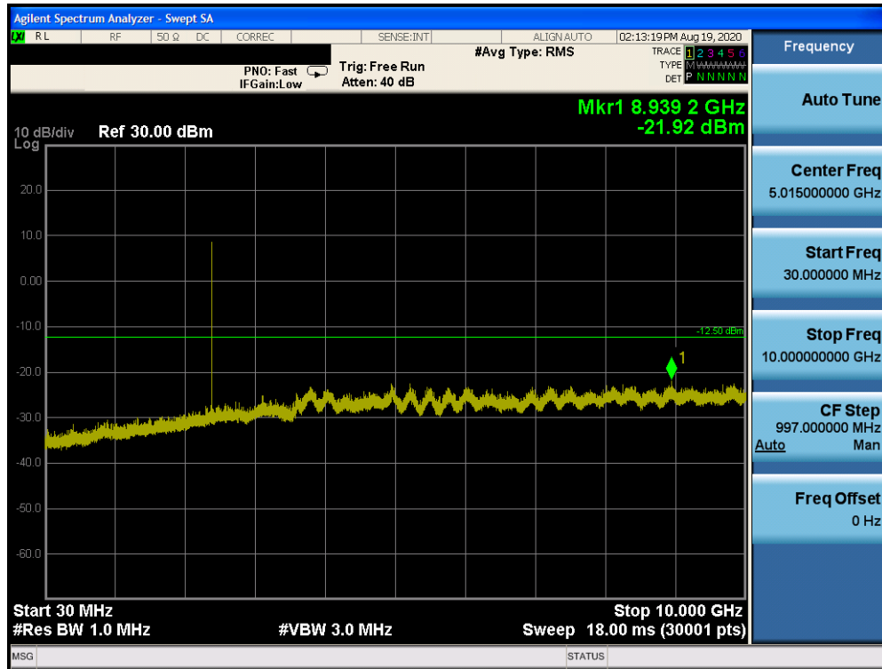
Plot 7-9. Conducted Spurious Plot (Bluetooth (LE), 1Mbps, iPA – Ch. 0)
