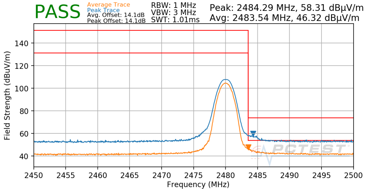
Plot 7-41. Radiated Restricted Upper Band Edge Measurement
