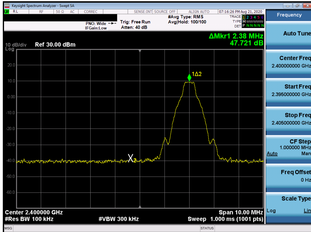
Plot 7-7. Band Edge Plot (Bluetooth with Hopping Disabled, GFSK, iPA – Ch. 0)
