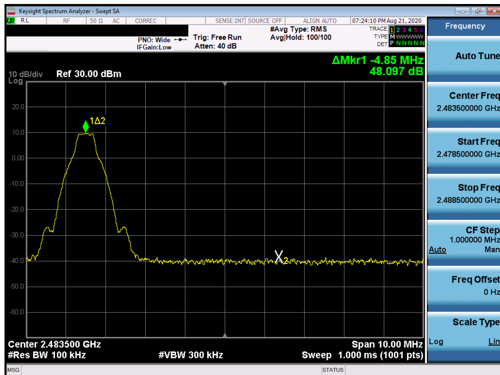
Plot 7-8. Band Edge Plot (Bluetooth with Hopping Disabled, GFSK, iPA – Ch. 78)
