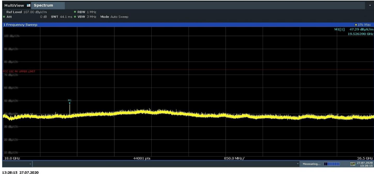
Plot 7-34. Radiated Spurious Emissions 18-26.5GHz (GFSK iPA – Ch.39, Pol. H)
