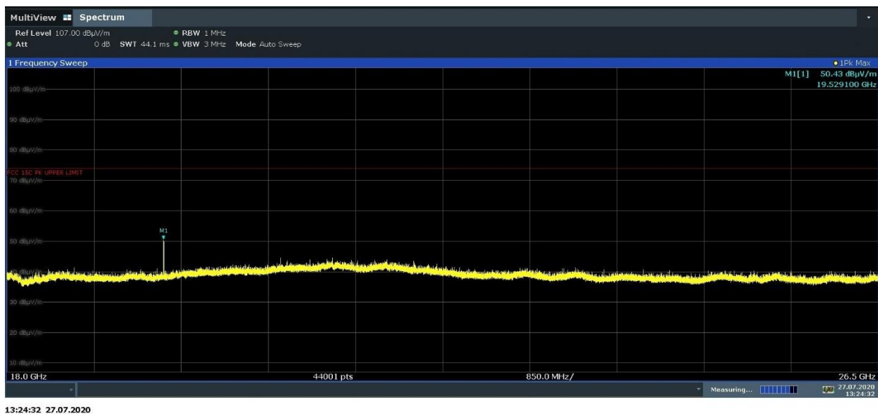
Plot 7-35. Radiated Spurious Emissions 18-26.5GHz (GFSK ePA – Ch. 39, Pol. V)
