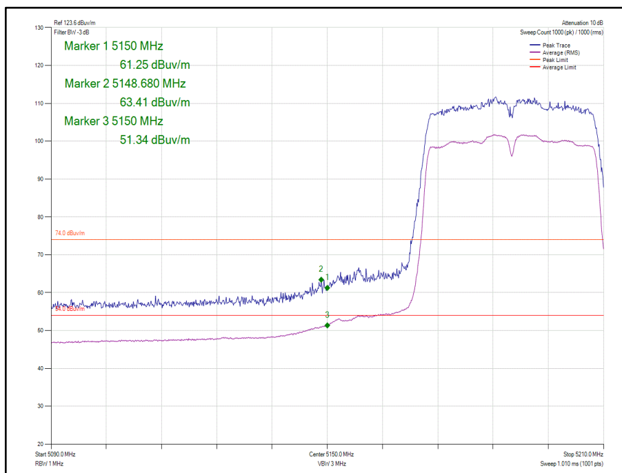
Figure 435 - 802.11n HT40 SDM Cores 0-1 - 5190 MHz Band Edge Frequency 5150 MHz
