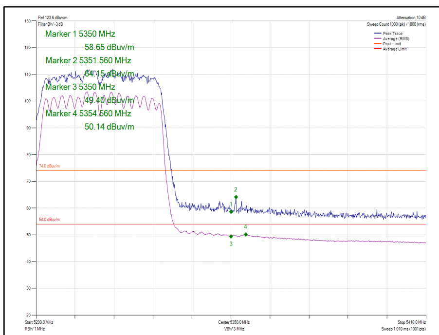
Figure 436 - 802.11n HT40 CDD Cores 0-1 - 5310 MHz Band Edge Frequency 5350 MHz
