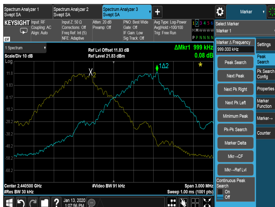
Figure 7 - GFSK
