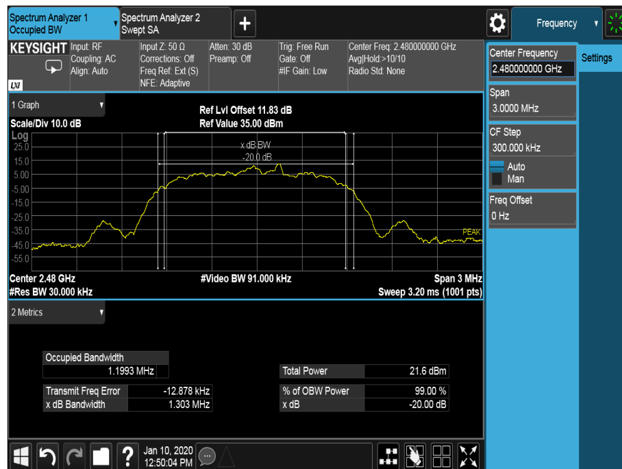
Figure 28 - 2480 MHz - 8-DPSK
