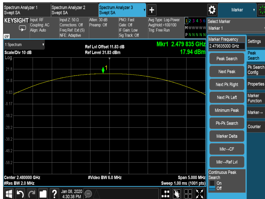
Figure 35 - 2480 MHz, GFSK - Maximum Output Power
