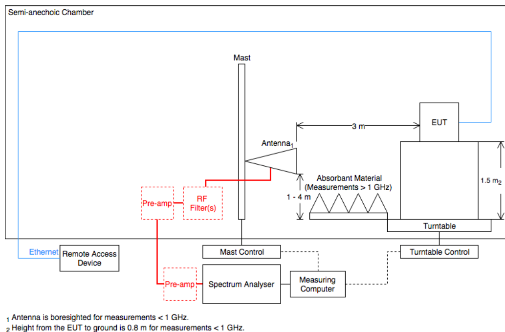
Figure 71 - Radiated Emissions Test Setup Diagram
