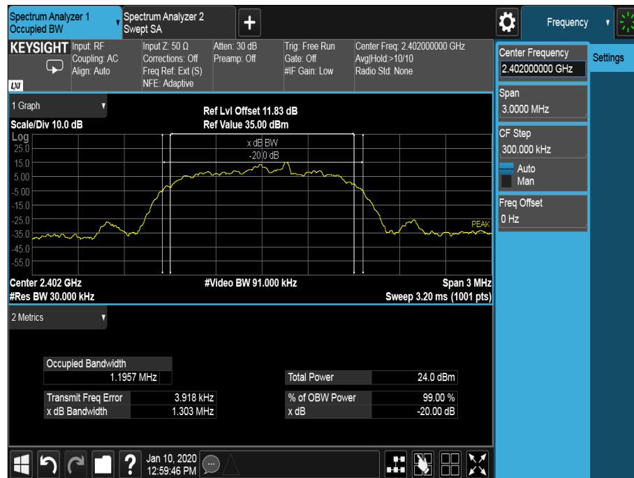
Figure 13 - 2402 MHz - 8-DPSK
