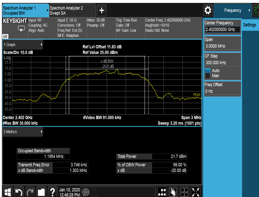
Figure 22 - 2402 MHz - 8-DPSK
