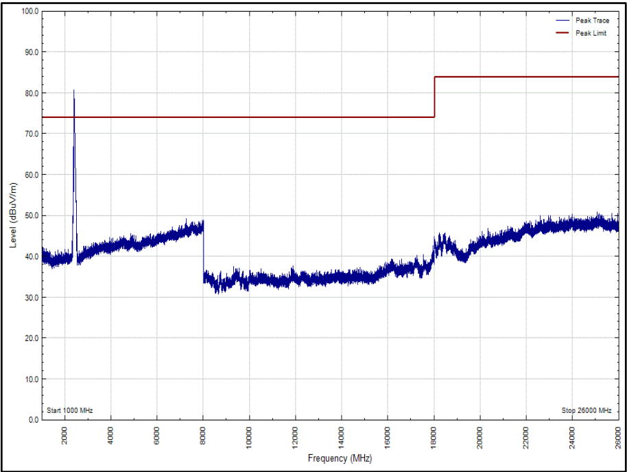
Figure 99 Figure 100 - 802.11n, Core 0-1, 2412 MHz - 1000 MHz to 26000 MHz, Vertical – Peak
