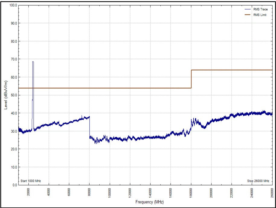
Figure 101 - 802.11n, Core 0-1, 2412 MHz - 1000 MHz to 26000 MHz, Vertical – Average
